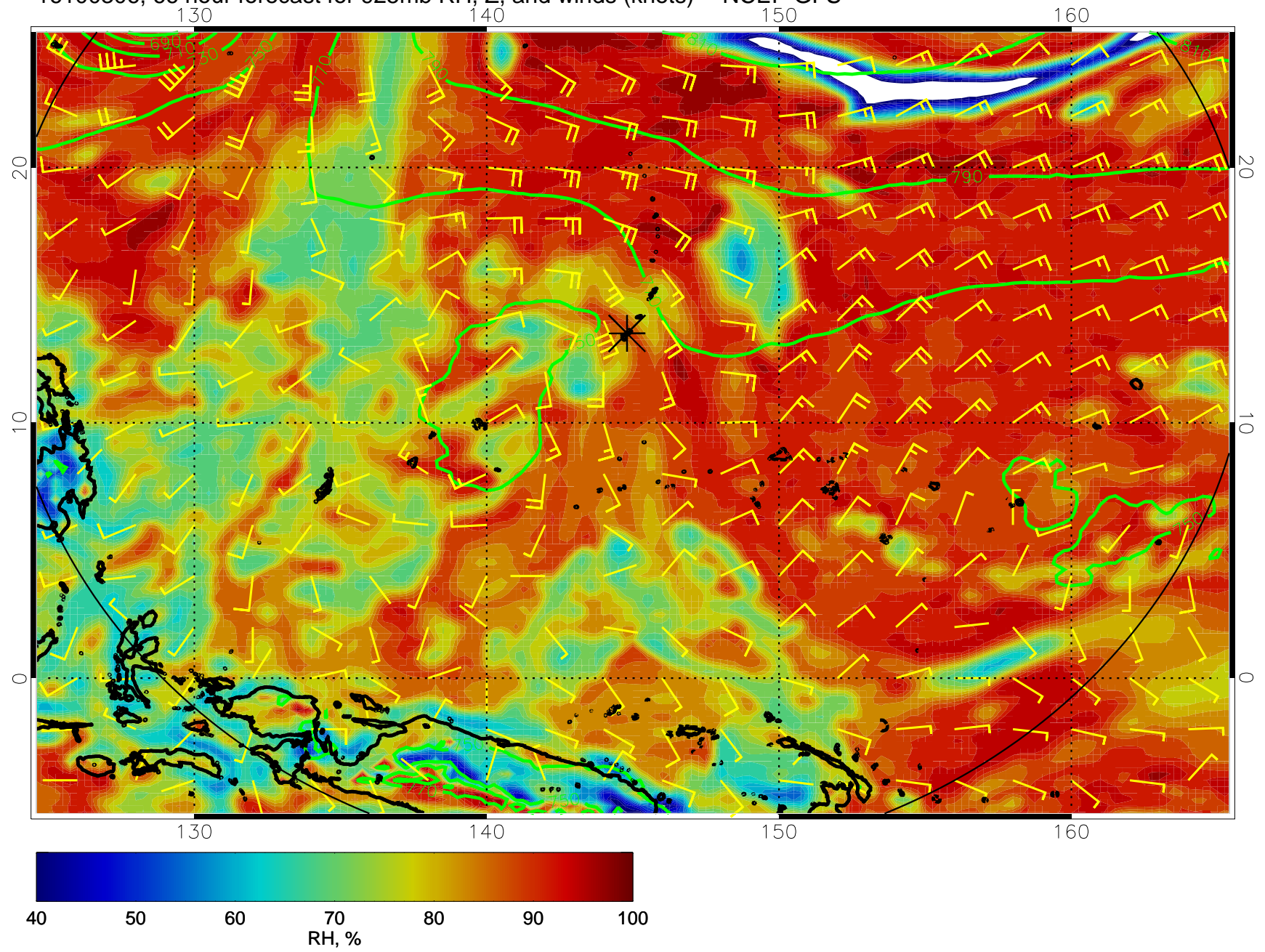
16100306, 66 hour forecast for 925mb RH, Z, and winds (knots) -- NCEP GFS
