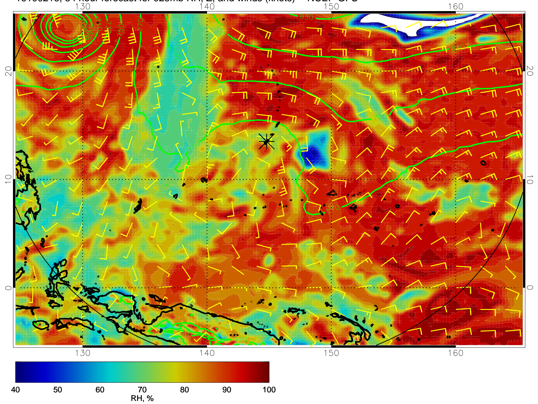
16100218, 54 hour forecast for 925mb RH, Z, and winds (knots) -- NCEP GFS
