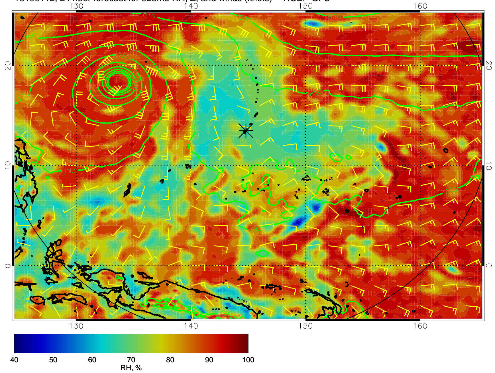
16100112, 24 hour forecast for 925mb RH, Z, and winds (knots) -- NCEP GFS
