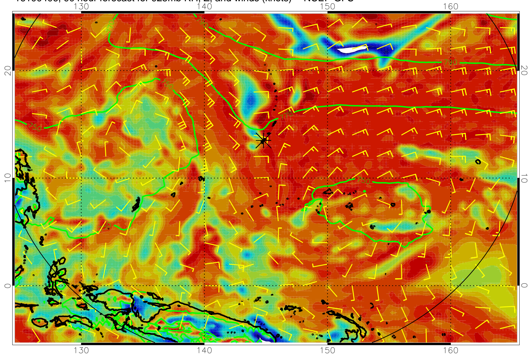
16100406, 90 hour forecast for 925mb RH, Z, and winds (knots) -- NCEP GFS
