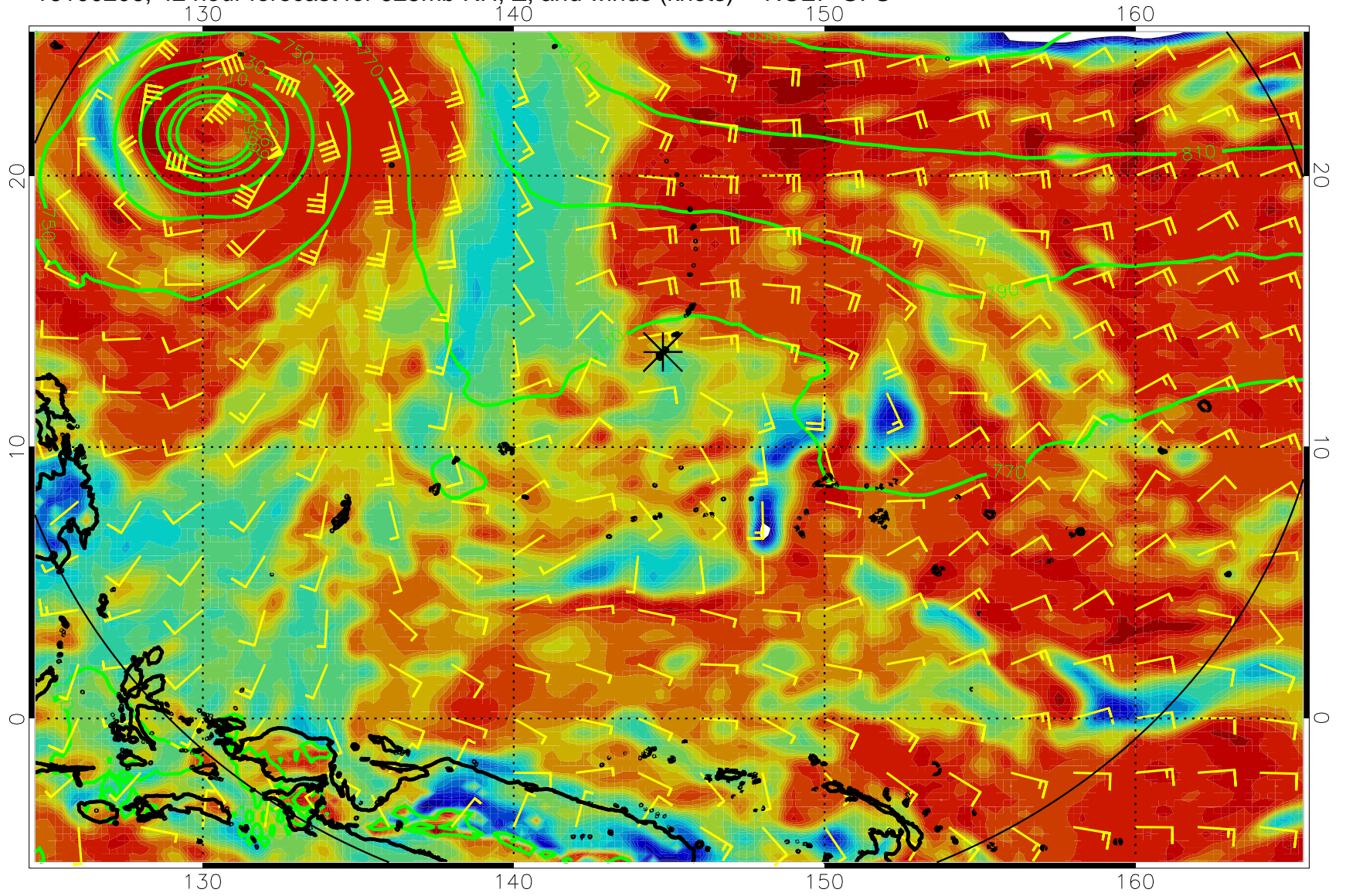
16100206, 42 hour forecast for 925mb RH, Z, and winds (knots) -- NCEP GFS
