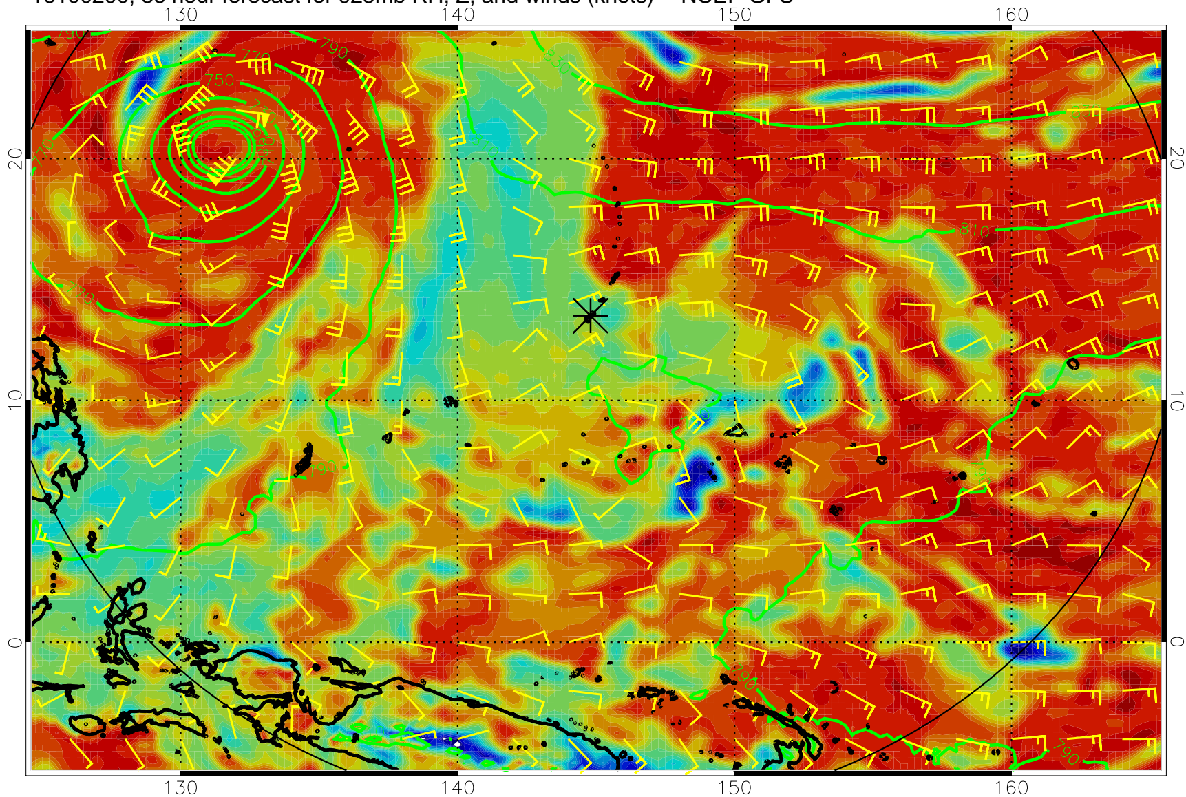
16100200, 36 hour forecast for 925mb RH, Z, and winds (knots) -- NCEP GFS
