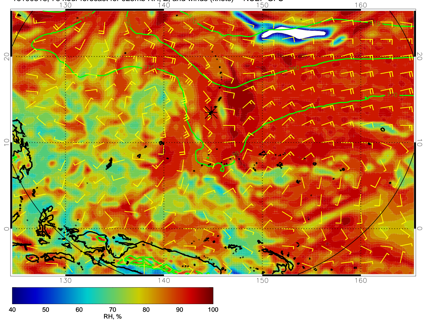
16100318, 78 hour forecast for 925mb RH, Z, and winds (knots) -- NCEP GFS
