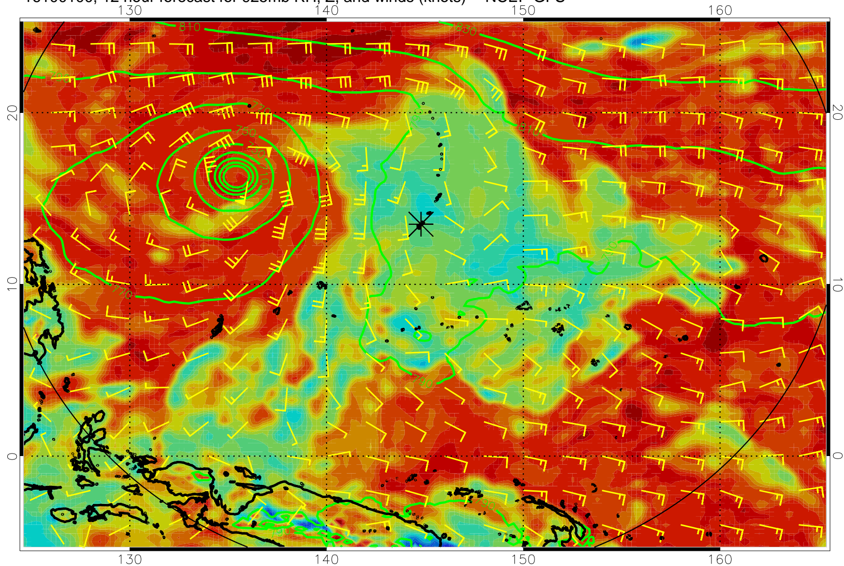
16100100, 12 hour forecast for 925mb RH, Z, and winds (knots) -- NCEP GFS
