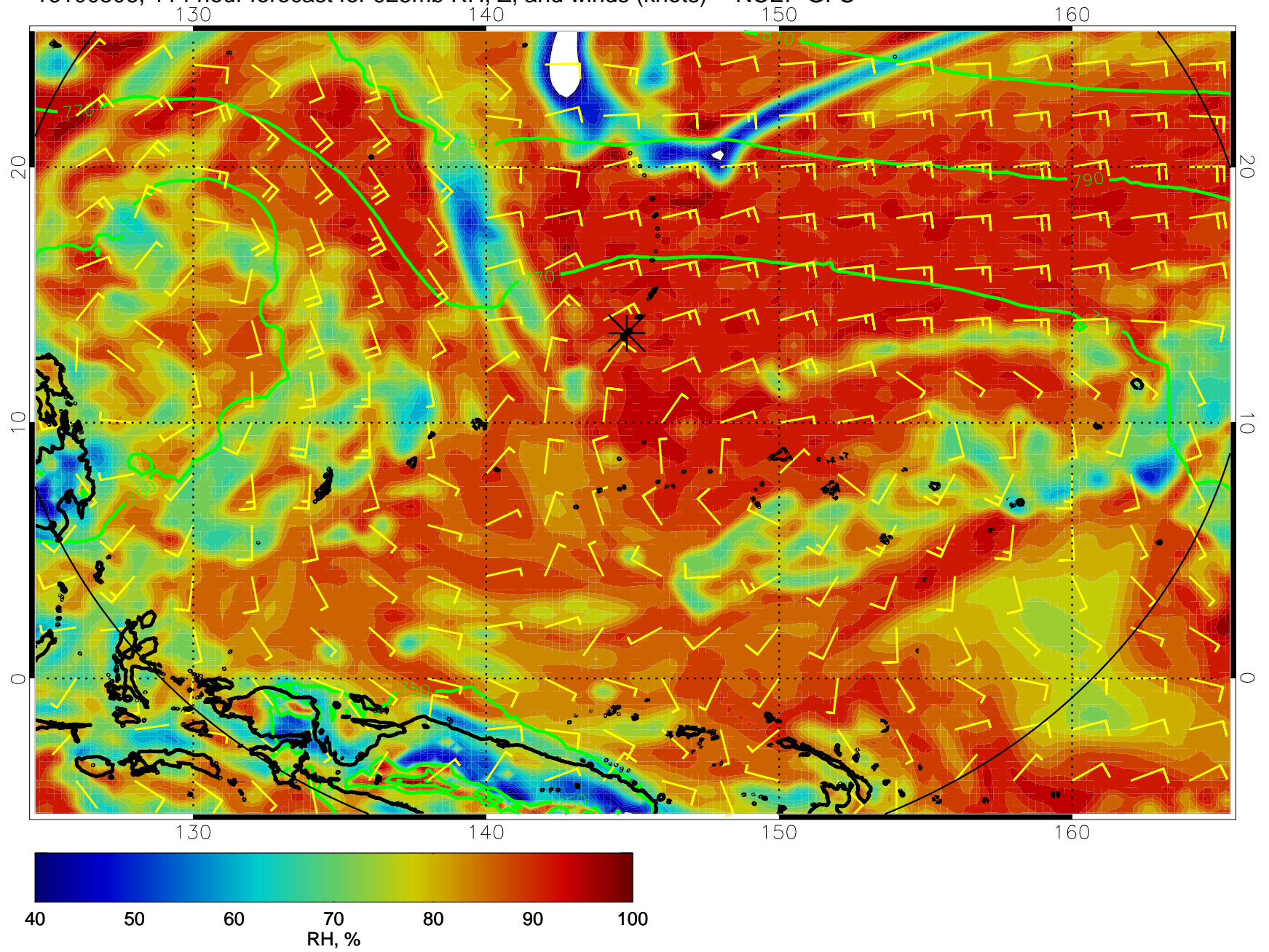
16100506, 114 hour forecast for 925mb RH, Z, and winds (knots) -- NCEP GFS
