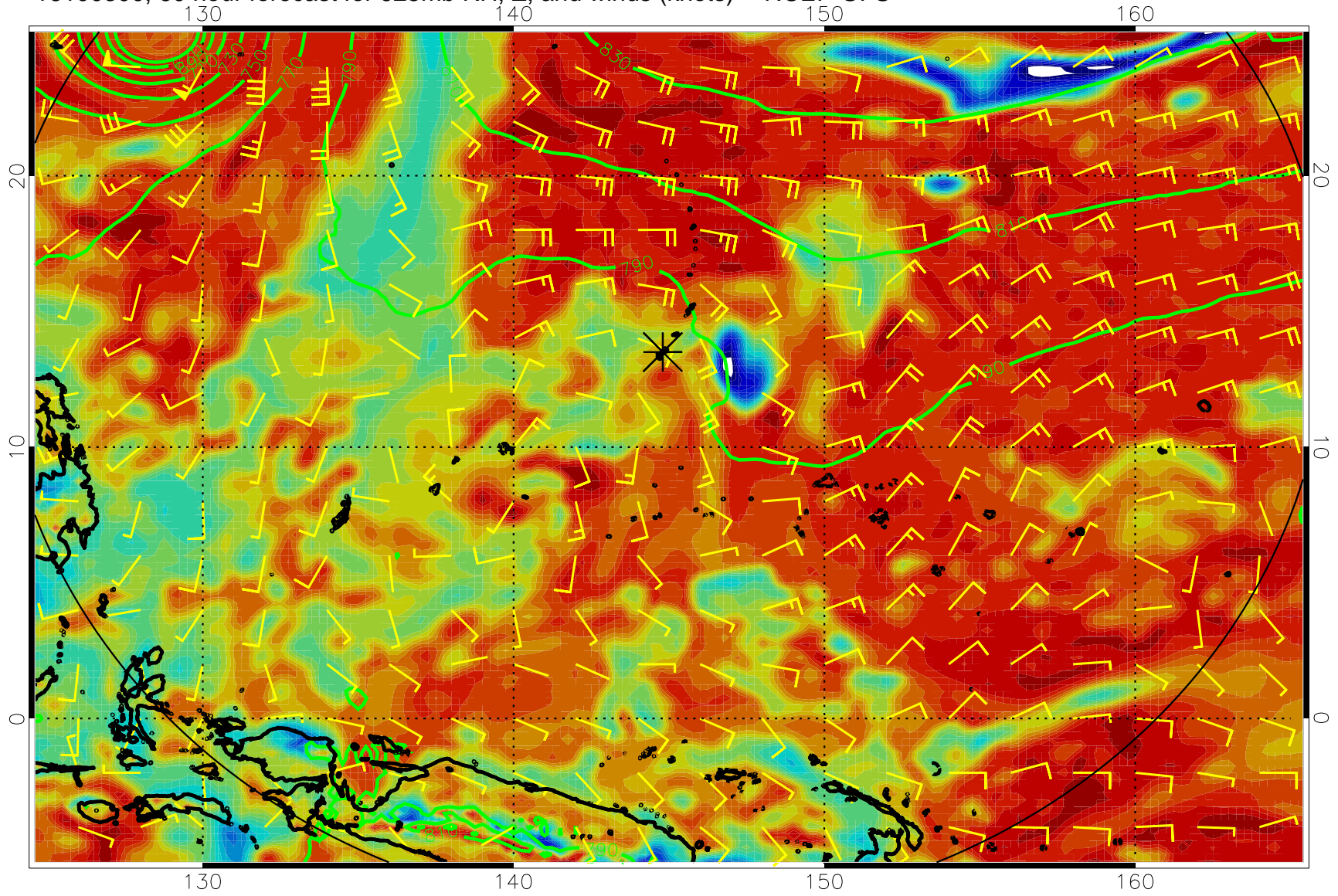
16100300, 60 hour forecast for 925mb RH, Z, and winds (knots) -- NCEP GFS
