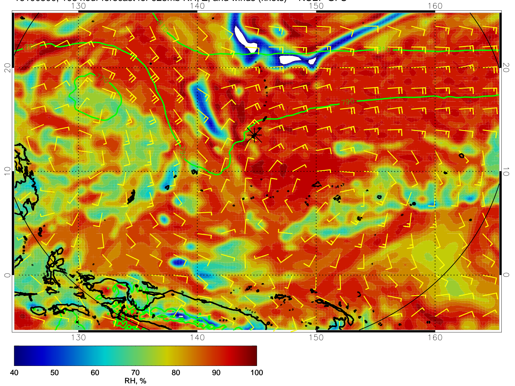
16100500, 108 hour forecast for 925mb RH, Z, and winds (knots) -- NCEP GFS
