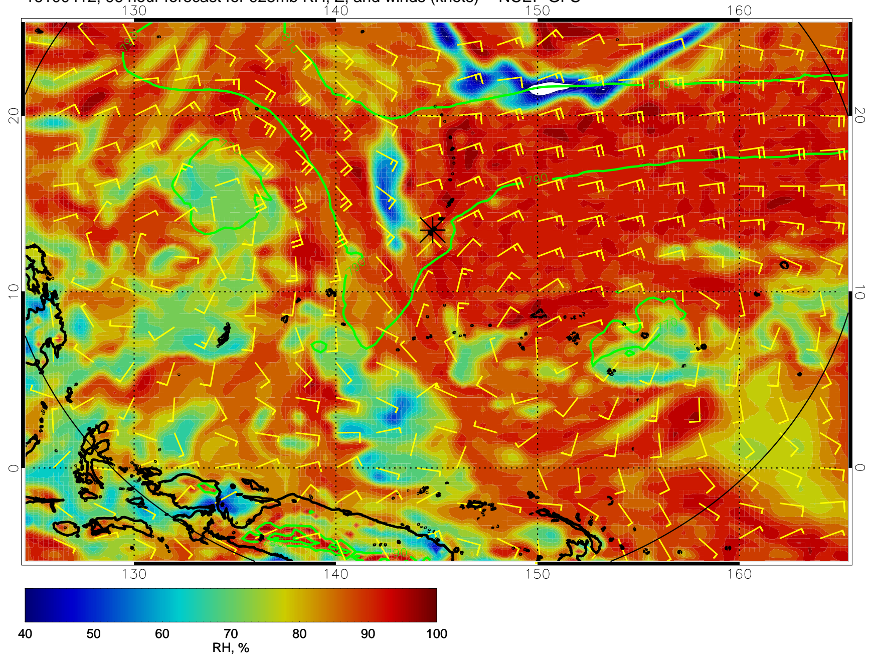
16100412, 96 hour forecast for 925mb RH, Z, and winds (knots) -- NCEP GFS
