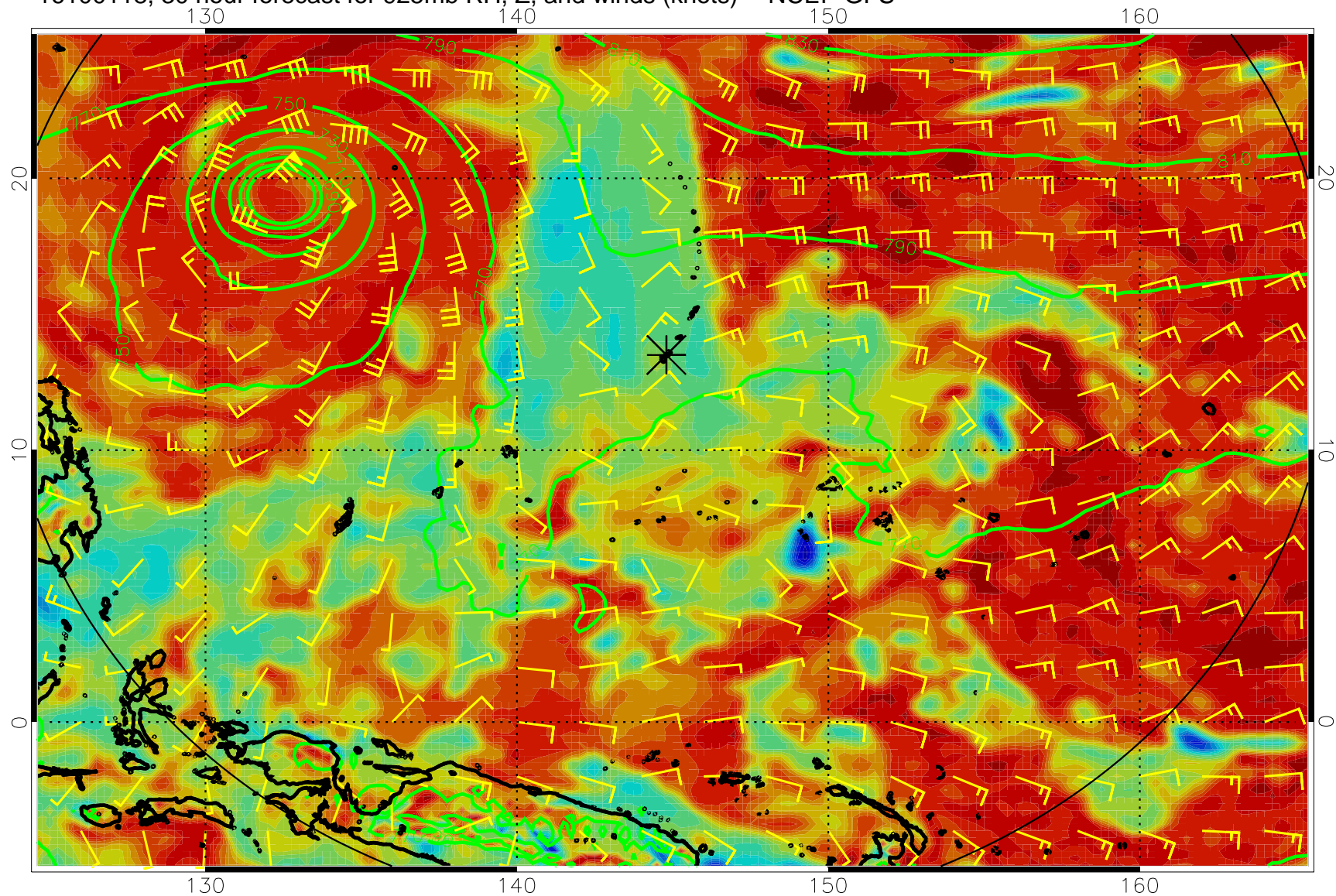
16100118, 30 hour forecast for 925mb RH, Z, and winds (knots) -- NCEP GFS
