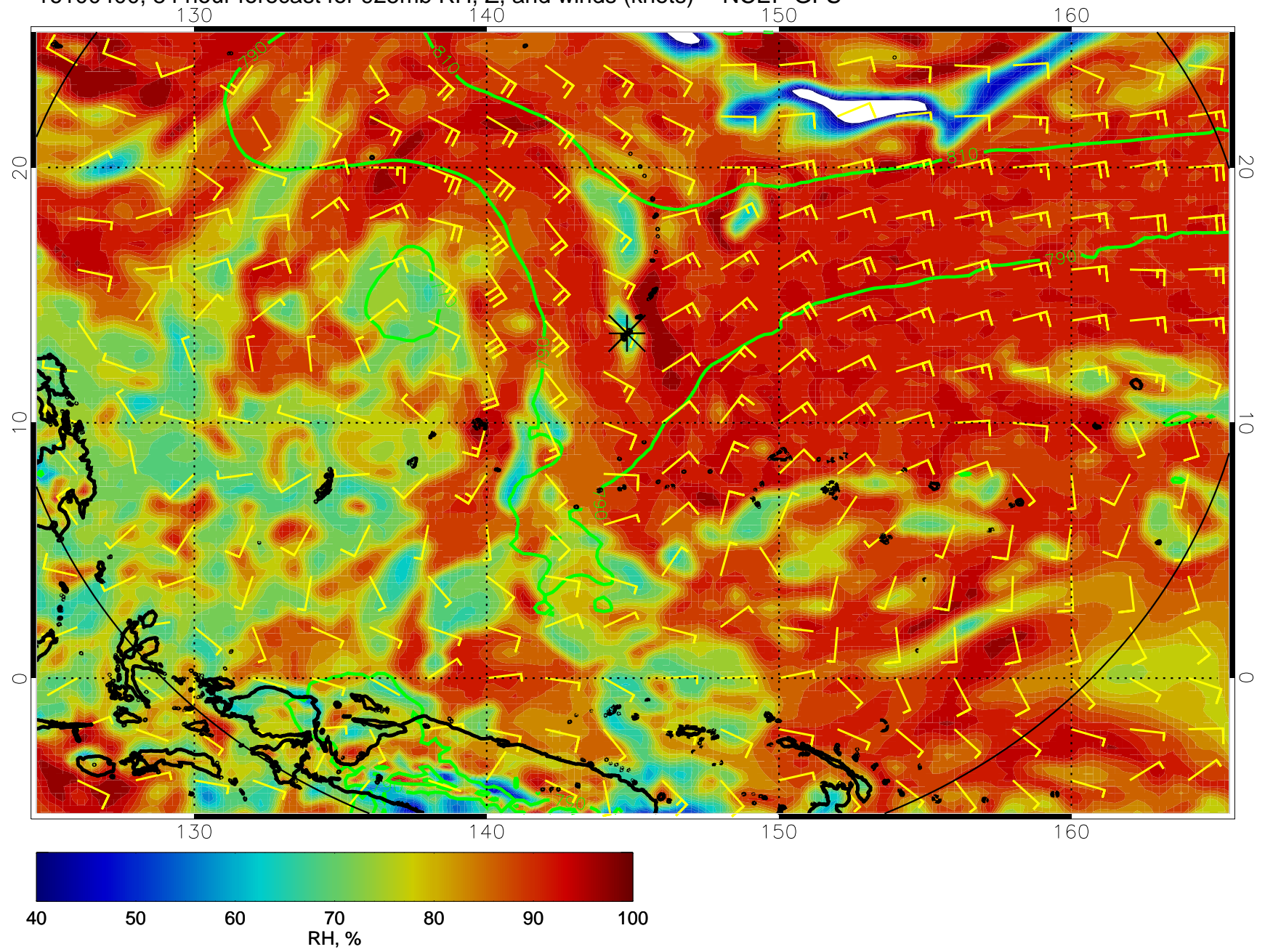
16100400, 84 hour forecast for 925mb RH, Z, and winds (knots) -- NCEP GFS
