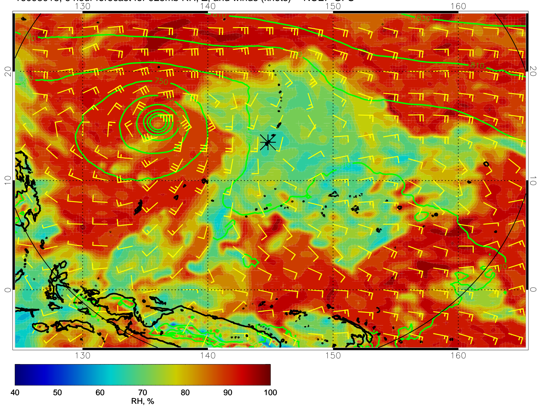
16093018, 6 hour forecast for 925mb RH, Z, and winds (knots) -- NCEP GFS
