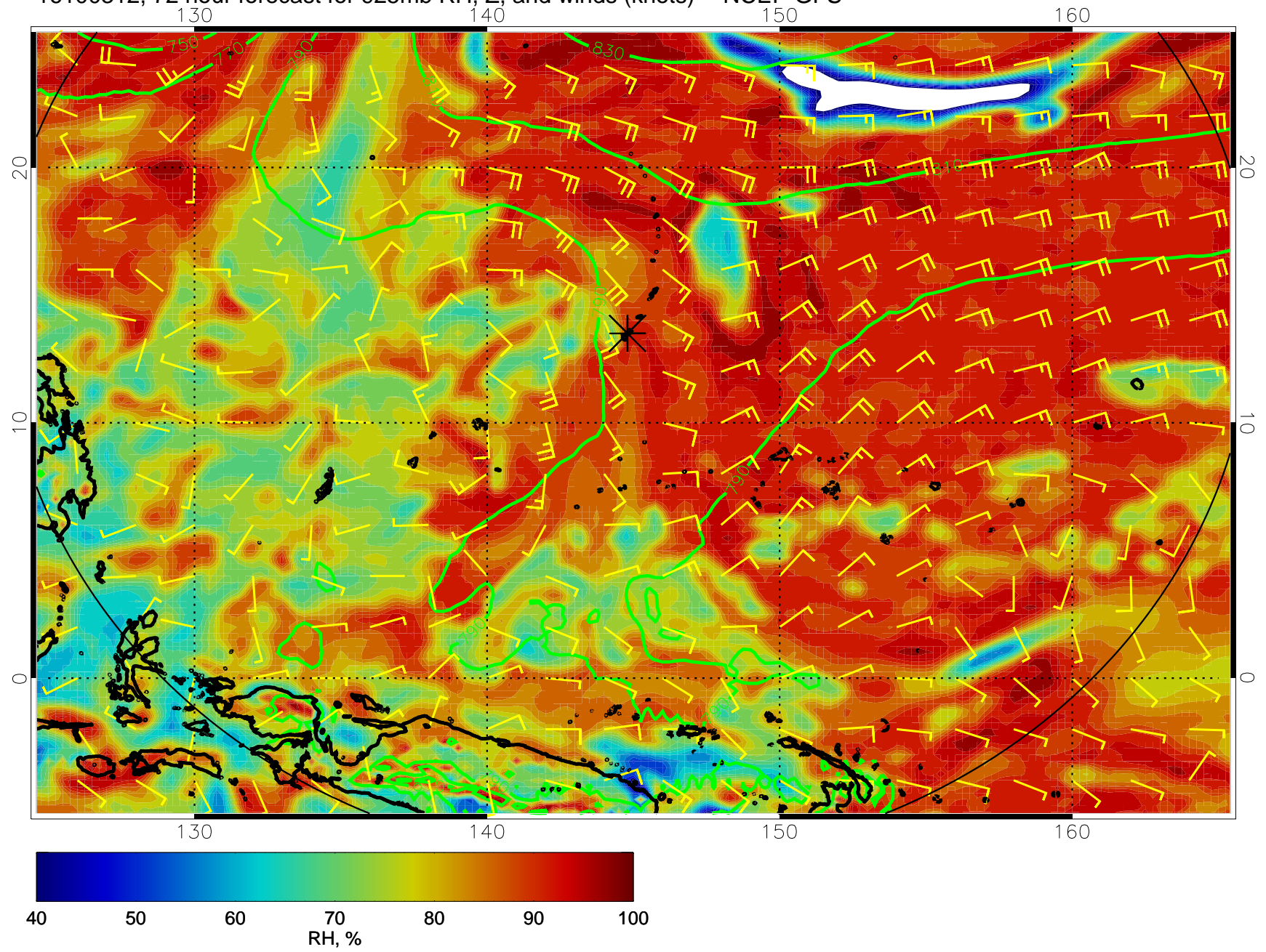
16100312, 72 hour forecast for 925mb RH, Z, and winds (knots) -- NCEP GFS
