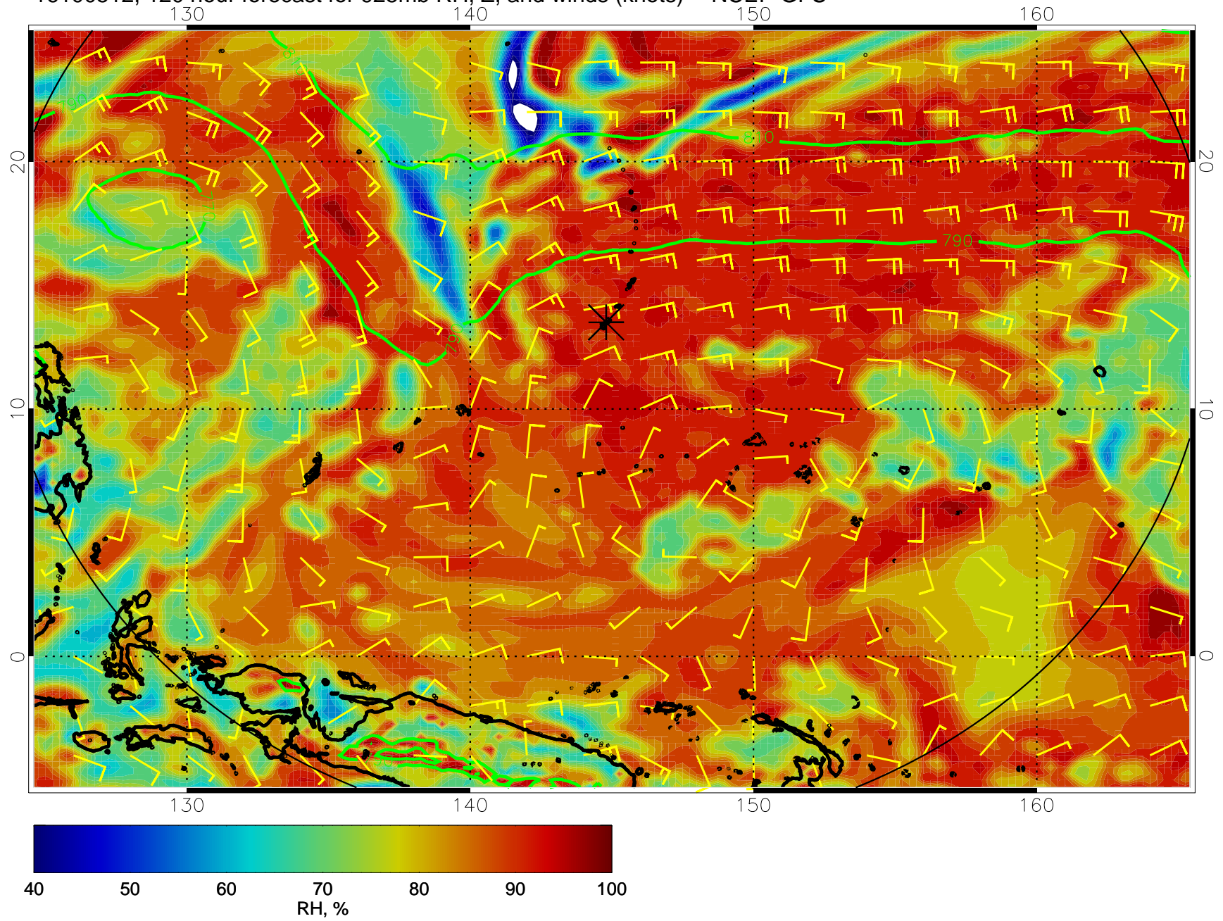
16100512, 120 hour forecast for 925mb RH, Z, and winds (knots) -- NCEP GFS
