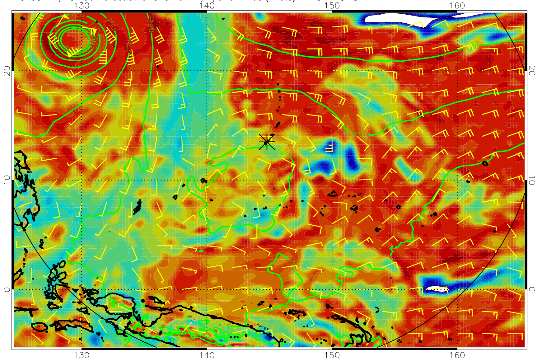
16100212, 48 hour forecast for 925mb RH, Z, and winds (knots) -- NCEP GFS
