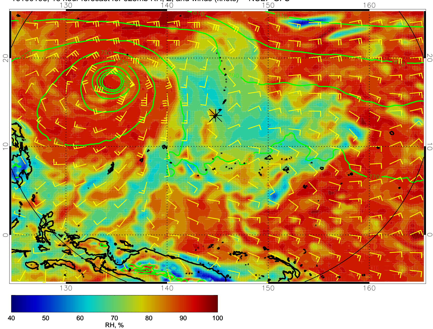
16100106, 18 hour forecast for 925mb RH, Z, and winds (knots) -- NCEP GFS
