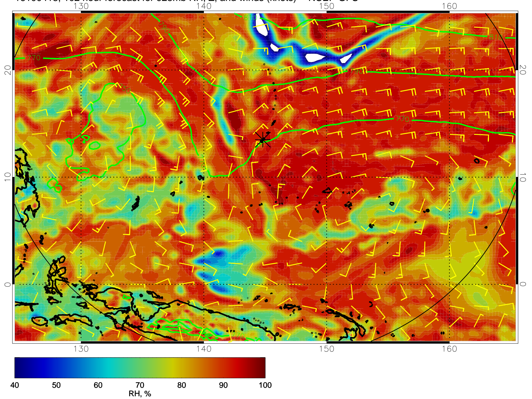
16100418, 102 hour forecast for 925mb RH, Z, and winds (knots) -- NCEP GFS
