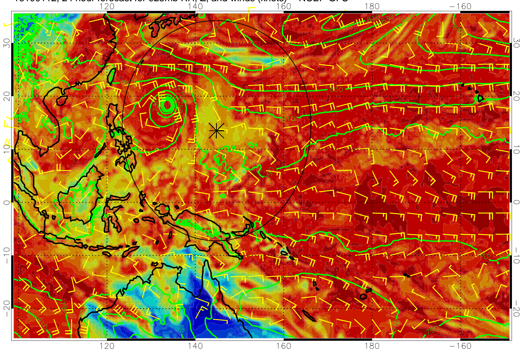
16100112, 24 hour forecast for 925mb RH, Z, and winds (knots) -- NCEP GFS
