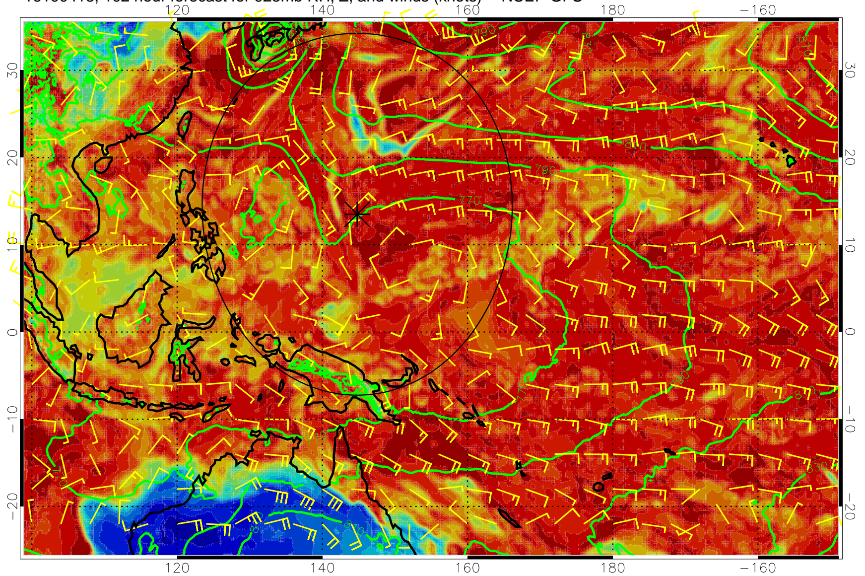
16100418, 102 hour forecast for 925mb RH, Z, and winds (knots) -- NCEP GFS
