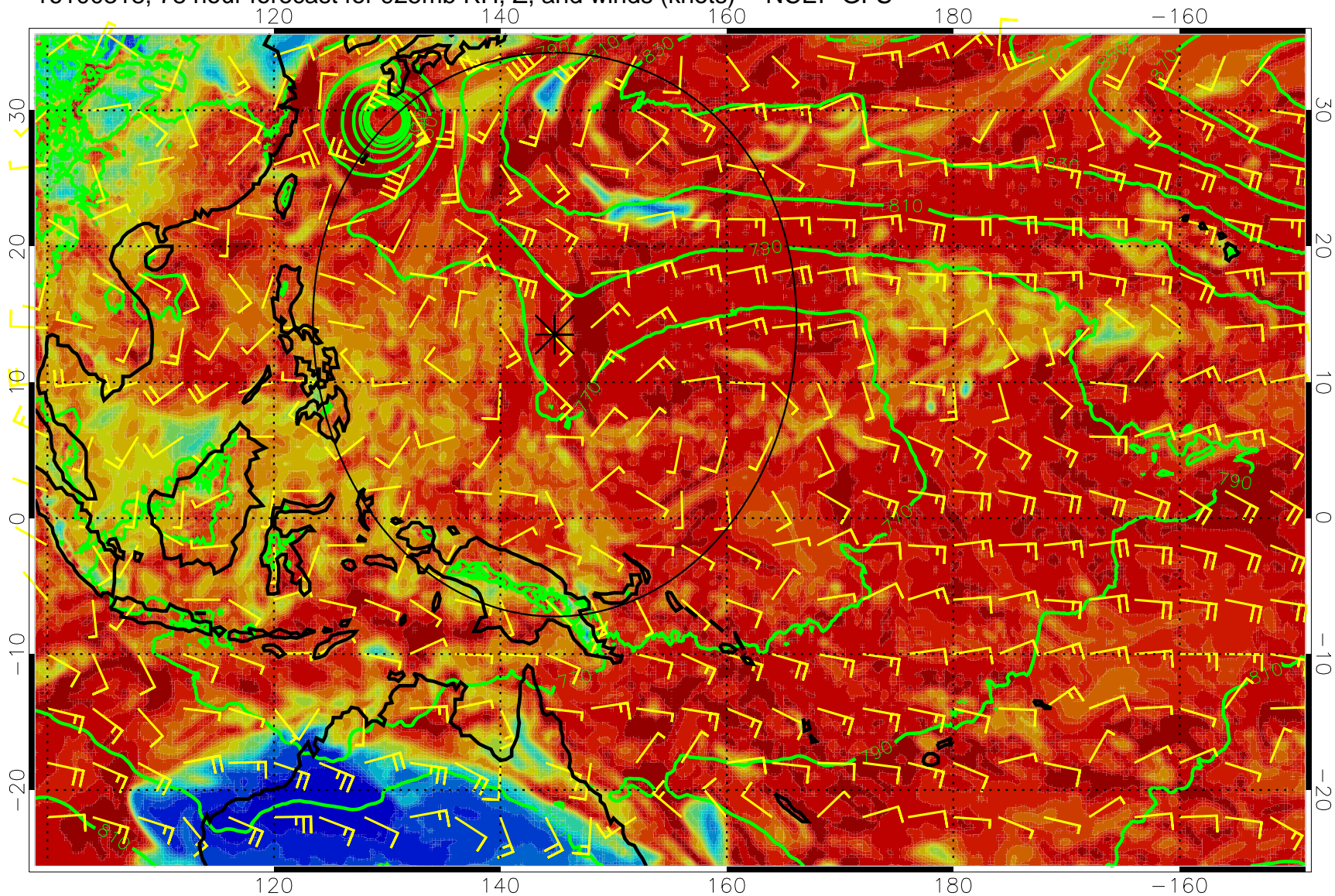
16100318, 78 hour forecast for 925mb RH, Z, and winds (knots) -- NCEP GFS
