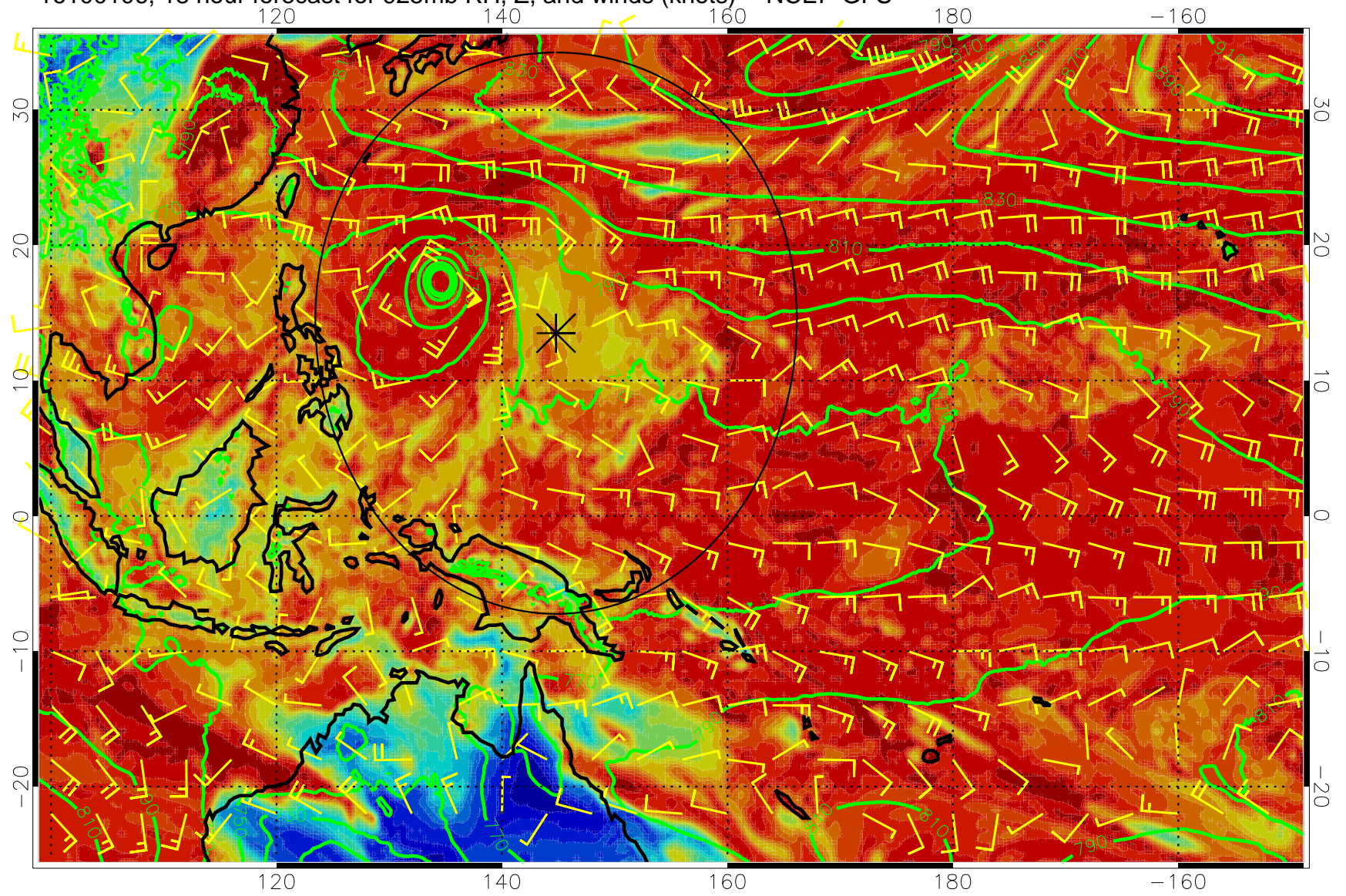
16100106, 18 hour forecast for 925mb RH, Z, and winds (knots) -- NCEP GFS
