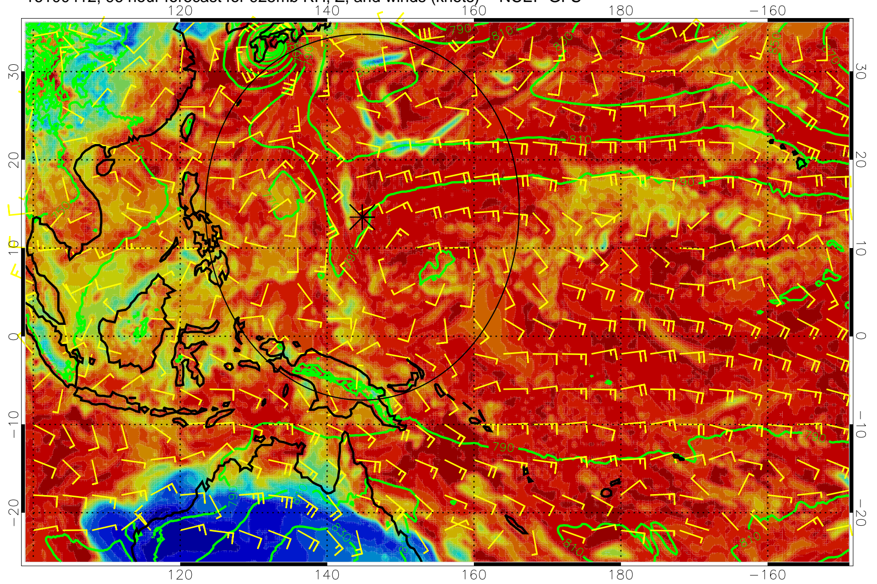
16100412, 96 hour forecast for 925mb RH, Z, and winds (knots) -- NCEP GFS
