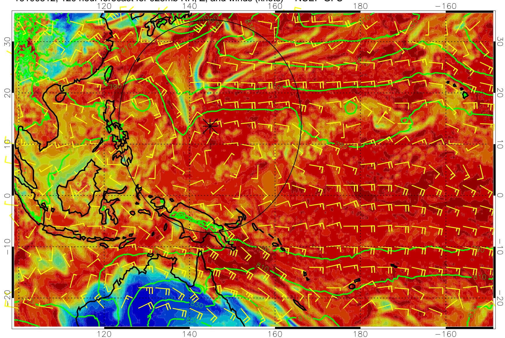
16100512, 120 hour forecast for 925mb RH, Z, and winds (knots) -- NCEP GFS
