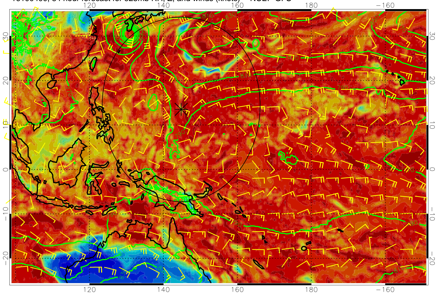
16100400, 84 hour forecast for 925mb RH, Z, and winds (knots) -- NCEP GFS
