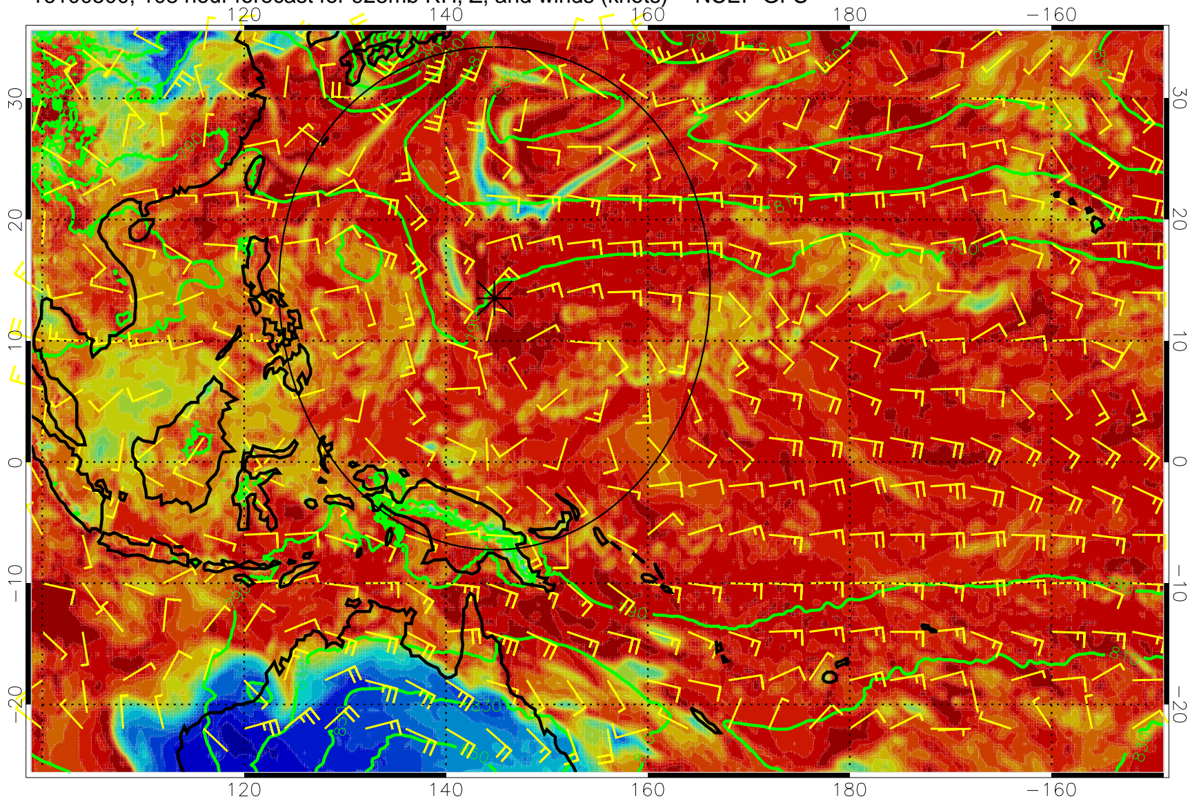
16100500, 108 hour forecast for 925mb RH, Z, and winds (knots) -- NCEP GFS
