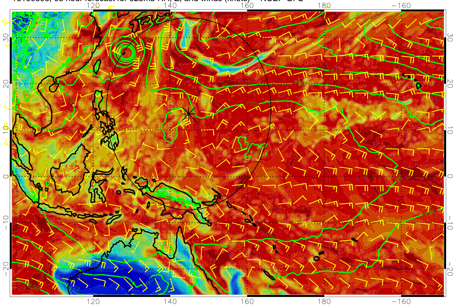
16100306, 66 hour forecast for 925mb RH, Z, and winds (knots) -- NCEP GFS
