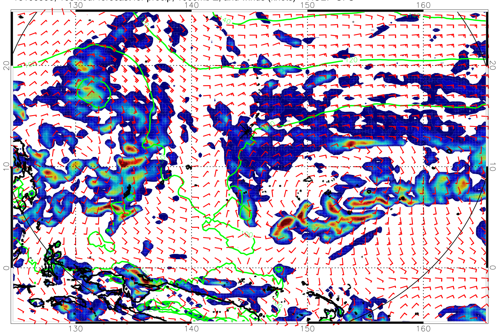
16100500, 108 hour forecast for precip, 1000mb Z, and winds (knots) -- NCEP GFS
