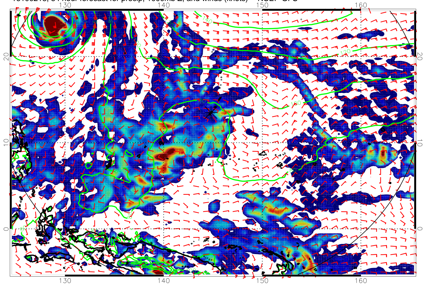
16100218, 54 hour forecast for precip, 1000mb Z, and winds (knots) -- NCEP GFS
