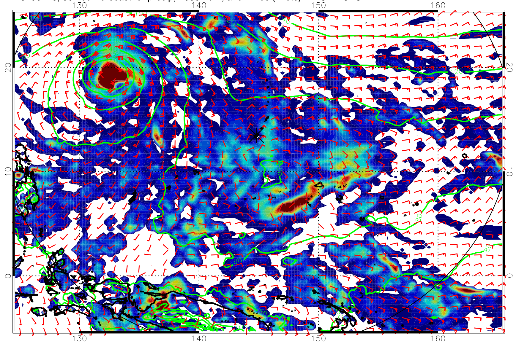
16100118, 30 hour forecast for precip, 1000mb Z, and winds (knots) -- NCEP GFS
