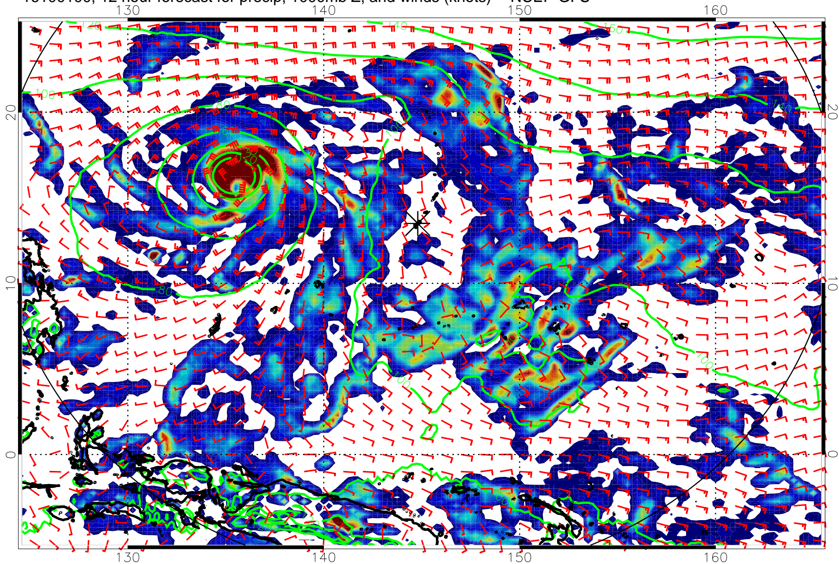
16100100, 12 hour forecast for precip, 1000mb Z, and winds (knots) -- NCEP GFS
