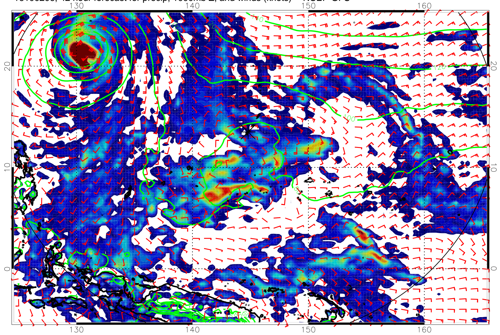
16100206, 42 hour forecast for precip, 1000mb Z, and winds (knots) -- NCEP GFS
