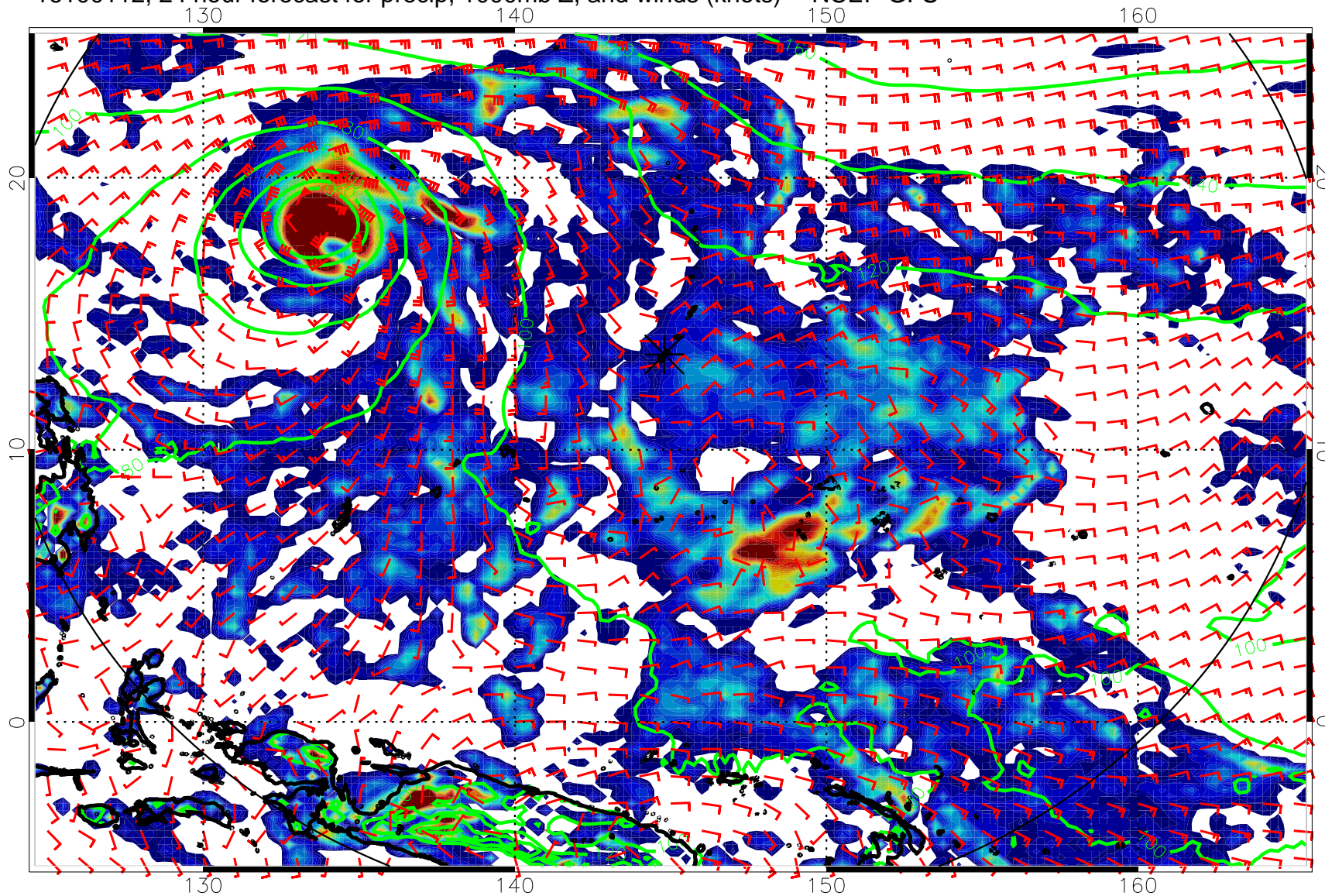
16100112, 24 hour forecast for precip, 1000mb Z, and winds (knots) -- NCEP GFS
