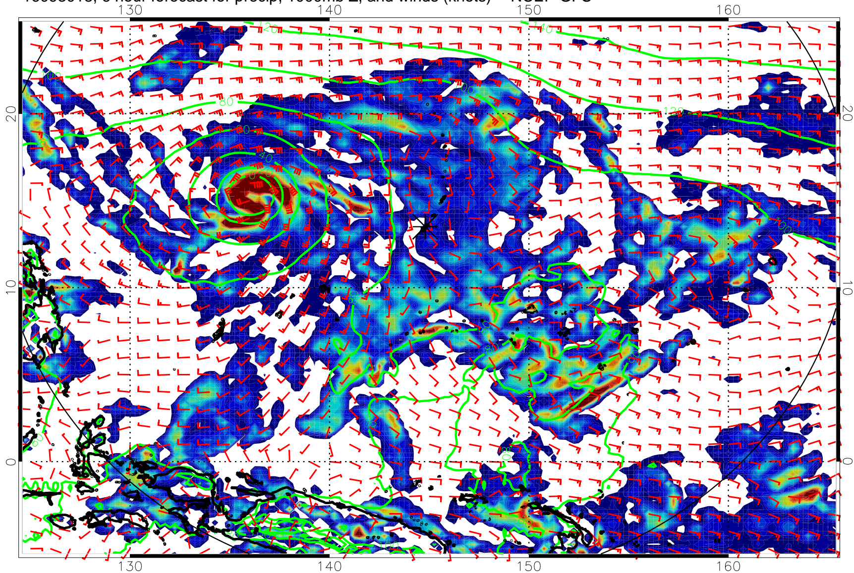
16093018, 6 hour forecast for precip, 1000mb Z, and winds (knots) -- NCEP GFS
