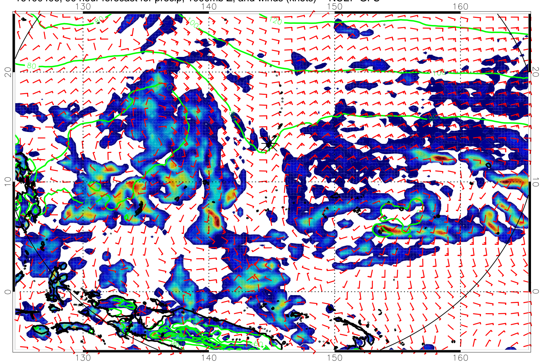
16100406, 90 hour forecast for precip, 1000mb Z, and winds (knots) -- NCEP GFS
