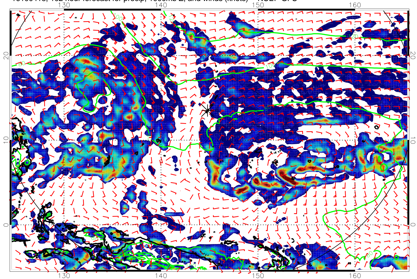
16100418, 102 hour forecast for precip, 1000mb Z, and winds (knots) -- NCEP GFS
