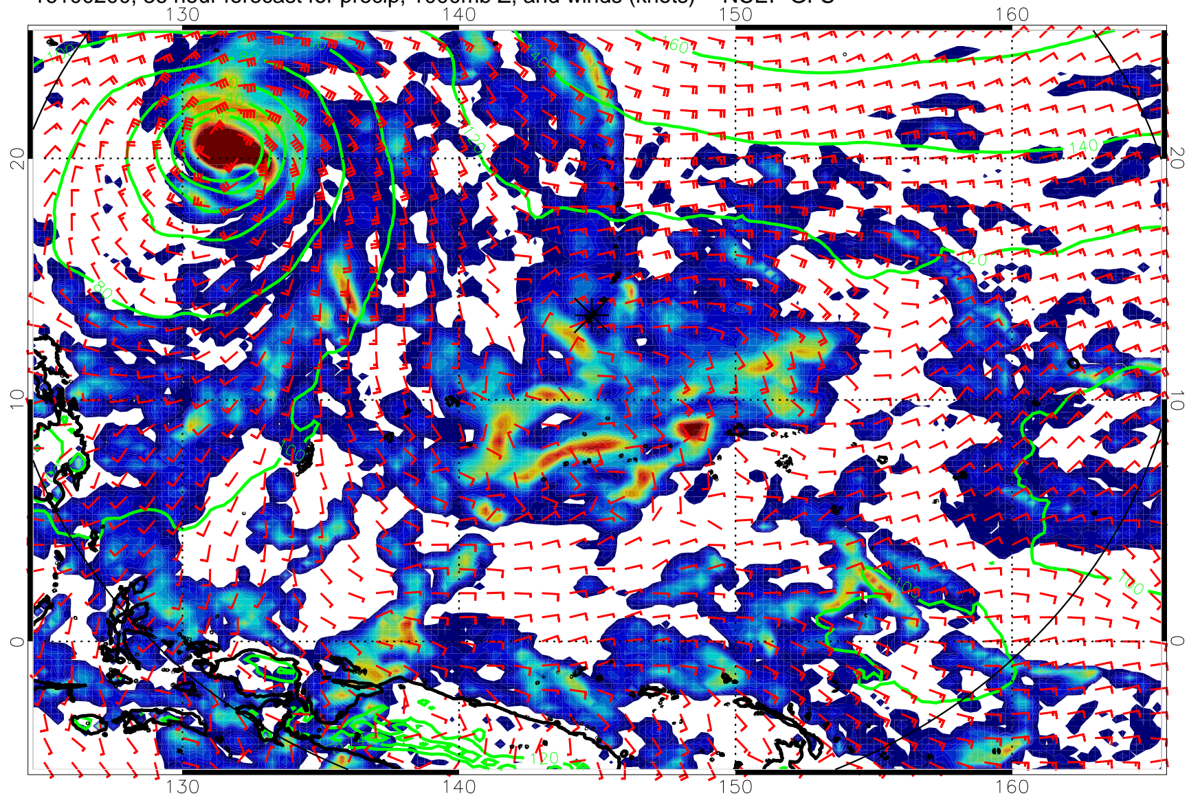
16100200, 36 hour forecast for precip, 1000mb Z, and winds (knots) -- NCEP GFS
