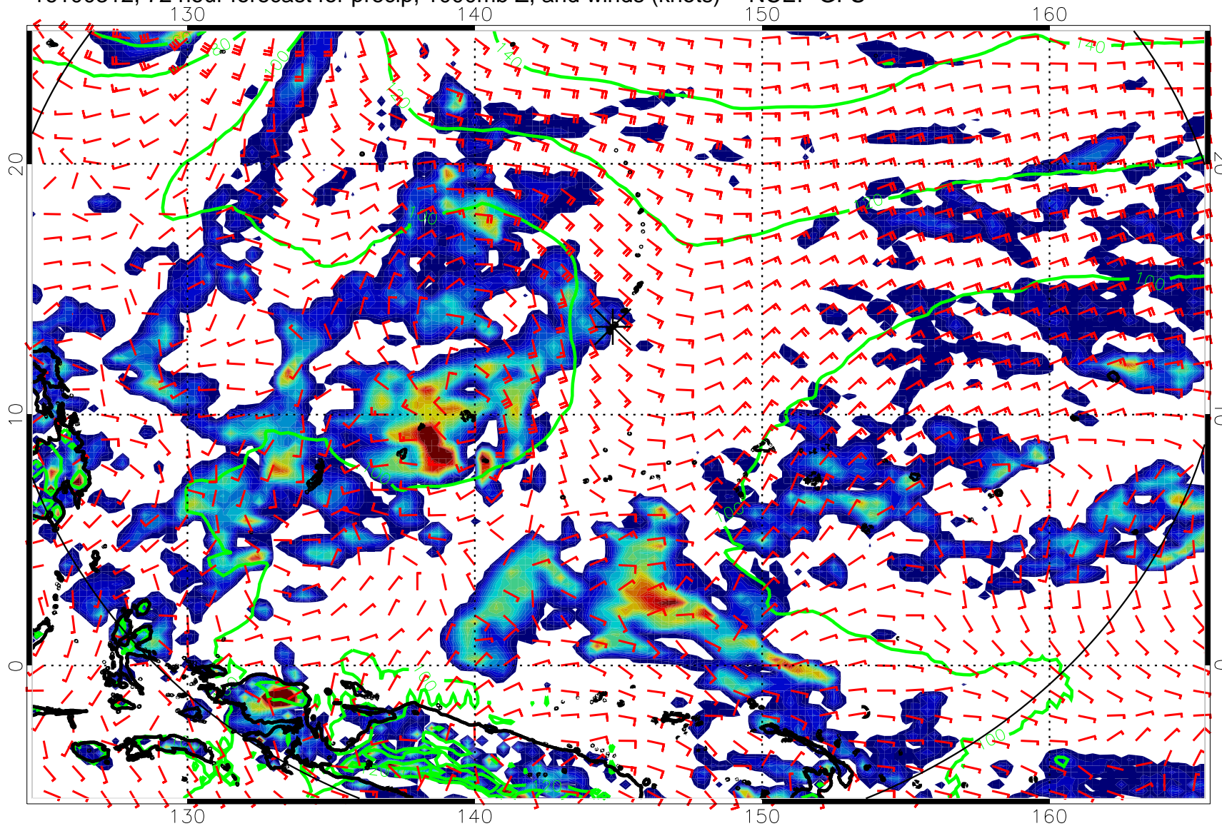
16100312, 72 hour forecast for precip, 1000mb Z, and winds (knots) -- NCEP GFS
