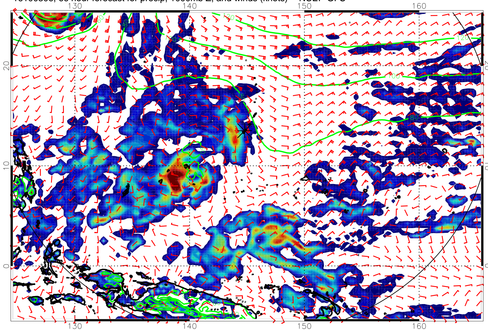
16100306, 66 hour forecast for precip, 1000mb Z, and winds (knots) -- NCEP GFS
