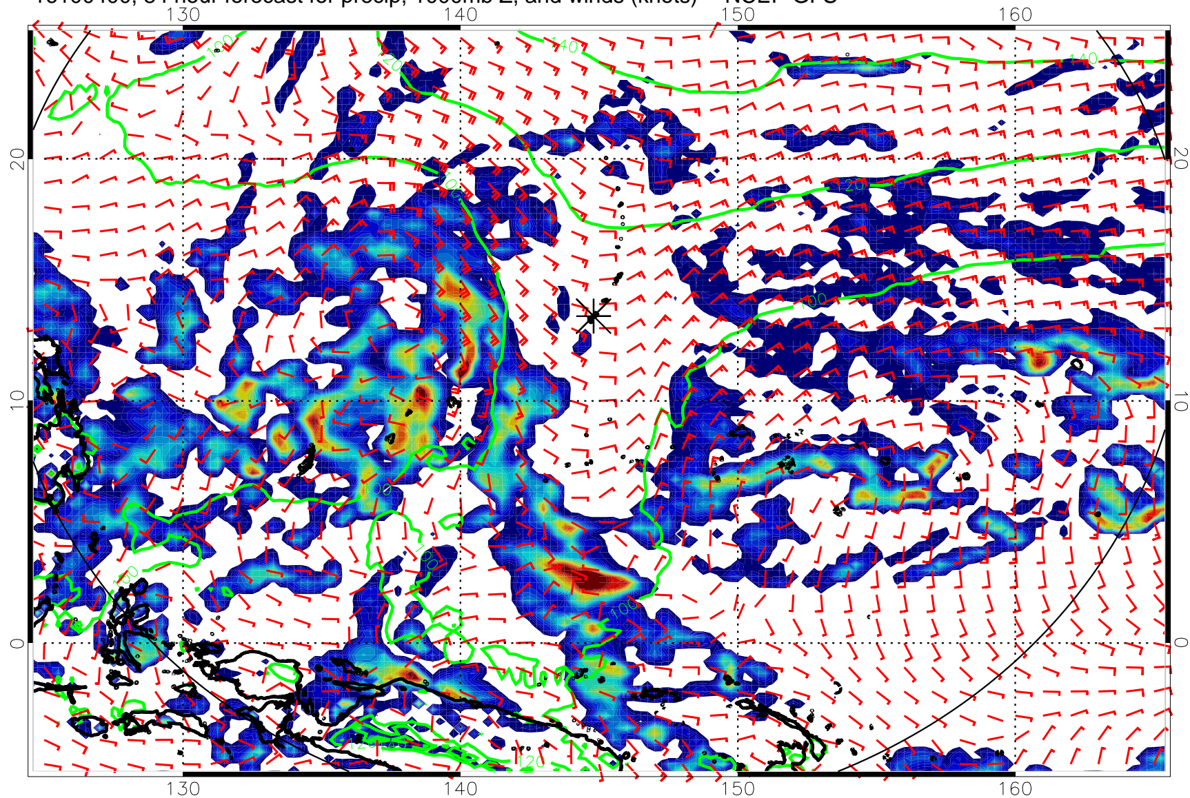
16100400, 84 hour forecast for precip, 1000mb Z, and winds (knots) -- NCEP GFS
