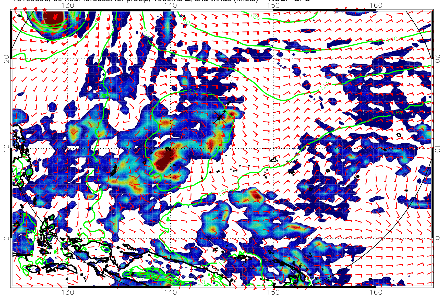
16100300, 60 hour forecast for precip, 1000mb Z, and winds (knots) -- NCEP GFS
