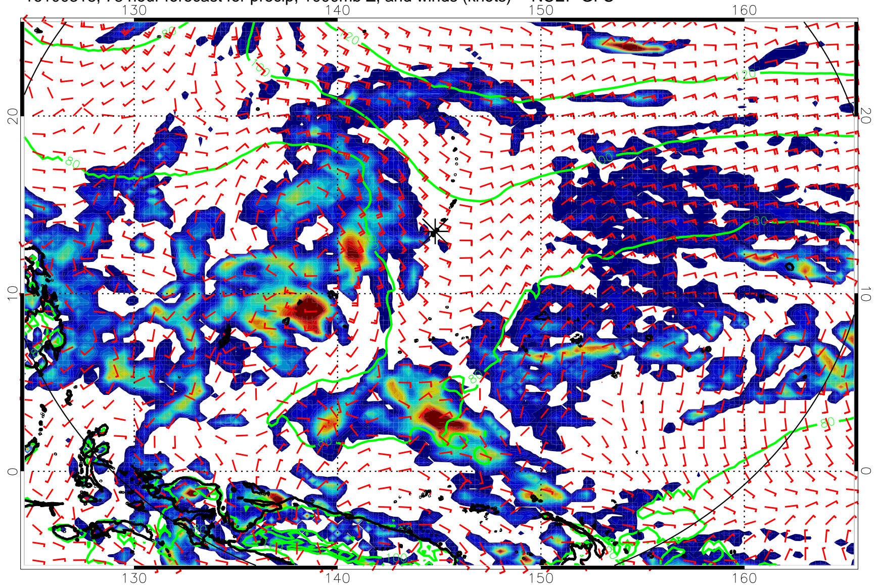
16100318, 78 hour forecast for precip, 1000mb Z, and winds (knots) -- NCEP GFS
