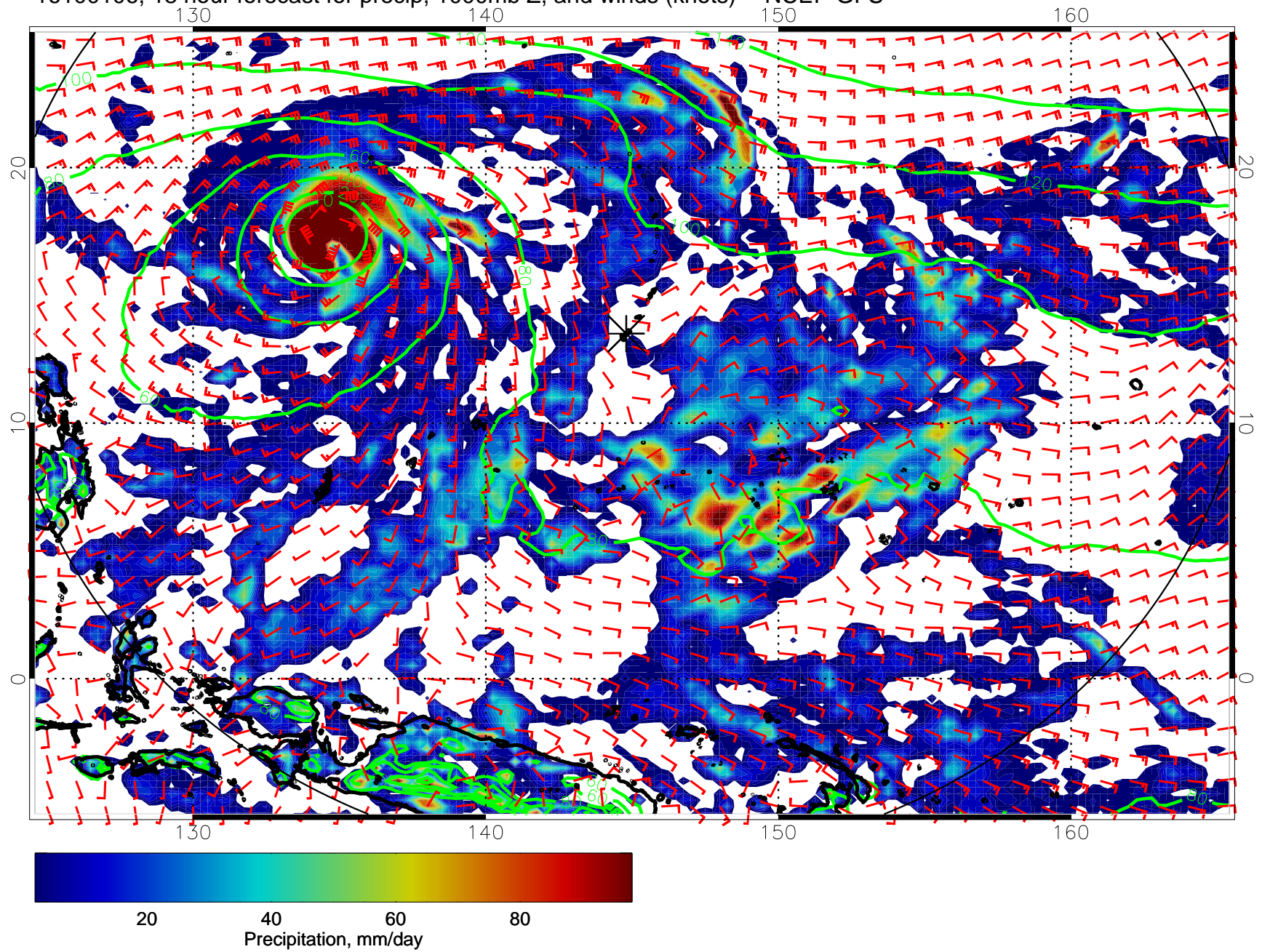
16100106, 18 hour forecast for precip, 1000mb Z, and winds (knots) -- NCEP GFS
