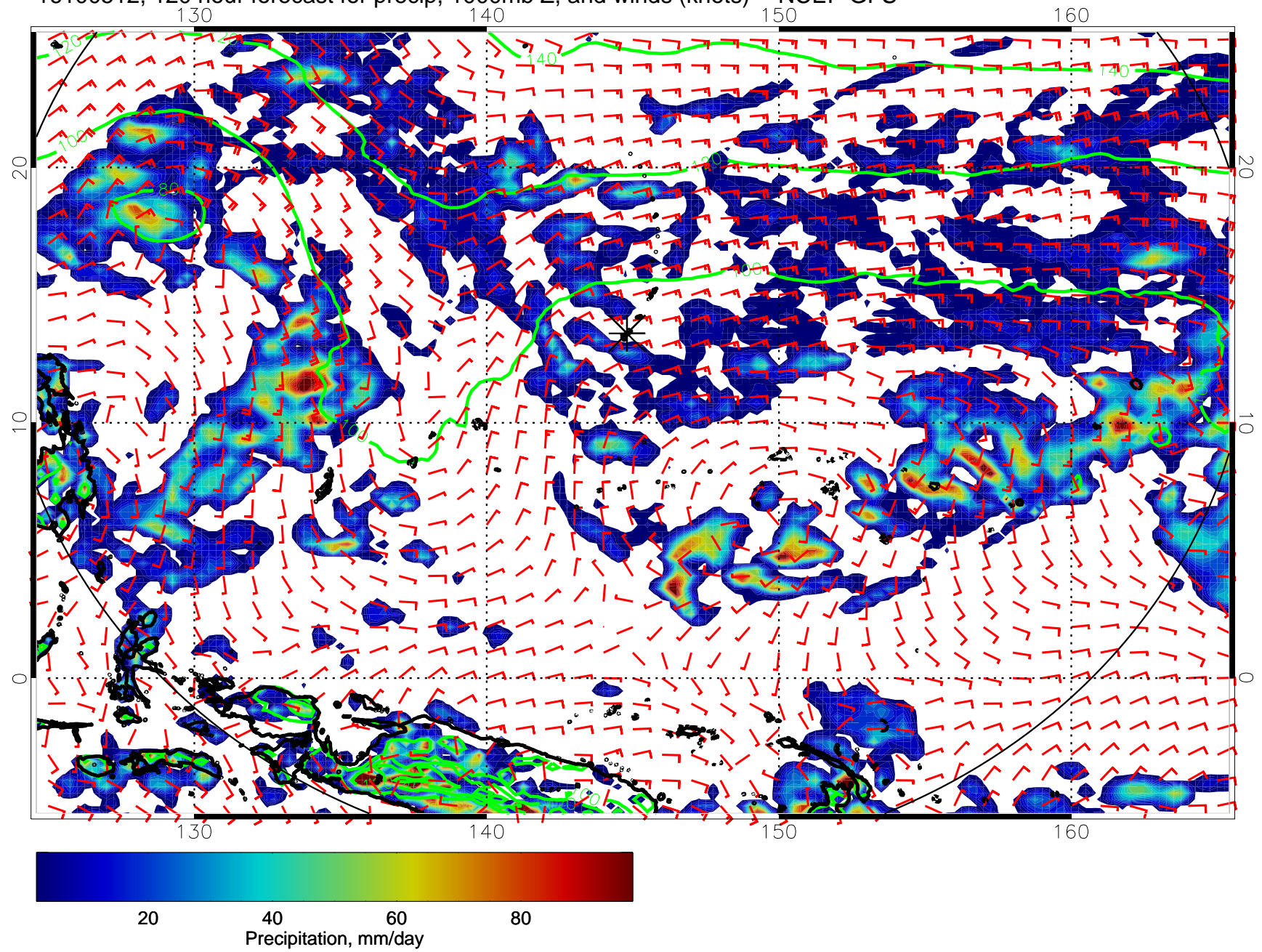
16100512, 120 hour forecast for precip, 1000mb Z, and winds (knots) -- NCEP GFS
