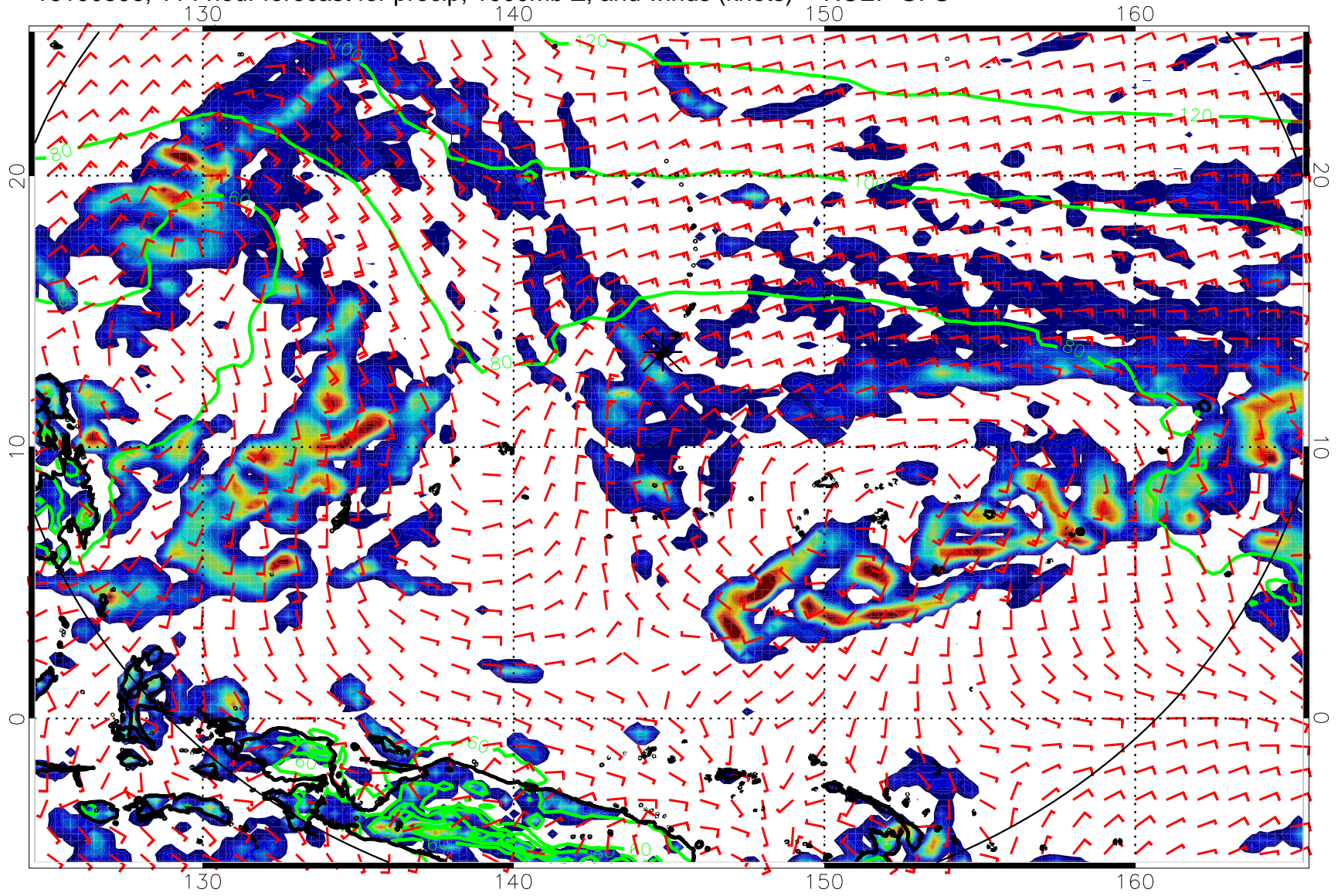
16100506, 114 hour forecast for precip, 1000mb Z, and winds (knots) -- NCEP GFS
