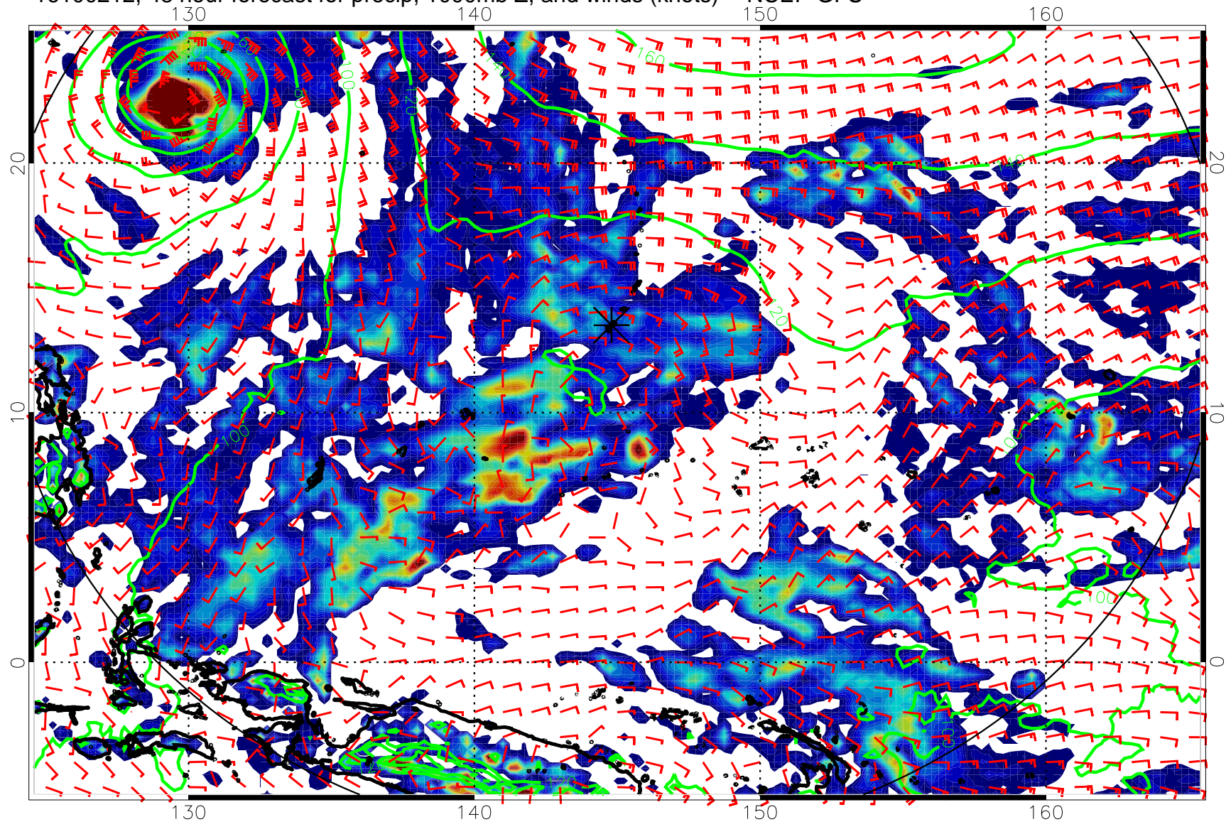
16100212, 48 hour forecast for precip, 1000mb Z, and winds (knots) -- NCEP GFS
