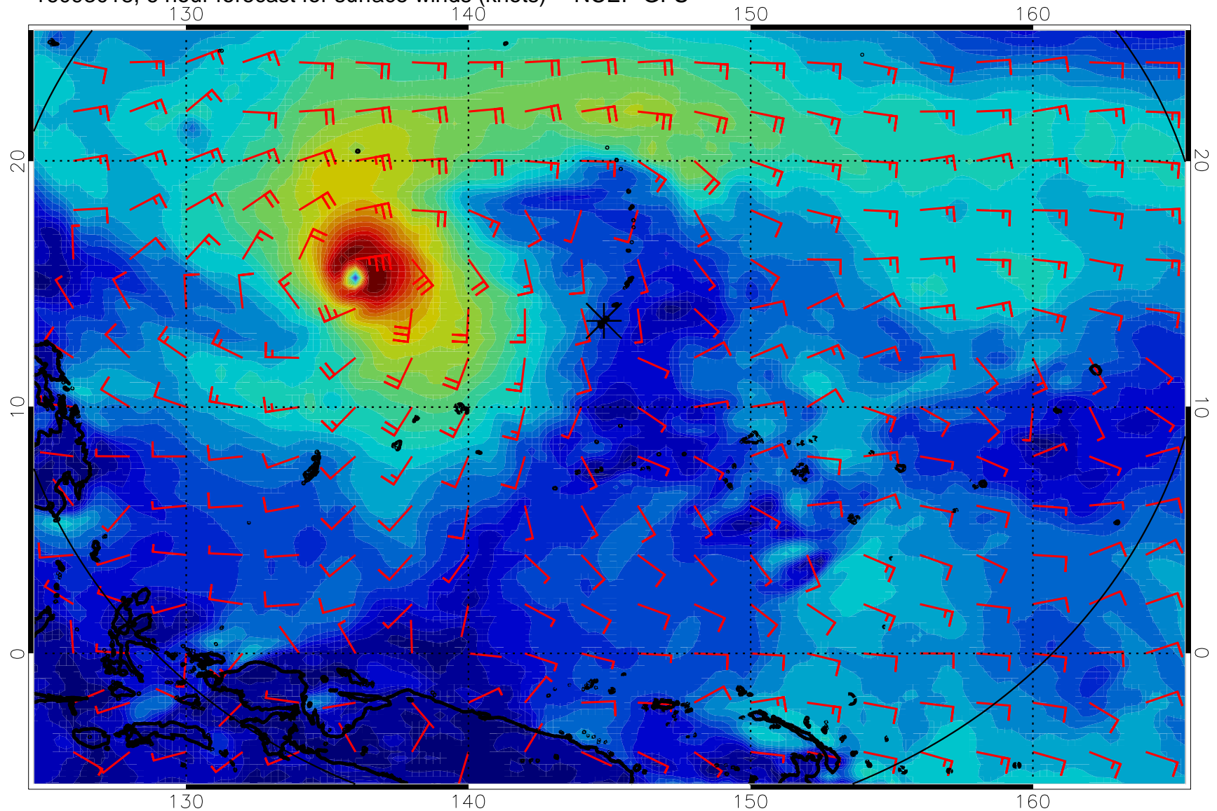
16093018, 6 hour forecast for surface winds (knots) -- NCEP GFS
