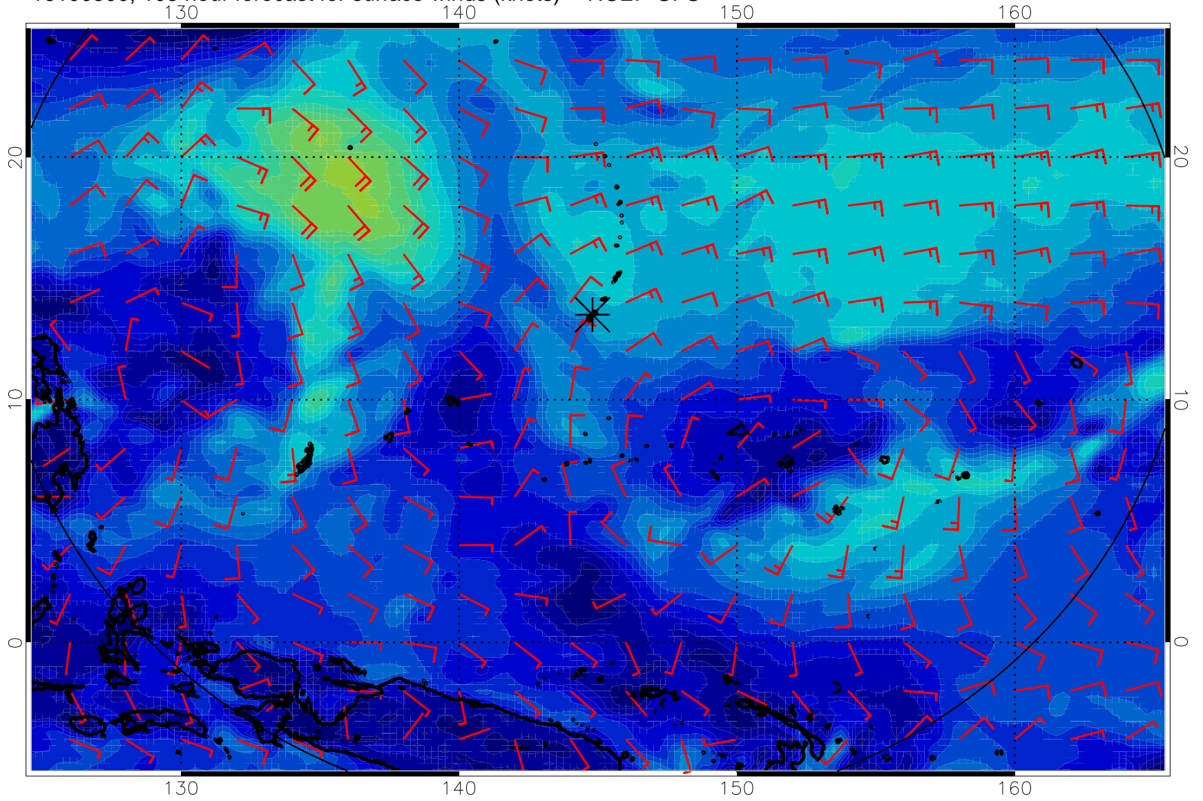
16100500, 108 hour forecast for surface winds (knots) -- NCEP GFS
