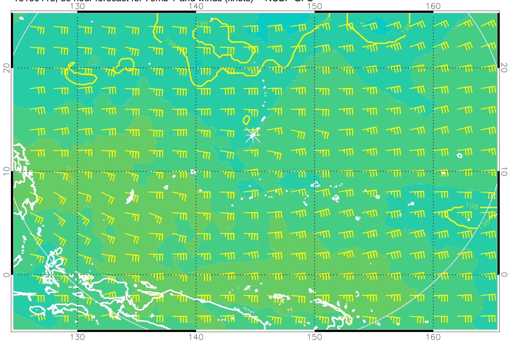
16100118, 30 hour forecast for 70mb T and winds (knots) -- NCEP GFS
