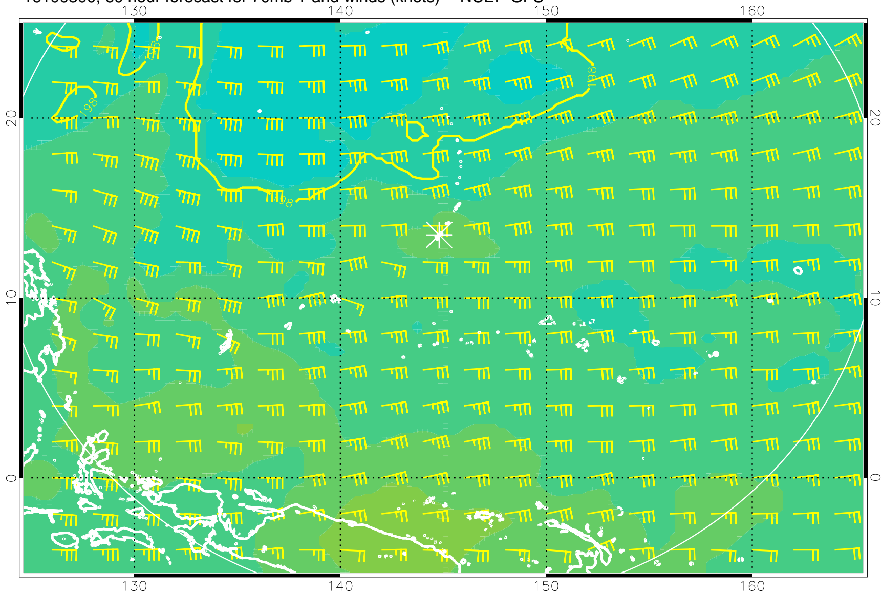
16100300, 60 hour forecast for 70mb T and winds (knots) -- NCEP GFS
