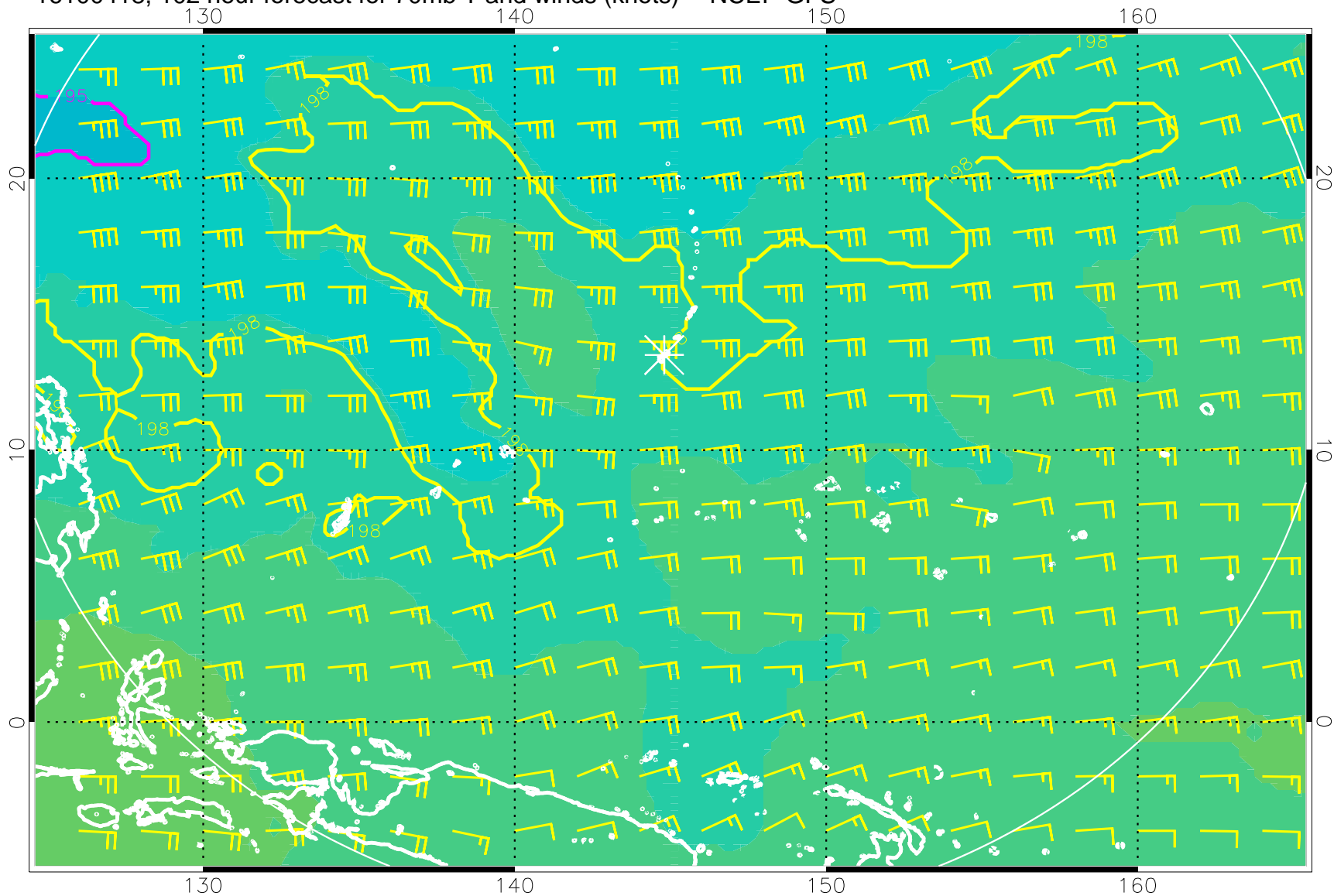
16100418, 102 hour forecast for 70mb T and winds (knots) -- NCEP GFS
