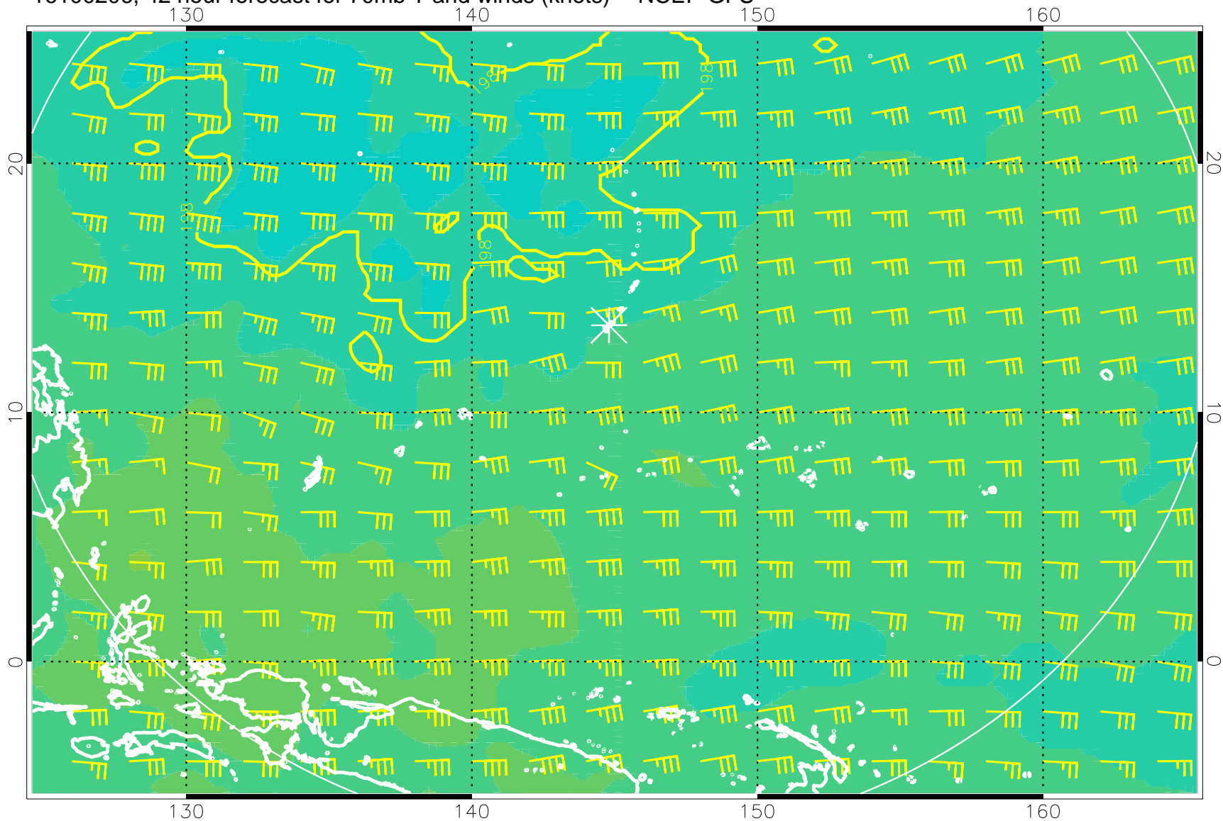
16100206, 42 hour forecast for 70mb T and winds (knots) -- NCEP GFS
