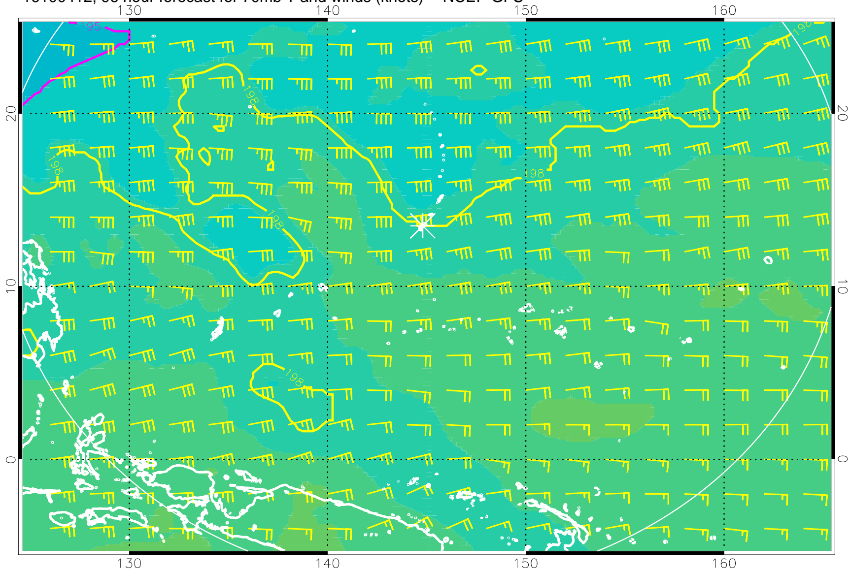
16100412, 96 hour forecast for 70mb T and winds (knots) -- NCEP GFS
