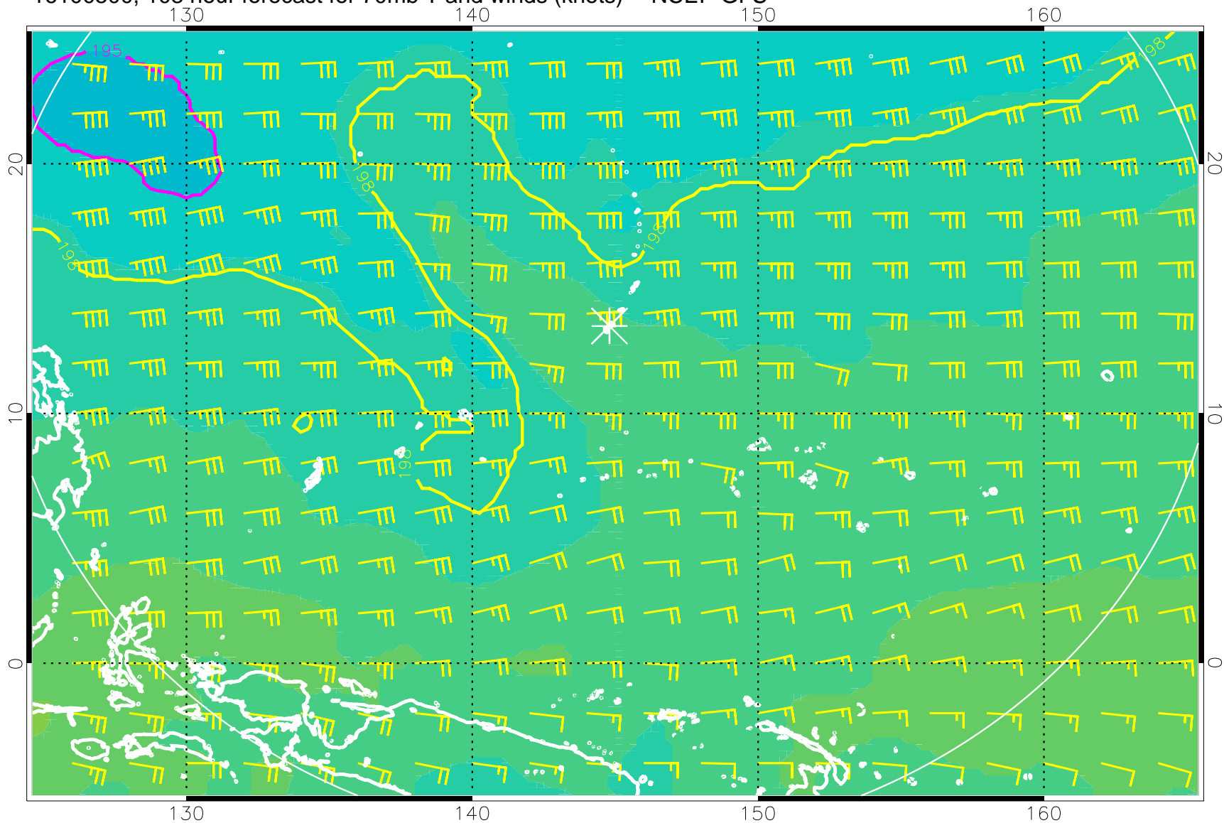
16100500, 108 hour forecast for 70mb T and winds (knots) -- NCEP GFS
