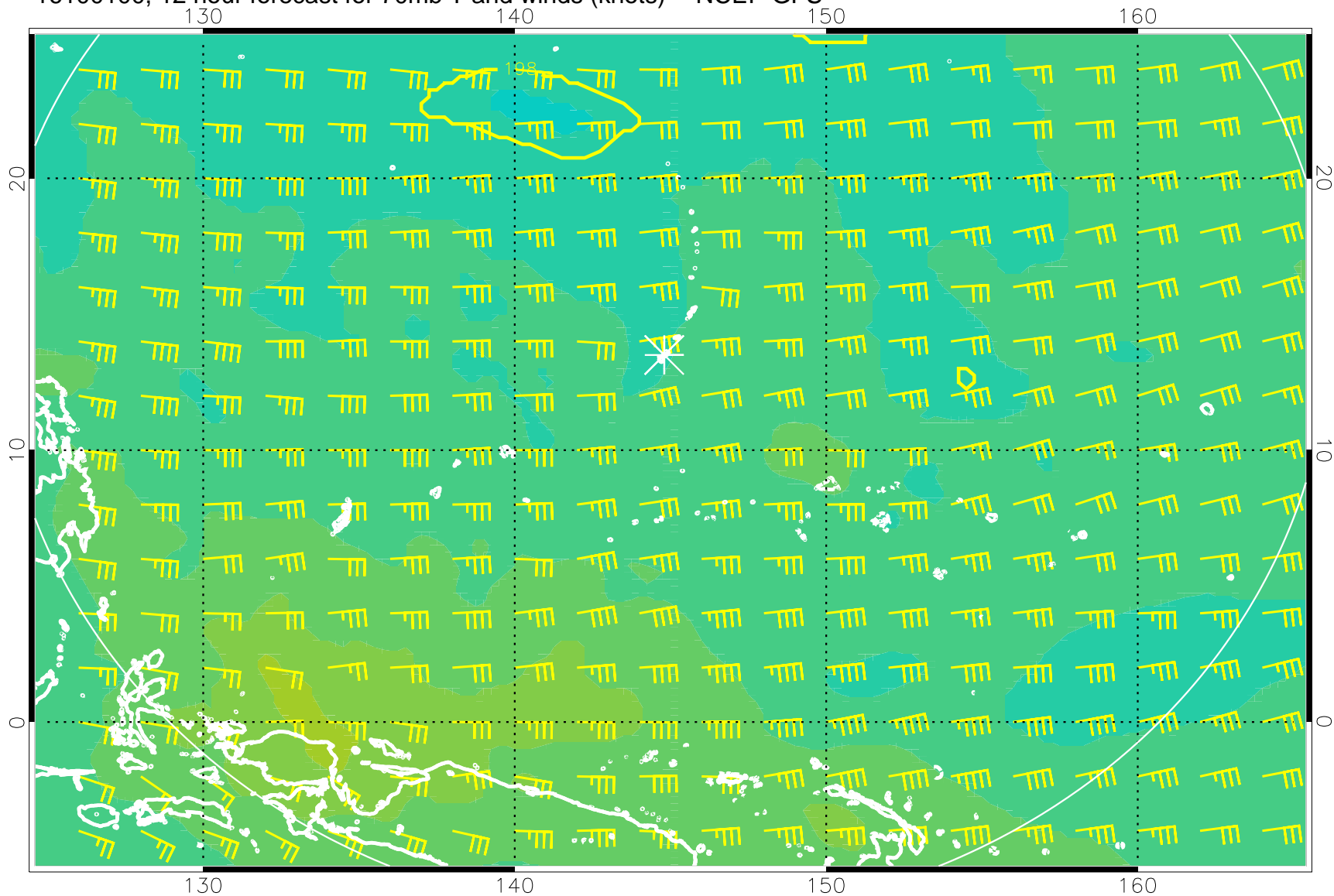
16100100, 12 hour forecast for 70mb T and winds (knots) -- NCEP GFS
