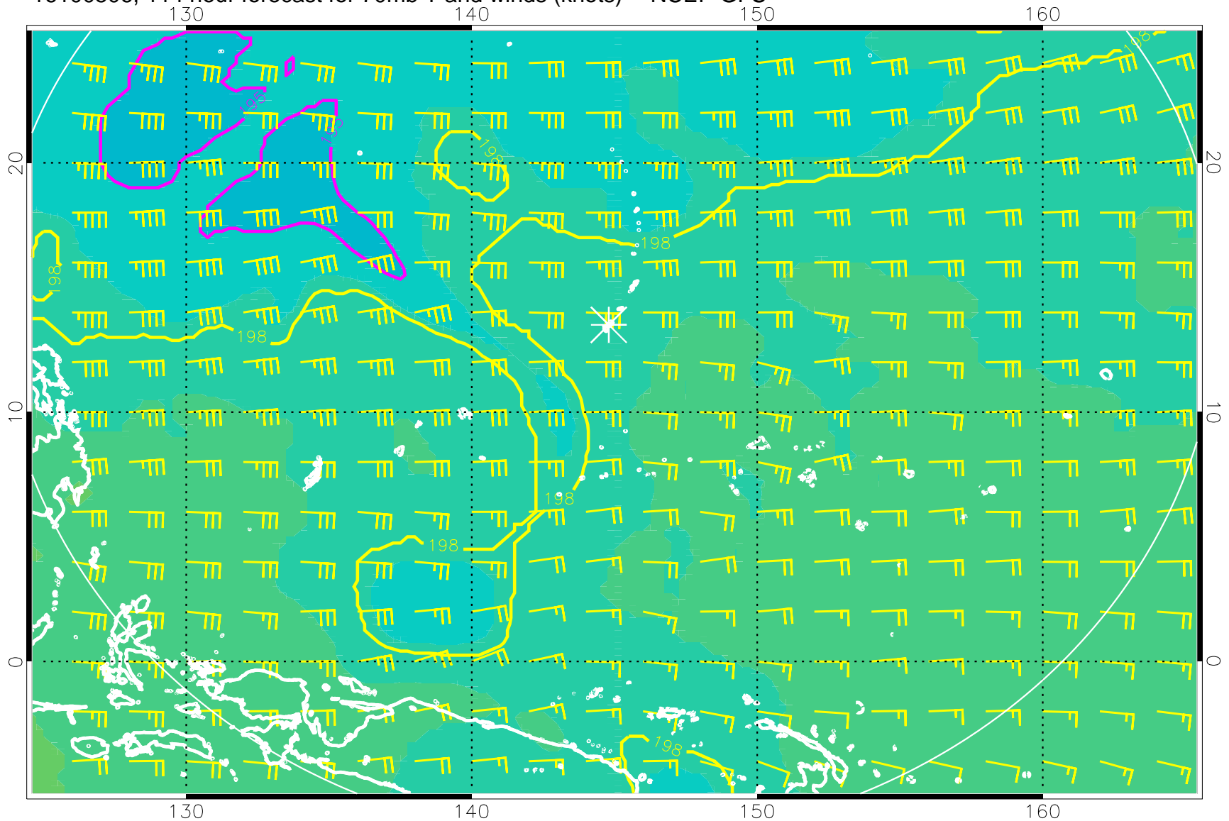
16100506, 114 hour forecast for 70mb T and winds (knots) -- NCEP GFS
