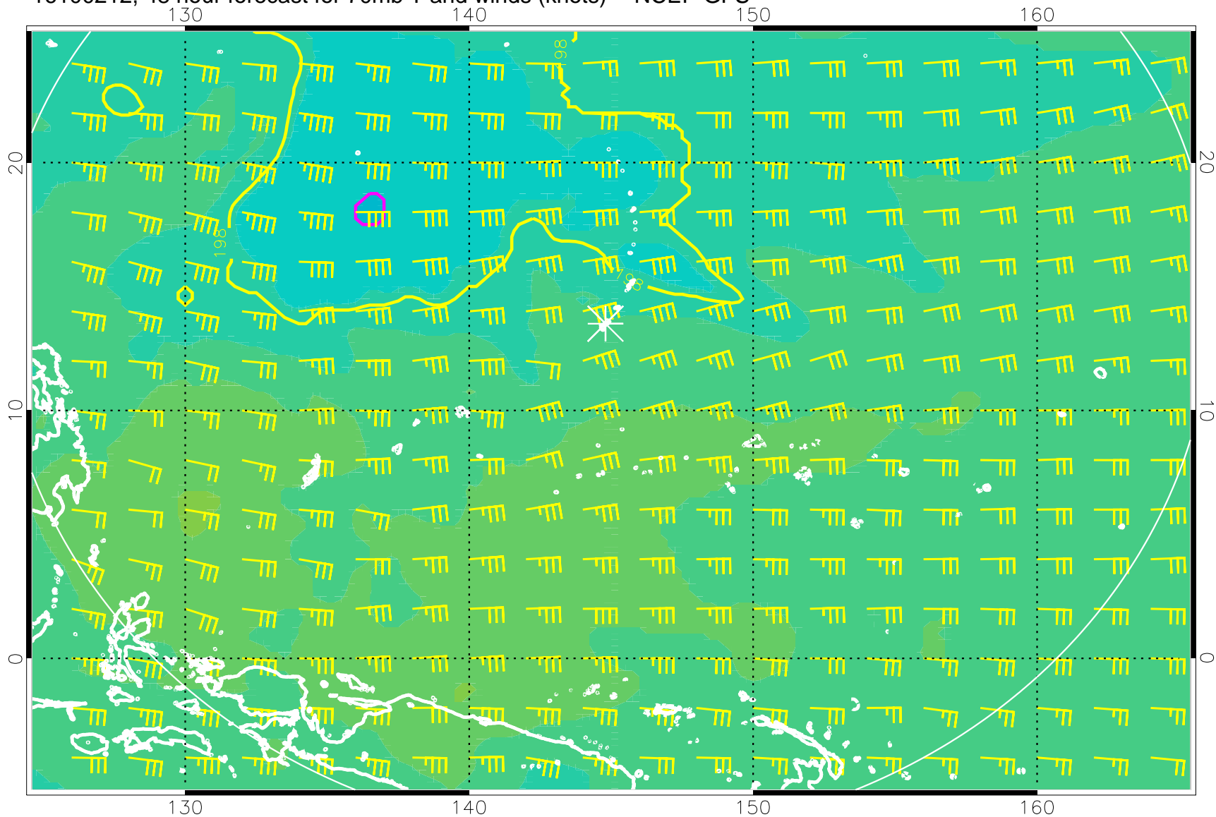
16100212, 48 hour forecast for 70mb T and winds (knots) -- NCEP GFS
