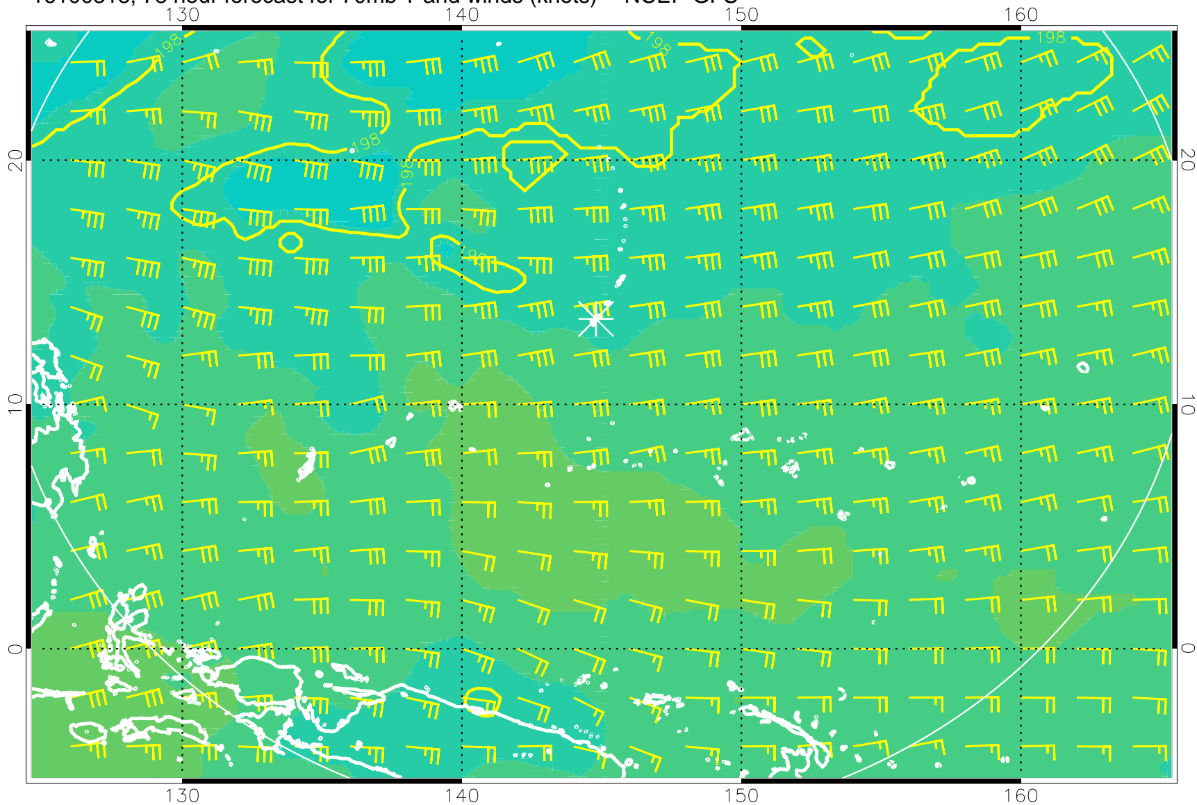
16100318, 78 hour forecast for 70mb T and winds (knots) -- NCEP GFS
