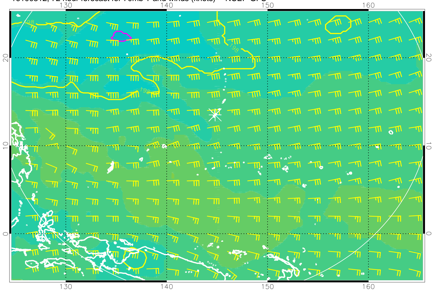
16100312, 72 hour forecast for 70mb T and winds (knots) -- NCEP GFS
