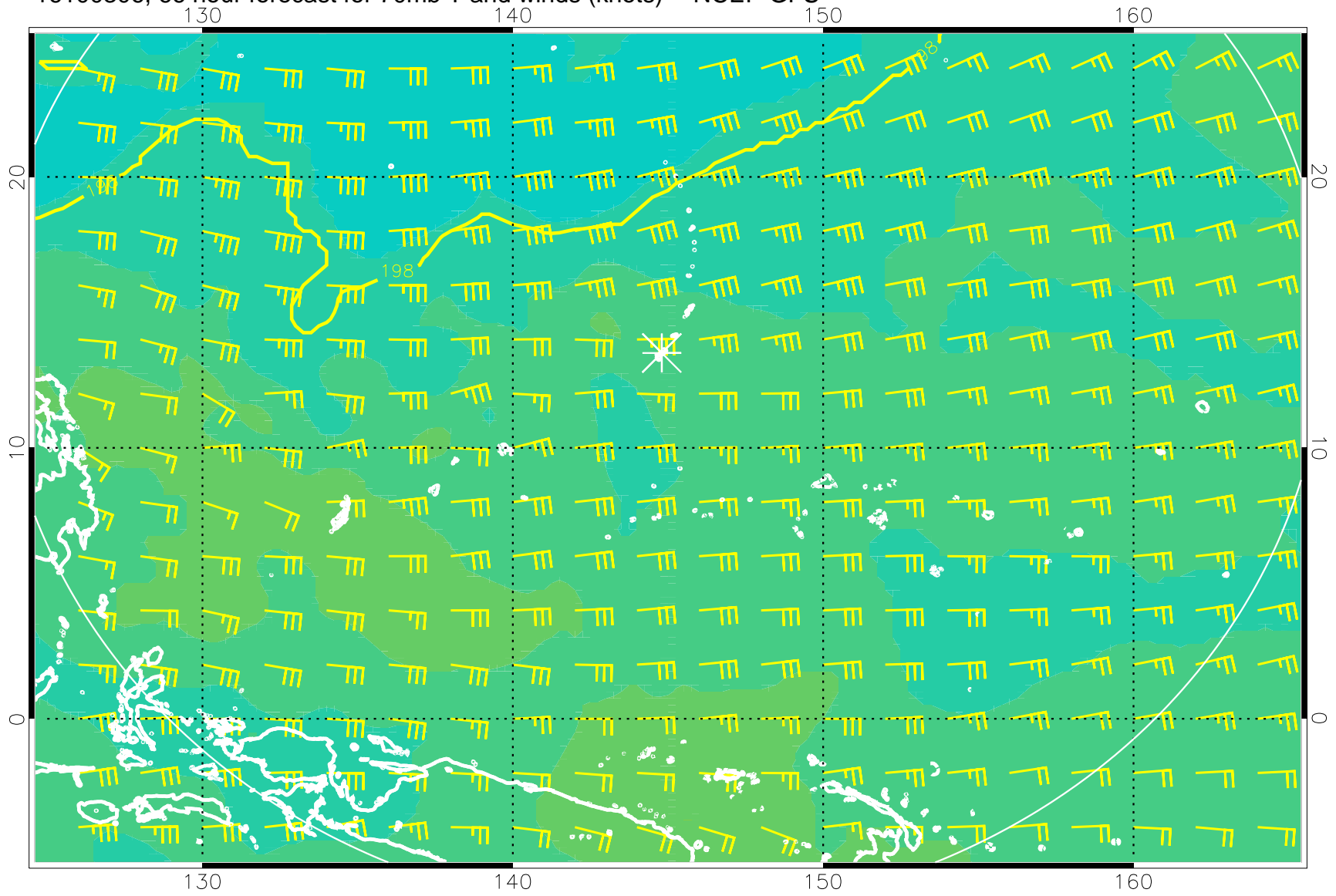
16100306, 66 hour forecast for 70mb T and winds (knots) -- NCEP GFS
