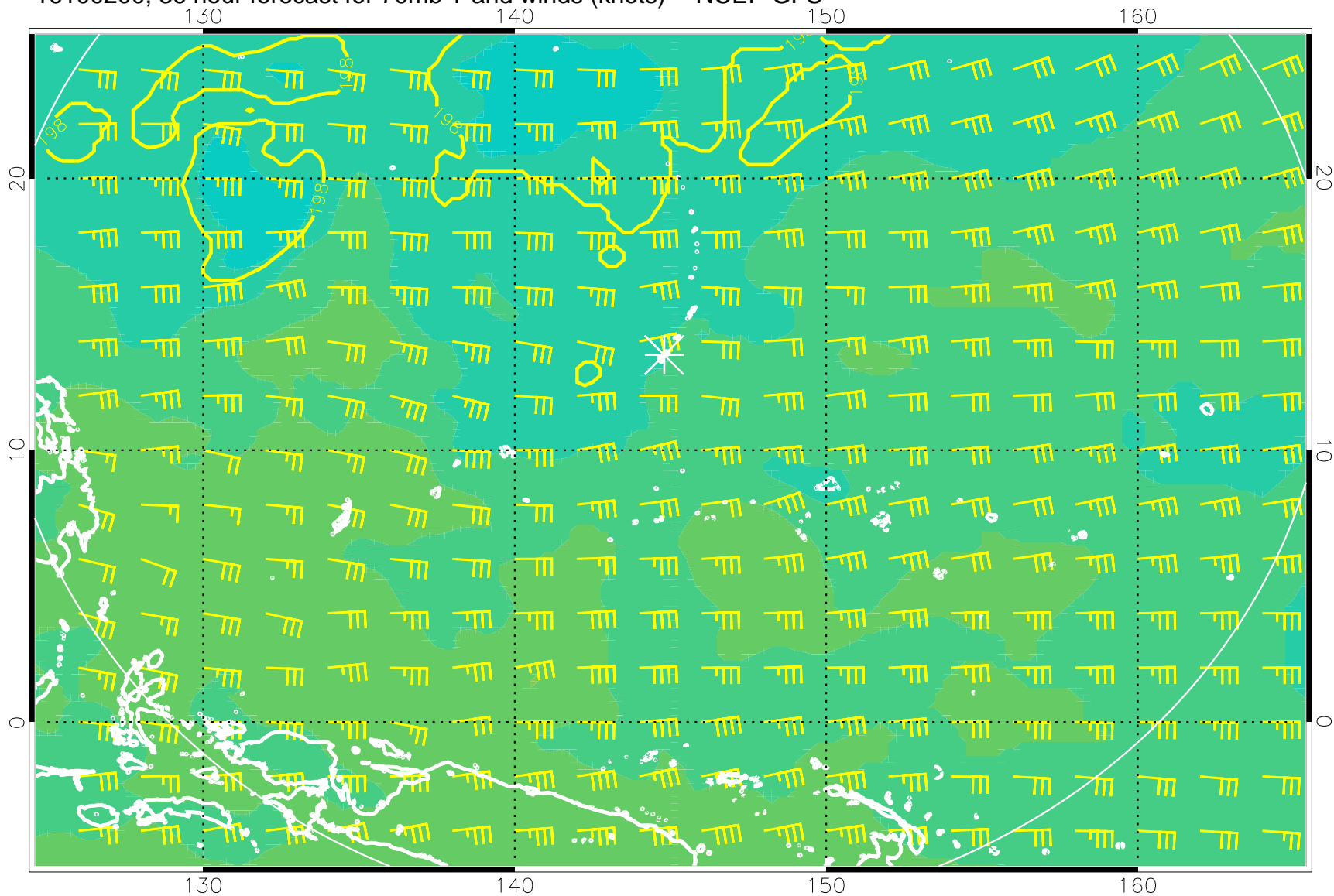
16100200, 36 hour forecast for 70mb T and winds (knots) -- NCEP GFS
