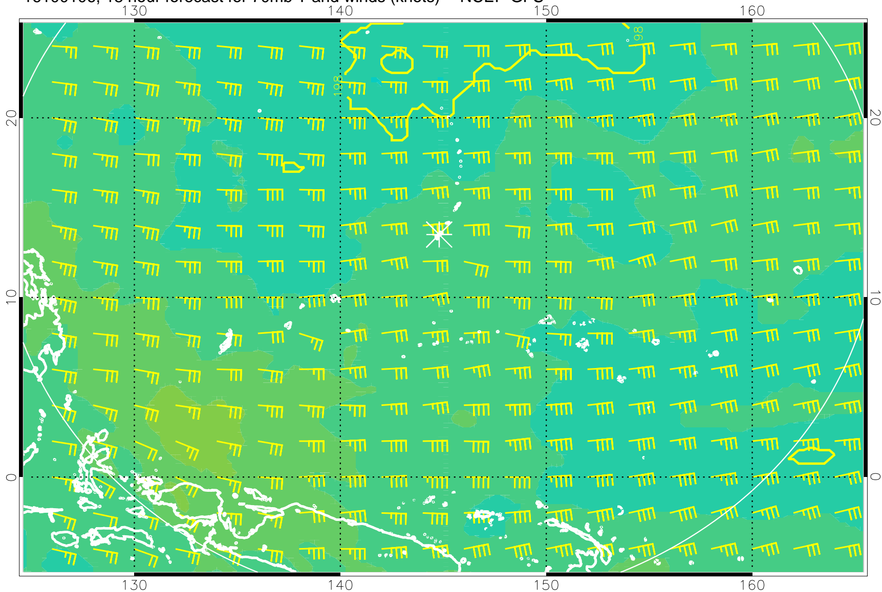
16100106, 18 hour forecast for 70mb T and winds (knots) -- NCEP GFS
