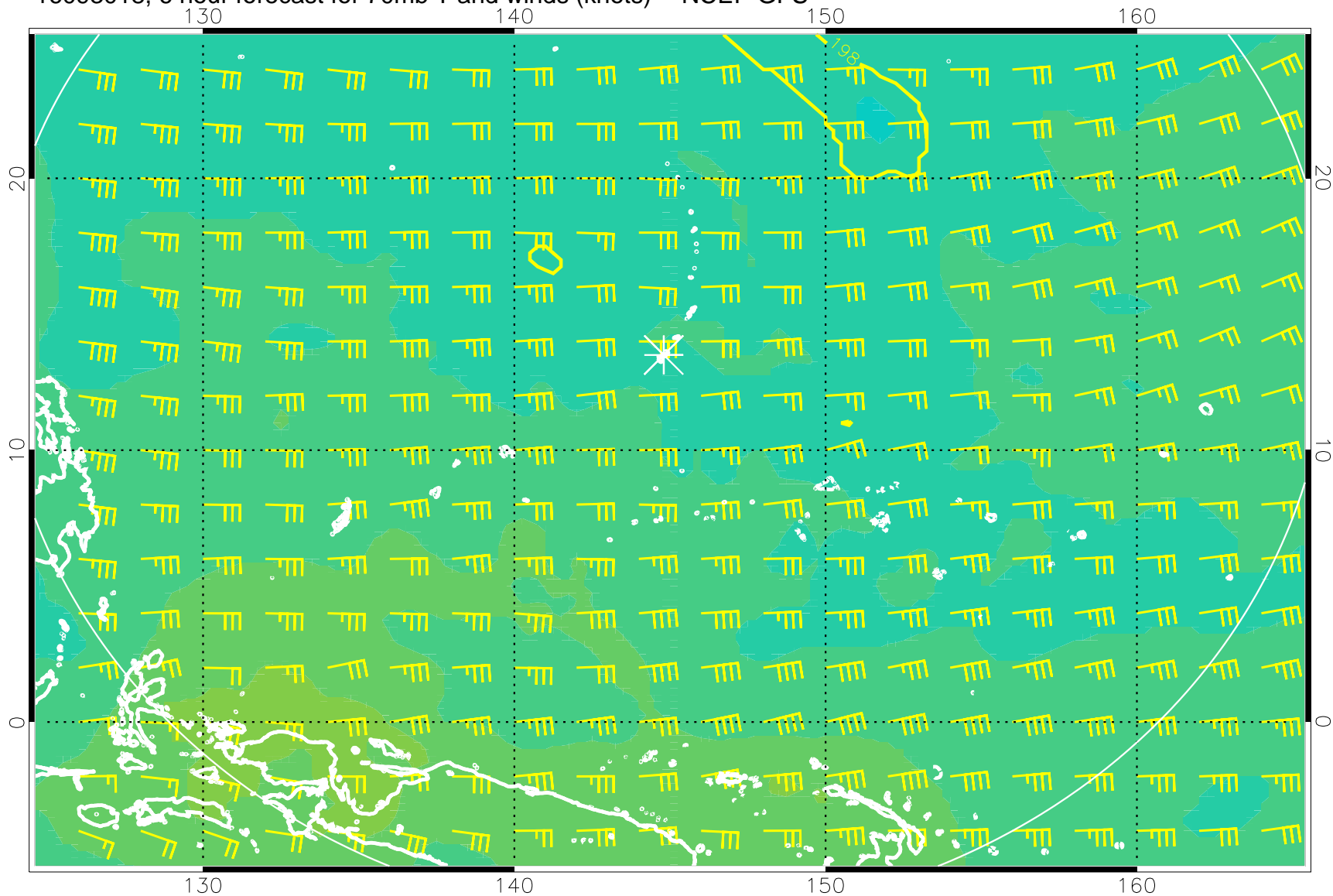
16093018, 6 hour forecast for 70mb T and winds (knots) -- NCEP GFS
