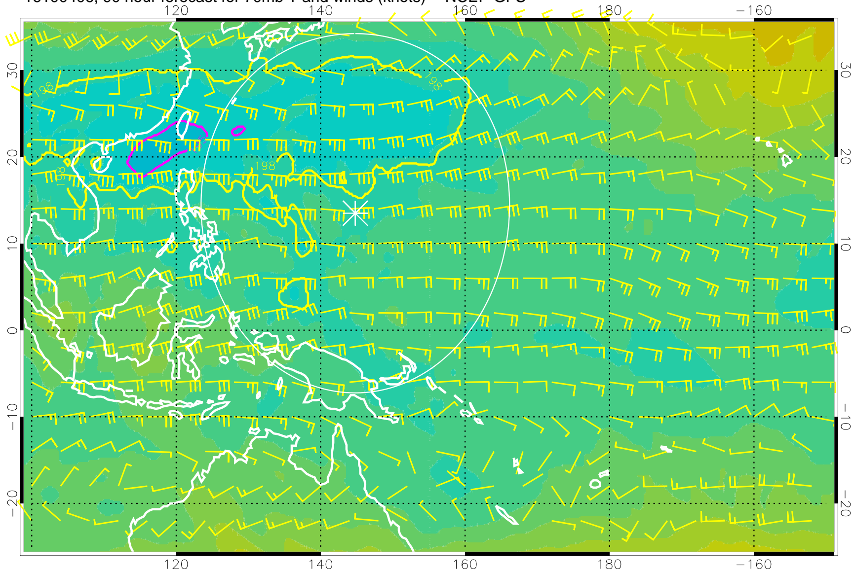
16100406, 90 hour forecast for 70mb T and winds (knots) -- NCEP GFS
