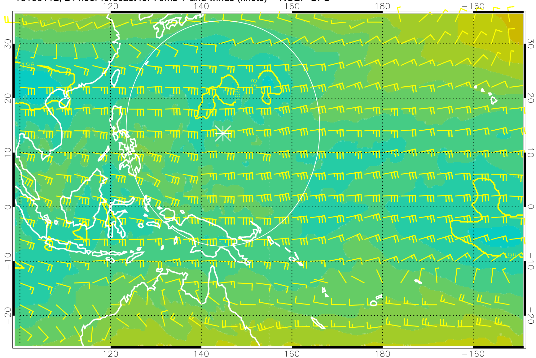
16100112, 24 hour forecast for 70mb T and winds (knots) -- NCEP GFS
