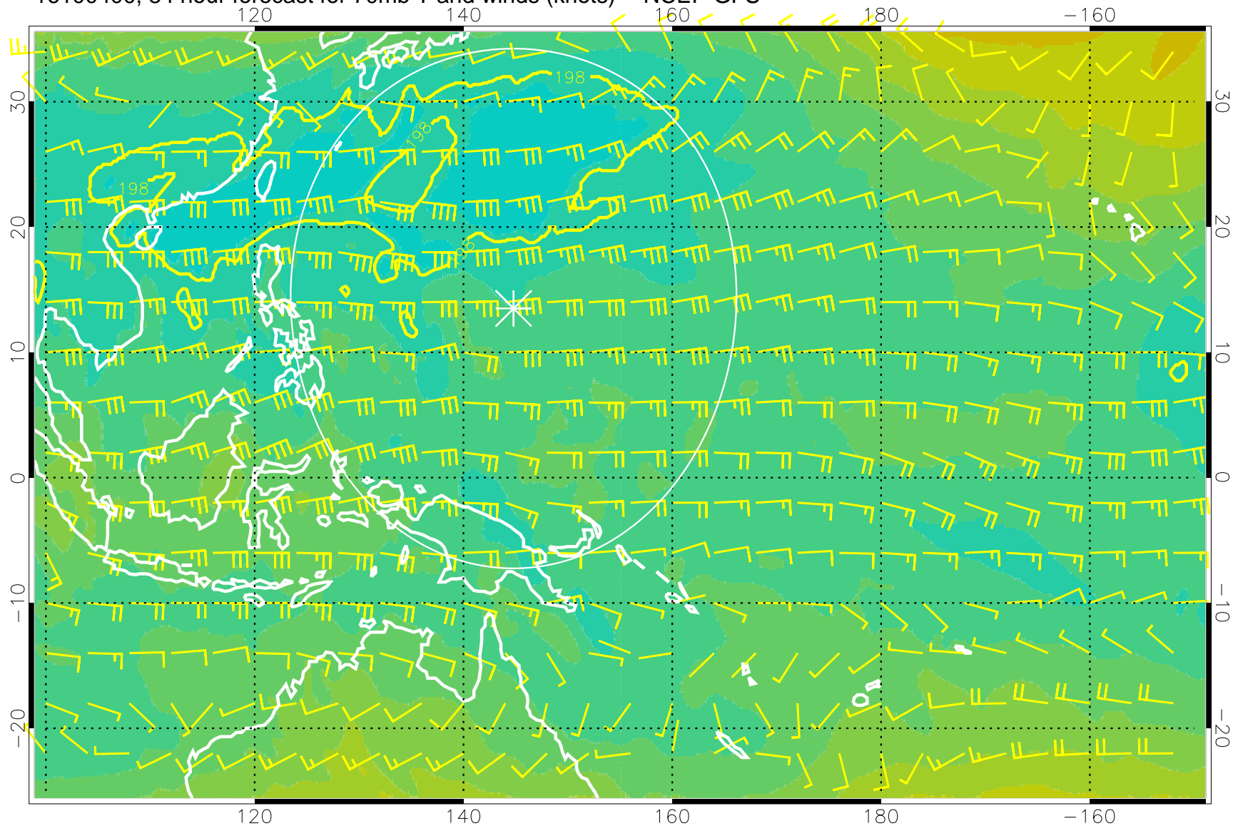
16100400, 84 hour forecast for 70mb T and winds (knots) -- NCEP GFS
