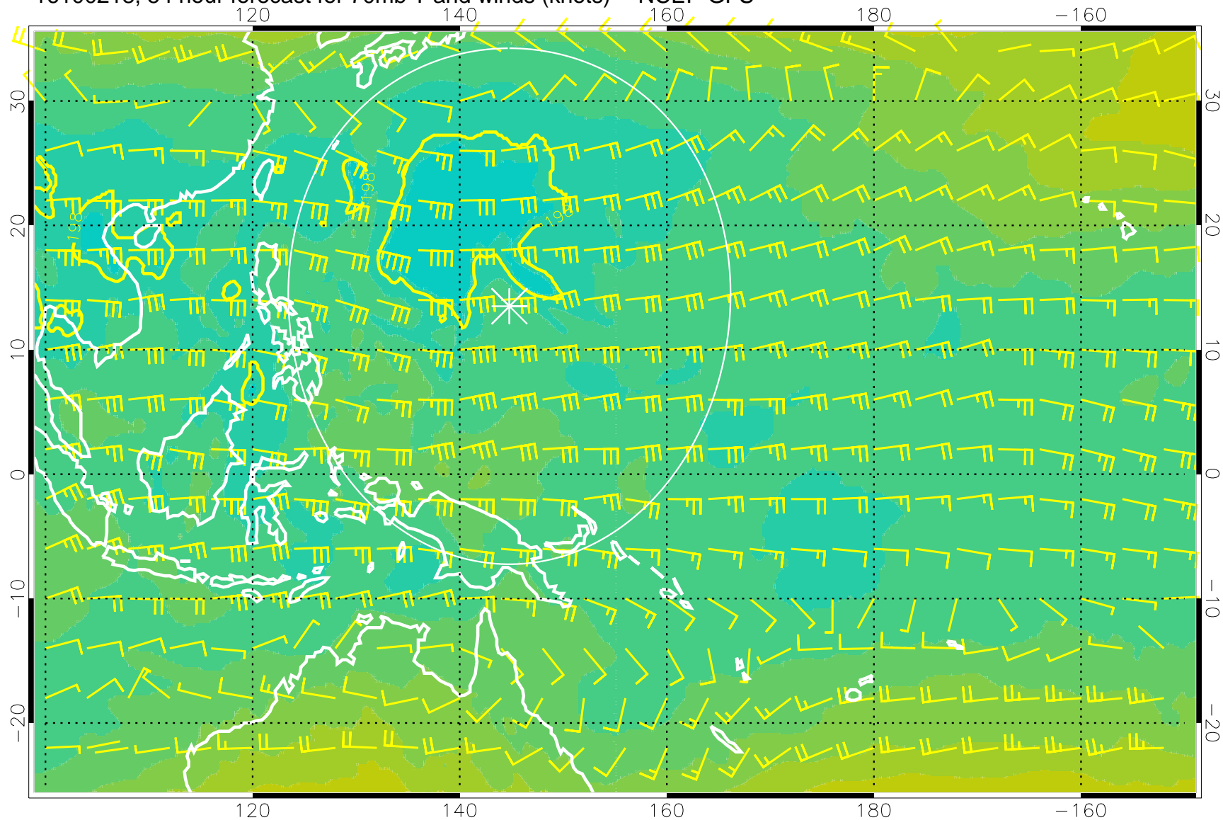
16100218, 54 hour forecast for 70mb T and winds (knots) -- NCEP GFS
