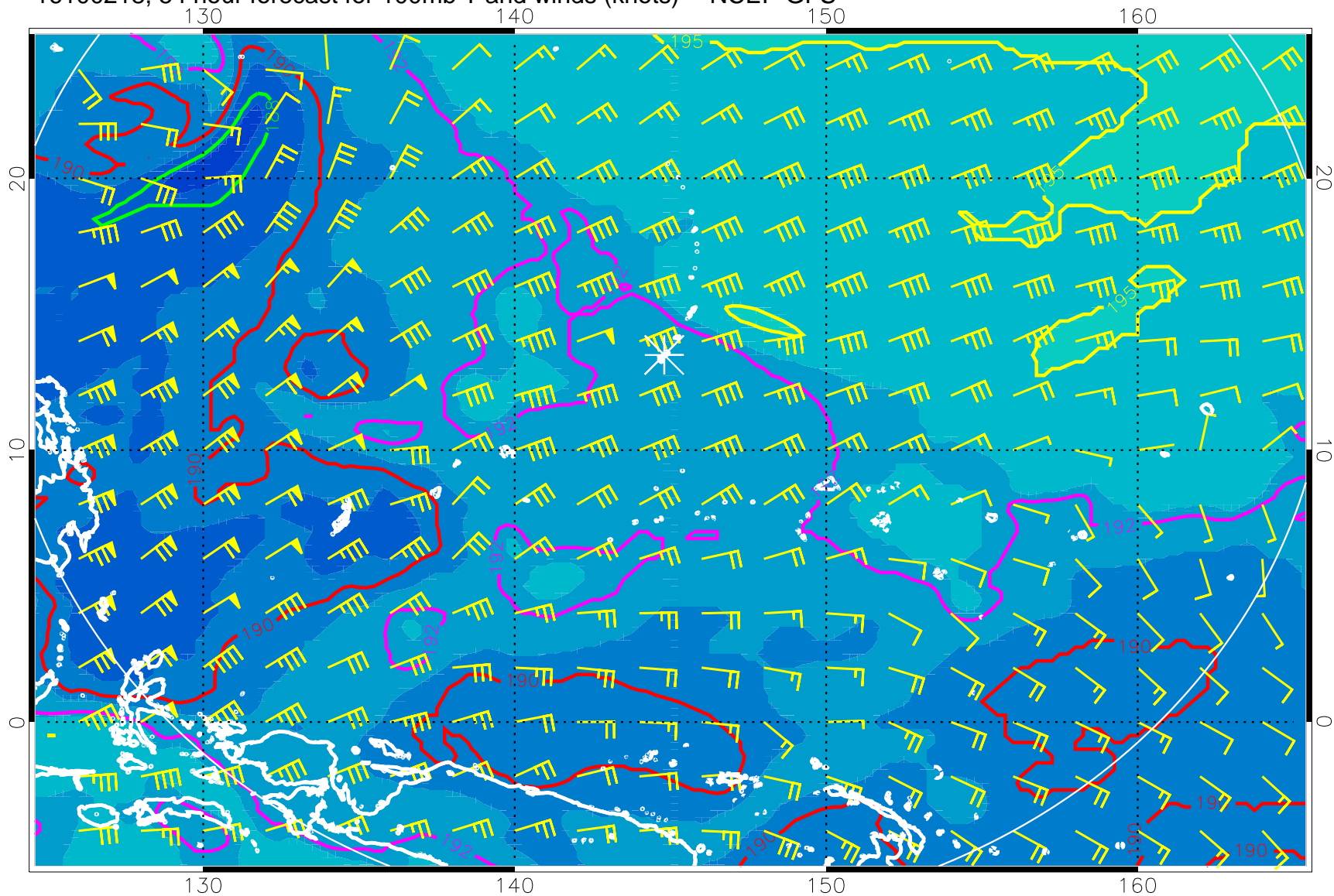
16100218, 54 hour forecast for 100mb T and winds (knots) -- NCEP GFS
