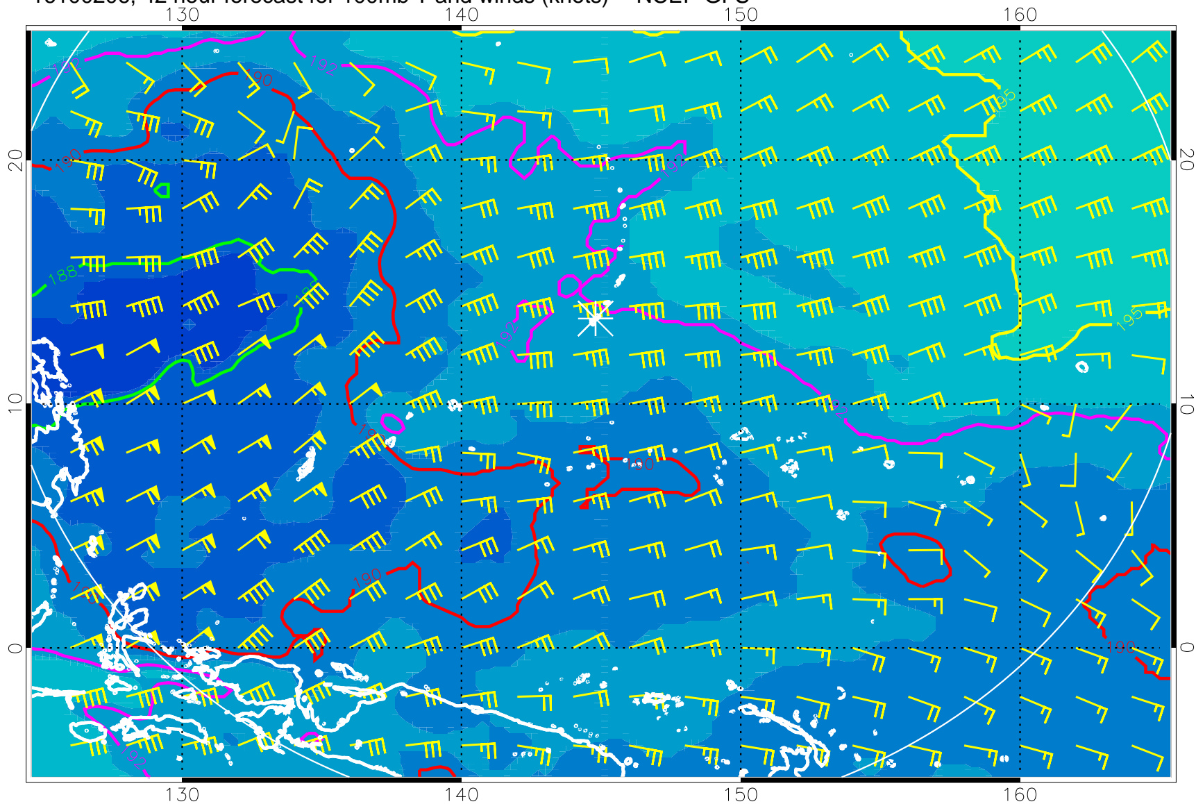
16100206, 42 hour forecast for 100mb T and winds (knots) -- NCEP GFS
