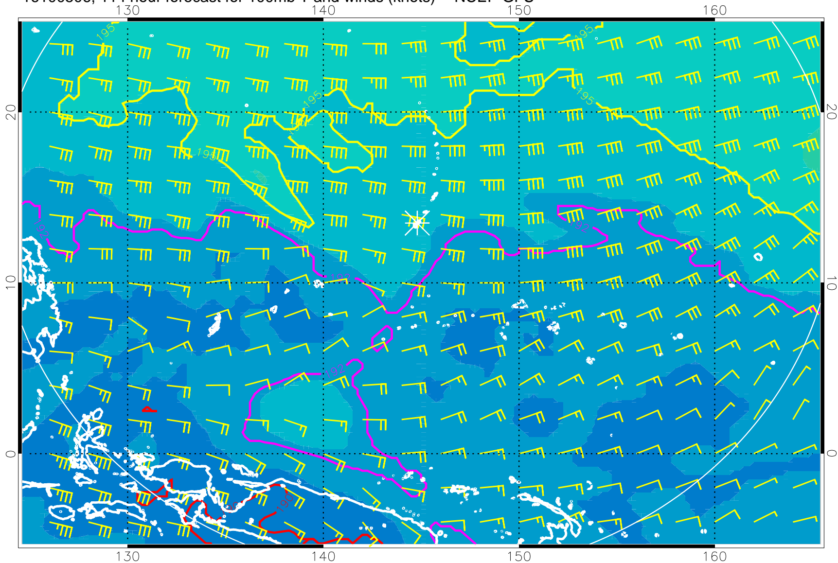
16100506, 114 hour forecast for 100mb T and winds (knots) -- NCEP GFS
