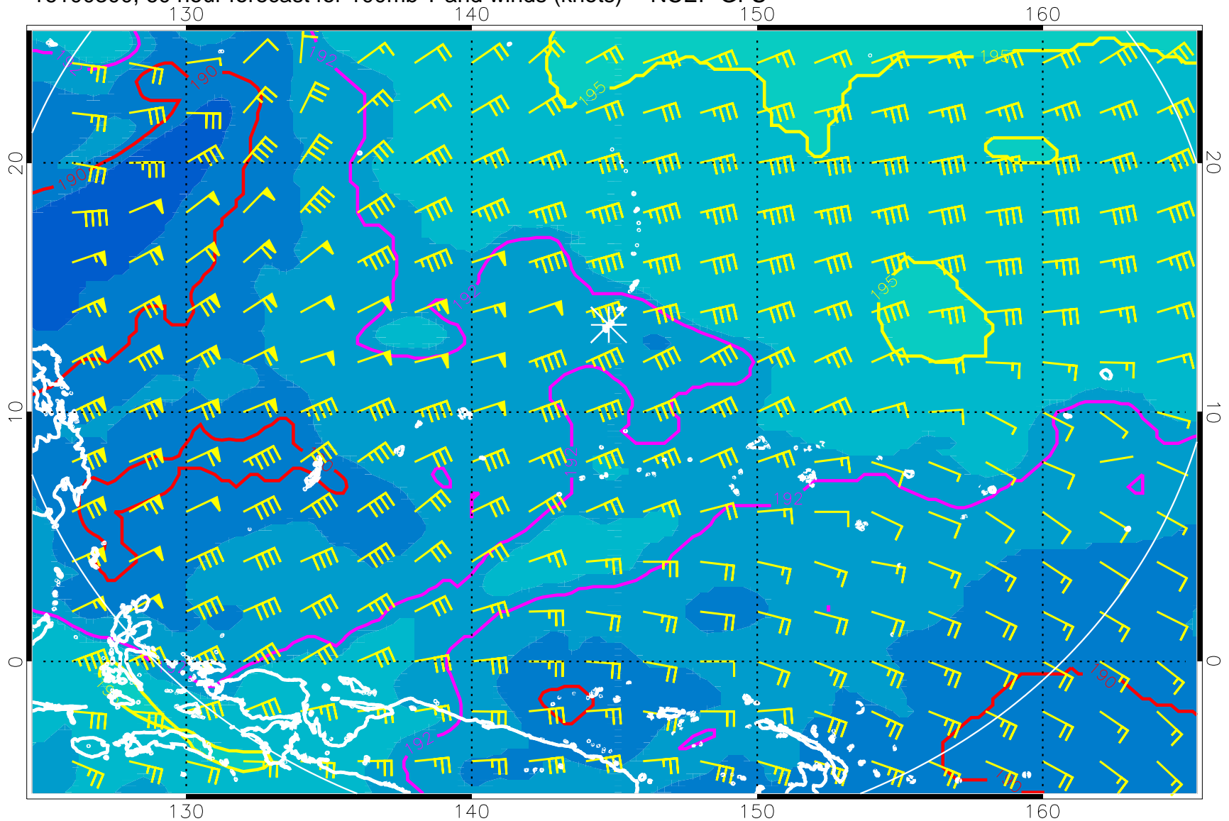
16100300, 60 hour forecast for 100mb T and winds (knots) -- NCEP GFS
