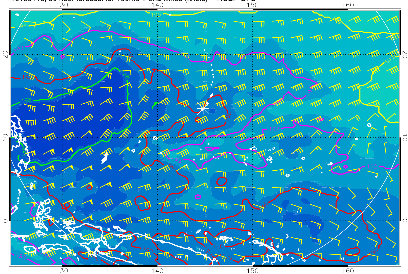
16100118, 30 hour forecast for 100mb T and winds (knots) -- NCEP GFS
