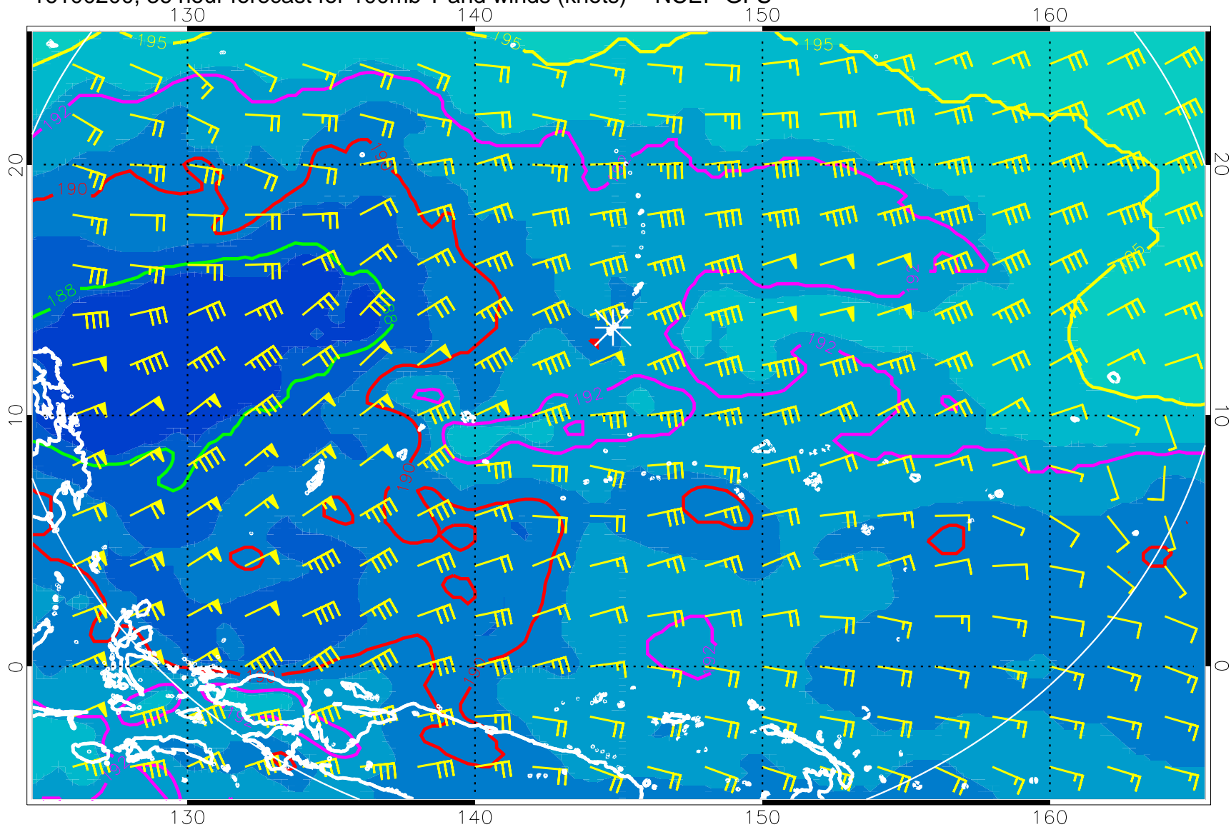
16100200, 36 hour forecast for 100mb T and winds (knots) -- NCEP GFS
