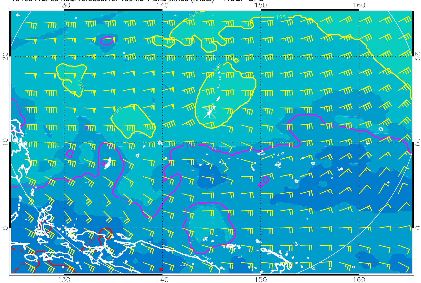
16100412, 96 hour forecast for 100mb T and winds (knots) -- NCEP GFS
