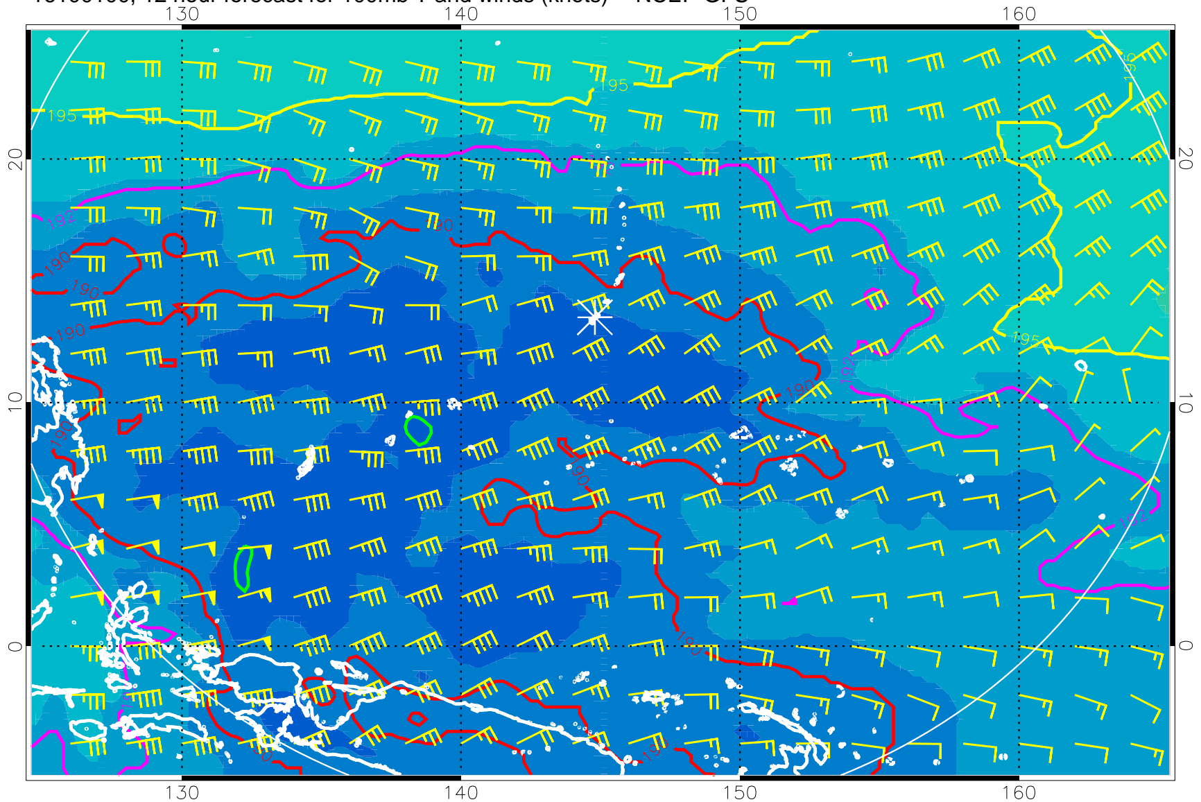
16100100, 12 hour forecast for 100mb T and winds (knots) -- NCEP GFS
