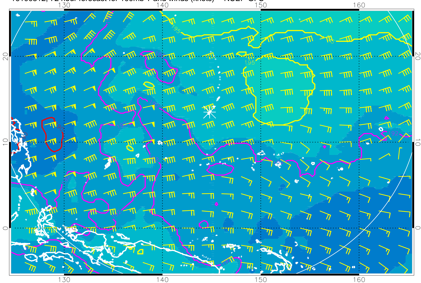
16100312, 72 hour forecast for 100mb T and winds (knots) -- NCEP GFS
