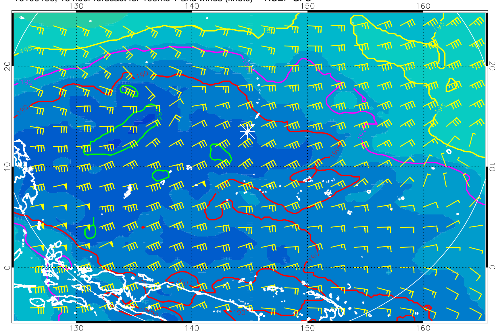
16100106, 18 hour forecast for 100mb T and winds (knots) -- NCEP GFS
