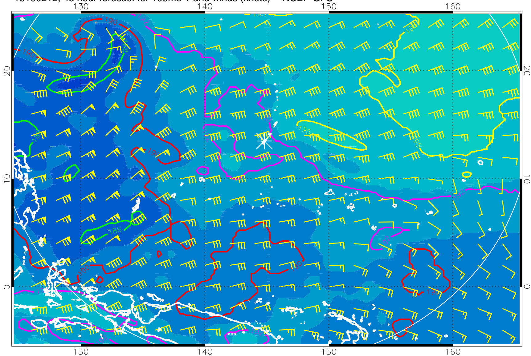
16100212, 48 hour forecast for 100mb T and winds (knots) -- NCEP GFS
