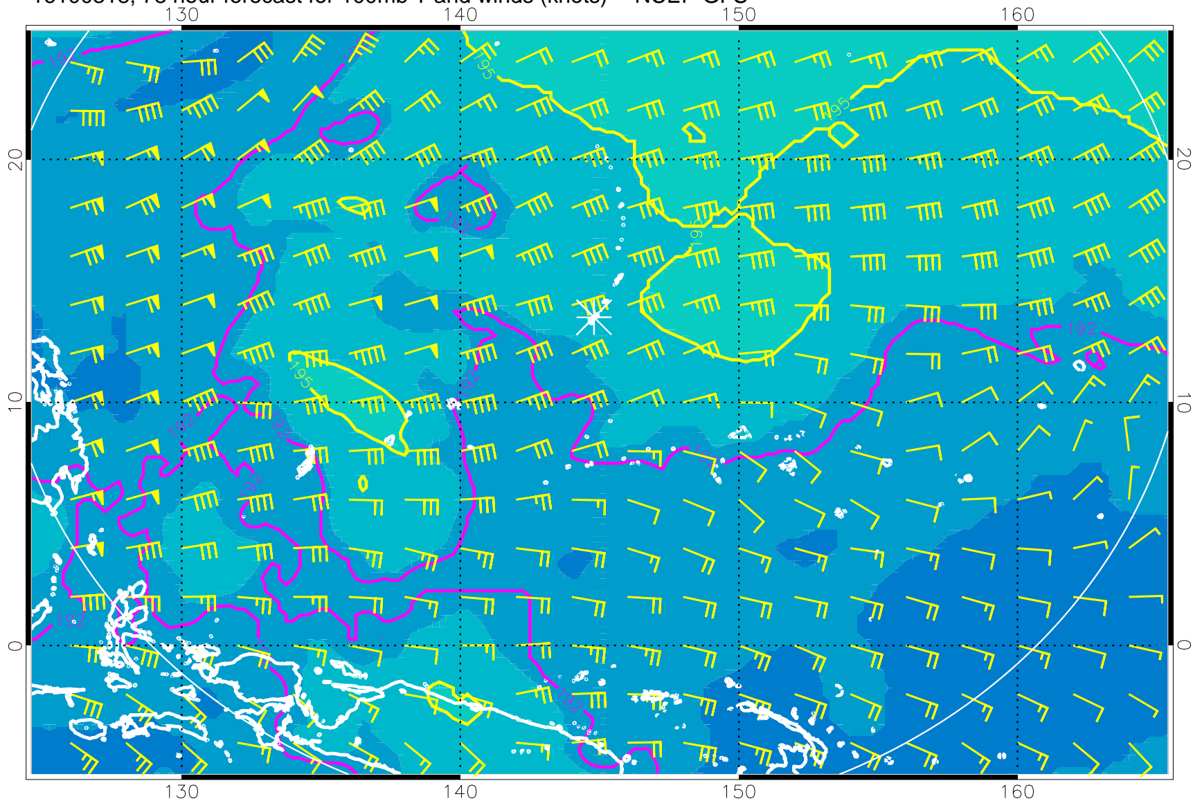
16100318, 78 hour forecast for 100mb T and winds (knots) -- NCEP GFS
