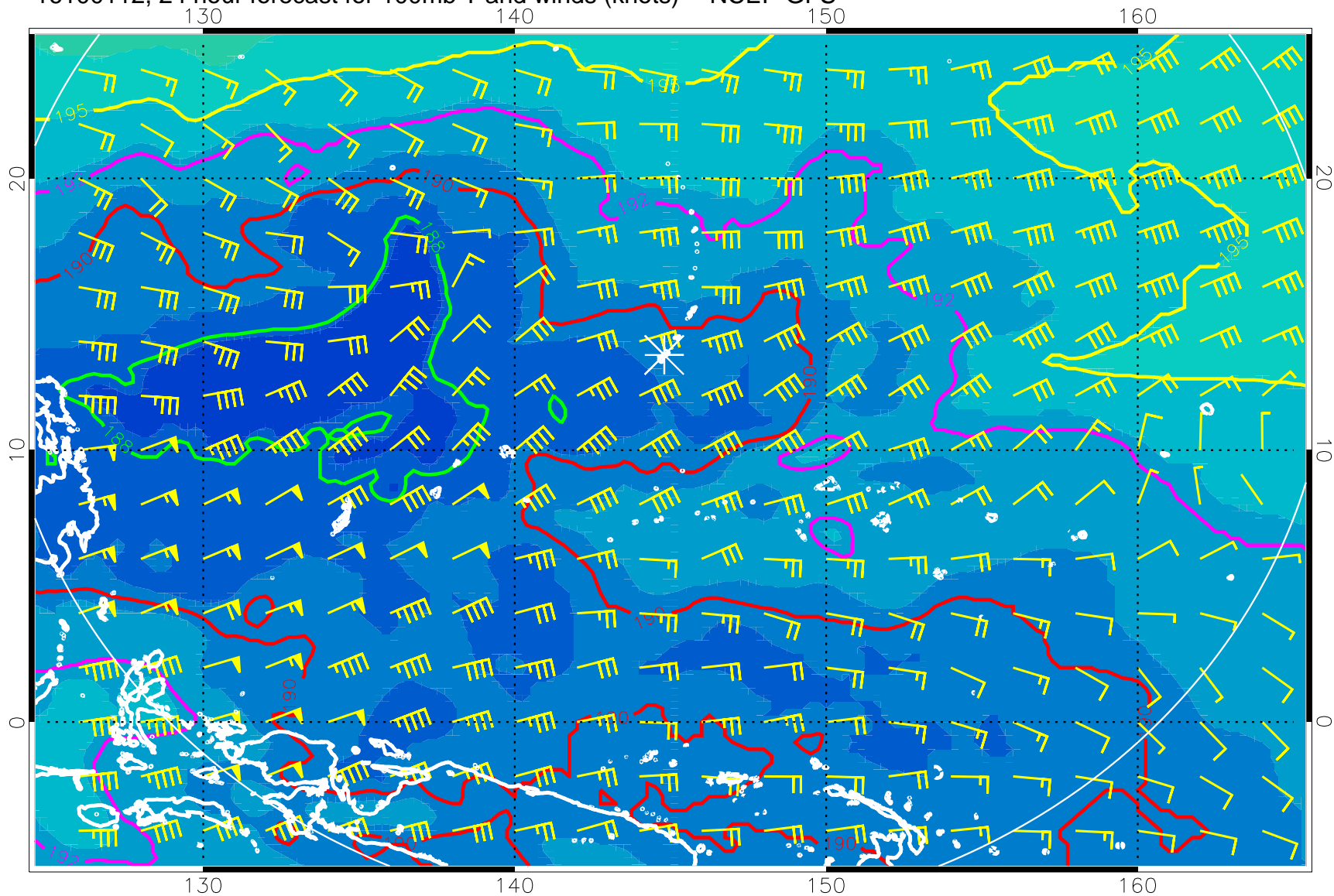
16100112, 24 hour forecast for 100mb T and winds (knots) -- NCEP GFS
