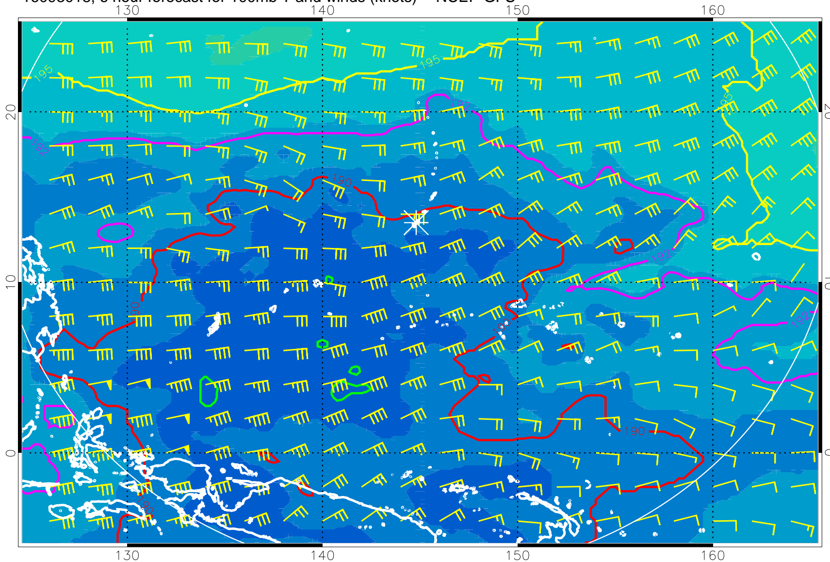
16093018, 6 hour forecast for 100mb T and winds (knots) -- NCEP GFS
