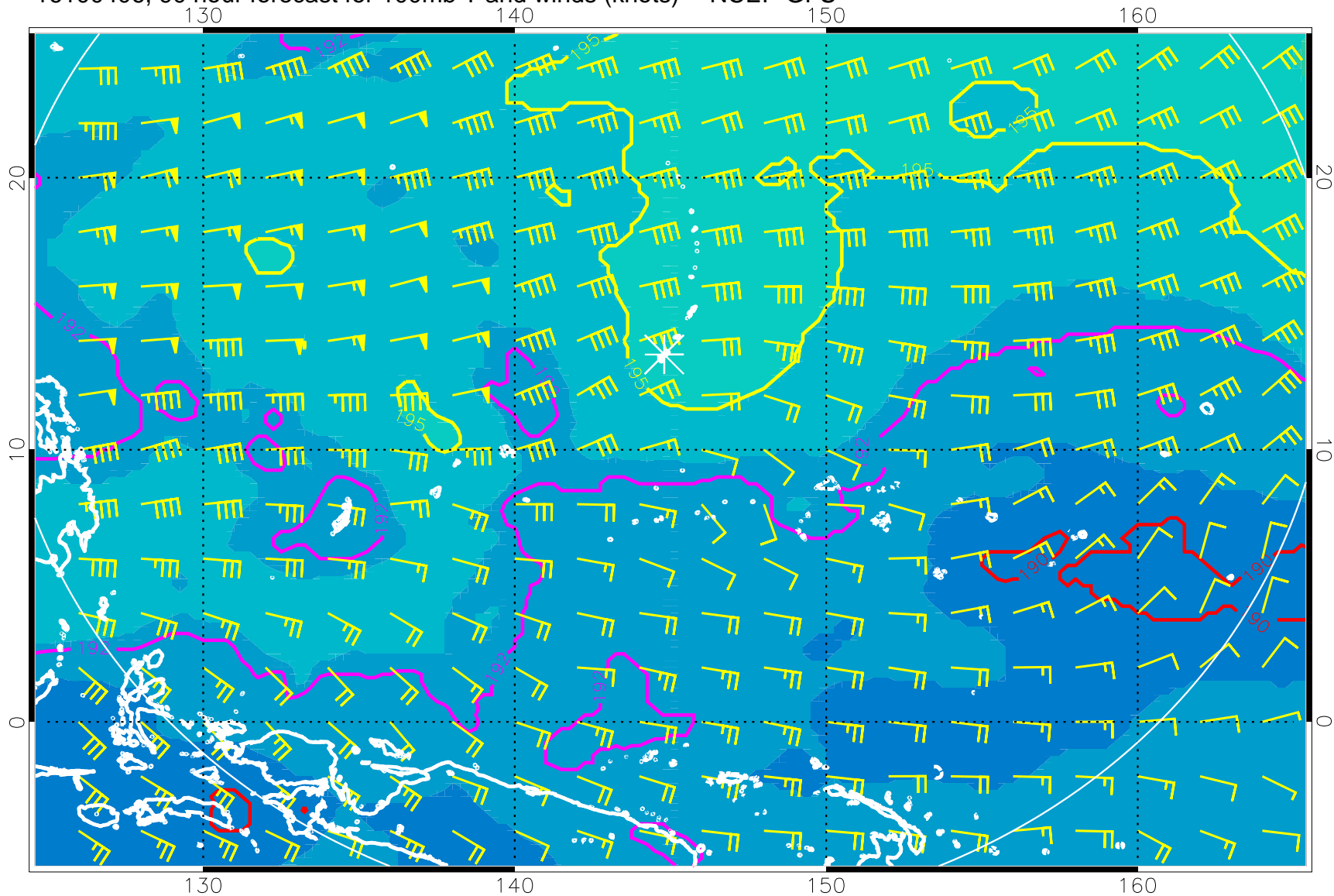
16100406, 90 hour forecast for 100mb T and winds (knots) -- NCEP GFS
