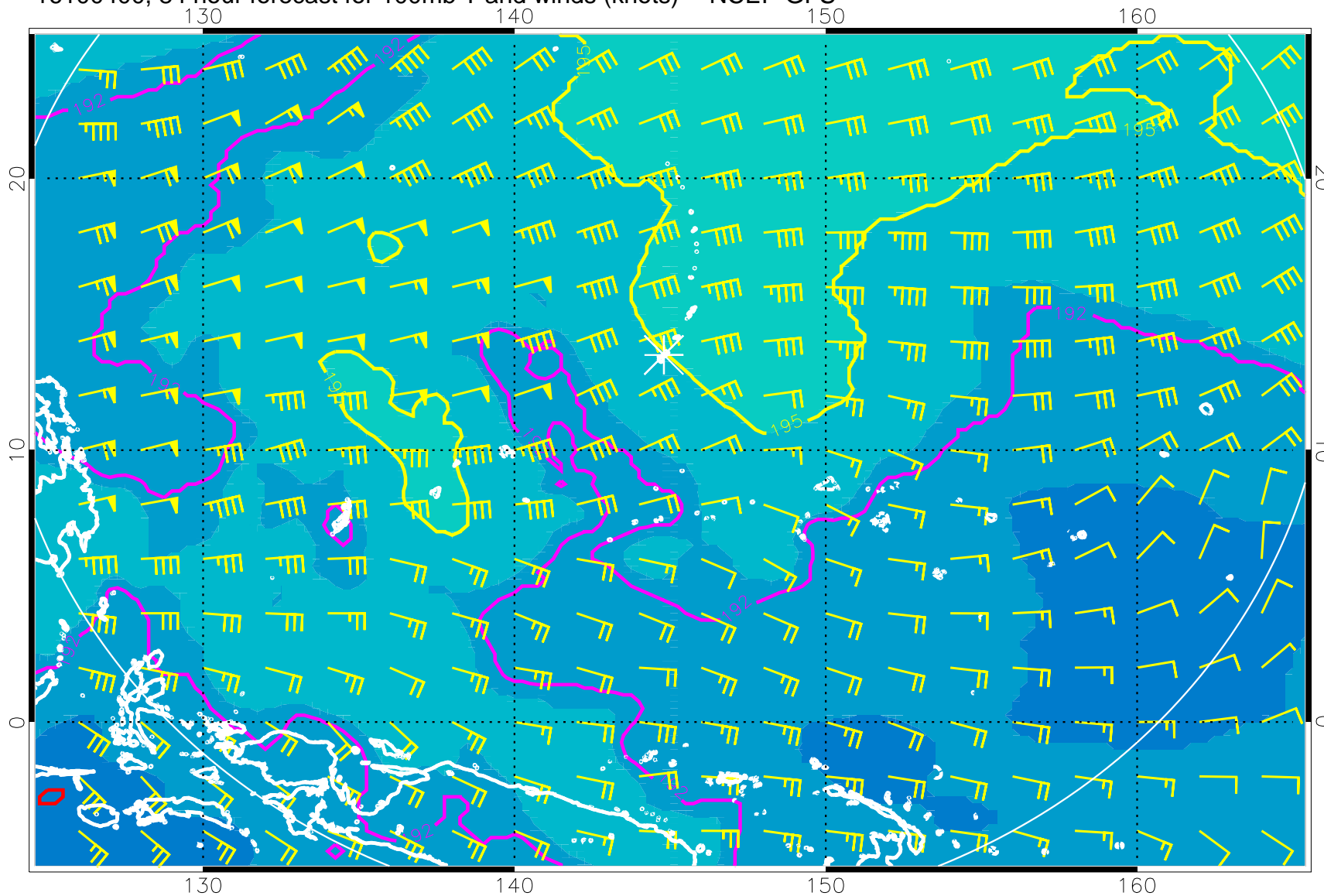
16100400, 84 hour forecast for 100mb T and winds (knots) -- NCEP GFS
