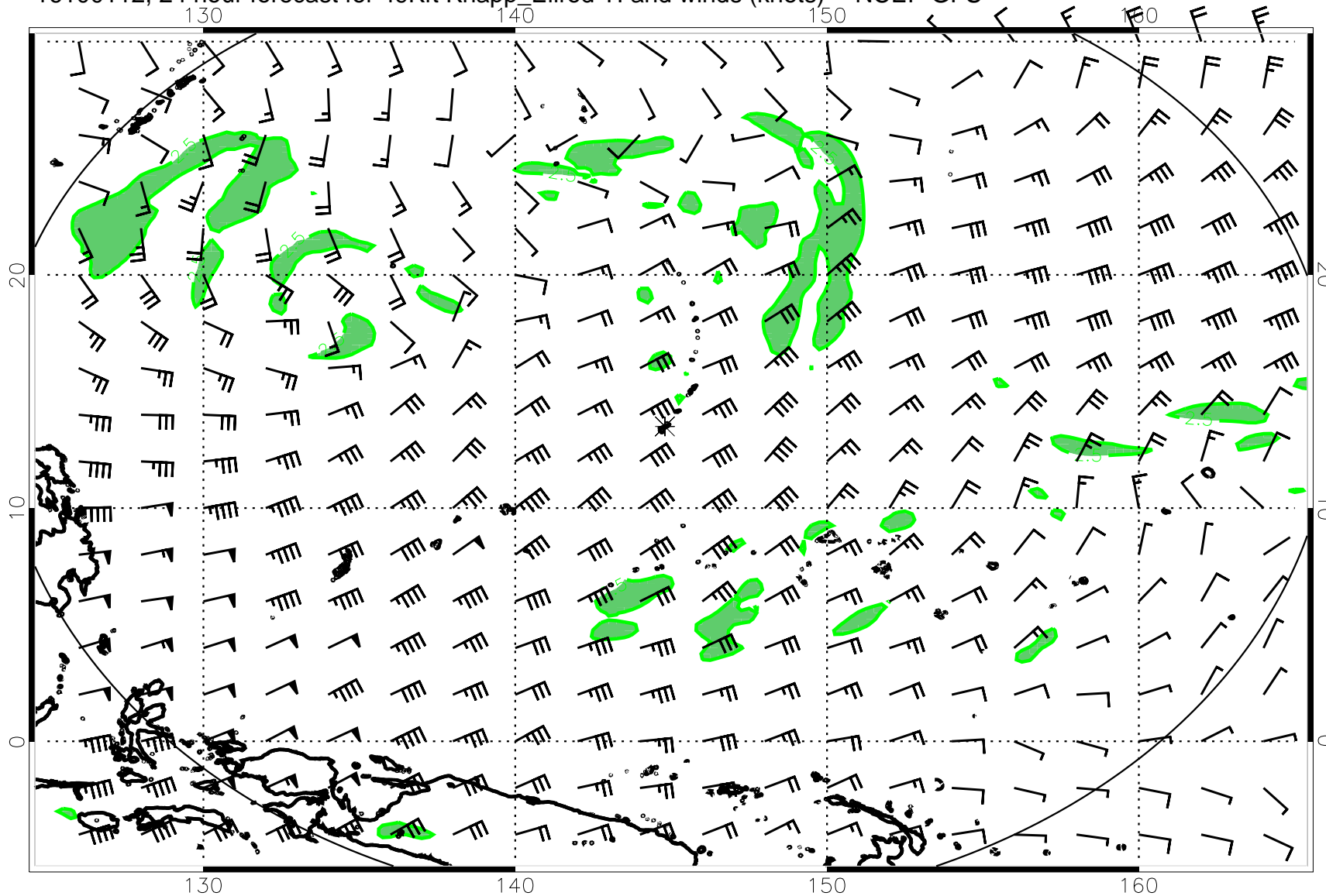
16100112, 24 hour forecast for 49Kft Knapp_Ellrod TI and winds (knots) -- NCEP GFS
