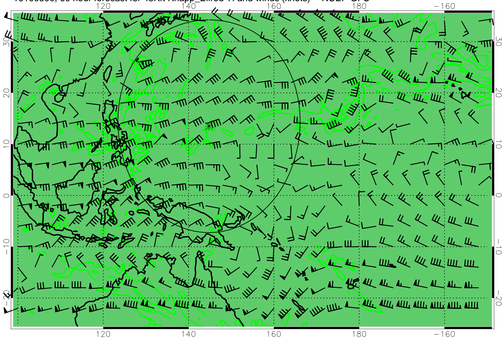
16100300, 60 hour forecast for 45Kft Knapp_Ellrod TI and winds (knots) -- NCEP GFS
