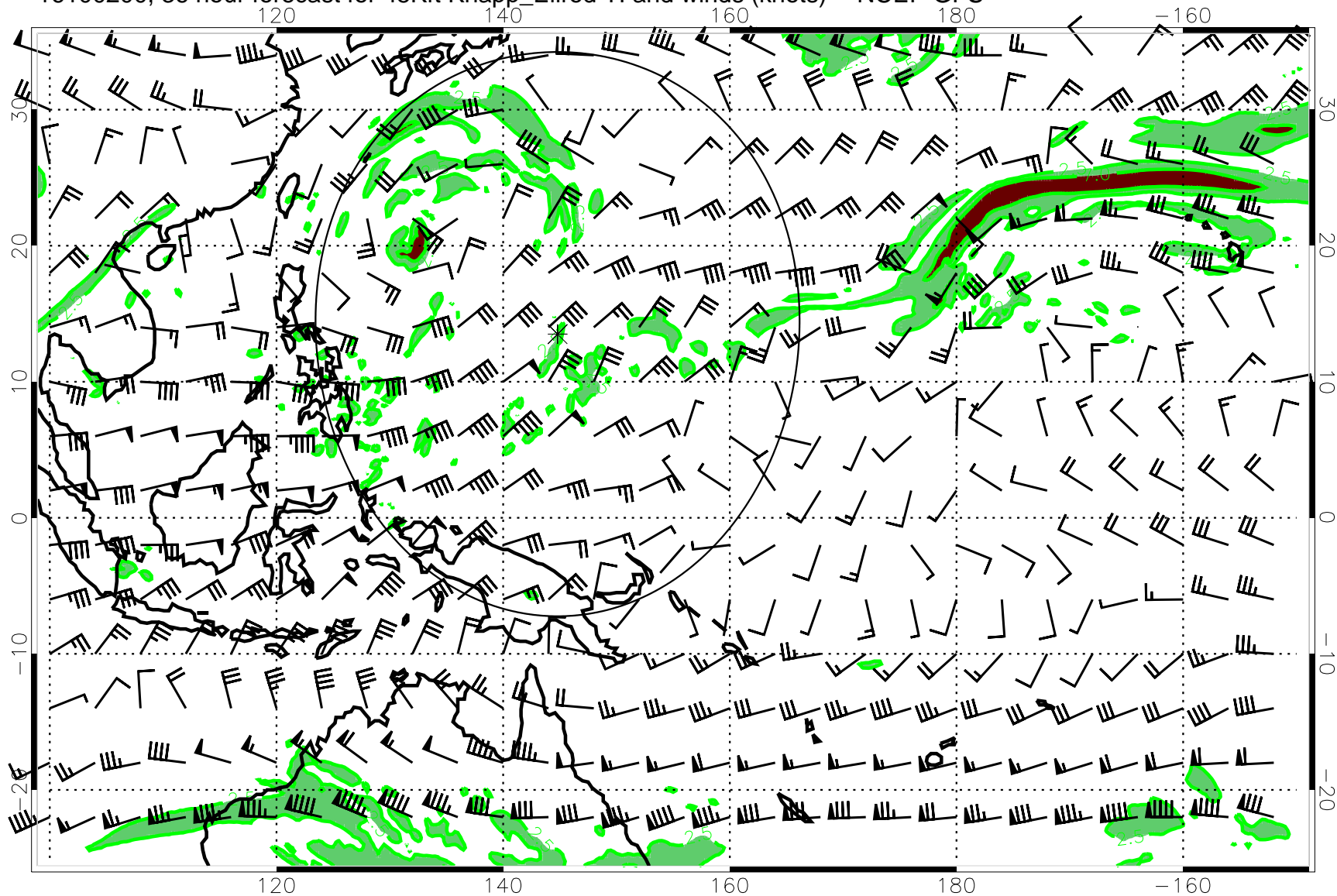
16100200, 36 hour forecast for 45Kft Knapp_Ellrod TI and winds (knots) -- NCEP GFS
