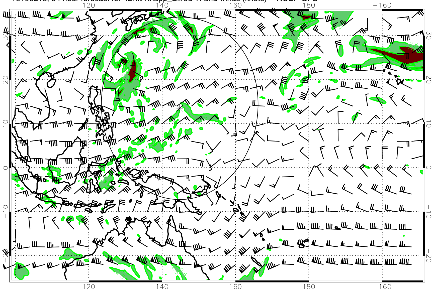
16100218, 54 hour forecast for 42Kft Knapp_Ellrod TI and winds (knots) -- NCEP GFS
