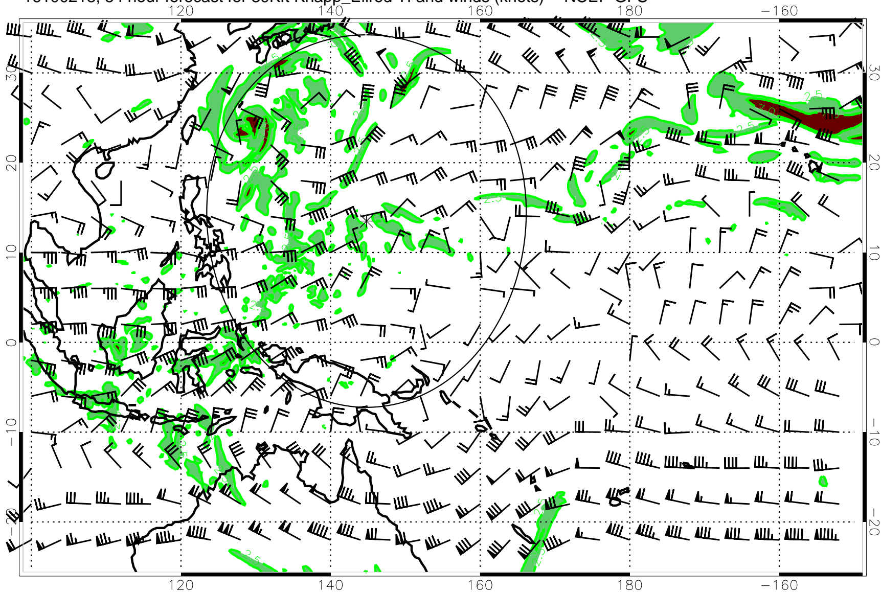
16100218, 54 hour forecast for 39Kft Knapp_Ellrod TI and winds (knots) -- NCEP GFS
