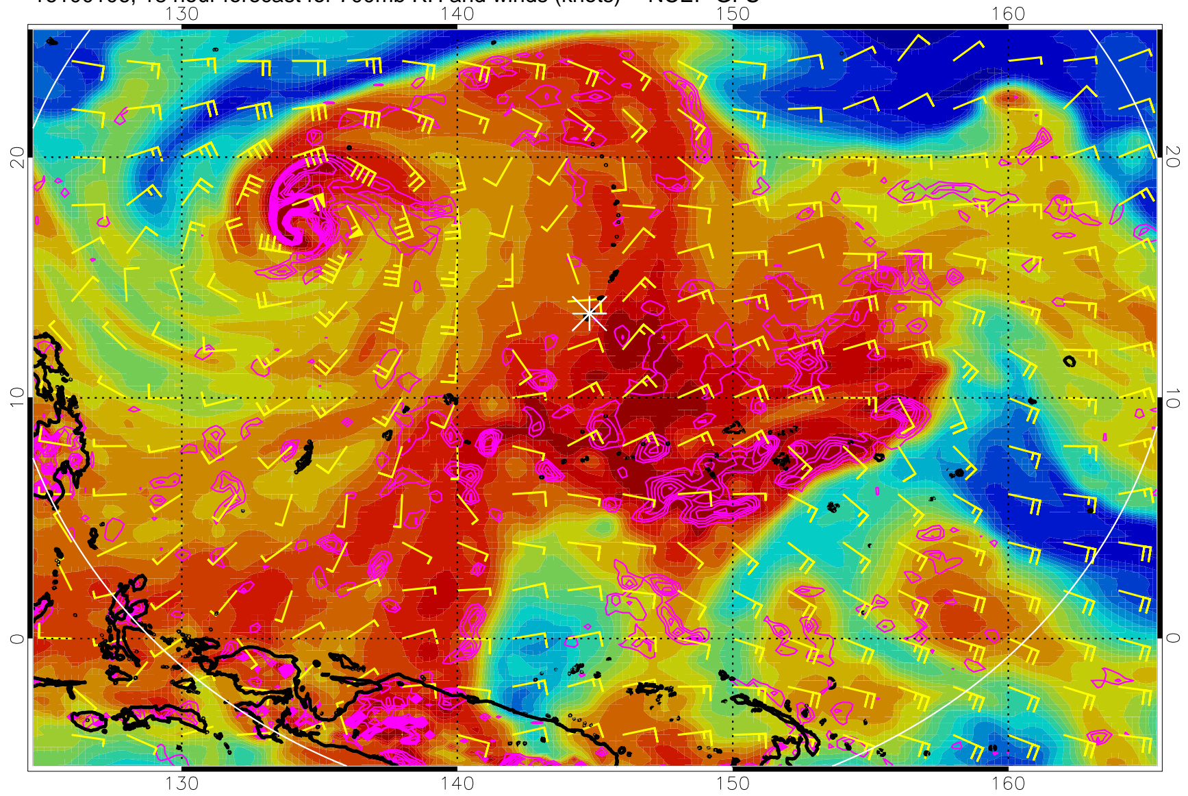
16100106, 18 hour forecast for 700mb RH and winds (knots) -- NCEP GFS
