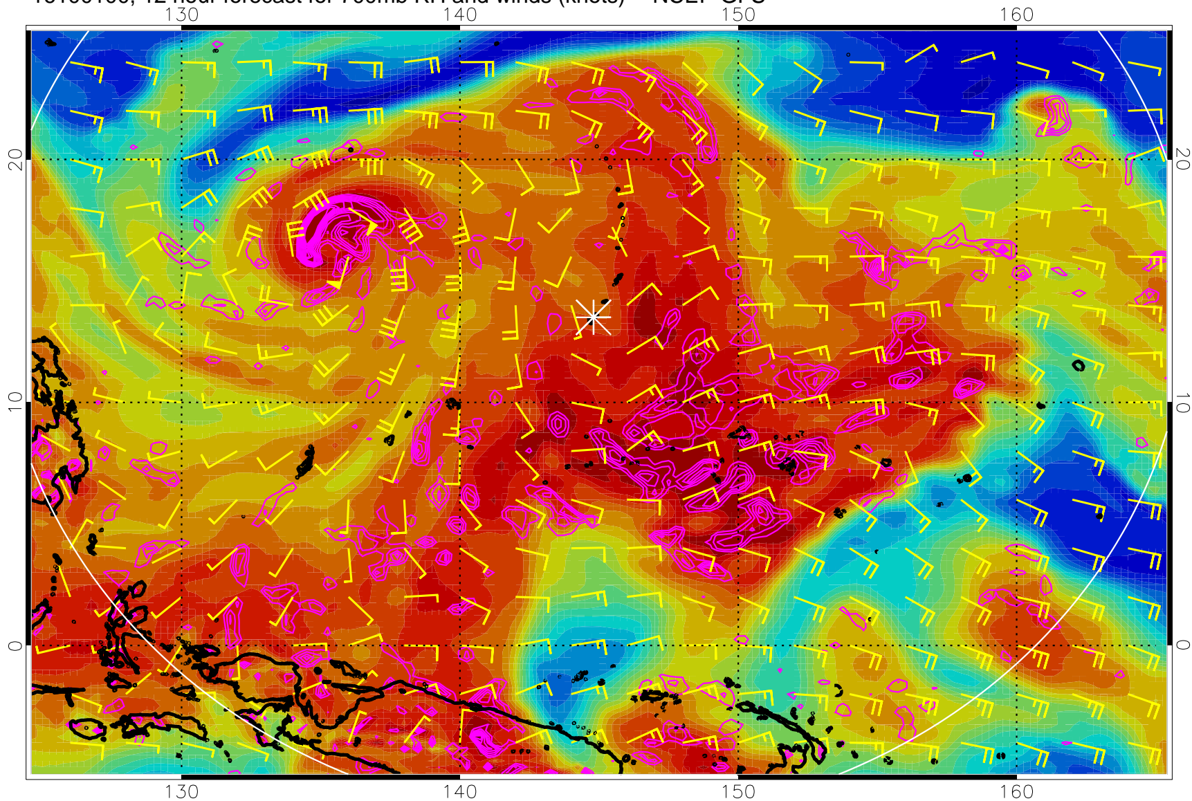
16100100, 12 hour forecast for 700mb RH and winds (knots) -- NCEP GFS
