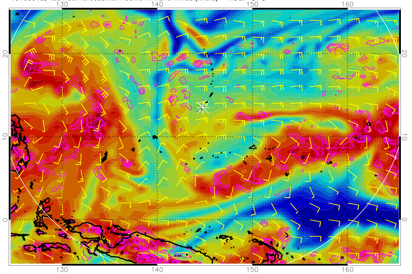
16100512, 120 hour forecast for 700mb RH and winds (knots) -- NCEP GFS
