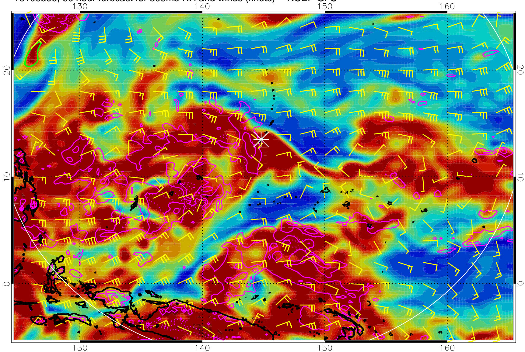
16100306, 66 hour forecast for 300mb RH and winds (knots) -- NCEP GFS
