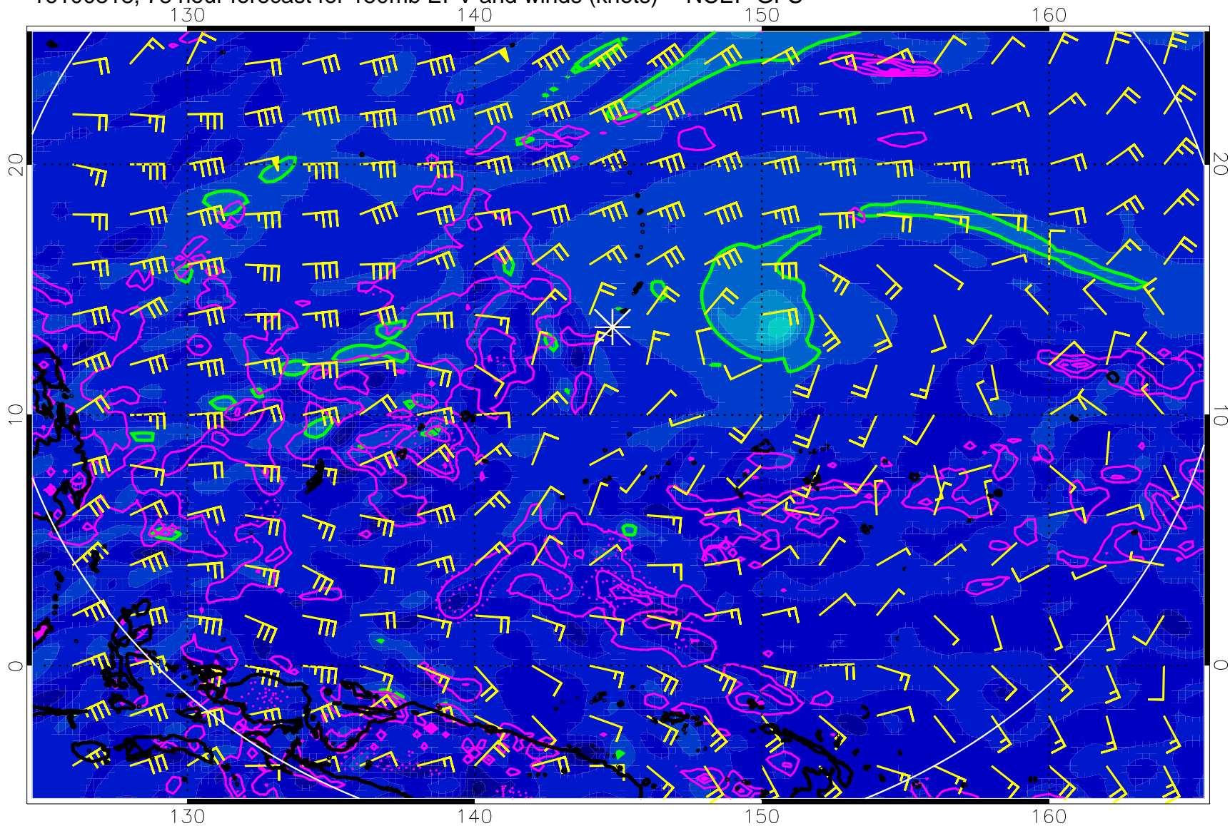
16100318, 78 hour forecast for 150mb EPV and winds (knots) -- NCEP GFS
