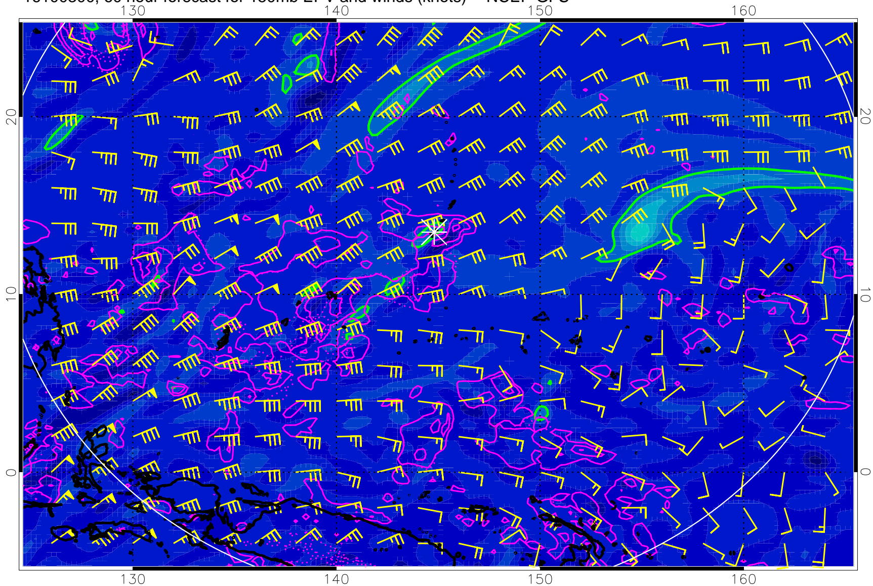
16100300, 60 hour forecast for 150mb EPV and winds (knots) -- NCEP GFS
