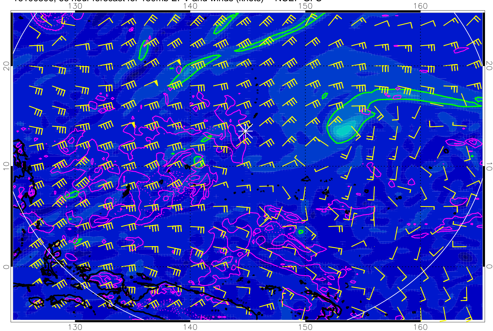
16100306, 66 hour forecast for 150mb EPV and winds (knots) -- NCEP GFS
