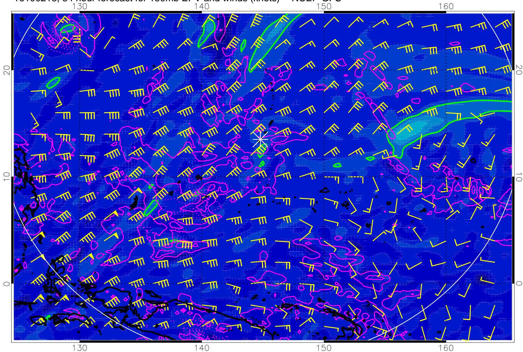
16100218, 54 hour forecast for 150mb EPV and winds (knots) -- NCEP GFS
