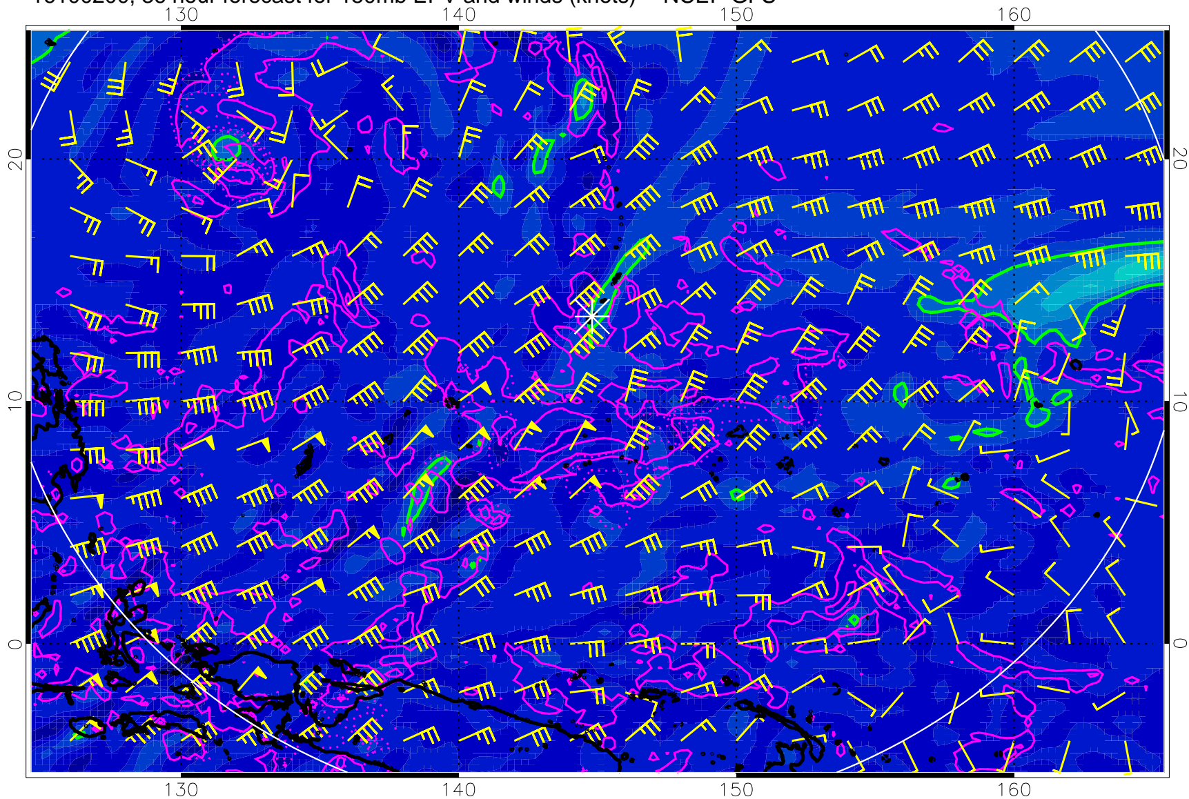
16100200, 36 hour forecast for 150mb EPV and winds (knots) -- NCEP GFS
