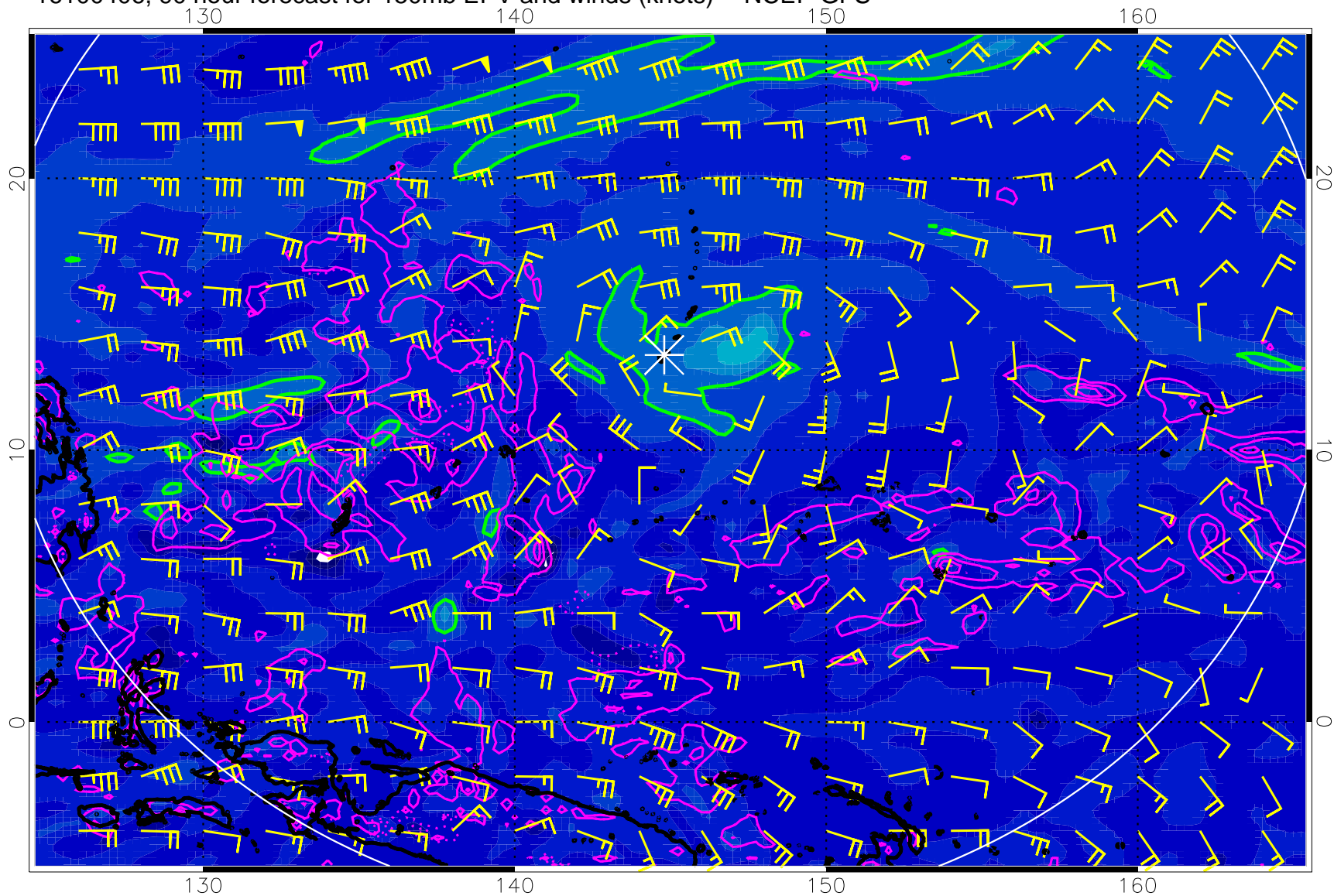
16100406, 90 hour forecast for 150mb EPV and winds (knots) -- NCEP GFS
