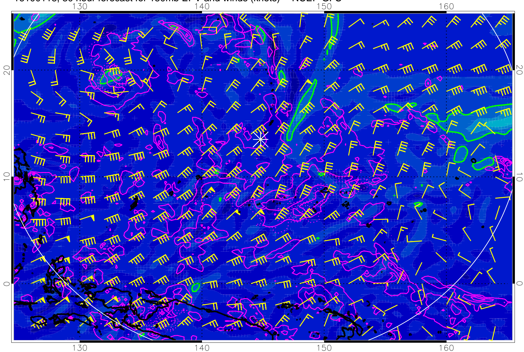
16100118, 30 hour forecast for 150mb EPV and winds (knots) -- NCEP GFS
