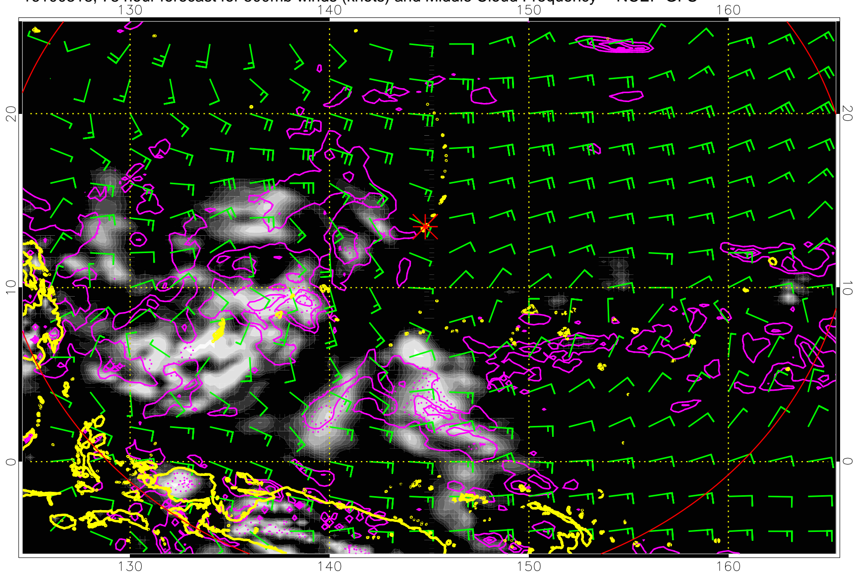
16100318, 78 hour forecast for 500mb winds (knots) and Middle Cloud Frequency -- NCEP GFS
