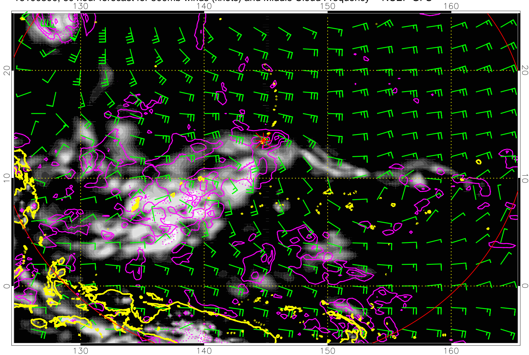
16100300, 60 hour forecast for 500mb winds (knots) and Middle Cloud Frequency -- NCEP GFS
