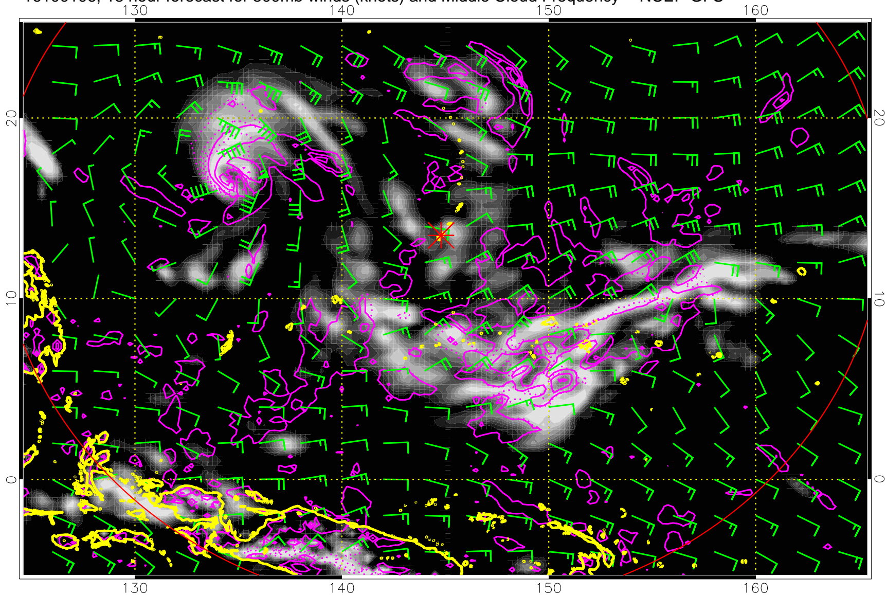
16100106, 18 hour forecast for 500mb winds (knots) and Middle Cloud Frequency -- NCEP GFS
