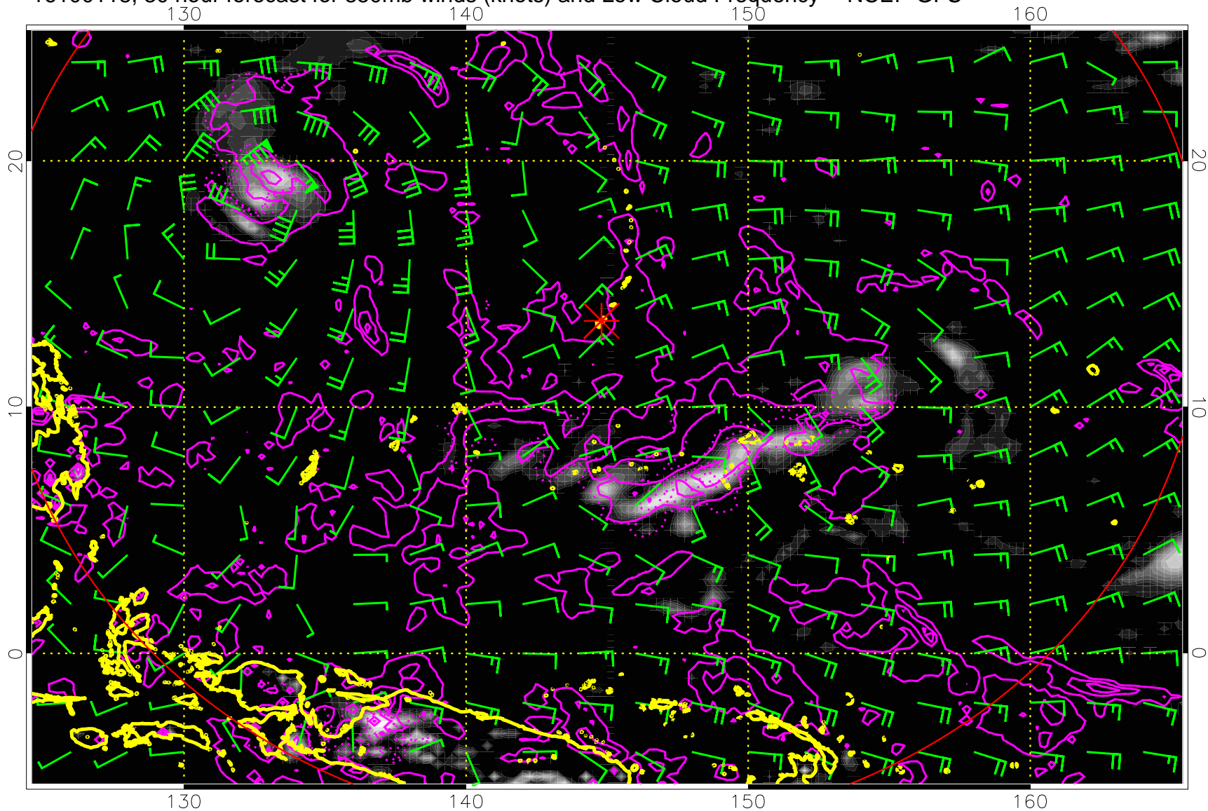
16100118, 30 hour forecast for 850mb winds (knots) and Low Cloud Frequency -- NCEP GFS
