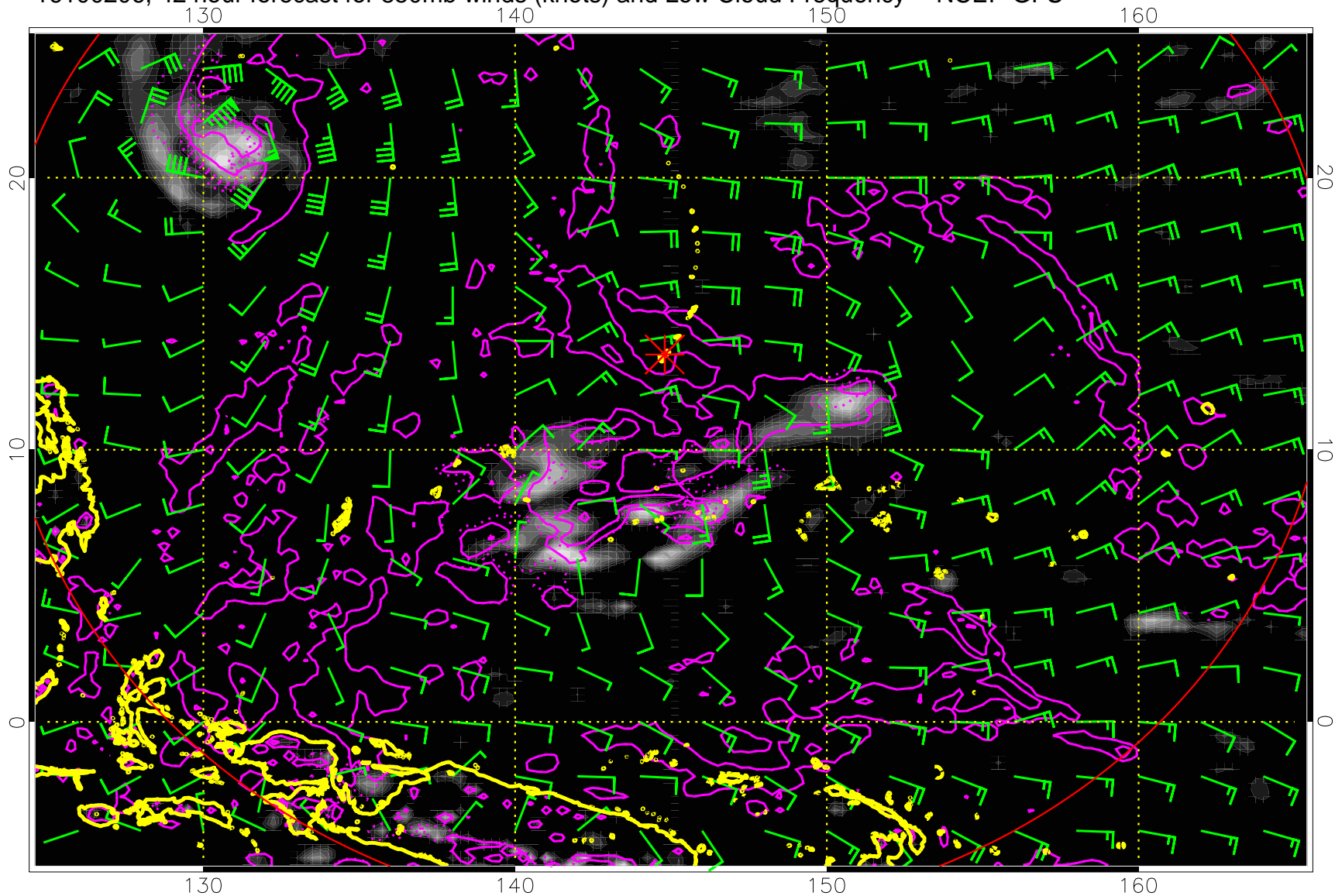
16100206, 42 hour forecast for 850mb winds (knots) and Low Cloud Frequency -- NCEP GFS
