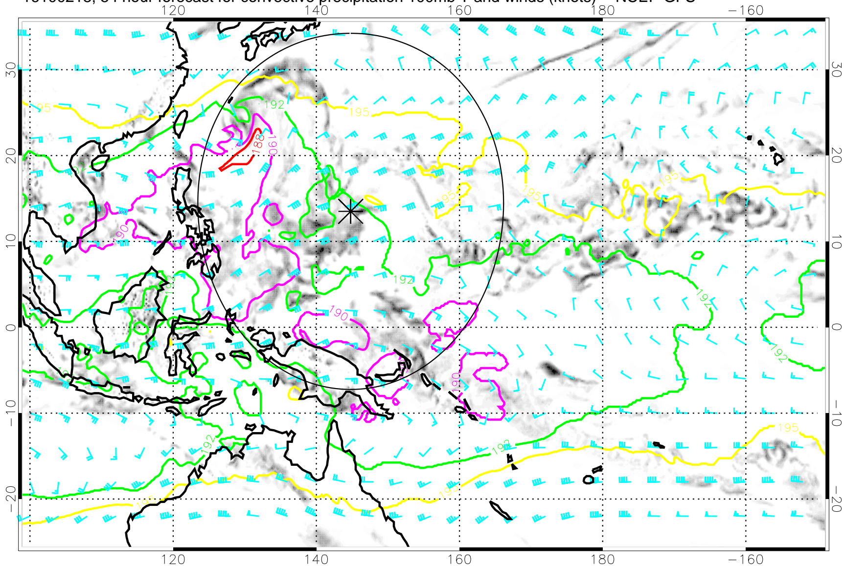
16100218, 54 hour forecast for convective precipitation 100mb T and winds (knots) -- NCEP GFS
