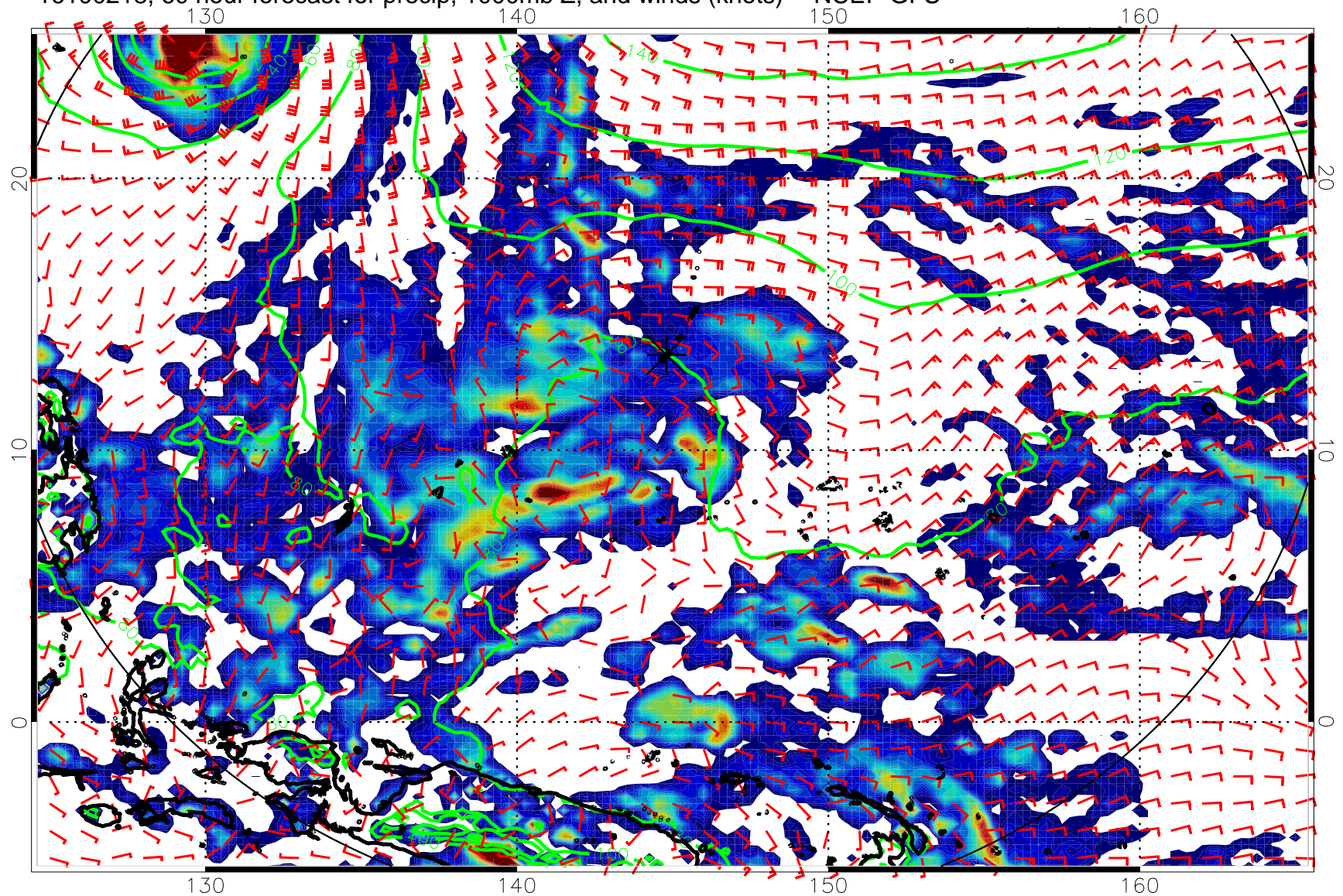
16100218, 60 hour forecast for precip, 1000mb Z, and winds (knots) -- NCEP GFS
