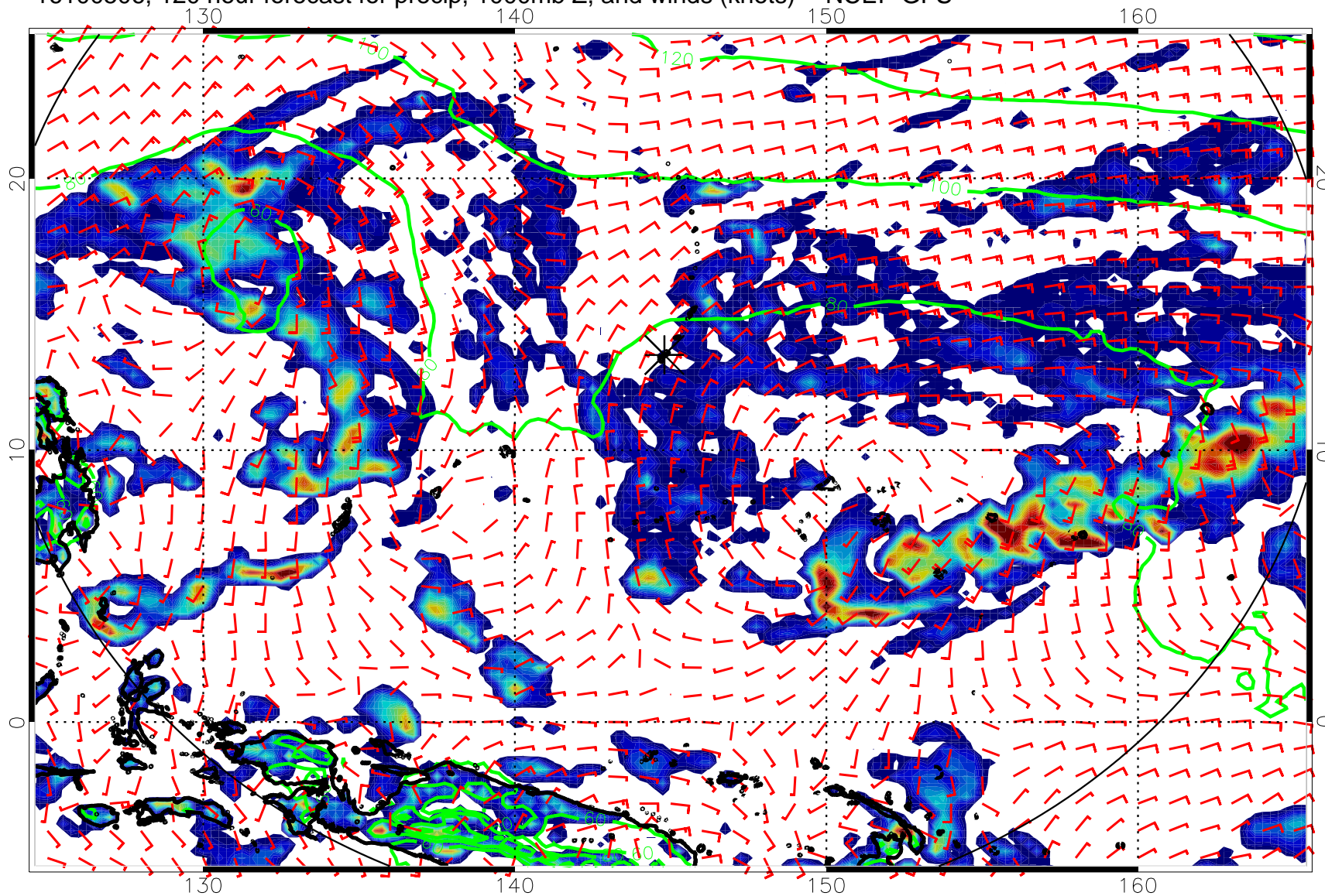
16100506, 120 hour forecast for precip, 1000mb Z, and winds (knots) -- NCEP GFS
