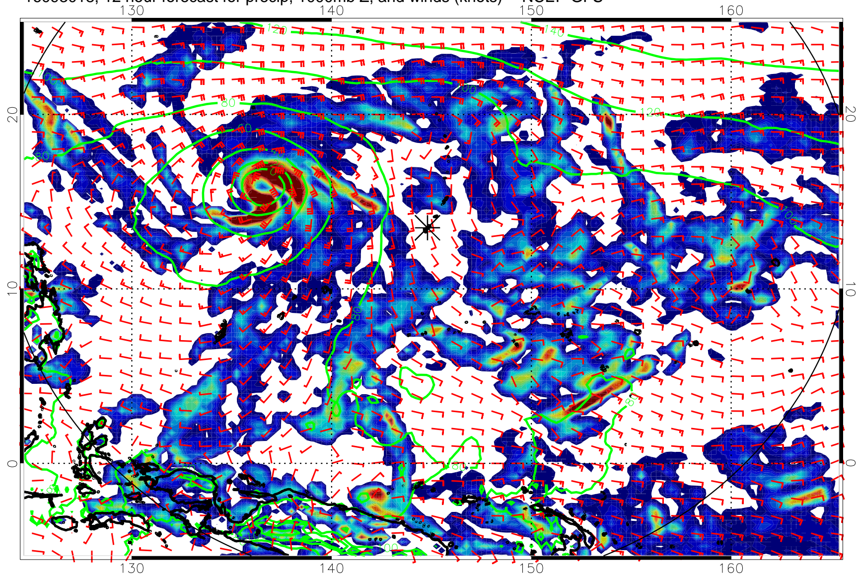
16093018, 12 hour forecast for precip, 1000mb Z, and winds (knots) -- NCEP GFS
