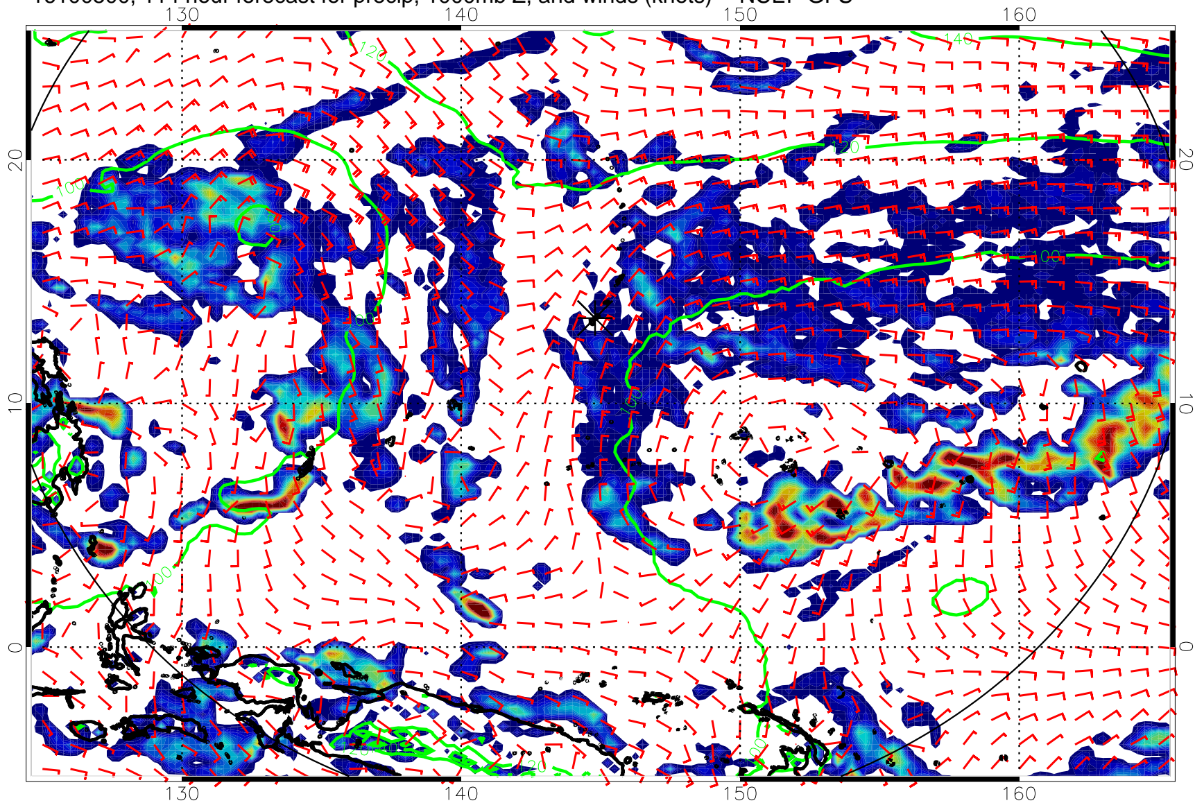
16100500, 114 hour forecast for precip, 1000mb Z, and winds (knots) -- NCEP GFS
