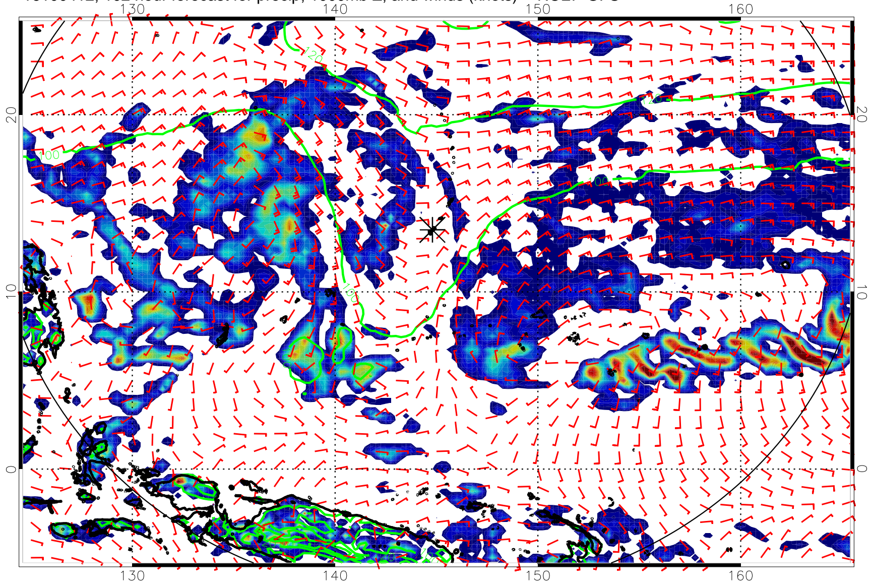
16100412, 102 hour forecast for precip, 1000mb Z, and winds (knots) -- NCEP GFS
