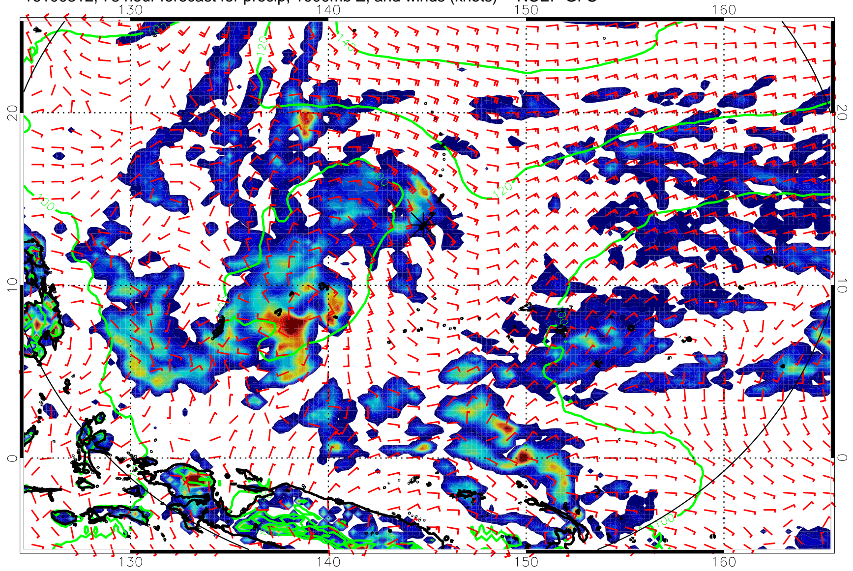
16100312, 78 hour forecast for precip, 1000mb Z, and winds (knots) -- NCEP GFS
