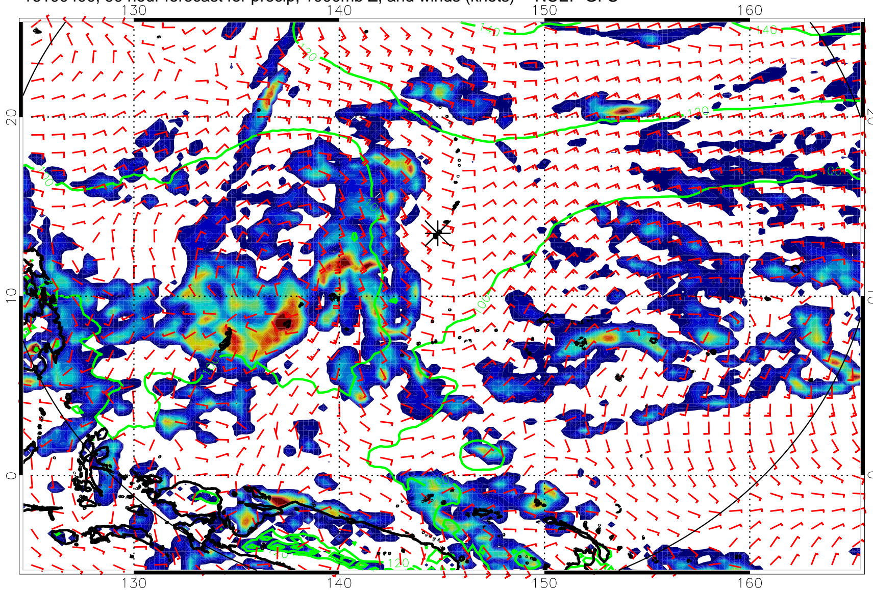
16100400, 90 hour forecast for precip, 1000mb Z, and winds (knots) -- NCEP GFS
