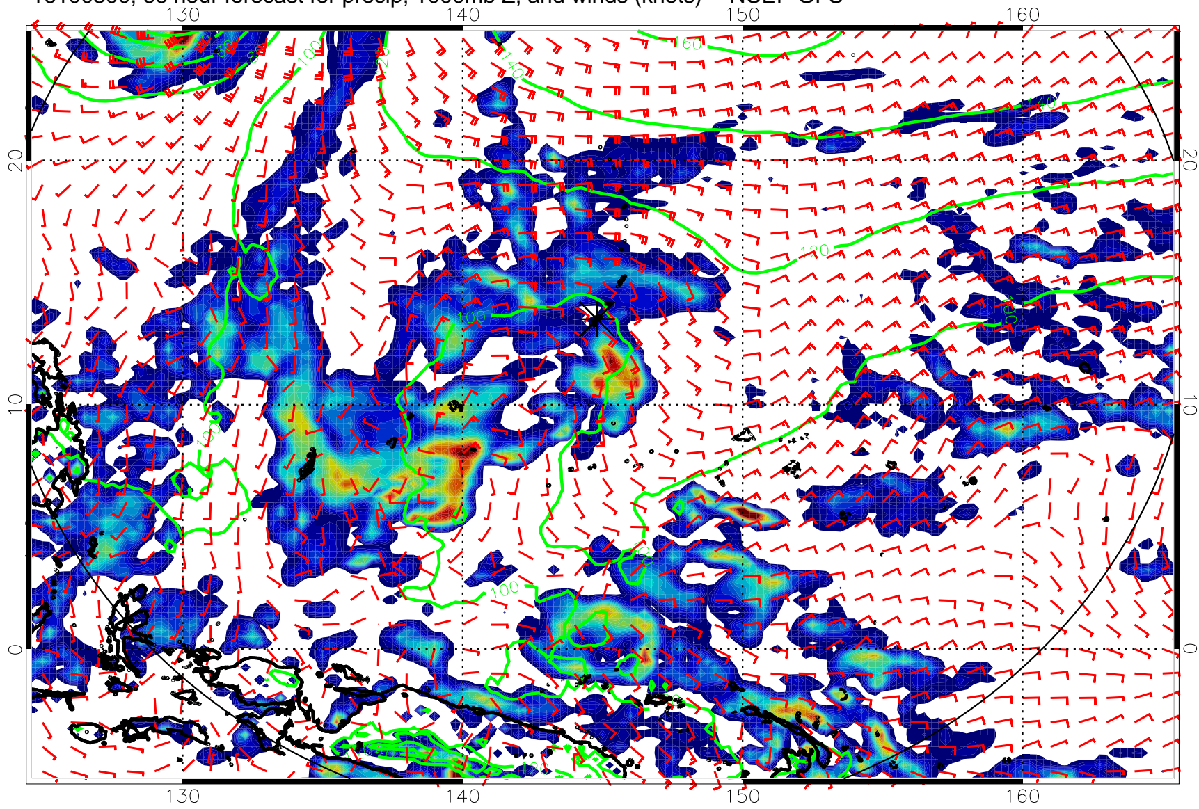
16100300, 66 hour forecast for precip, 1000mb Z, and winds (knots) -- NCEP GFS
