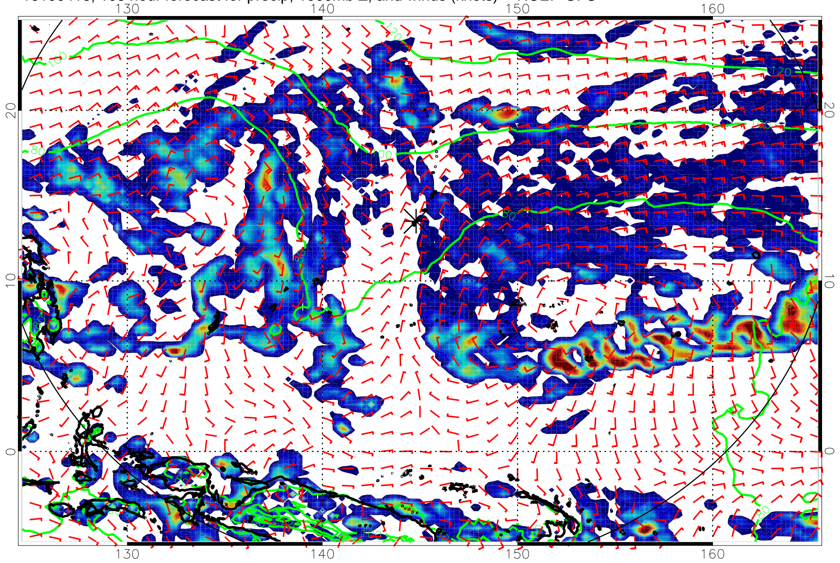
16100418, 108 hour forecast for precip, 1000mb Z, and winds (knots) -- NCEP GFS
