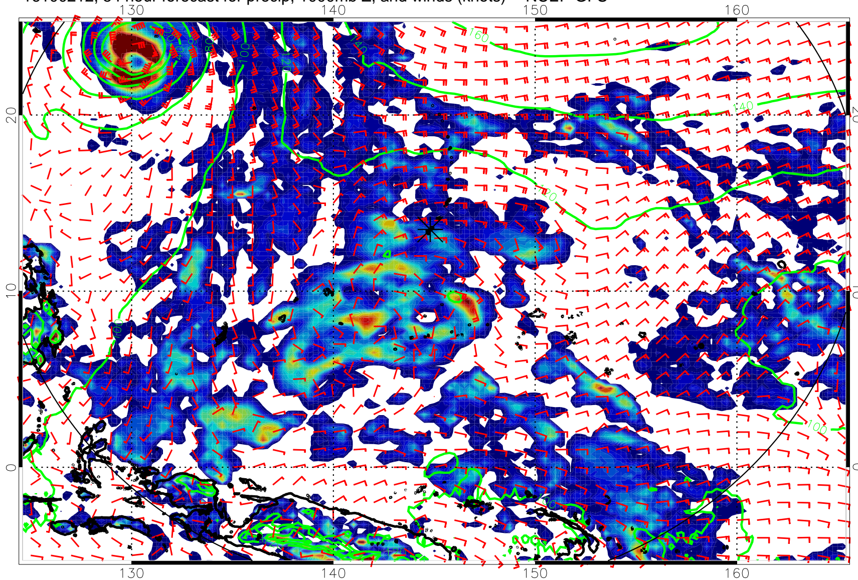
16100212, 54 hour forecast for precip, 1000mb Z, and winds (knots) -- NCEP GFS
