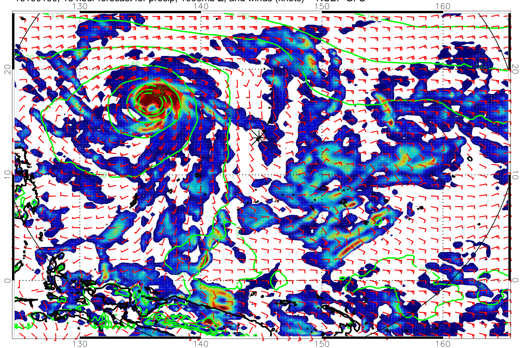
16100100, 18 hour forecast for precip, 1000mb Z, and winds (knots) -- NCEP GFS
