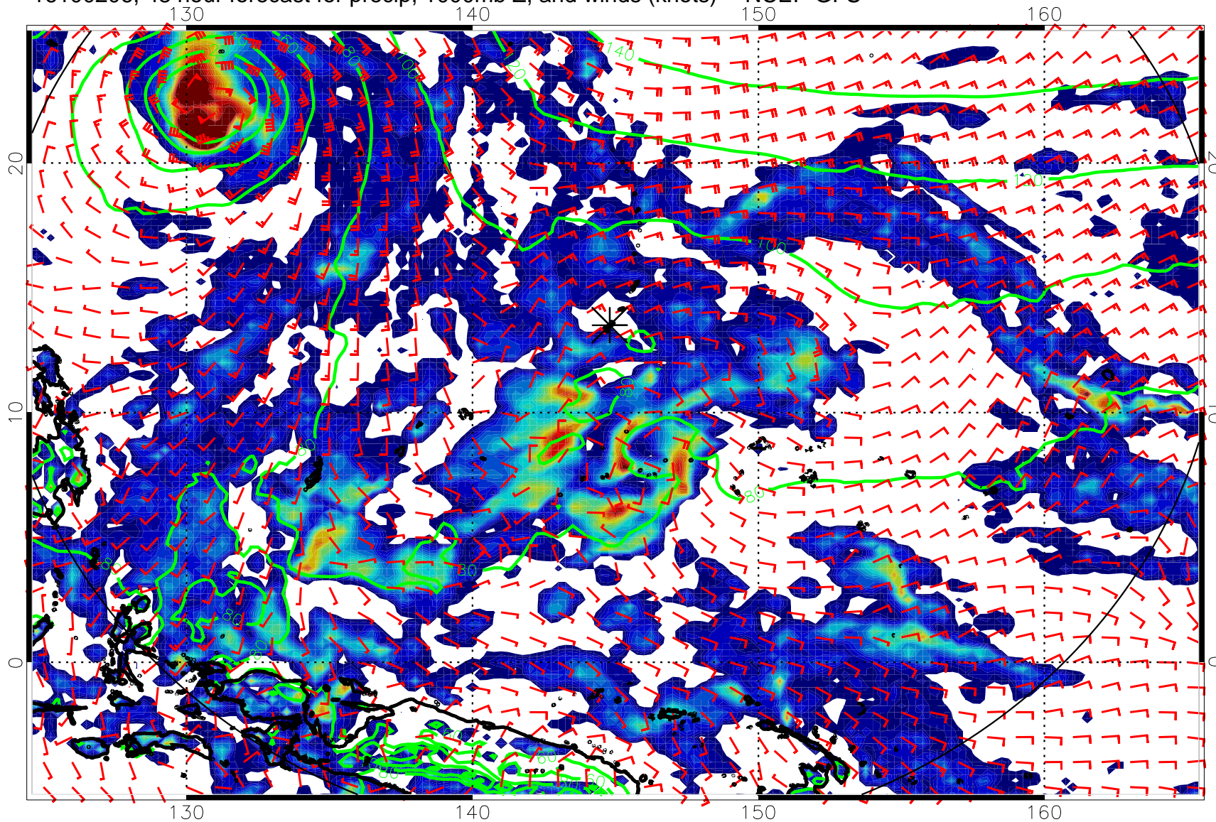
16100206, 48 hour forecast for precip, 1000mb Z, and winds (knots) -- NCEP GFS
