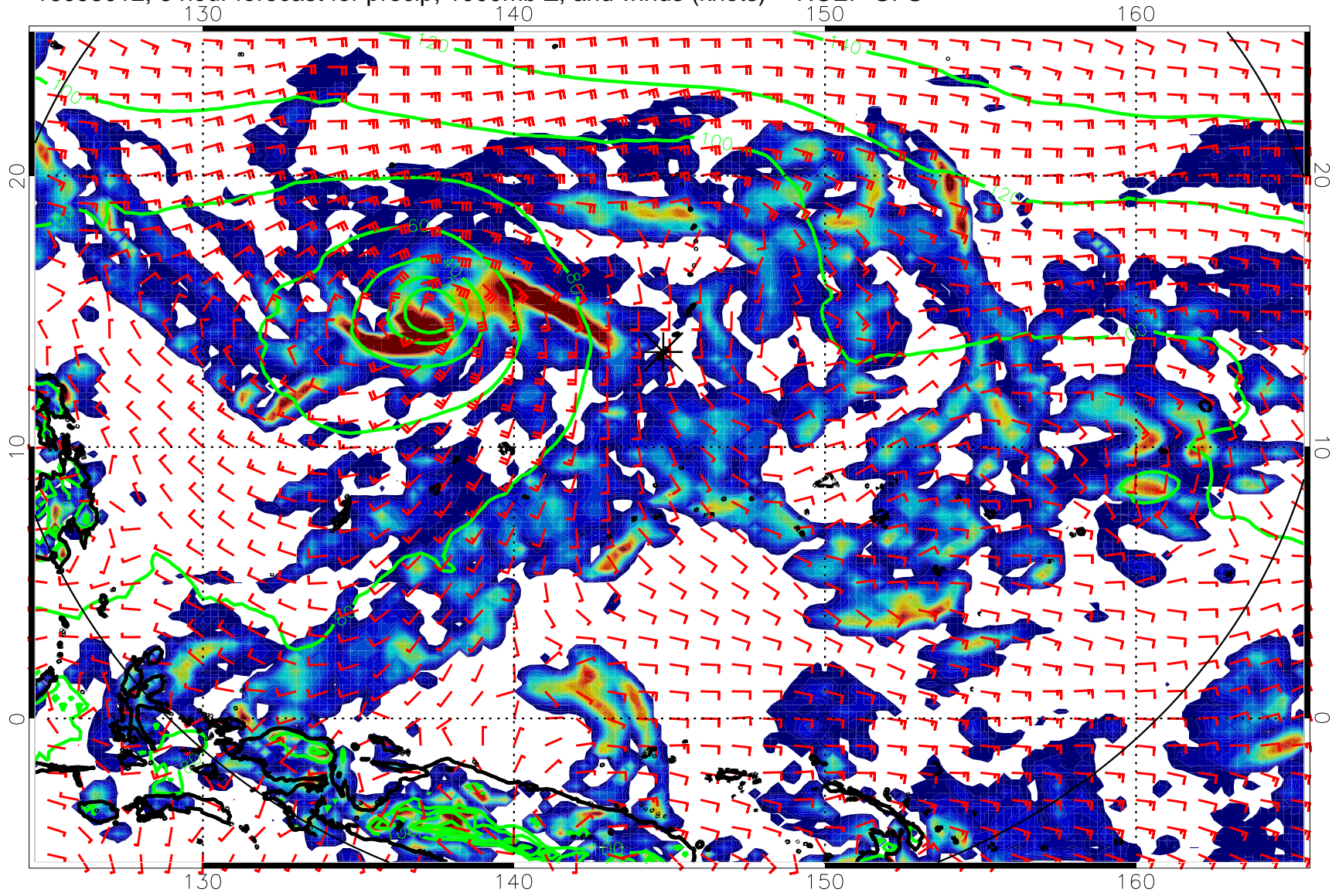
16093012, 6 hour forecast for precip, 1000mb Z, and winds (knots) -- NCEP GFS
