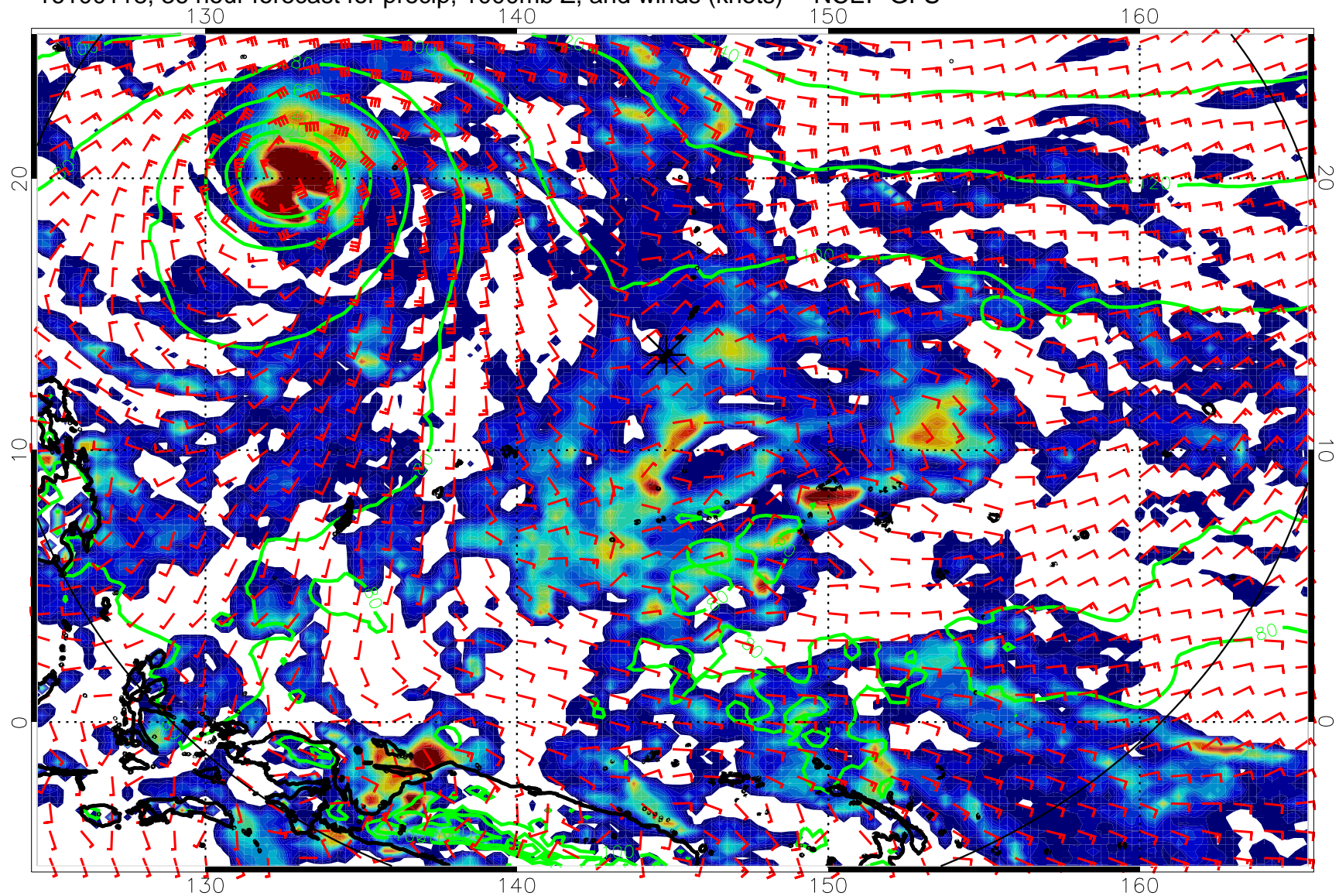
16100118, 36 hour forecast for precip, 1000mb Z, and winds (knots) -- NCEP GFS
