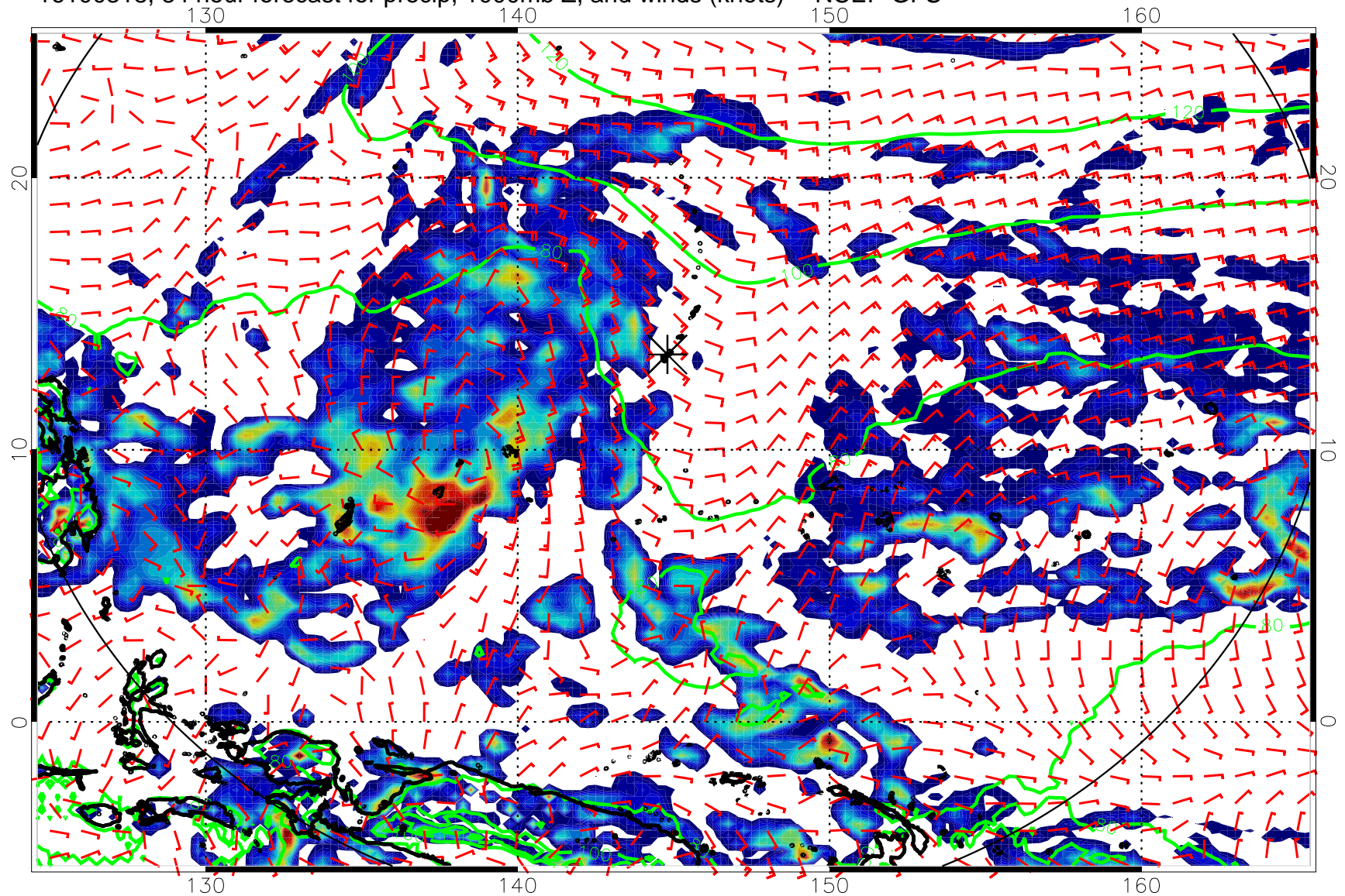
16100318, 84 hour forecast for precip, 1000mb Z, and winds (knots) -- NCEP GFS
