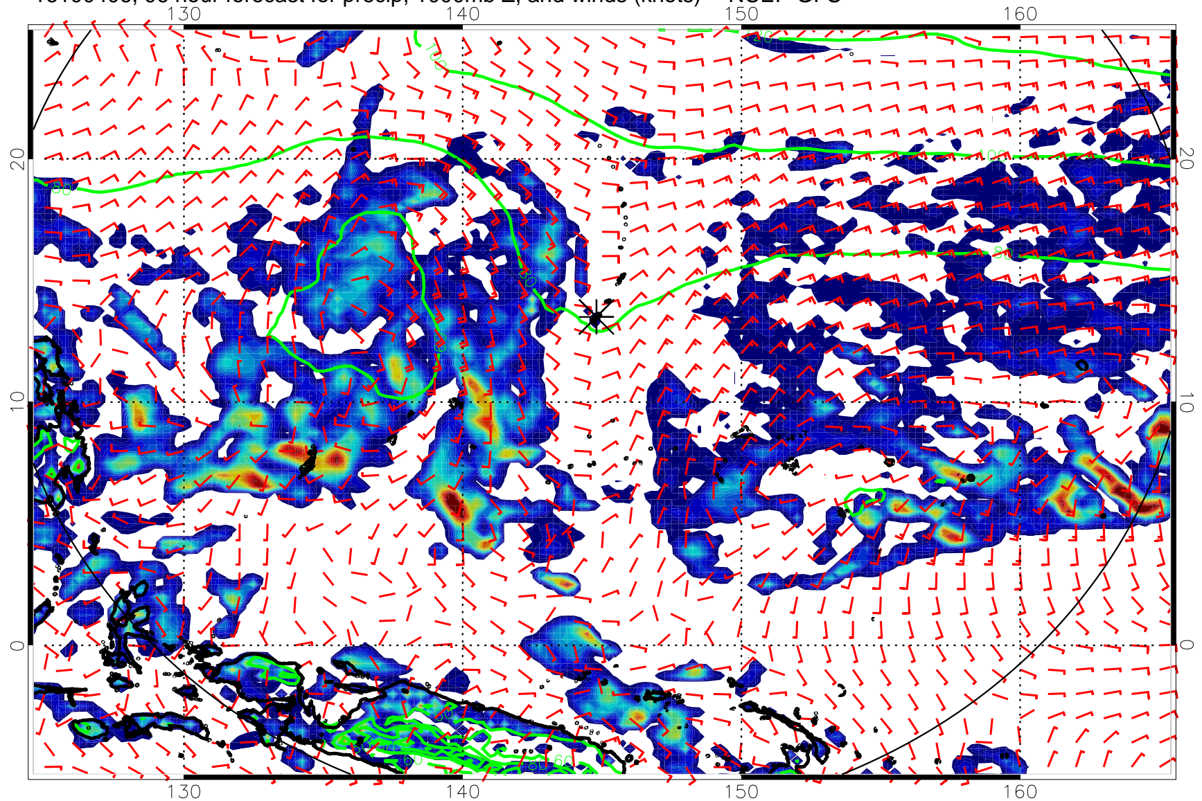
16100406, 96 hour forecast for precip, 1000mb Z, and winds (knots) -- NCEP GFS
