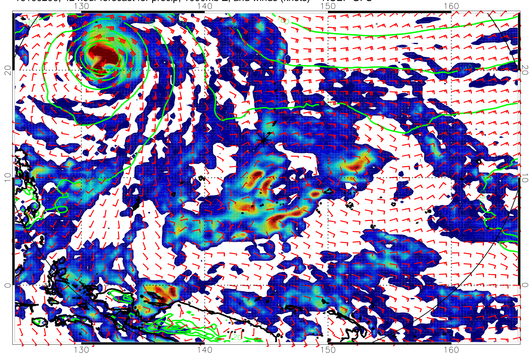
16100200, 42 hour forecast for precip, 1000mb Z, and winds (knots) -- NCEP GFS
