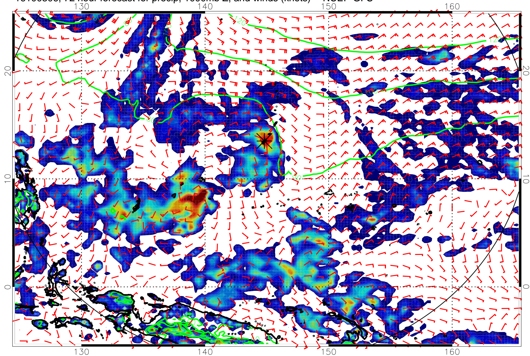
16100306, 72 hour forecast for precip, 1000mb Z, and winds (knots) -- NCEP GFS
