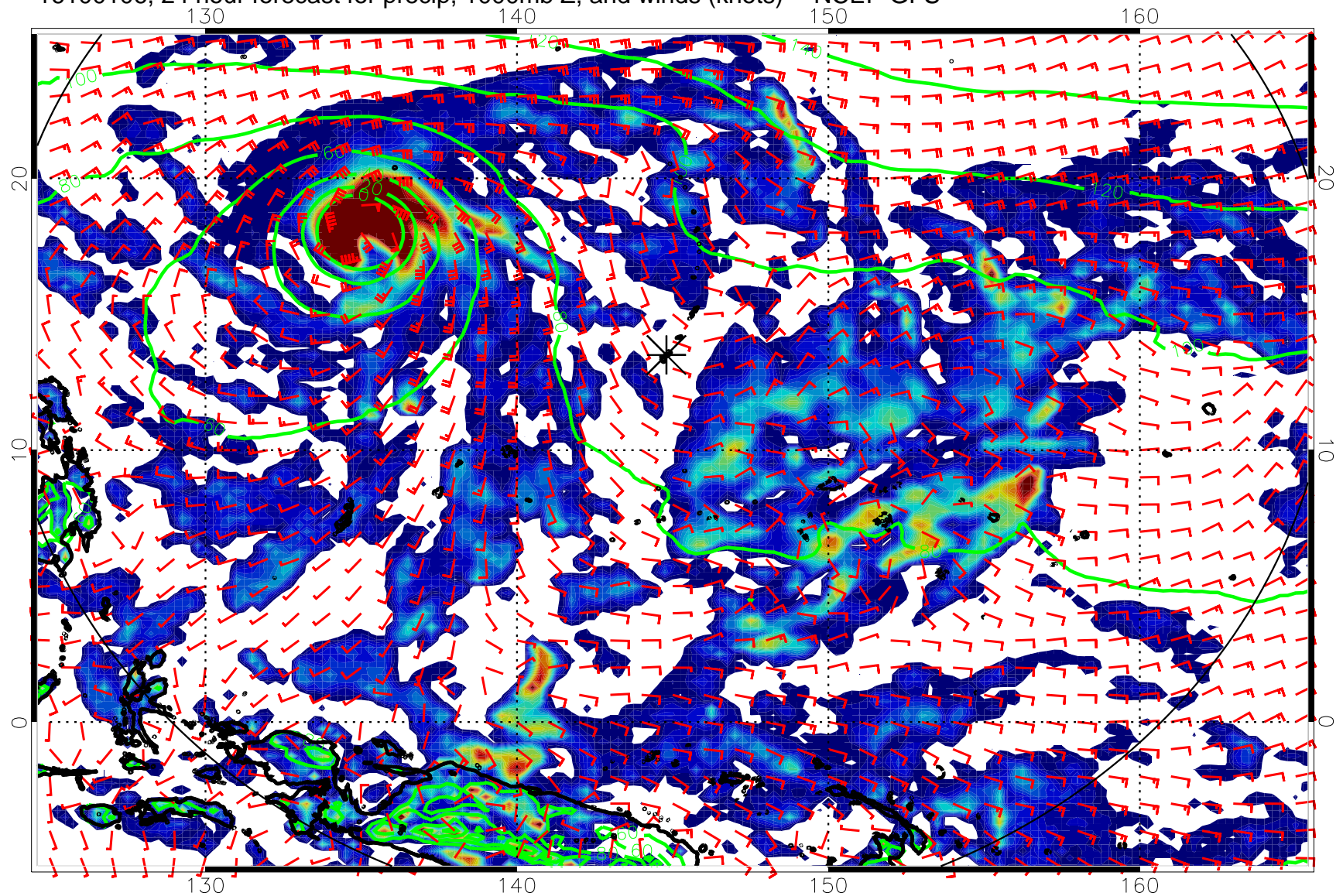
16100106, 24 hour forecast for precip, 1000mb Z, and winds (knots) -- NCEP GFS
