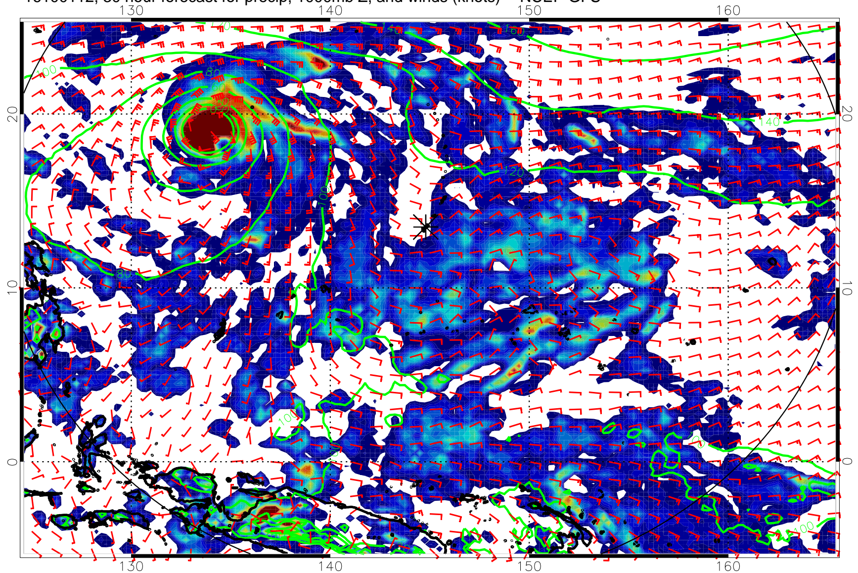
16100112, 30 hour forecast for precip, 1000mb Z, and winds (knots) -- NCEP GFS
