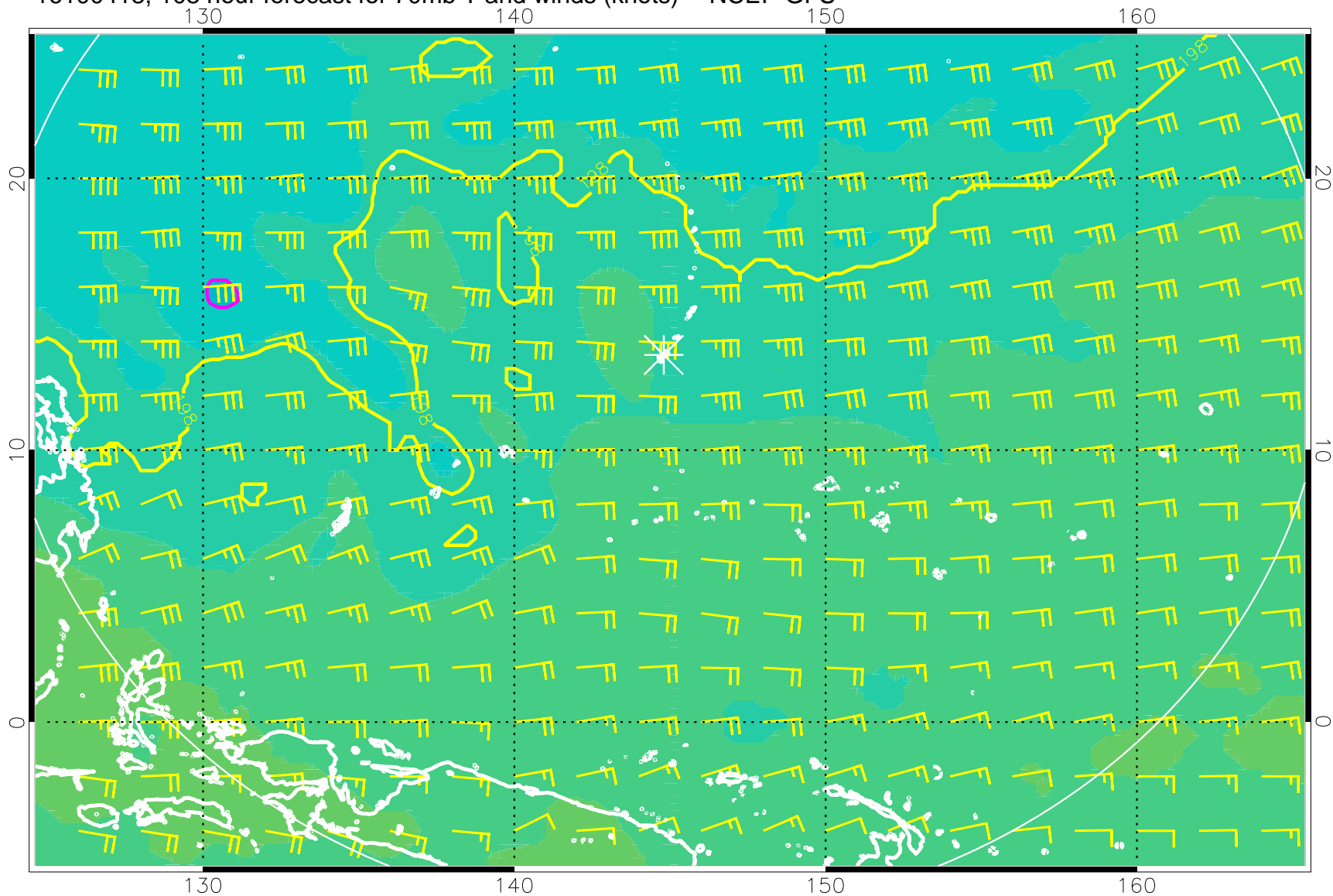
16100418, 108 hour forecast for 70mb T and winds (knots) -- NCEP GFS
