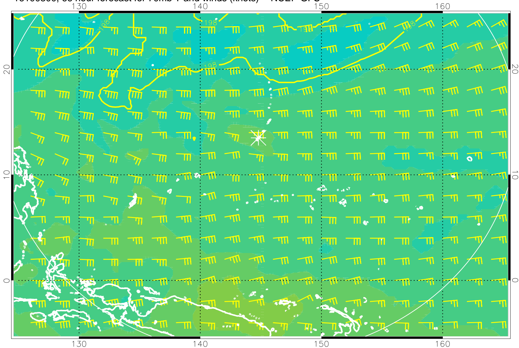
16100300, 66 hour forecast for 70mb T and winds (knots) -- NCEP GFS
