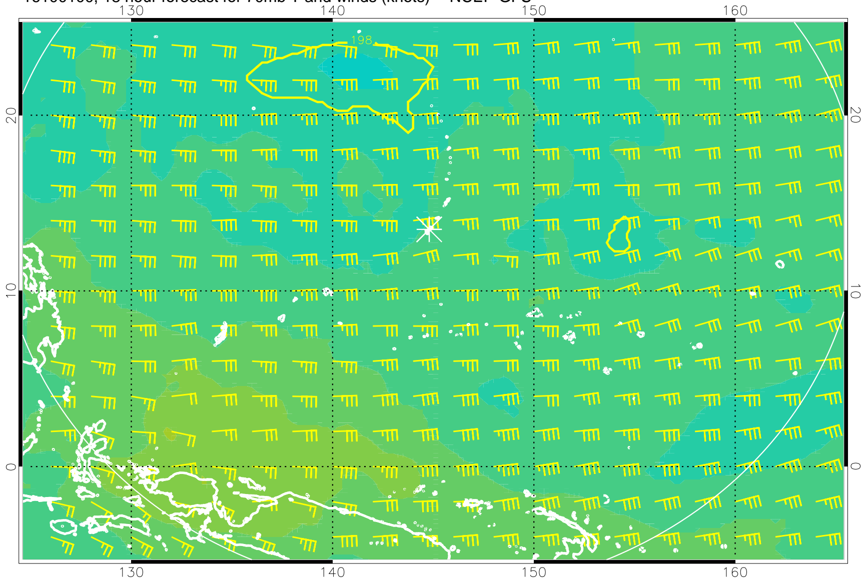
16100100, 18 hour forecast for 70mb T and winds (knots) -- NCEP GFS
