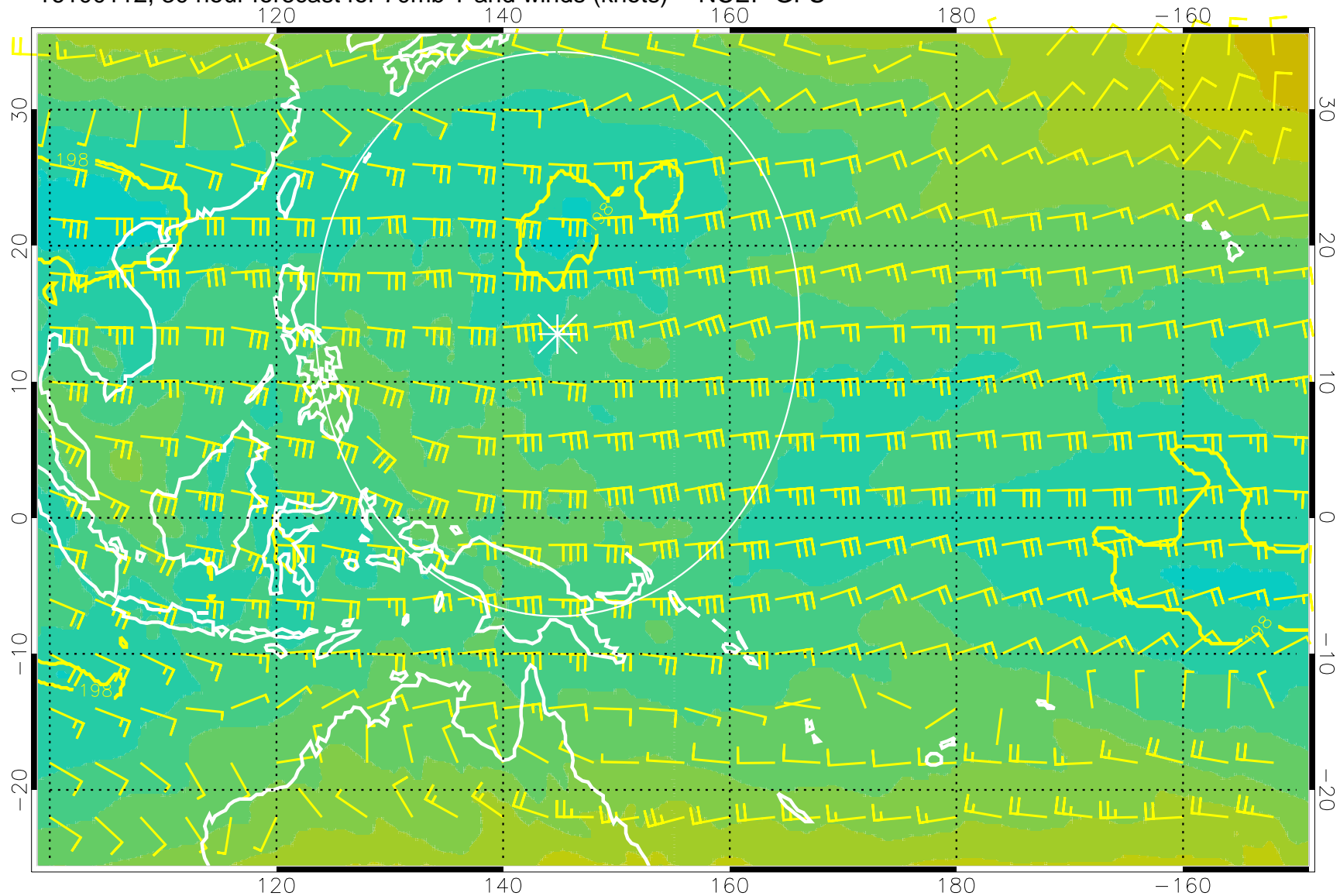
16100112, 30 hour forecast for 70mb T and winds (knots) -- NCEP GFS
