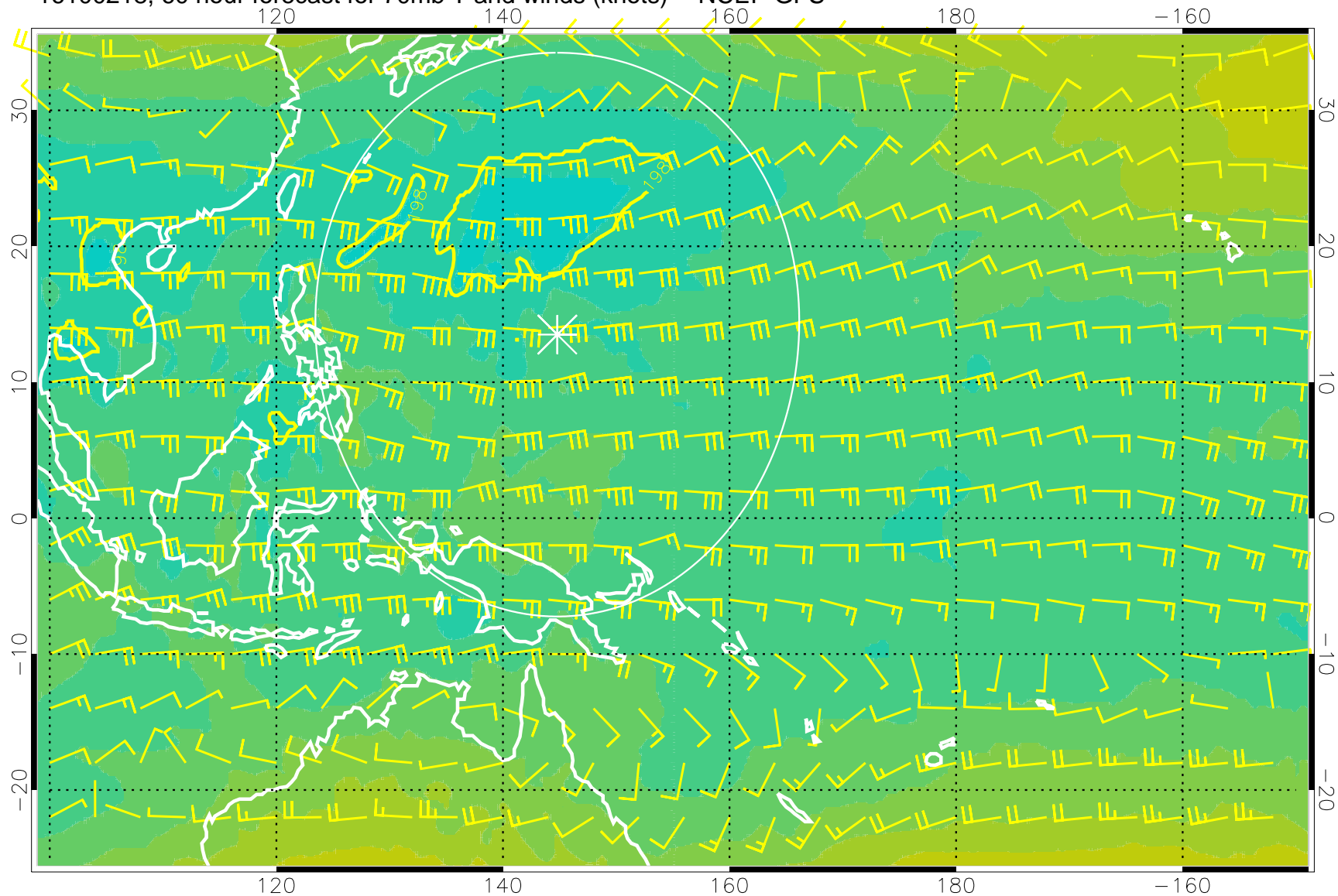
16100218, 60 hour forecast for 70mb T and winds (knots) -- NCEP GFS
