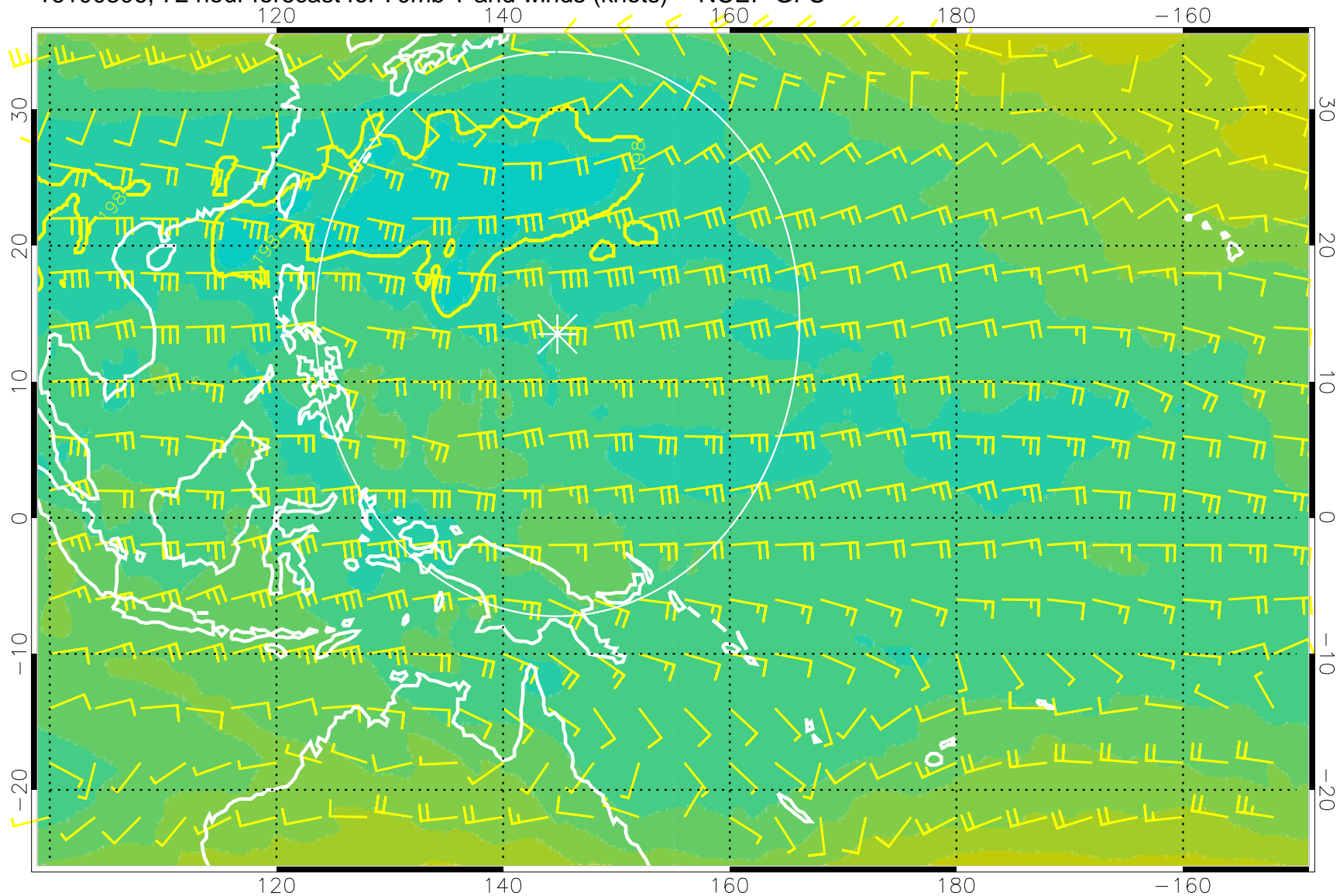
16100306, 72 hour forecast for 70mb T and winds (knots) -- NCEP GFS
