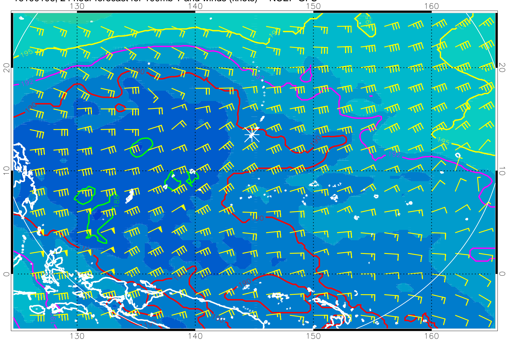
16100106, 24 hour forecast for 100mb T and winds (knots) -- NCEP GFS
