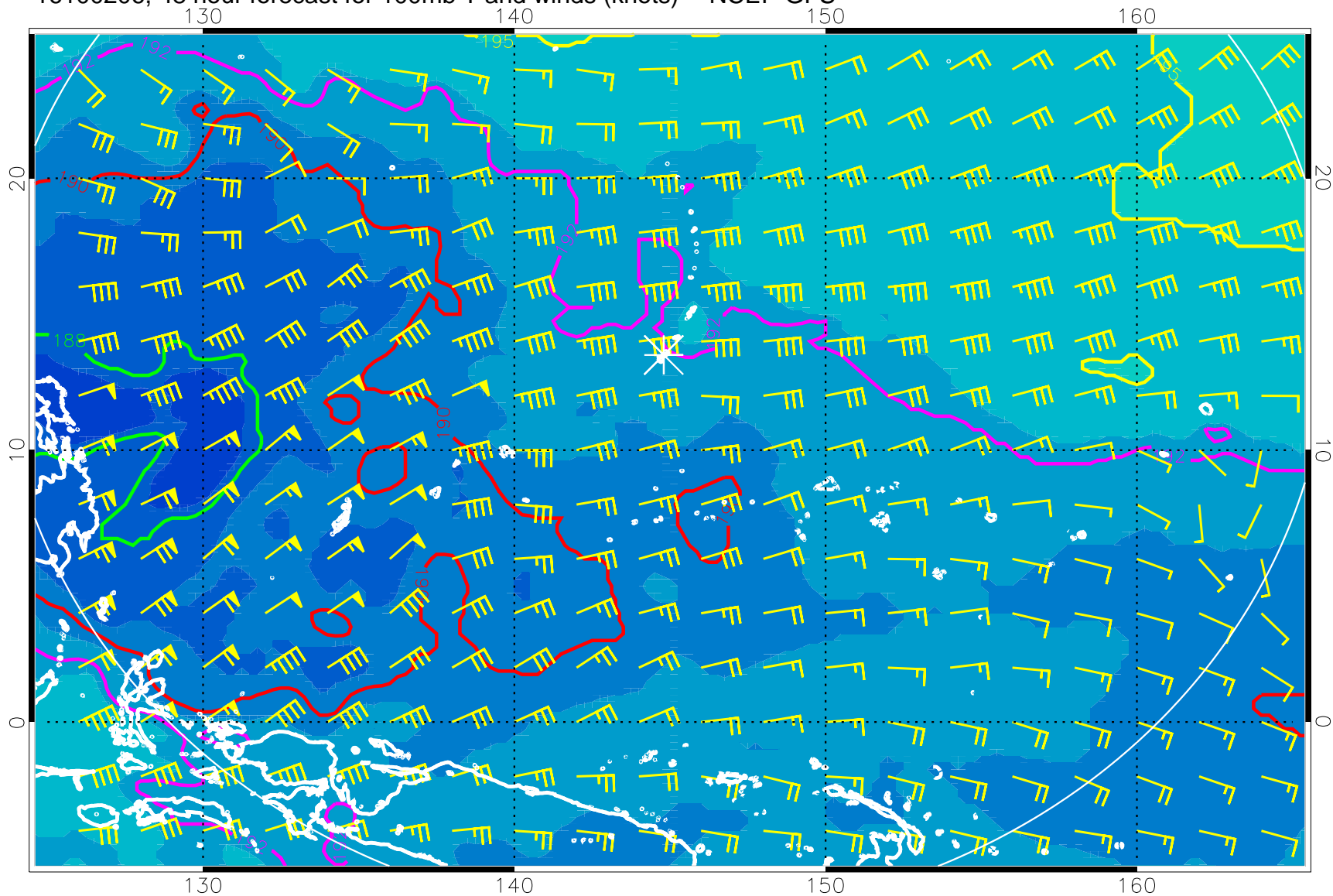
16100206, 48 hour forecast for 100mb T and winds (knots) -- NCEP GFS
