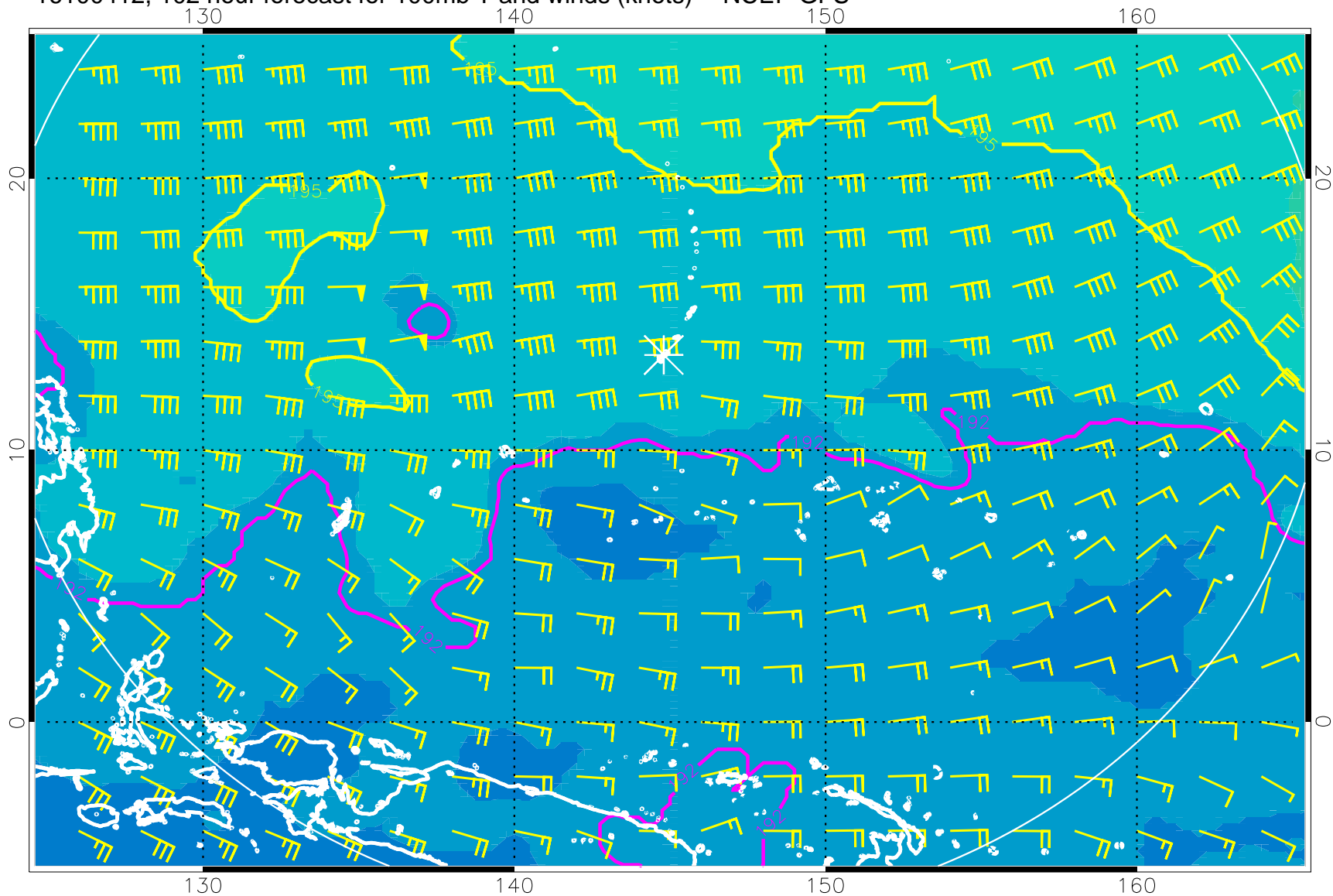
16100412, 102 hour forecast for 100mb T and winds (knots) -- NCEP GFS
