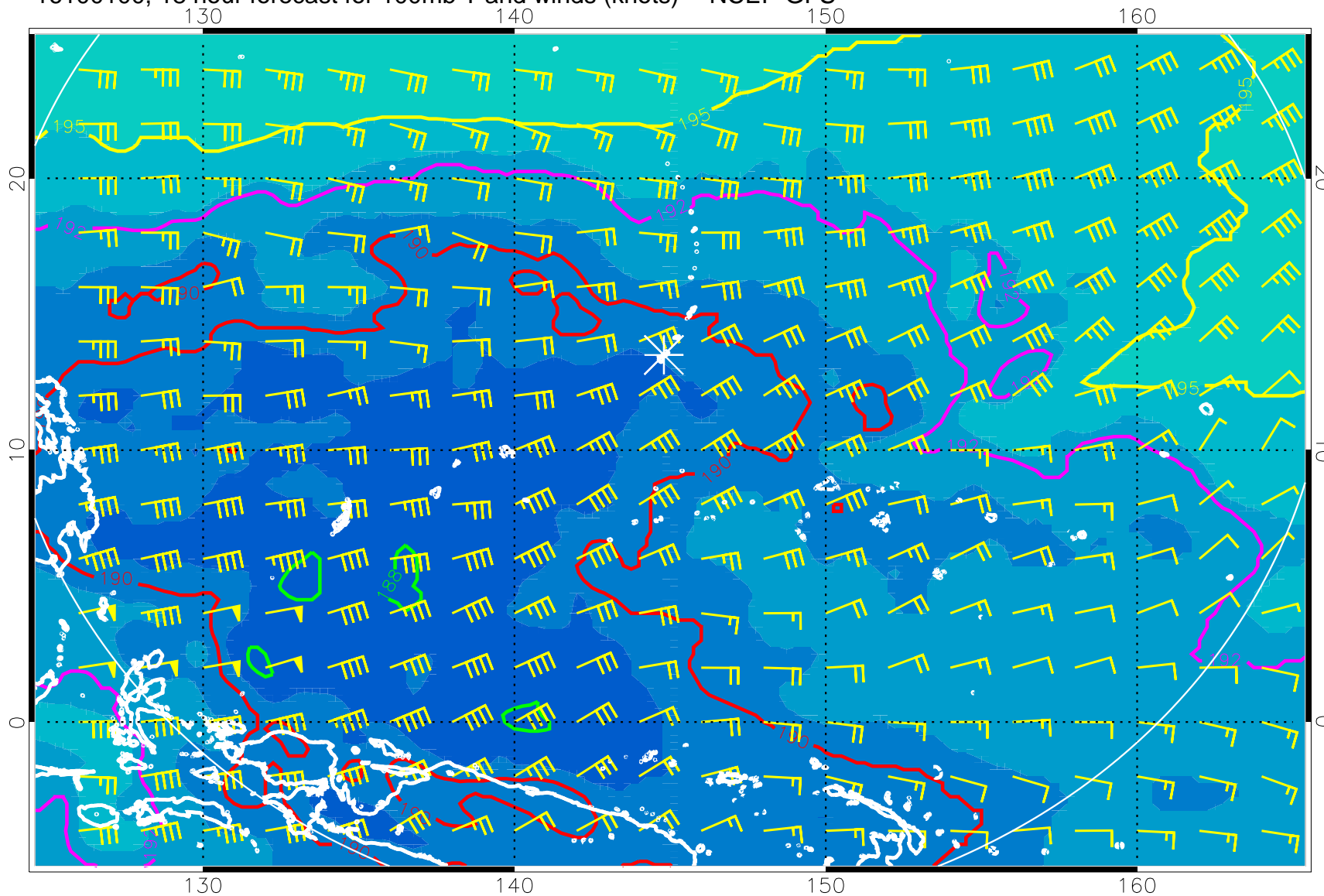
16100100, 18 hour forecast for 100mb T and winds (knots) -- NCEP GFS
