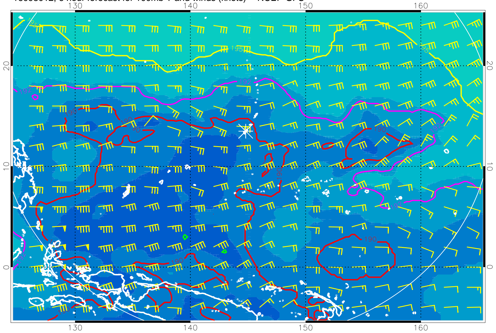
16093012, 6 hour forecast for 100mb T and winds (knots) -- NCEP GFS
