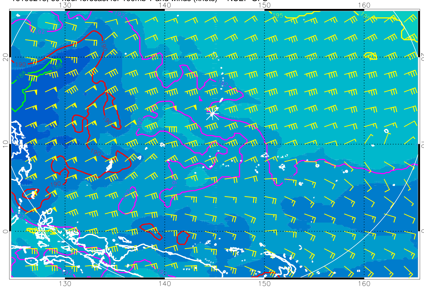
16100218, 60 hour forecast for 100mb T and winds (knots) -- NCEP GFS
