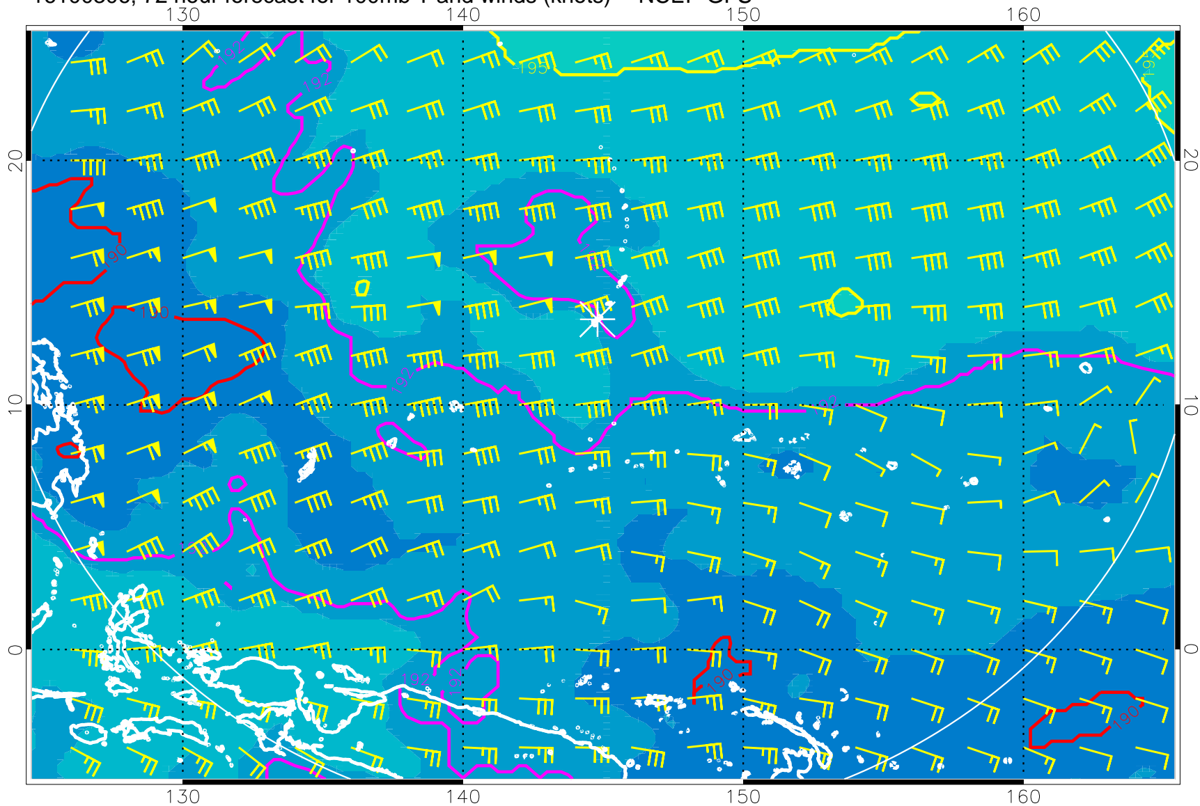
16100306, 72 hour forecast for 100mb T and winds (knots) -- NCEP GFS
