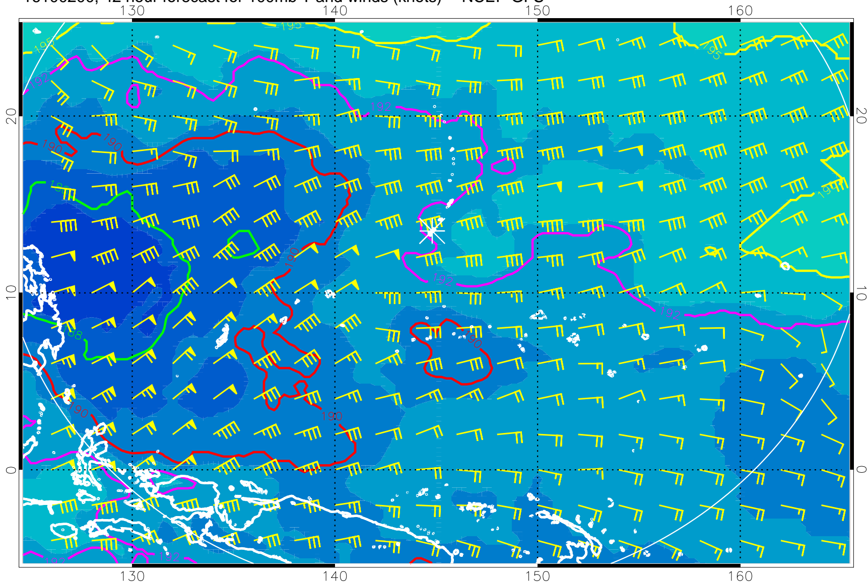
16100200, 42 hour forecast for 100mb T and winds (knots) -- NCEP GFS
