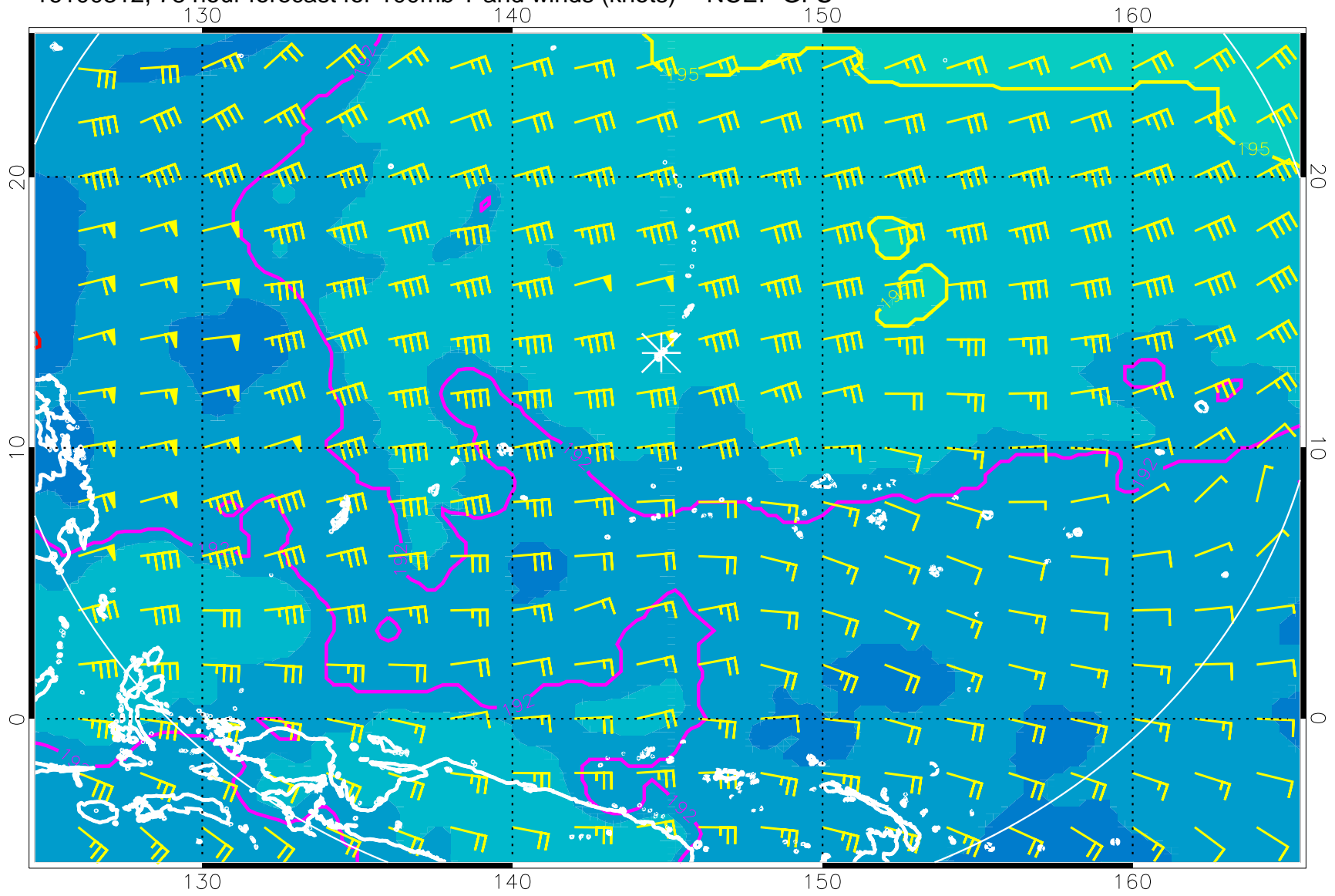
16100312, 78 hour forecast for 100mb T and winds (knots) -- NCEP GFS
