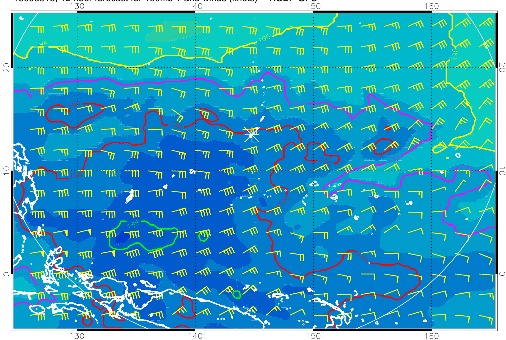
16093018, 12 hour forecast for 100mb T and winds (knots) -- NCEP GFS
