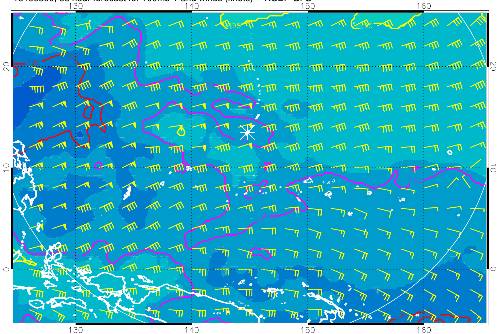
16100300, 66 hour forecast for 100mb T and winds (knots) -- NCEP GFS
