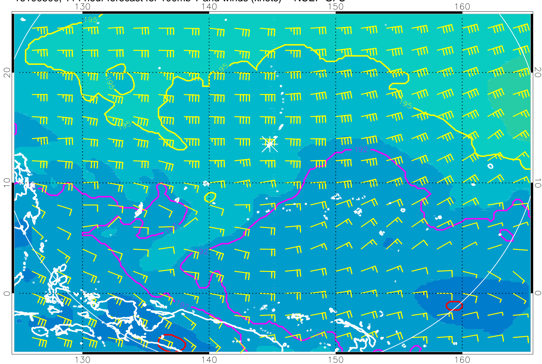
16100500, 114 hour forecast for 100mb T and winds (knots) -- NCEP GFS
