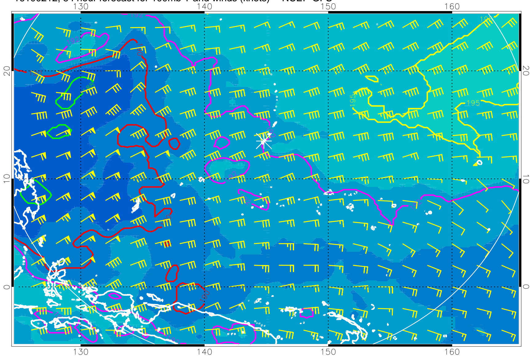
16100212, 54 hour forecast for 100mb T and winds (knots) -- NCEP GFS
