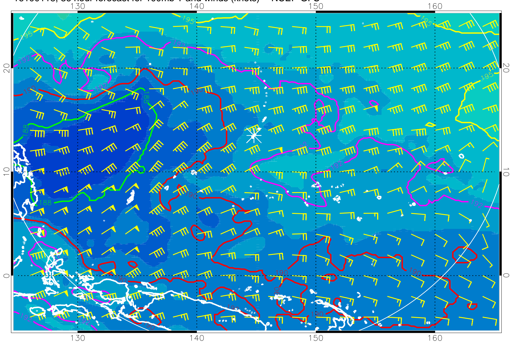
16100118, 36 hour forecast for 100mb T and winds (knots) -- NCEP GFS
