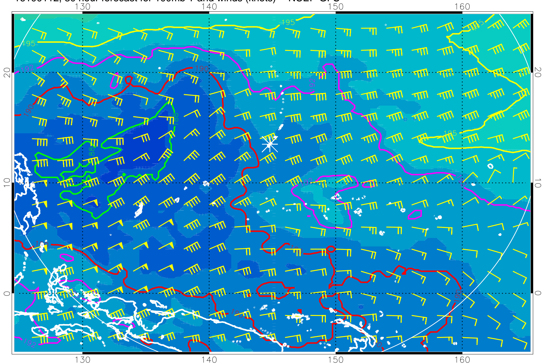
16100112, 30 hour forecast for 100mb T and winds (knots) -- NCEP GFS
