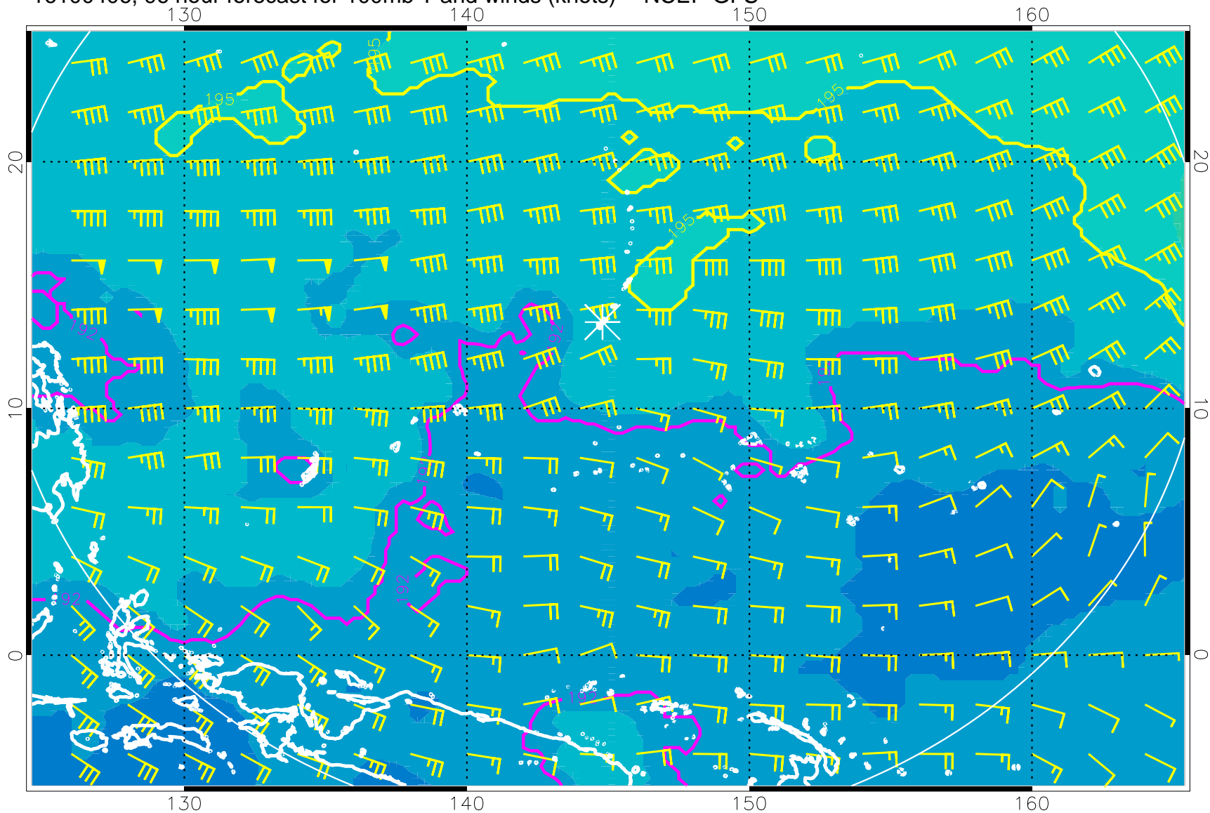
16100406, 96 hour forecast for 100mb T and winds (knots) -- NCEP GFS
