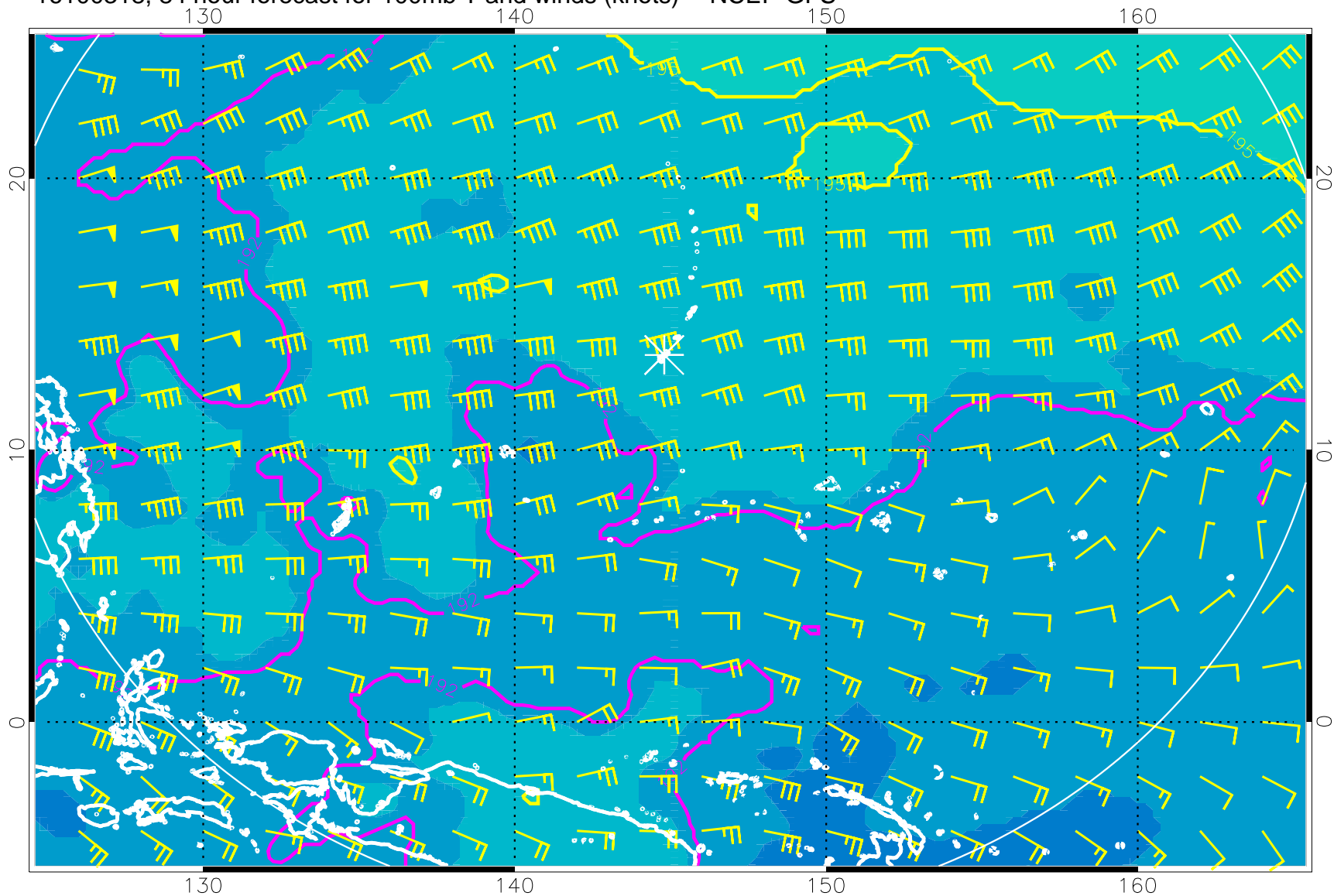
16100318, 84 hour forecast for 100mb T and winds (knots) -- NCEP GFS
