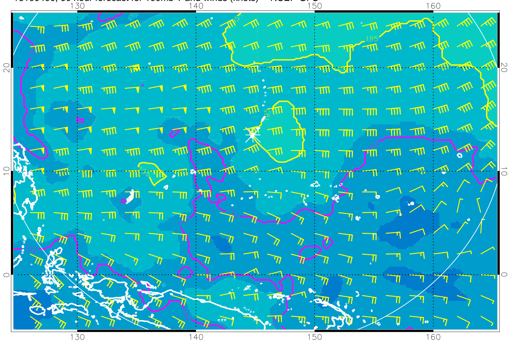
16100400, 90 hour forecast for 100mb T and winds (knots) -- NCEP GFS
