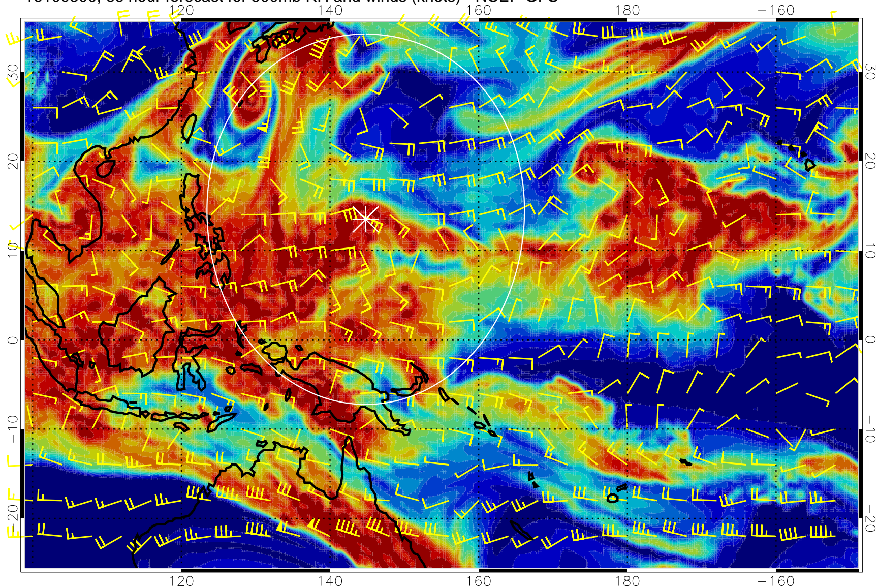
16100300, 66 hour forecast for 500mb RH and winds (knots) - NCEP GFS
