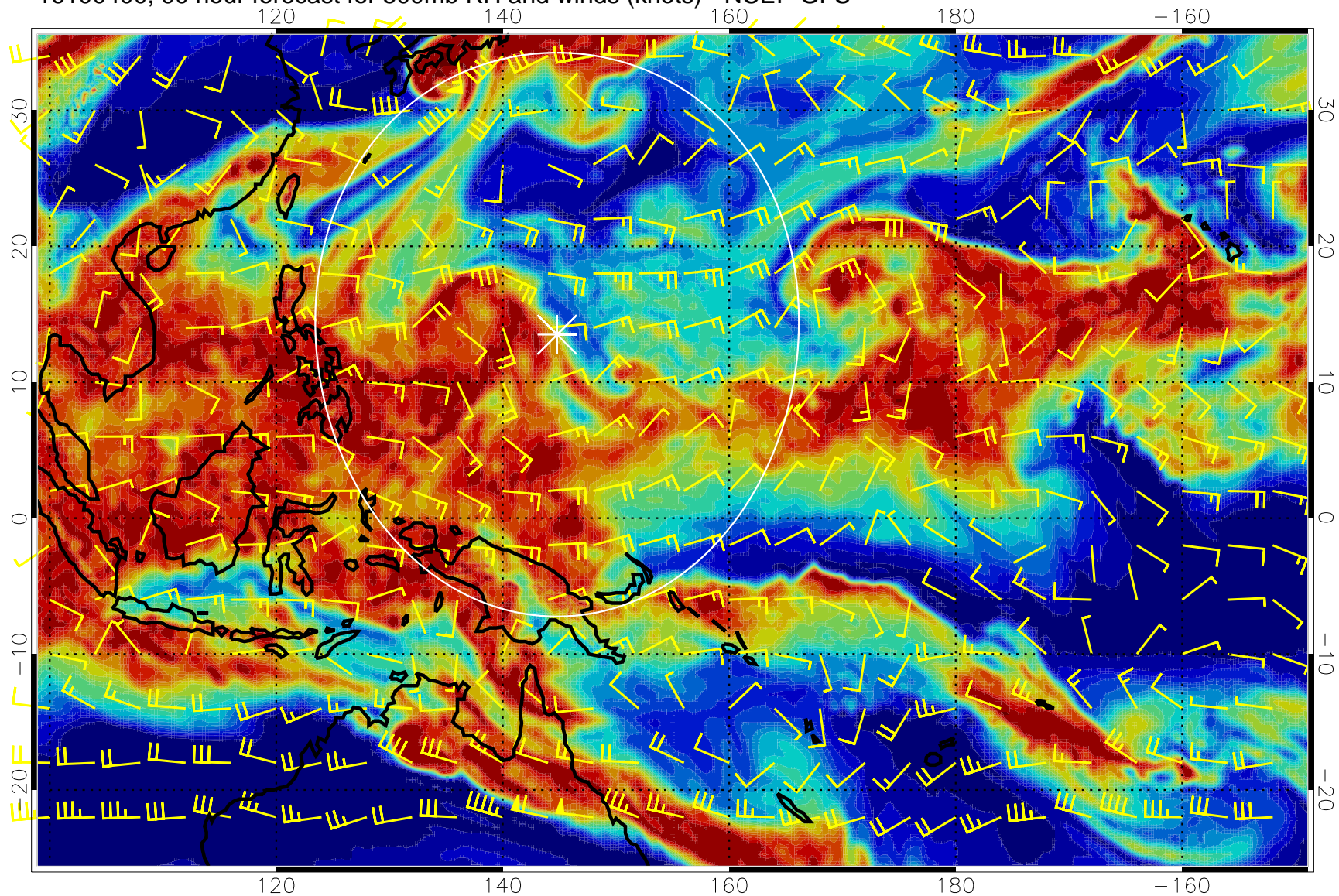
16100400, 90 hour forecast for 500mb RH and winds (knots) - NCEP GFS
