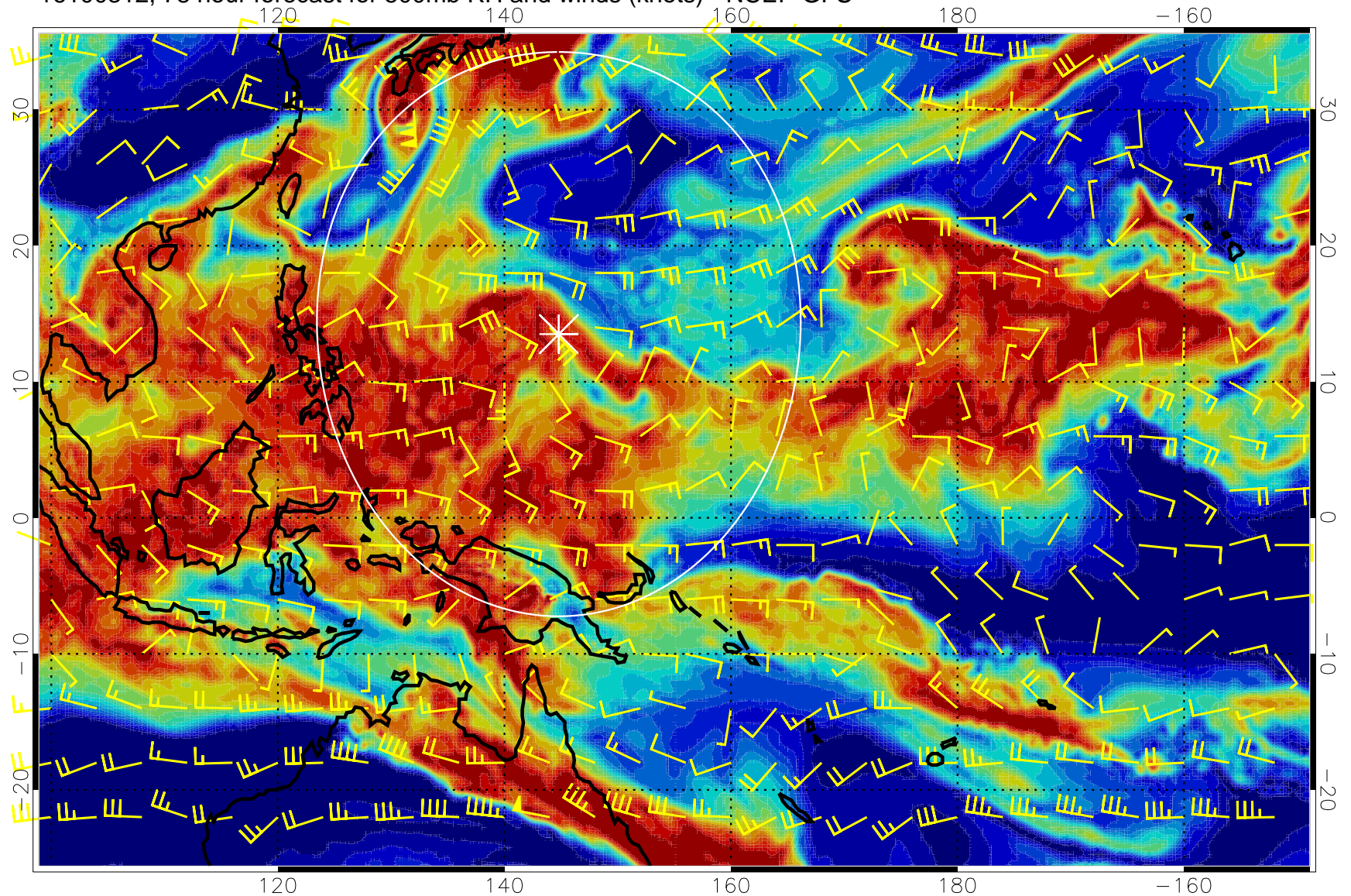
16100312, 78 hour forecast for 500mb RH and winds (knots) - NCEP GFS
