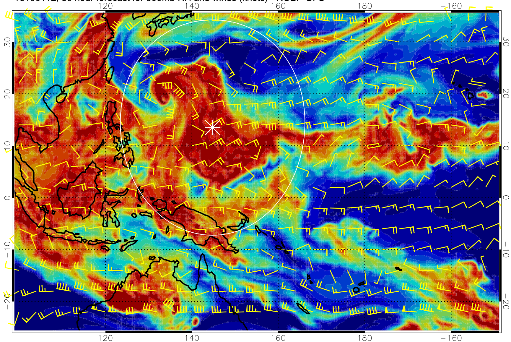
16100112, 30 hour forecast for 500mb RH and winds (knots) - NCEP GFS
