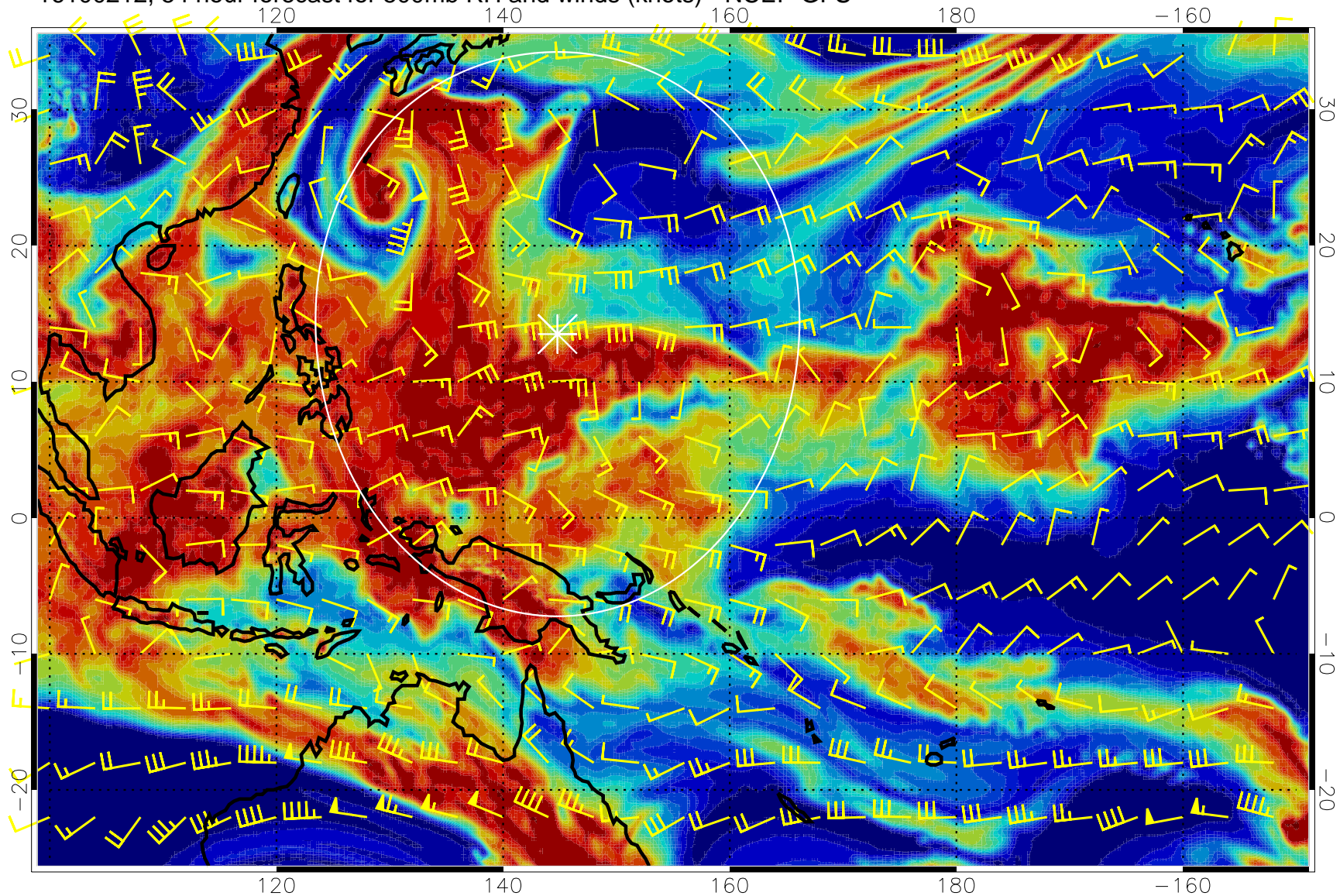
16100212, 54 hour forecast for 500mb RH and winds (knots) - NCEP GFS
