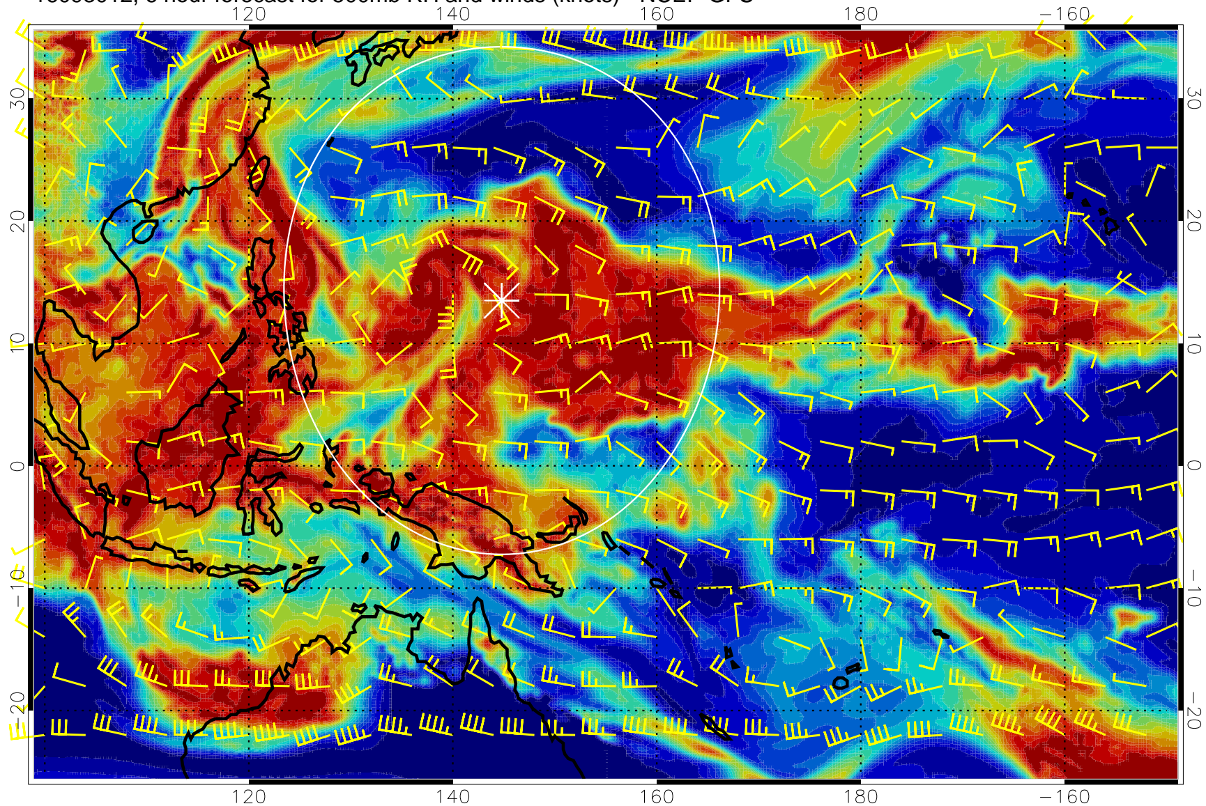
16093012, 6 hour forecast for 500mb RH and winds (knots) - NCEP GFS
