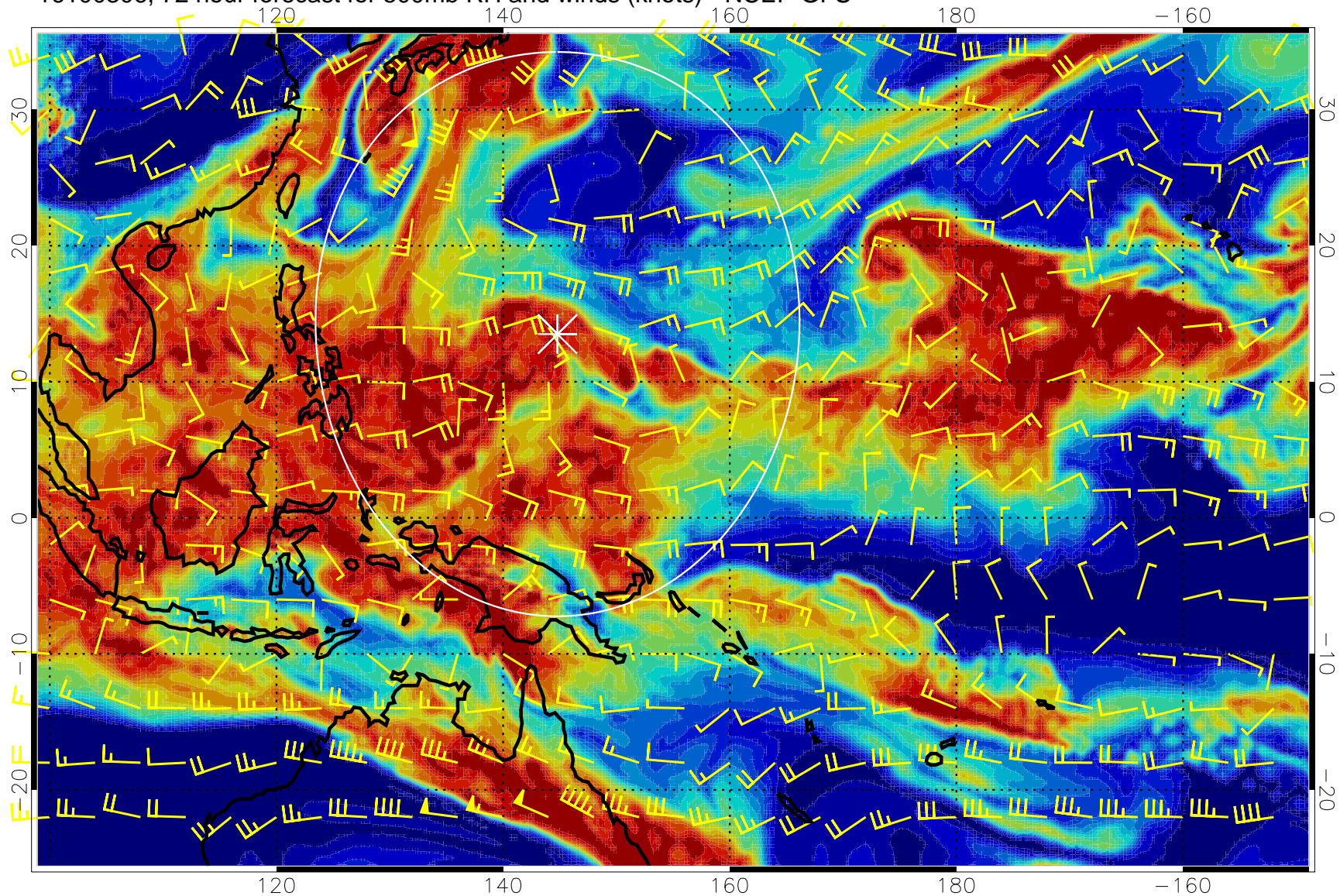
16100306, 72 hour forecast for 500mb RH and winds (knots) - NCEP GFS
