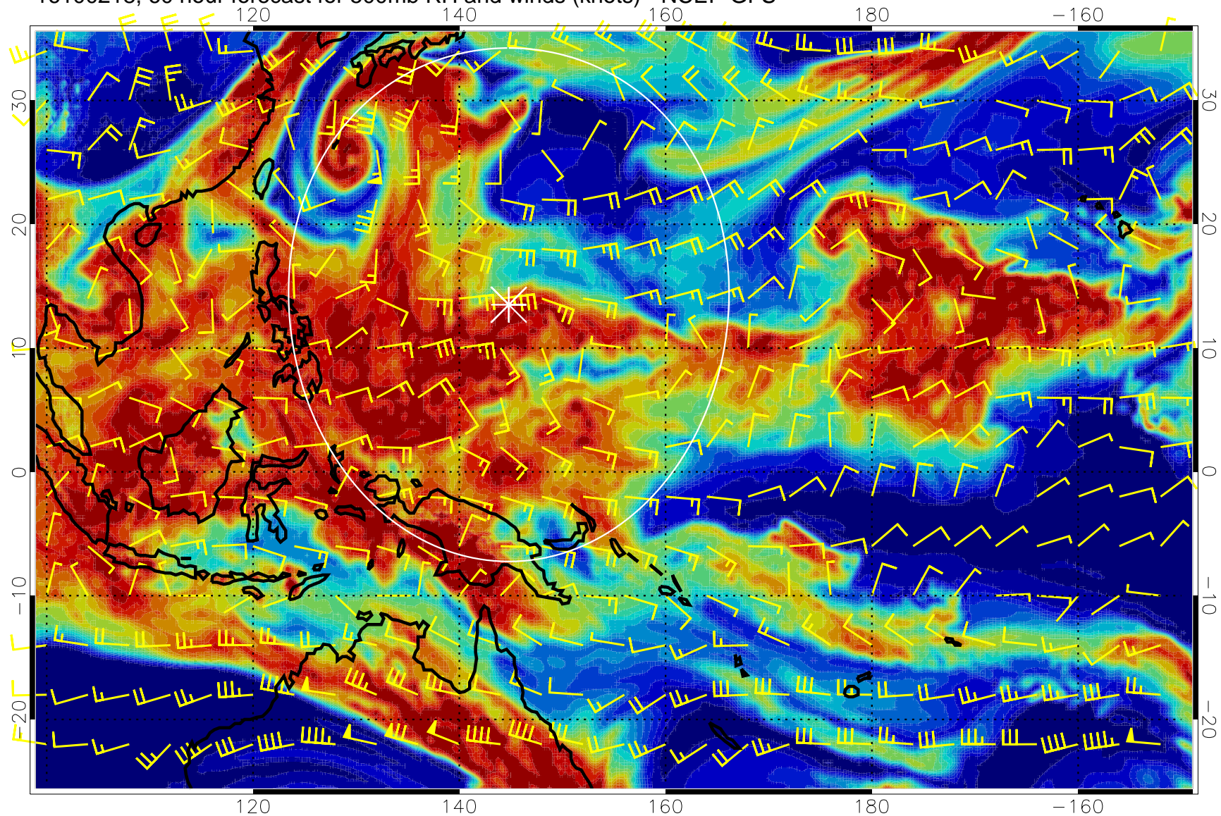
16100218, 60 hour forecast for 500mb RH and winds (knots) - NCEP GFS
