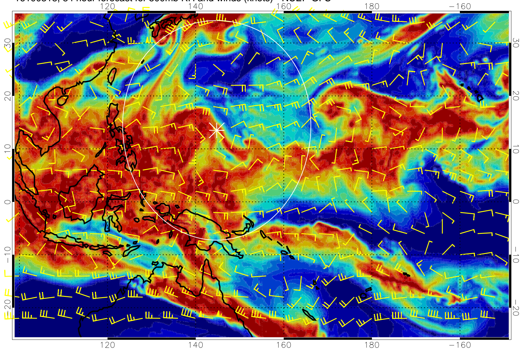
16100318, 84 hour forecast for 500mb RH and winds (knots) - NCEP GFS
