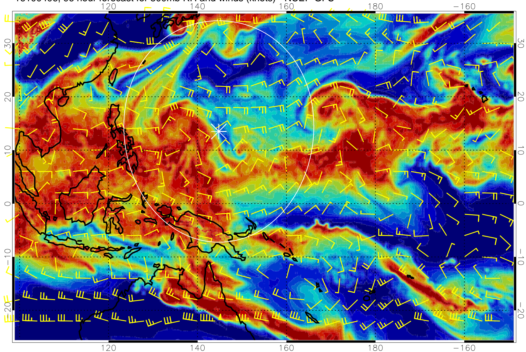
16100406, 96 hour forecast for 500mb RH and winds (knots) - NCEP GFS
