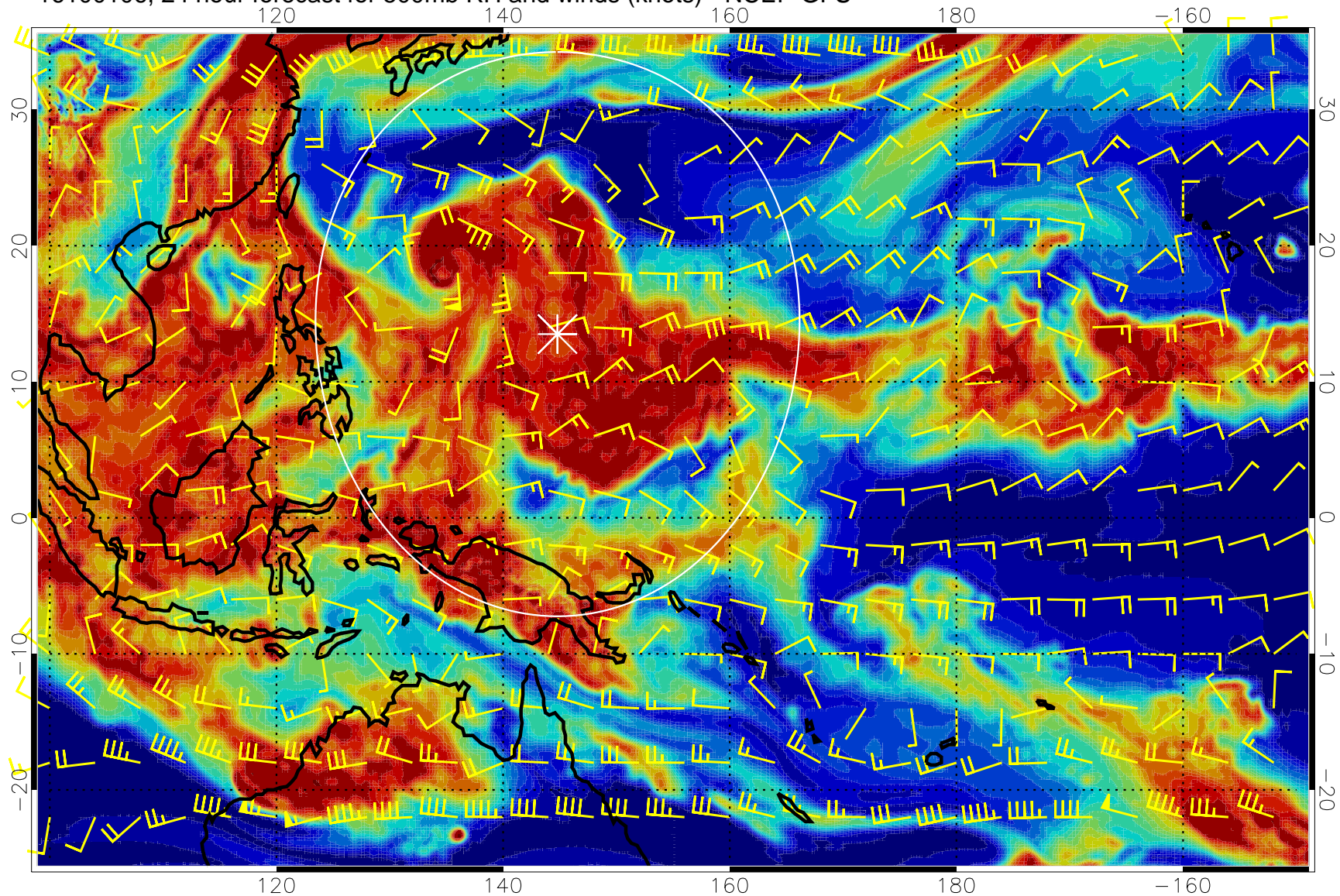
16100106, 24 hour forecast for 500mb RH and winds (knots) - NCEP GFS
