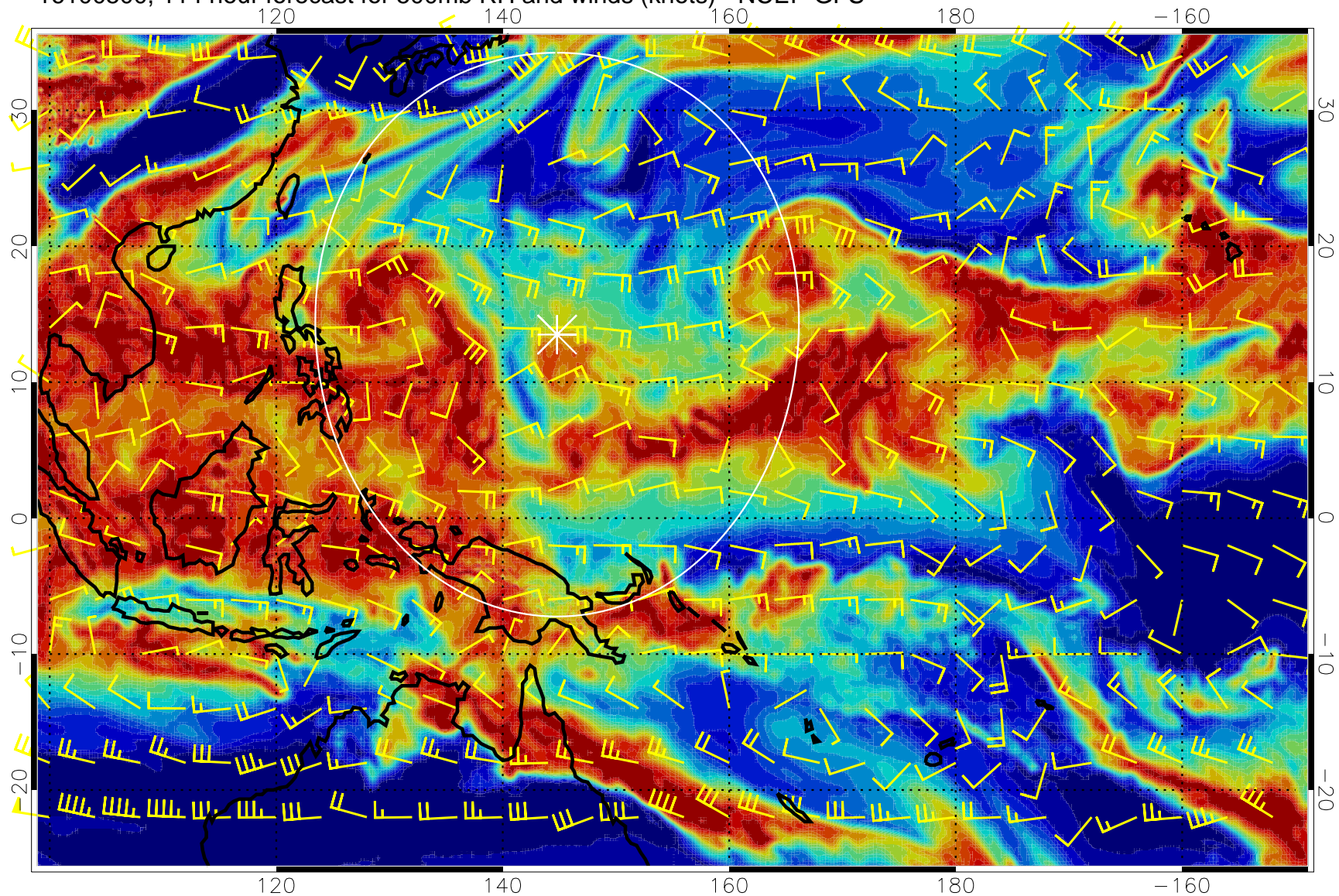
16100500, 114 hour forecast for 500mb RH and winds (knots) - NCEP GFS
