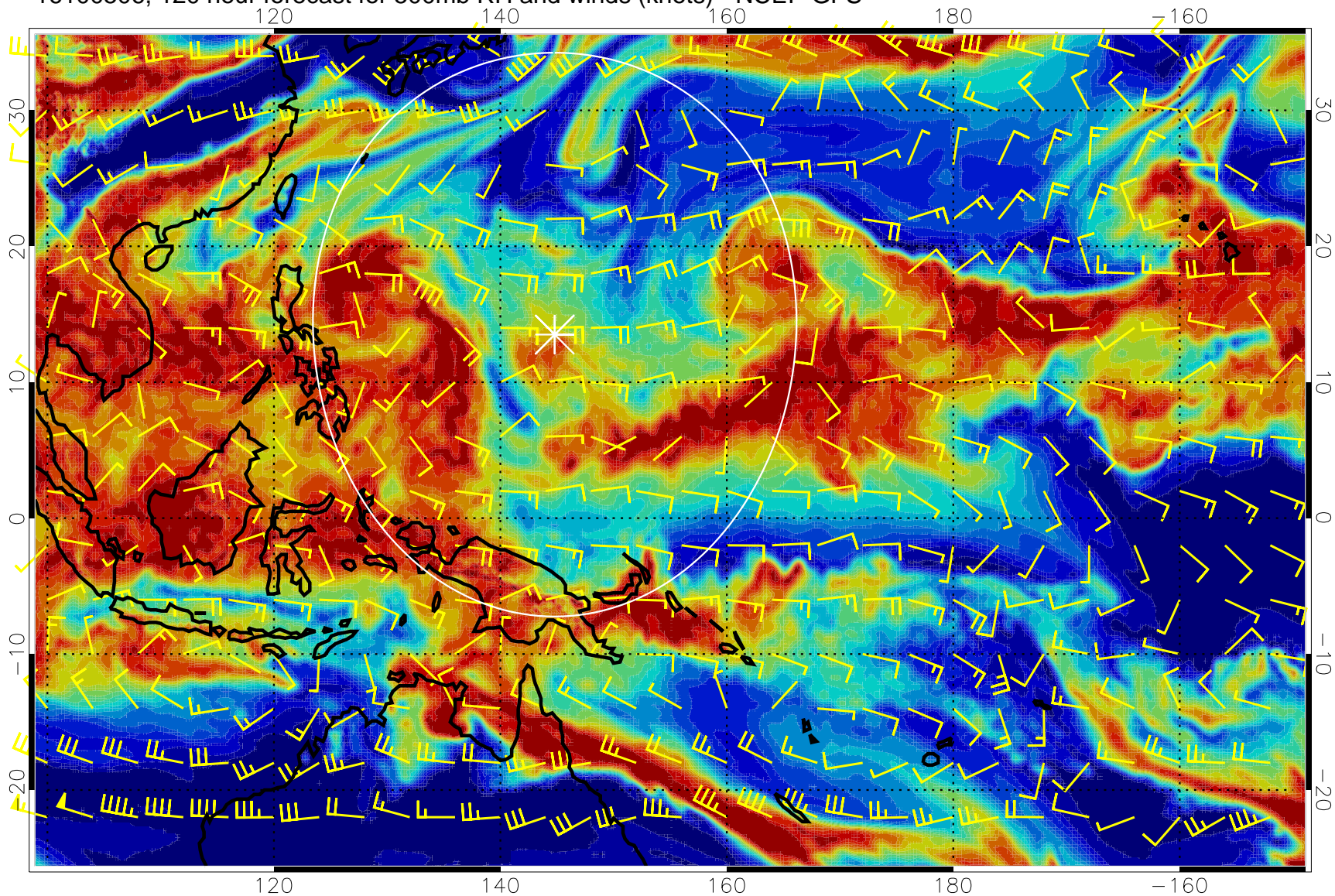
16100506, 120 hour forecast for 500mb RH and winds (knots) - NCEP GFS
