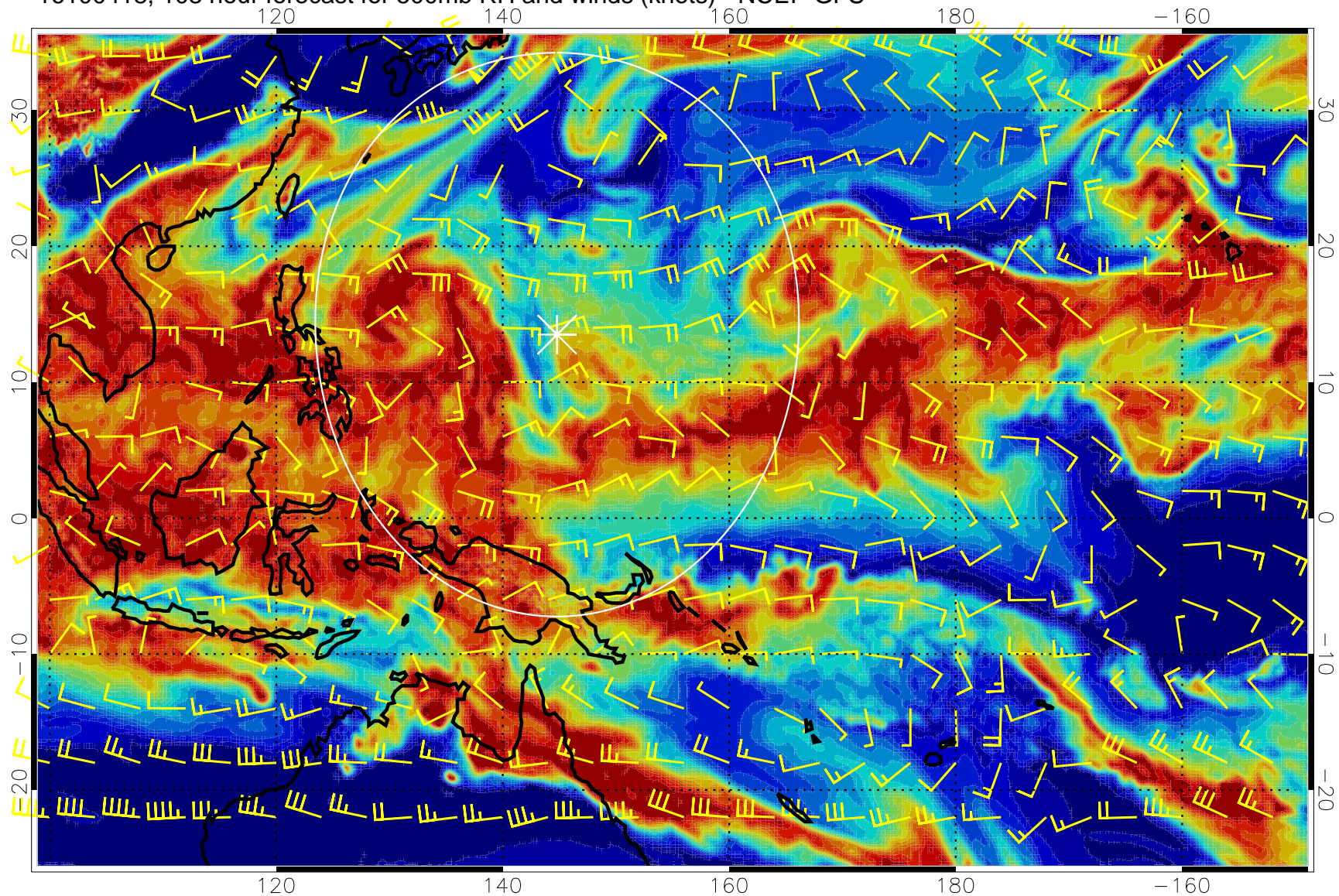
16100418, 108 hour forecast for 500mb RH and winds (knots) - NCEP GFS
