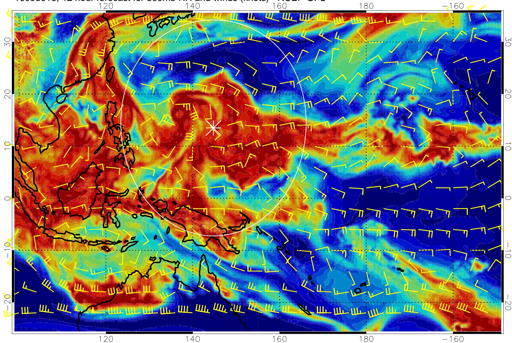
16093018, 12 hour forecast for 500mb RH and winds (knots) - NCEP GFS
