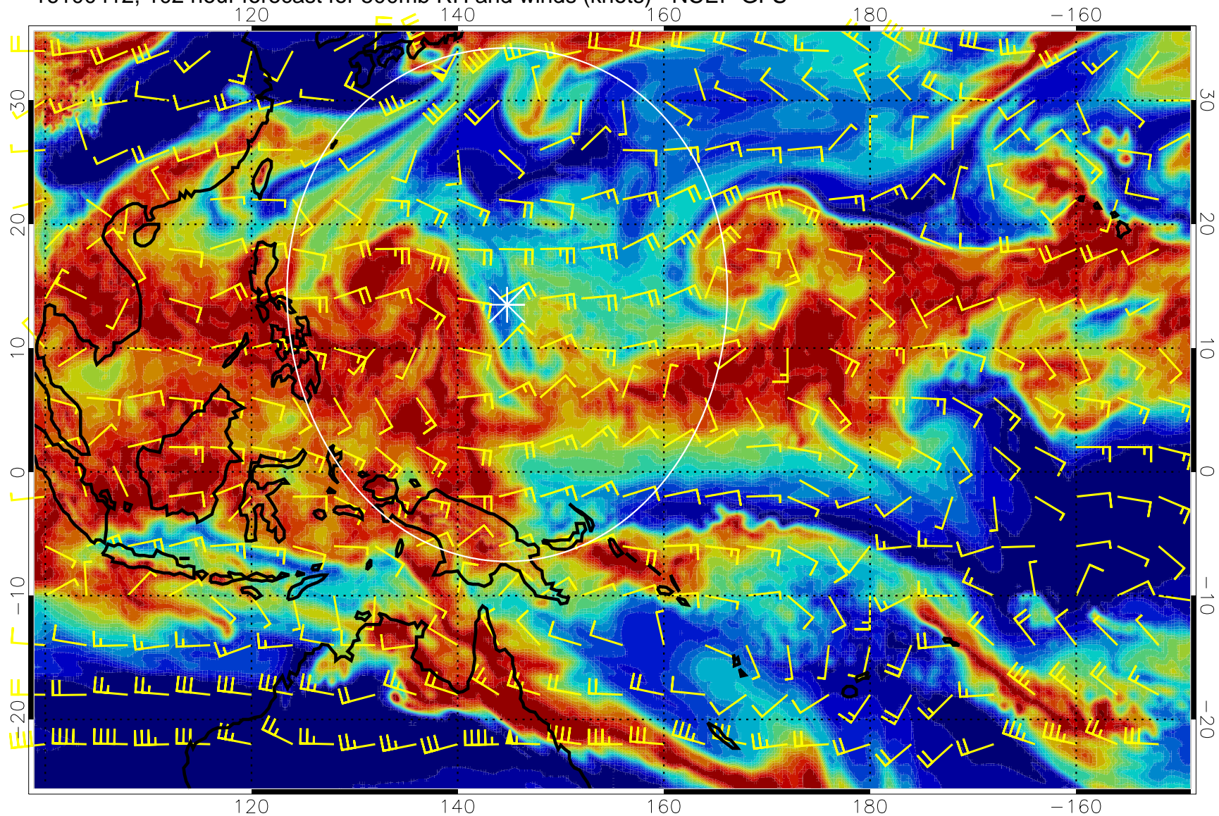
16100412, 102 hour forecast for 500mb RH and winds (knots) - NCEP GFS
