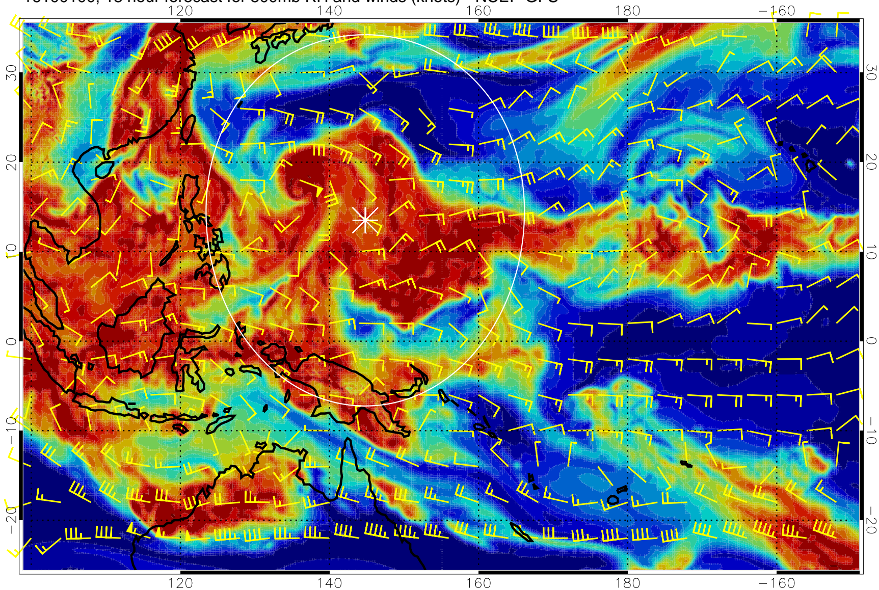
16100100, 18 hour forecast for 500mb RH and winds (knots) - NCEP GFS
