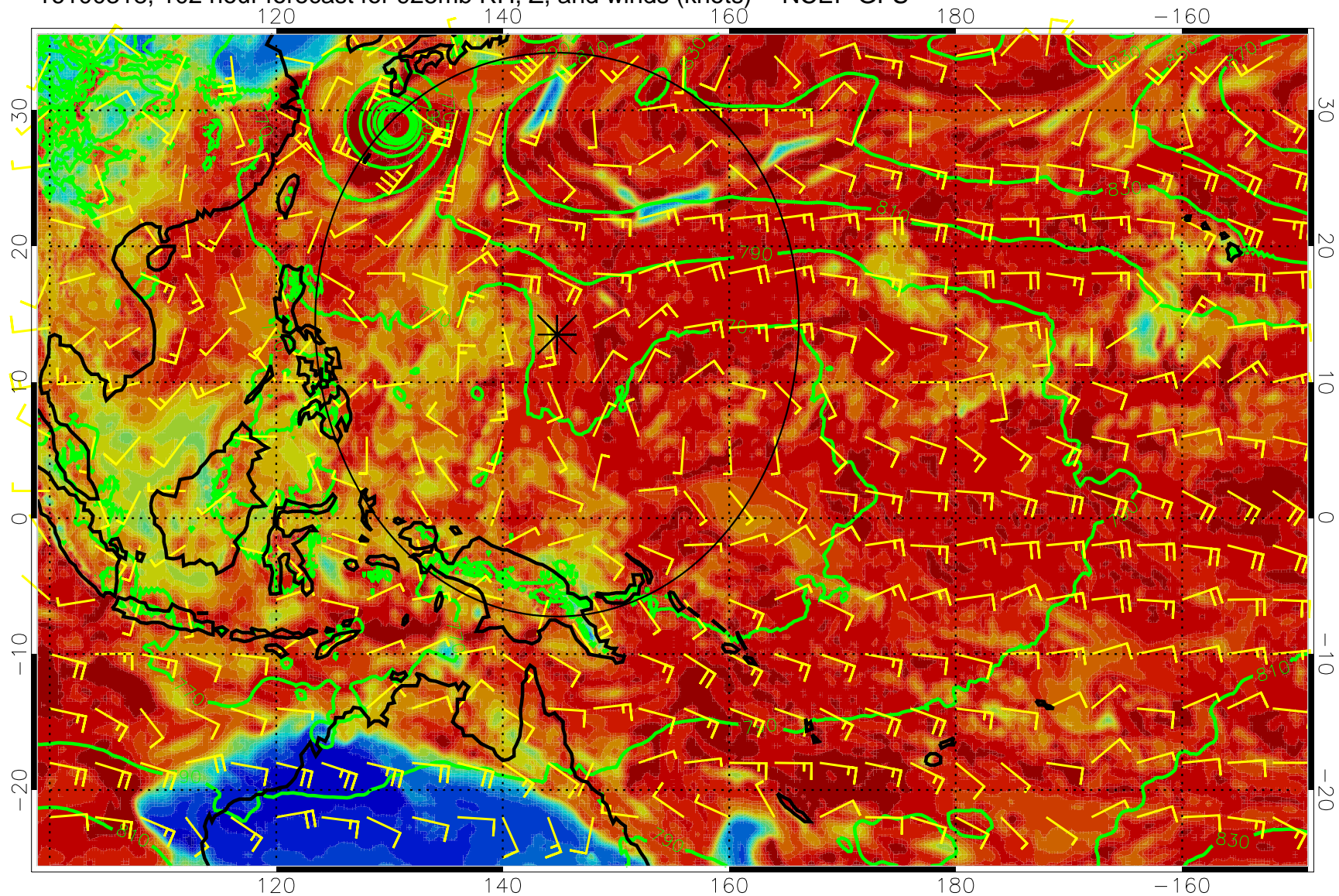
16100318, 102 hour forecast for 925mb RH, Z, and winds (knots) -- NCEP GFS
