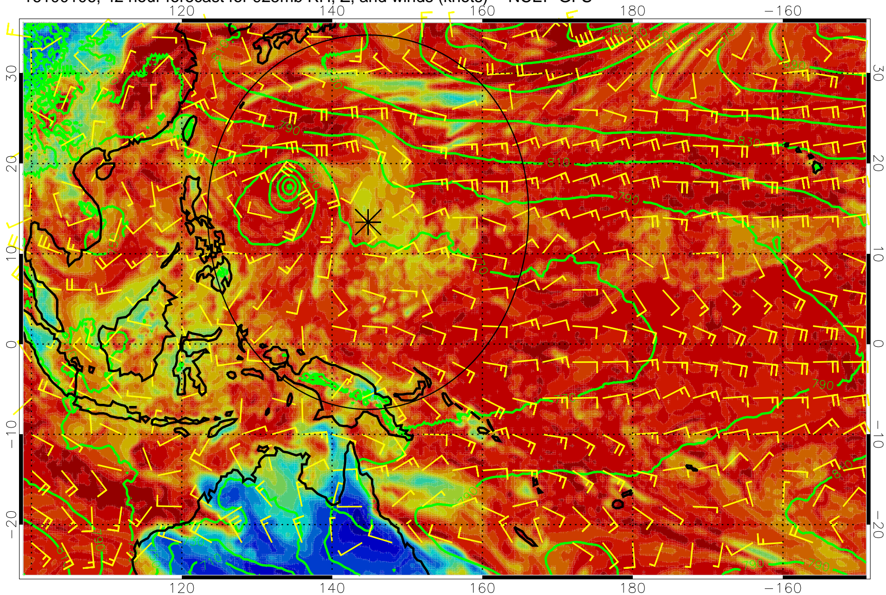
16100106, 42 hour forecast for 925mb RH, Z, and winds (knots) -- NCEP GFS
