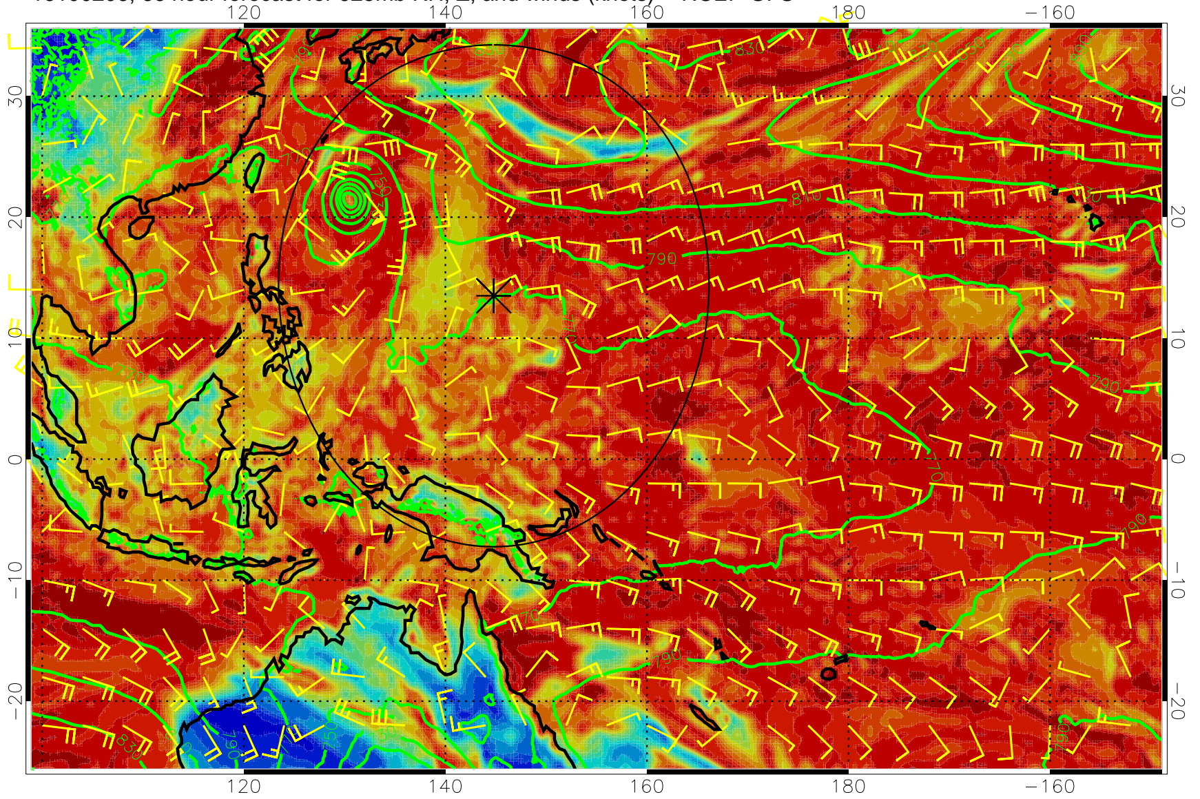
16100206, 66 hour forecast for 925mb RH, Z, and winds (knots) -- NCEP GFS
