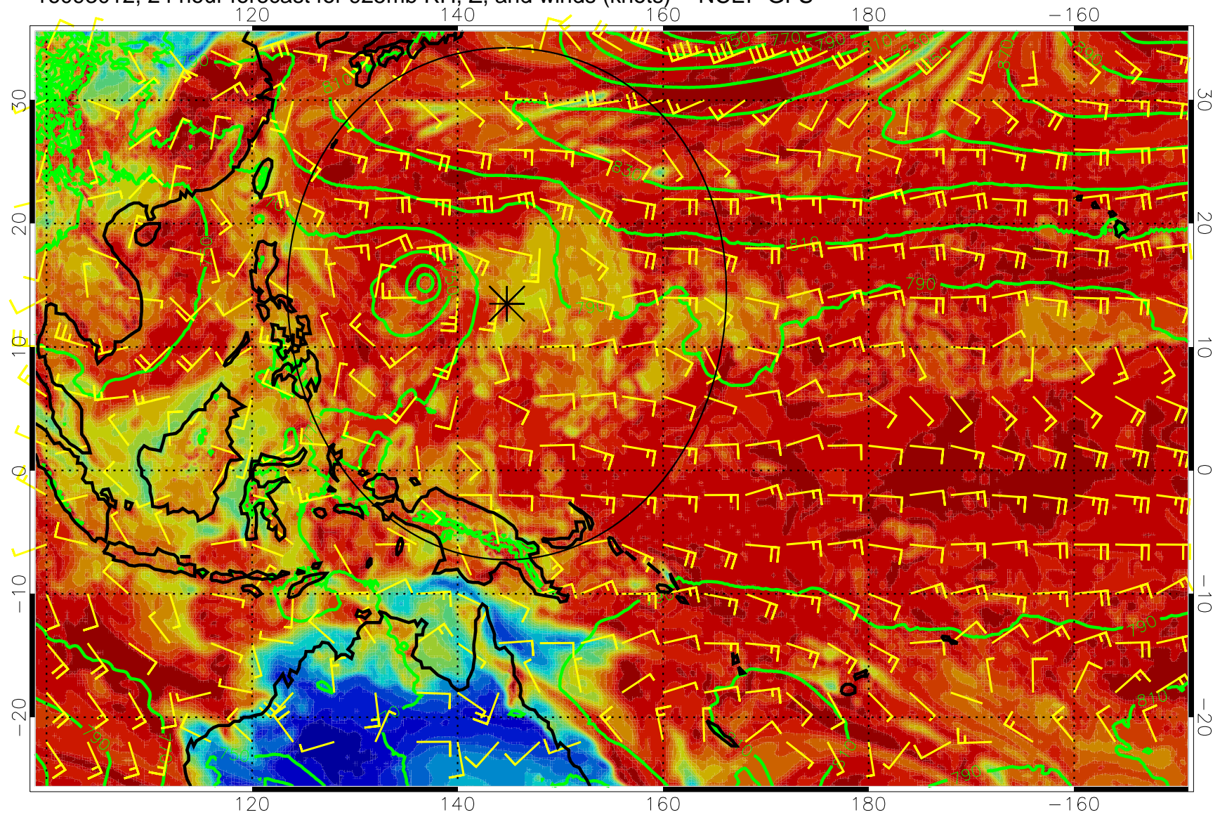
16093012, 24 hour forecast for 925mb RH, Z, and winds (knots) -- NCEP GFS
