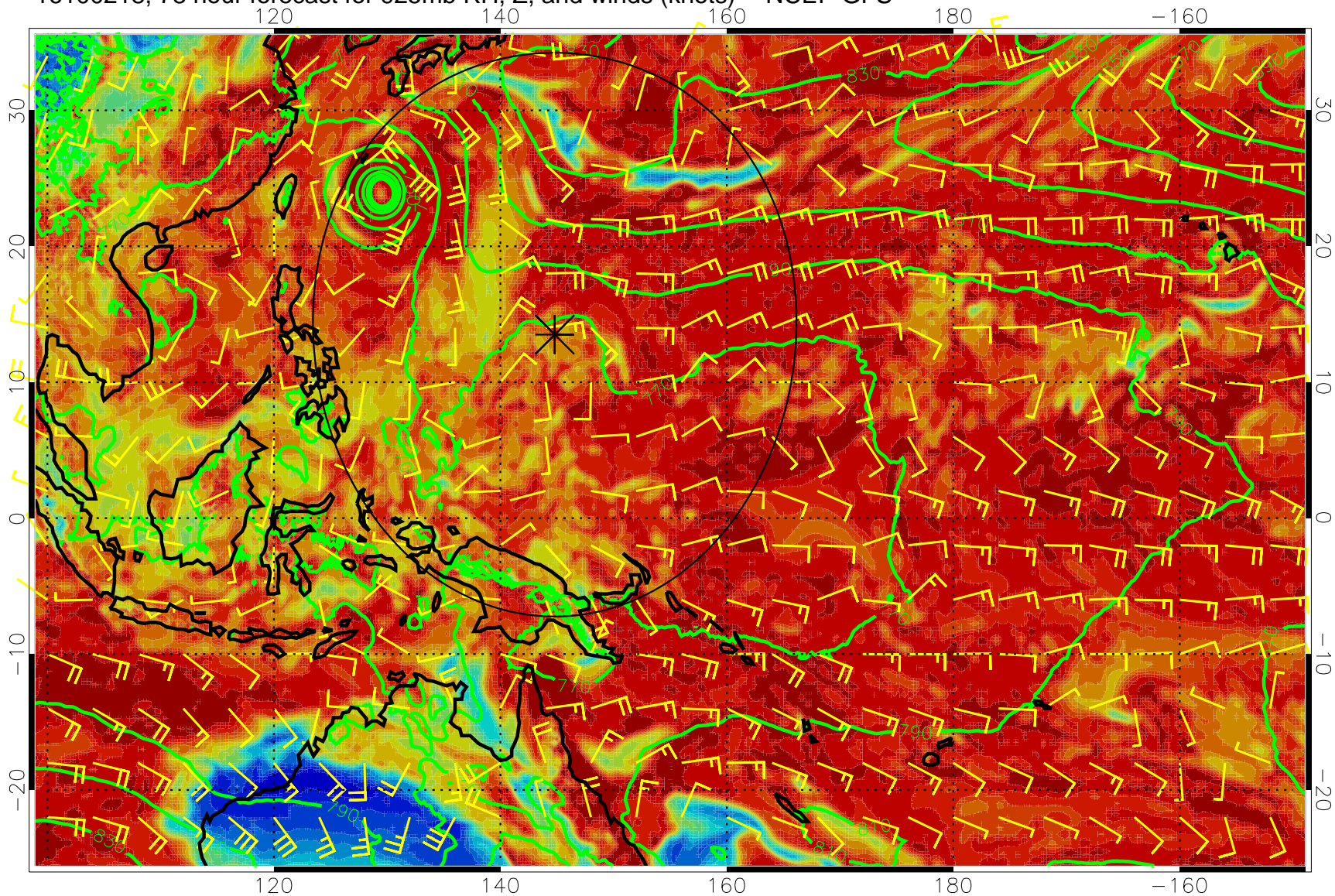
16100218, 78 hour forecast for 925mb RH, Z, and winds (knots) -- NCEP GFS
