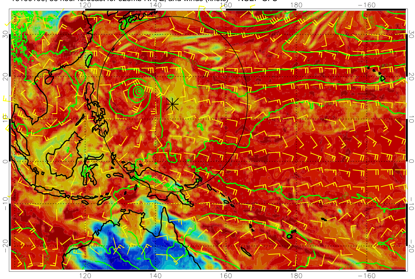
16100100, 36 hour forecast for 925mb RH, Z, and winds (knots) -- NCEP GFS
