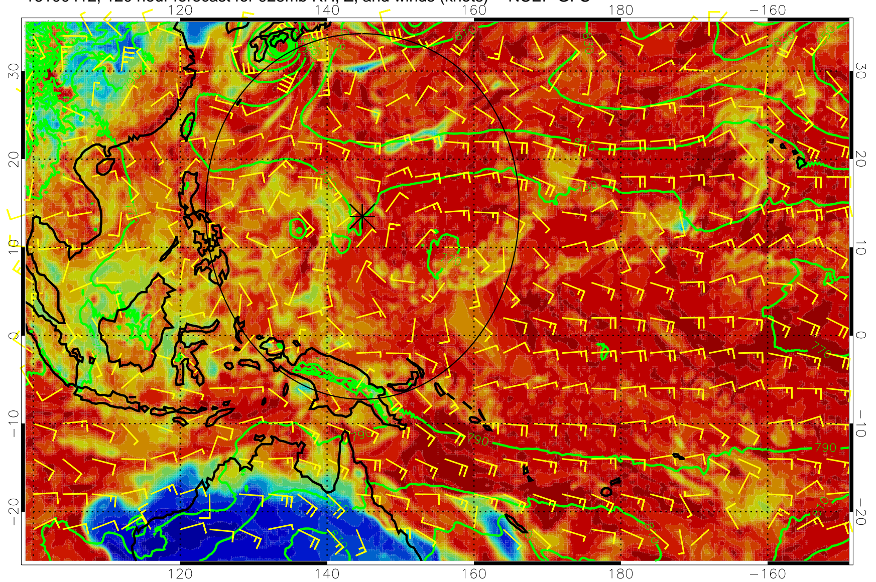
16100412, 120 hour forecast for 925mb RH, Z, and winds (knots) -- NCEP GFS
