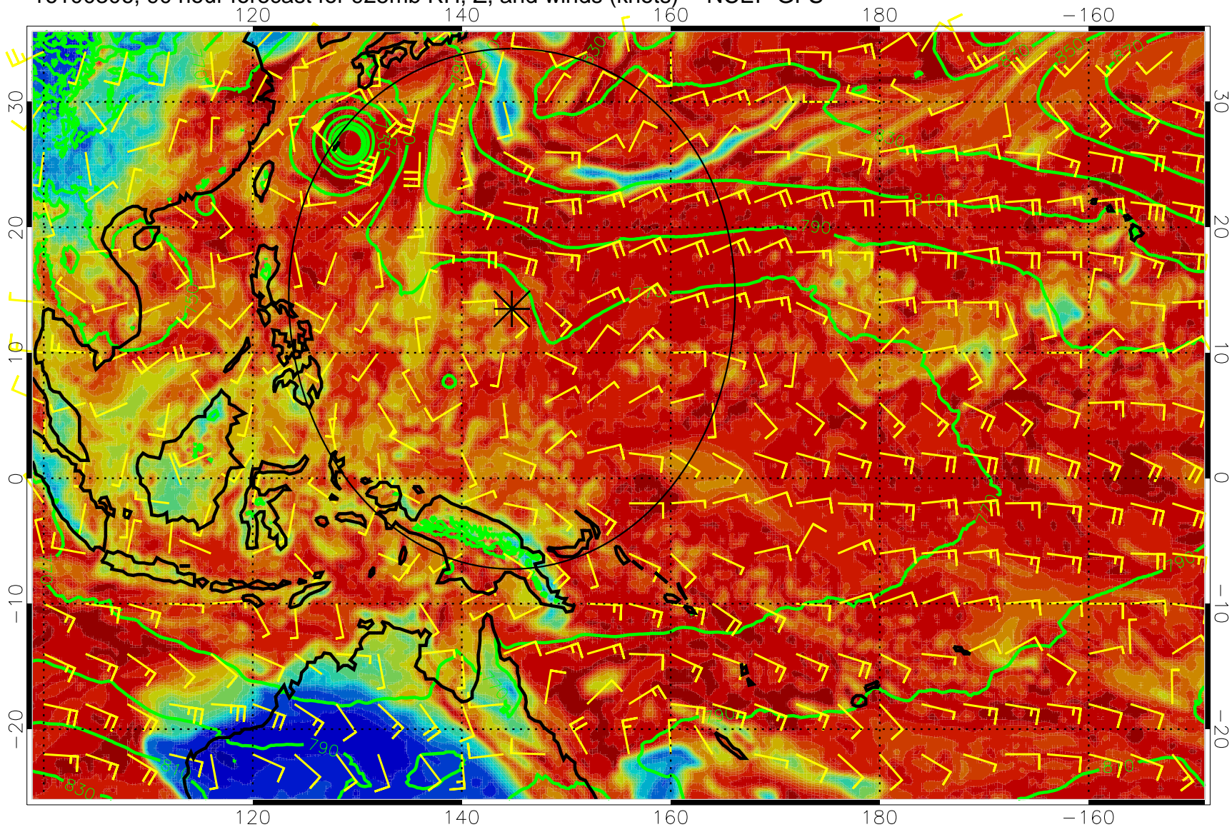
16100306, 90 hour forecast for 925mb RH, Z, and winds (knots) -- NCEP GFS
