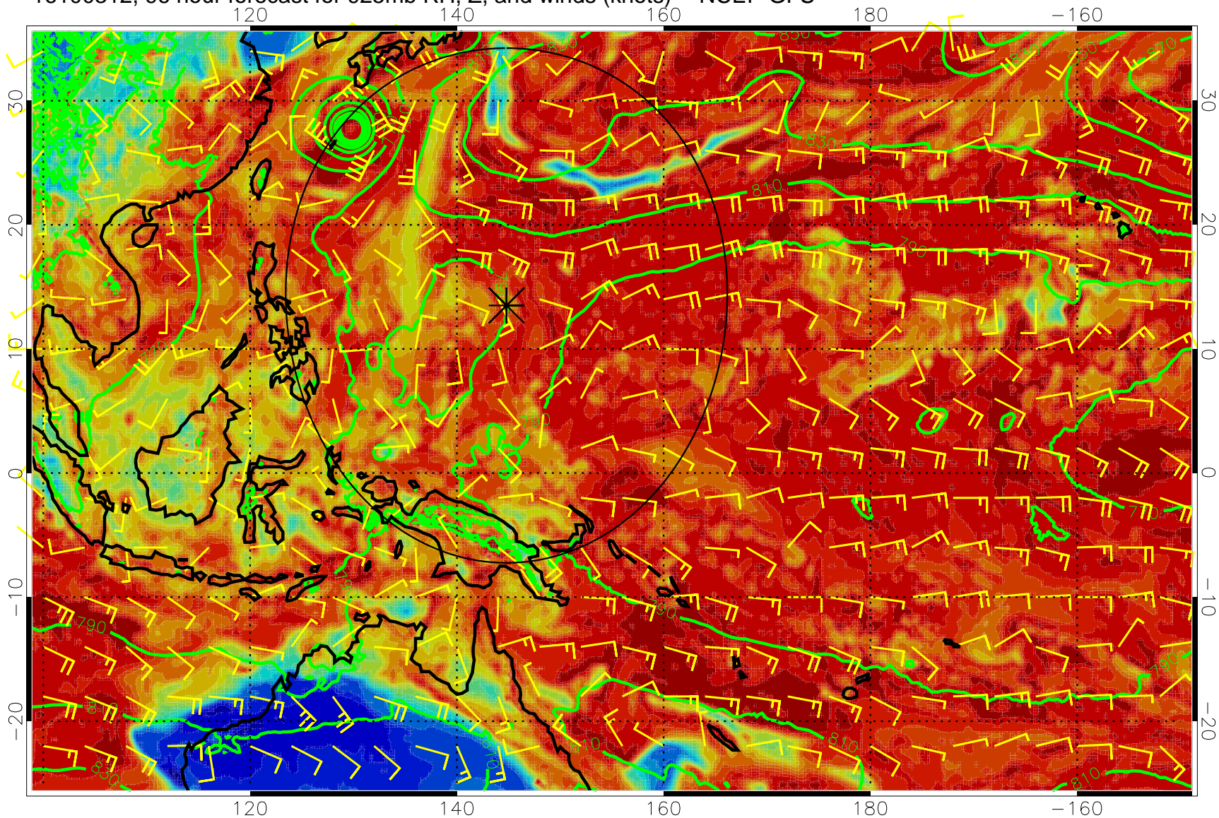
16100312, 96 hour forecast for 925mb RH, Z, and winds (knots) -- NCEP GFS
