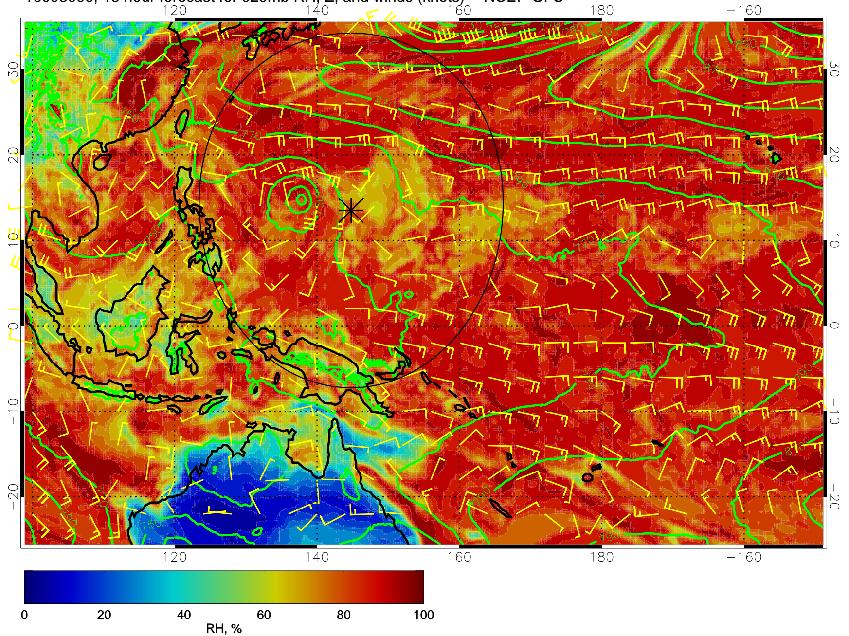
16093006, 18 hour forecast for 925mb RH, Z, and winds (knots) -- NCEP GFS
