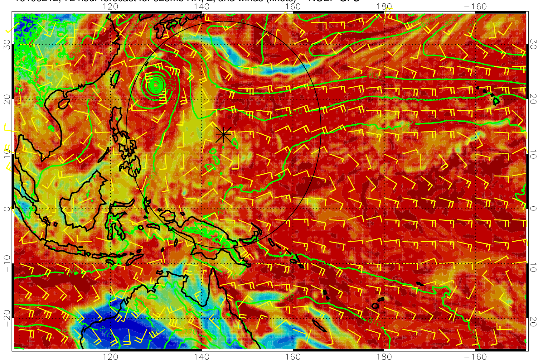
16100212, 72 hour forecast for 925mb RH, Z, and winds (knots) -- NCEP GFS
