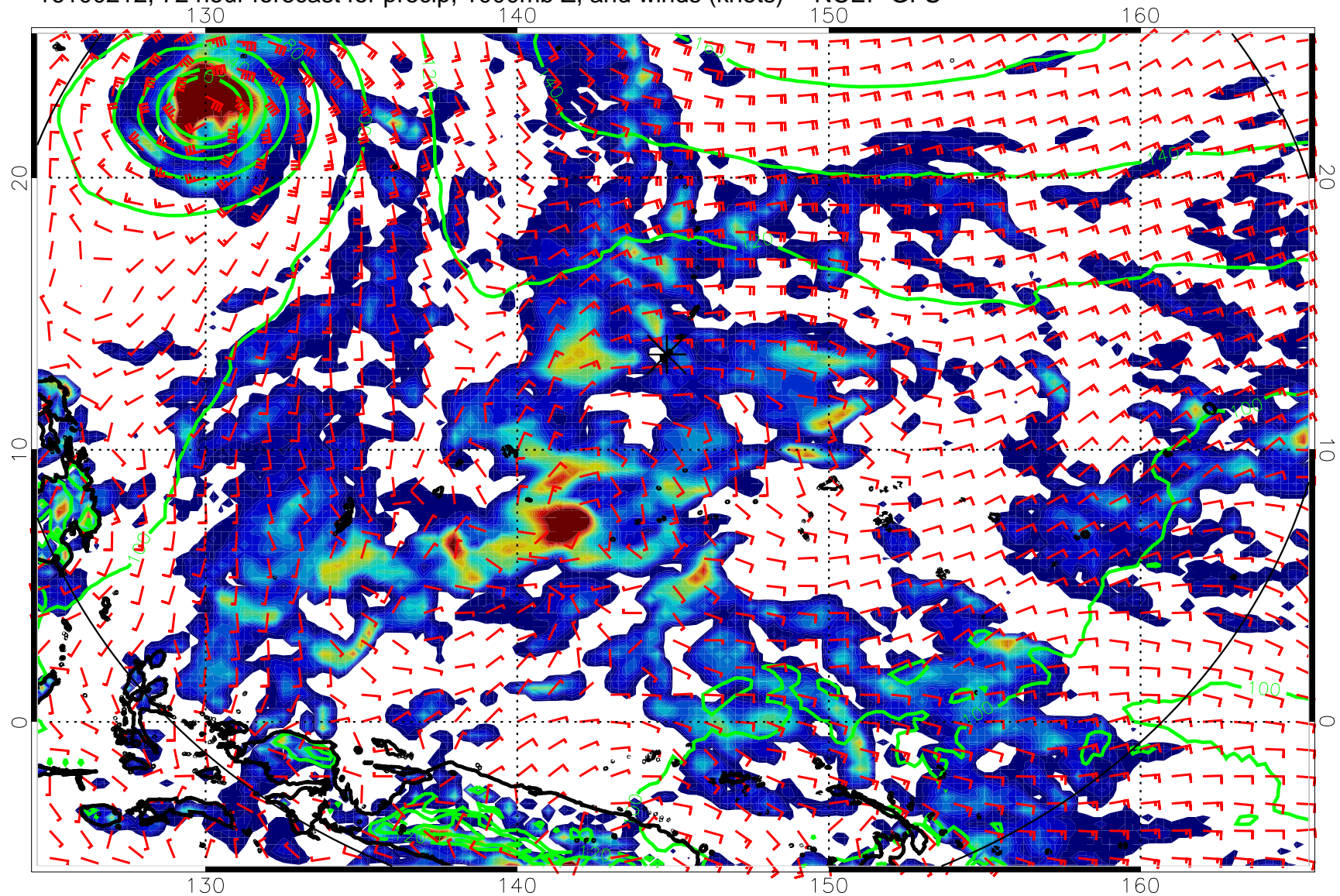
16100212, 72 hour forecast for precip, 1000mb Z, and winds (knots) -- NCEP GFS
