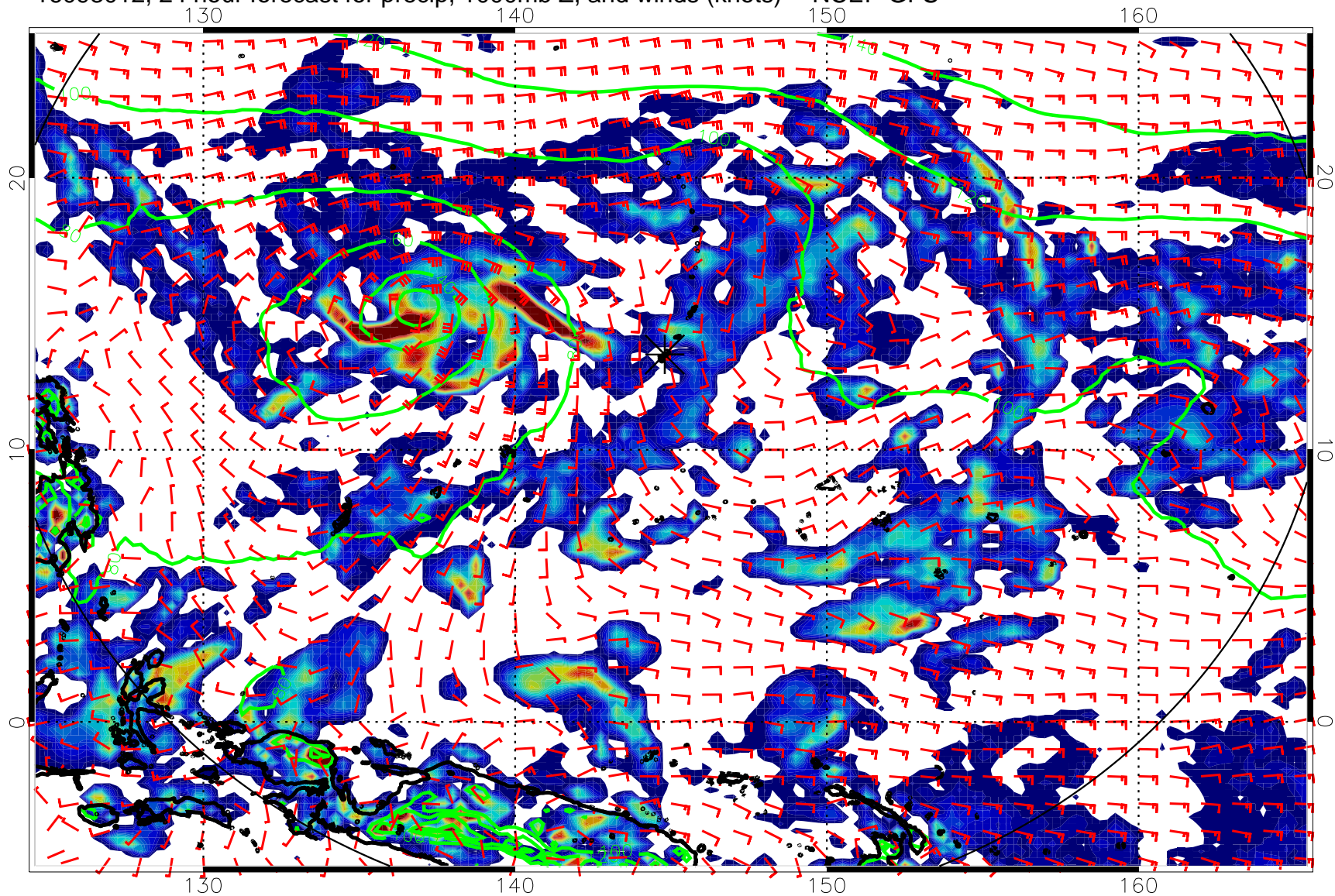
16093012, 24 hour forecast for precip, 1000mb Z, and winds (knots) -- NCEP GFS
