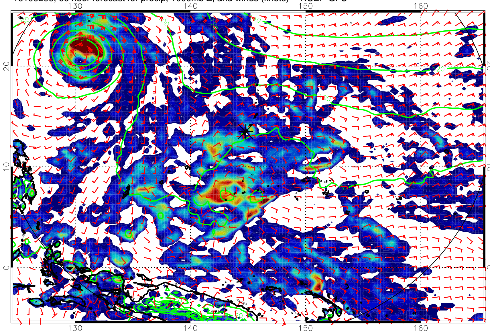
16100206, 66 hour forecast for precip, 1000mb Z, and winds (knots) -- NCEP GFS
