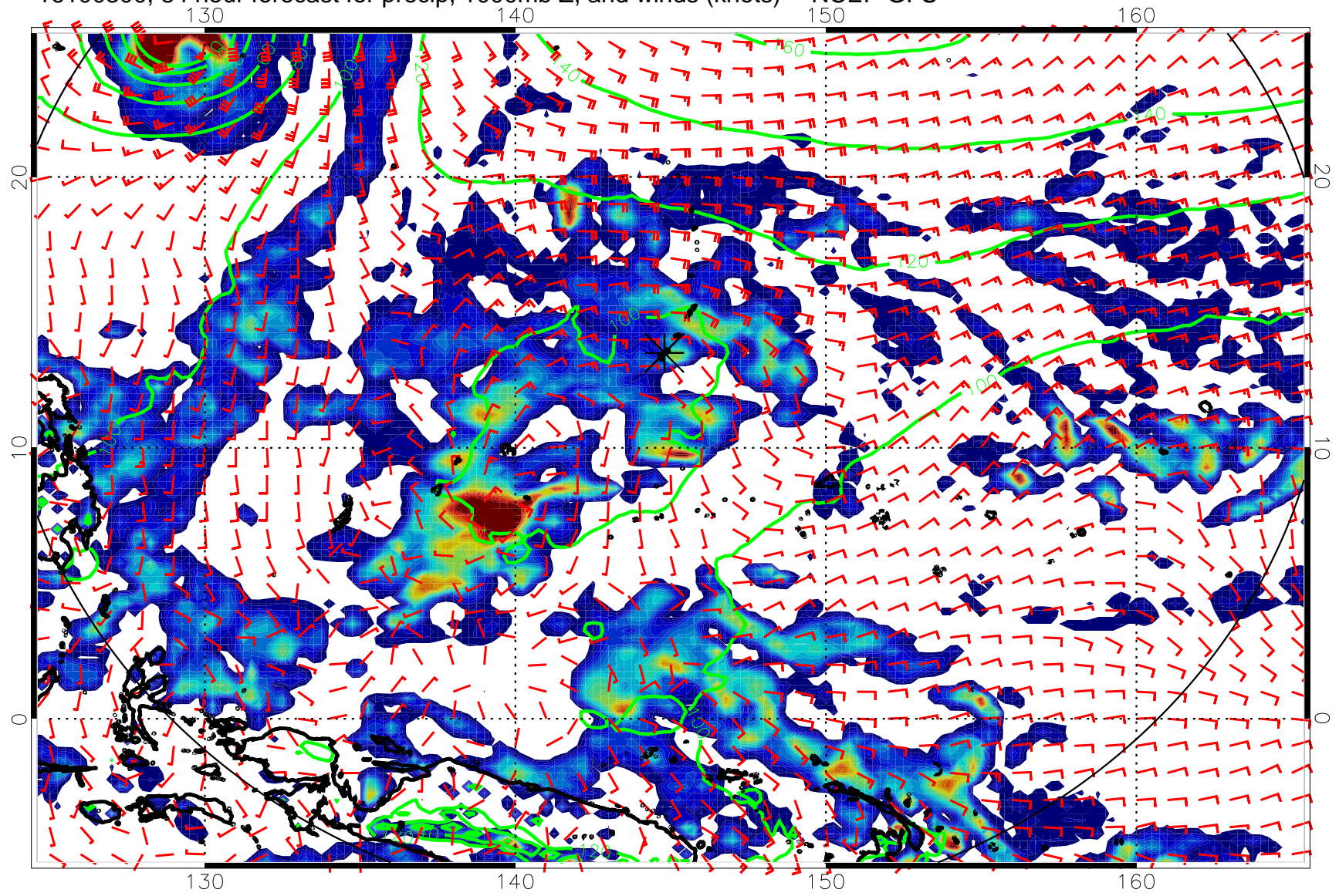
16100300, 84 hour forecast for precip, 1000mb Z, and winds (knots) -- NCEP GFS
