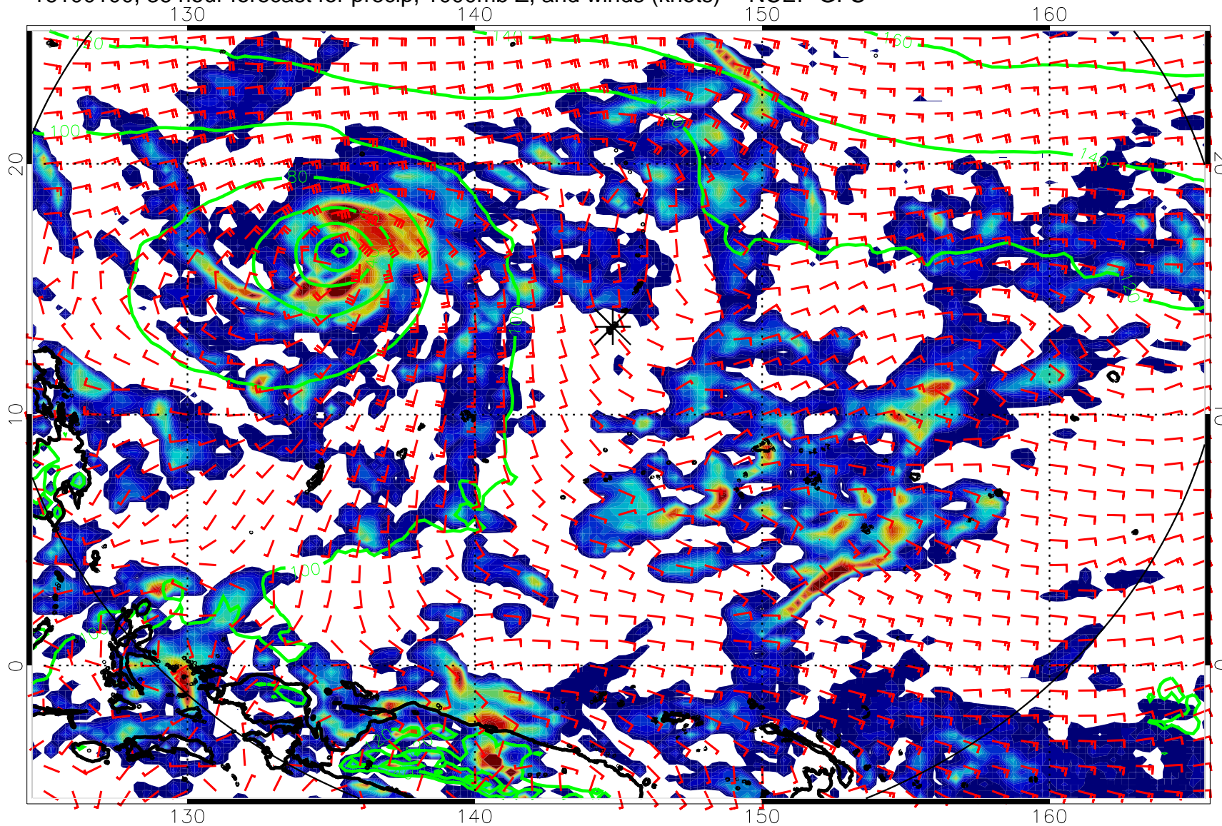
16100100, 36 hour forecast for precip, 1000mb Z, and winds (knots) -- NCEP GFS
