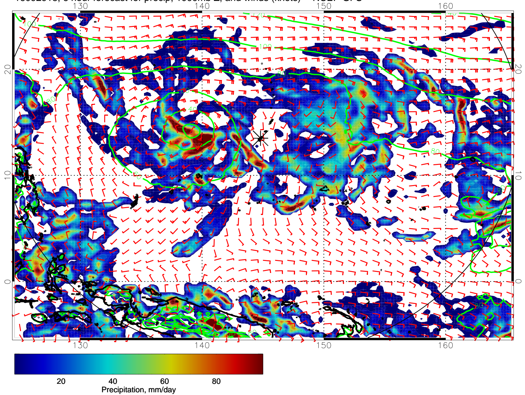
16092918, 6 hour forecast for precip, 1000mb Z, and winds (knots) -- NCEP GFS
