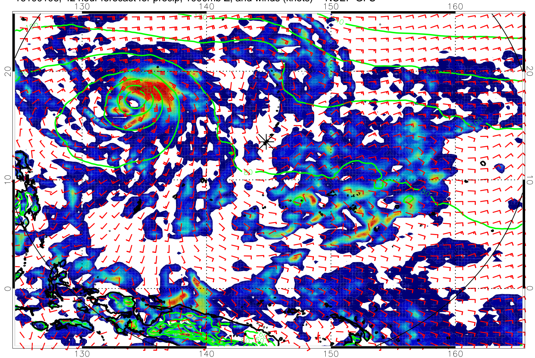
16100106, 42 hour forecast for precip, 1000mb Z, and winds (knots) -- NCEP GFS
