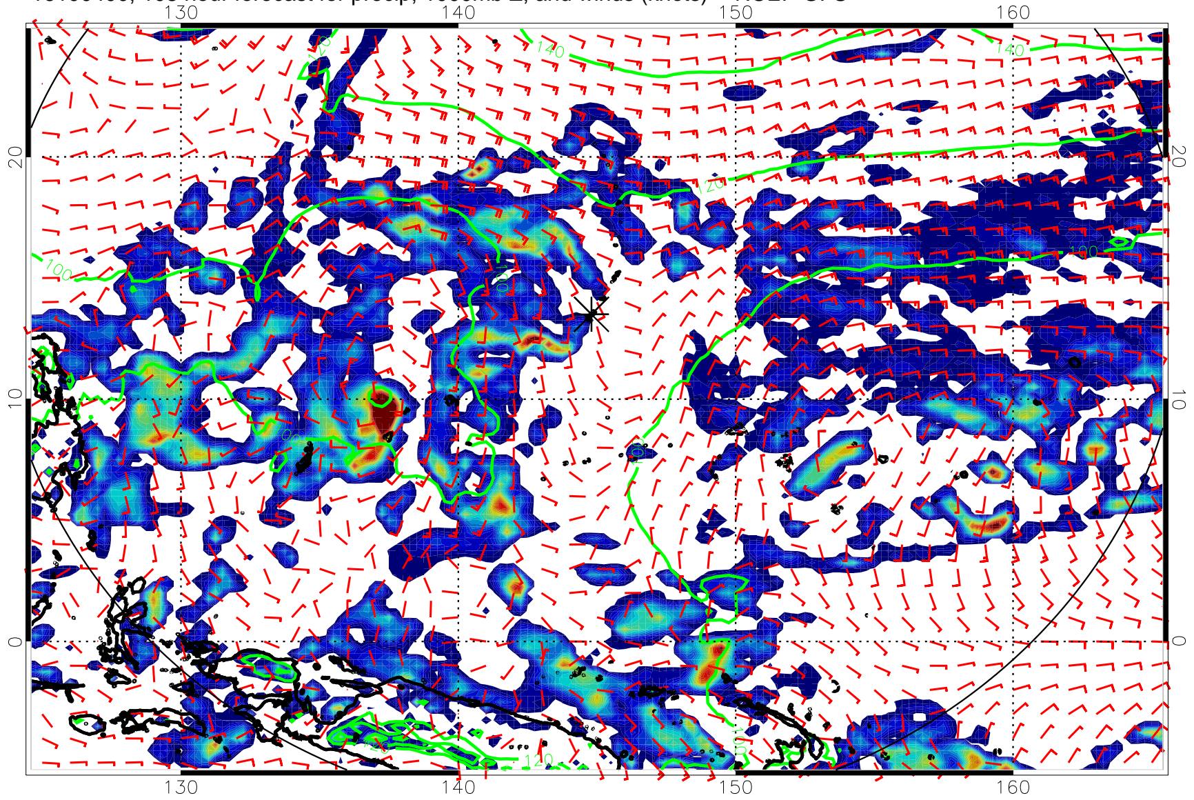
16100400, 108 hour forecast for precip, 1000mb Z, and winds (knots) -- NCEP GFS
