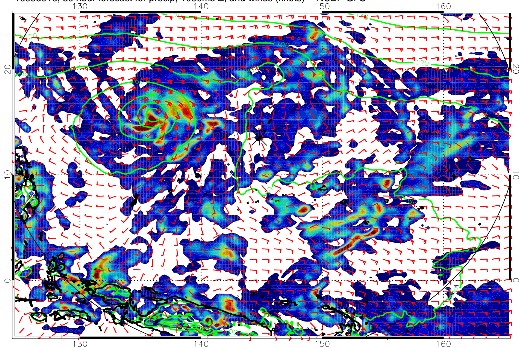
16093018, 30 hour forecast for precip, 1000mb Z, and winds (knots) -- NCEP GFS
