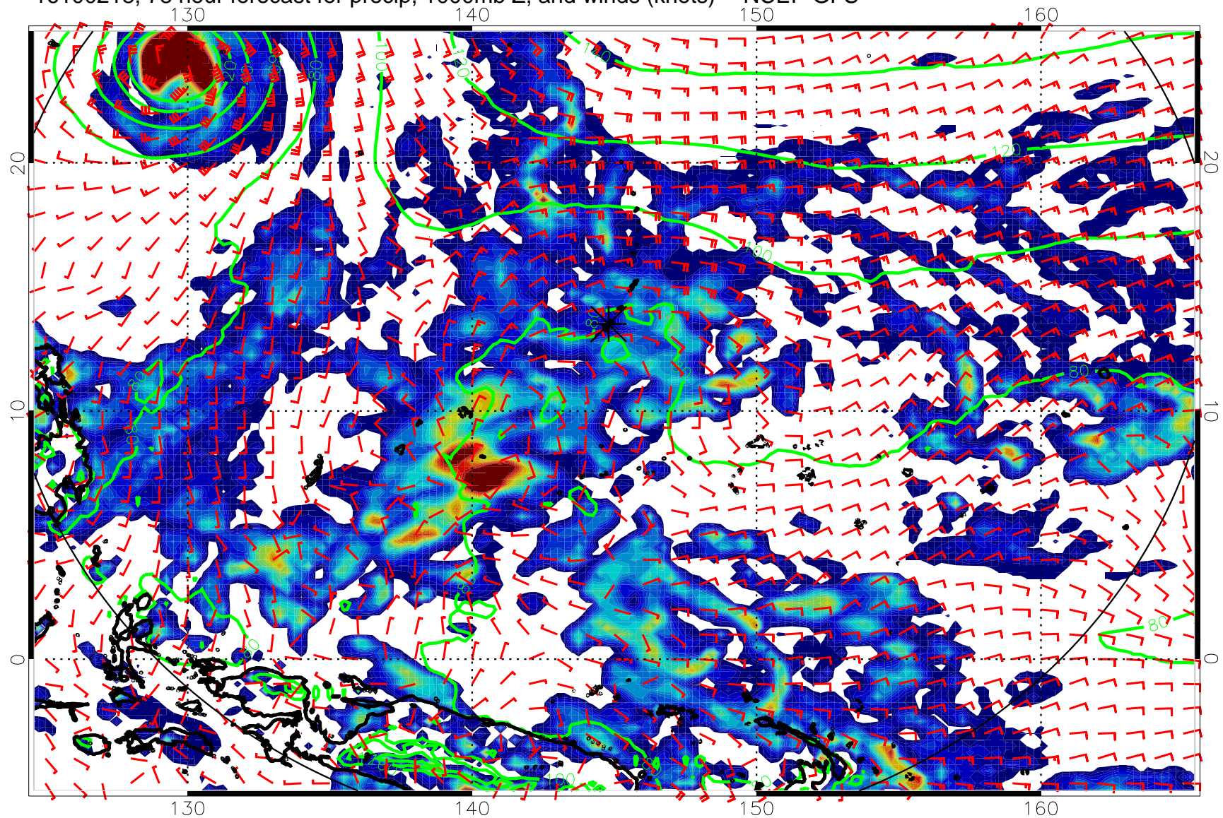
16100218, 78 hour forecast for precip, 1000mb Z, and winds (knots) -- NCEP GFS
