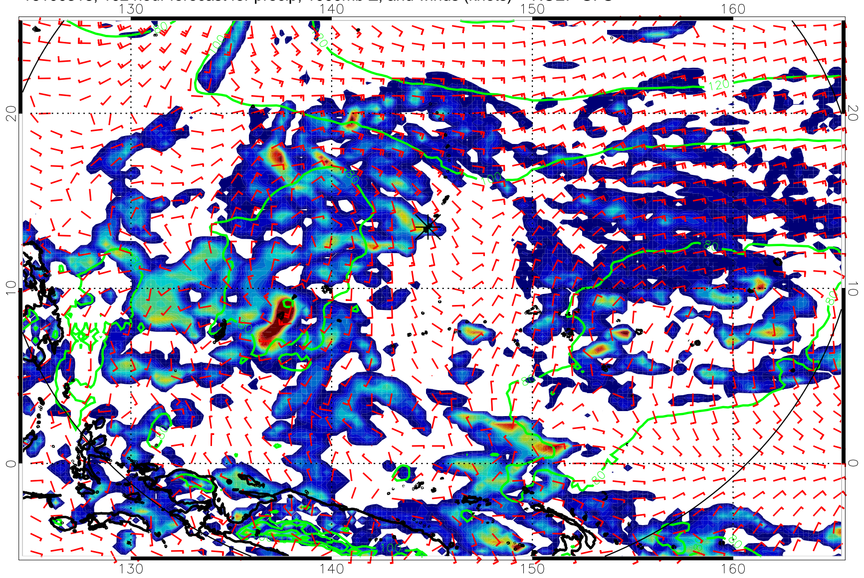
16100318, 102 hour forecast for precip, 1000mb Z, and winds (knots) -- NCEP GFS
