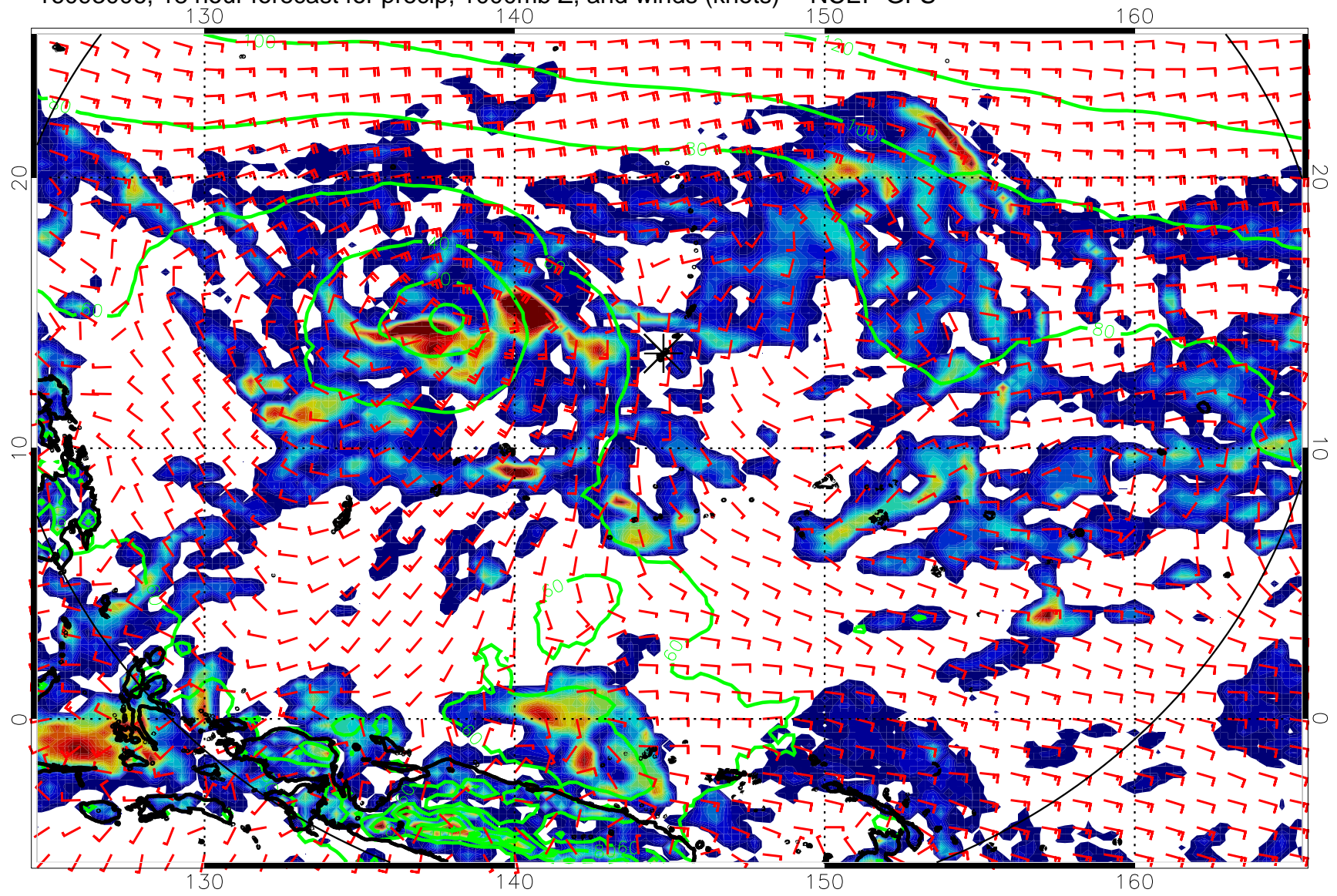
16093006, 18 hour forecast for precip, 1000mb Z, and winds (knots) -- NCEP GFS
