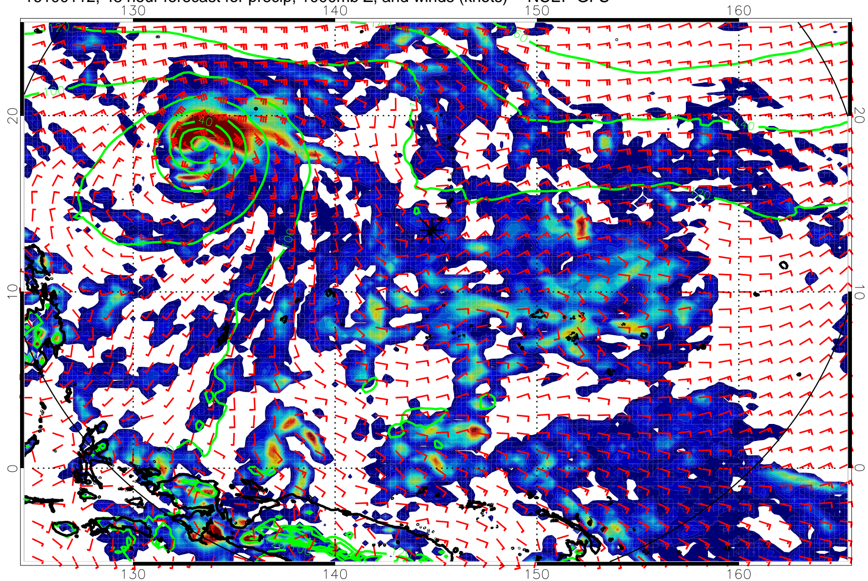
16100112, 48 hour forecast for precip, 1000mb Z, and winds (knots) -- NCEP GFS
