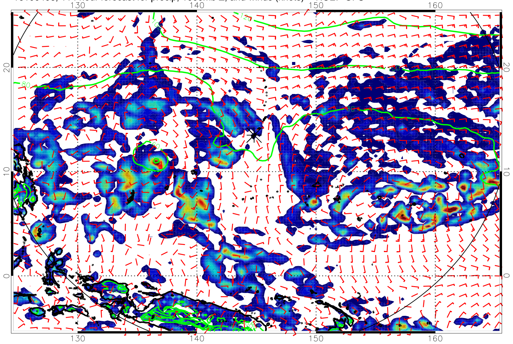
16100406, 114 hour forecast for precip, 1000mb Z, and winds (knots) -- NCEP GFS
