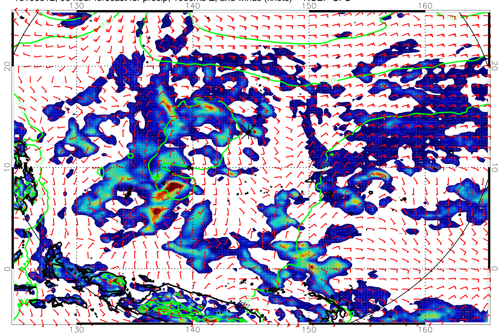
16100312, 96 hour forecast for precip, 1000mb Z, and winds (knots) -- NCEP GFS
