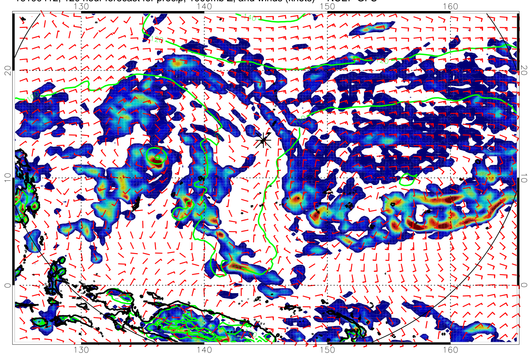
16100412, 120 hour forecast for precip, 1000mb Z, and winds (knots) -- NCEP GFS
