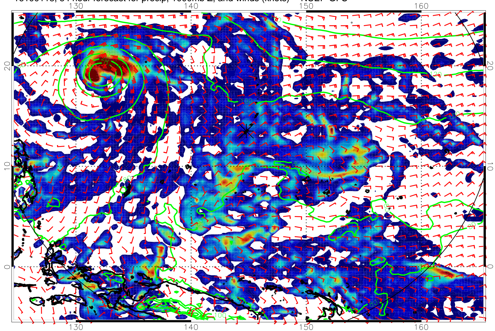
16100118, 54 hour forecast for precip, 1000mb Z, and winds (knots) -- NCEP GFS
