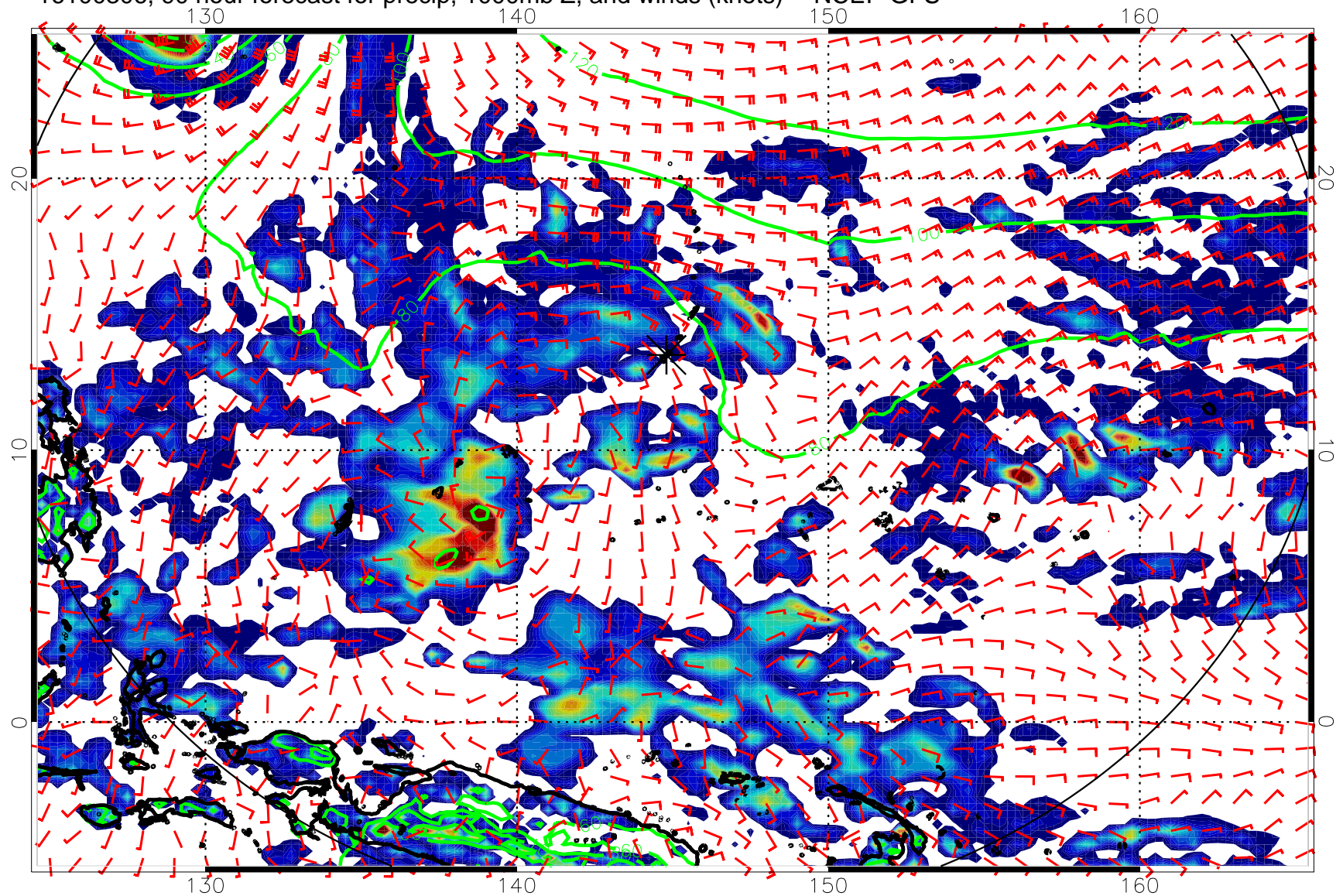
16100306, 90 hour forecast for precip, 1000mb Z, and winds (knots) -- NCEP GFS
