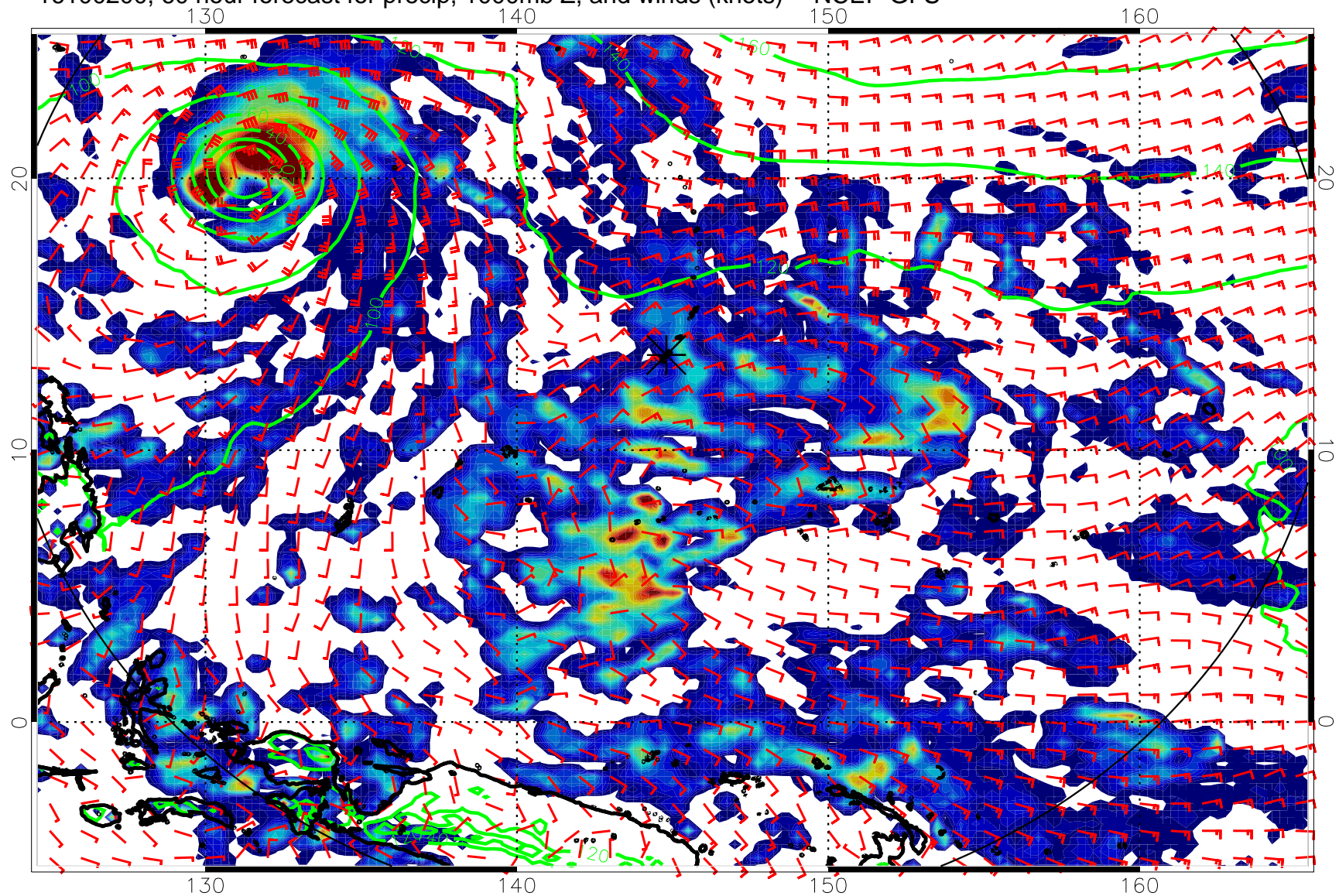
16100200, 60 hour forecast for precip, 1000mb Z, and winds (knots) -- NCEP GFS
