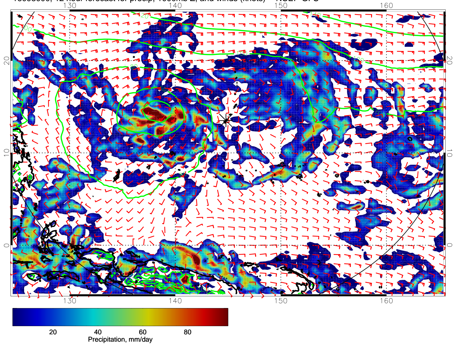
16093000, 12 hour forecast for precip, 1000mb Z, and winds (knots) -- NCEP GFS
