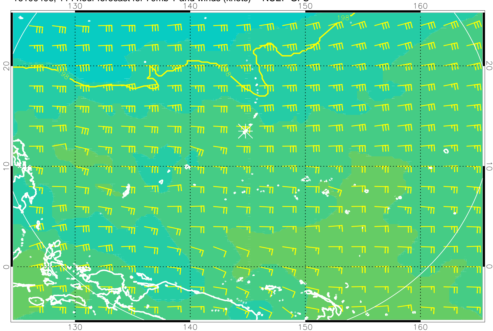
16100406, 114 hour forecast for 70mb T and winds (knots) -- NCEP GFS
