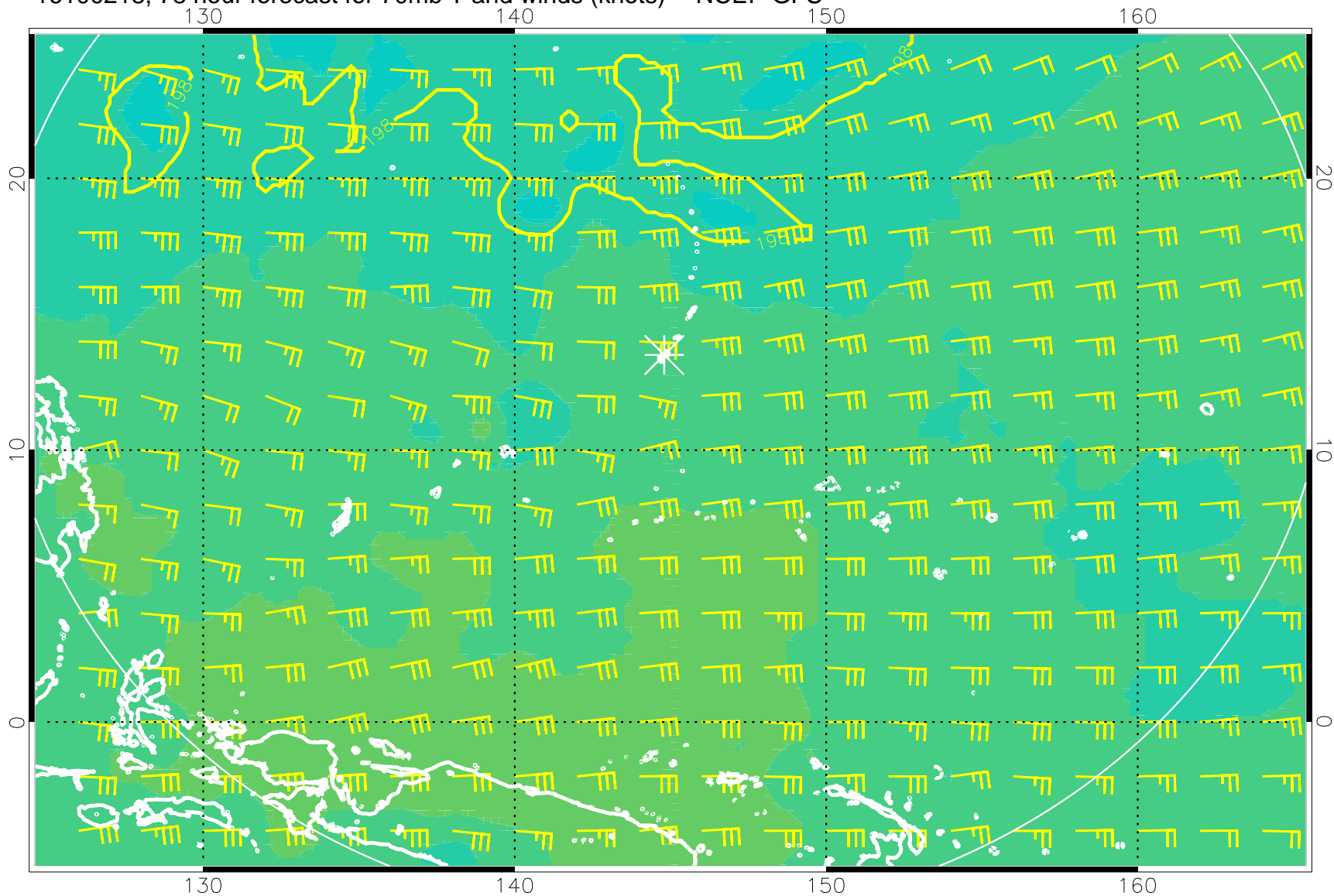
16100218, 78 hour forecast for 70mb T and winds (knots) -- NCEP GFS
