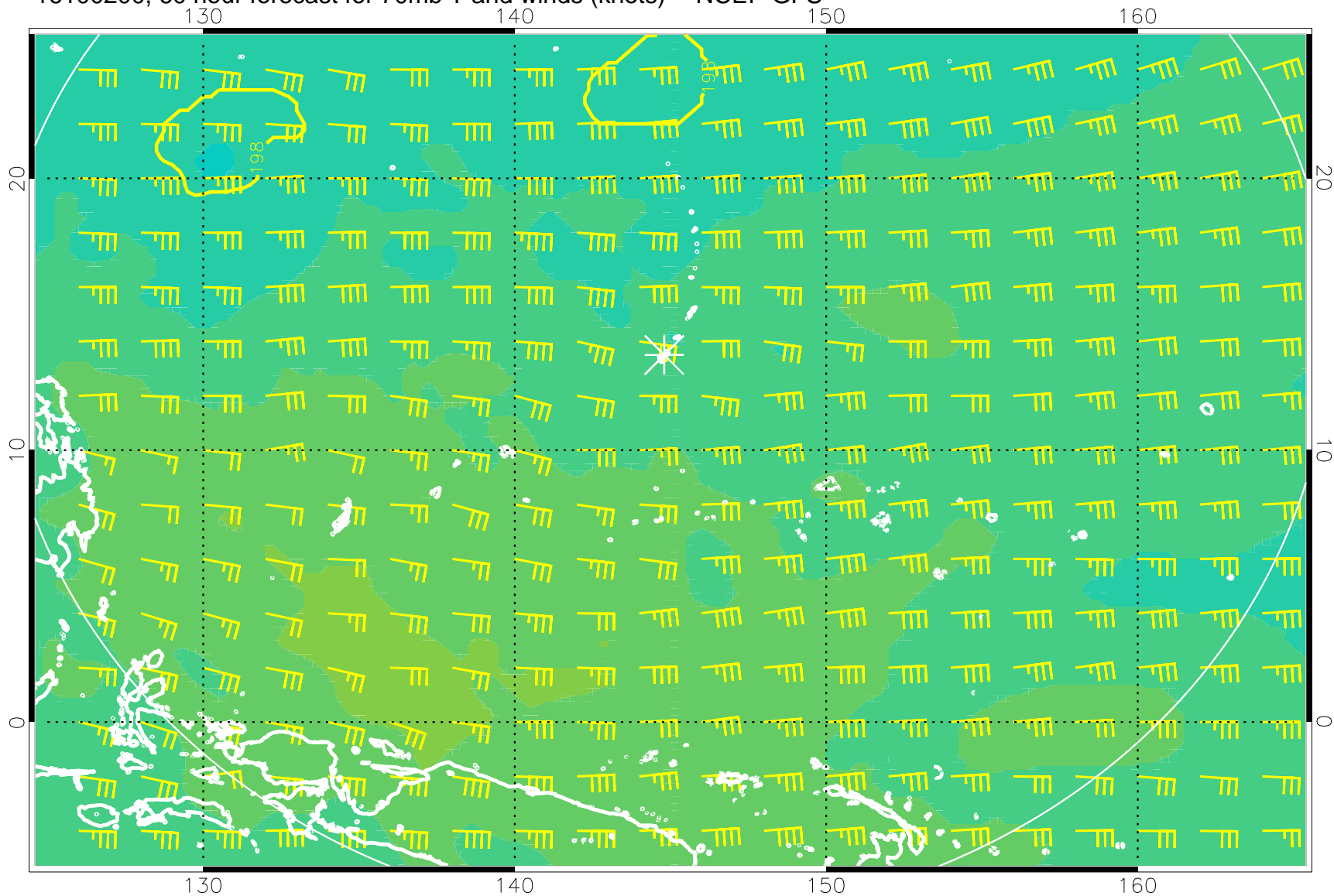
16100200, 60 hour forecast for 70mb T and winds (knots) -- NCEP GFS
