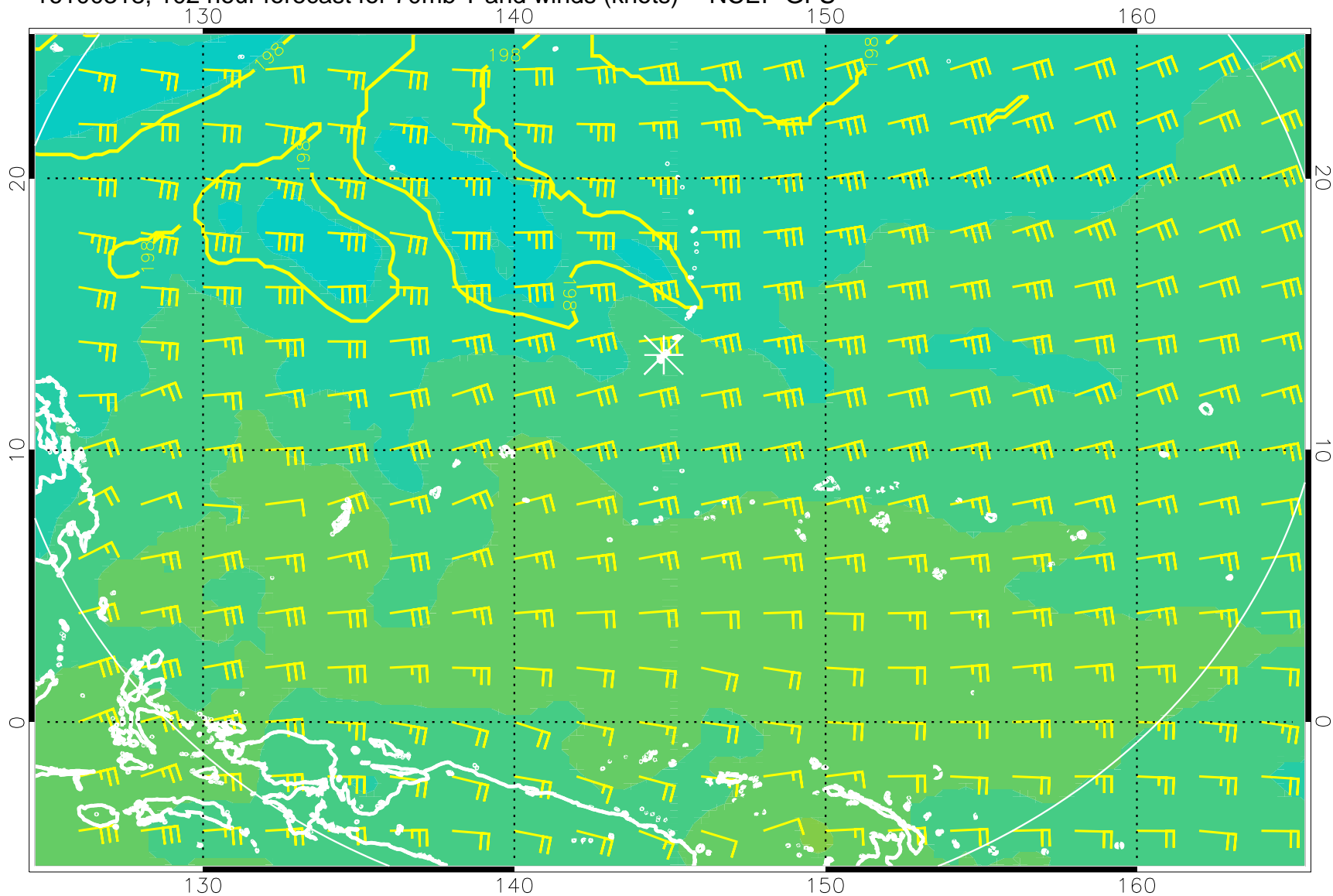
16100318, 102 hour forecast for 70mb T and winds (knots) -- NCEP GFS
