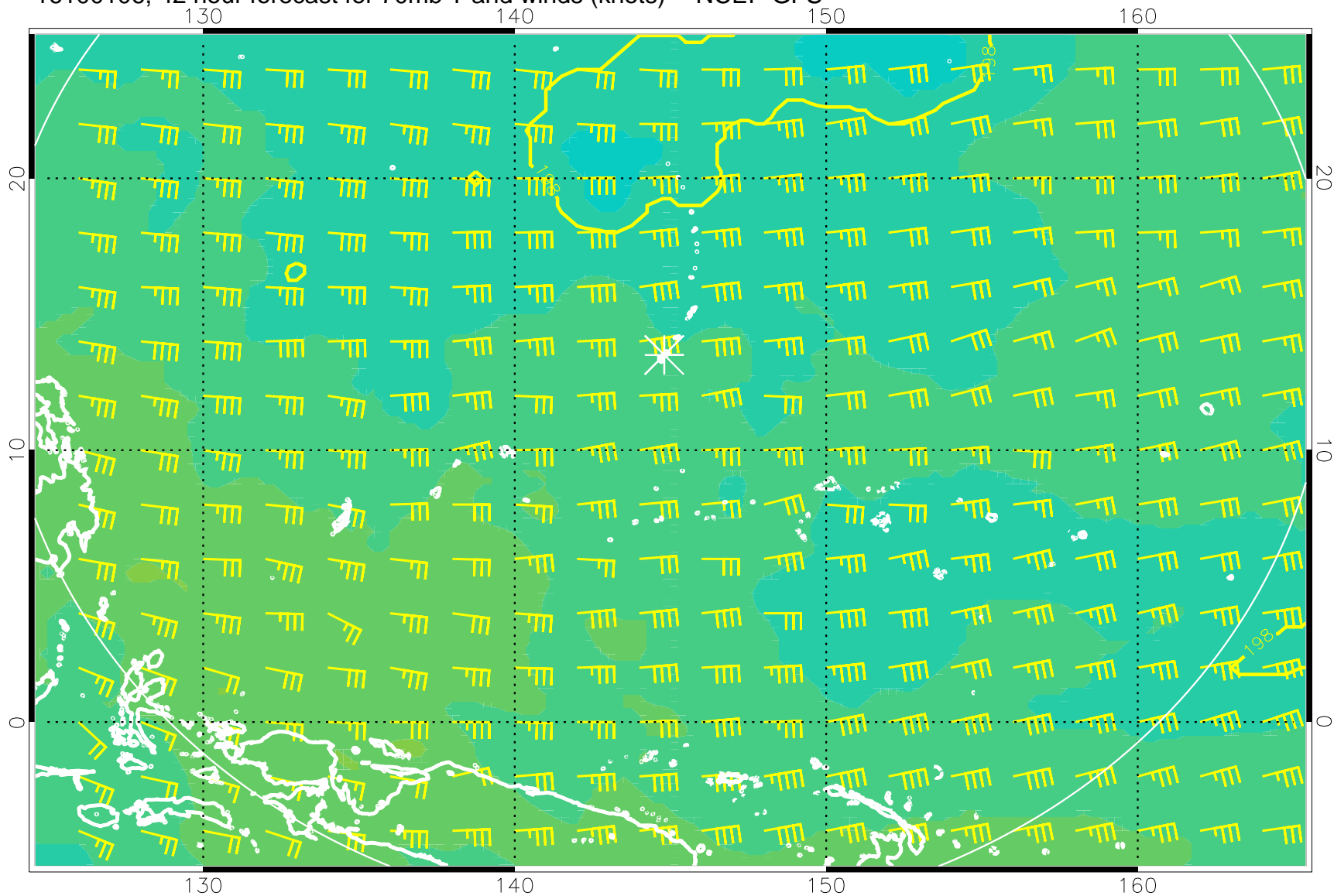
16100106, 42 hour forecast for 70mb T and winds (knots) -- NCEP GFS
