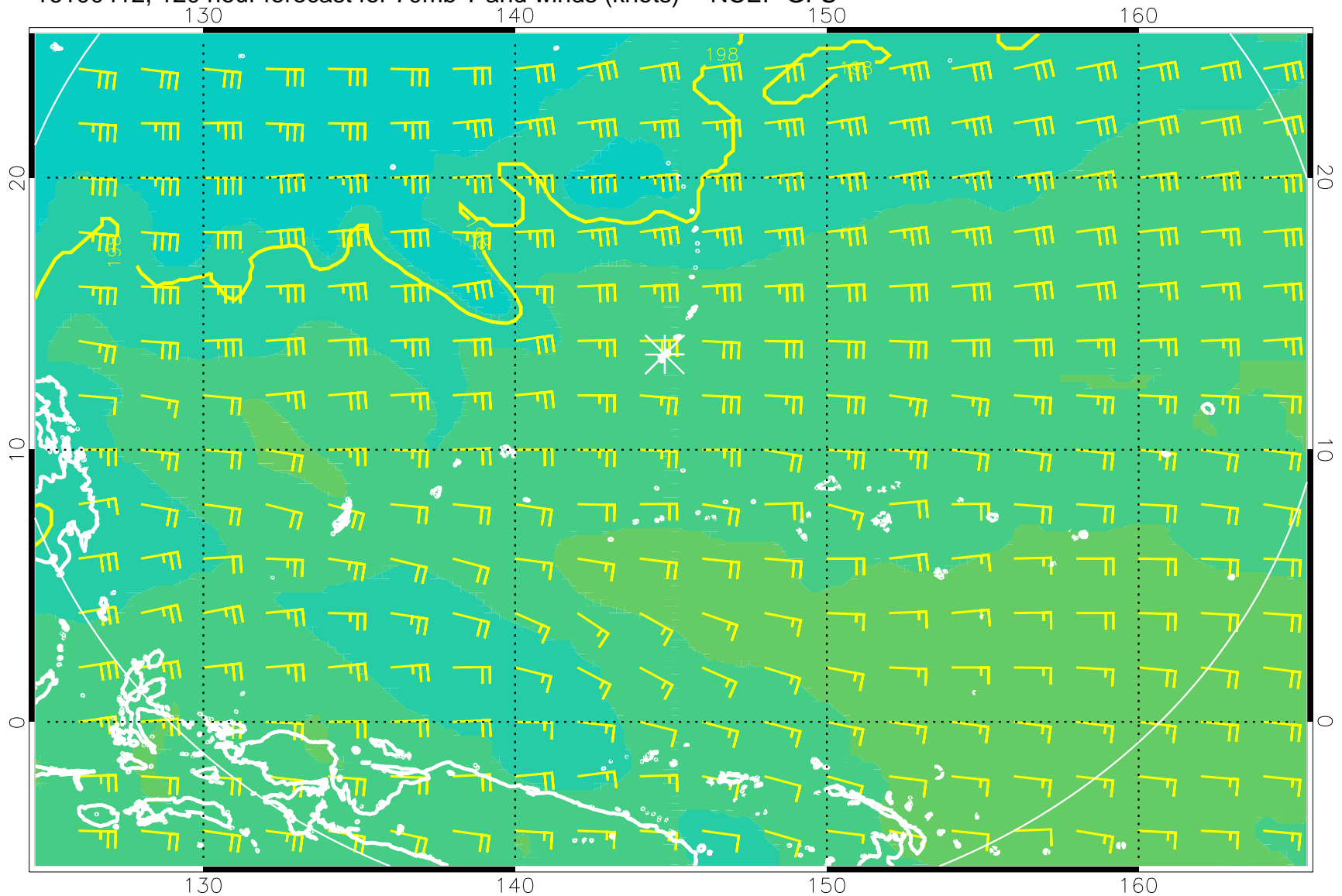
16100412, 120 hour forecast for 70mb T and winds (knots) -- NCEP GFS
