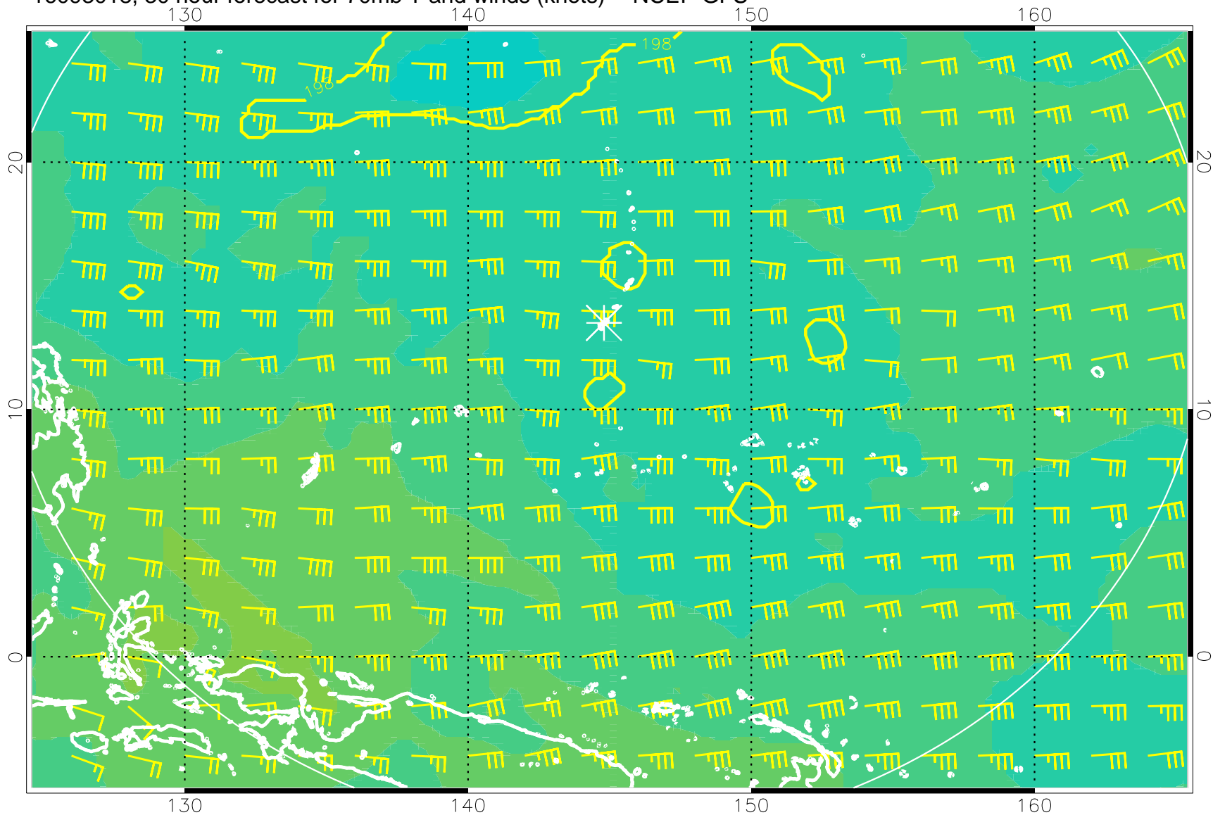
16093018, 30 hour forecast for 70mb T and winds (knots) -- NCEP GFS
