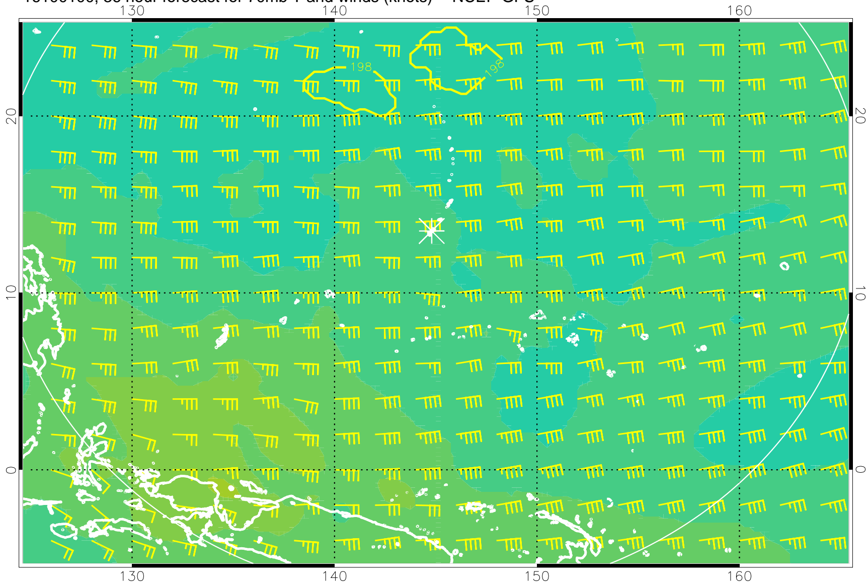
16100100, 36 hour forecast for 70mb T and winds (knots) -- NCEP GFS
