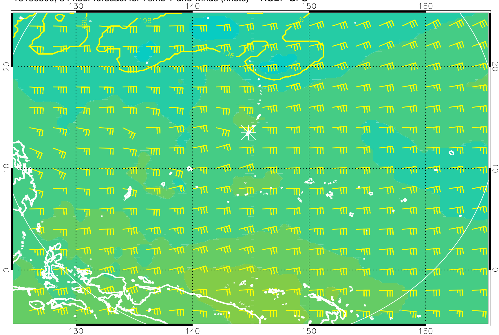
16100300, 84 hour forecast for 70mb T and winds (knots) -- NCEP GFS
