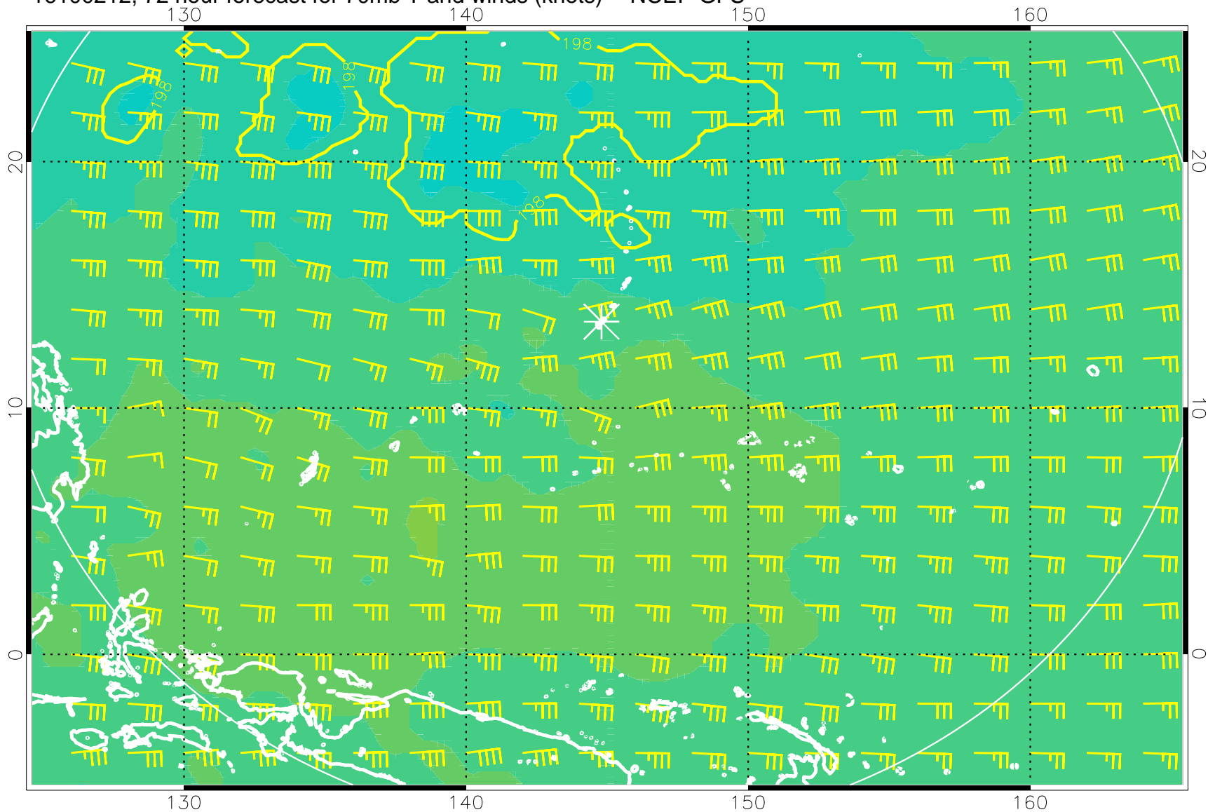
16100212, 72 hour forecast for 70mb T and winds (knots) -- NCEP GFS
