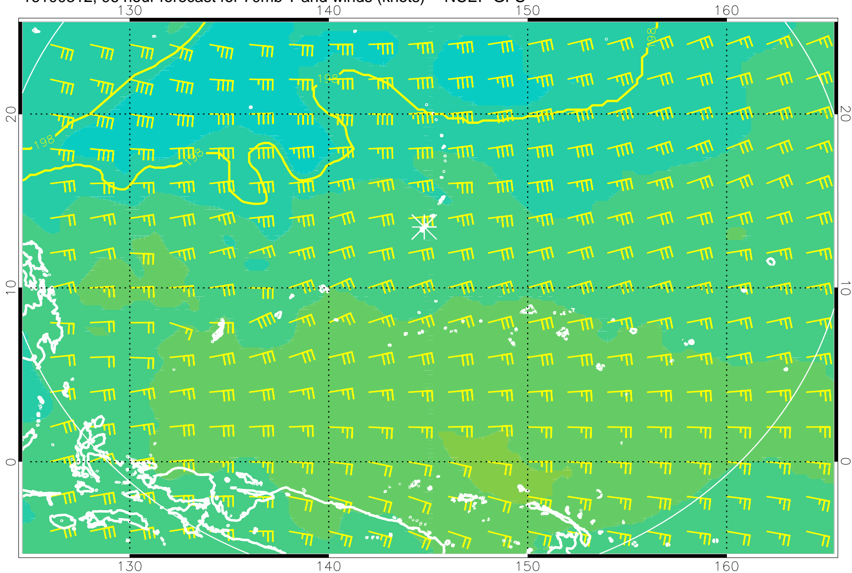
16100312, 96 hour forecast for 70mb T and winds (knots) -- NCEP GFS
