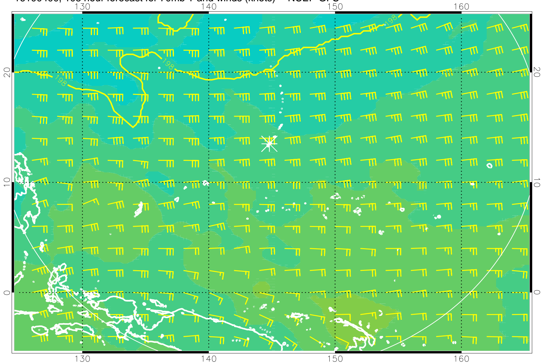
16100400, 108 hour forecast for 70mb T and winds (knots) -- NCEP GFS
