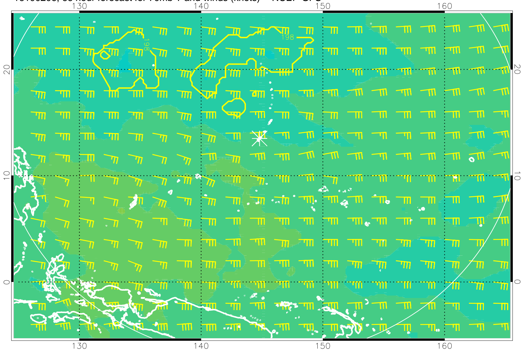
16100206, 66 hour forecast for 70mb T and winds (knots) -- NCEP GFS
