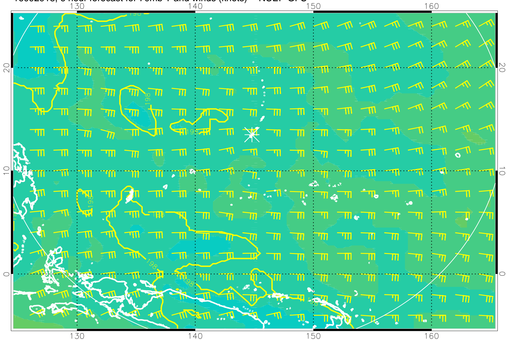
16092918, 6 hour forecast for 70mb T and winds (knots) -- NCEP GFS
