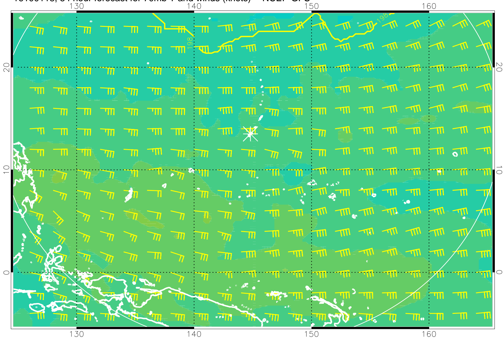
16100118, 54 hour forecast for 70mb T and winds (knots) -- NCEP GFS
