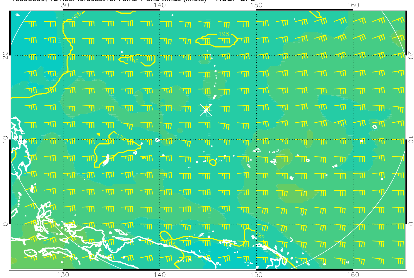
16093000, 12 hour forecast for 70mb T and winds (knots) -- NCEP GFS
