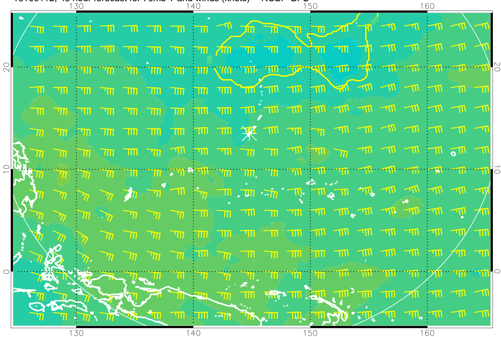
16100112, 48 hour forecast for 70mb T and winds (knots) -- NCEP GFS
