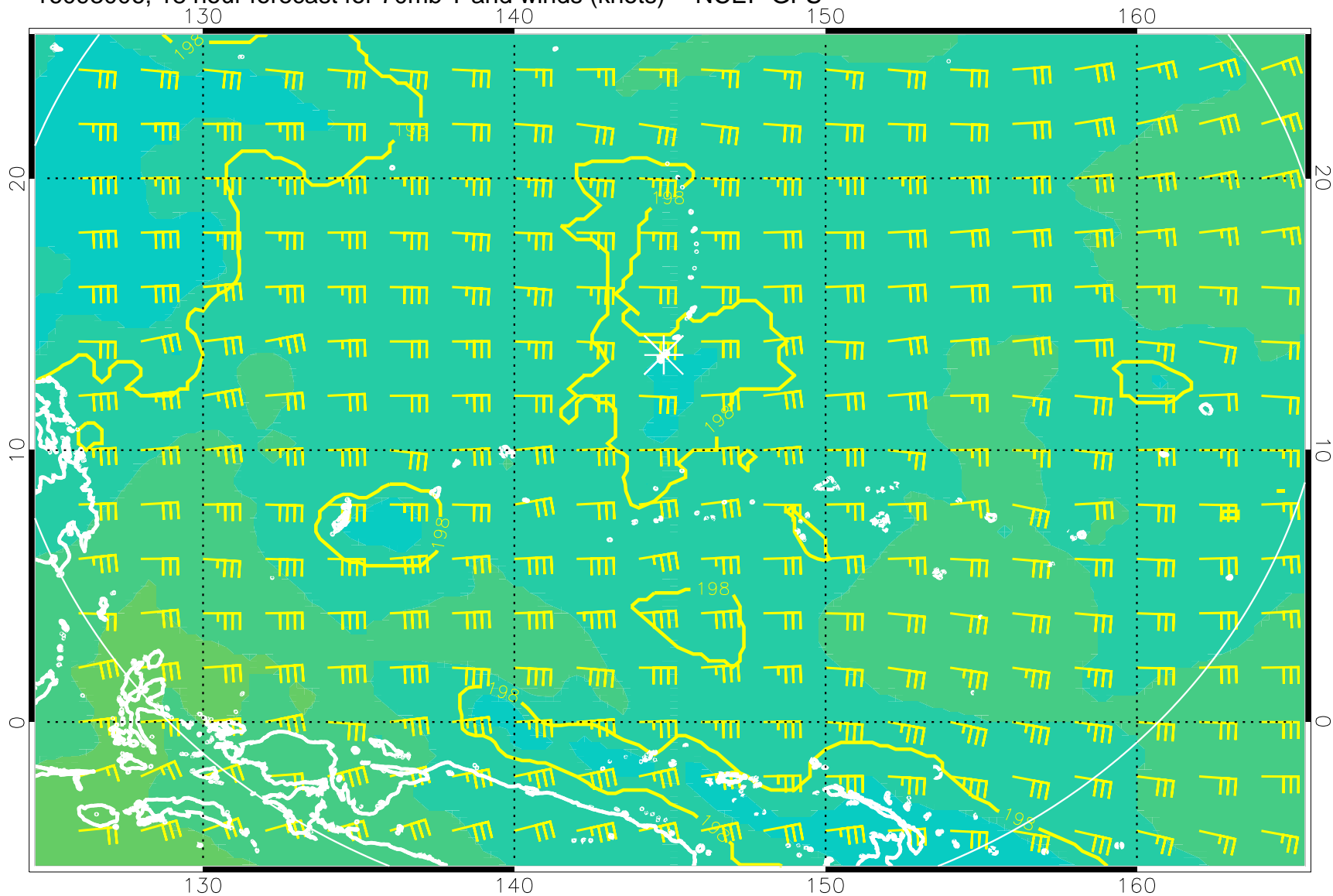
16093006, 18 hour forecast for 70mb T and winds (knots) -- NCEP GFS
