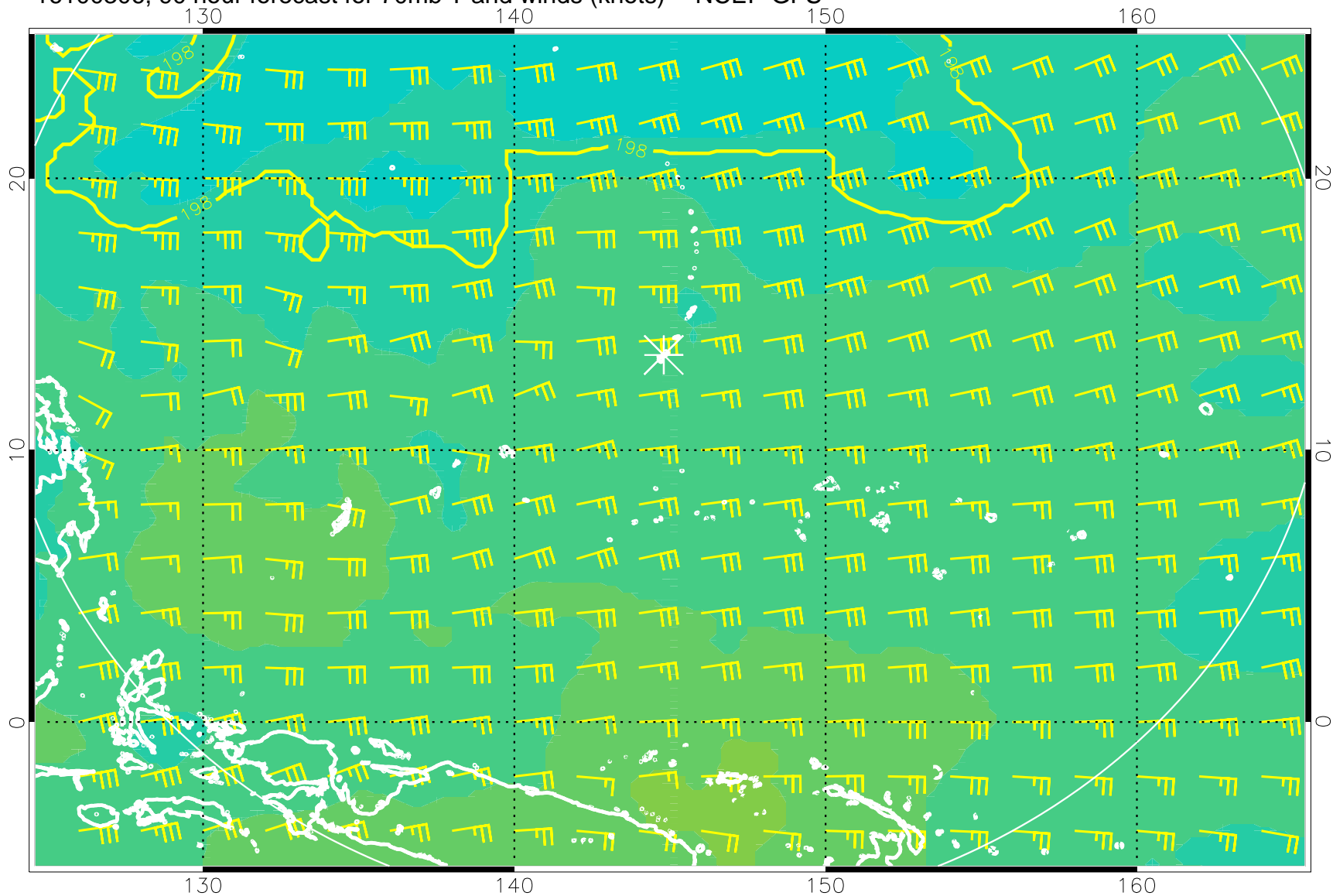
16100306, 90 hour forecast for 70mb T and winds (knots) -- NCEP GFS
