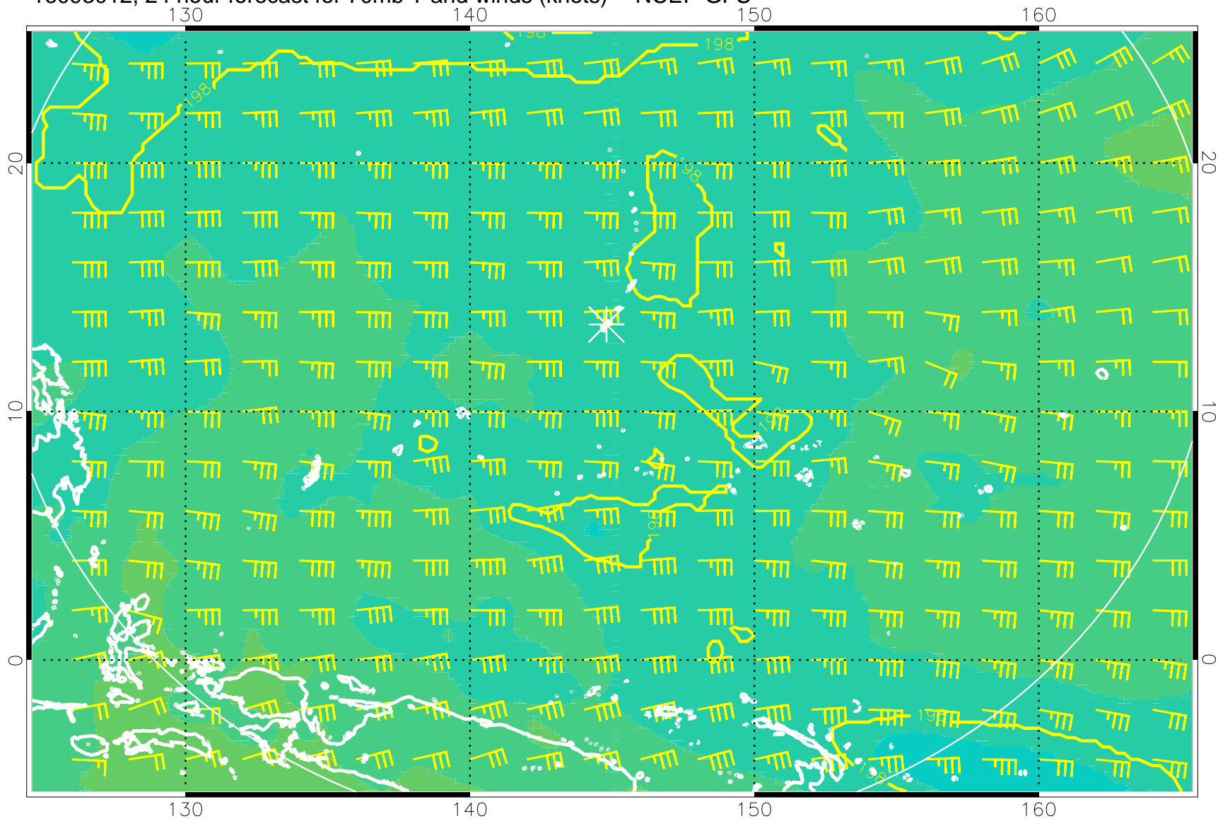
16093012, 24 hour forecast for 70mb T and winds (knots) -- NCEP GFS
