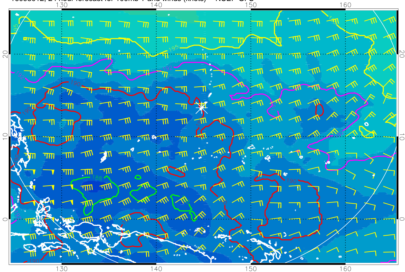
16093012, 24 hour forecast for 100mb T and winds (knots) -- NCEP GFS
