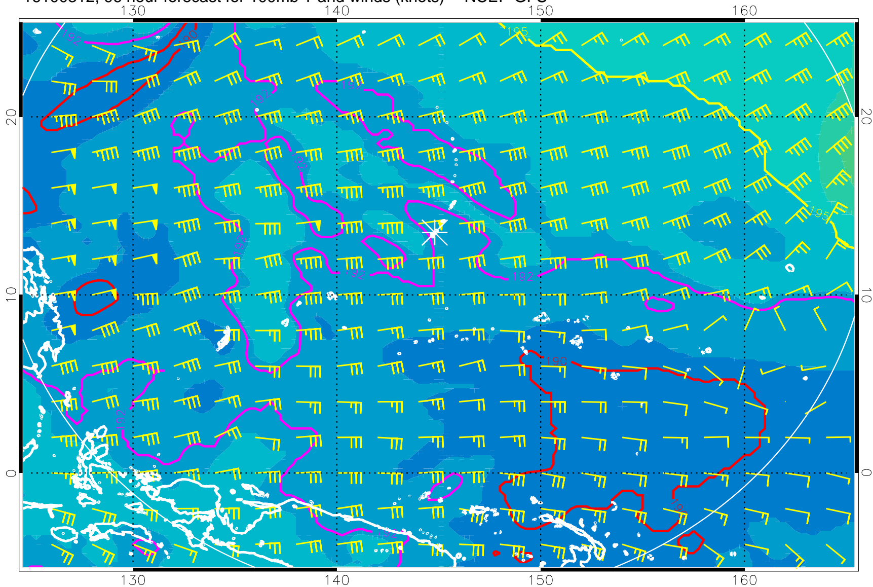
16100312, 96 hour forecast for 100mb T and winds (knots) -- NCEP GFS
