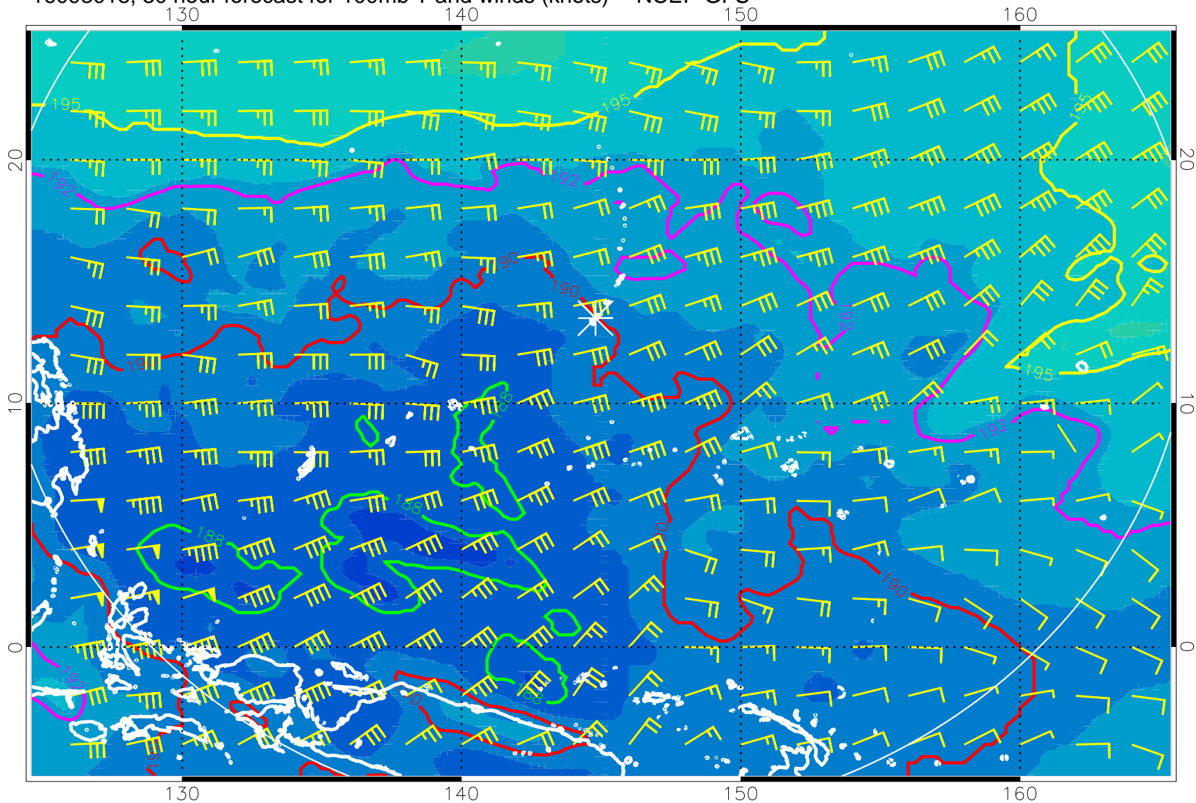
16093018, 30 hour forecast for 100mb T and winds (knots) -- NCEP GFS
