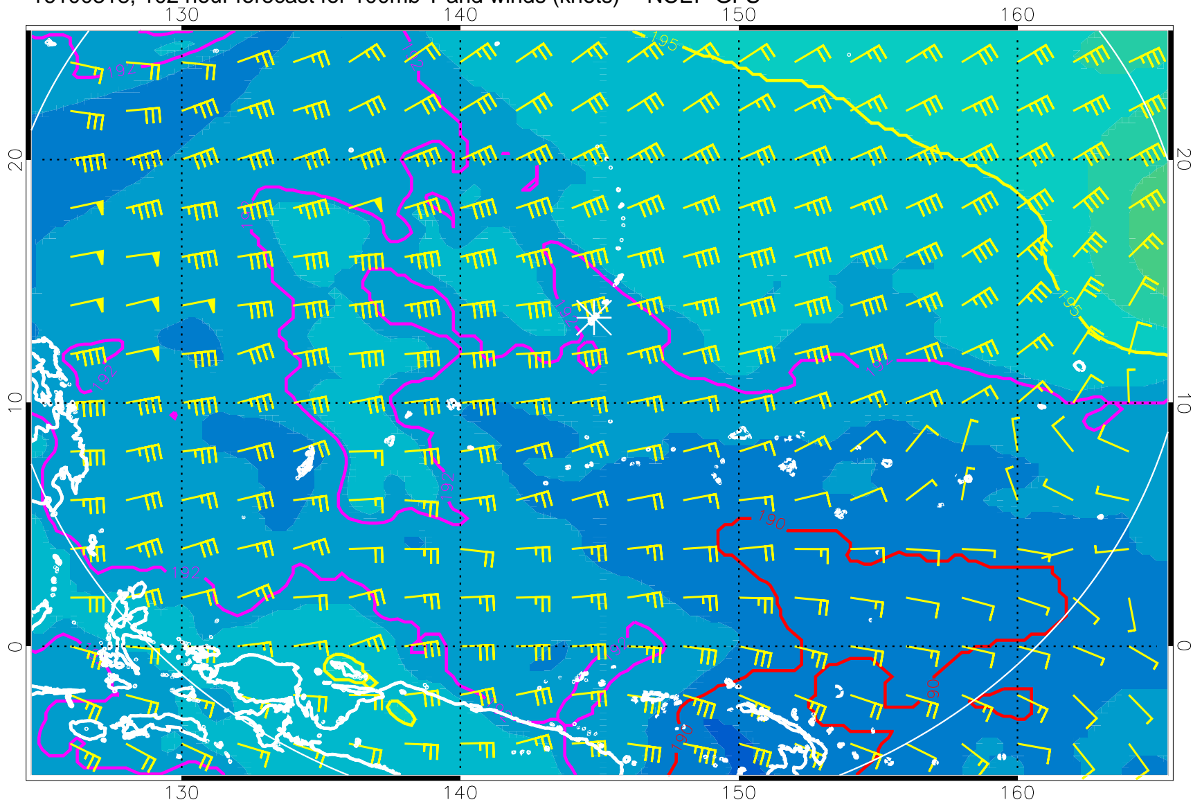
16100318, 102 hour forecast for 100mb T and winds (knots) -- NCEP GFS
