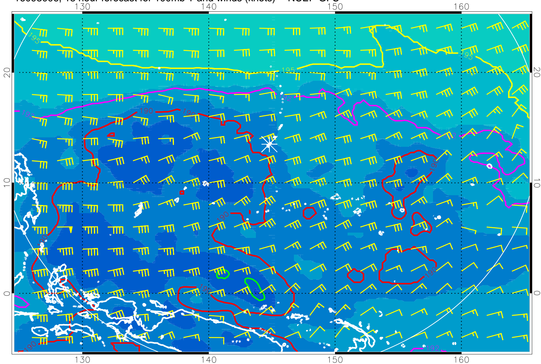
16093006, 18 hour forecast for 100mb T and winds (knots) -- NCEP GFS
