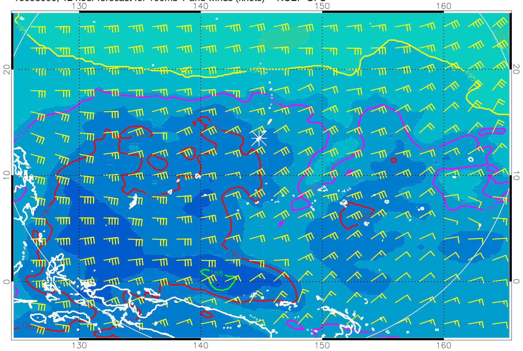
16093000, 12 hour forecast for 100mb T and winds (knots) -- NCEP GFS
