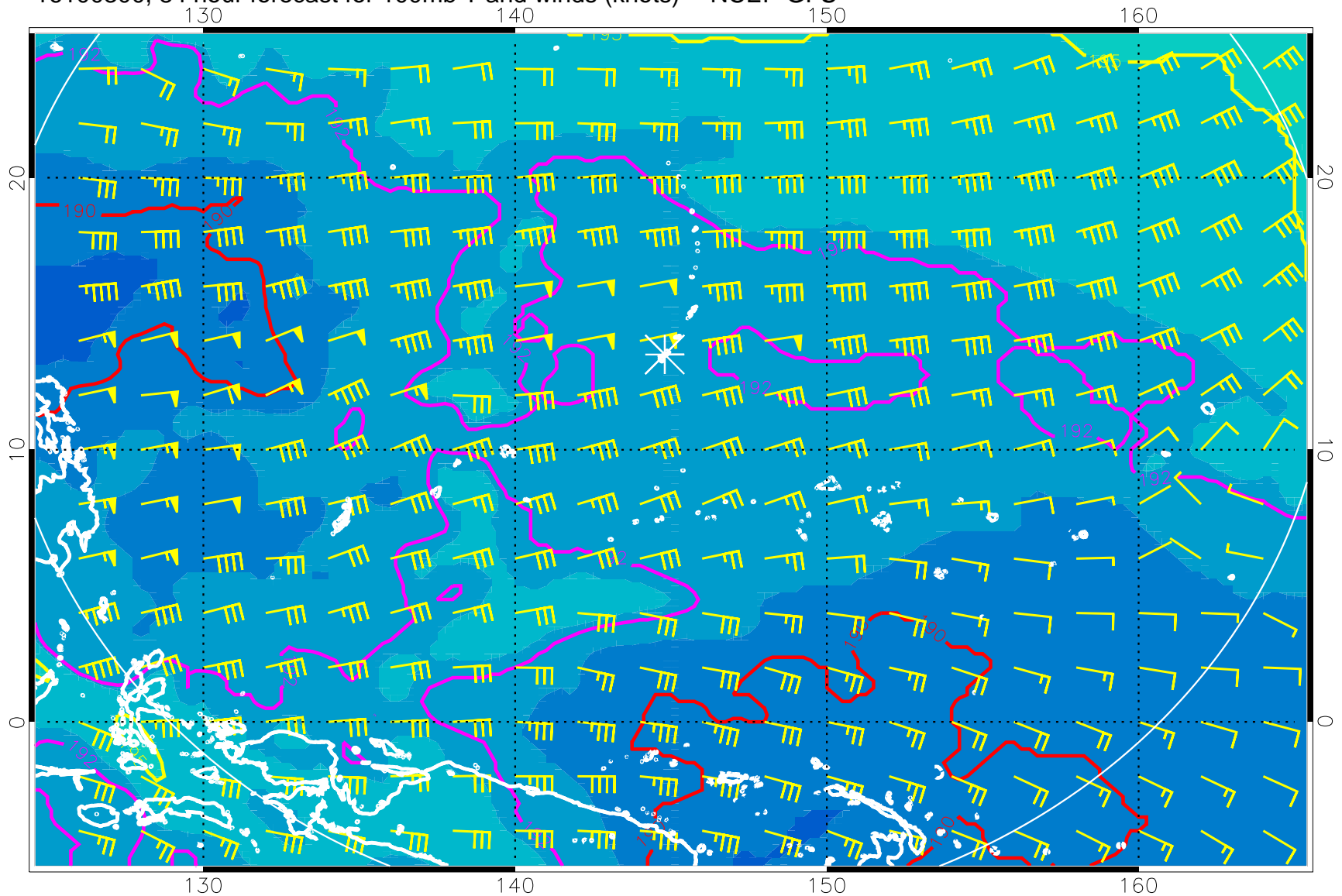
16100300, 84 hour forecast for 100mb T and winds (knots) -- NCEP GFS
