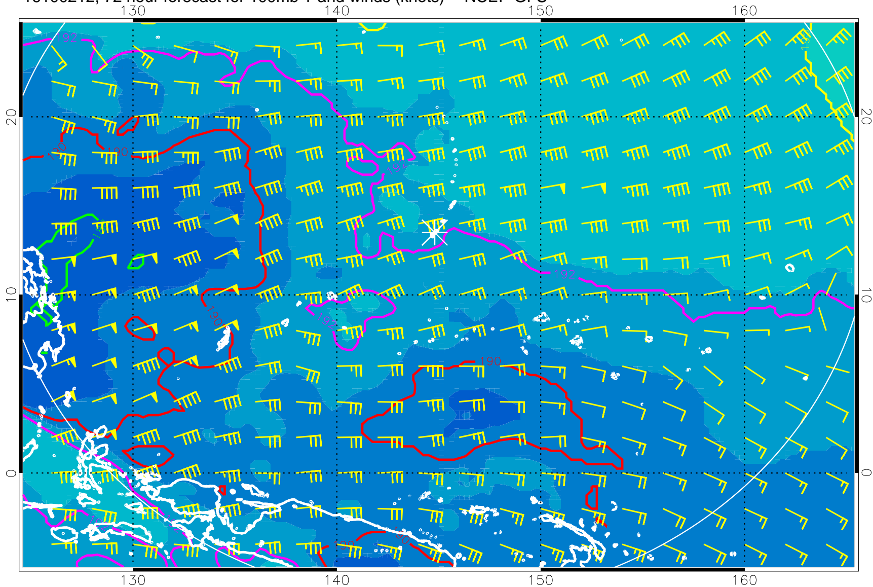
16100212, 72 hour forecast for 100mb T and winds (knots) -- NCEP GFS
