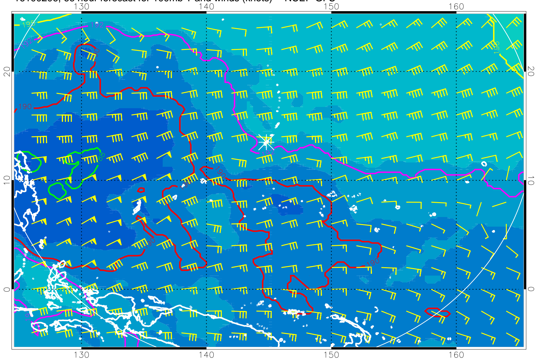
16100206, 66 hour forecast for 100mb T and winds (knots) -- NCEP GFS
