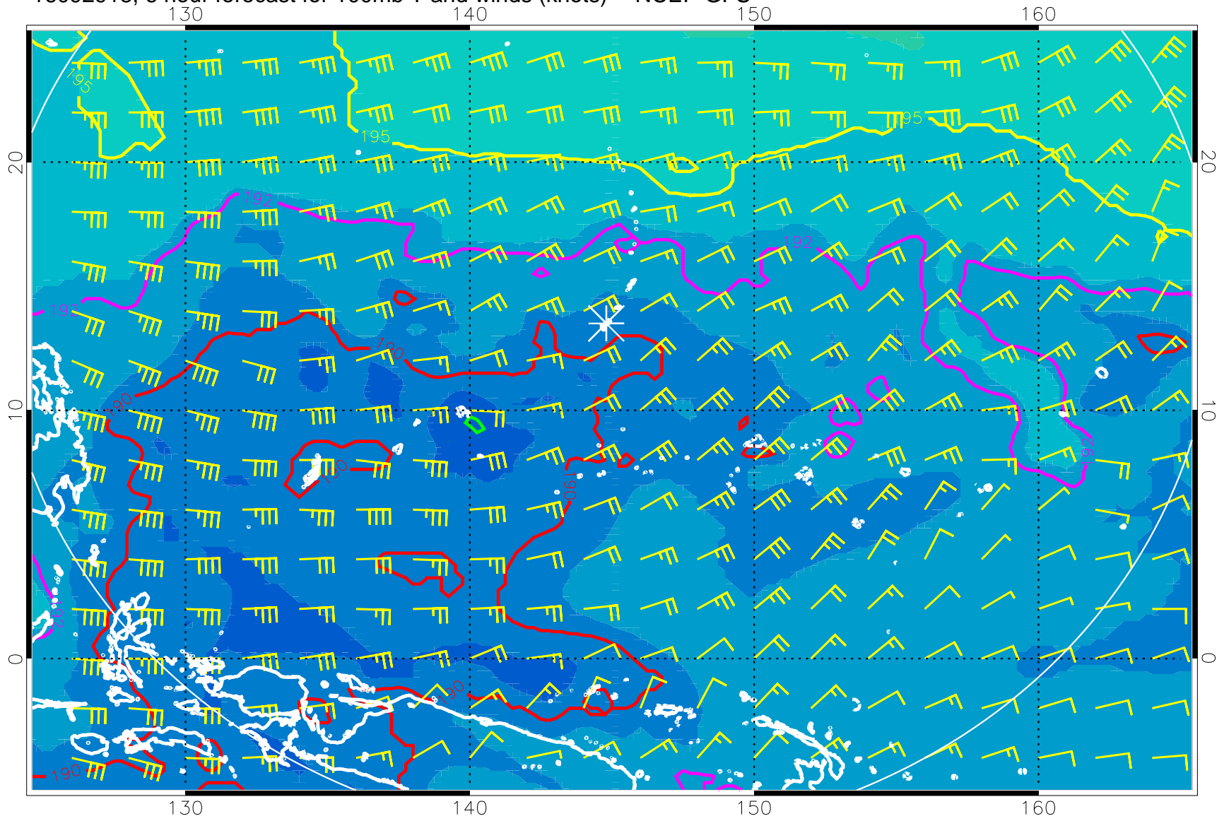
16092918, 6 hour forecast for 100mb T and winds (knots) -- NCEP GFS
