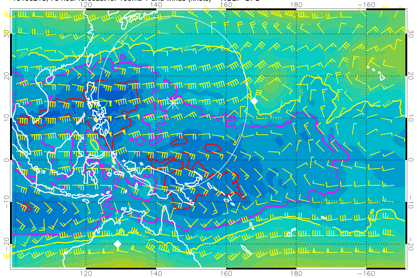
16100218, 78 hour forecast for 100mb T and winds (knots) -- NCEP GFS
