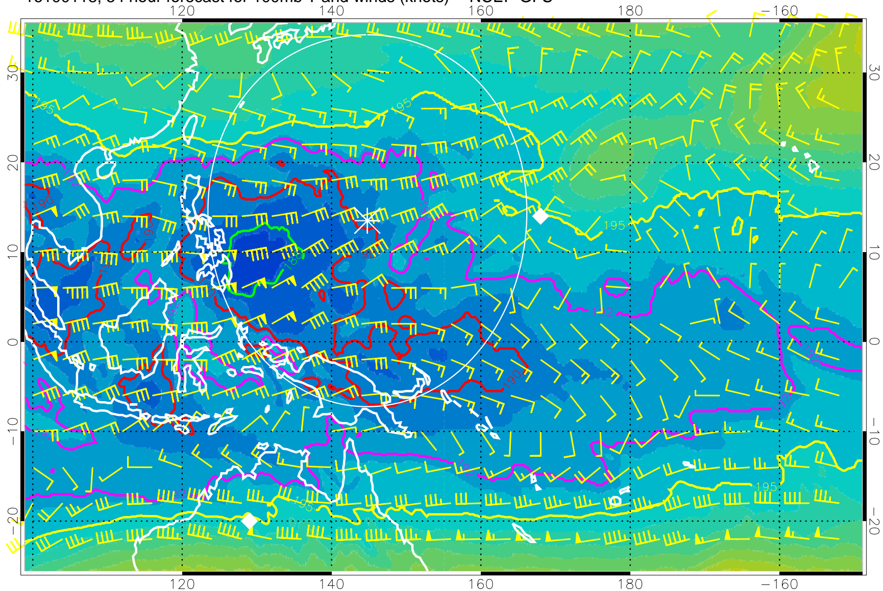
16100118, 54 hour forecast for 100mb T and winds (knots) -- NCEP GFS
