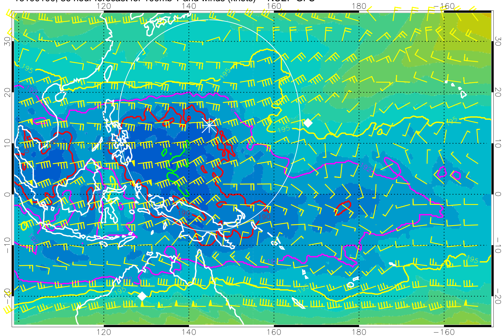
16100100, 36 hour forecast for 100mb T and winds (knots) -- NCEP GFS
