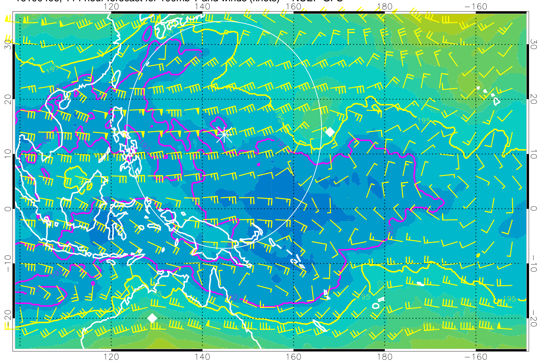
16100406, 114 hour forecast for 100mb T and winds (knots) -- NCEP GFS
