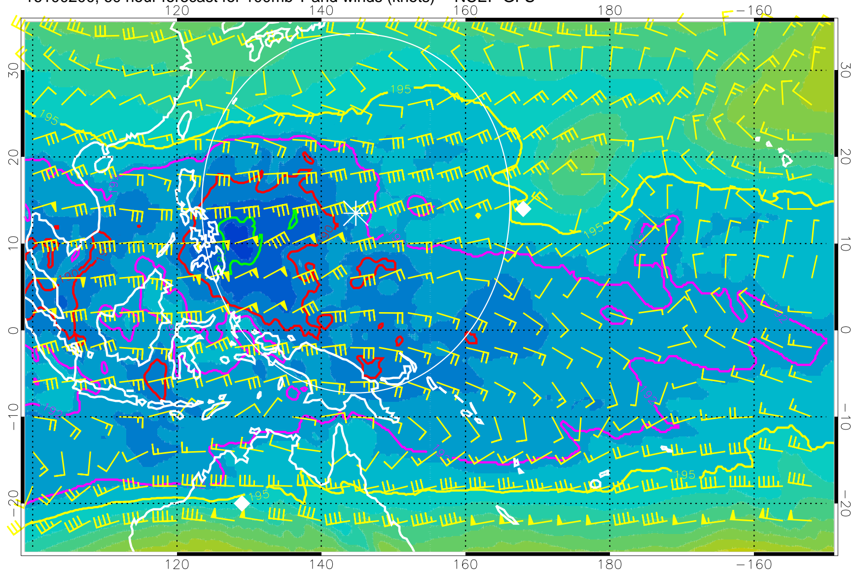
16100200, 60 hour forecast for 100mb T and winds (knots) -- NCEP GFS
