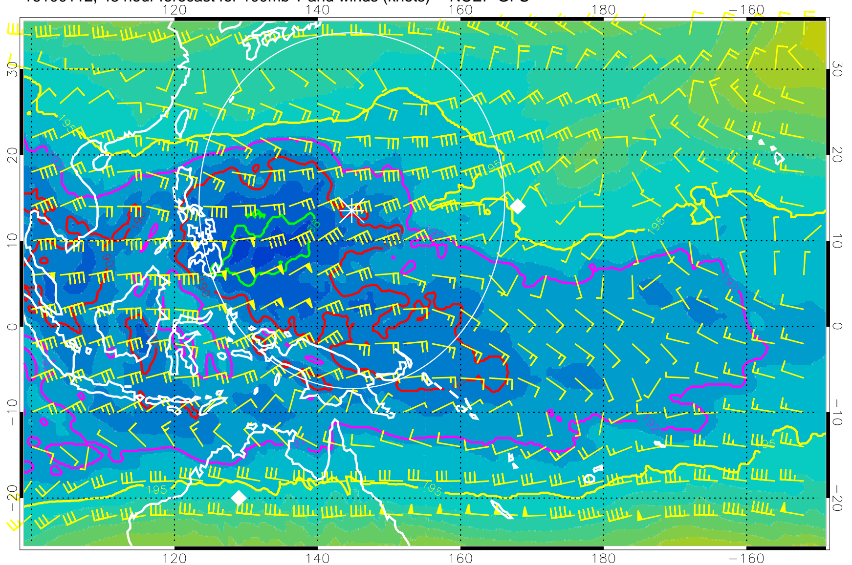
16100112, 48 hour forecast for 100mb T and winds (knots) -- NCEP GFS
