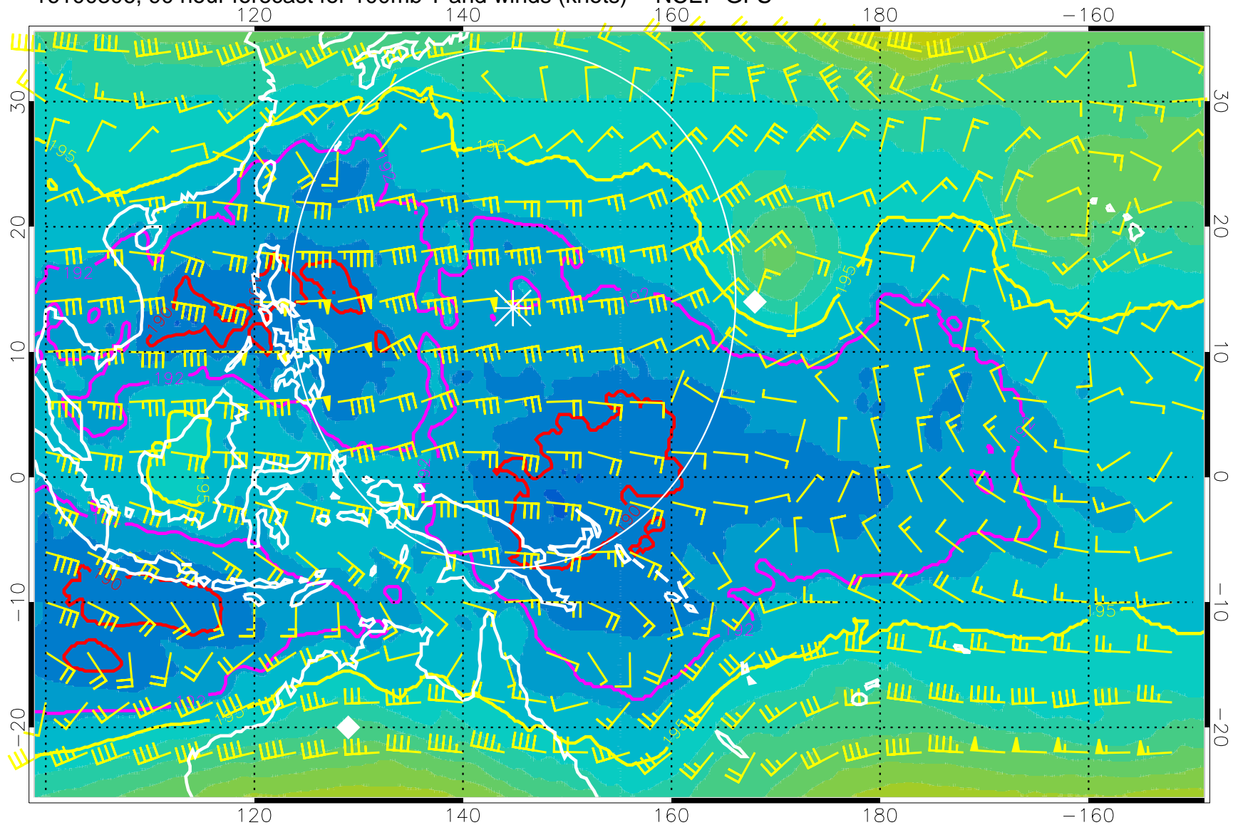
16100306, 90 hour forecast for 100mb T and winds (knots) -- NCEP GFS
