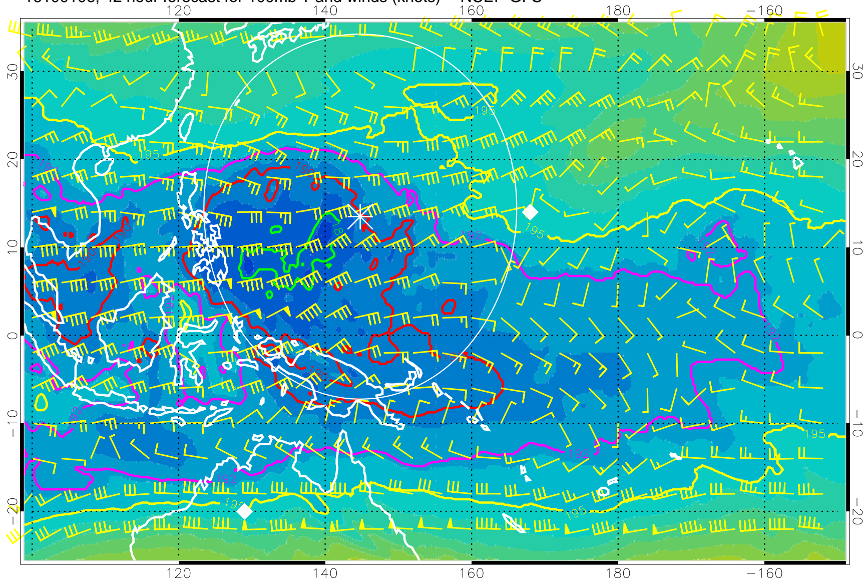
16100106, 42 hour forecast for 100mb T and winds (knots) -- NCEP GFS
