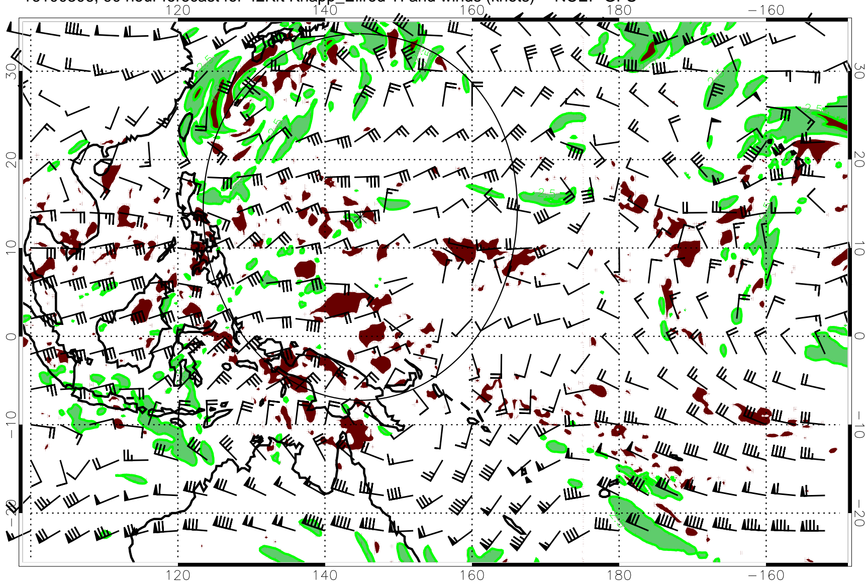
16100306, 90 hour forecast for 42Kft Knapp_Ellrod TI and winds (knots) -- NCEP GFS
