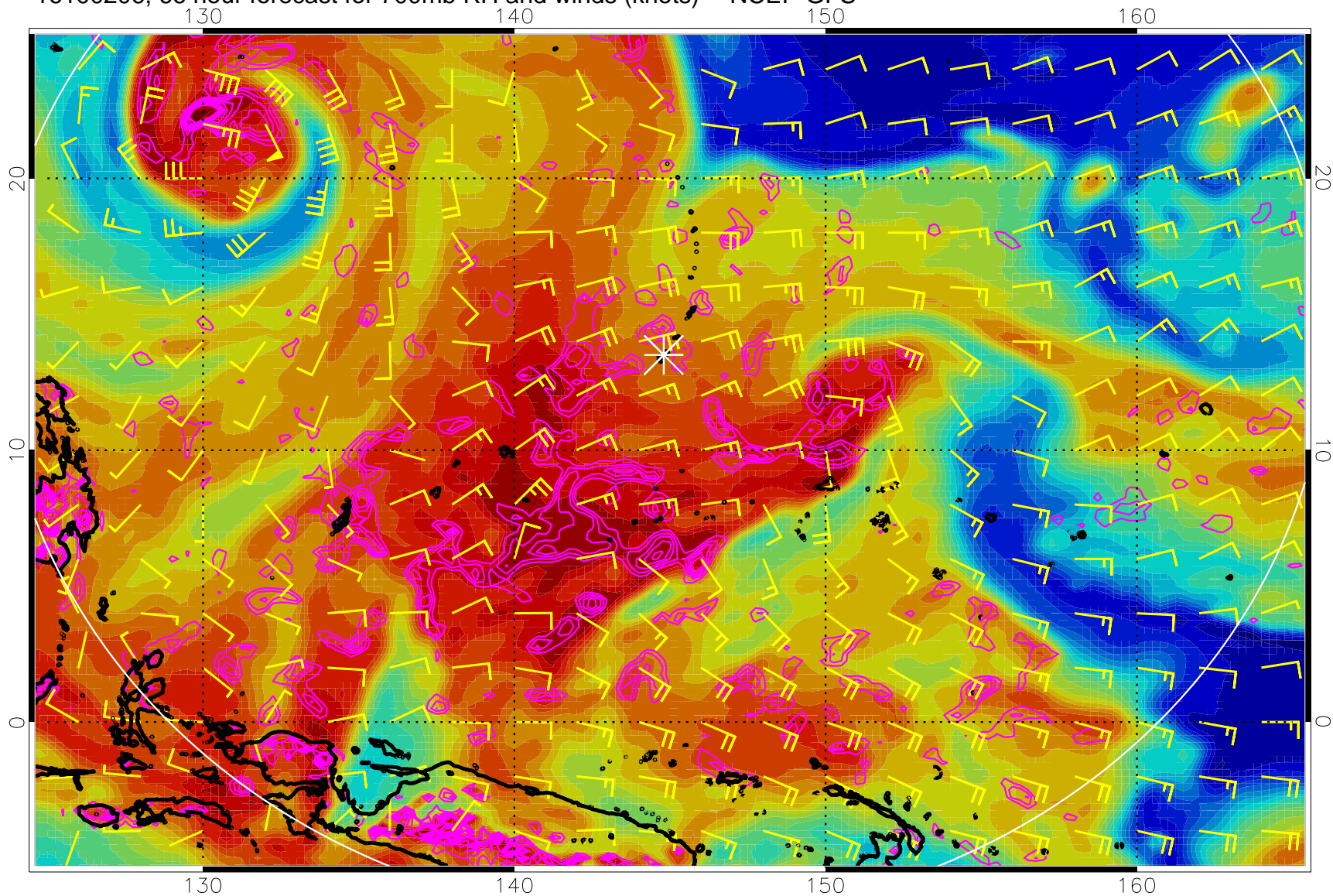
16100206, 66 hour forecast for 700mb RH and winds (knots) -- NCEP GFS
