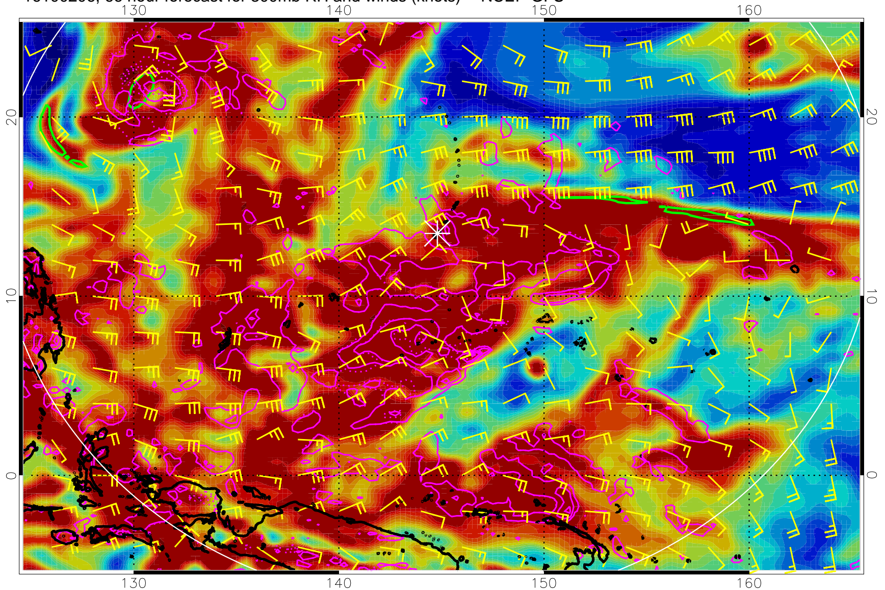
16100206, 66 hour forecast for 300mb RH and winds (knots) -- NCEP GFS
