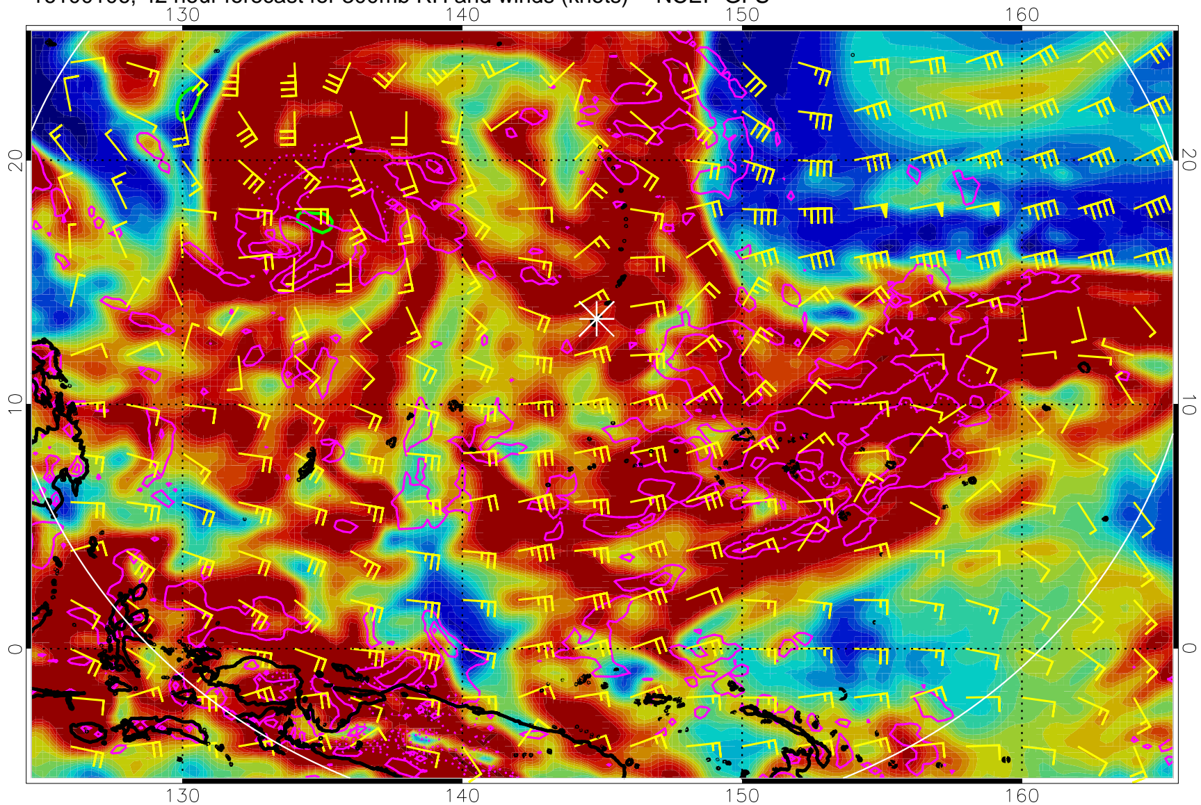
16100106, 42 hour forecast for 300mb RH and winds (knots) -- NCEP GFS
