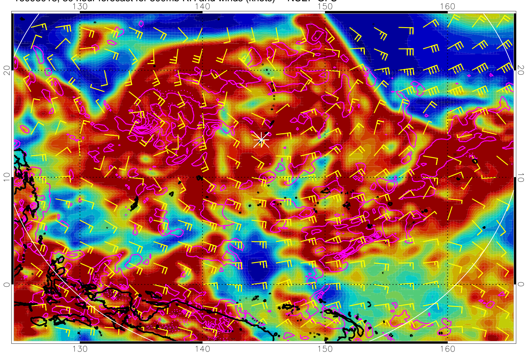
16093018, 30 hour forecast for 300mb RH and winds (knots) -- NCEP GFS
