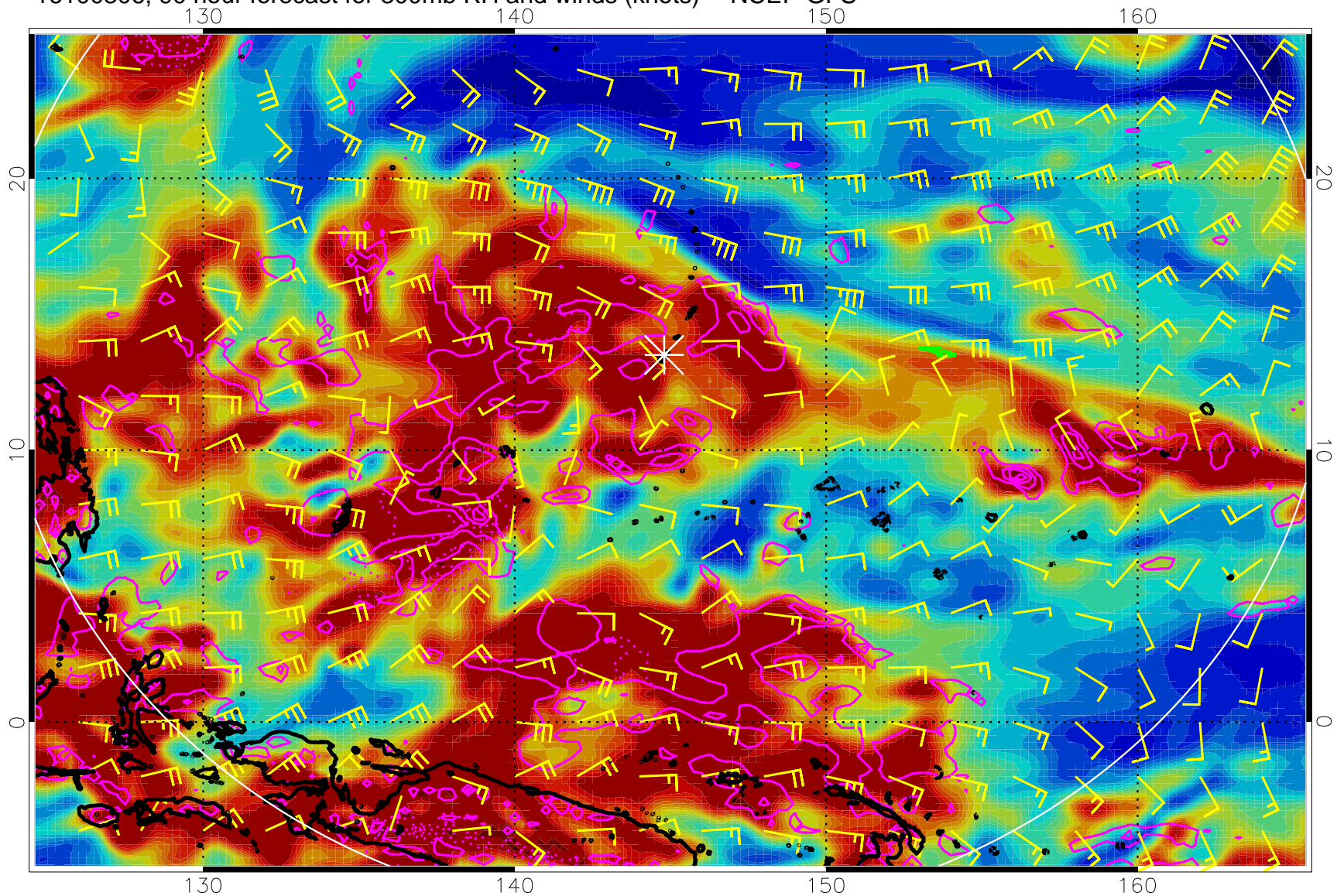
16100306, 90 hour forecast for 300mb RH and winds (knots) -- NCEP GFS
