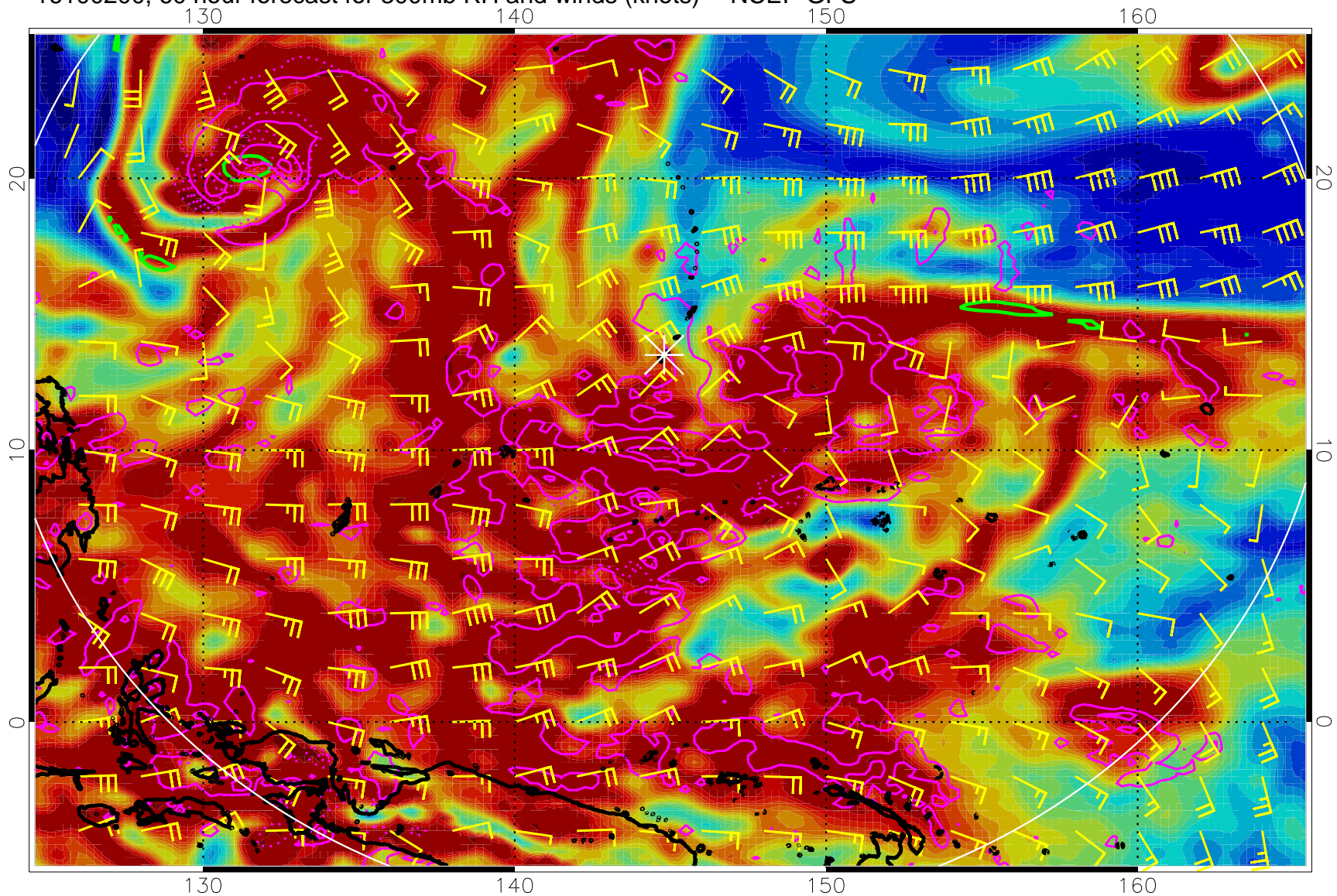
16100200, 60 hour forecast for 300mb RH and winds (knots) -- NCEP GFS
