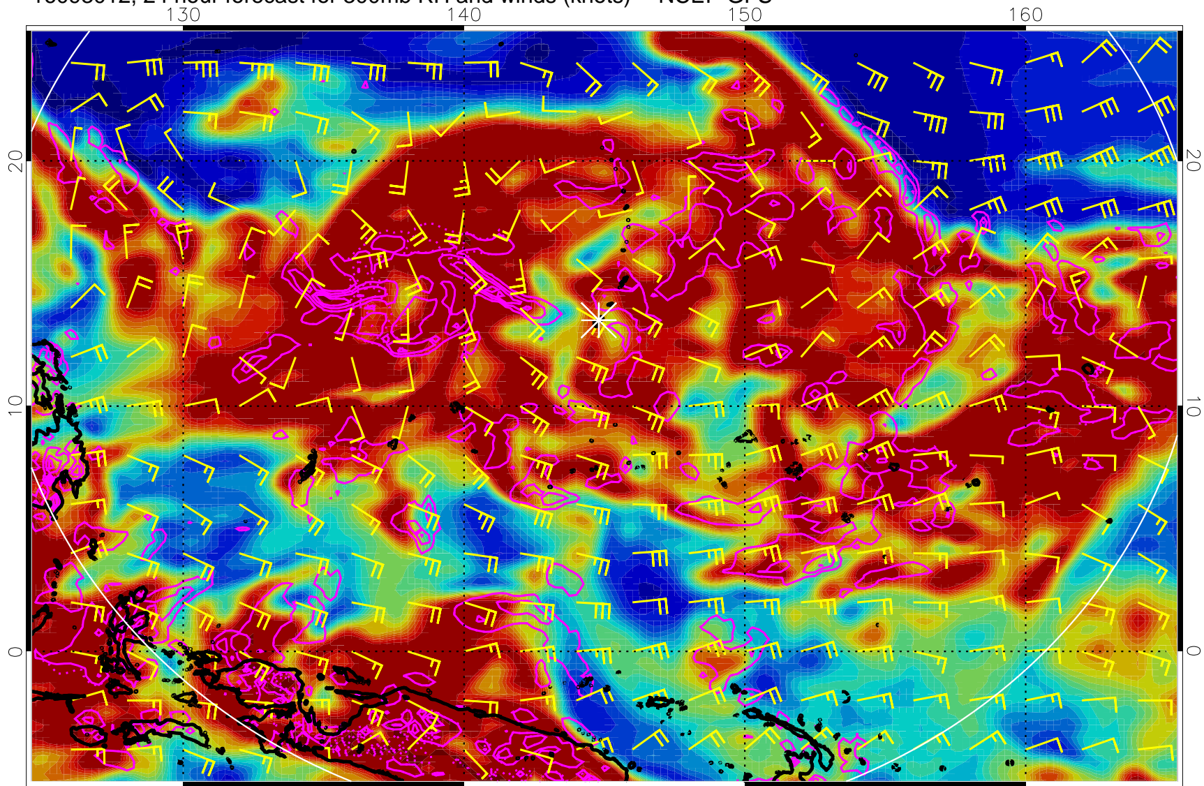
16093012, 24 hour forecast for 300mb RH and winds (knots) -- NCEP GFS
