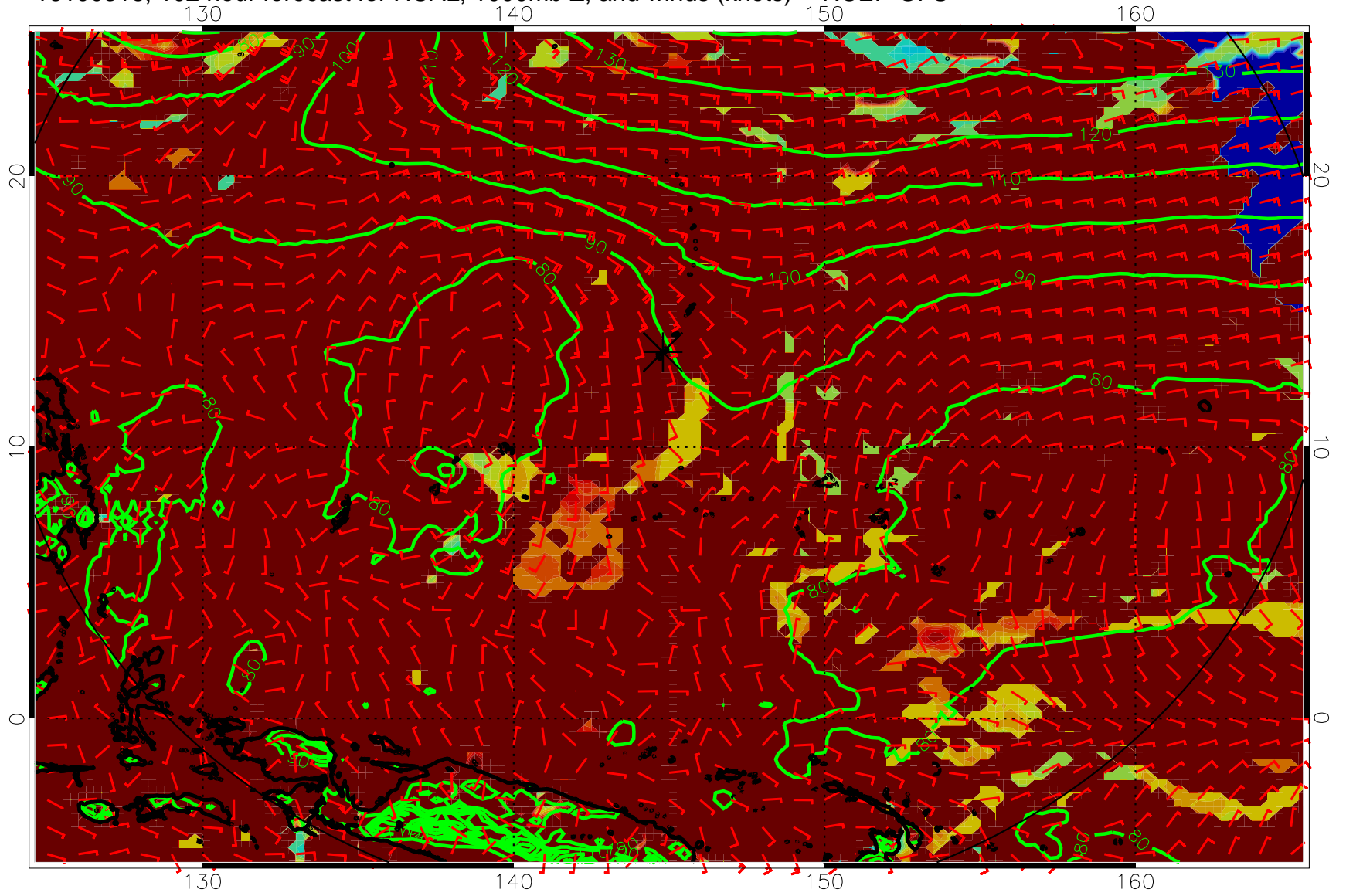
16100318, 102 hour forecast for HCAL, 1000mb Z, and winds (knots) -- NCEP GFS
