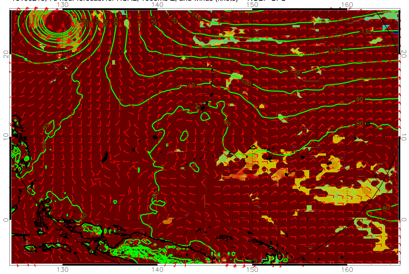
16100218, 78 hour forecast for HCAL, 1000mb Z, and winds (knots) -- NCEP GFS
