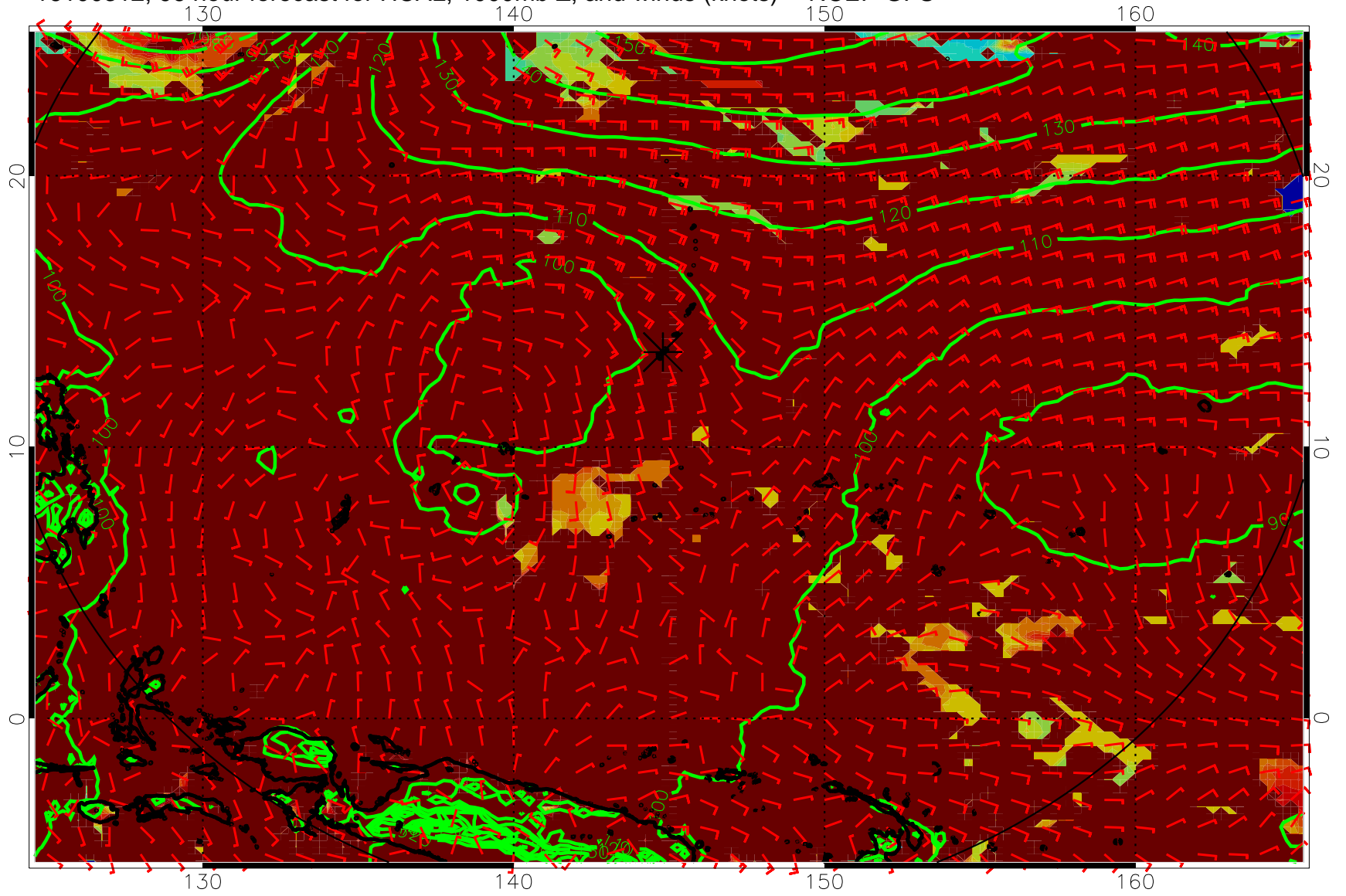
16100312, 96 hour forecast for HCAL, 1000mb Z, and winds (knots) -- NCEP GFS
