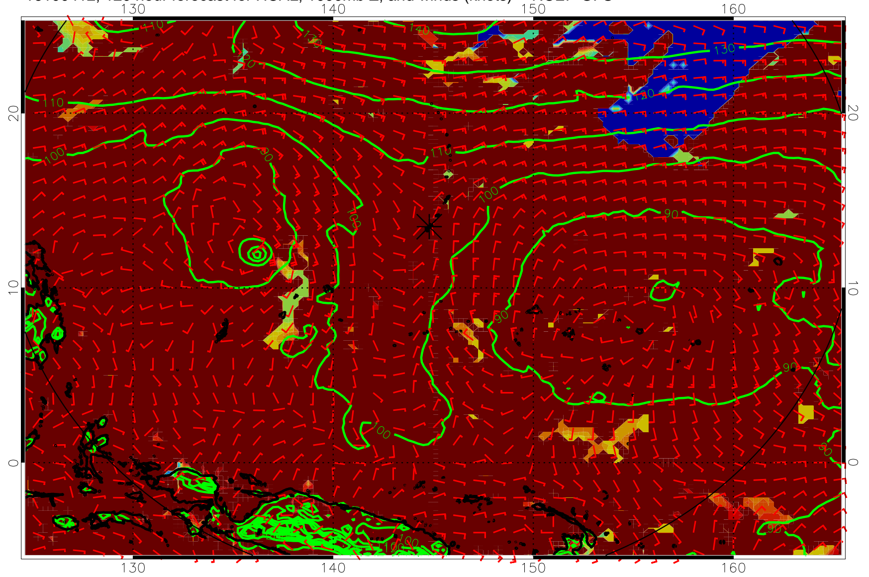
16100412, 120 hour forecast for HCAL, 1000mb Z, and winds (knots) -- NCEP GFS
