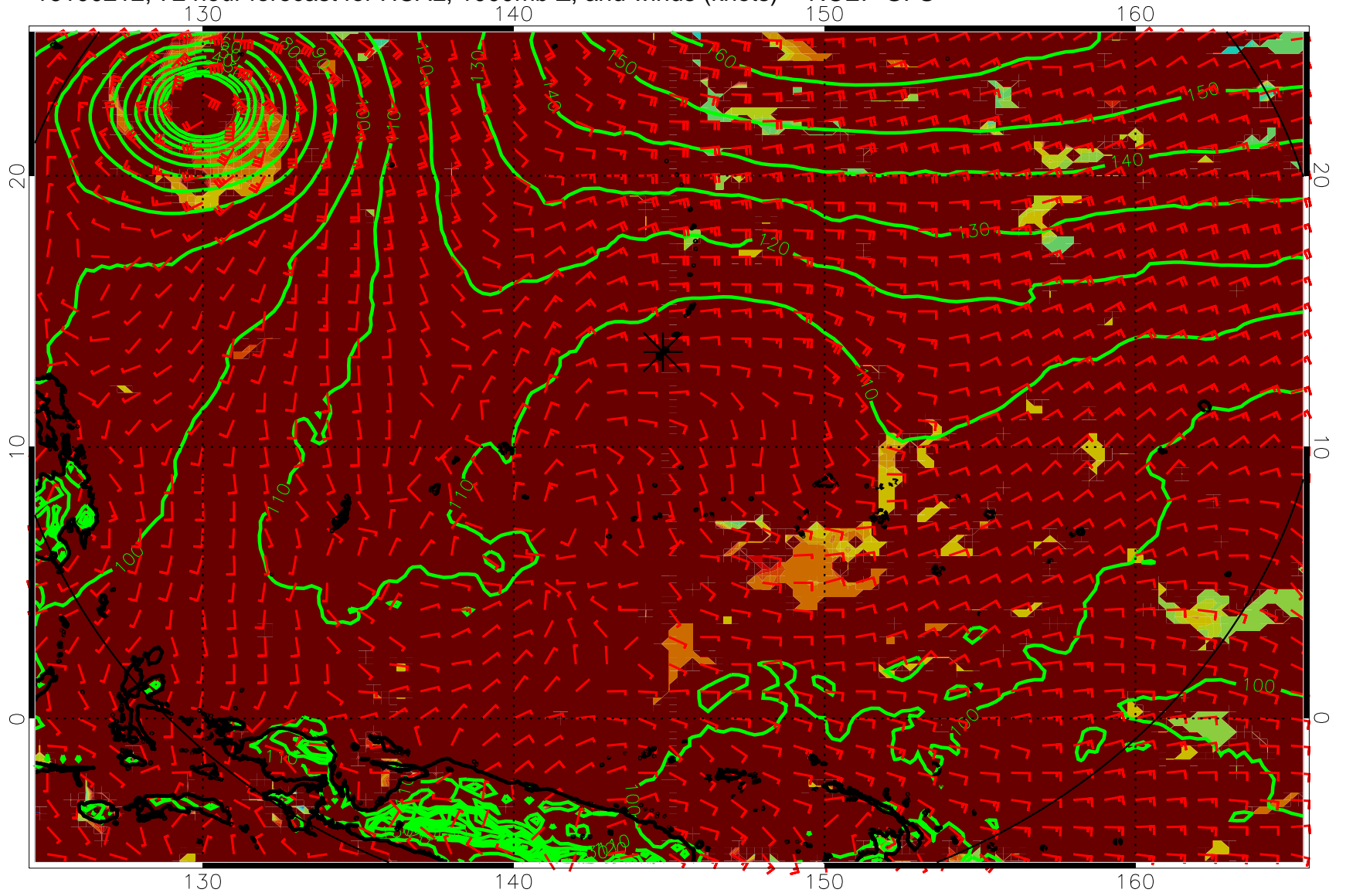
16100212, 72 hour forecast for HCAL, 1000mb Z, and winds (knots) -- NCEP GFS
