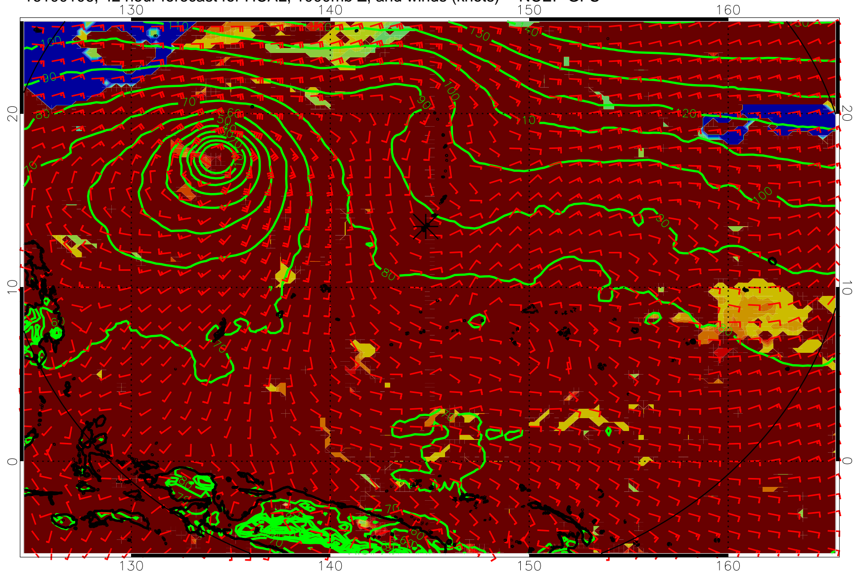
16100106, 42 hour forecast for HCAL, 1000mb Z, and winds (knots) -- NCEP GFS
