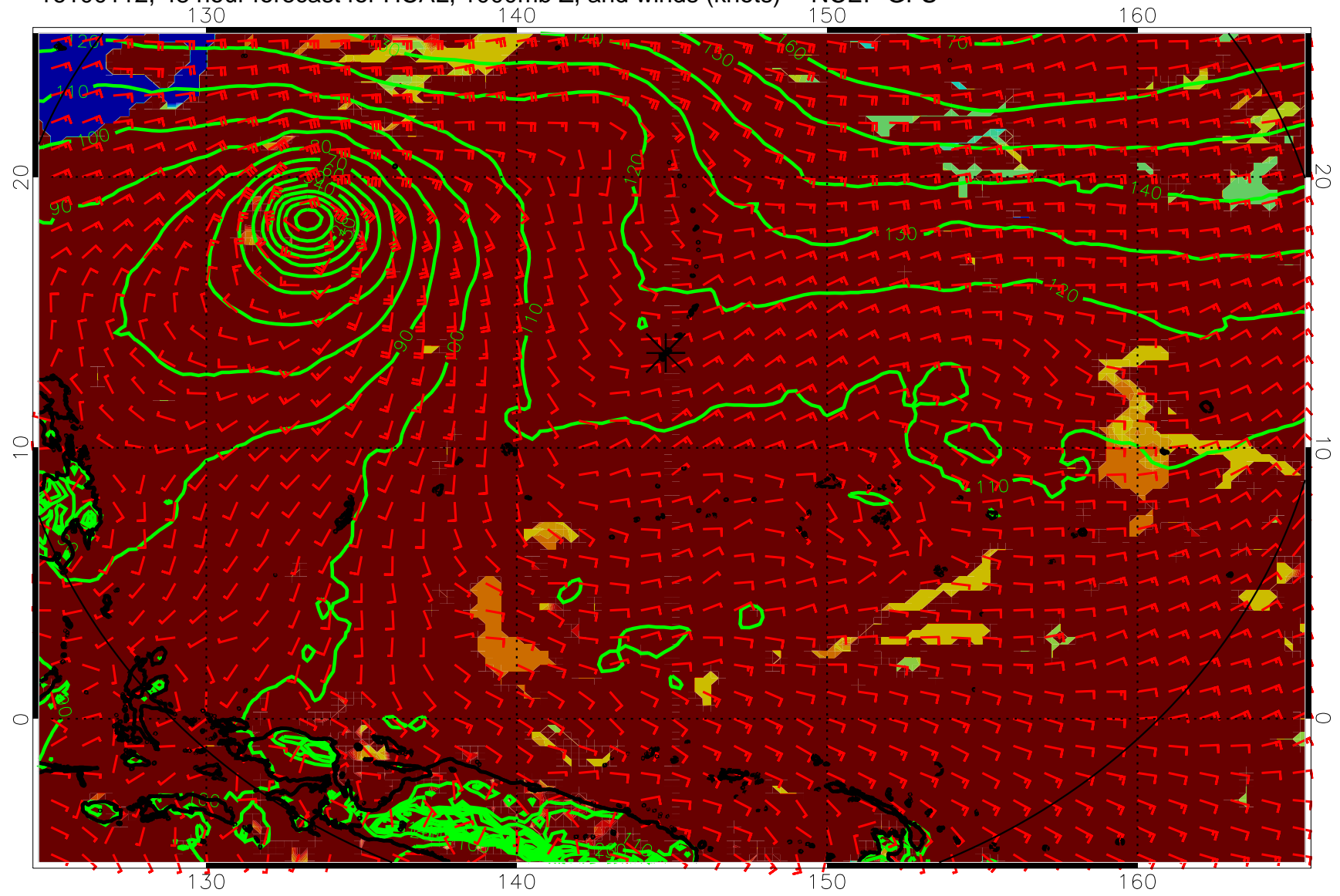
16100112, 48 hour forecast for HCAL, 1000mb Z, and winds (knots) -- NCEP GFS
