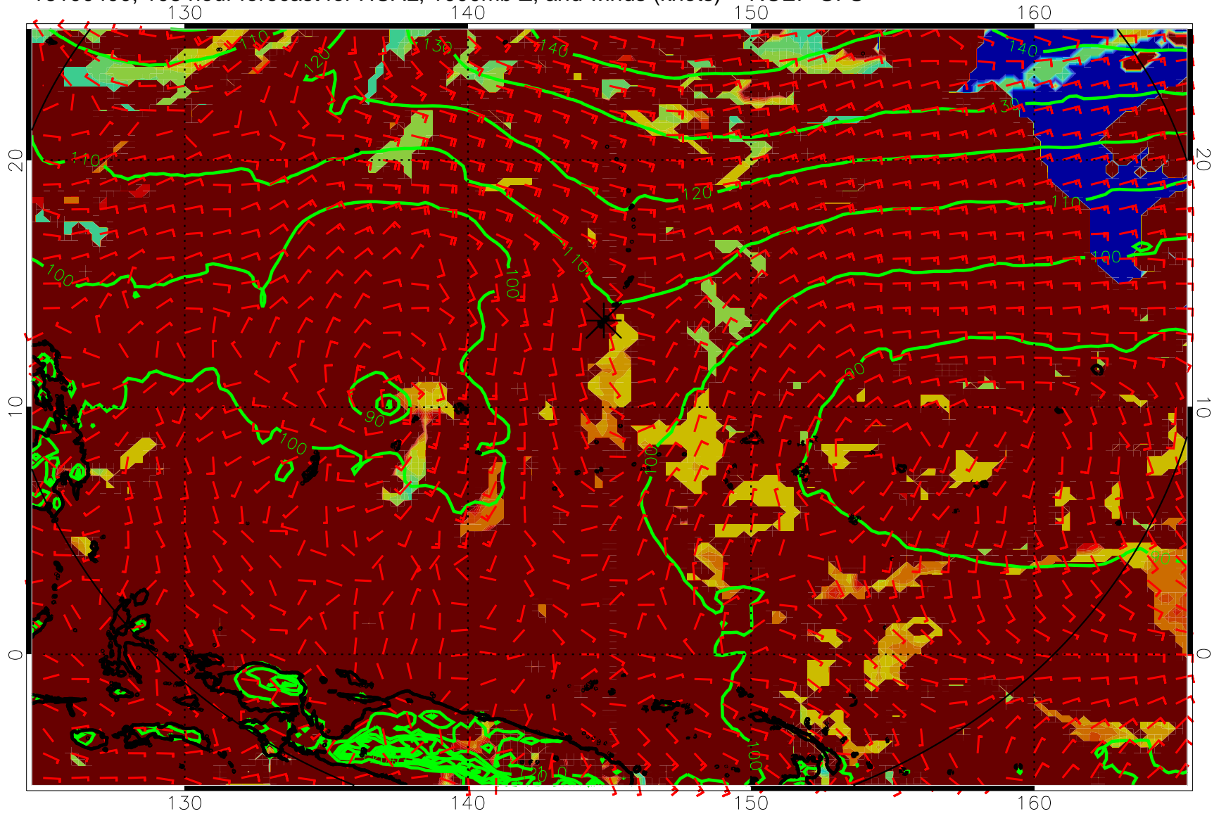
16100400, 108 hour forecast for HCAL, 1000mb Z, and winds (knots) -- NCEP GFS
