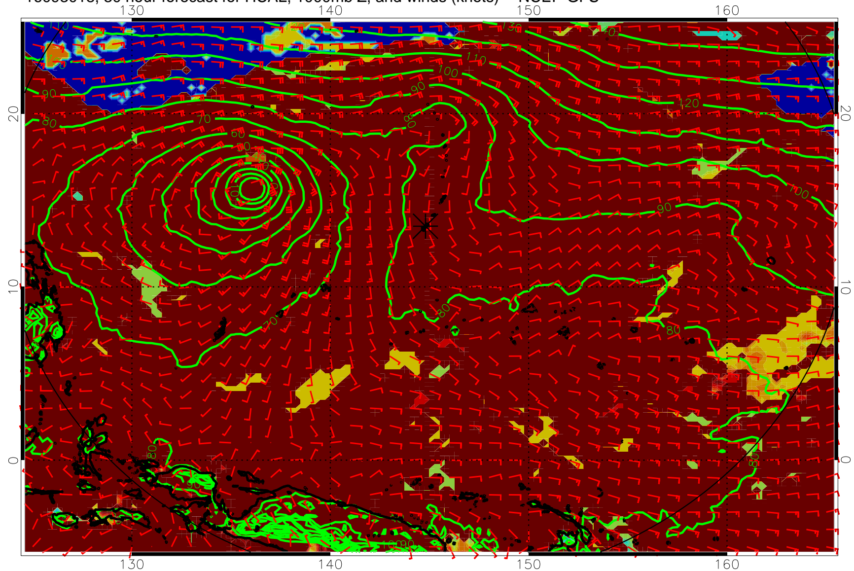
16093018, 30 hour forecast for HCAL, 1000mb Z, and winds (knots) -- NCEP GFS
