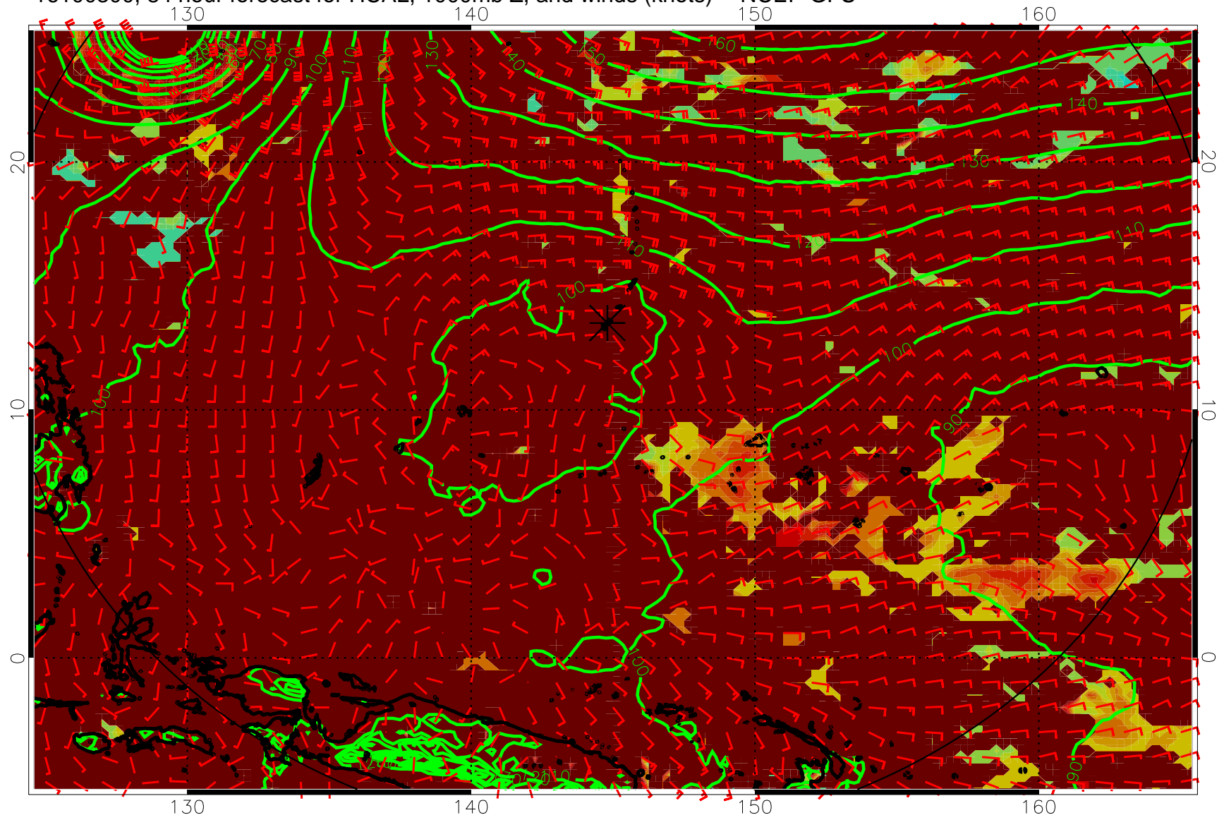
16100300, 84 hour forecast for HCAL, 1000mb Z, and winds (knots) -- NCEP GFS
