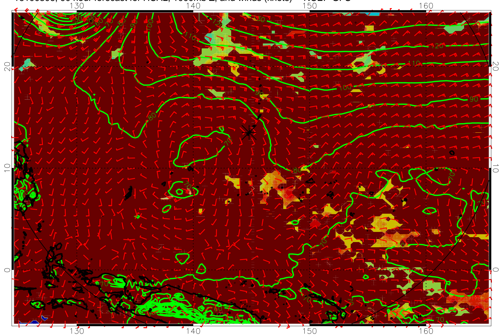
16100306, 90 hour forecast for HCAL, 1000mb Z, and winds (knots) -- NCEP GFS
