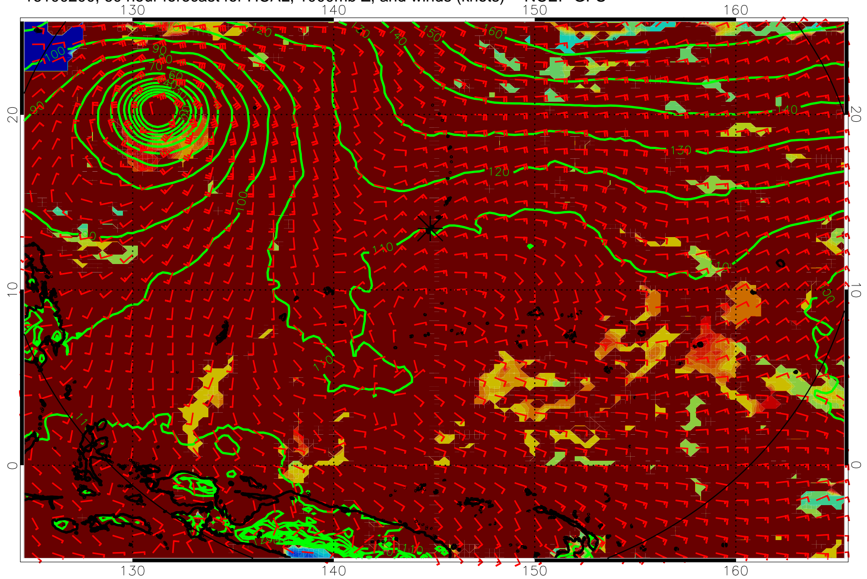
16100200, 60 hour forecast for HCAL, 1000mb Z, and winds (knots) -- NCEP GFS
