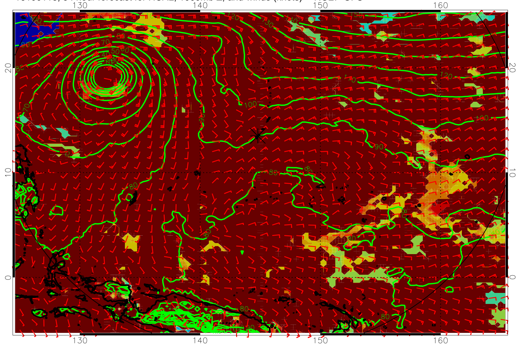
16100118, 54 hour forecast for HCAL, 1000mb Z, and winds (knots) -- NCEP GFS
