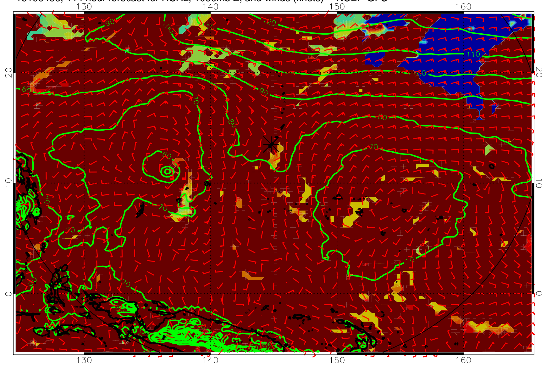
16100406, 114 hour forecast for HCAL, 1000mb Z, and winds (knots) -- NCEP GFS
