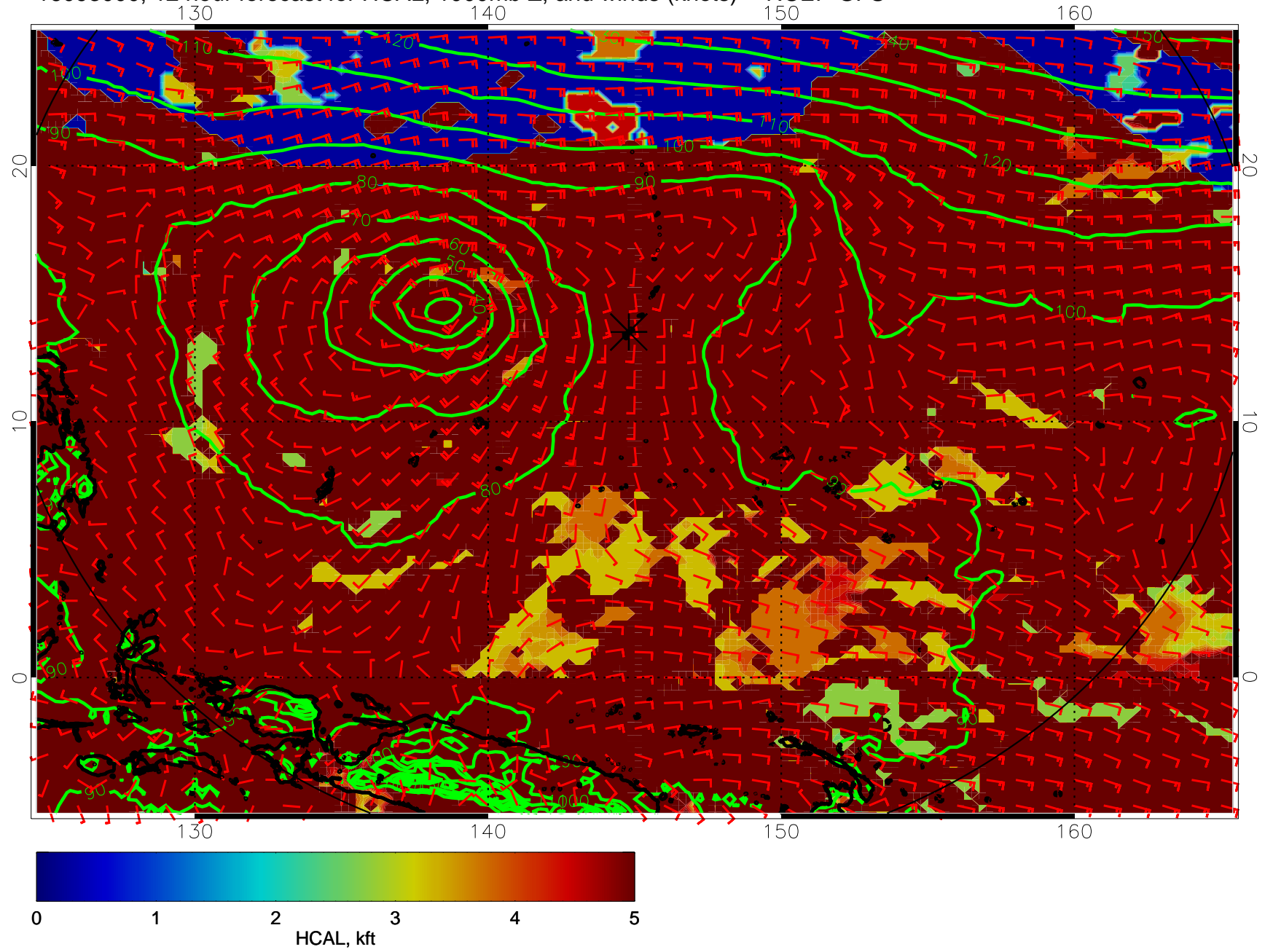
16093000, 12 hour forecast for HCAL, 1000mb Z, and winds (knots) -- NCEP GFS
