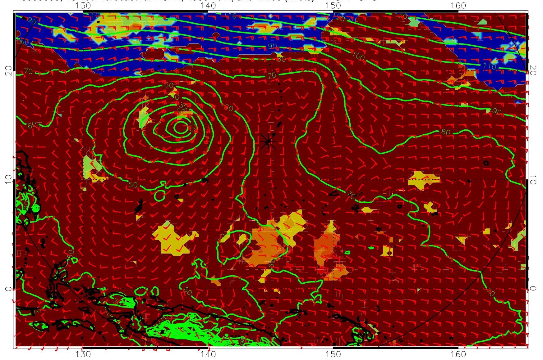
16093006, 18 hour forecast for HCAL, 1000mb Z, and winds (knots) -- NCEP GFS
