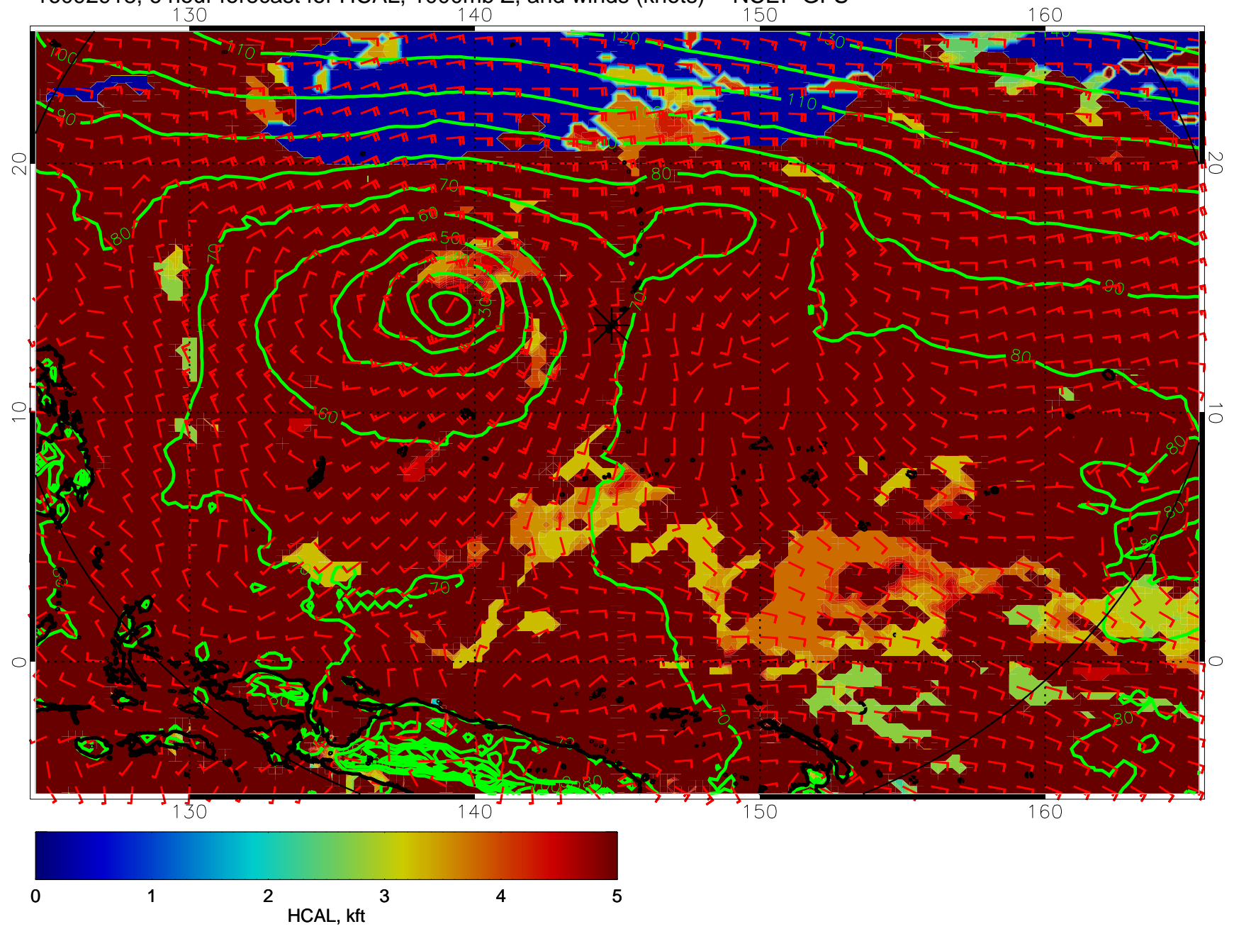
16092918, 6 hour forecast for HCAL, 1000mb Z, and winds (knots) -- NCEP GFS
