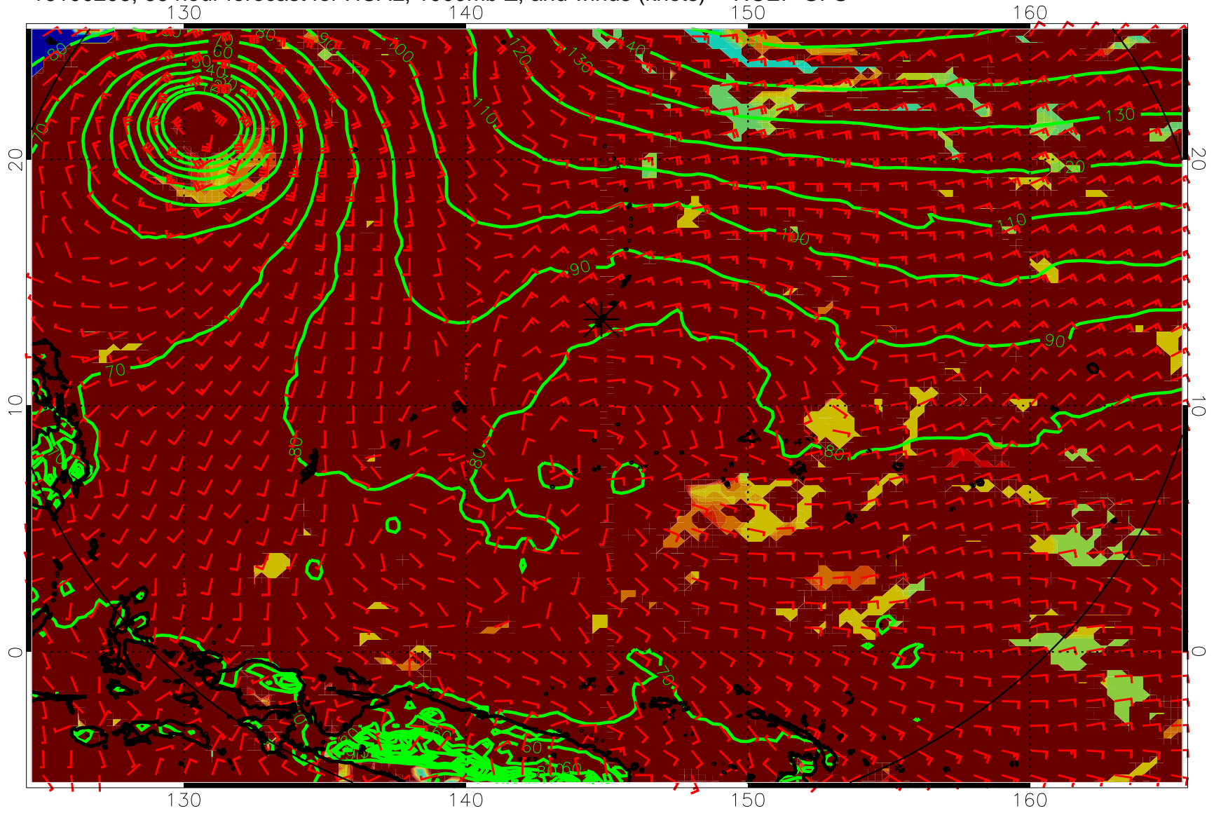
16100206, 66 hour forecast for HCAL, 1000mb Z, and winds (knots) -- NCEP GFS
