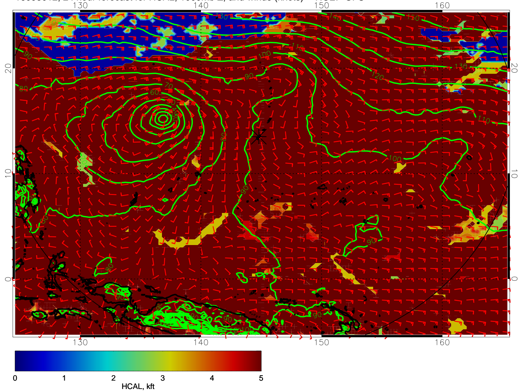
16093012, 24 hour forecast for HCAL, 1000mb Z, and winds (knots) -- NCEP GFS
