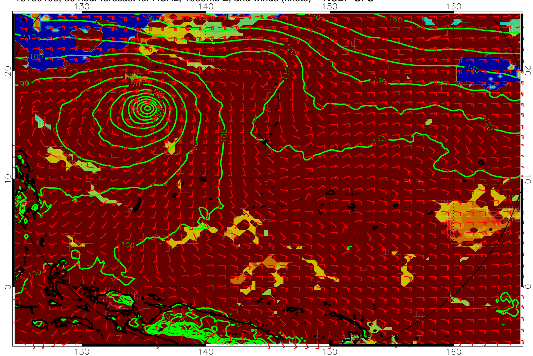
16100100, 36 hour forecast for HCAL, 1000mb Z, and winds (knots) -- NCEP GFS
