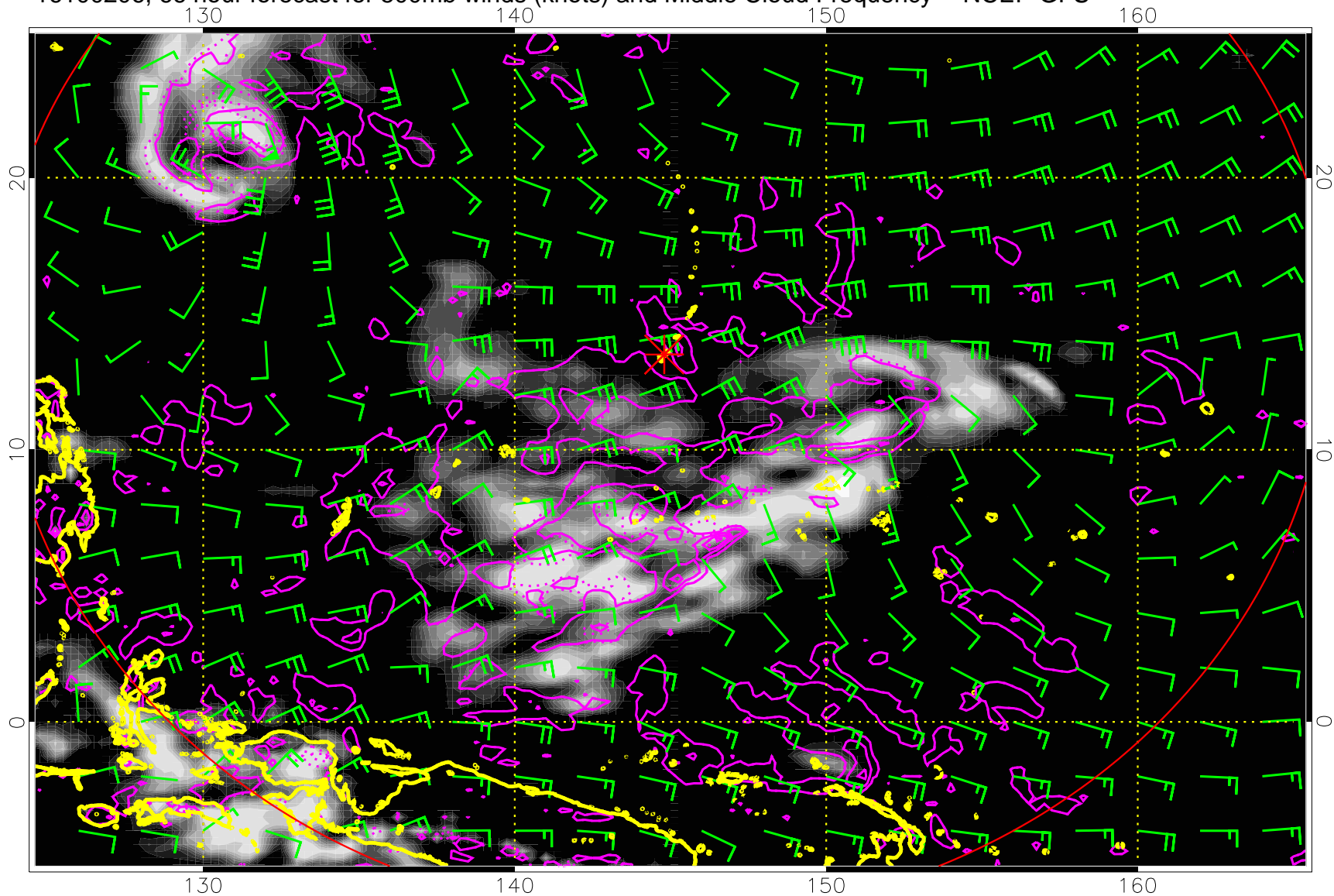
16100206, 66 hour forecast for 500mb winds (knots) and Middle Cloud Frequency -- NCEP GFS
