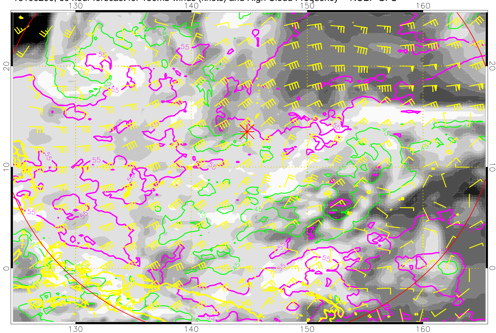
16100200, 60 hour forecast for 150mb winds (knots) and High Cloud Frequency -- NCEP GFS
