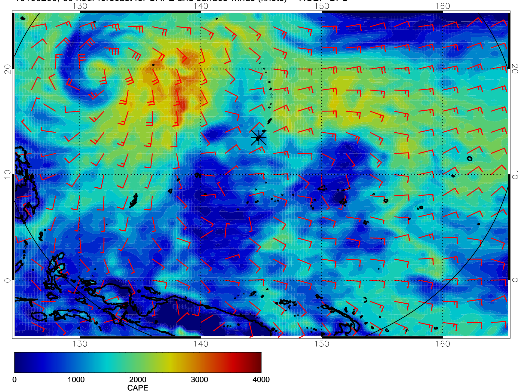
16100200, 60 hour forecast for CAPE and surface winds (knots) -- NCEP GFS
