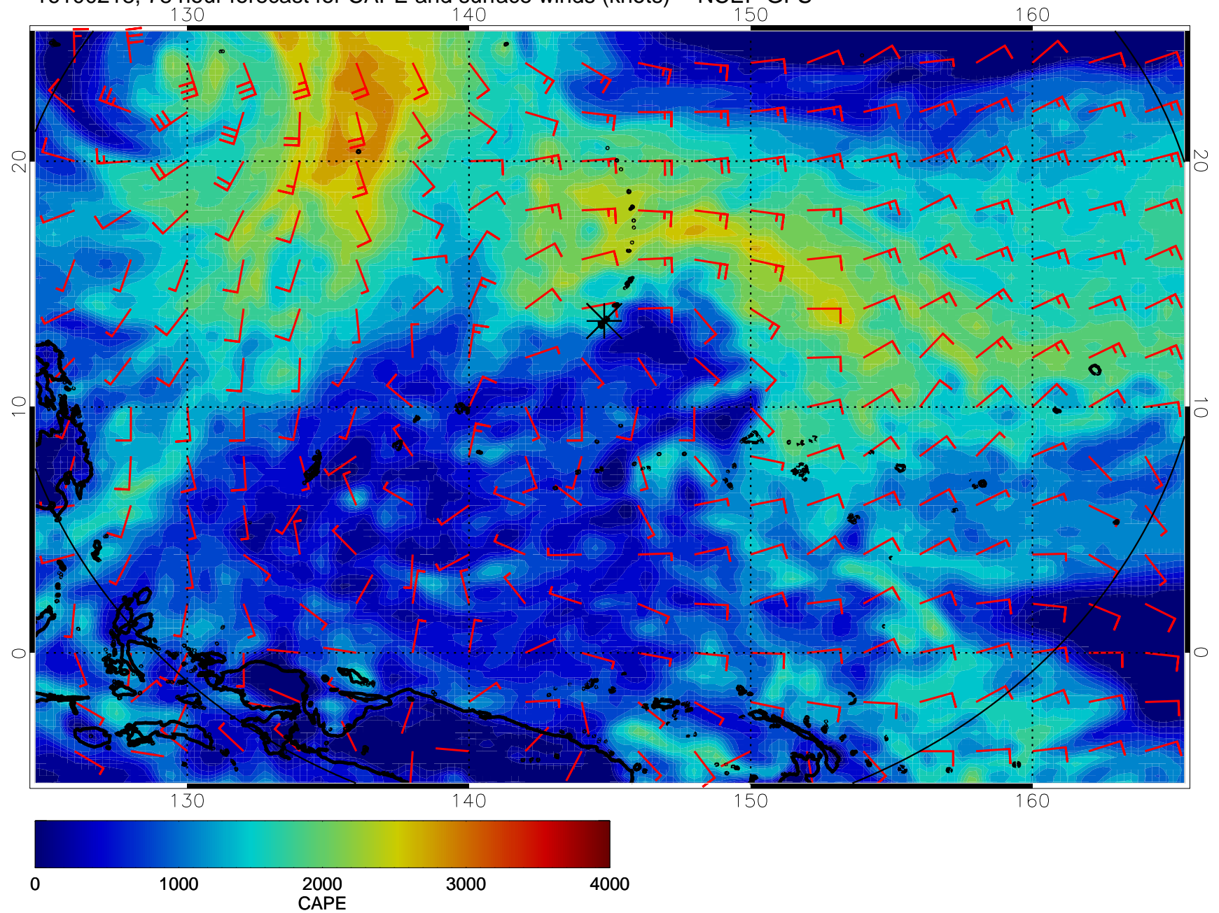
16100218, 78 hour forecast for CAPE and surface winds (knots) -- NCEP GFS
