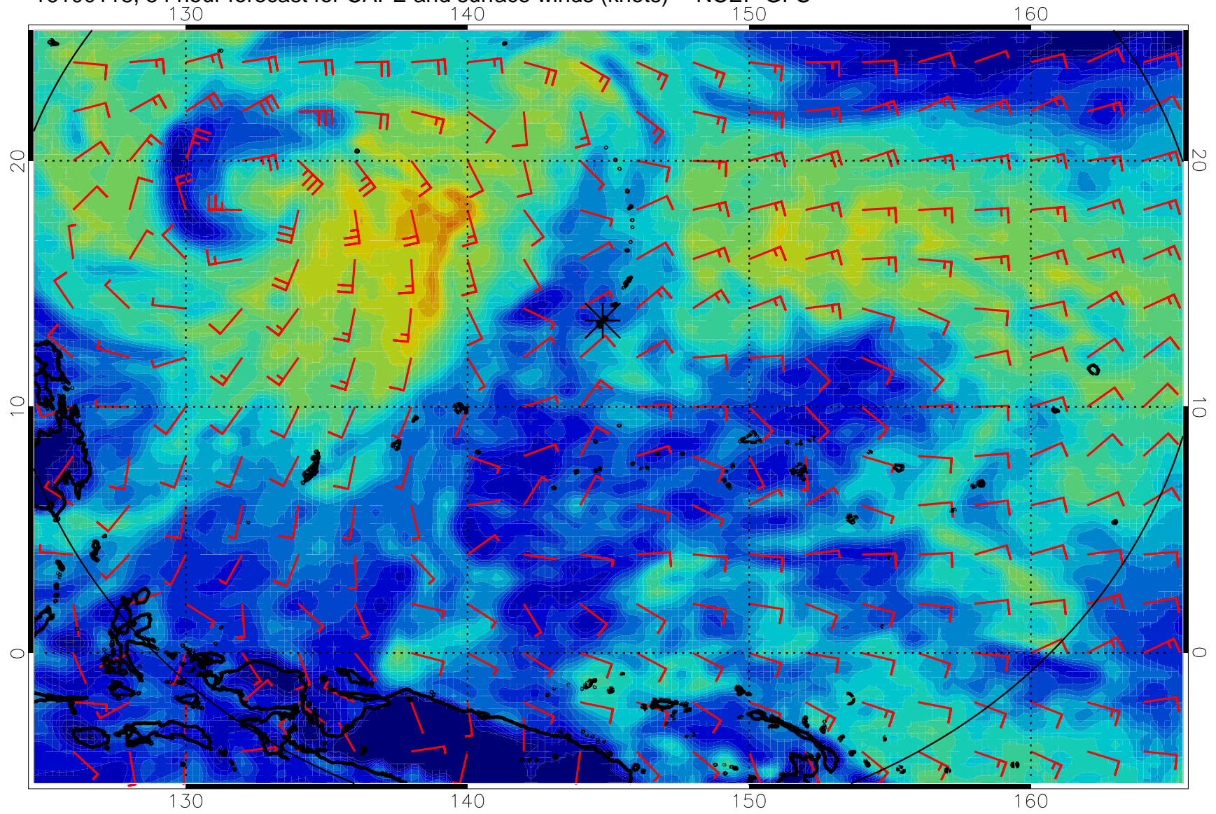
16100118, 54 hour forecast for CAPE and surface winds (knots) -- NCEP GFS
