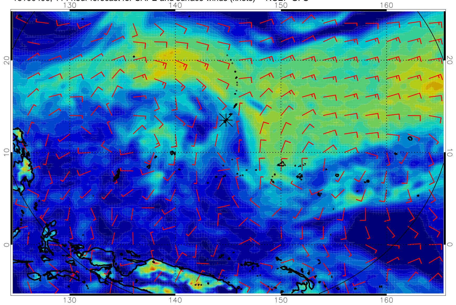
16100406, 114 hour forecast for CAPE and surface winds (knots) -- NCEP GFS
