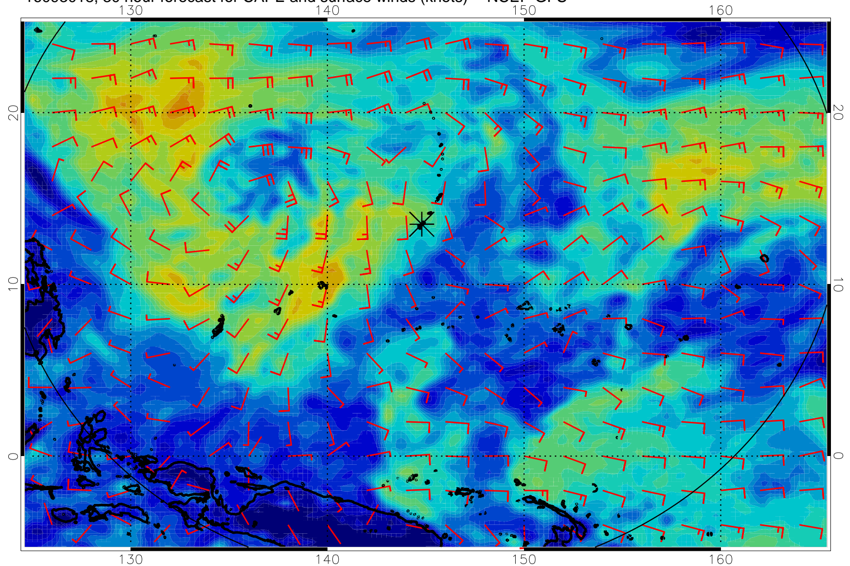
16093018, 30 hour forecast for CAPE and surface winds (knots) -- NCEP GFS
