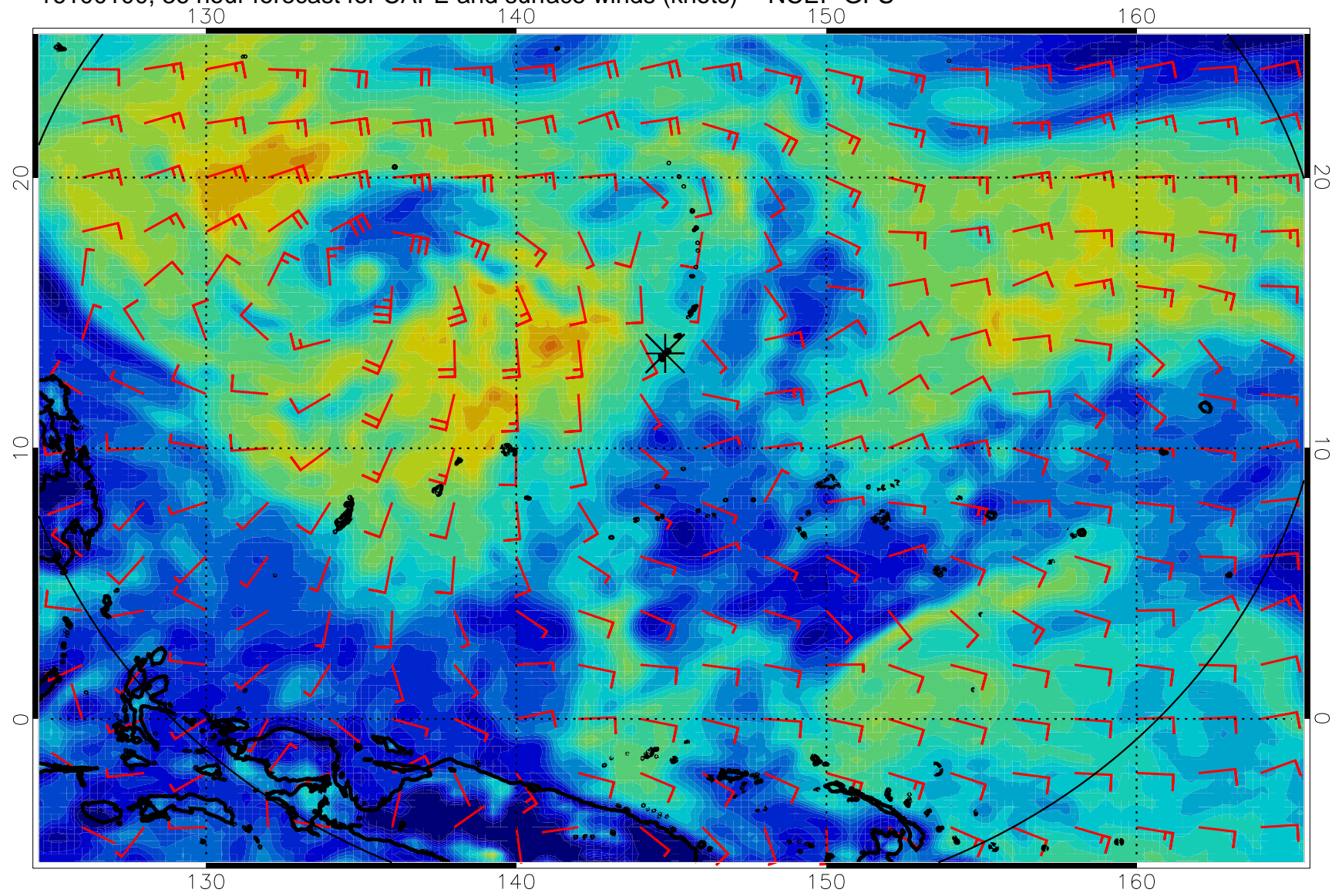
16100100, 36 hour forecast for CAPE and surface winds (knots) -- NCEP GFS
