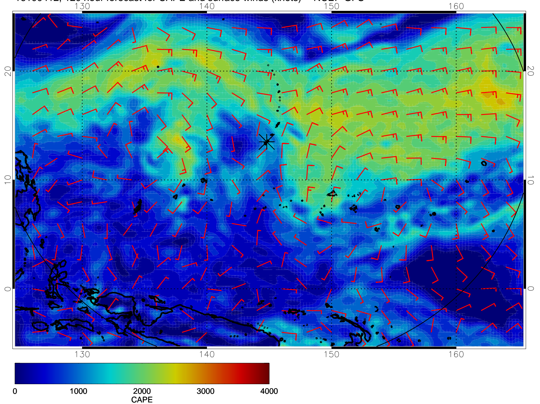
16100412, 120 hour forecast for CAPE and surface winds (knots) -- NCEP GFS
