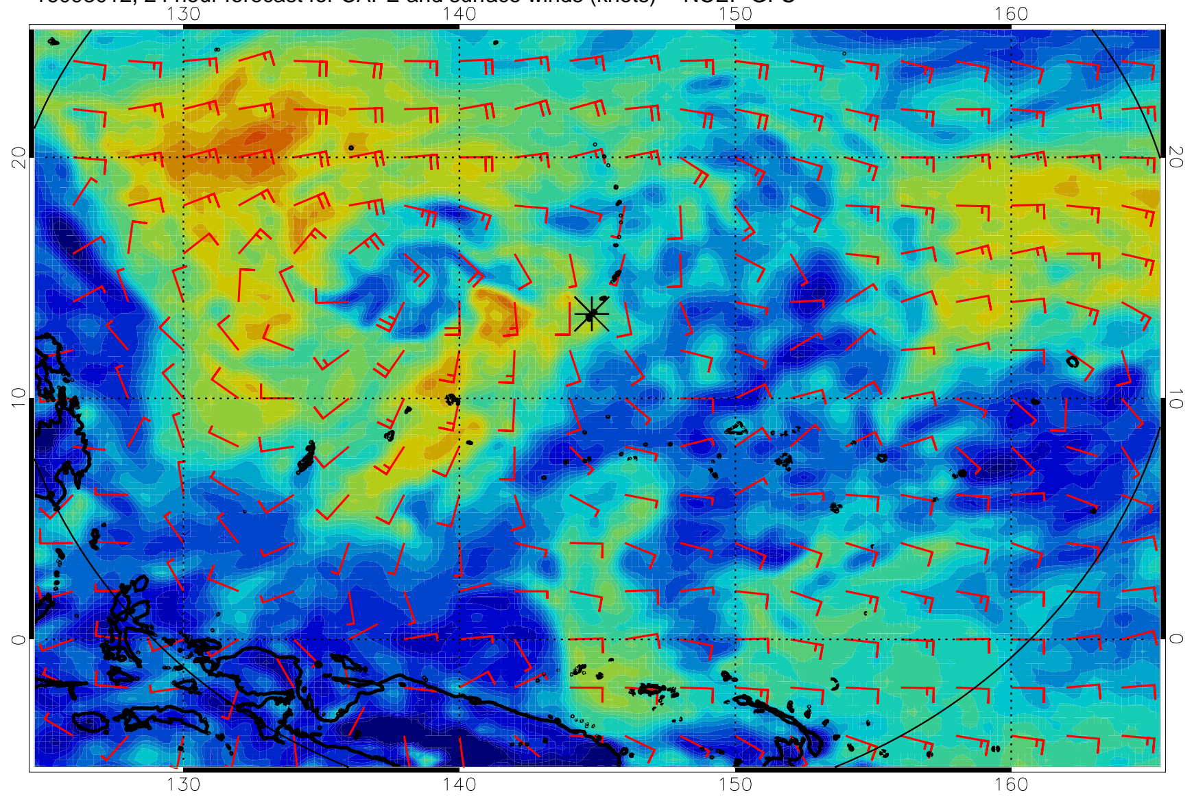
16093012, 24 hour forecast for CAPE and surface winds (knots) -- NCEP GFS
