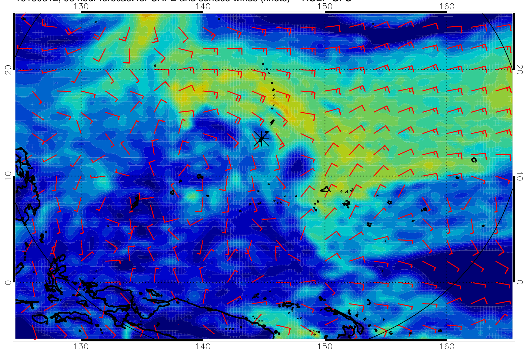
16100312, 96 hour forecast for CAPE and surface winds (knots) -- NCEP GFS
