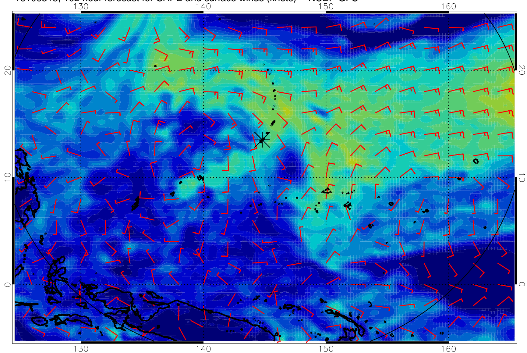
16100318, 102 hour forecast for CAPE and surface winds (knots) -- NCEP GFS
