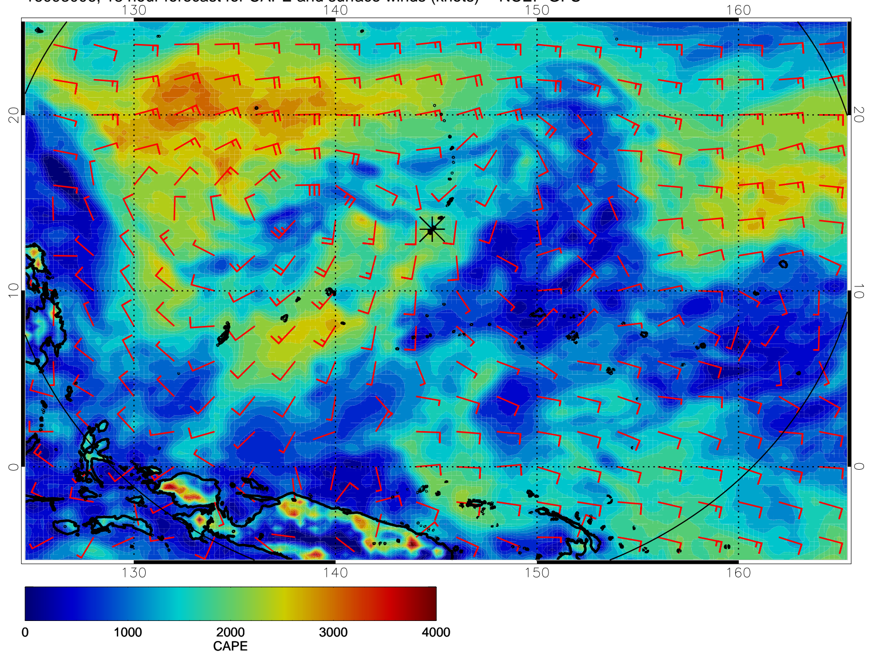
16093006, 18 hour forecast for CAPE and surface winds (knots) -- NCEP GFS
