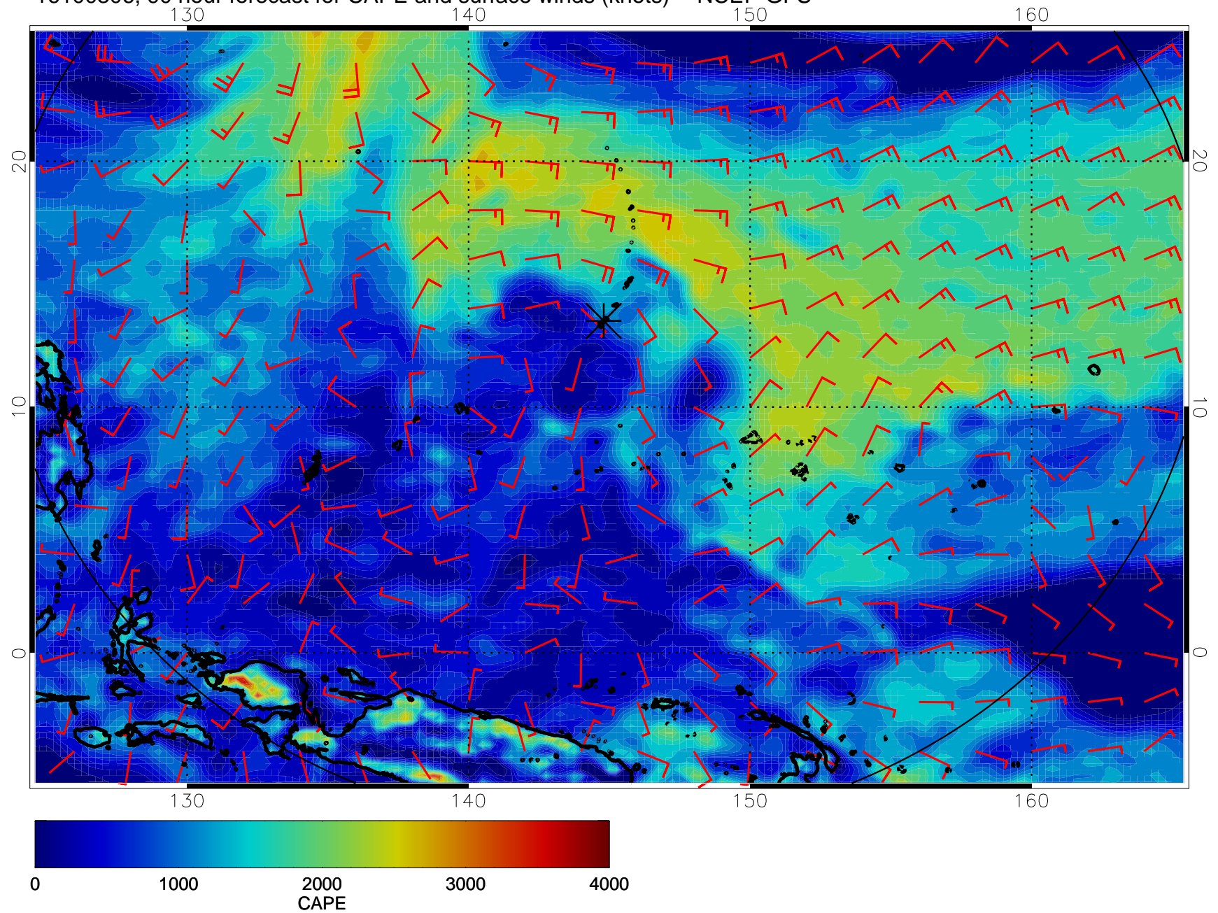
16100306, 90 hour forecast for CAPE and surface winds (knots) -- NCEP GFS
