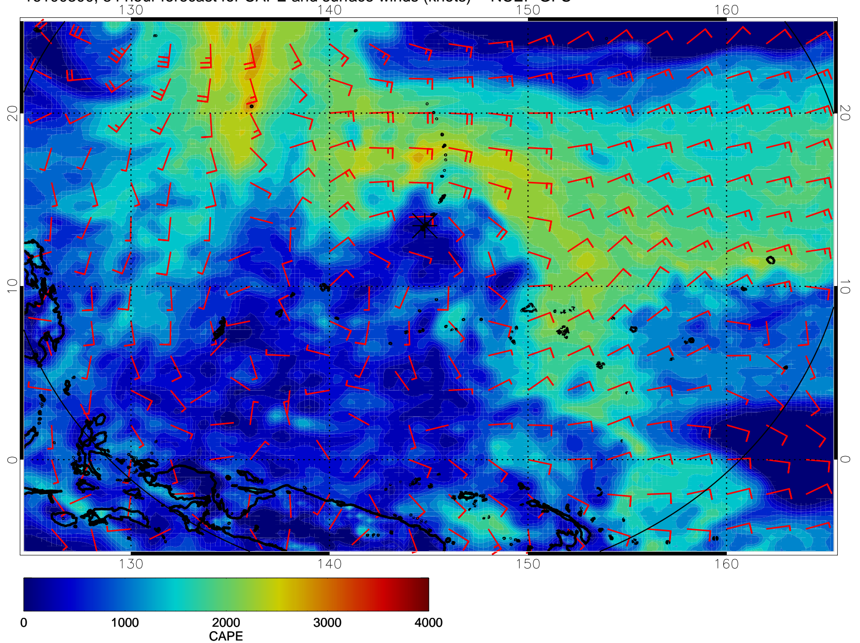
16100300, 84 hour forecast for CAPE and surface winds (knots) -- NCEP GFS
