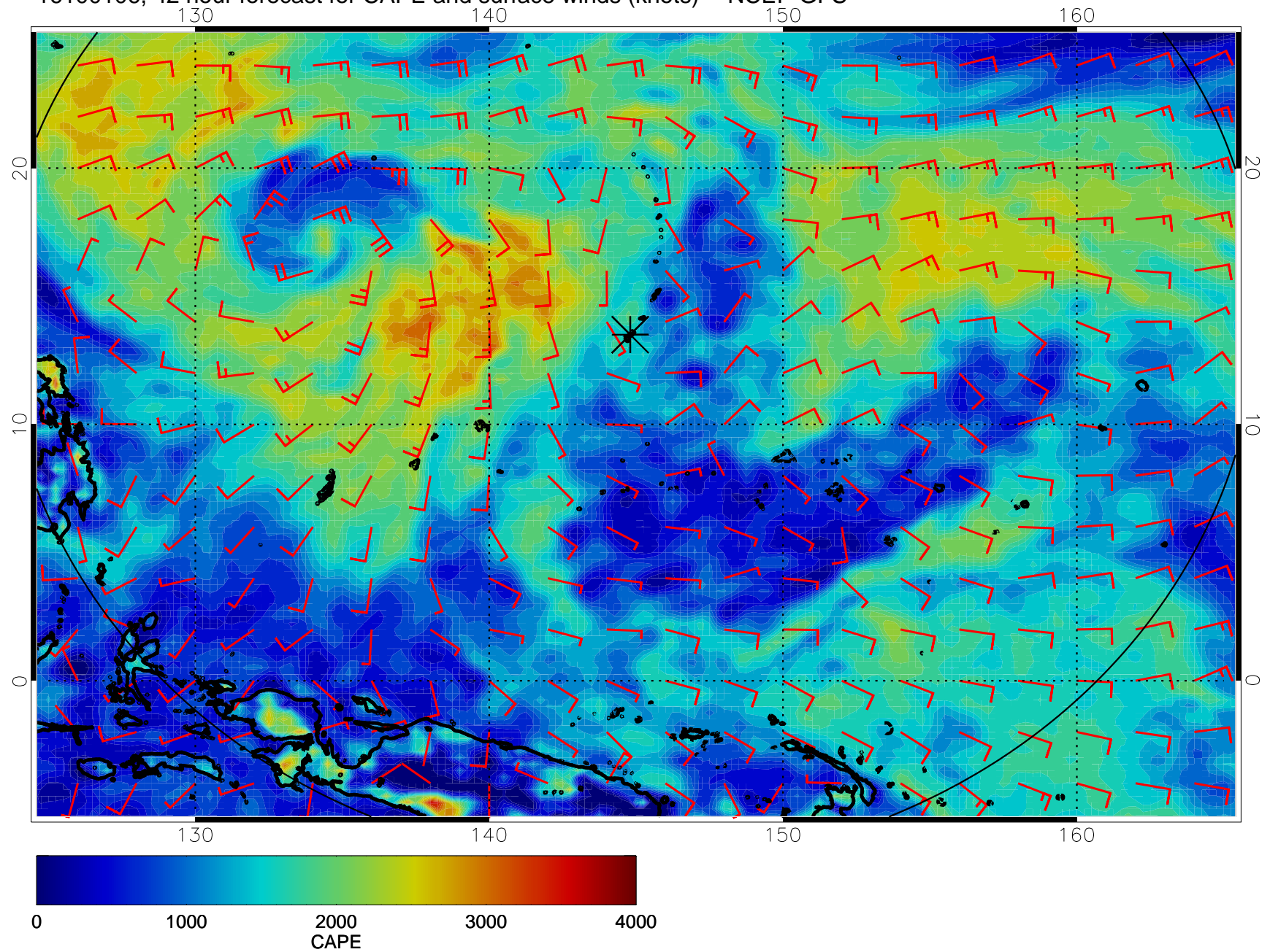
16100106, 42 hour forecast for CAPE and surface winds (knots) -- NCEP GFS
