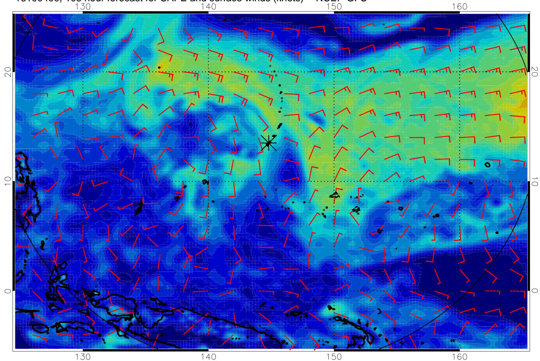
16100400, 108 hour forecast for CAPE and surface winds (knots) -- NCEP GFS
