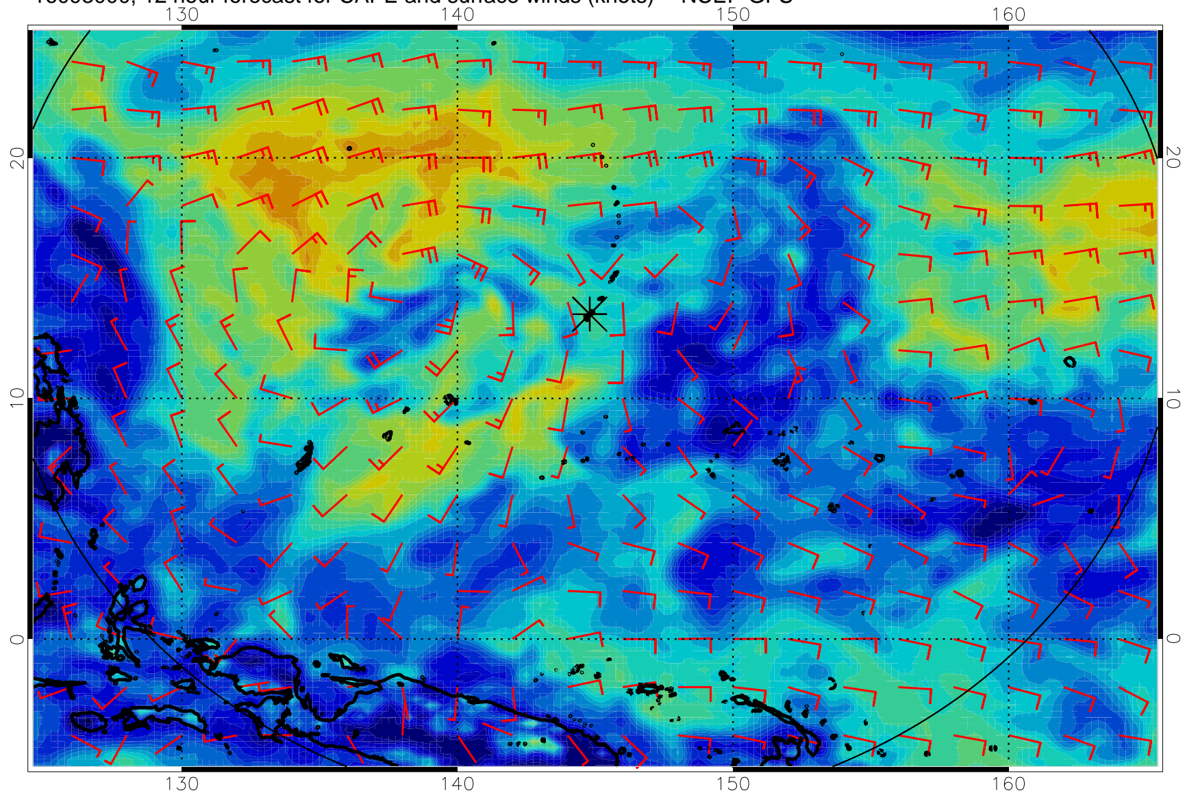
16093000, 12 hour forecast for CAPE and surface winds (knots) -- NCEP GFS
