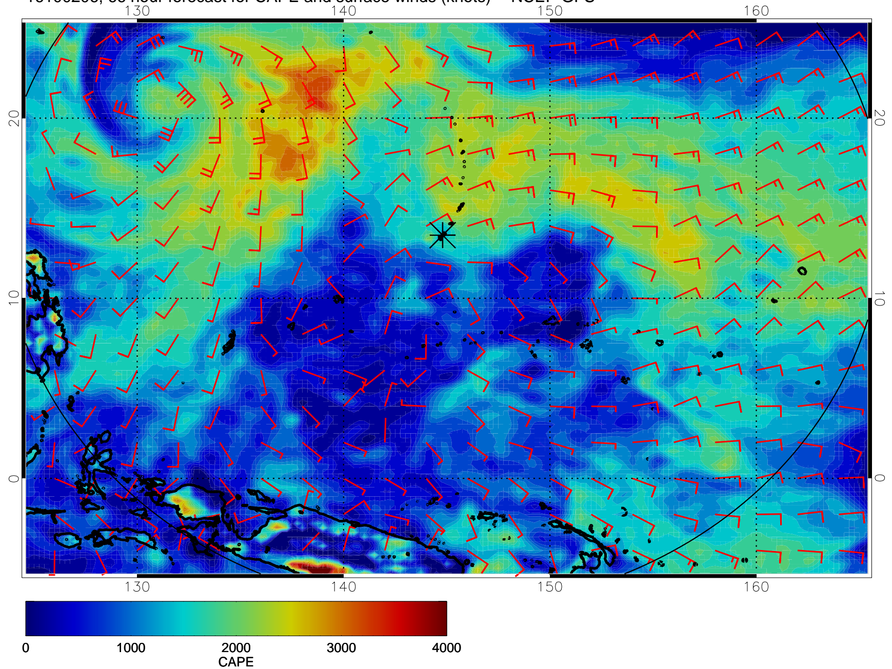
16100206, 66 hour forecast for CAPE and surface winds (knots) -- NCEP GFS
