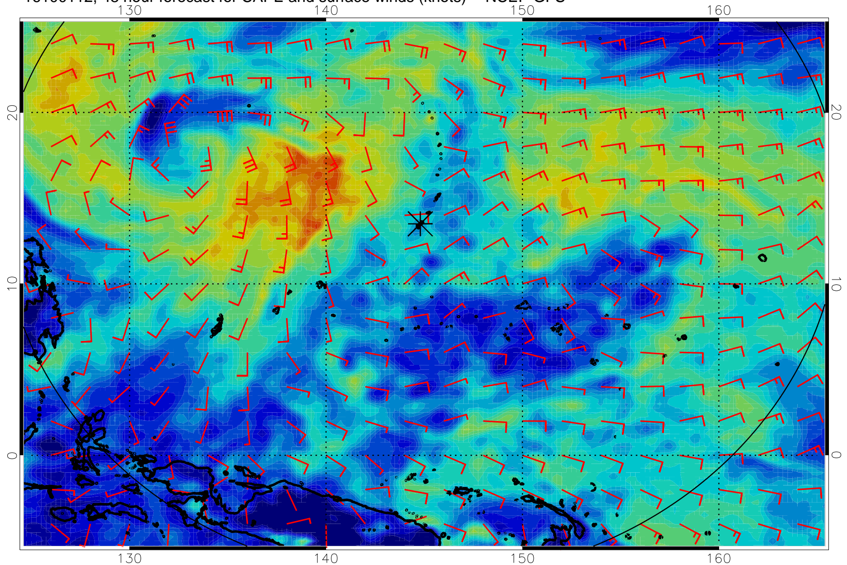
16100112, 48 hour forecast for CAPE and surface winds (knots) -- NCEP GFS
