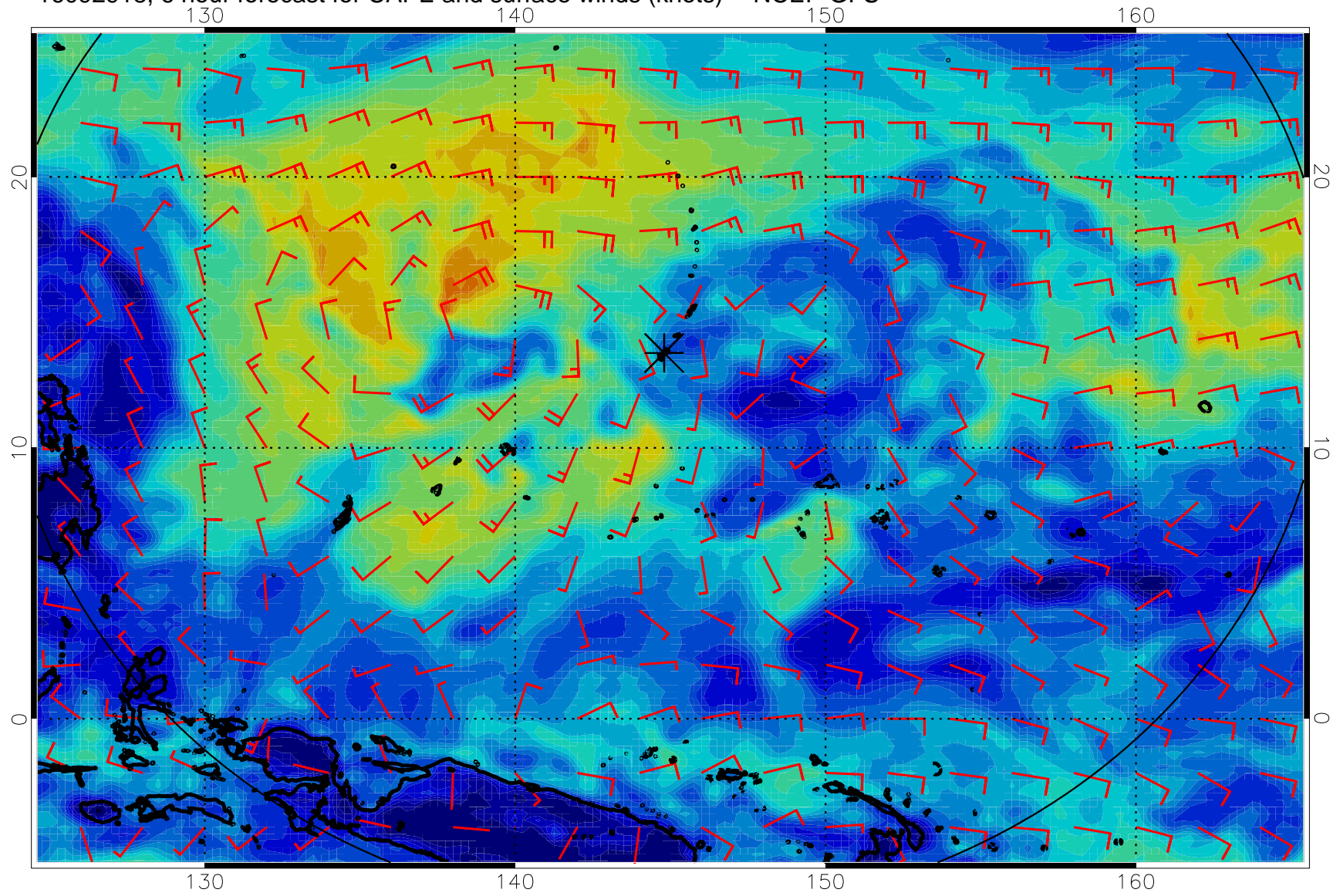
16092918, 6 hour forecast for CAPE and surface winds (knots) -- NCEP GFS
