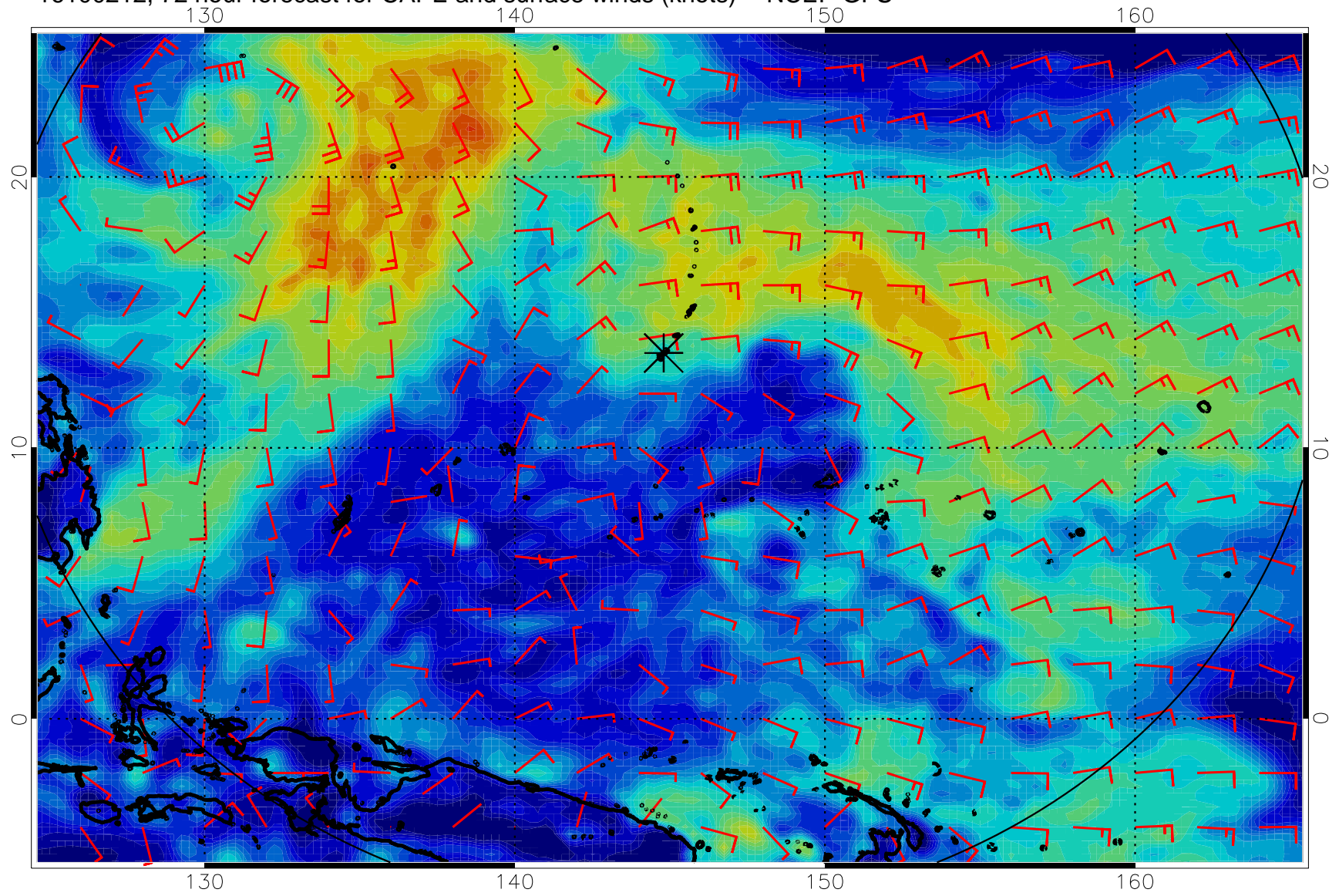
16100212, 72 hour forecast for CAPE and surface winds (knots) -- NCEP GFS
