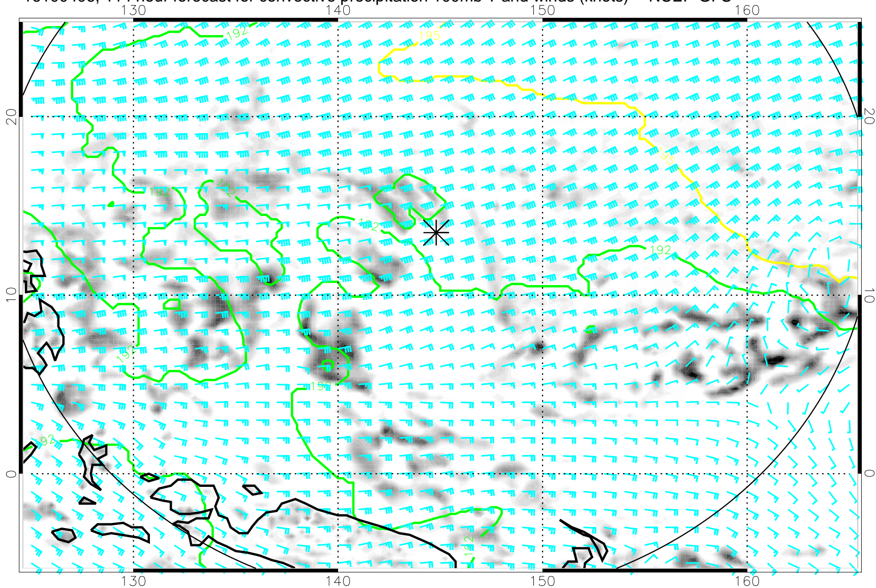
16100406, 114 hour forecast for convective precipitation 100mb T and winds (knots) -- NCEP GFS
