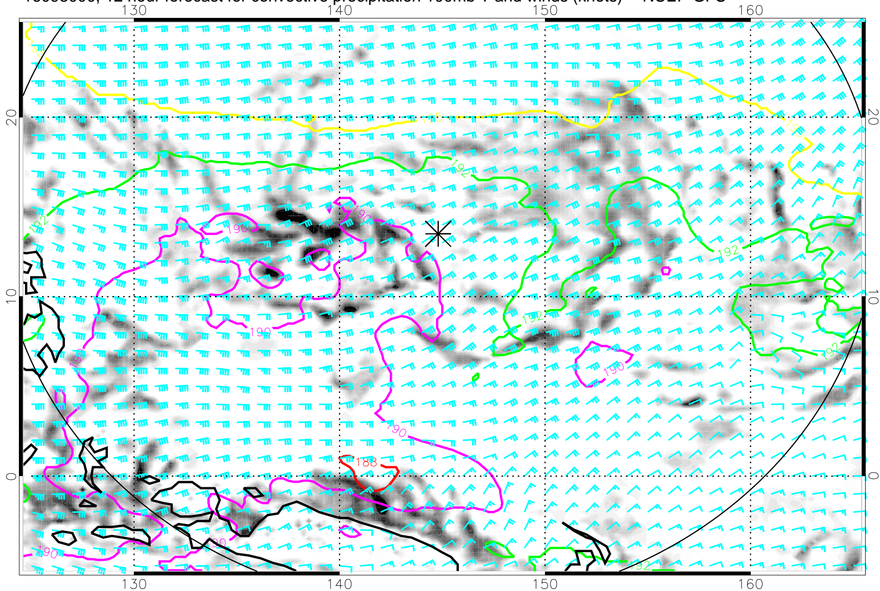
16093000, 12 hour forecast for convective precipitation 100mb T and winds (knots) -- NCEP GFS
