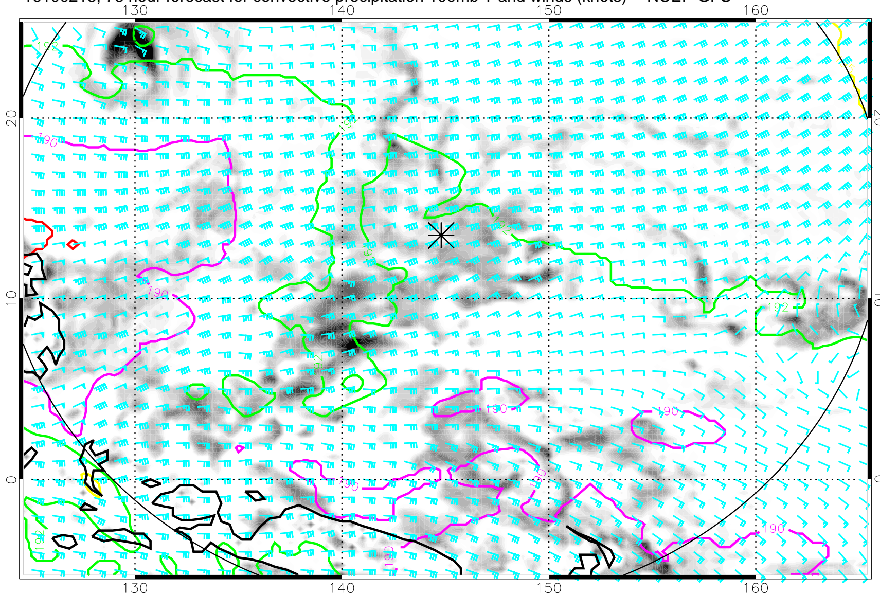
16100218, 78 hour forecast for convective precipitation 100mb T and winds (knots) -- NCEP GFS
