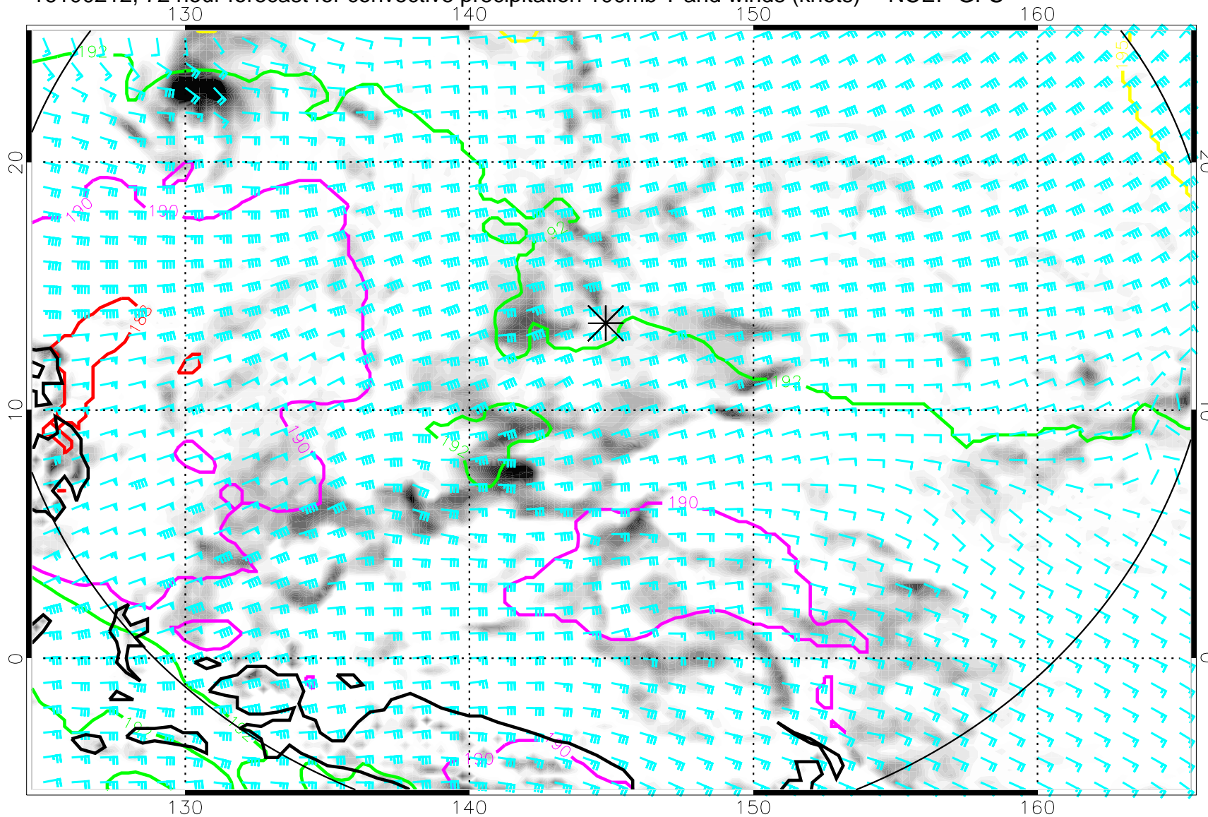
16100212, 72 hour forecast for convective precipitation 100mb T and winds (knots) -- NCEP GFS
