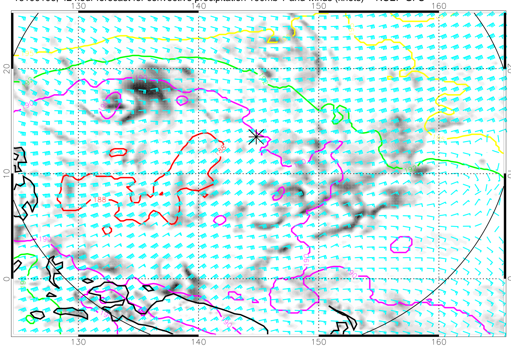
16100106, 42 hour forecast for convective precipitation 100mb T and winds (knots) -- NCEP GFS
