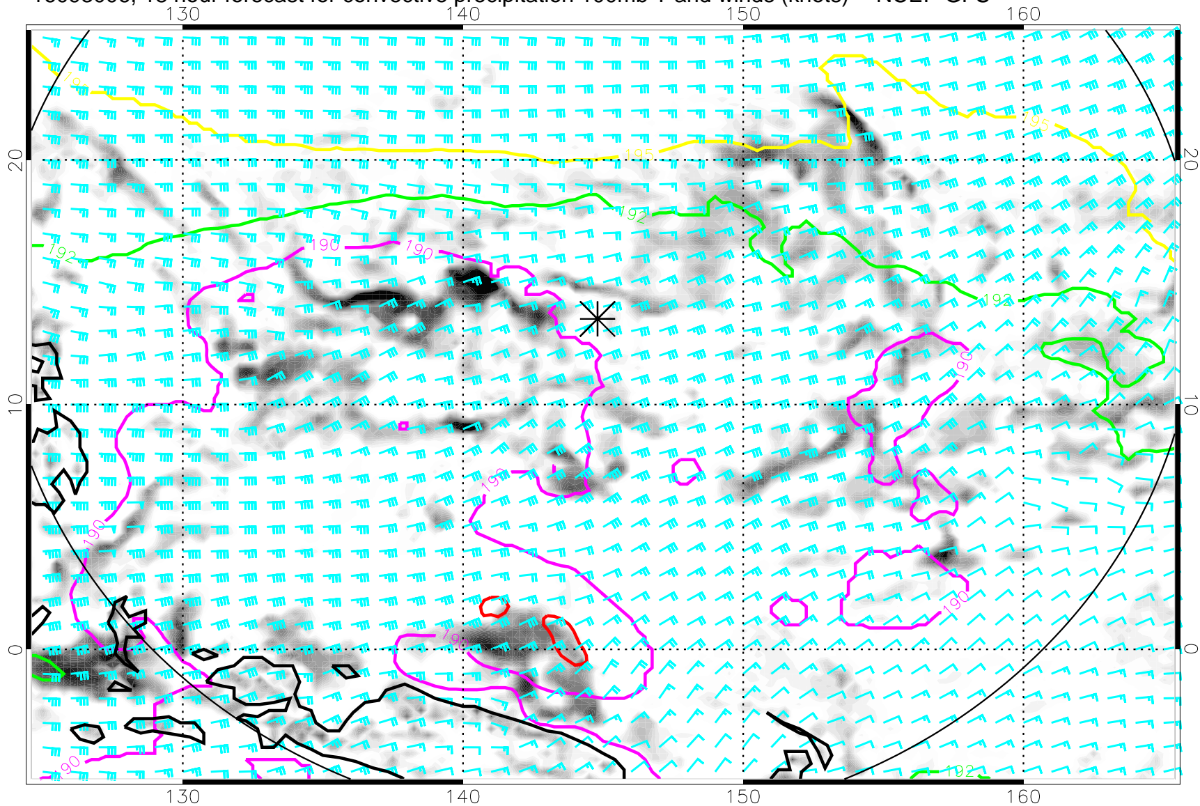
16093006, 18 hour forecast for convective precipitation 100mb T and winds (knots) -- NCEP GFS
