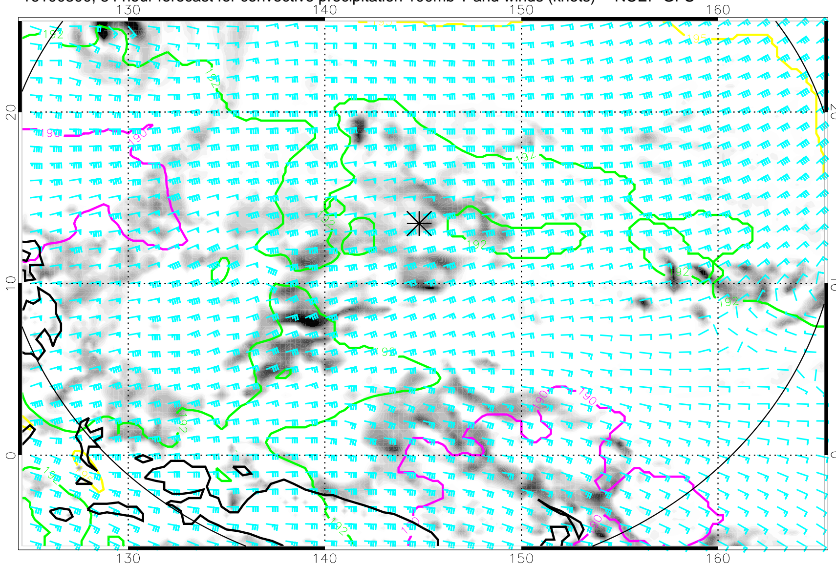
16100300, 84 hour forecast for convective precipitation 100mb T and winds (knots) -- NCEP GFS
