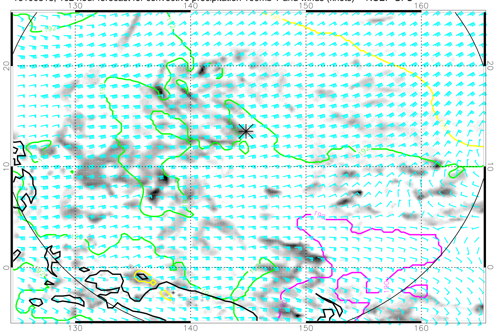
16100318, 102 hour forecast for convective precipitation 100mb T and winds (knots) -- NCEP GFS
