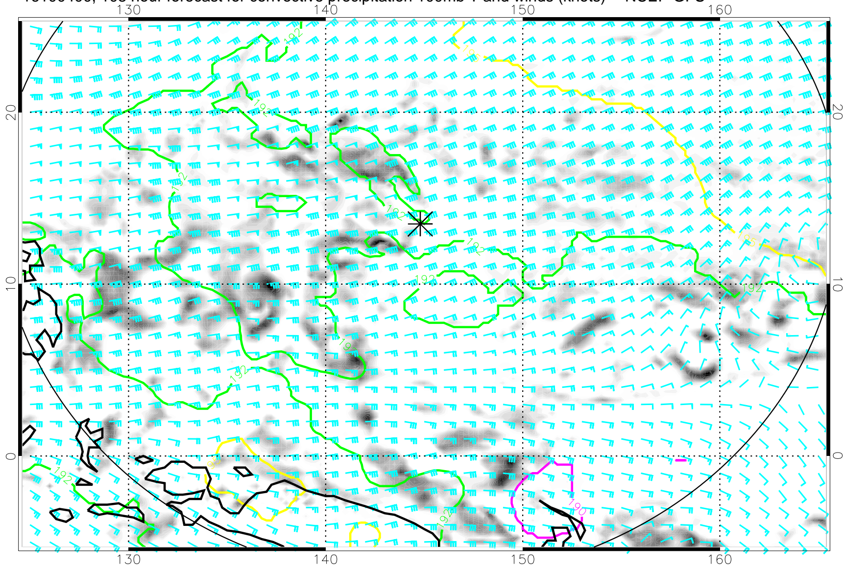
16100400, 108 hour forecast for convective precipitation 100mb T and winds (knots) -- NCEP GFS
