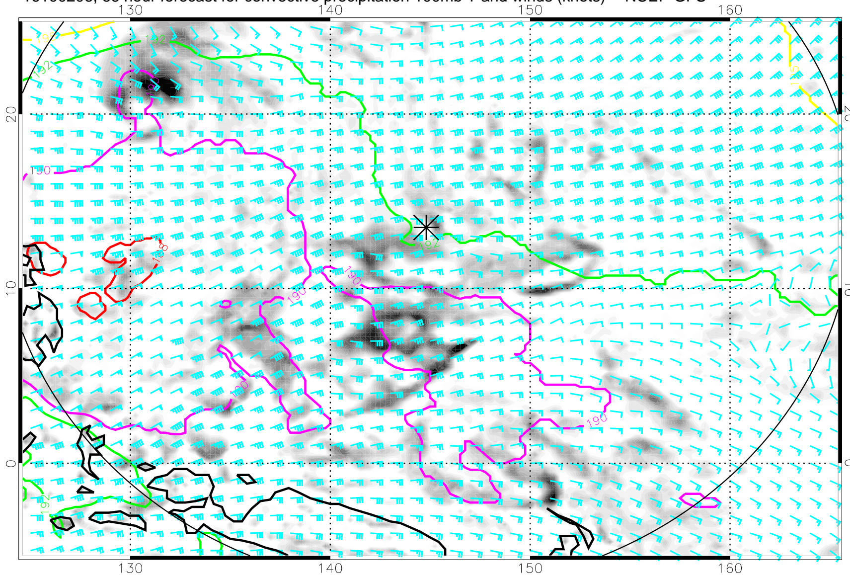
16100206, 66 hour forecast for convective precipitation 100mb T and winds (knots) -- NCEP GFS
