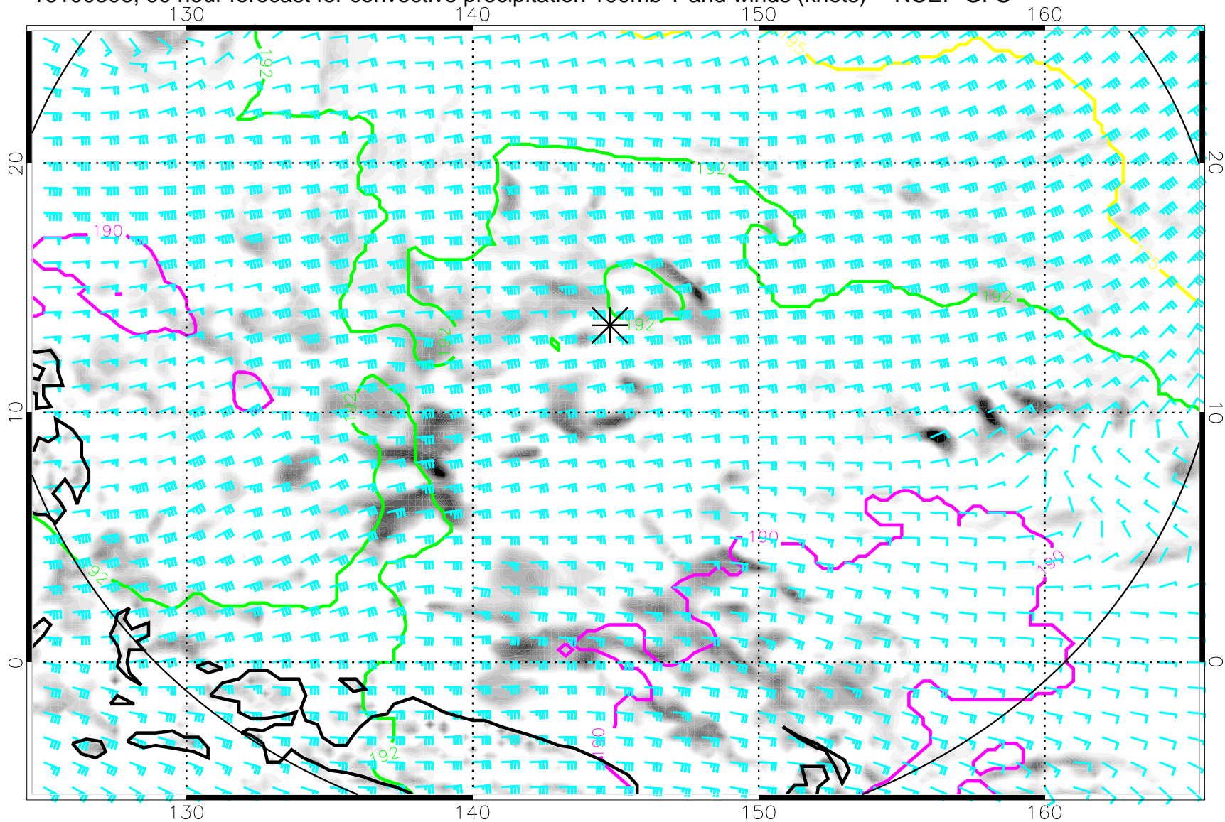
16100306, 90 hour forecast for convective precipitation 100mb T and winds (knots) -- NCEP GFS
