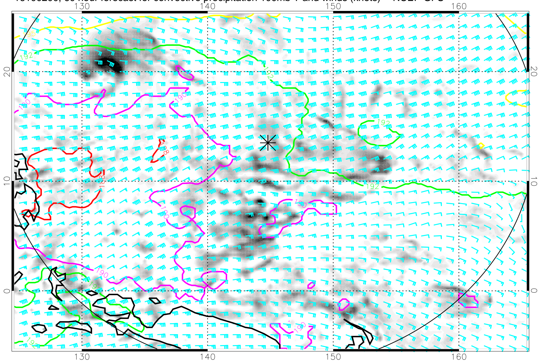
16100200, 60 hour forecast for convective precipitation 100mb T and winds (knots) -- NCEP GFS
