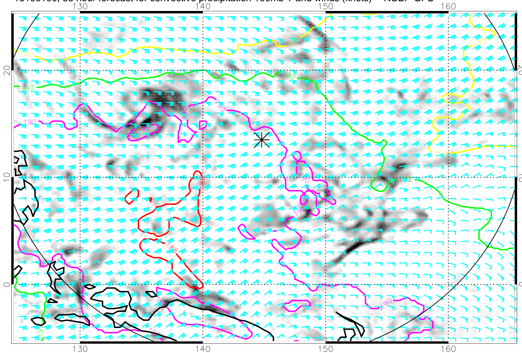
16100100, 36 hour forecast for convective precipitation 100mb T and winds (knots) -- NCEP GFS
