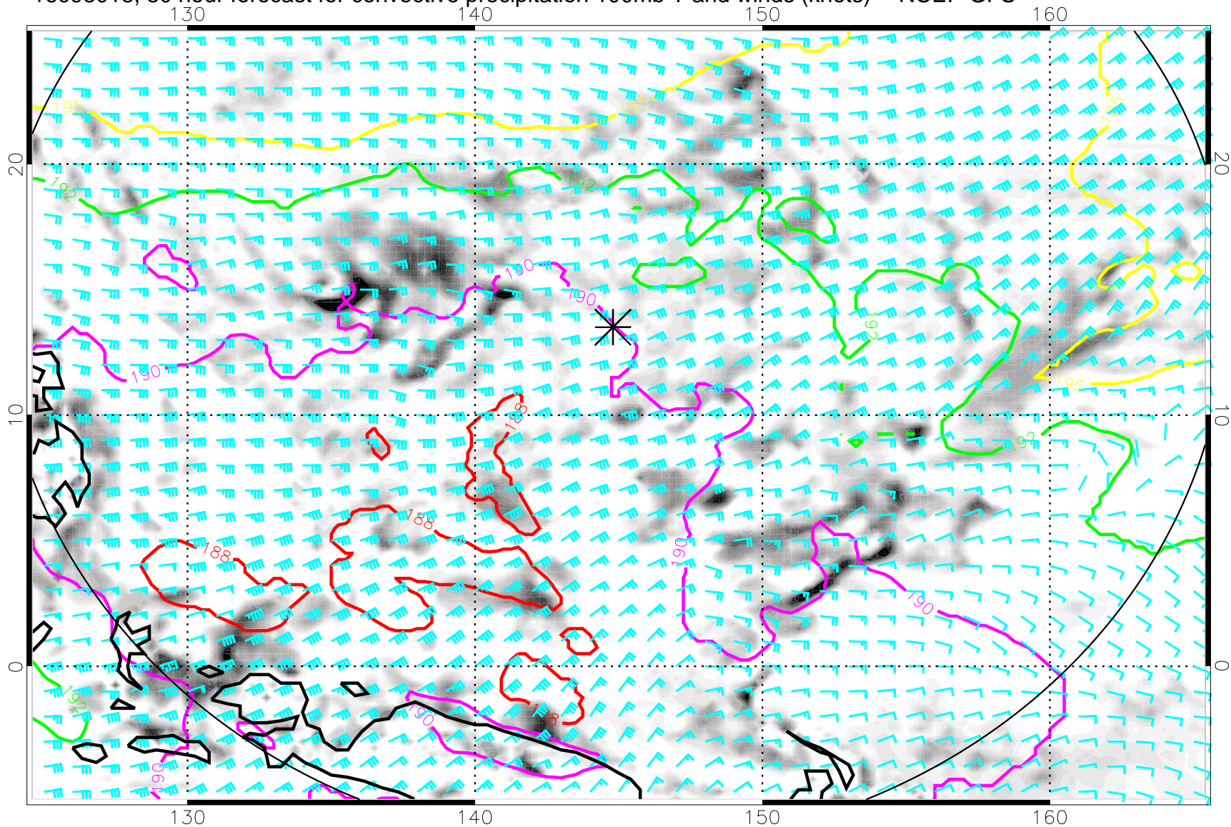
16093018, 30 hour forecast for convective precipitation 100mb T and winds (knots) -- NCEP GFS
