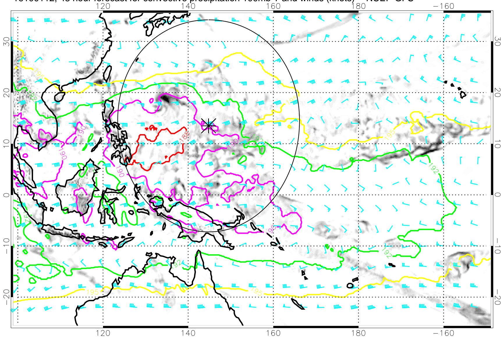
16100112, 48 hour forecast for convective precipitation 100mb T and winds (knots) -- NCEP GFS
