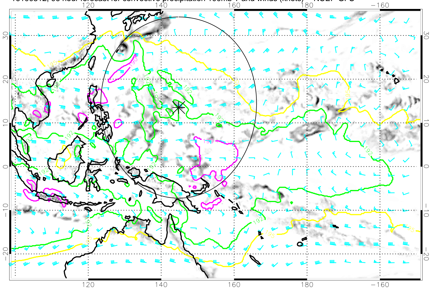
16100312, 96 hour forecast for convective precipitation 100mb T and winds (knots) -- NCEP GFS
