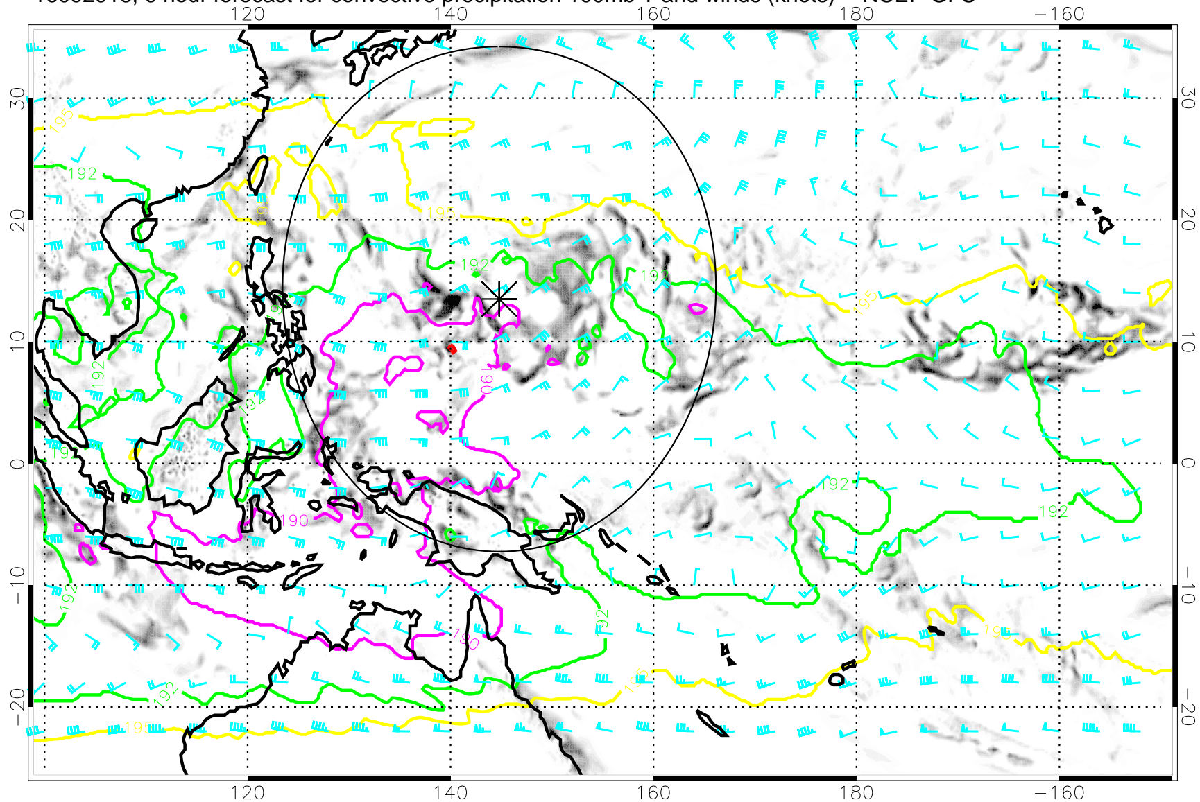
16092918, 6 hour forecast for convective precipitation 100mb T and winds (knots) -- NCEP GFS
