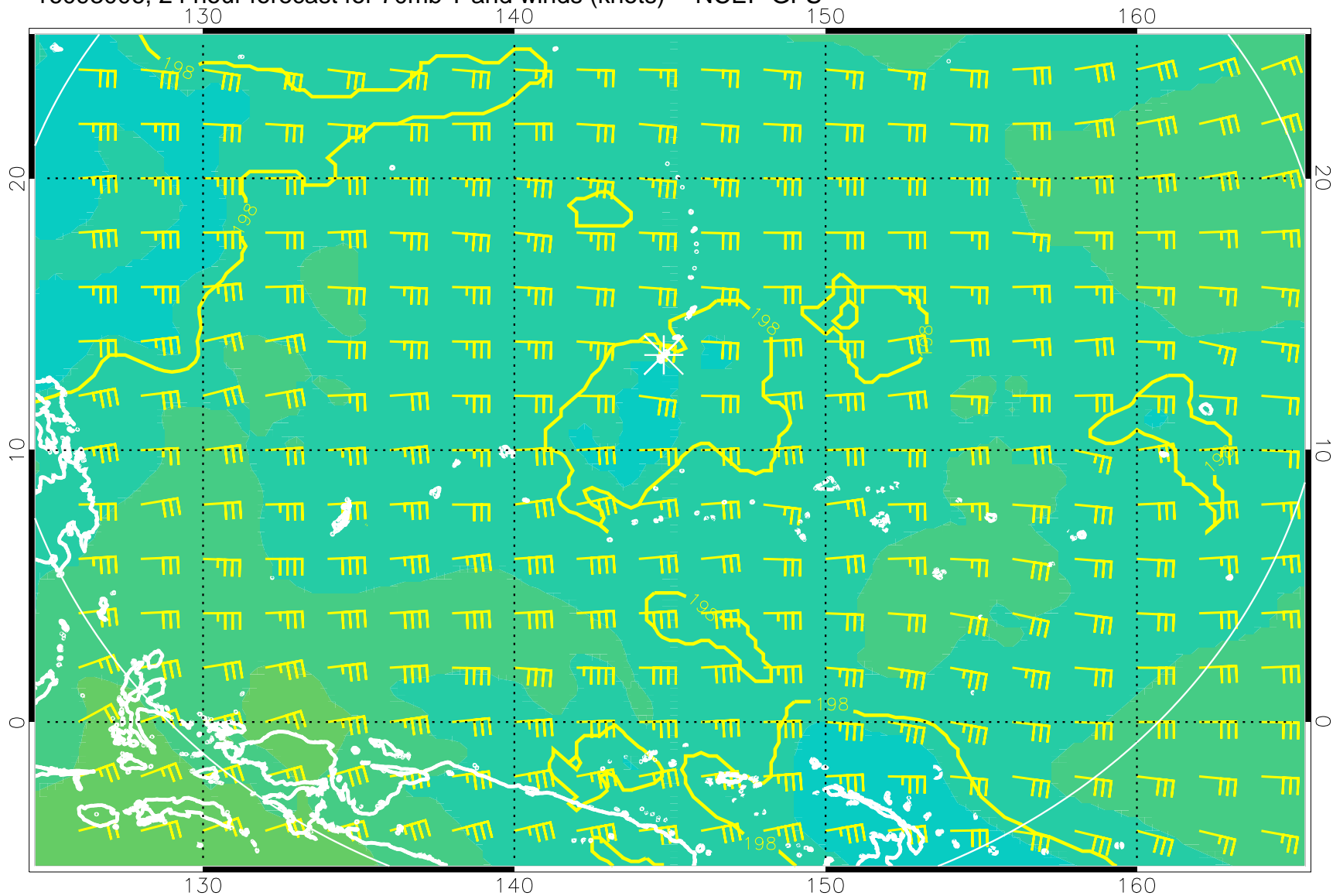
16093006, 24 hour forecast for 70mb T and winds (knots) -- NCEP GFS
