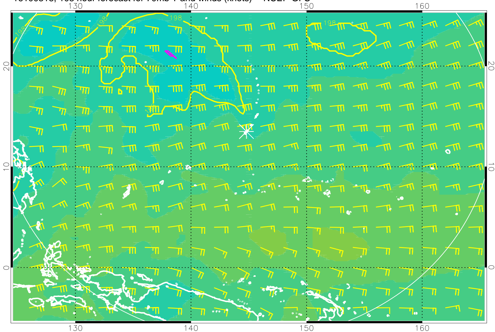
16100318, 108 hour forecast for 70mb T and winds (knots) -- NCEP GFS
