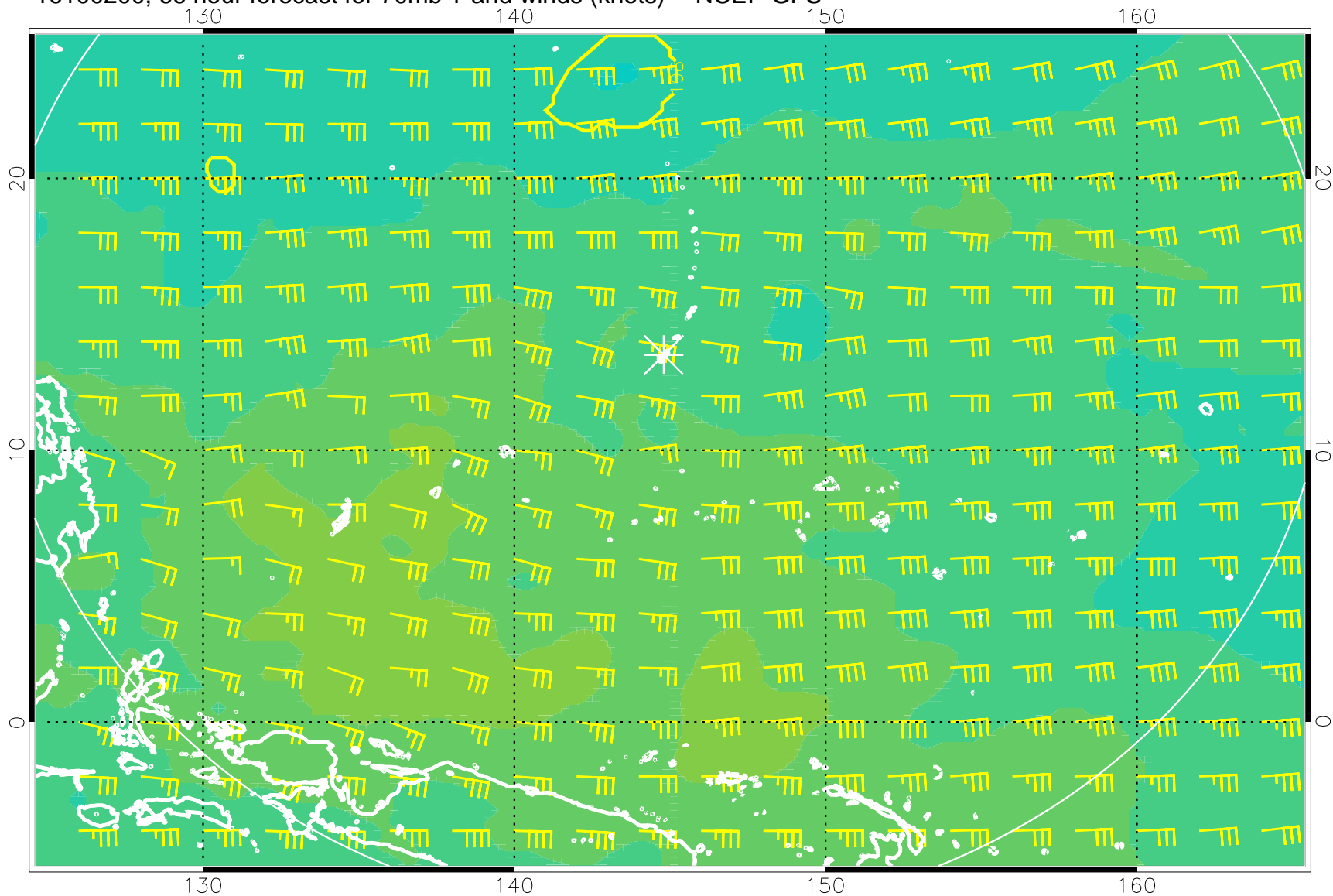
16100200, 66 hour forecast for 70mb T and winds (knots) -- NCEP GFS
