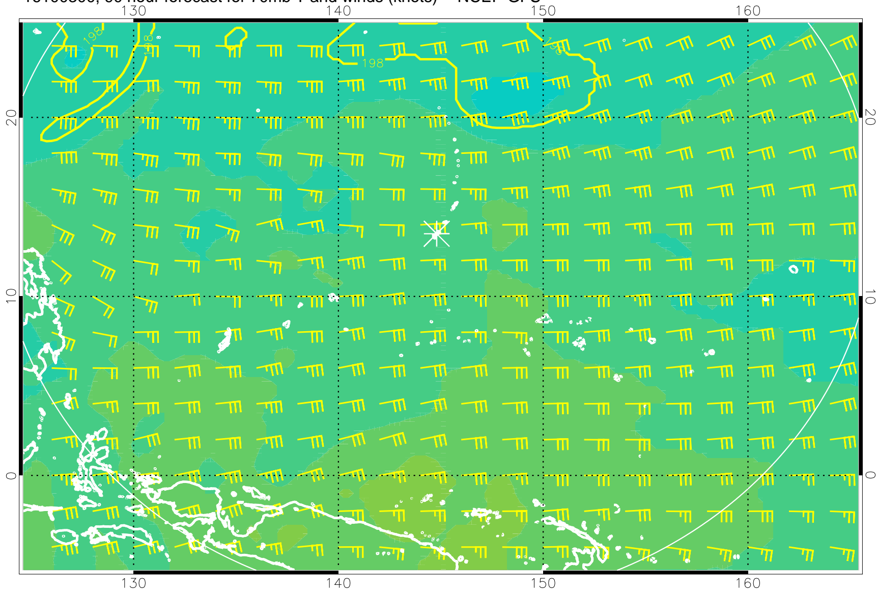
16100300, 90 hour forecast for 70mb T and winds (knots) -- NCEP GFS
