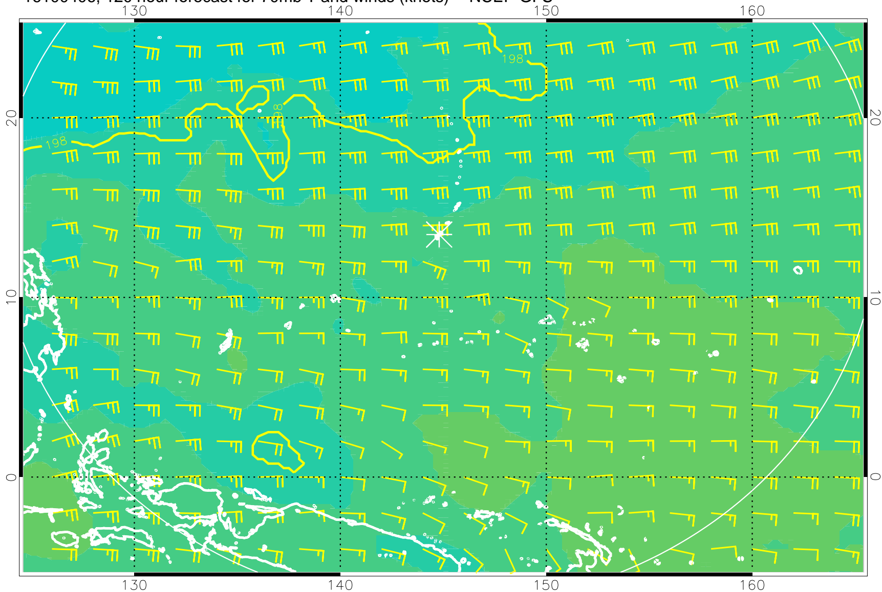
16100406, 120 hour forecast for 70mb T and winds (knots) -- NCEP GFS
