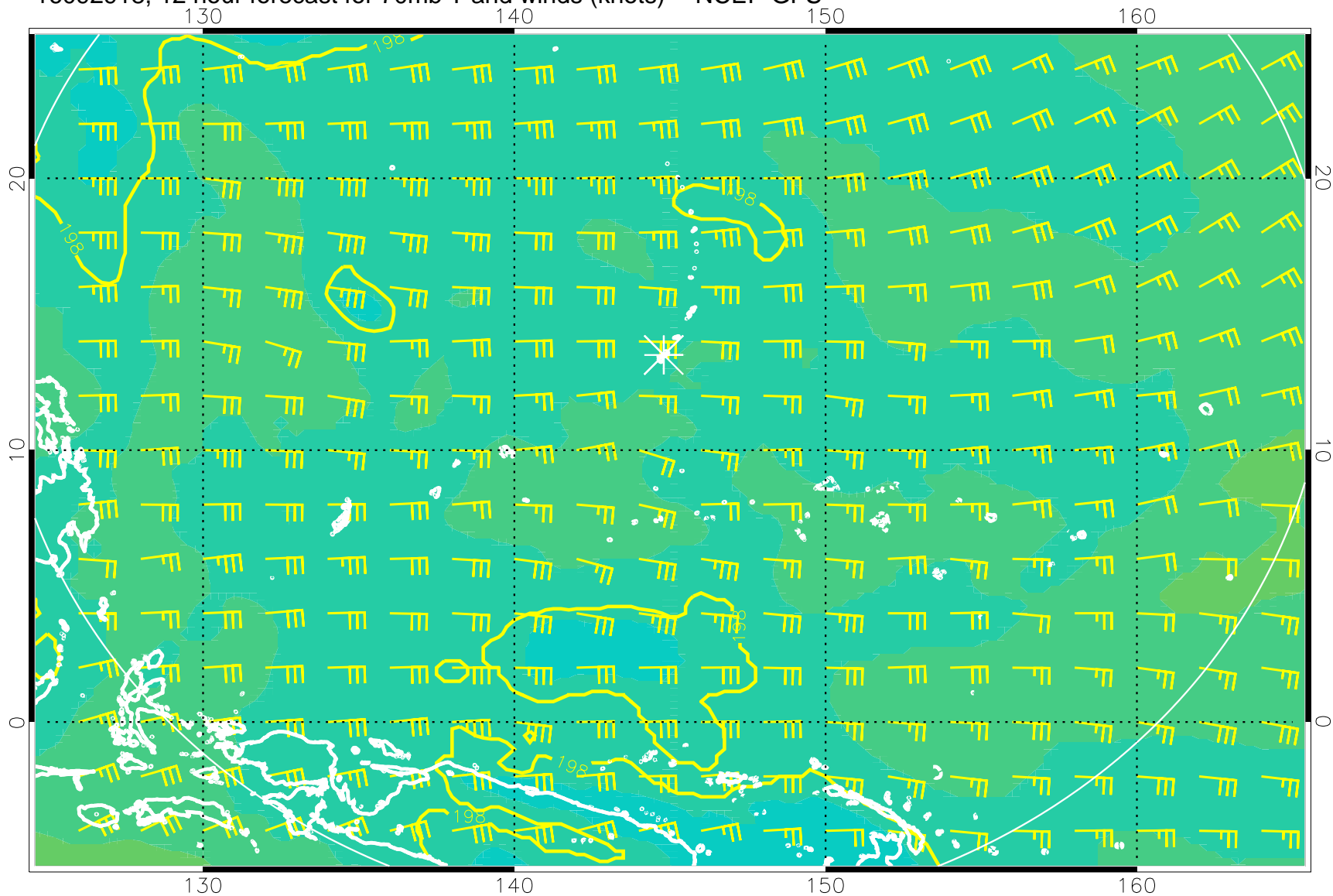
16092918, 12 hour forecast for 70mb T and winds (knots) -- NCEP GFS
