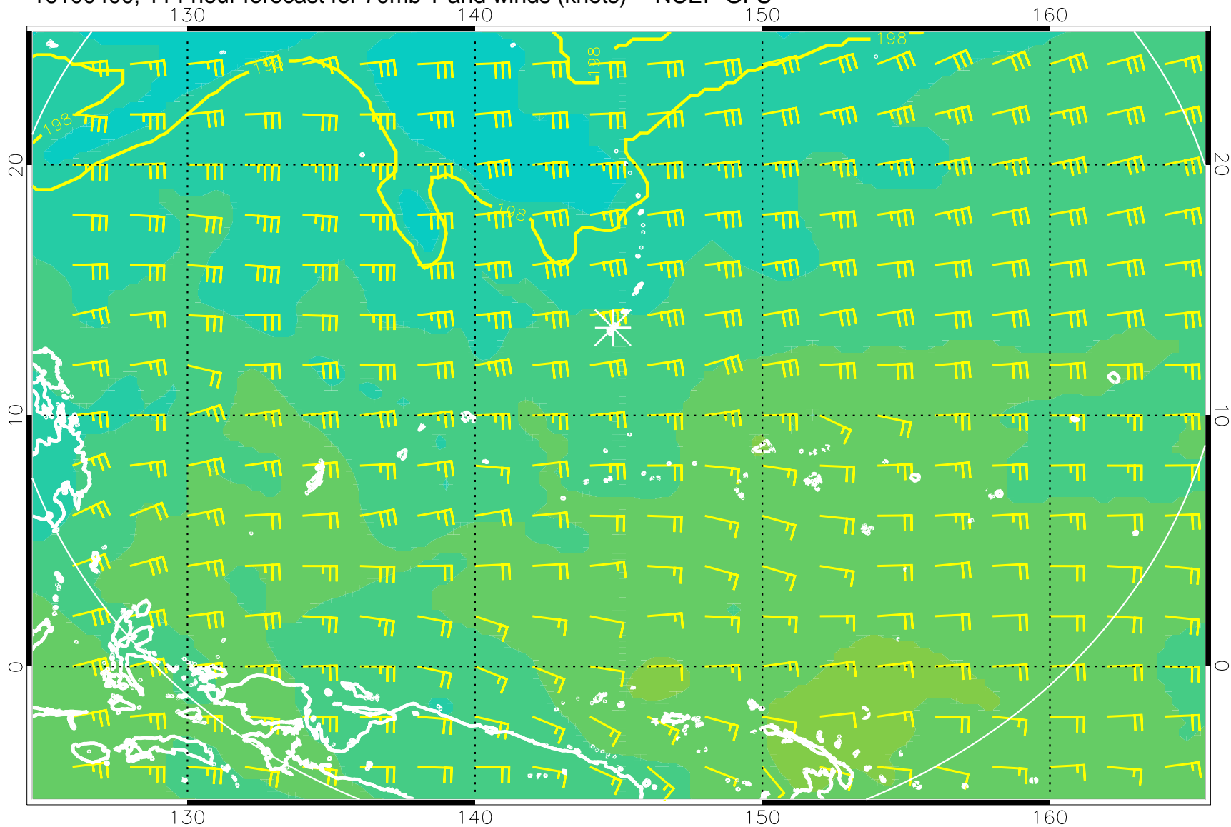
16100400, 114 hour forecast for 70mb T and winds (knots) -- NCEP GFS
