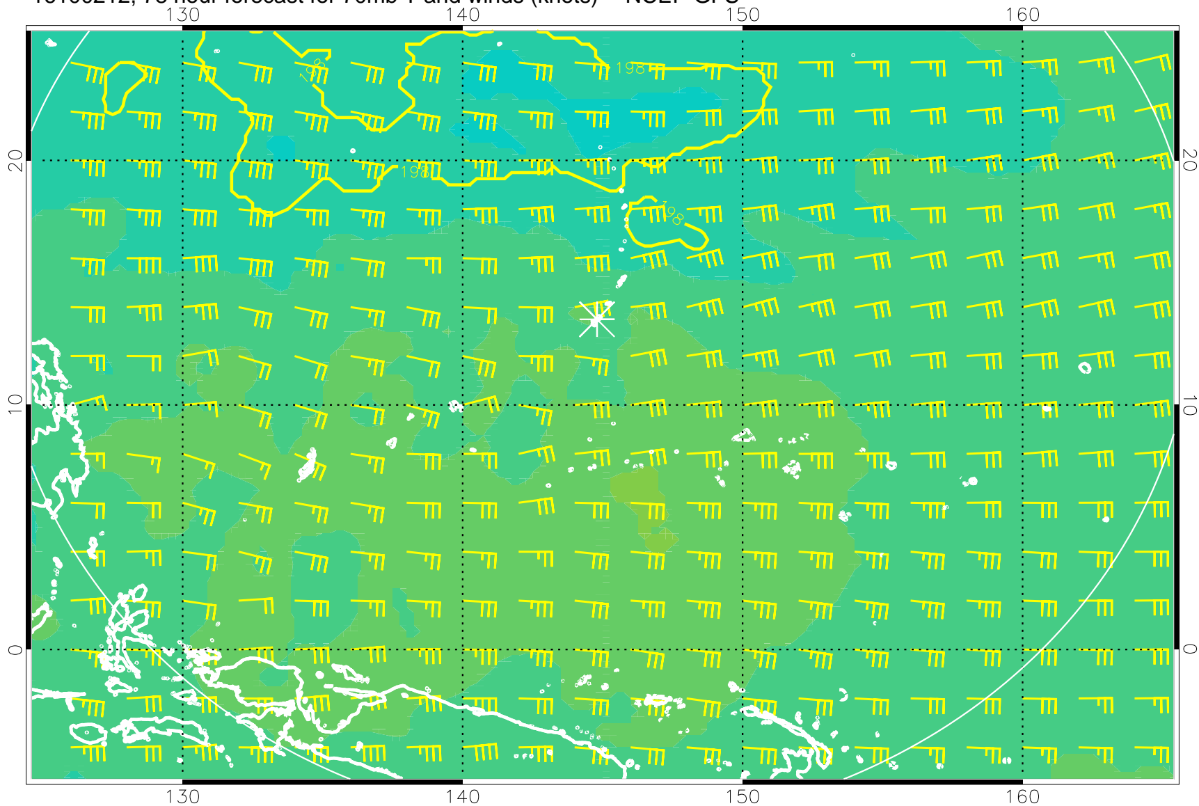
16100212, 78 hour forecast for 70mb T and winds (knots) -- NCEP GFS
