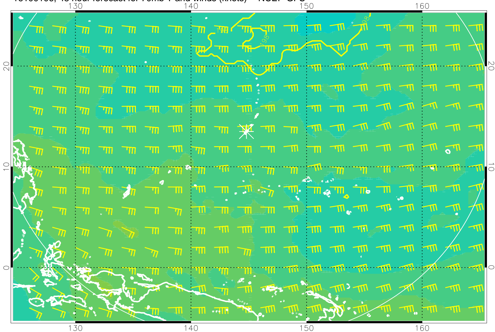
16100106, 48 hour forecast for 70mb T and winds (knots) -- NCEP GFS
