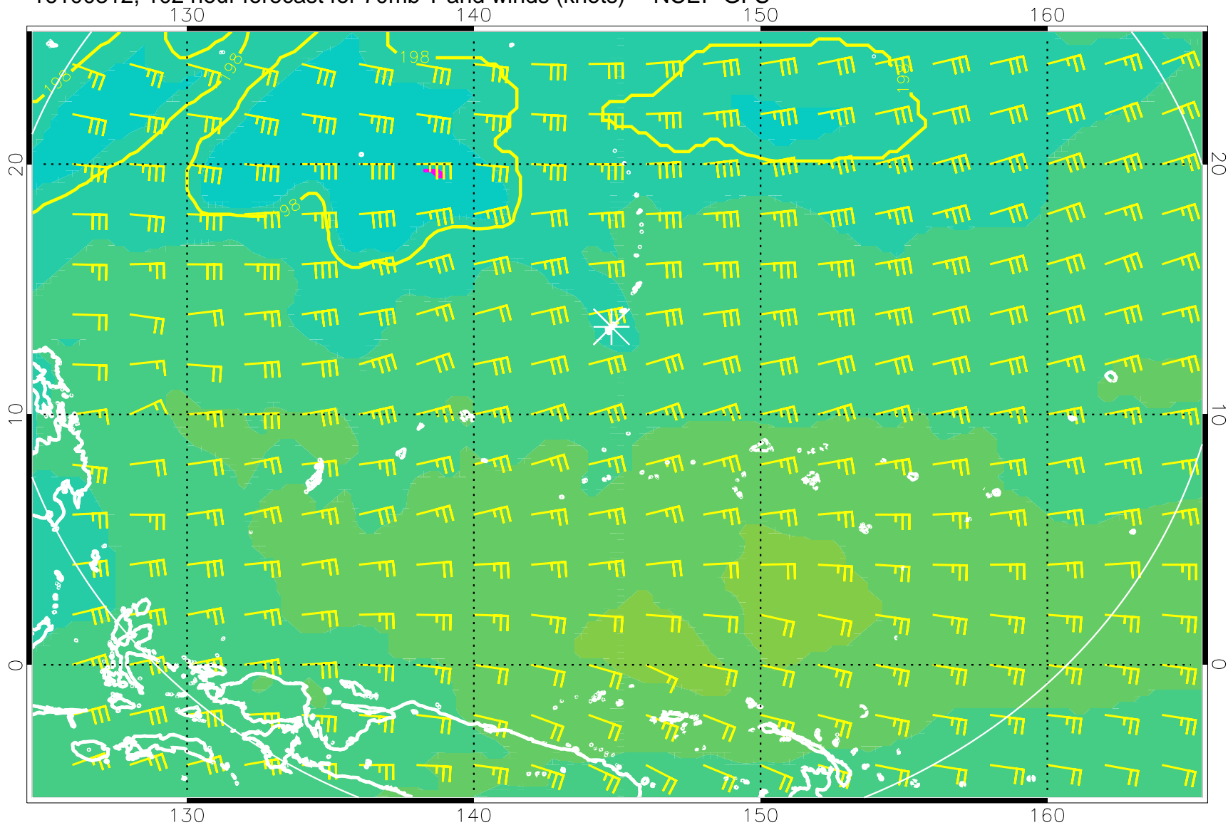
16100312, 102 hour forecast for 70mb T and winds (knots) -- NCEP GFS
