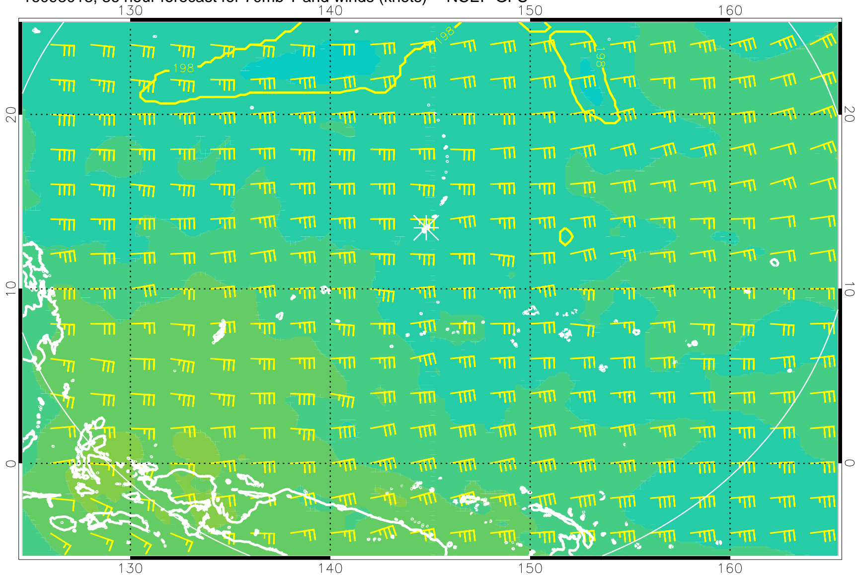
16093018, 36 hour forecast for 70mb T and winds (knots) -- NCEP GFS
