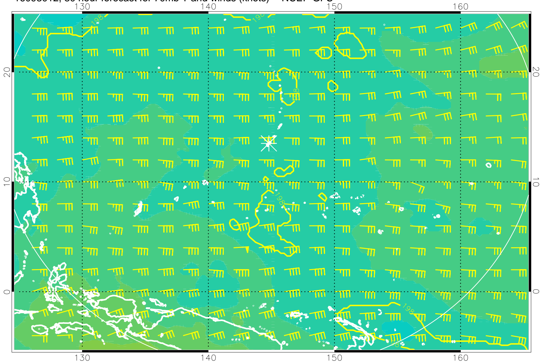
16093012, 30 hour forecast for 70mb T and winds (knots) -- NCEP GFS
