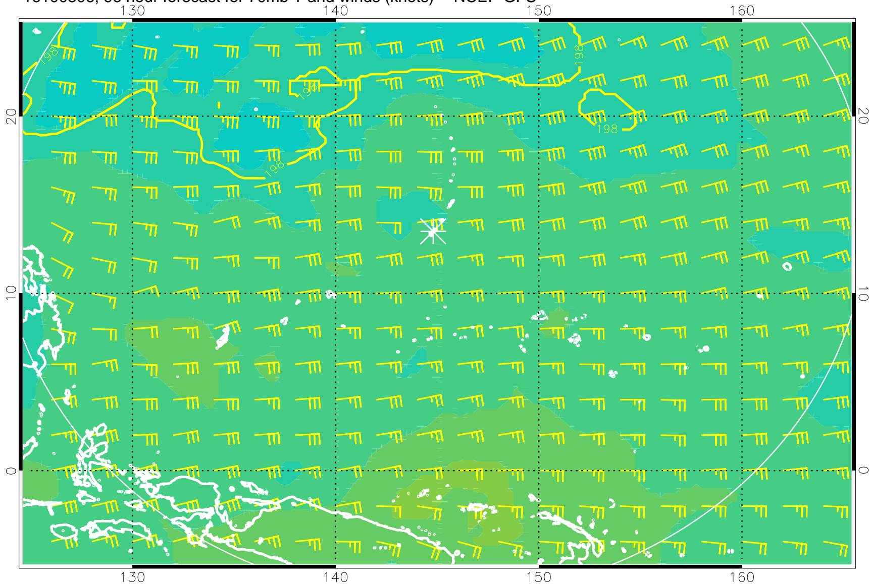
16100306, 96 hour forecast for 70mb T and winds (knots) -- NCEP GFS
