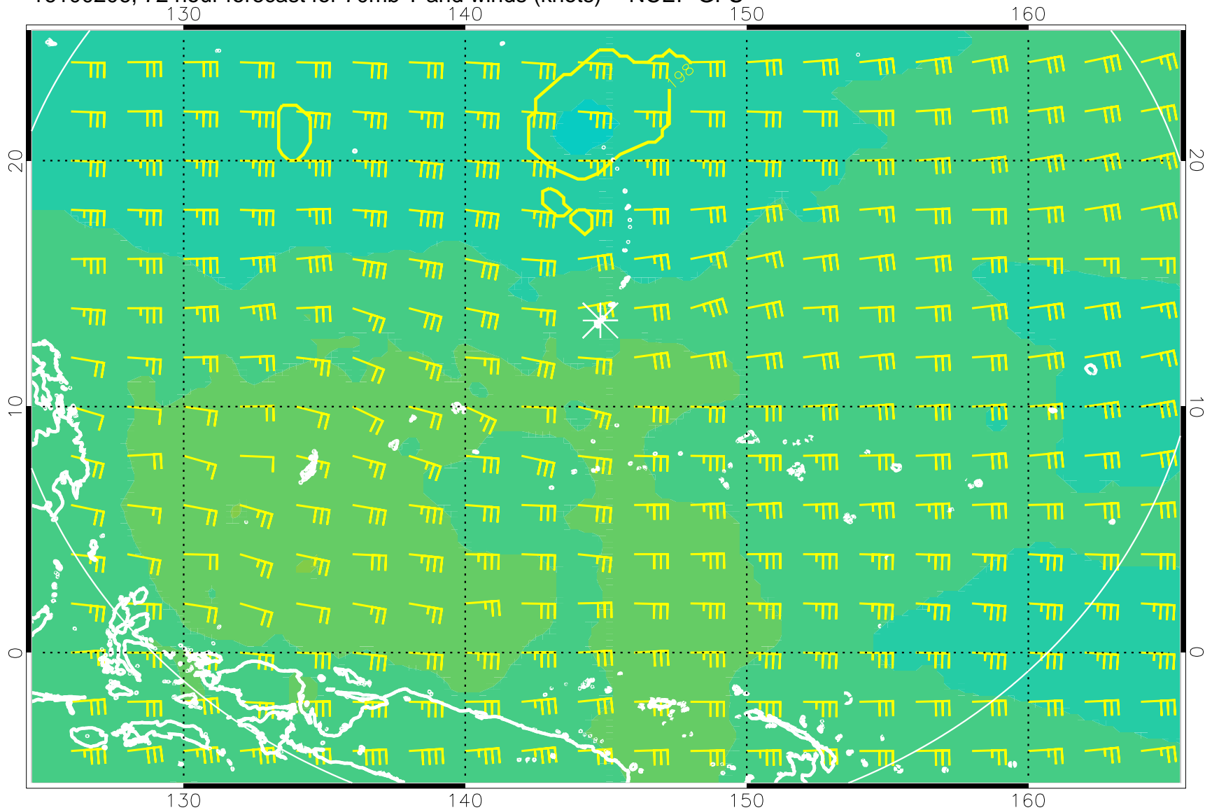
16100206, 72 hour forecast for 70mb T and winds (knots) -- NCEP GFS
