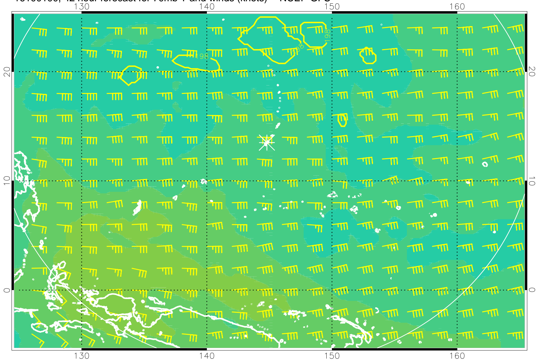
16100100, 42 hour forecast for 70mb T and winds (knots) -- NCEP GFS
