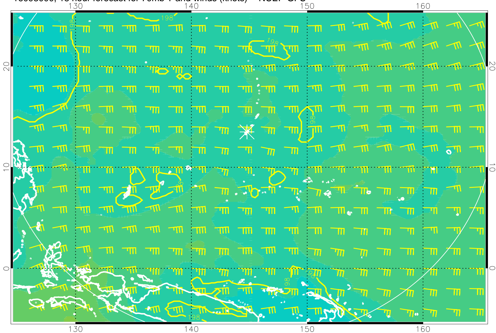
16093000, 18 hour forecast for 70mb T and winds (knots) -- NCEP GFS
