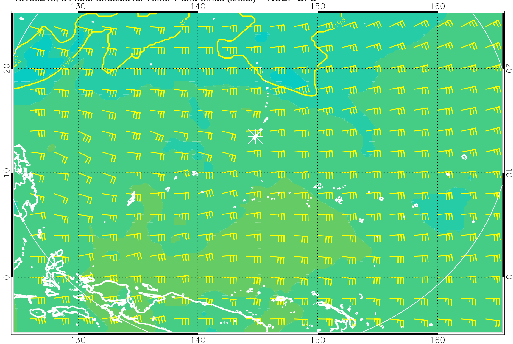
16100218, 84 hour forecast for 70mb T and winds (knots) -- NCEP GFS
