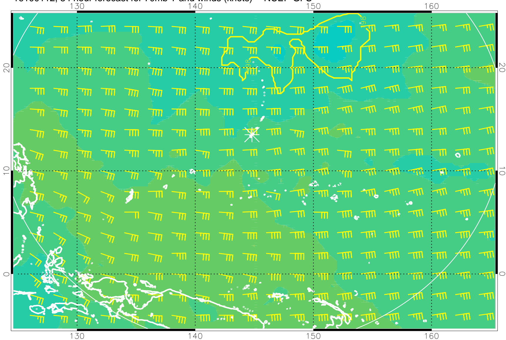
16100112, 54 hour forecast for 70mb T and winds (knots) -- NCEP GFS
