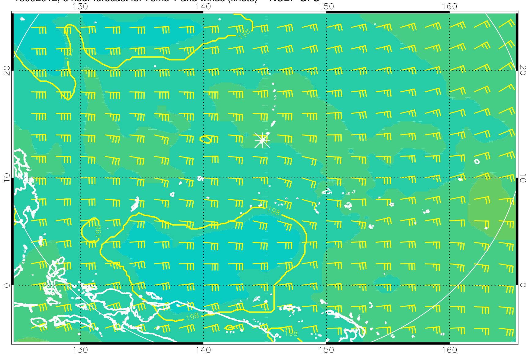
16092912, 6 hour forecast for 70mb T and winds (knots) -- NCEP GFS
