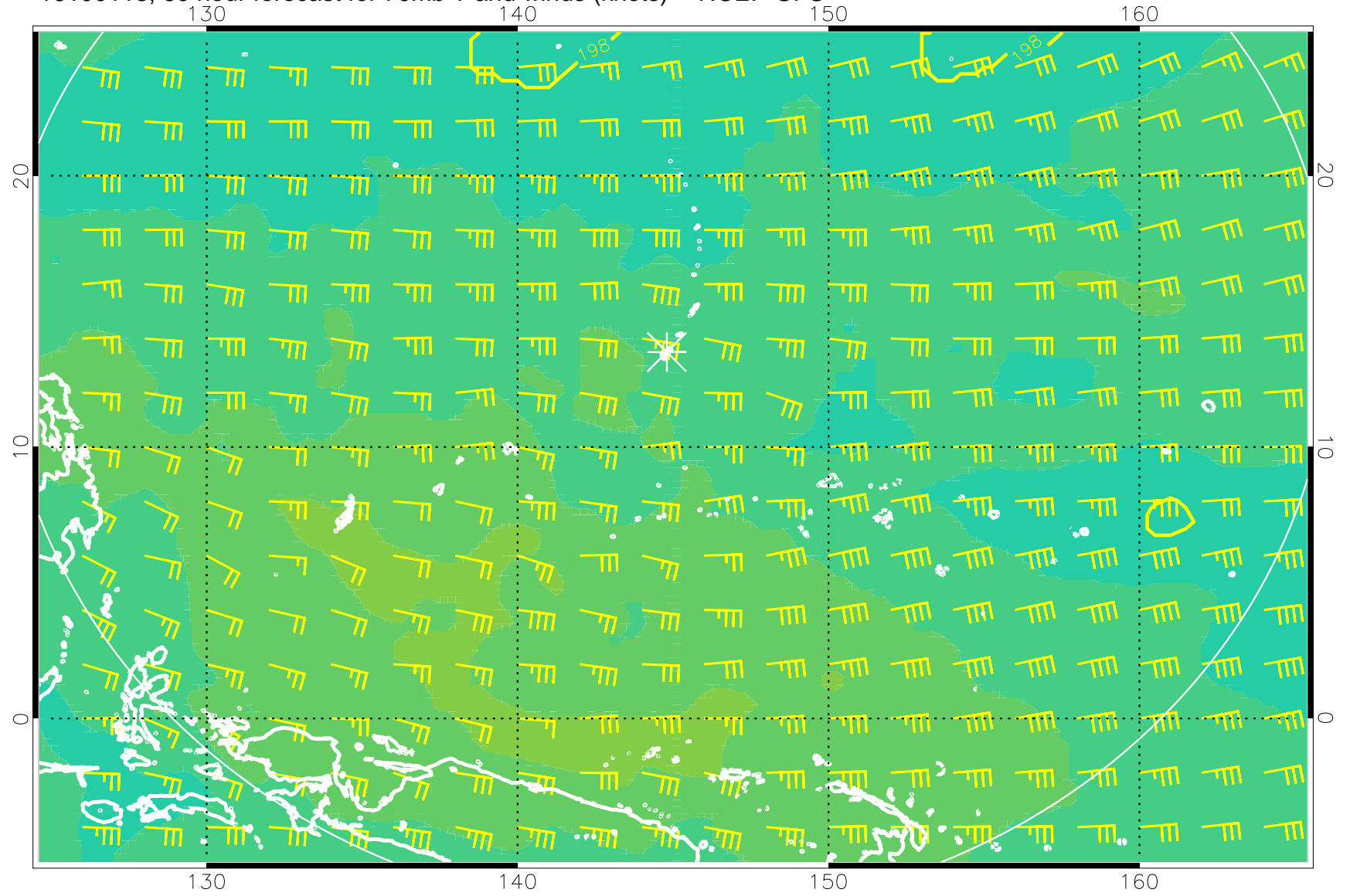
16100118, 60 hour forecast for 70mb T and winds (knots) -- NCEP GFS
