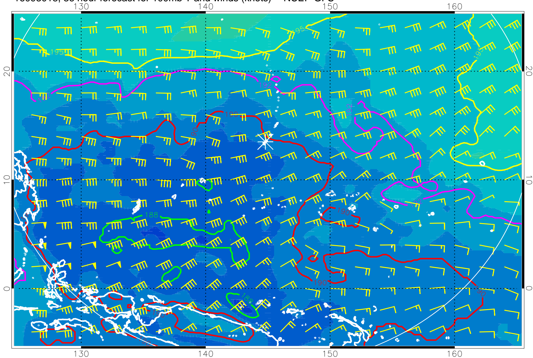
16093018, 36 hour forecast for 100mb T and winds (knots) -- NCEP GFS
