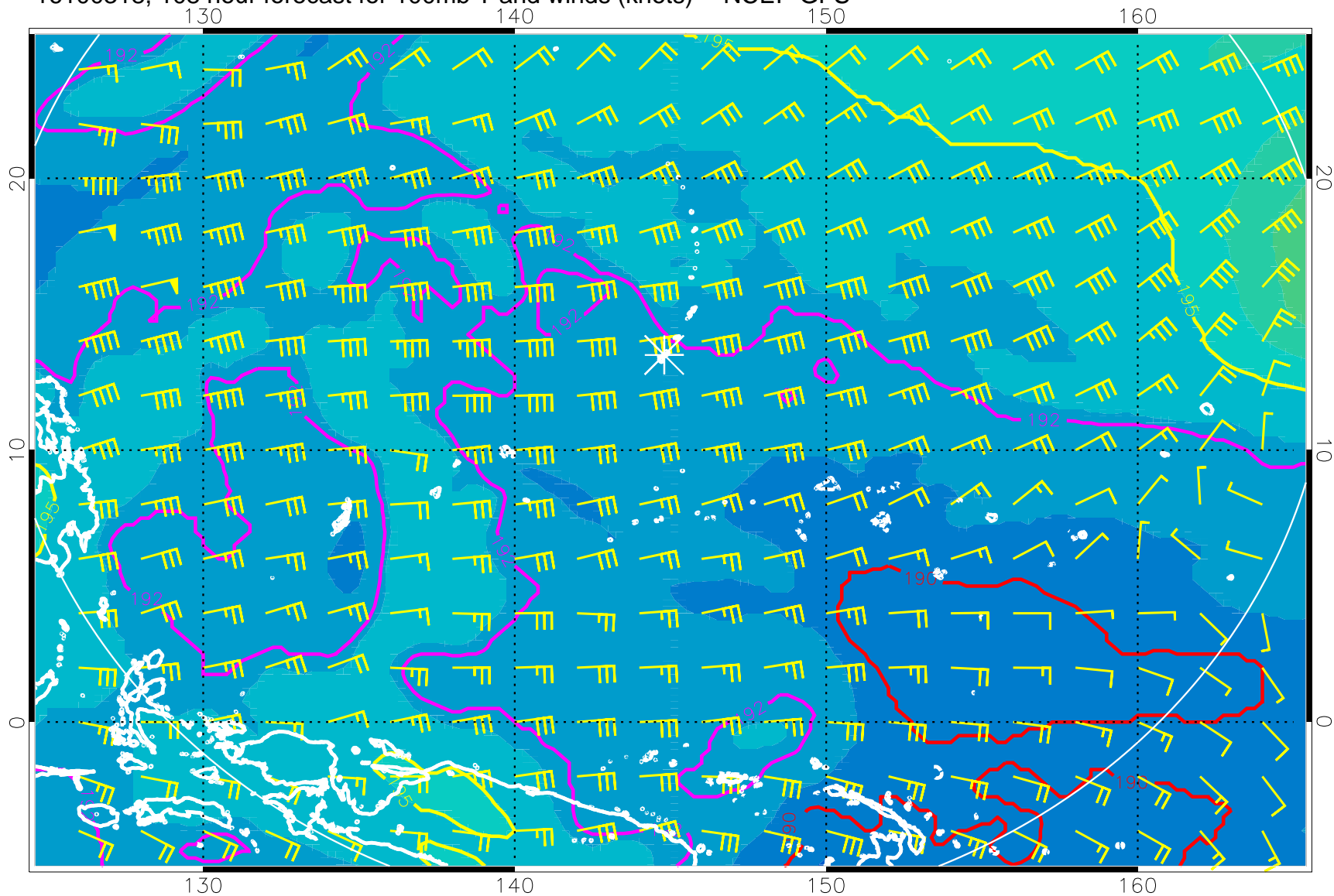
16100318, 108 hour forecast for 100mb T and winds (knots) -- NCEP GFS
