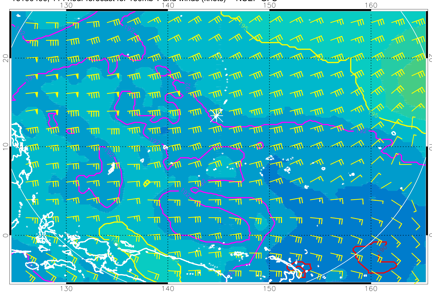
16100400, 114 hour forecast for 100mb T and winds (knots) -- NCEP GFS
