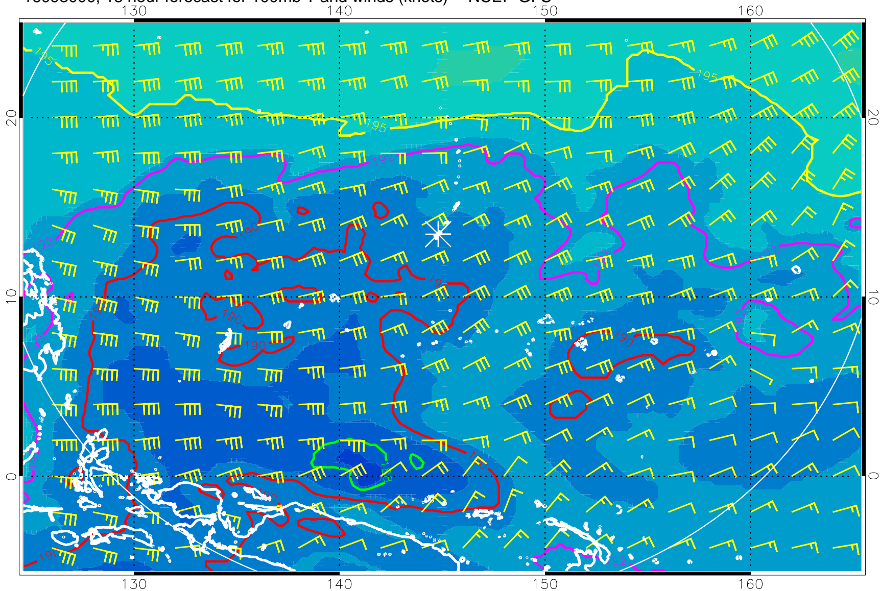
16093000, 18 hour forecast for 100mb T and winds (knots) -- NCEP GFS
