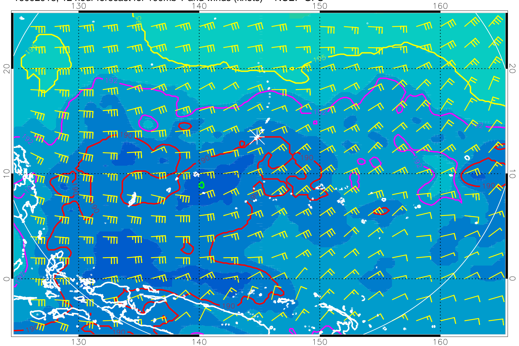
16092918, 12 hour forecast for 100mb T and winds (knots) -- NCEP GFS
