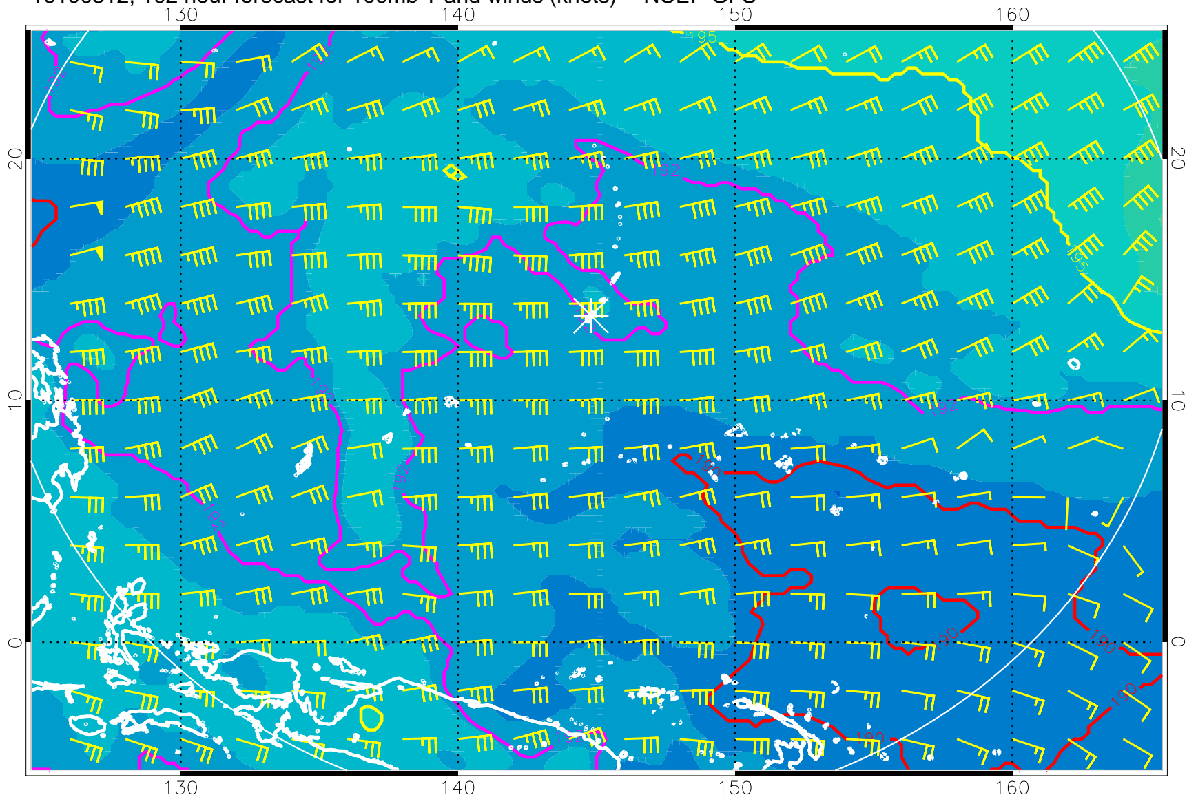
16100312, 102 hour forecast for 100mb T and winds (knots) -- NCEP GFS
