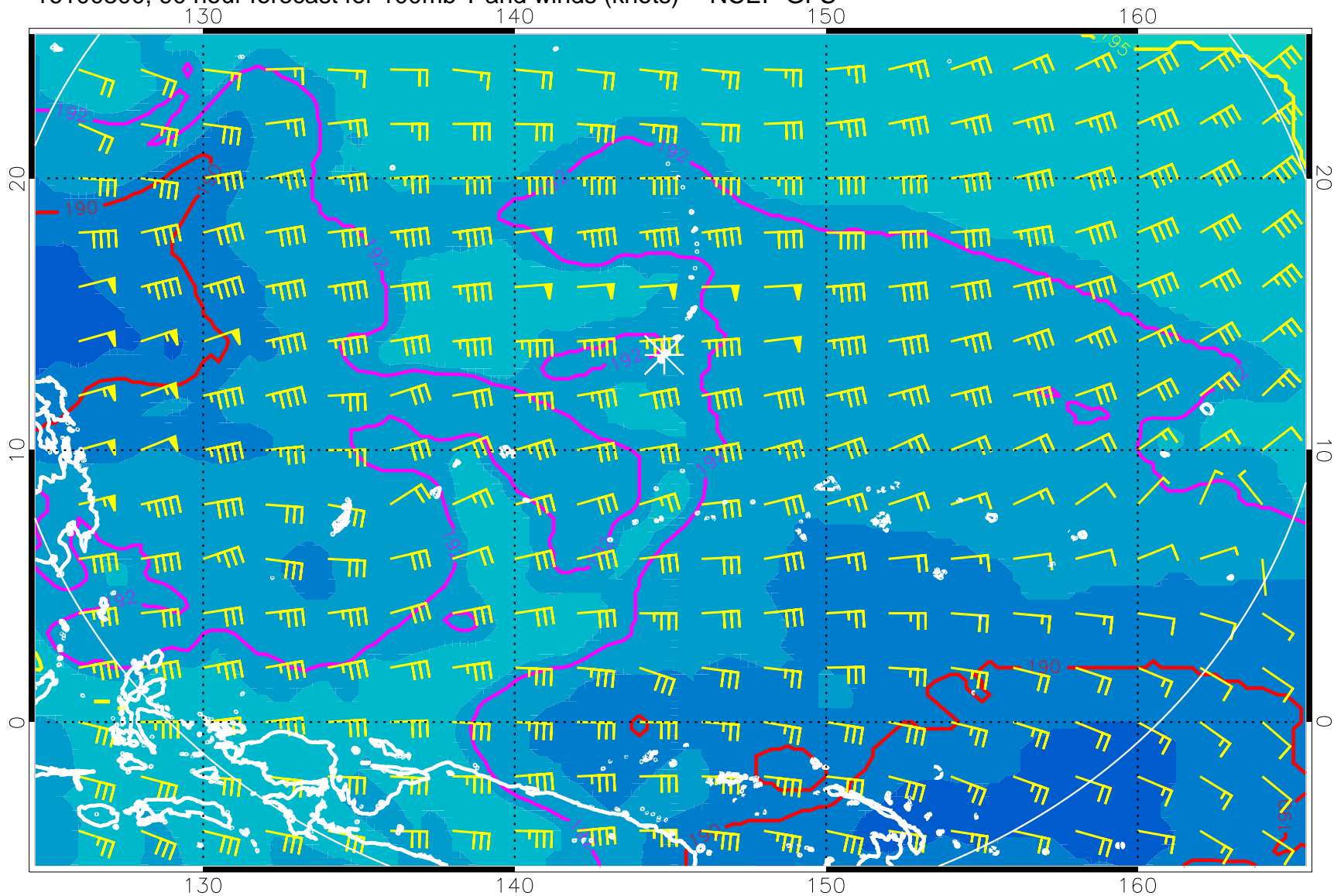
16100300, 90 hour forecast for 100mb T and winds (knots) -- NCEP GFS
