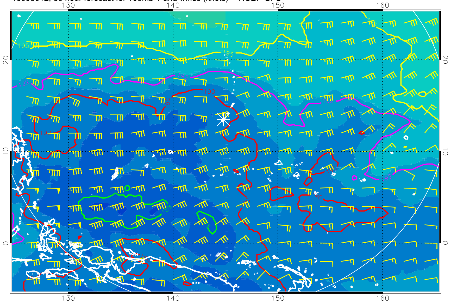
16093012, 30 hour forecast for 100mb T and winds (knots) -- NCEP GFS
