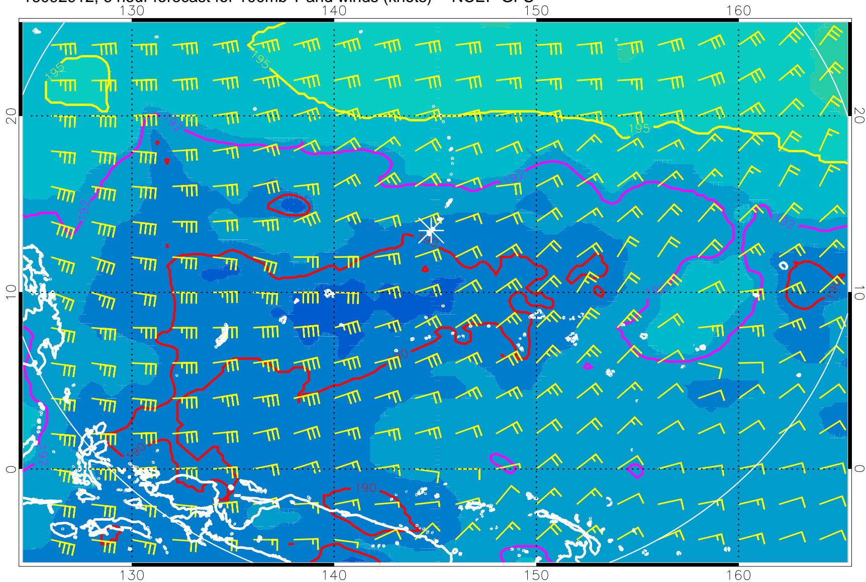
16092912, 6 hour forecast for 100mb T and winds (knots) -- NCEP GFS
