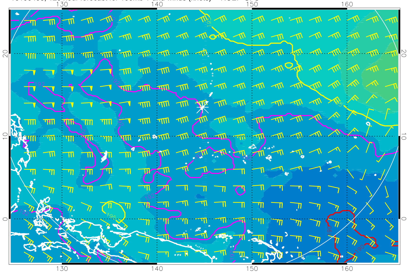
16100406, 120 hour forecast for 100mb T and winds (knots) -- NCEP GFS
