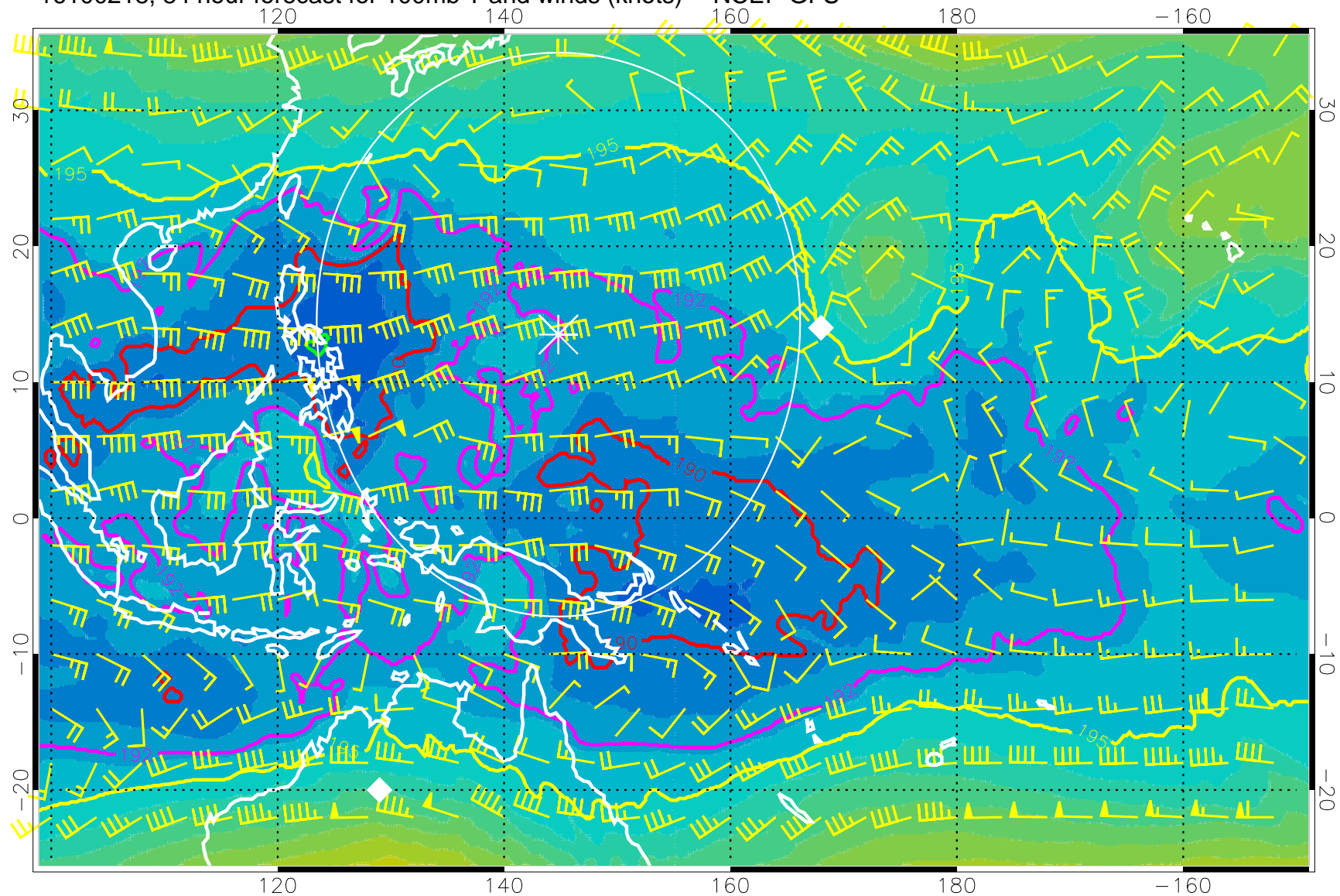
16100218, 84 hour forecast for 100mb T and winds (knots) -- NCEP GFS
