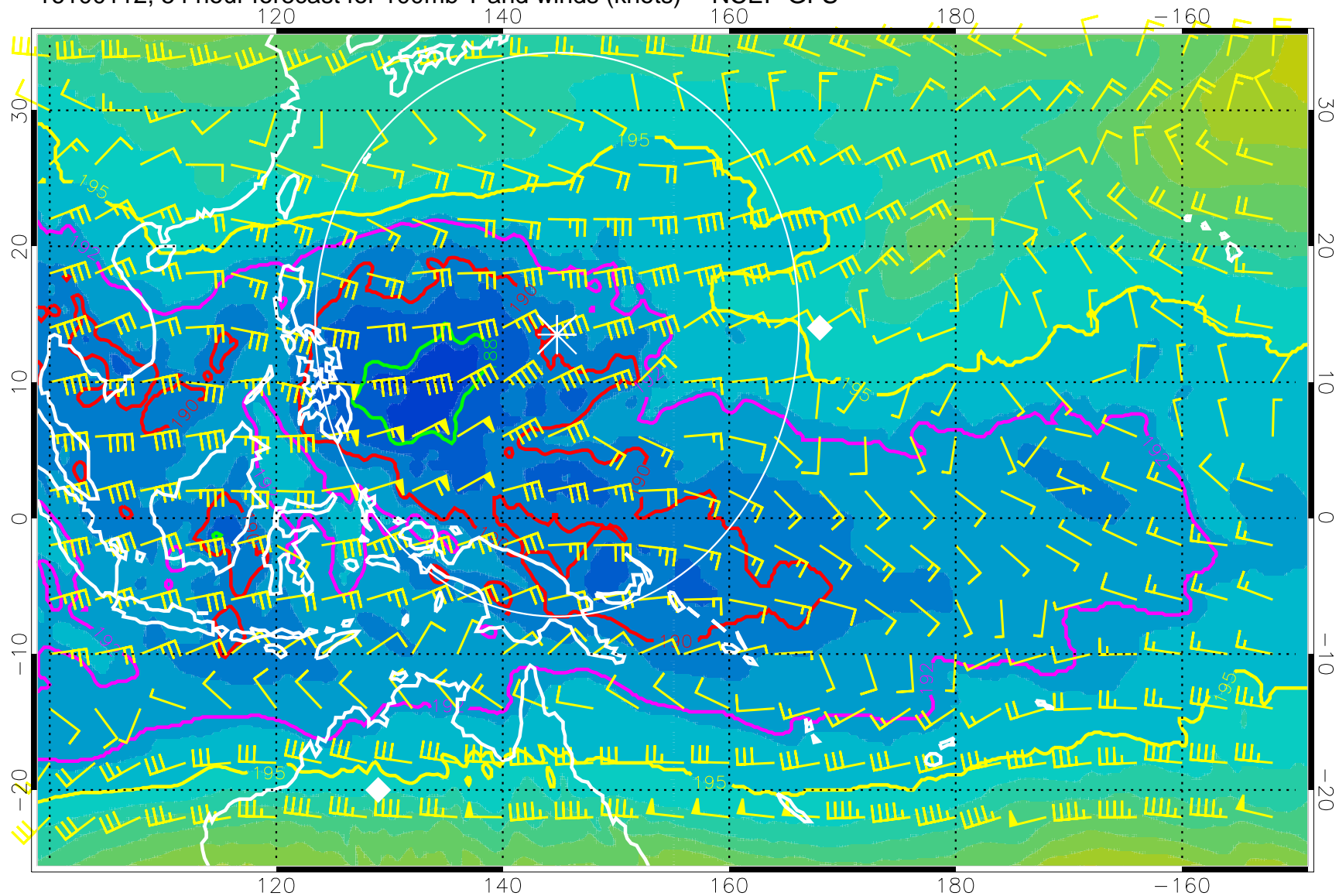
16100112, 54 hour forecast for 100mb T and winds (knots) -- NCEP GFS
