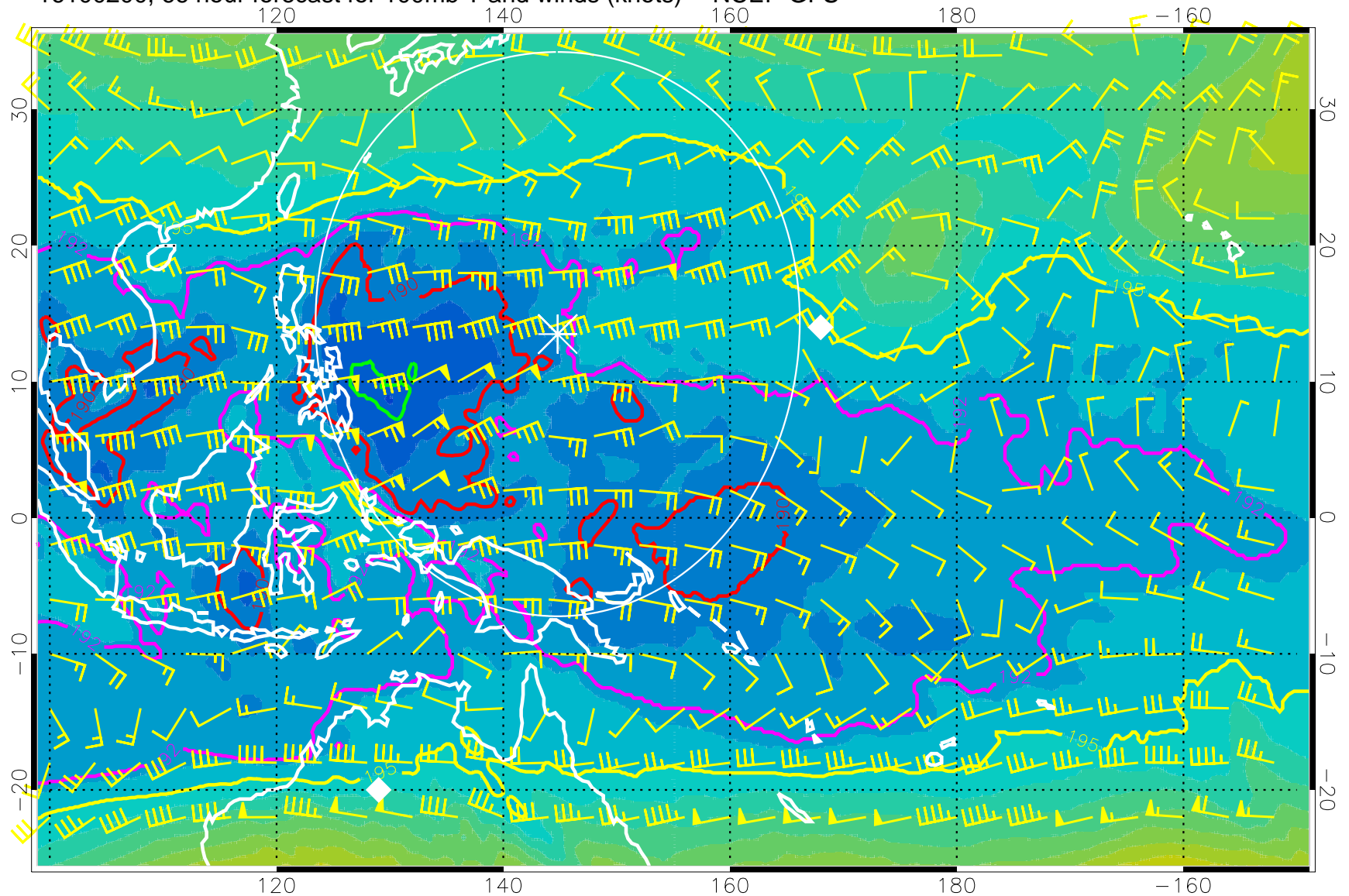
16100200, 66 hour forecast for 100mb T and winds (knots) -- NCEP GFS
