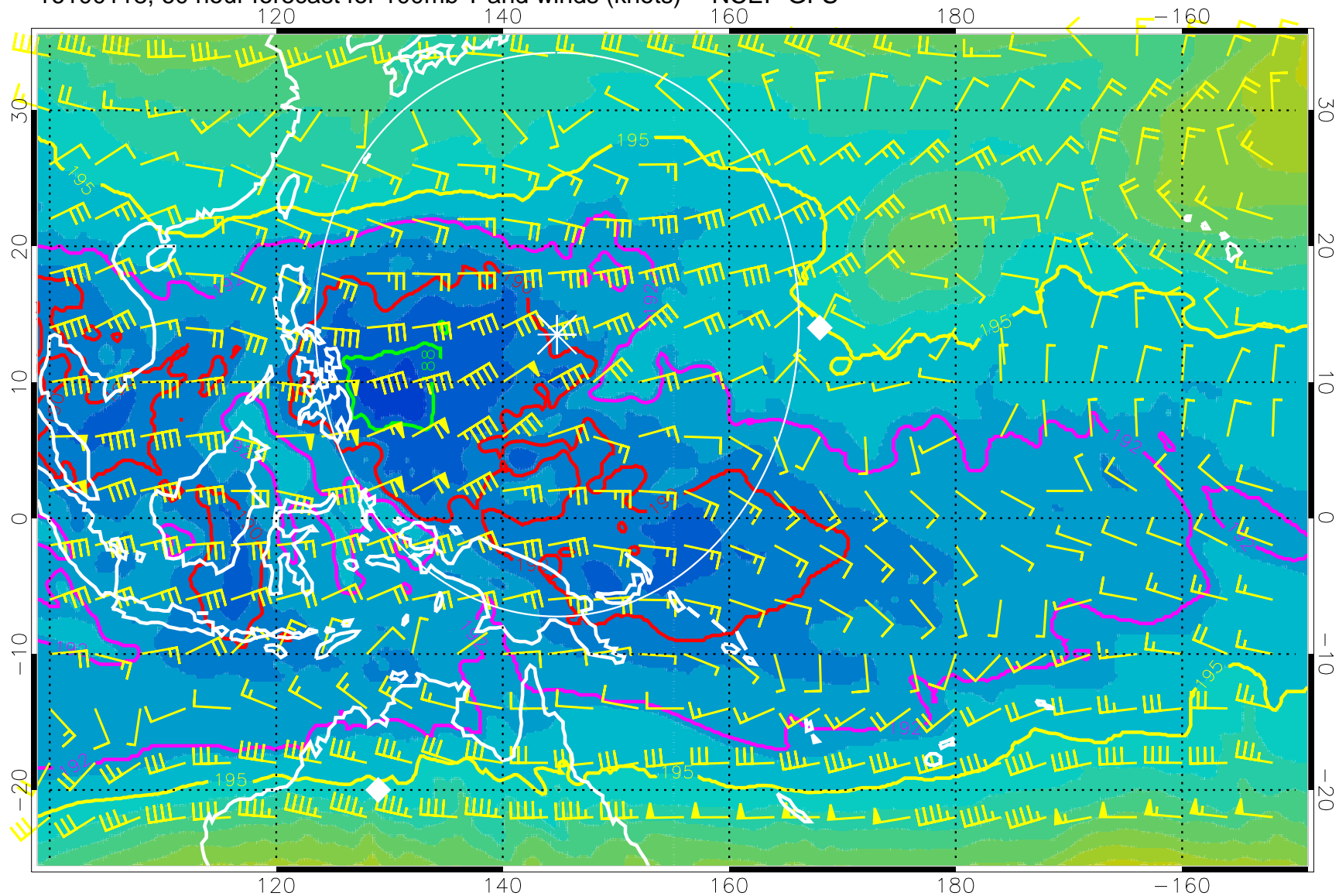
16100118, 60 hour forecast for 100mb T and winds (knots) -- NCEP GFS
