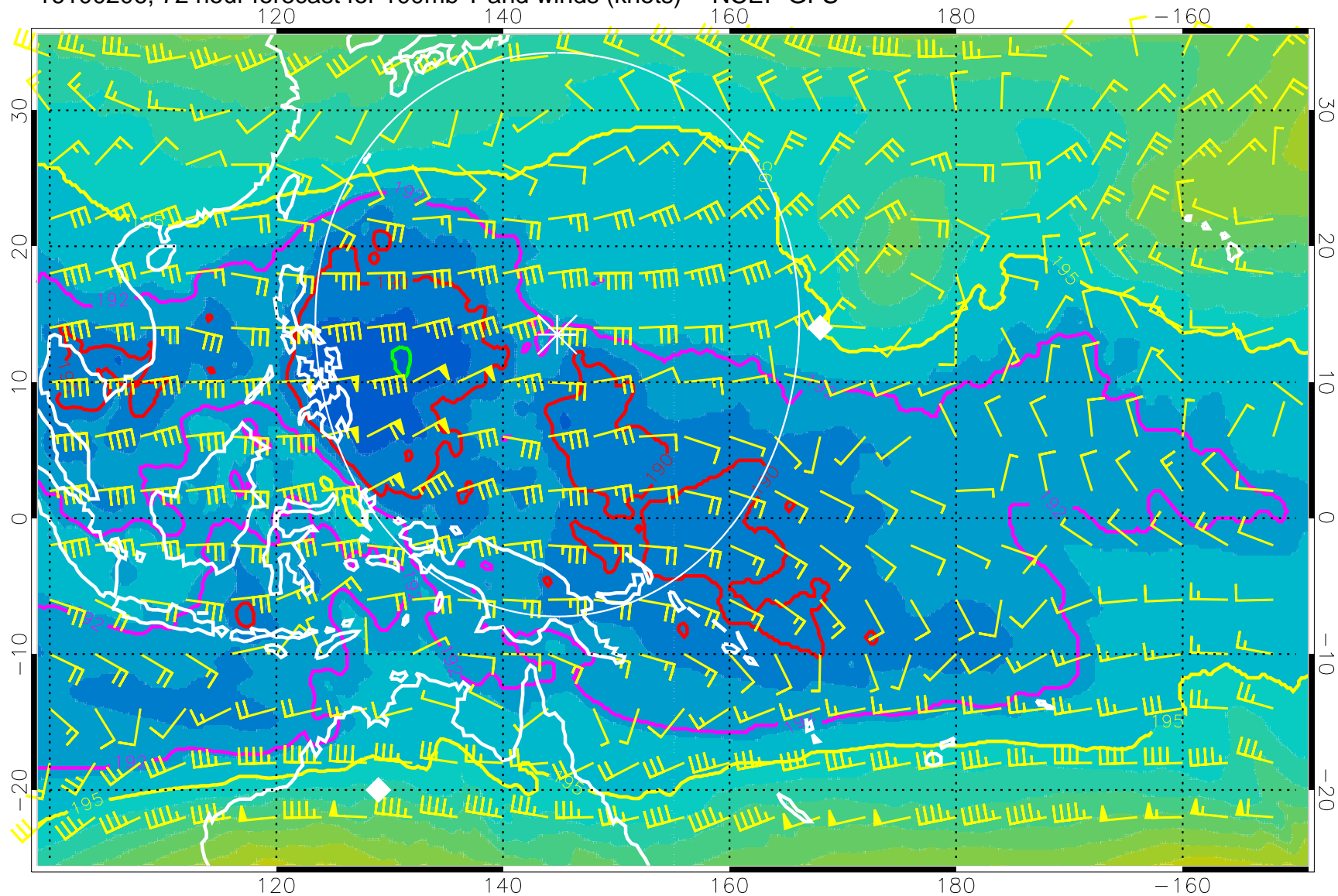
16100206, 72 hour forecast for 100mb T and winds (knots) -- NCEP GFS
