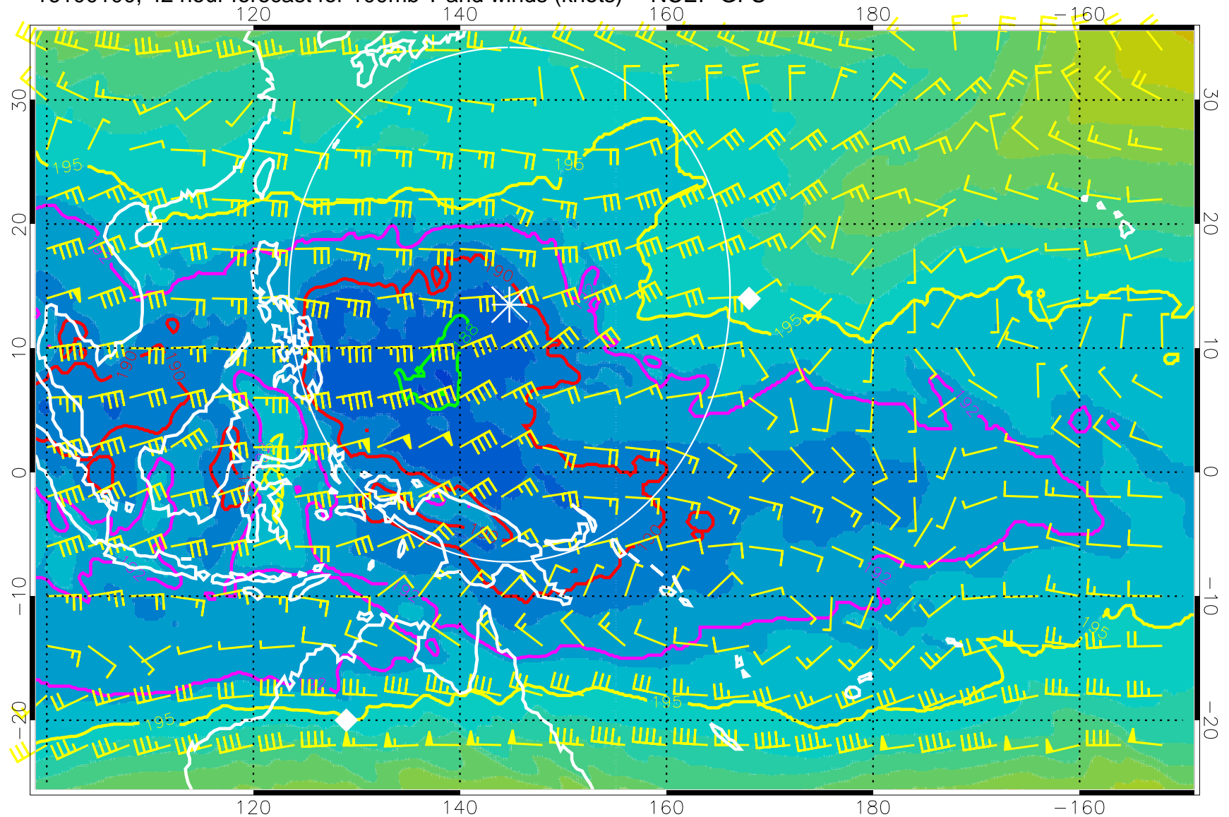
16100100, 42 hour forecast for 100mb T and winds (knots) -- NCEP GFS
