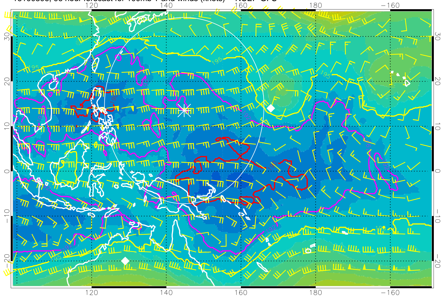
16100306, 96 hour forecast for 100mb T and winds (knots) -- NCEP GFS
