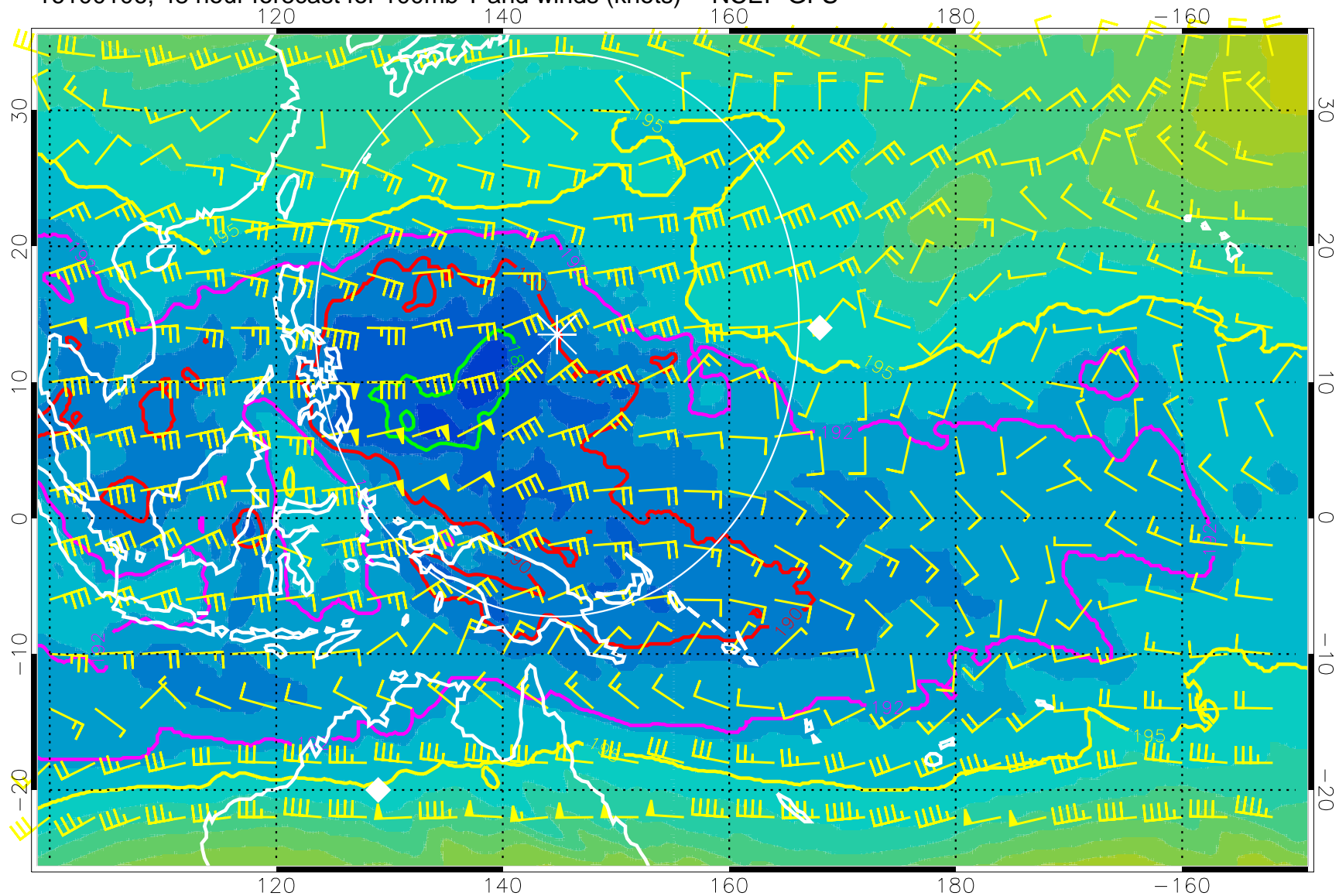
16100106, 48 hour forecast for 100mb T and winds (knots) -- NCEP GFS
