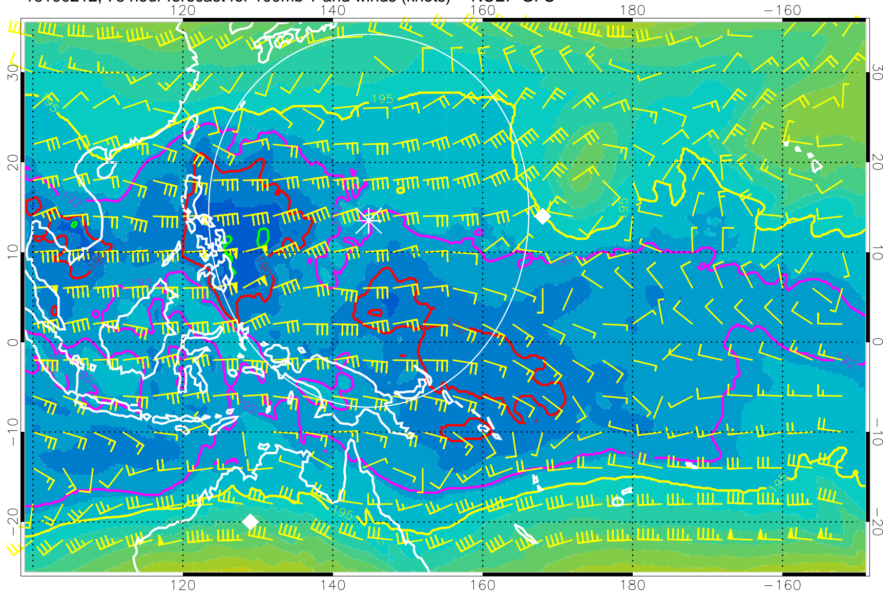
16100212, 78 hour forecast for 100mb T and winds (knots) -- NCEP GFS
