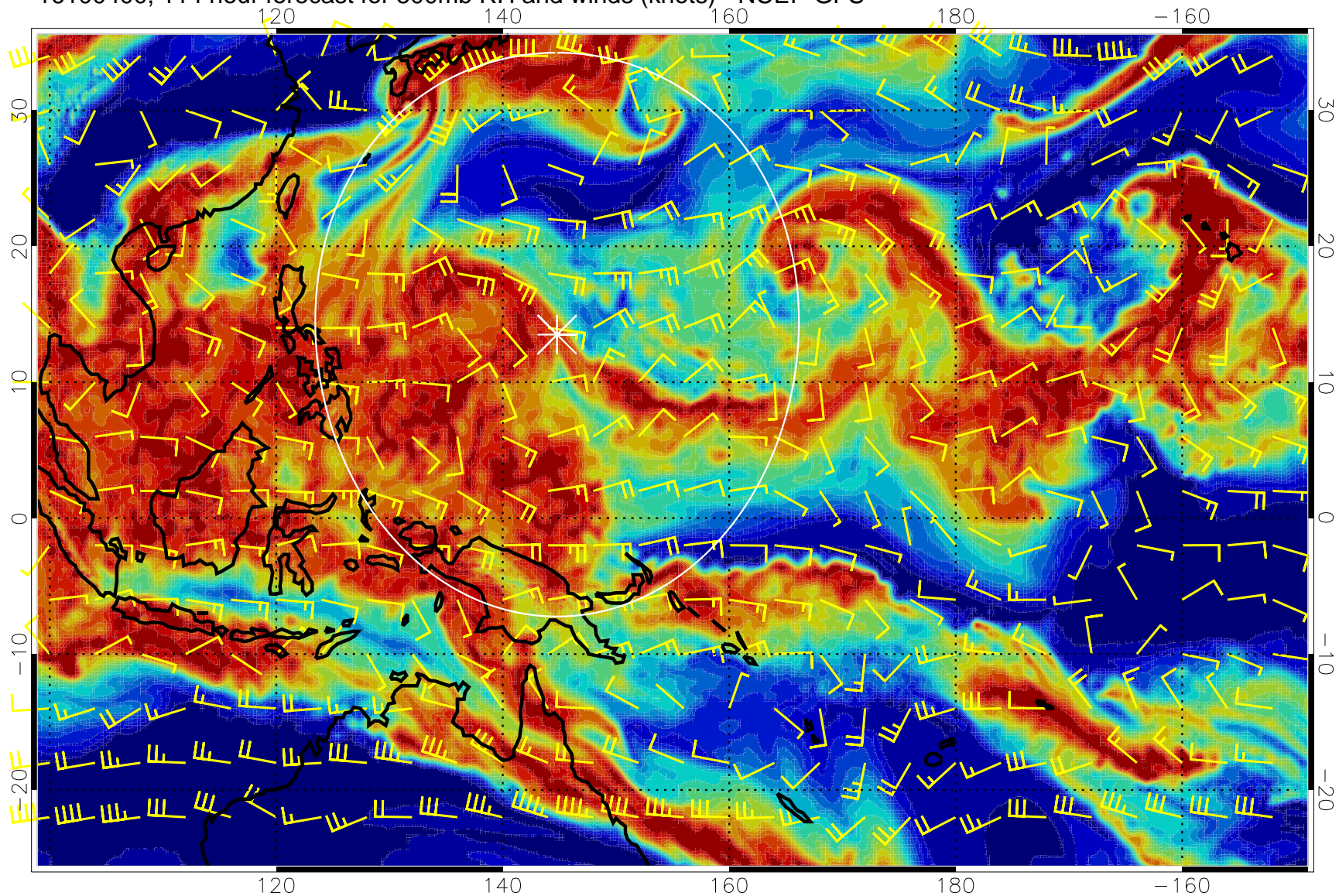
16100400, 114 hour forecast for 500mb RH and winds (knots) - NCEP GFS
