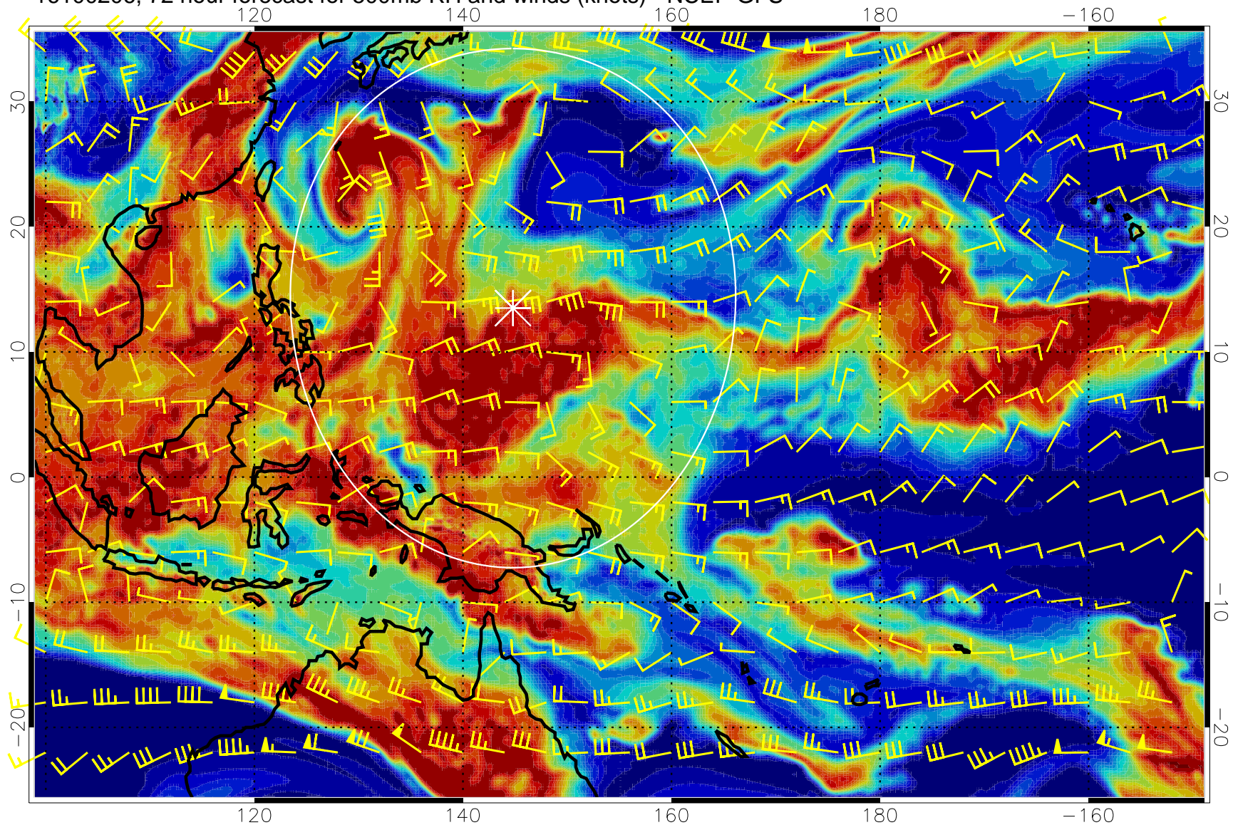
16100206, 72 hour forecast for 500mb RH and winds (knots) - NCEP GFS
