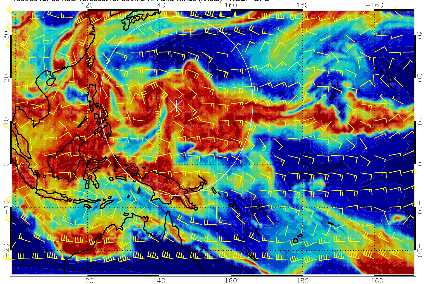
16093012, 30 hour forecast for 500mb RH and winds (knots) - NCEP GFS
