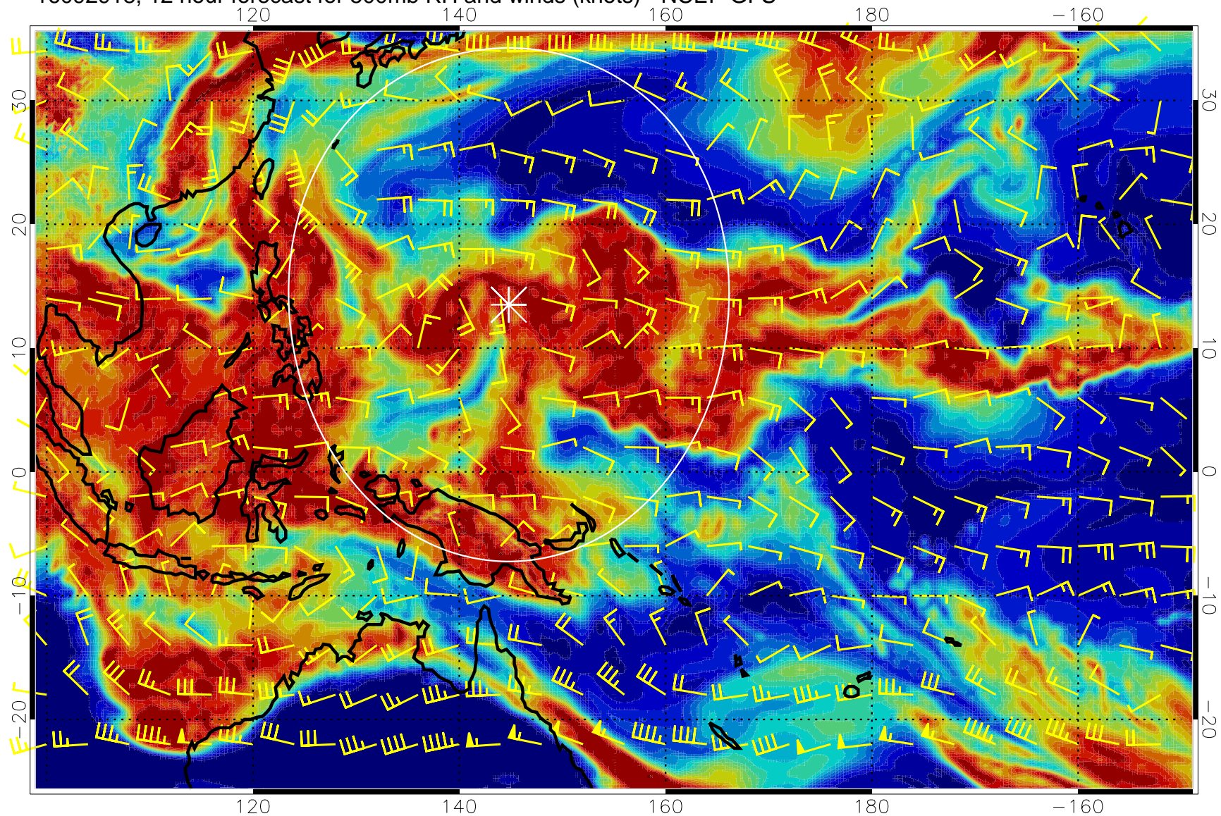
16092918, 12 hour forecast for 500mb RH and winds (knots) - NCEP GFS
