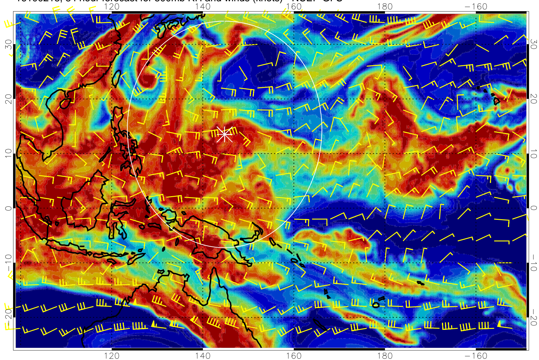
16100218, 84 hour forecast for 500mb RH and winds (knots) - NCEP GFS
