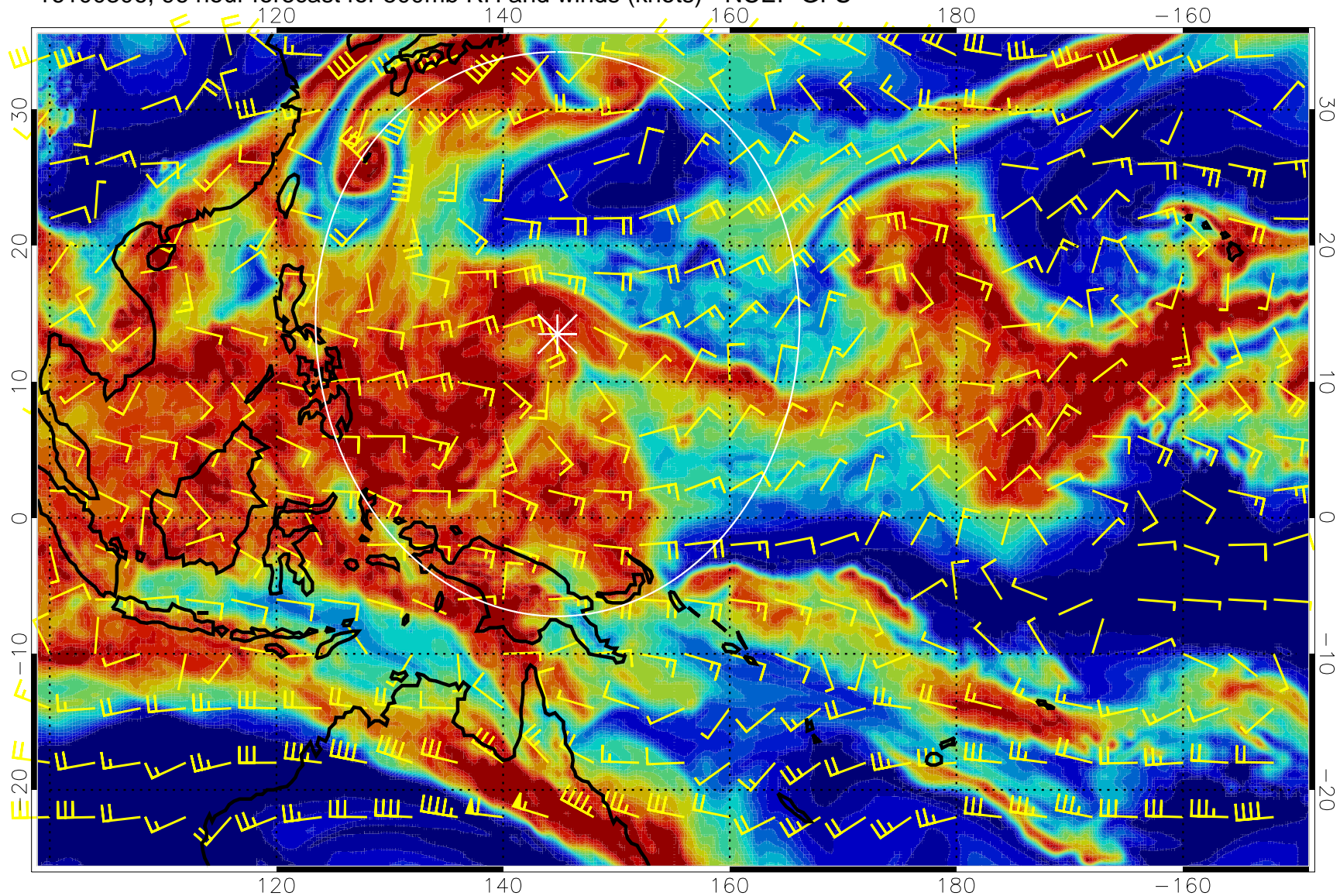
16100306, 96 hour forecast for 500mb RH and winds (knots) - NCEP GFS
