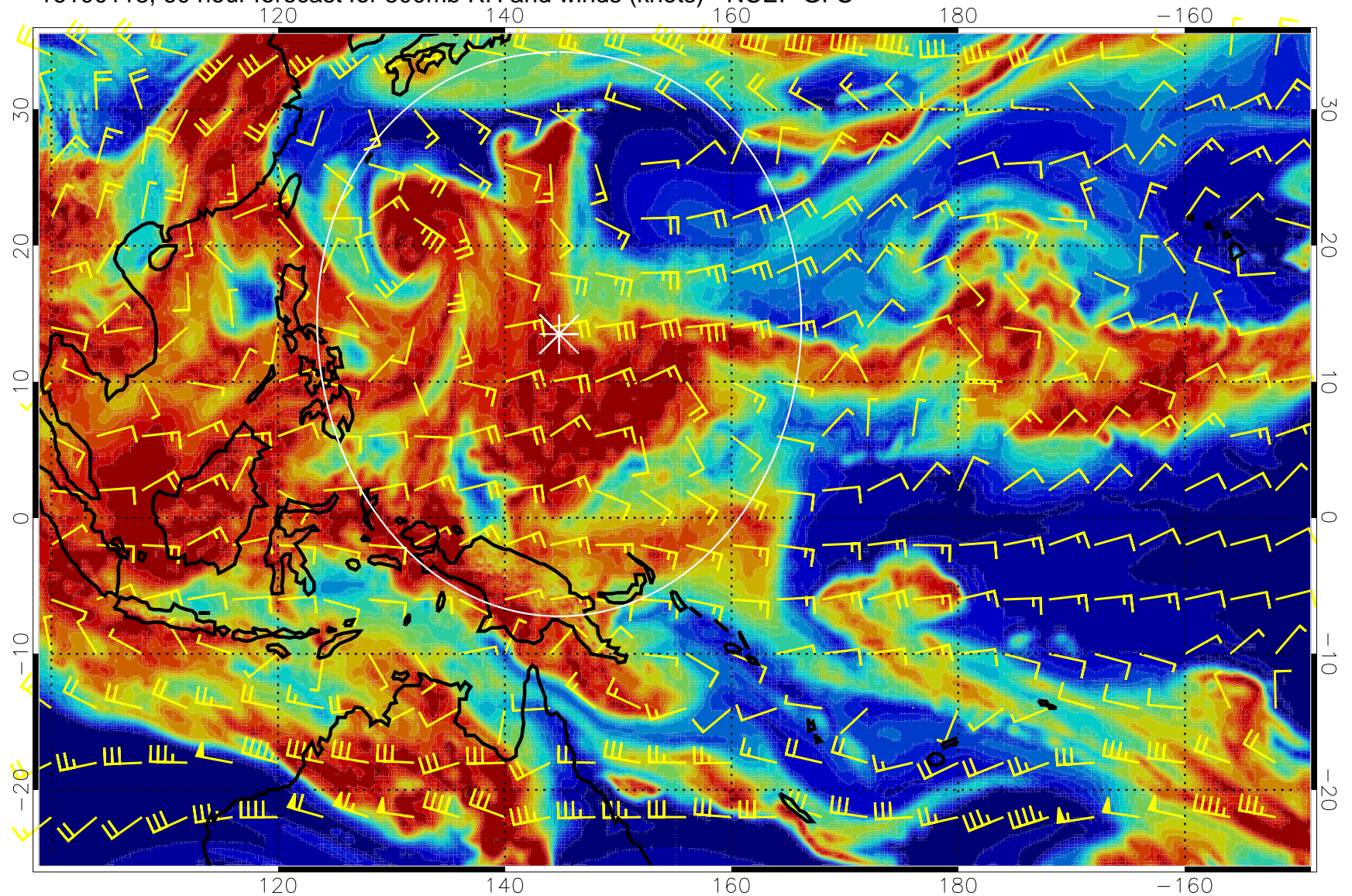
16100118, 60 hour forecast for 500mb RH and winds (knots) - NCEP GFS
