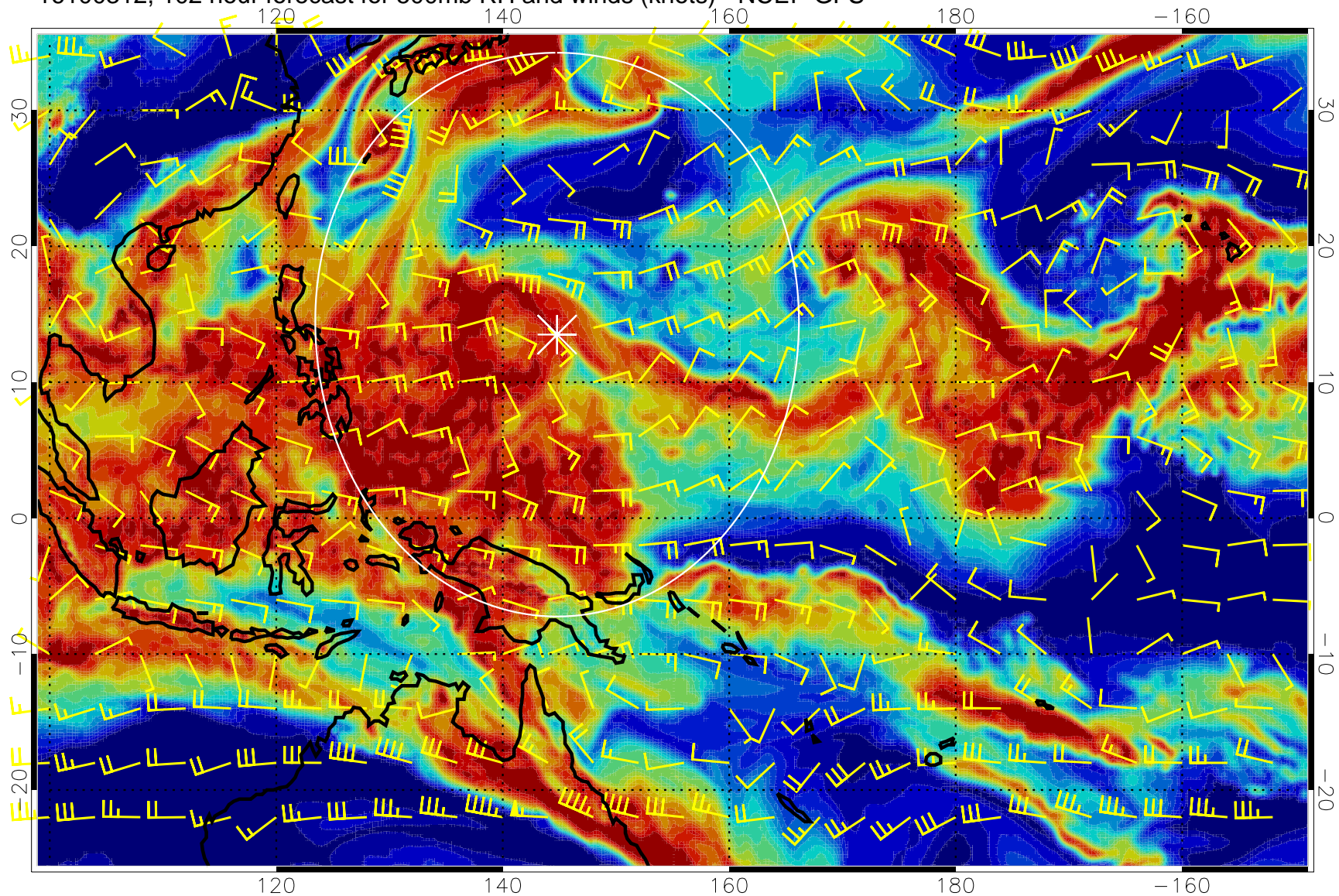
16100312, 102 hour forecast for 500mb RH and winds (knots) - NCEP GFS
