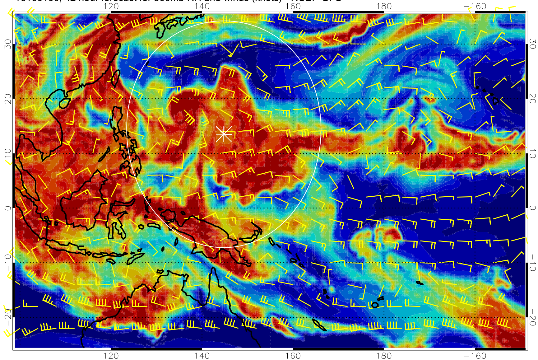
16100100, 42 hour forecast for 500mb RH and winds (knots) - NCEP GFS
