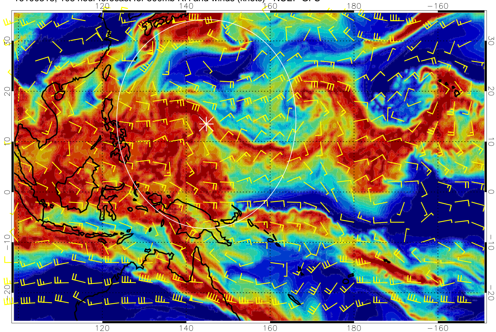
16100318, 108 hour forecast for 500mb RH and winds (knots) - NCEP GFS
