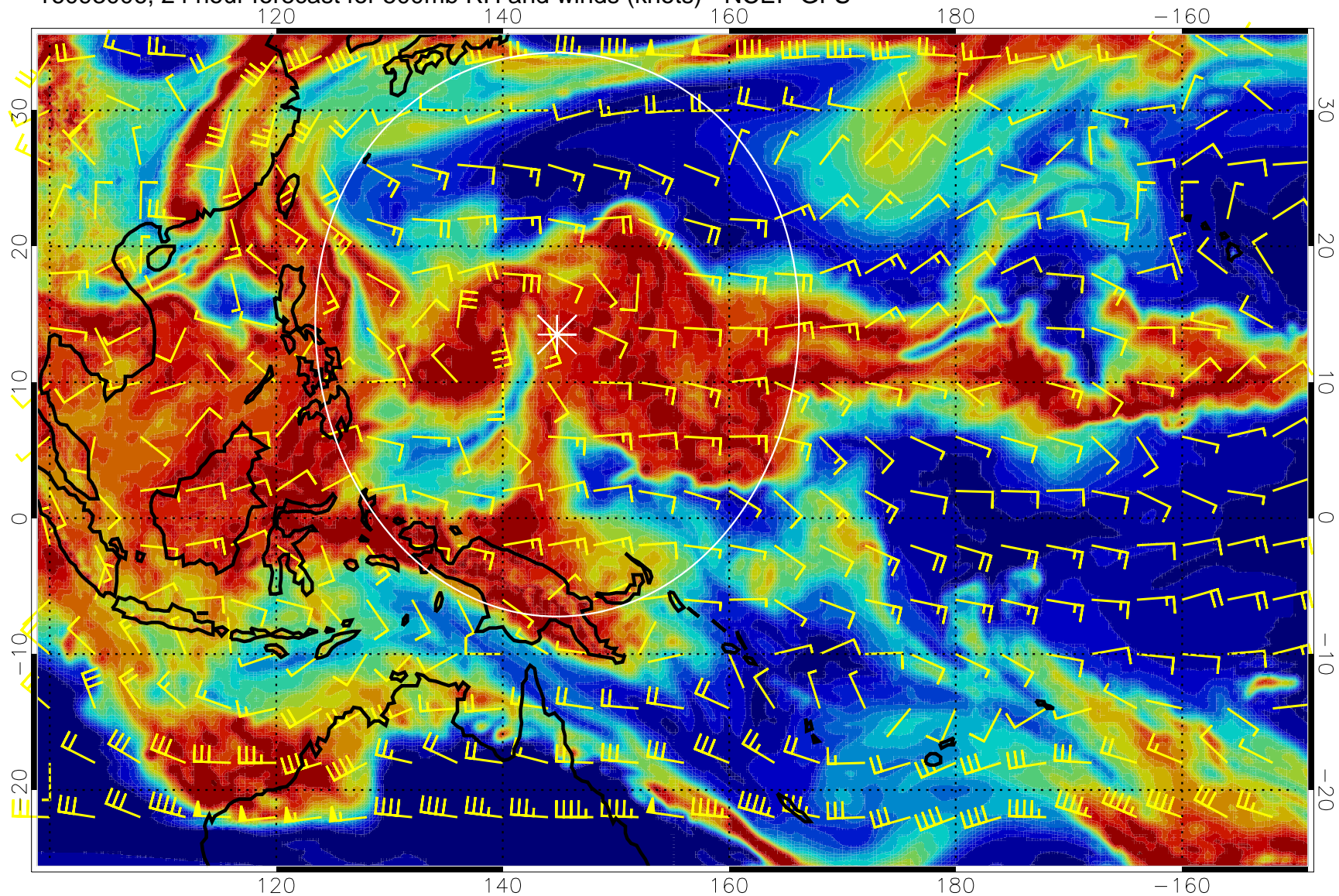
16093006, 24 hour forecast for 500mb RH and winds (knots) - NCEP GFS
