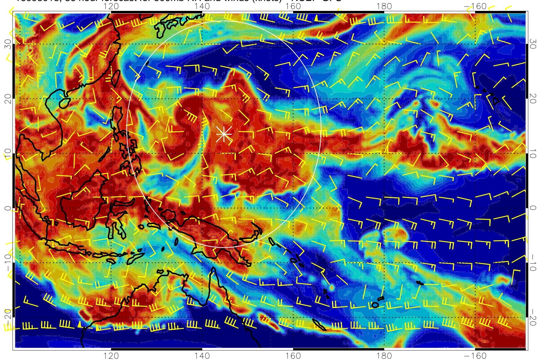
16093018, 36 hour forecast for 500mb RH and winds (knots) - NCEP GFS
