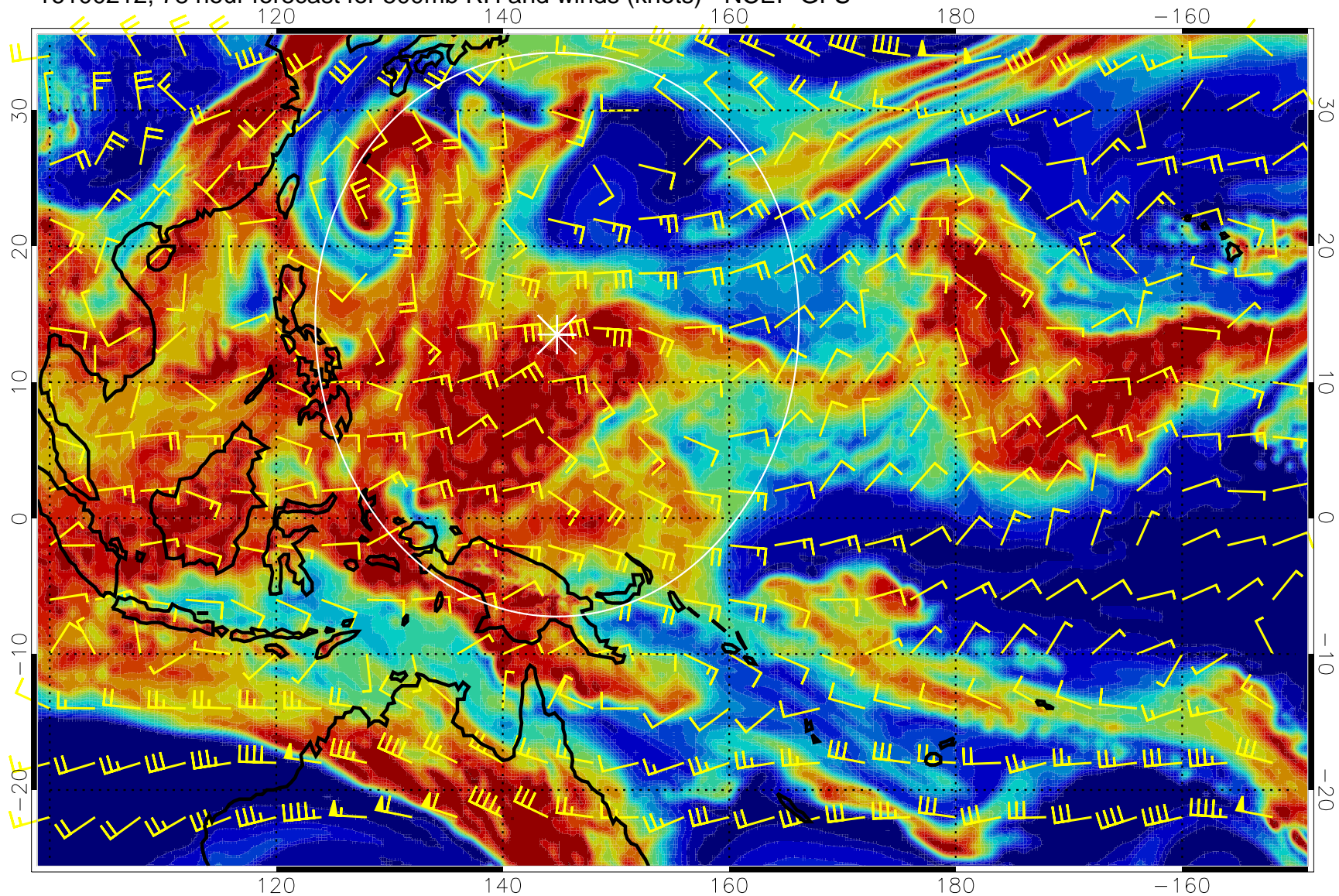
16100212, 78 hour forecast for 500mb RH and winds (knots) - NCEP GFS
