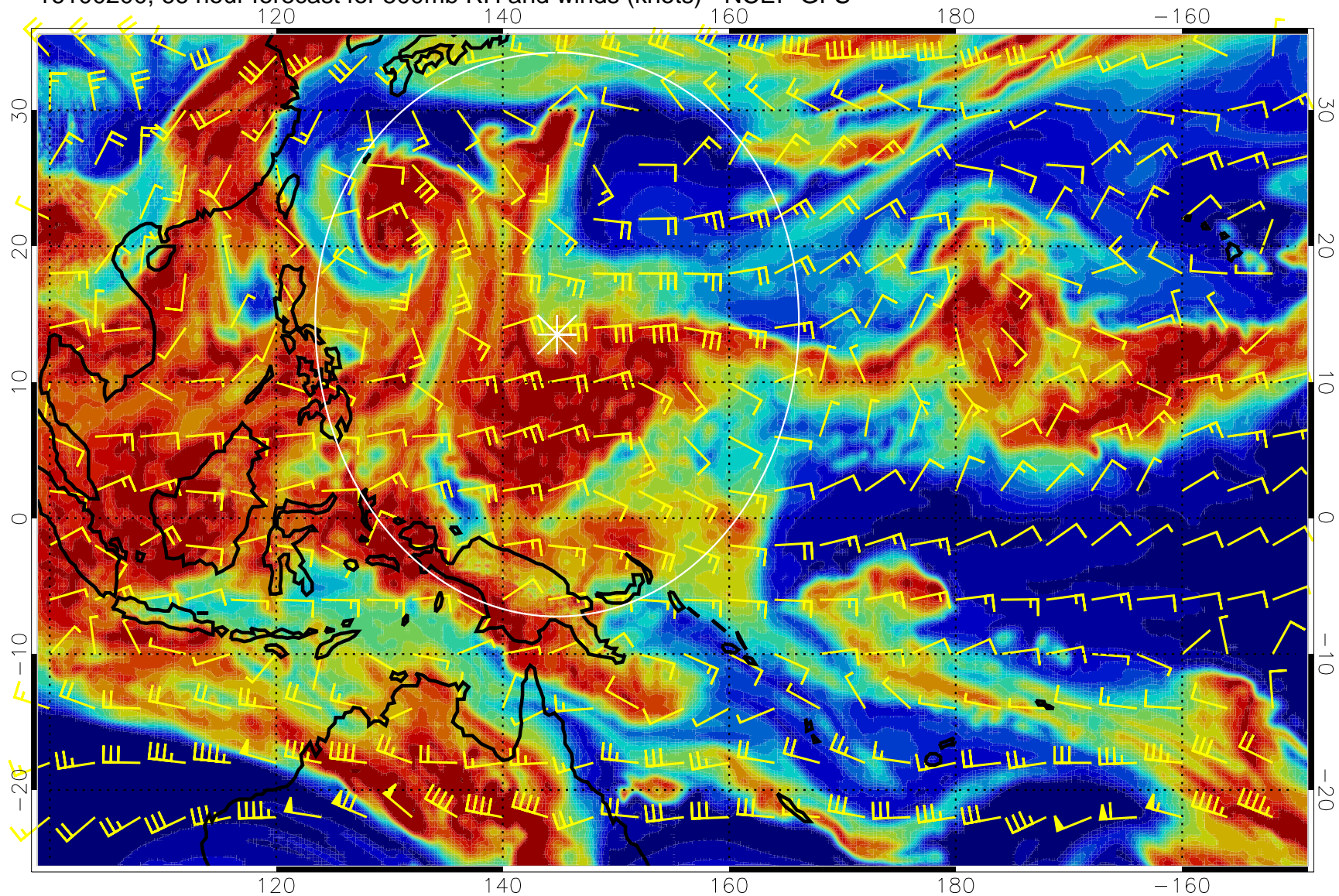
16100200, 66 hour forecast for 500mb RH and winds (knots) - NCEP GFS
