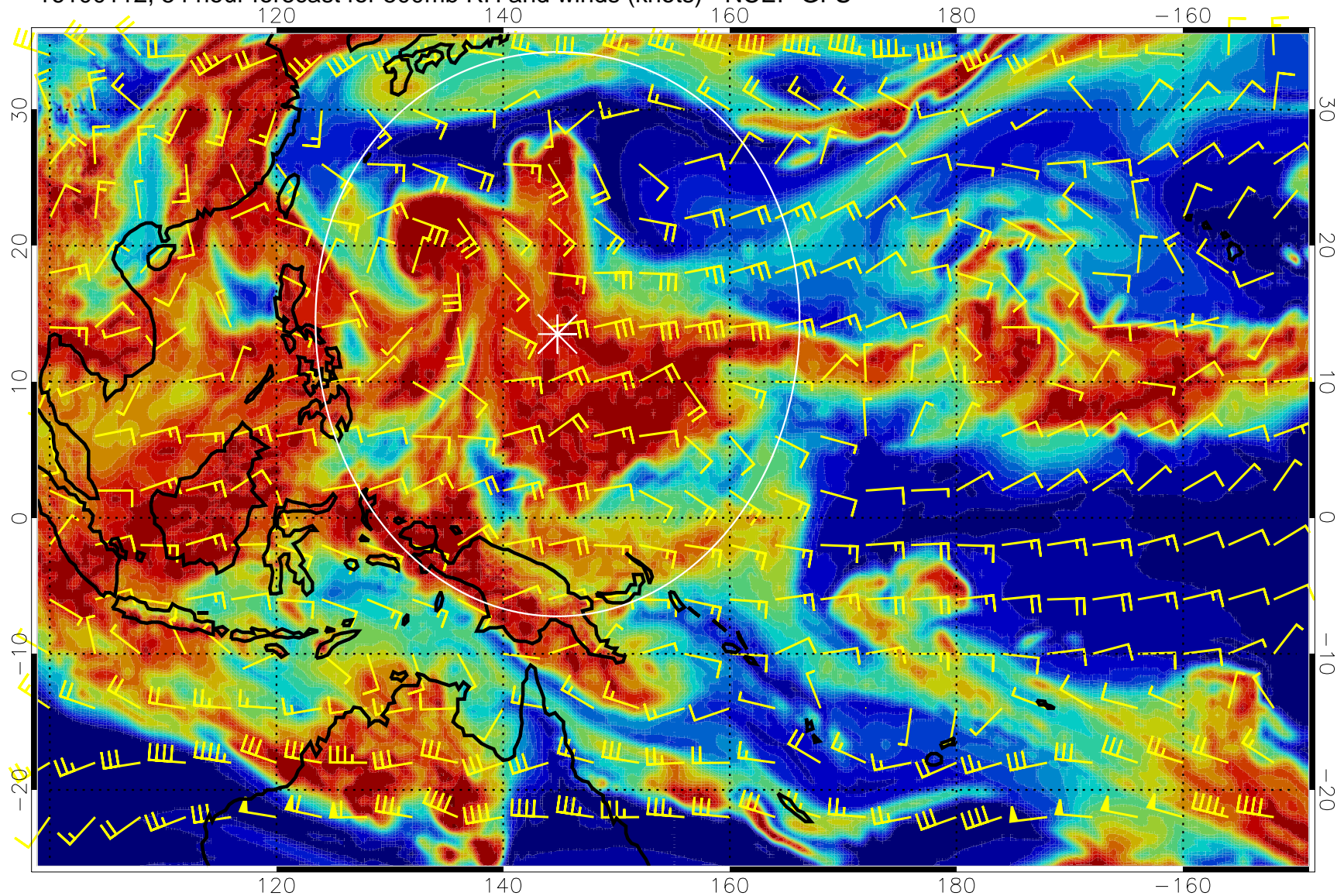
16100112, 54 hour forecast for 500mb RH and winds (knots) - NCEP GFS
