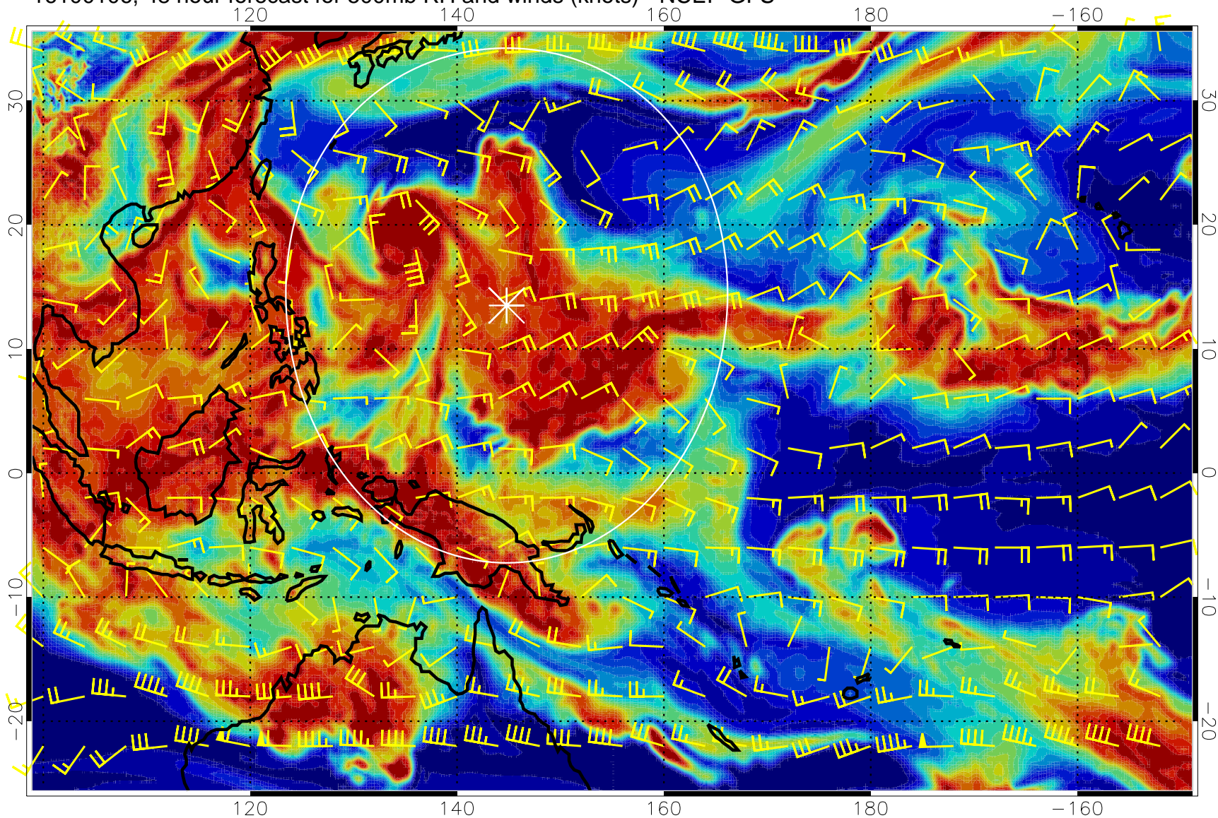
16100106, 48 hour forecast for 500mb RH and winds (knots) - NCEP GFS
