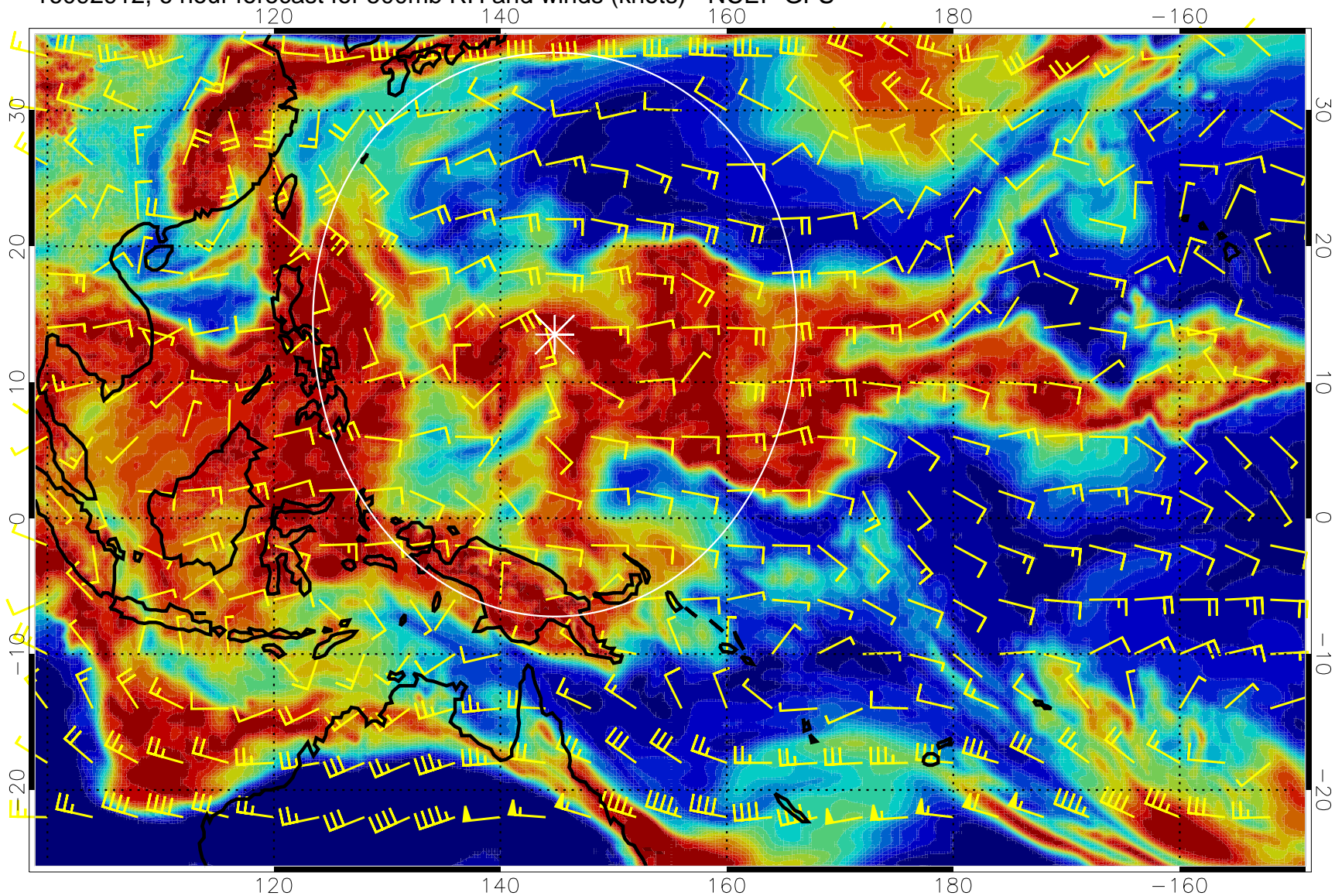
16092912, 6 hour forecast for 500mb RH and winds (knots) - NCEP GFS
