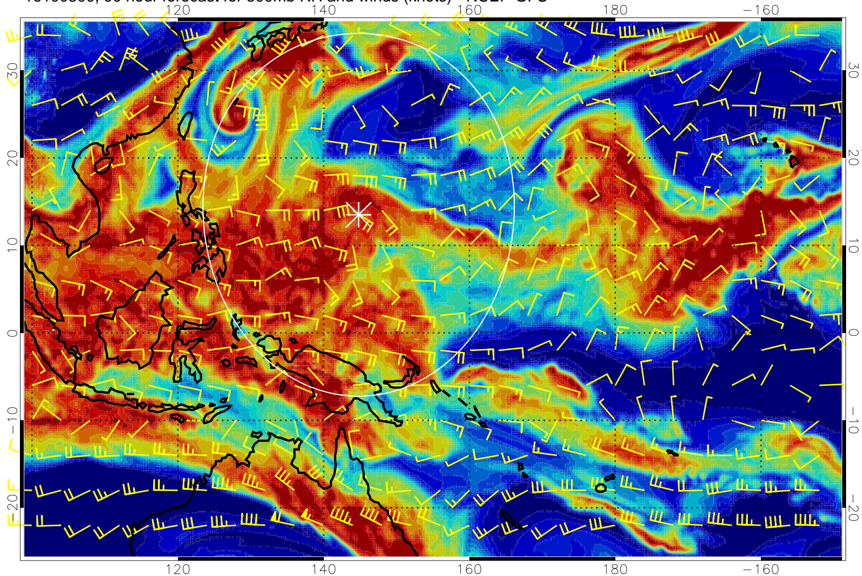
16100300, 90 hour forecast for 500mb RH and winds (knots) - NCEP GFS
