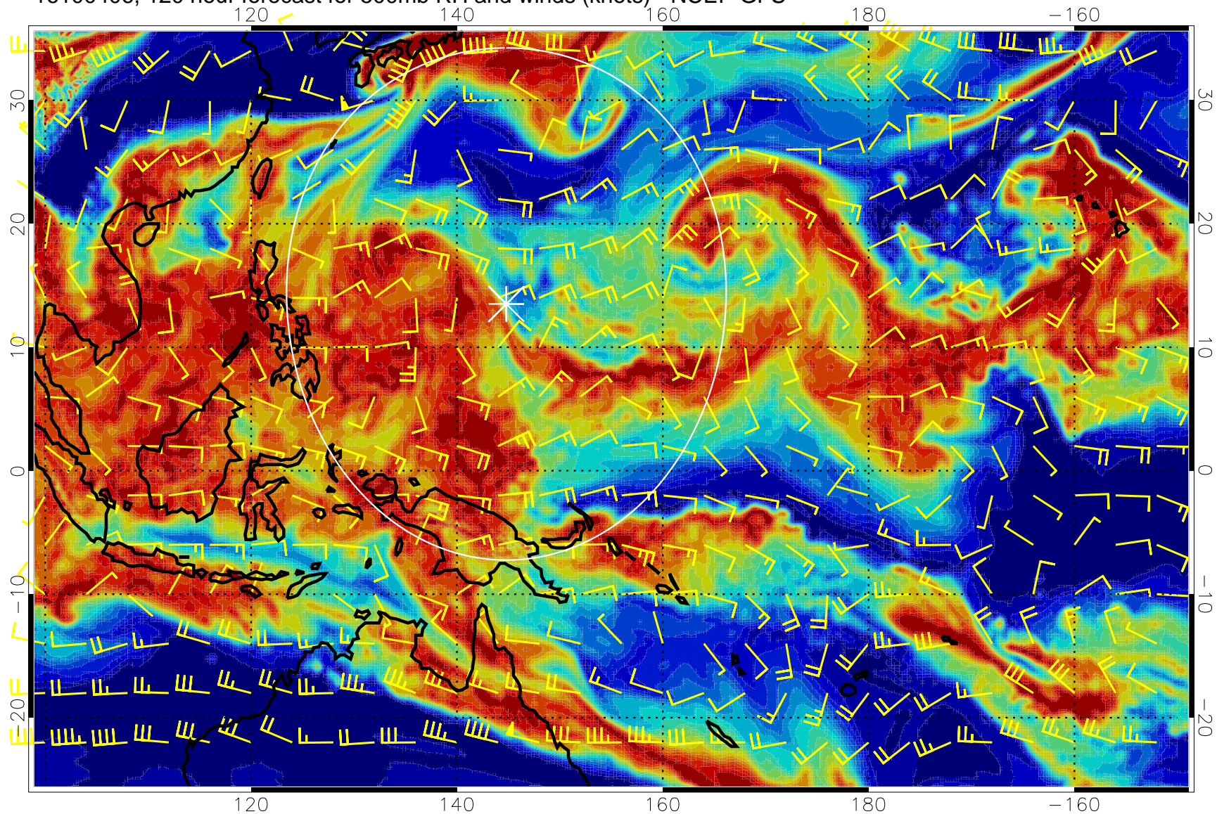
16100406, 120 hour forecast for 500mb RH and winds (knots) - NCEP GFS
