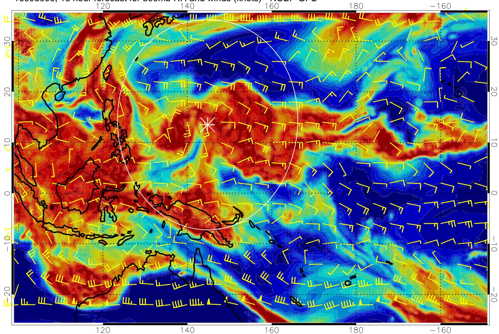
16093000, 18 hour forecast for 500mb RH and winds (knots) - NCEP GFS
