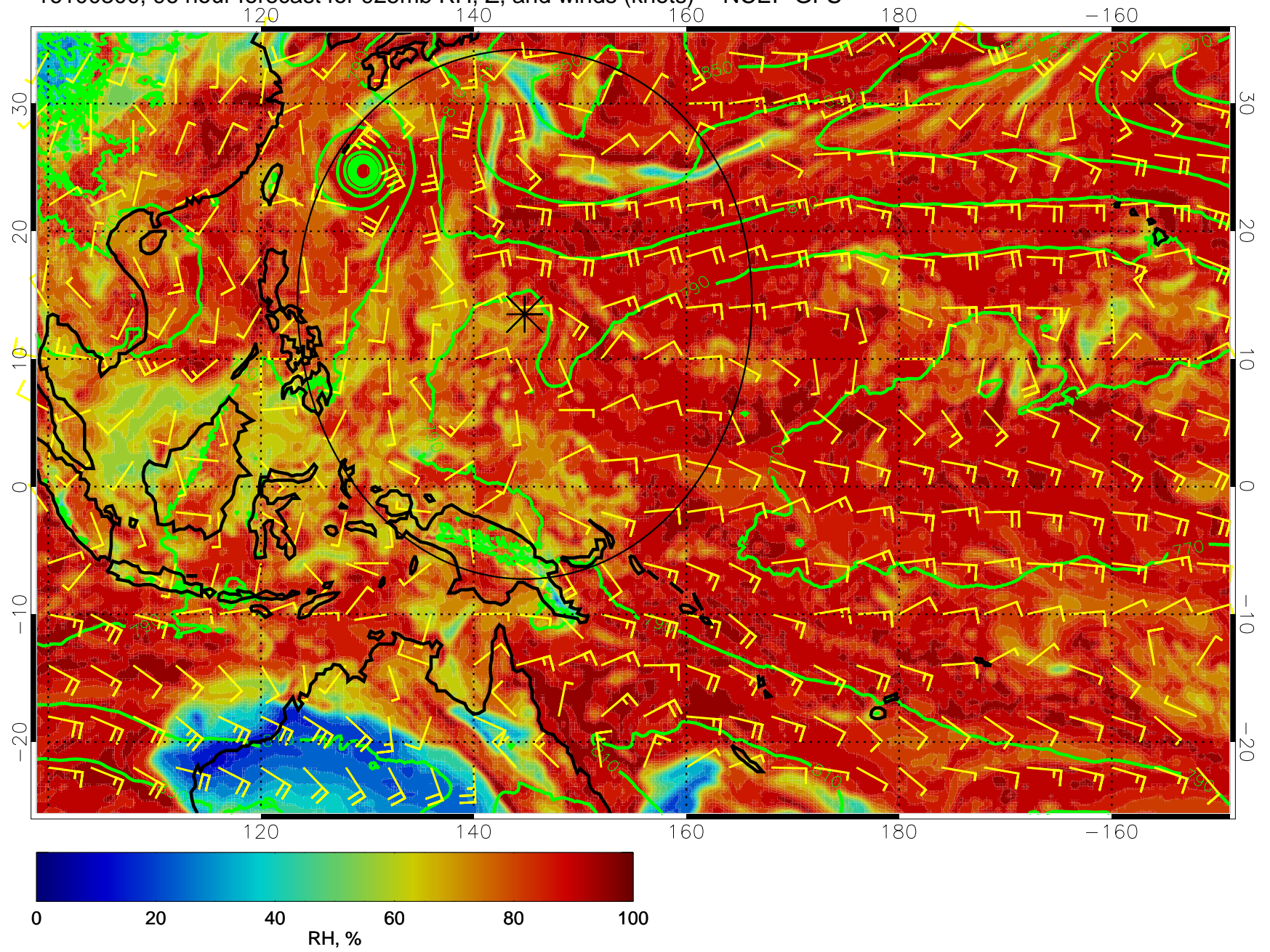
16100300, 96 hour forecast for 925mb RH, Z, and winds (knots) -- NCEP GFS
