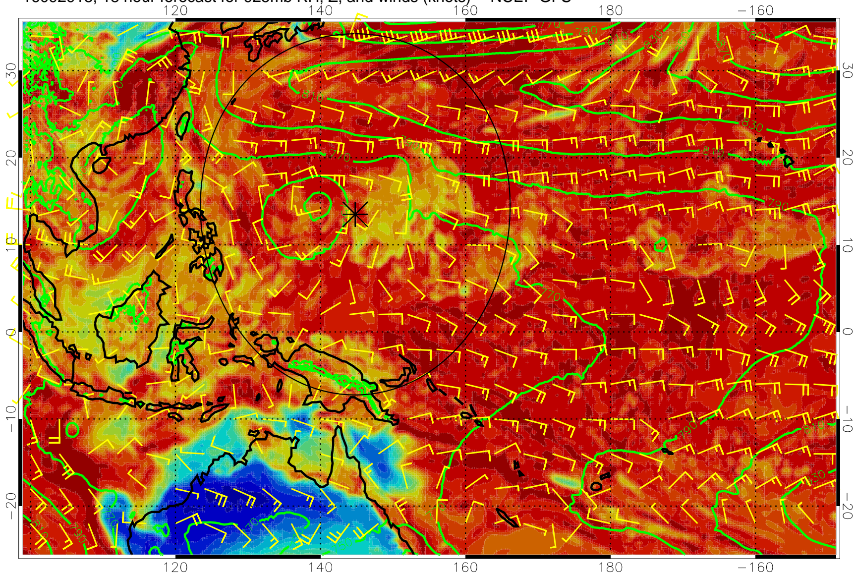
16092918, 18 hour forecast for 925mb RH, Z, and winds (knots) -- NCEP GFS
