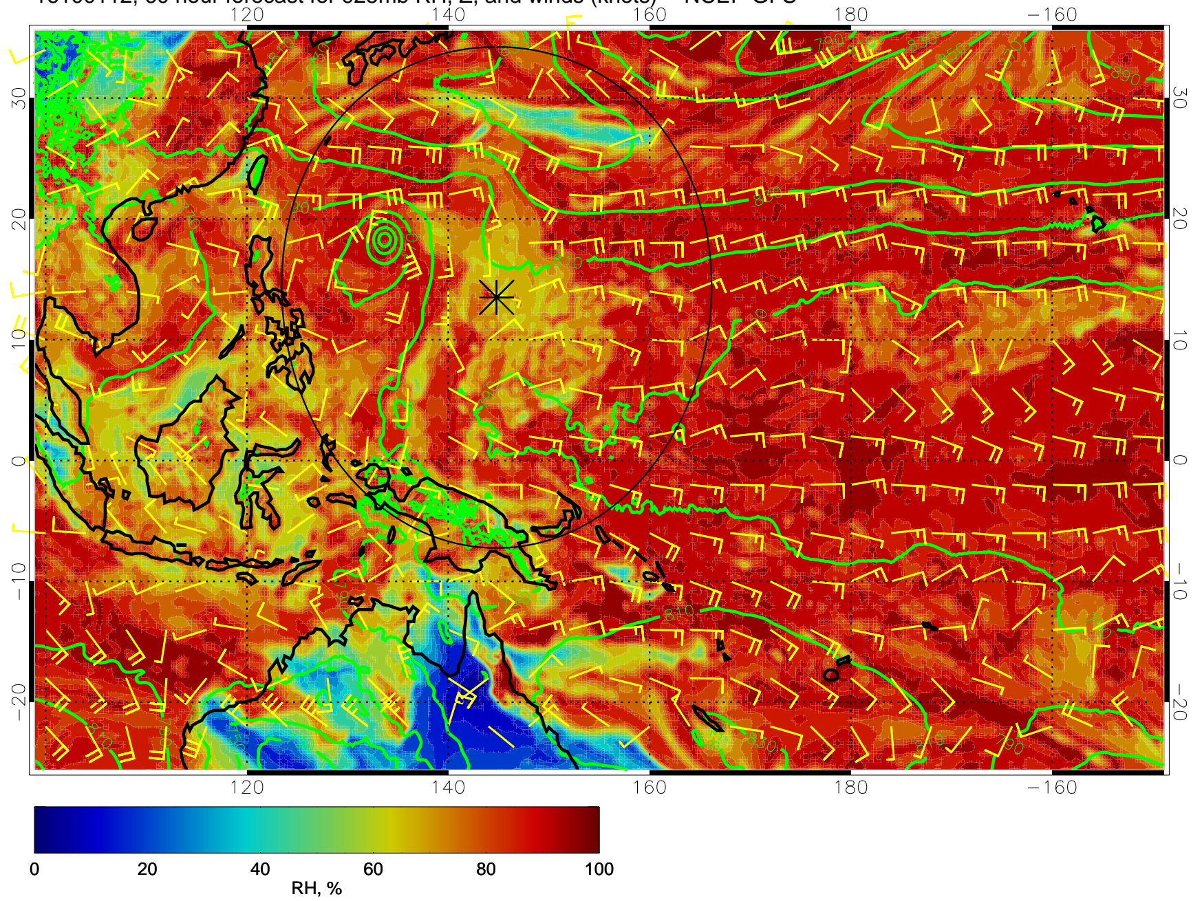
16100112, 60 hour forecast for 925mb RH, Z, and winds (knots) -- NCEP GFS
