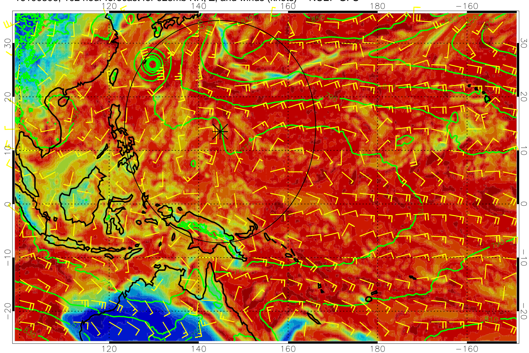
16100306, 102 hour forecast for 925mb RH, Z, and winds (knots) -- NCEP GFS
