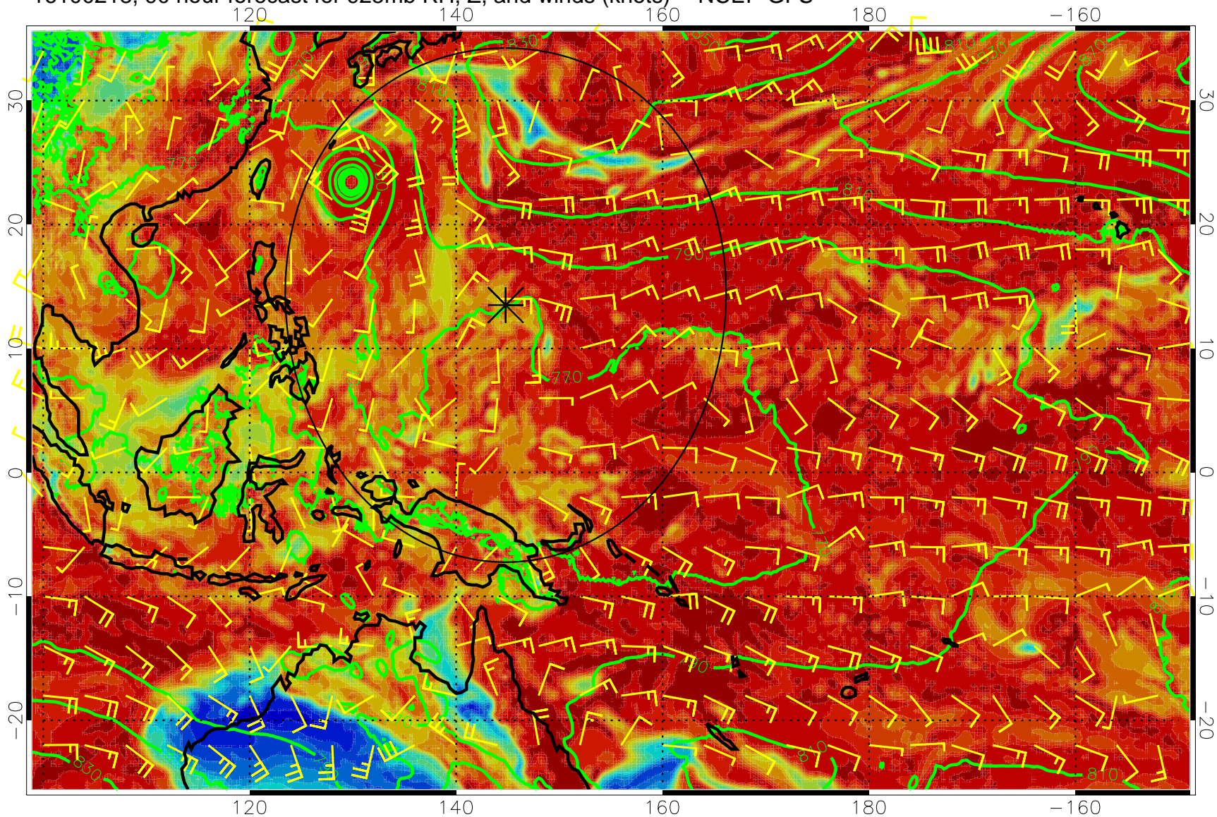
16100218, 90 hour forecast for 925mb RH, Z, and winds (knots) -- NCEP GFS
