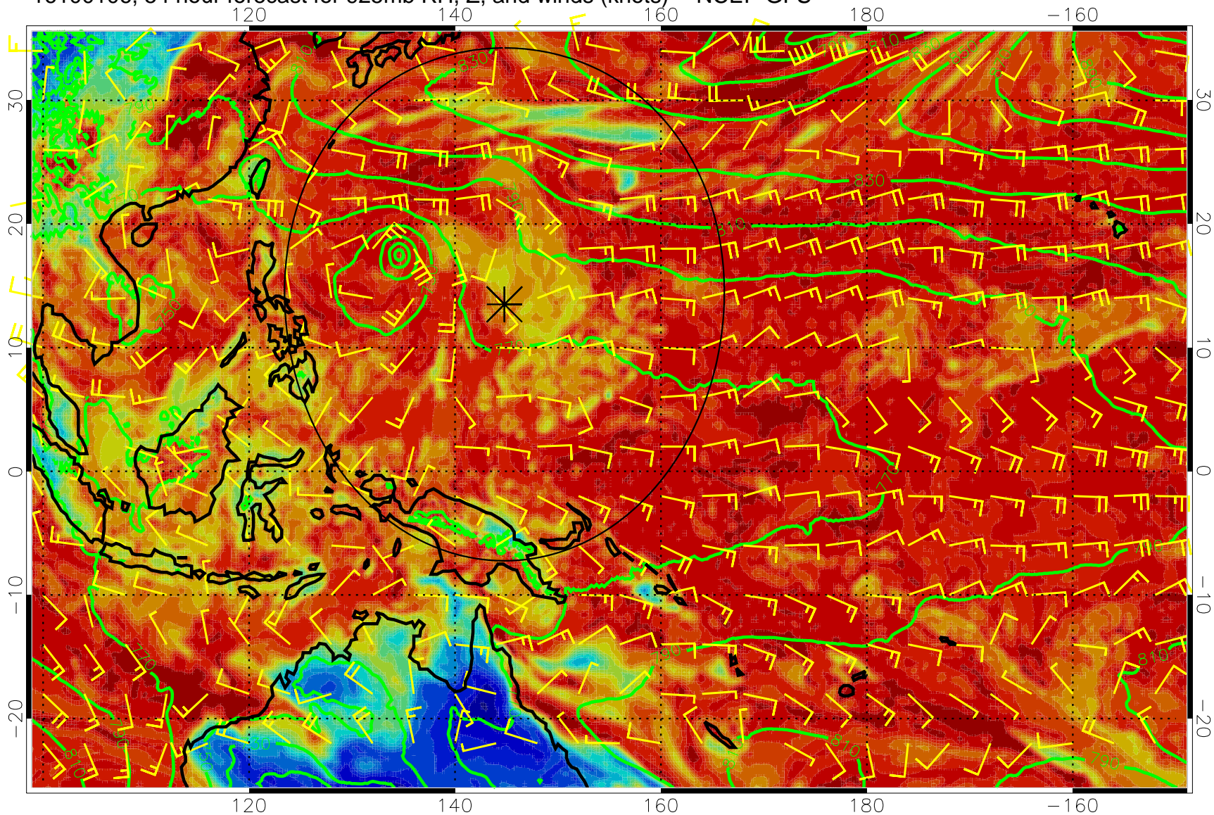
16100106, 54 hour forecast for 925mb RH, Z, and winds (knots) -- NCEP GFS
