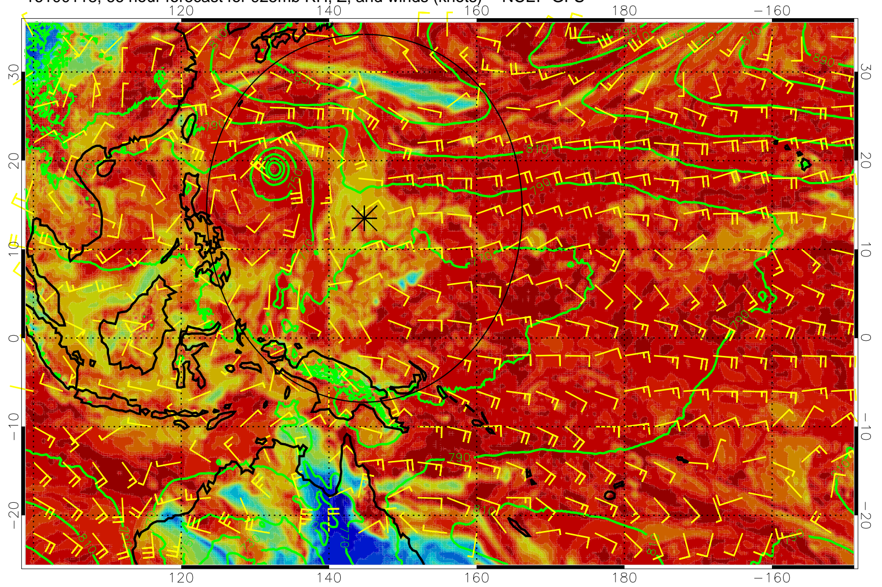
16100118, 66 hour forecast for 925mb RH, Z, and winds (knots) -- NCEP GFS
