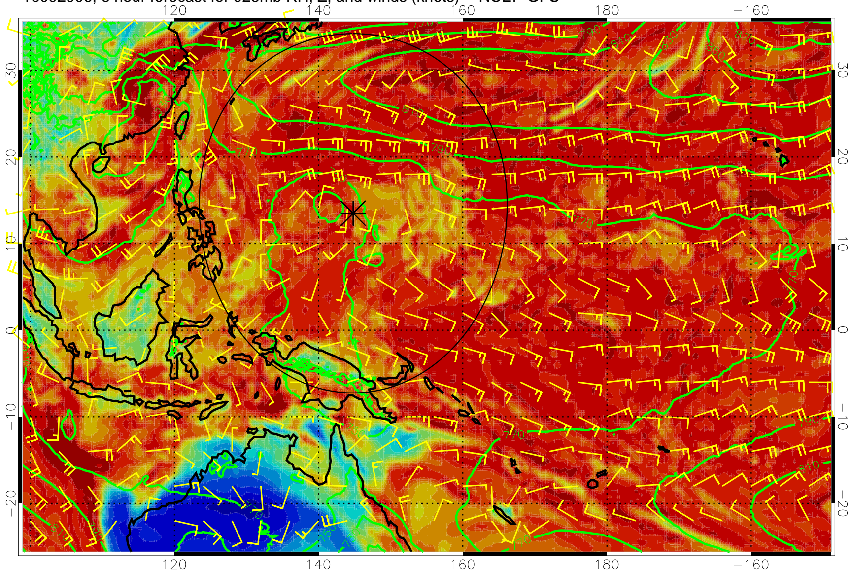
16092906, 6 hour forecast for 925mb RH, Z, and winds (knots) -- NCEP GFS
