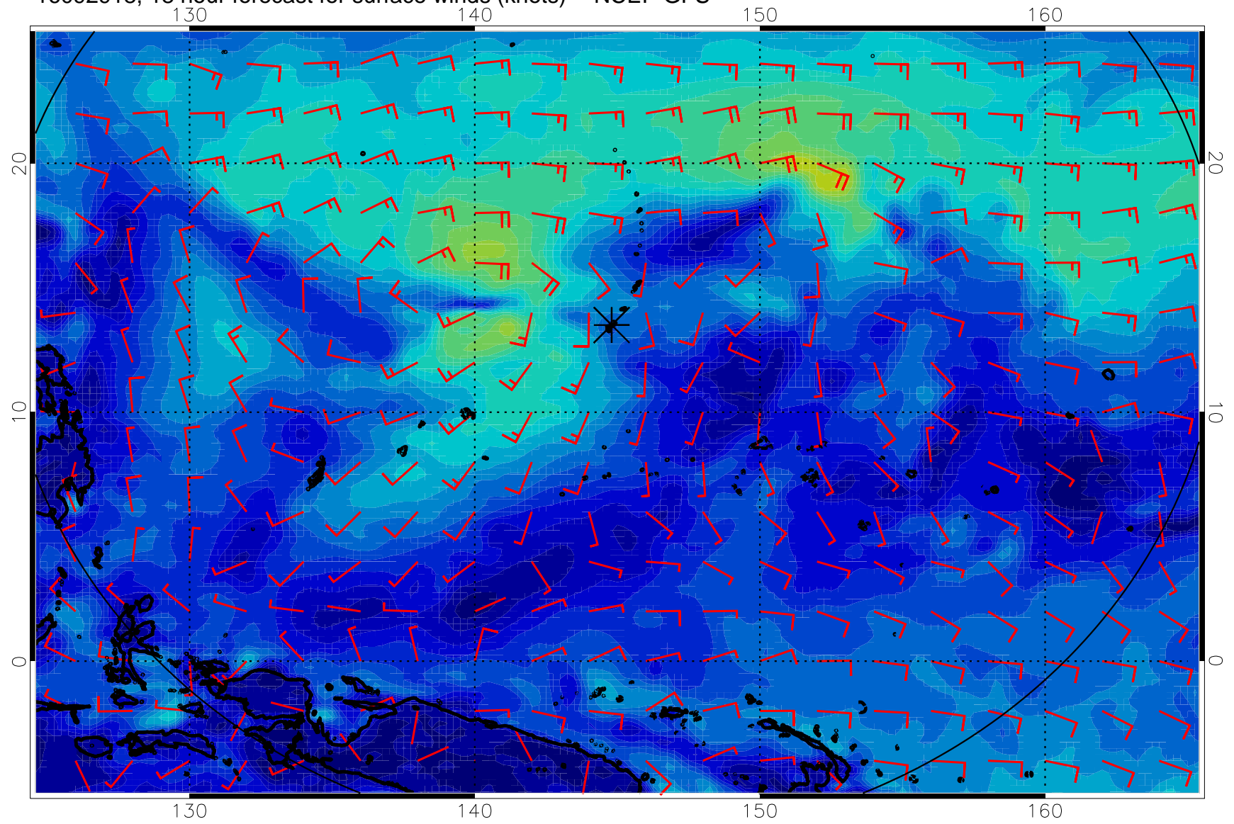
16092918, 18 hour forecast for surface winds (knots) -- NCEP GFS
