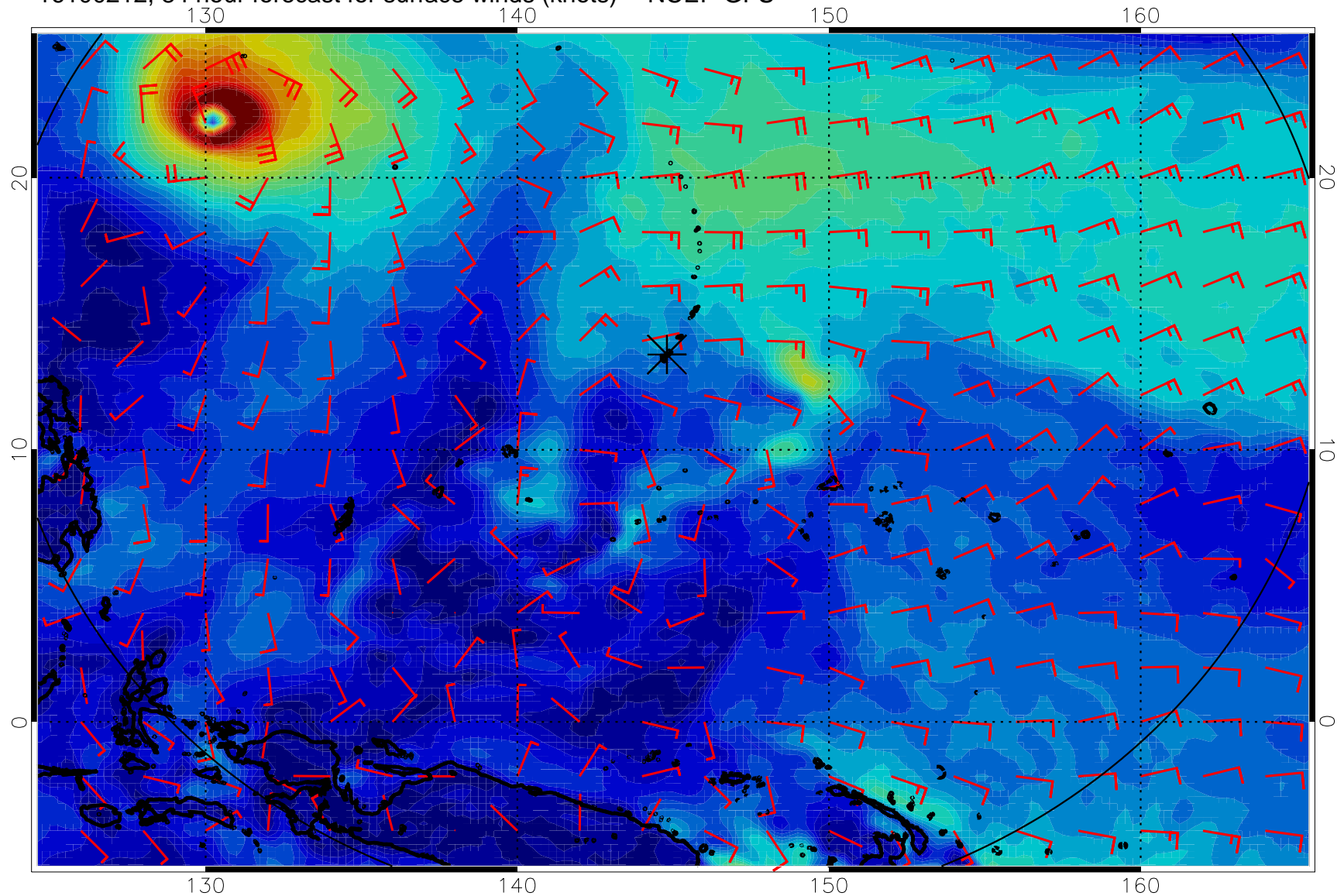
16100212, 84 hour forecast for surface winds (knots) -- NCEP GFS
