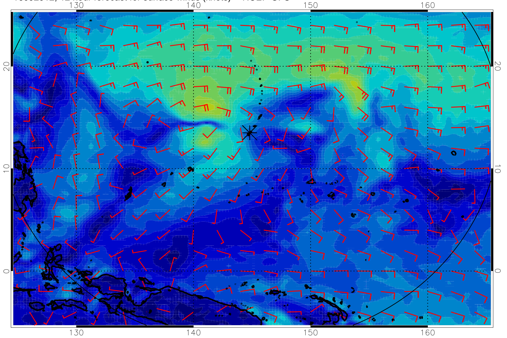
16092912, 12 hour forecast for surface winds (knots) -- NCEP GFS
