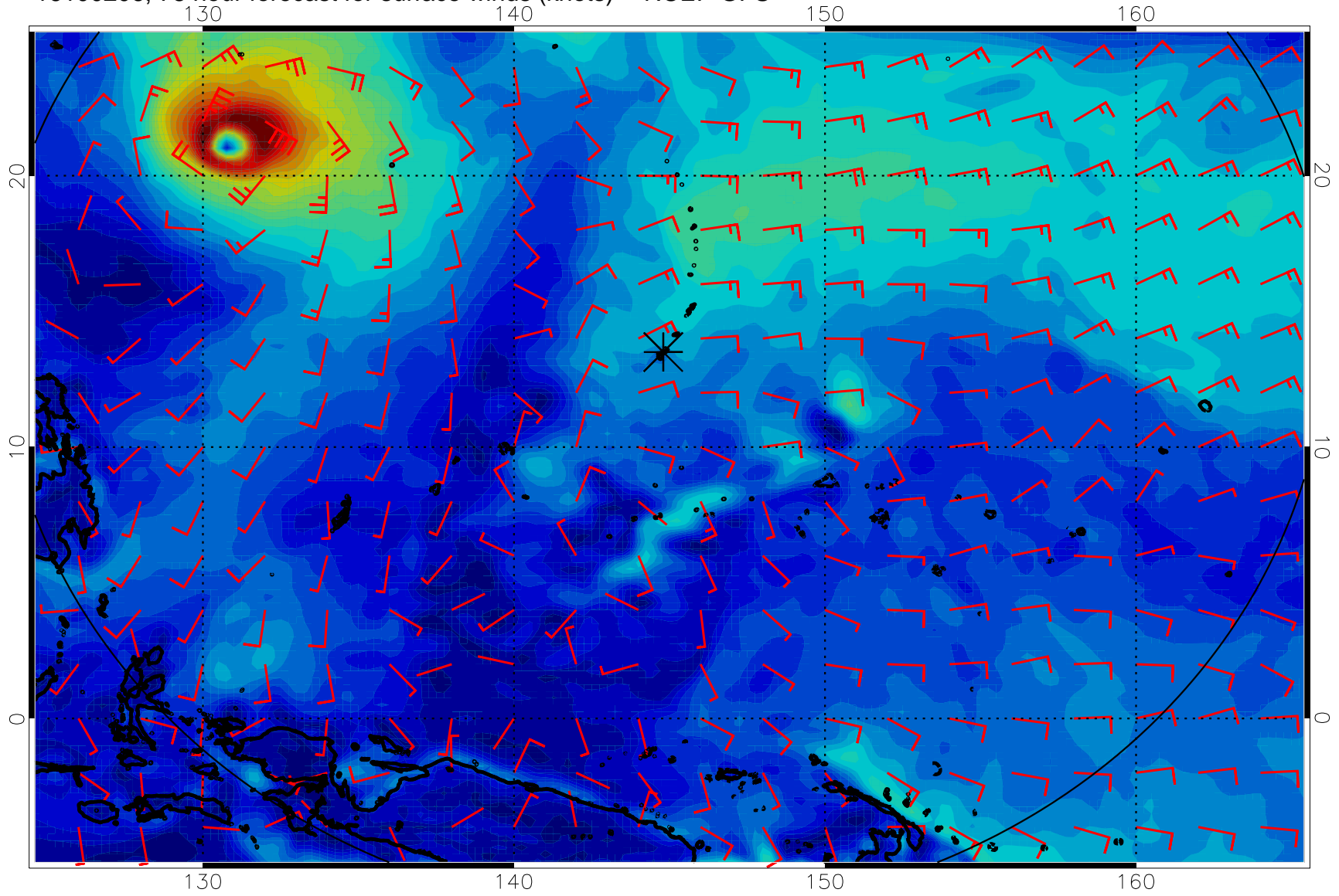
16100206, 78 hour forecast for surface winds (knots) -- NCEP GFS
