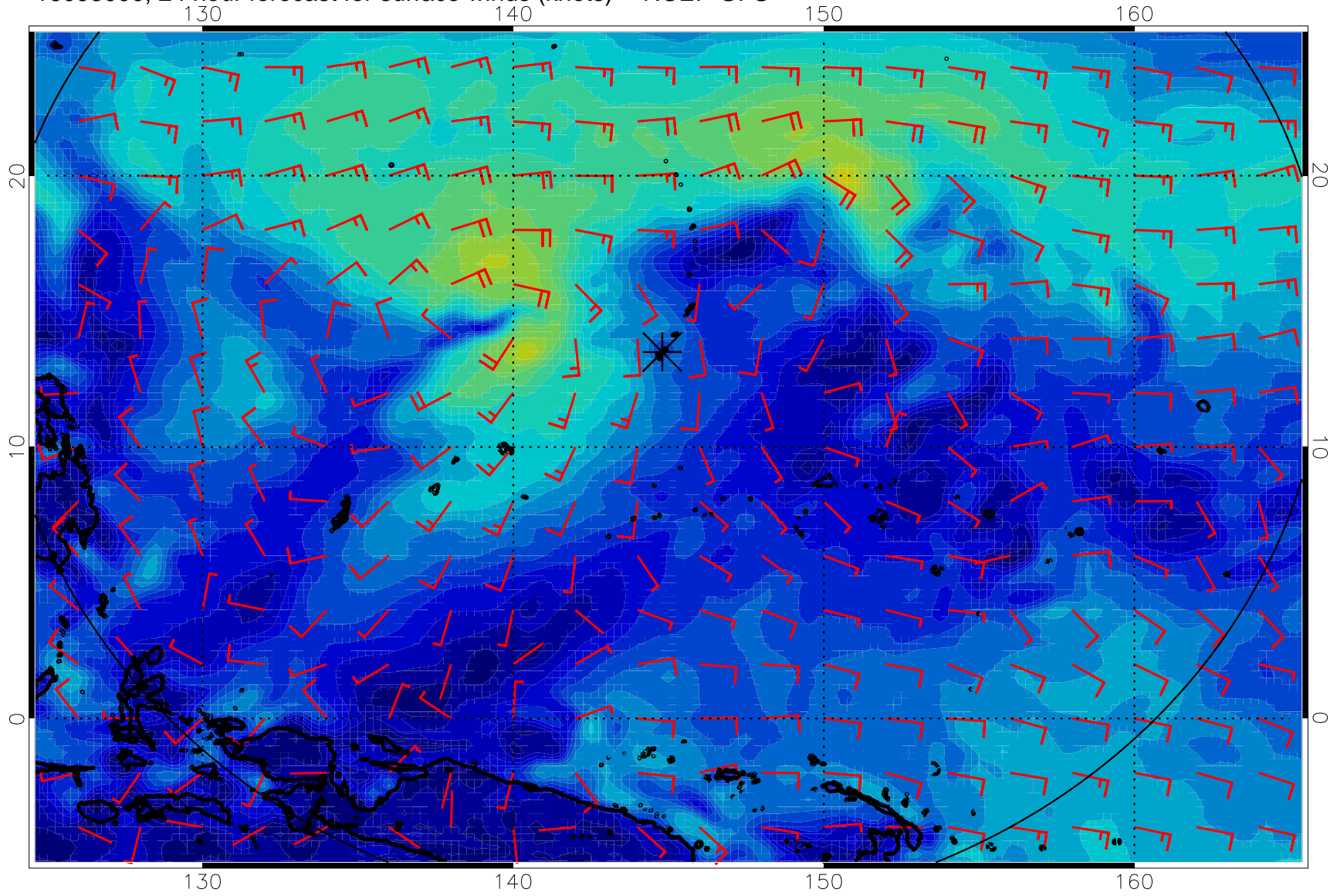
16093000, 24 hour forecast for surface winds (knots) -- NCEP GFS
