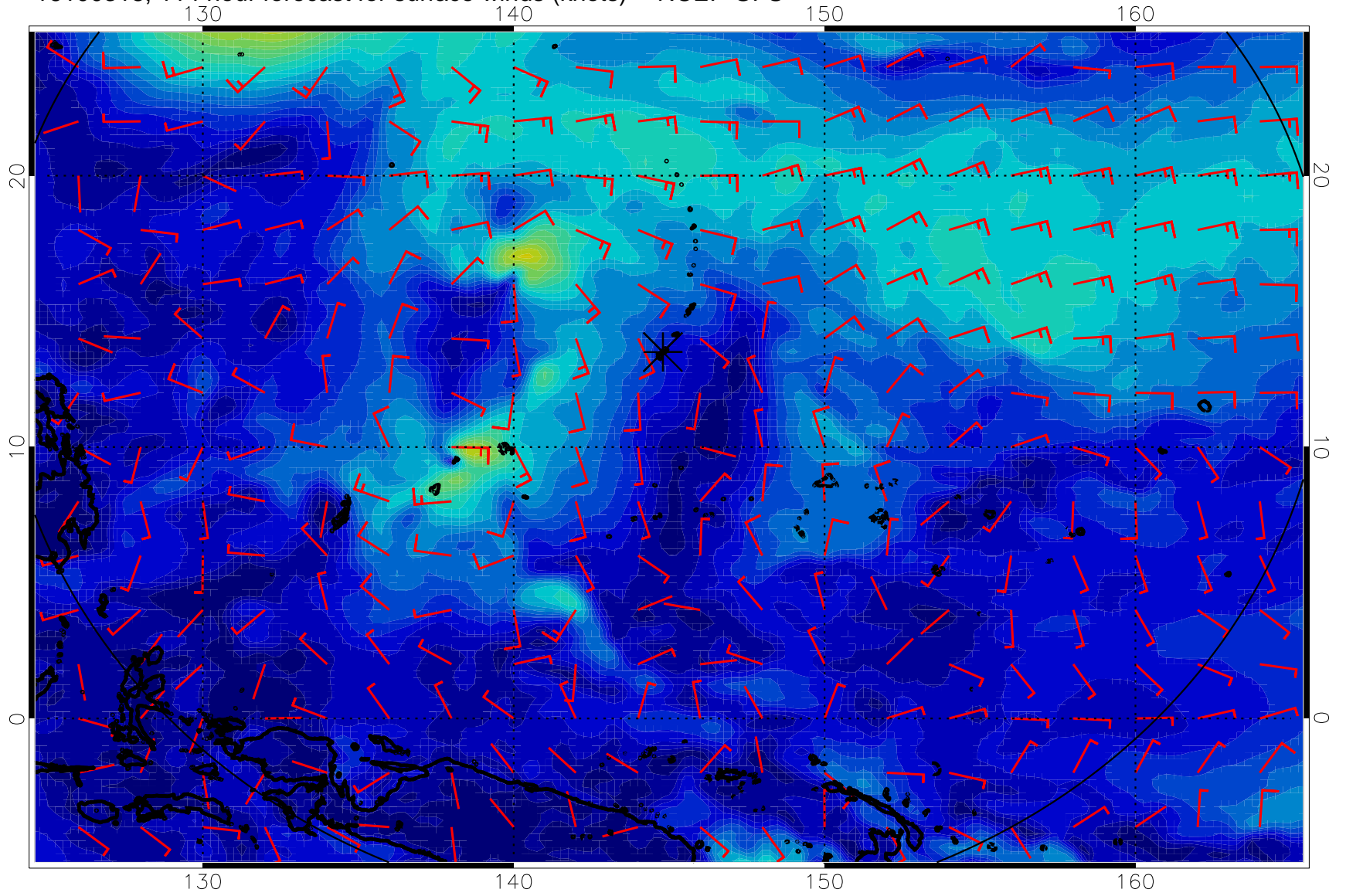
16100318, 114 hour forecast for surface winds (knots) -- NCEP GFS
