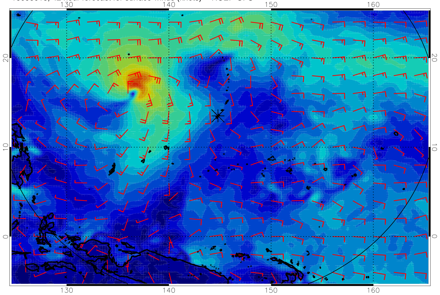
16093018, 42 hour forecast for surface winds (knots) -- NCEP GFS
