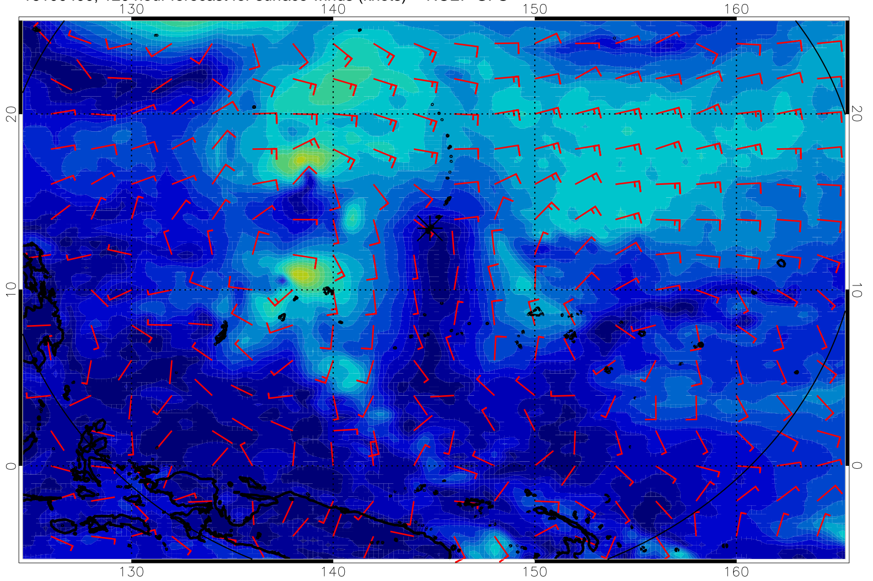
16100400, 120 hour forecast for surface winds (knots) -- NCEP GFS
