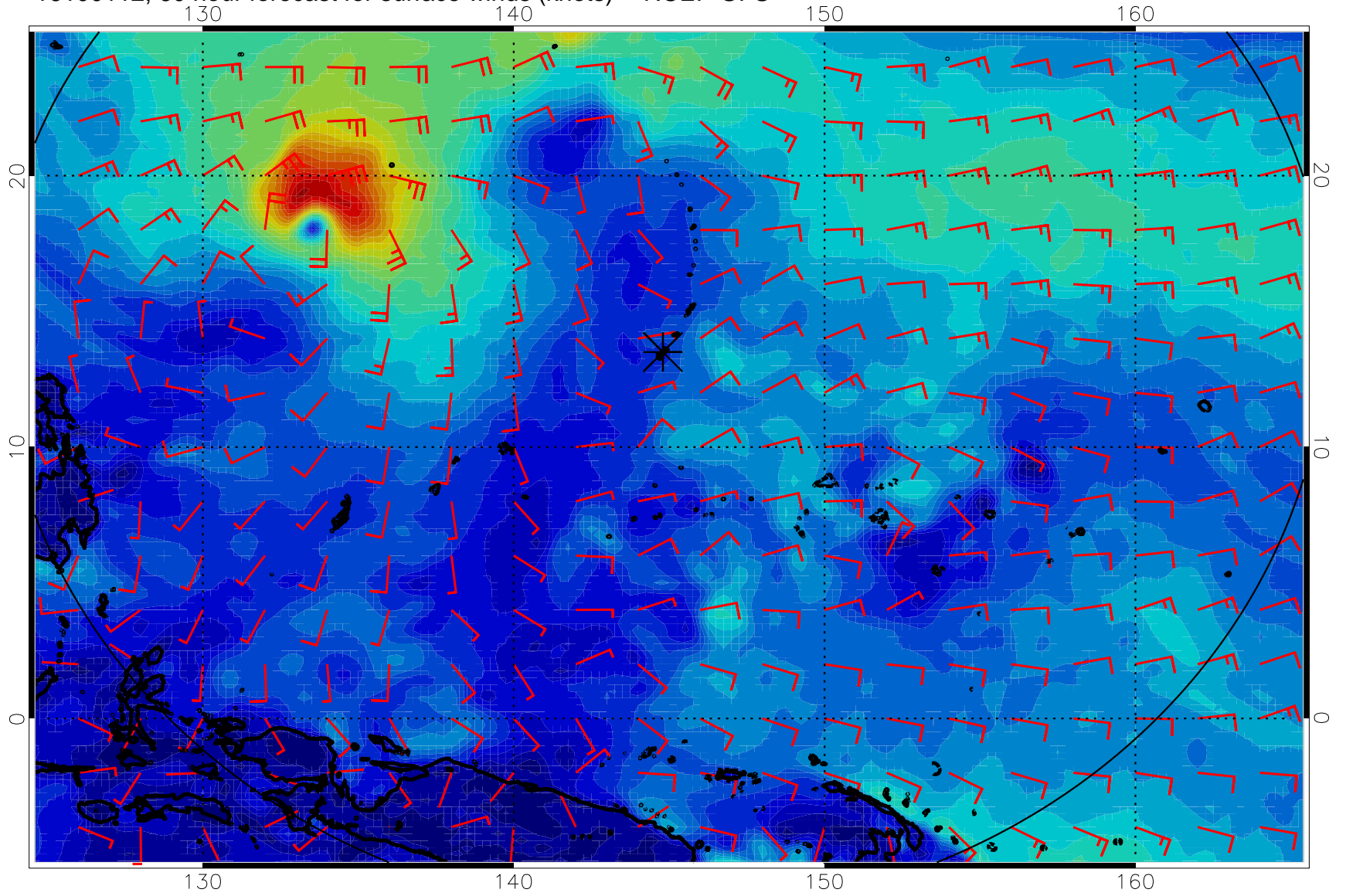
16100112, 60 hour forecast for surface winds (knots) -- NCEP GFS
