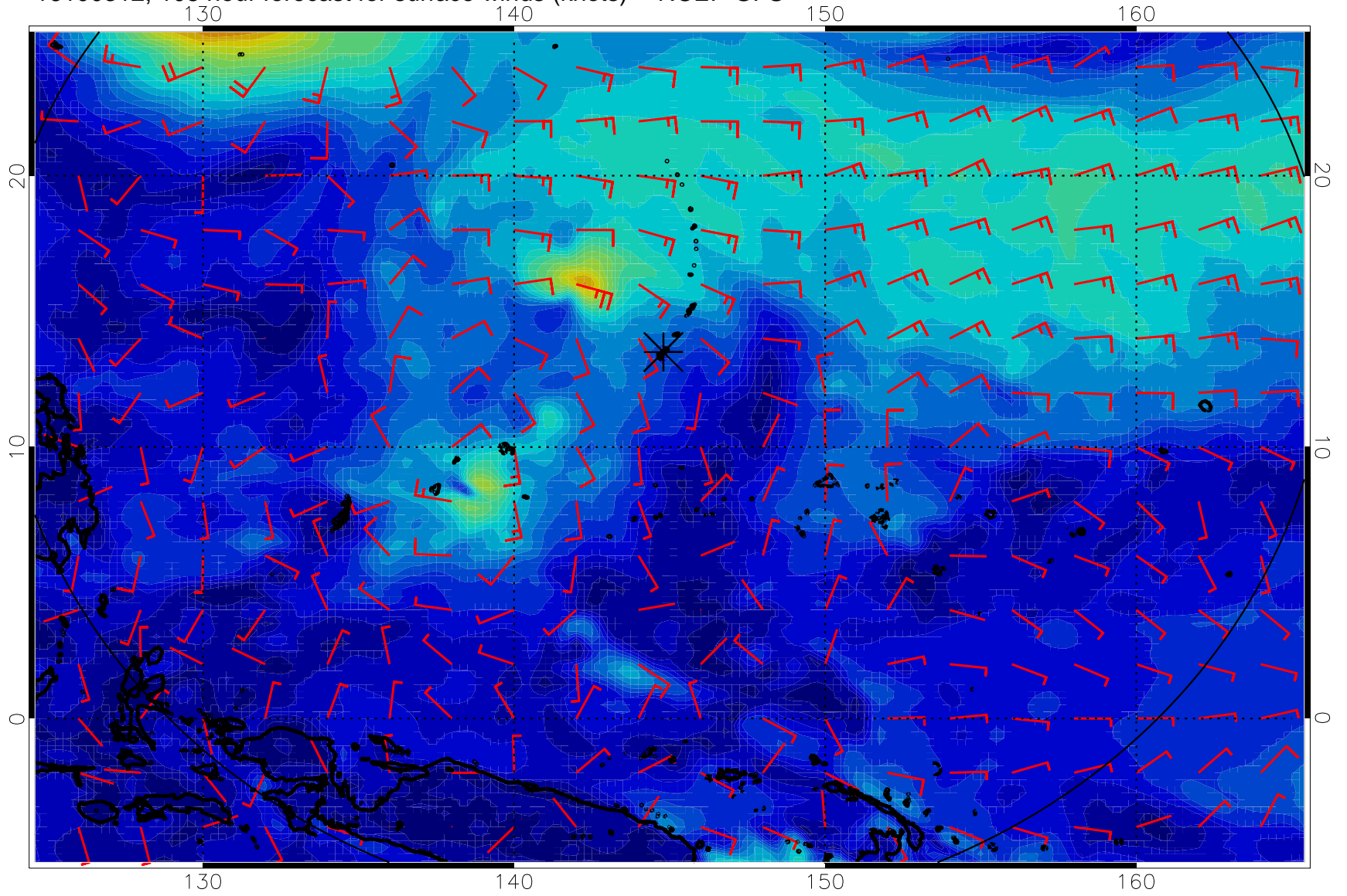
16100312, 108 hour forecast for surface winds (knots) -- NCEP GFS
