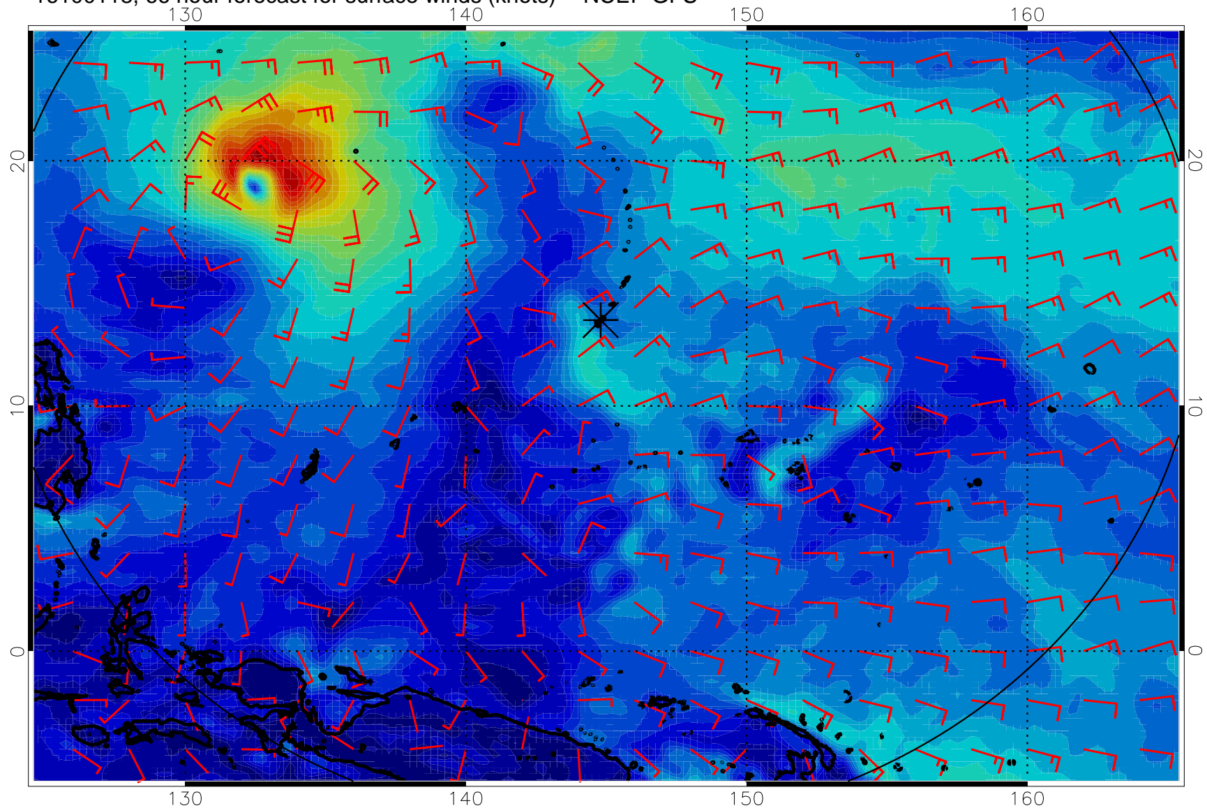
16100118, 66 hour forecast for surface winds (knots) -- NCEP GFS
