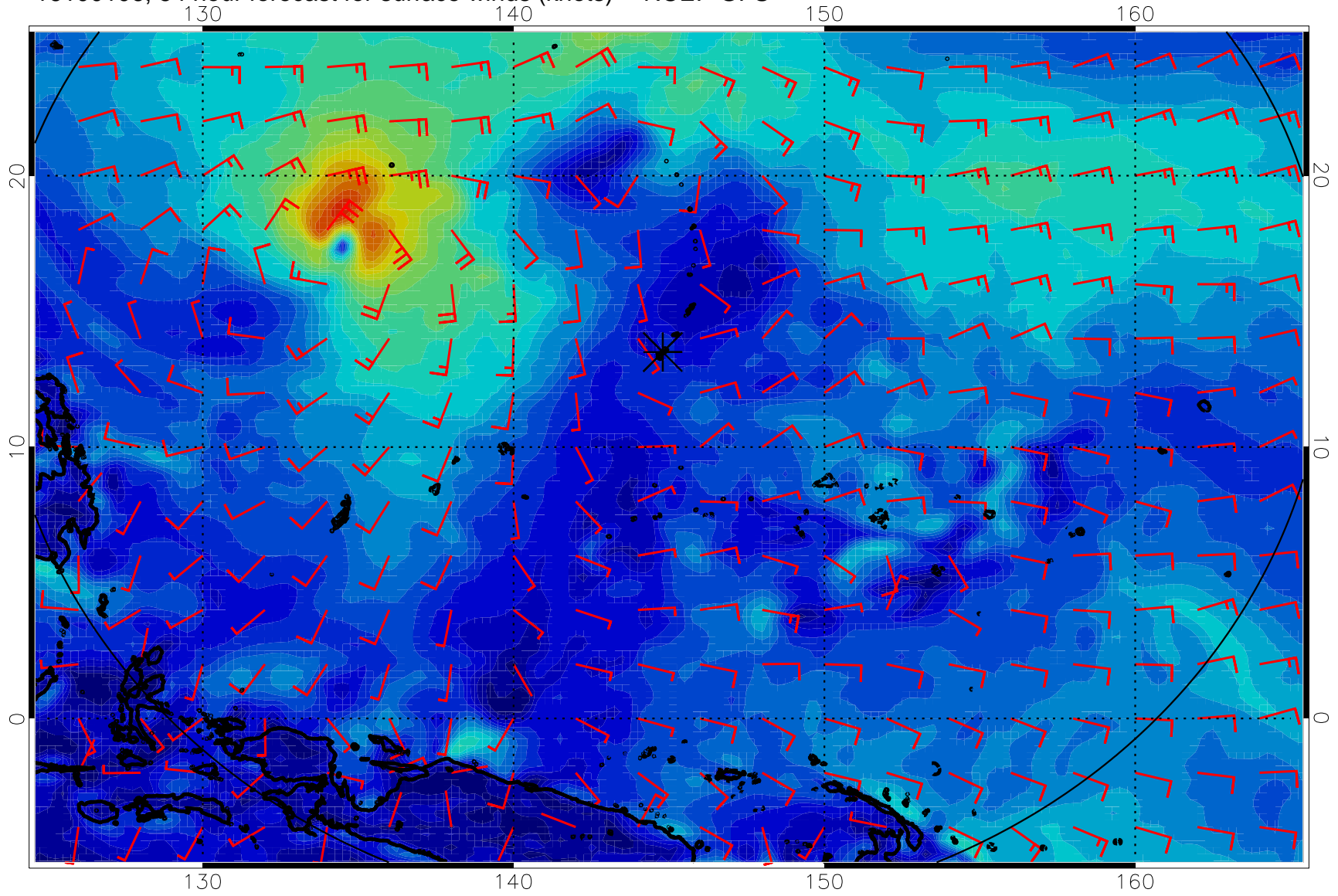
16100106, 54 hour forecast for surface winds (knots) -- NCEP GFS
