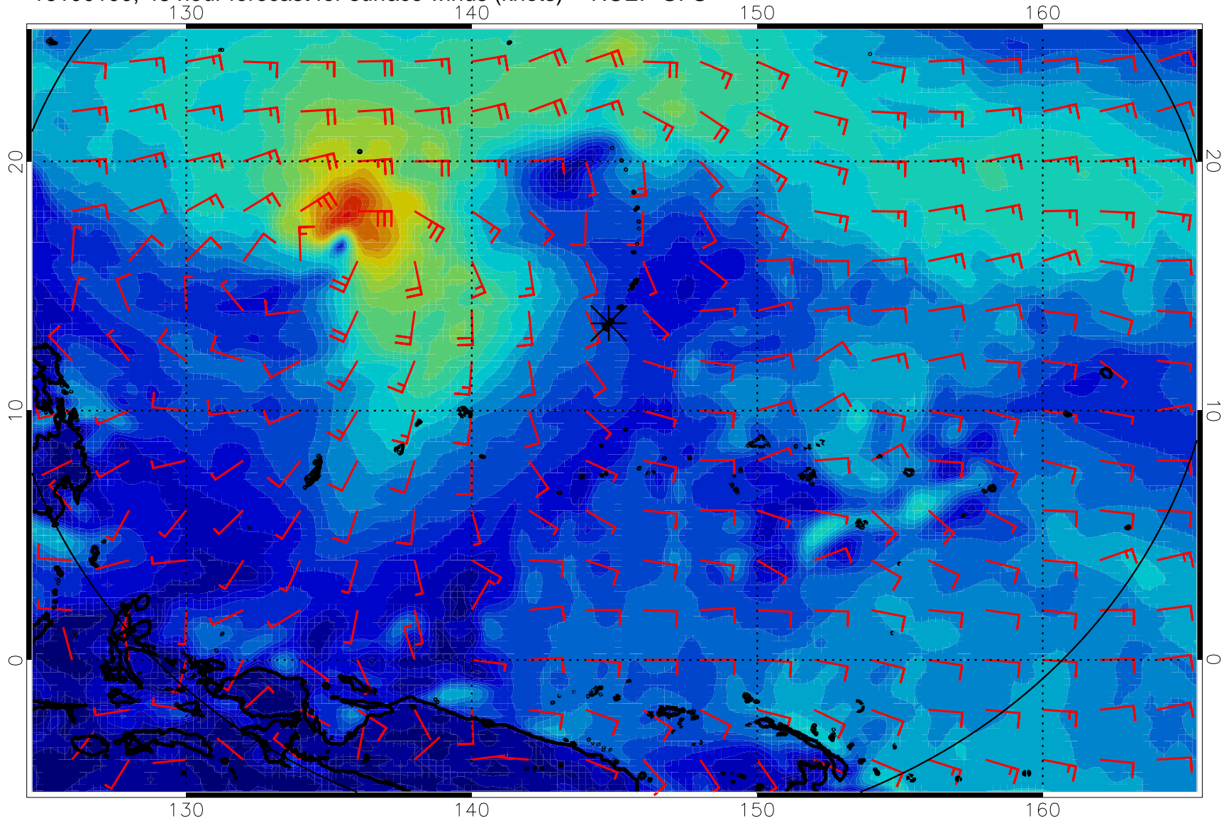
16100100, 48 hour forecast for surface winds (knots) -- NCEP GFS
