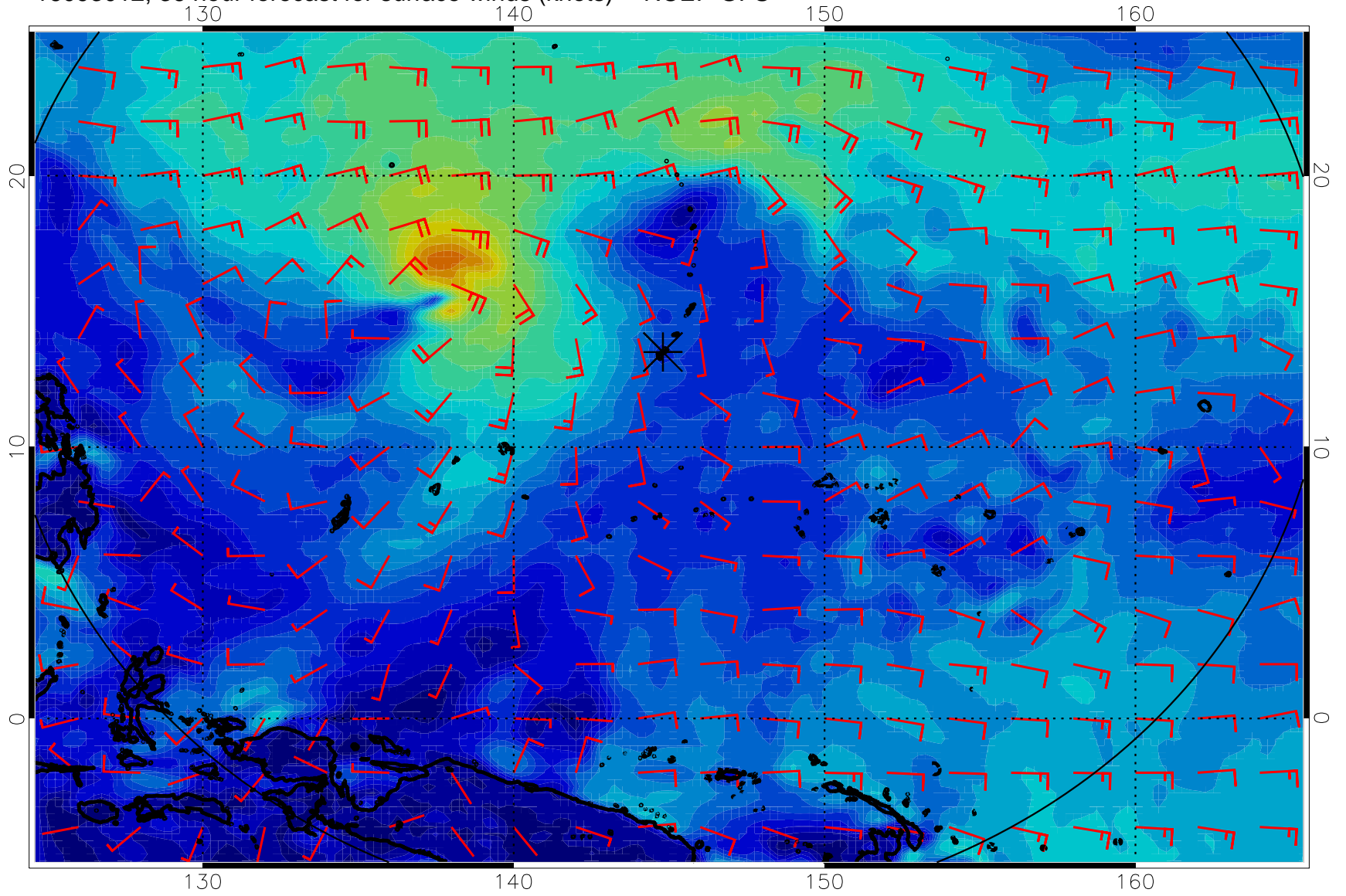
16093012, 36 hour forecast for surface winds (knots) -- NCEP GFS
