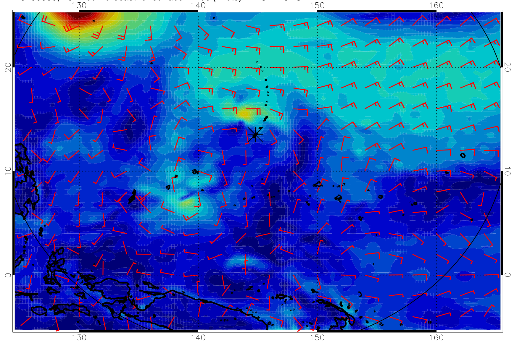
16100306, 102 hour forecast for surface winds (knots) -- NCEP GFS
