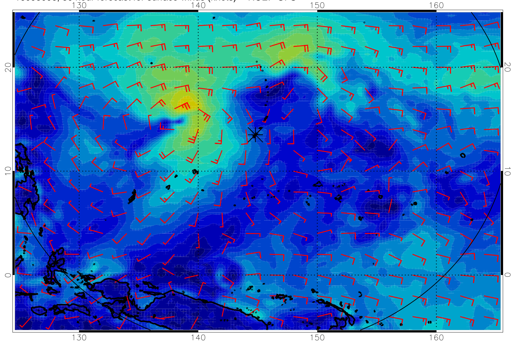
16093006, 30 hour forecast for surface winds (knots) -- NCEP GFS
