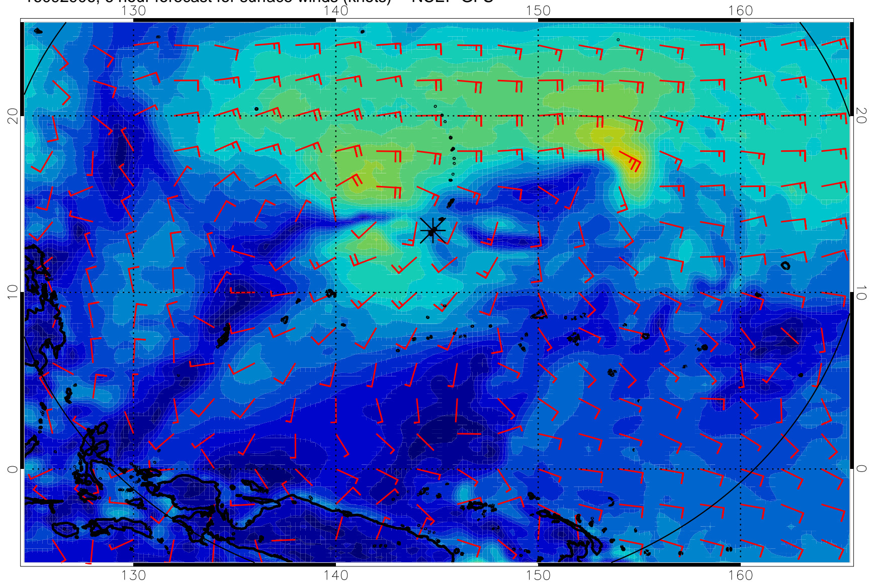
16092906, 6 hour forecast for surface winds (knots) -- NCEP GFS
