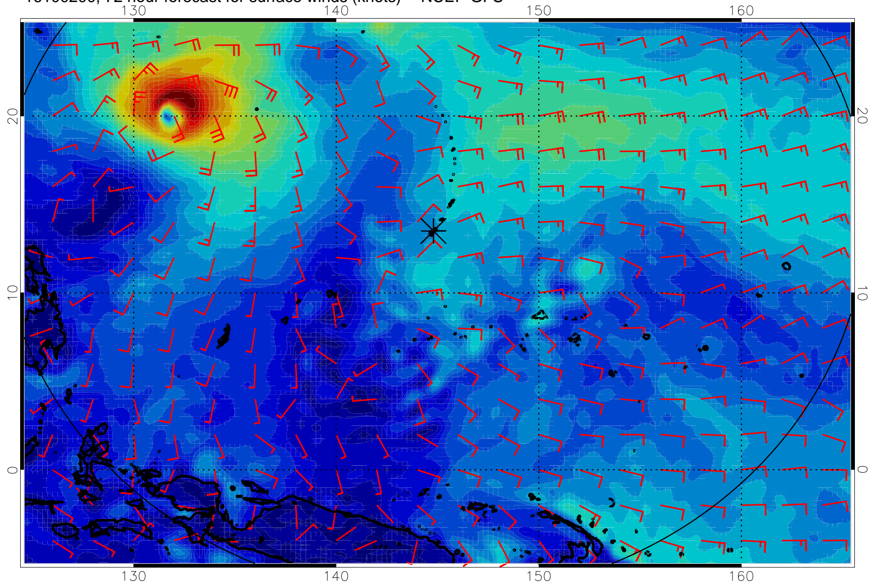
16100200, 72 hour forecast for surface winds (knots) -- NCEP GFS
