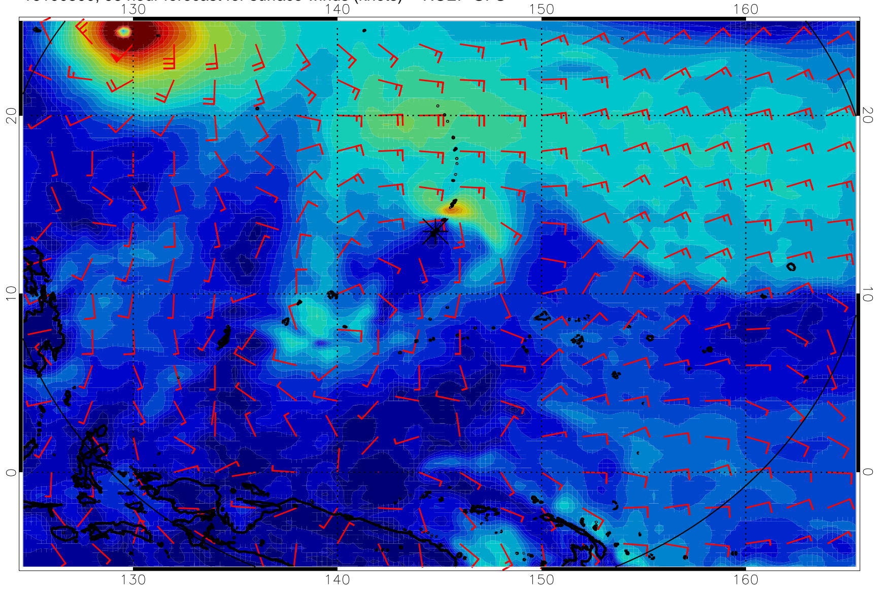
16100300, 96 hour forecast for surface winds (knots) -- NCEP GFS
