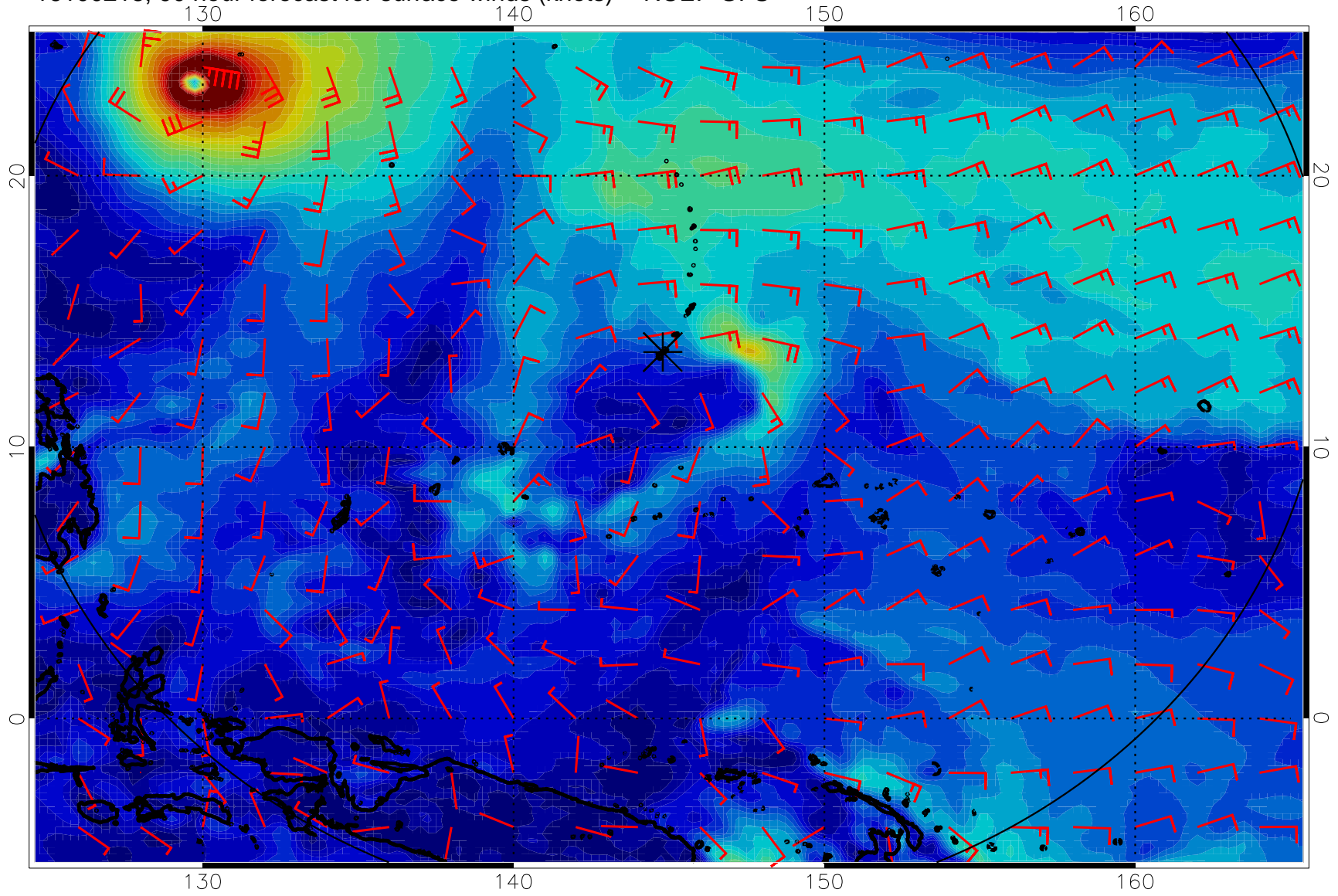
16100218, 90 hour forecast for surface winds (knots) -- NCEP GFS
