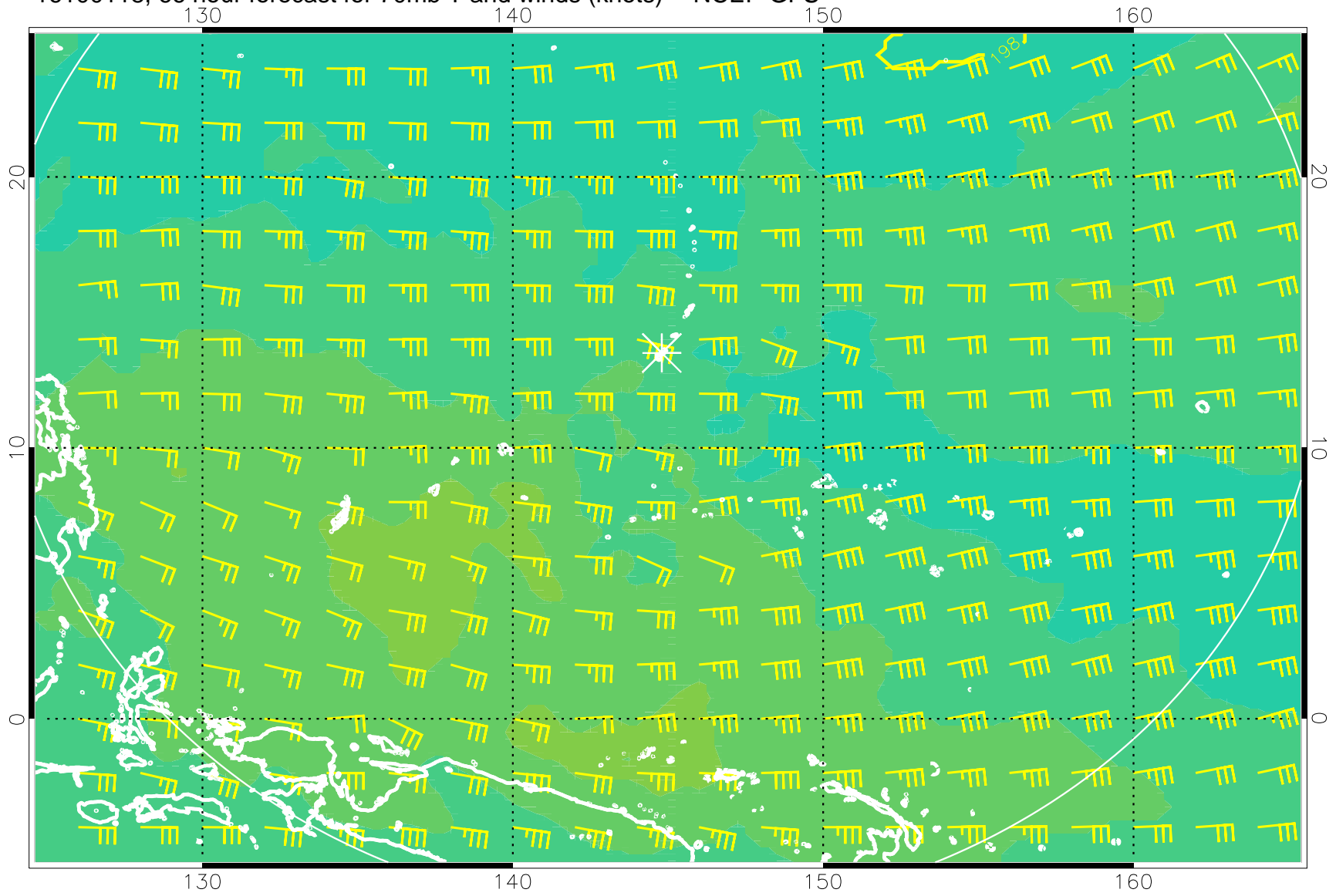
16100118, 66 hour forecast for 70mb T and winds (knots) -- NCEP GFS
