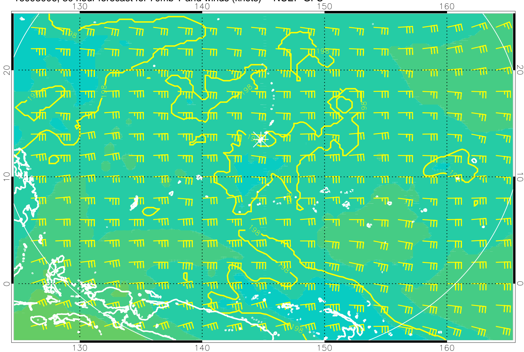
16093006, 30 hour forecast for 70mb T and winds (knots) -- NCEP GFS
