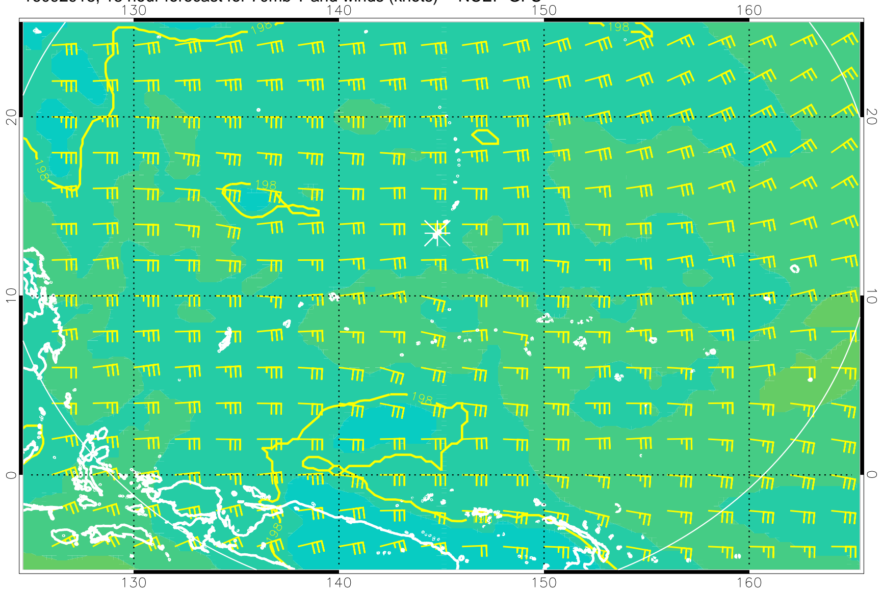
16092918, 18 hour forecast for 70mb T and winds (knots) -- NCEP GFS
