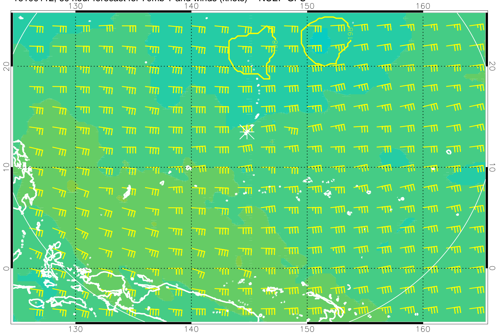
16100112, 60 hour forecast for 70mb T and winds (knots) -- NCEP GFS
