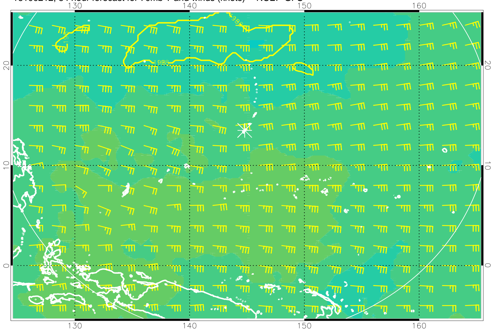
16100212, 84 hour forecast for 70mb T and winds (knots) -- NCEP GFS
