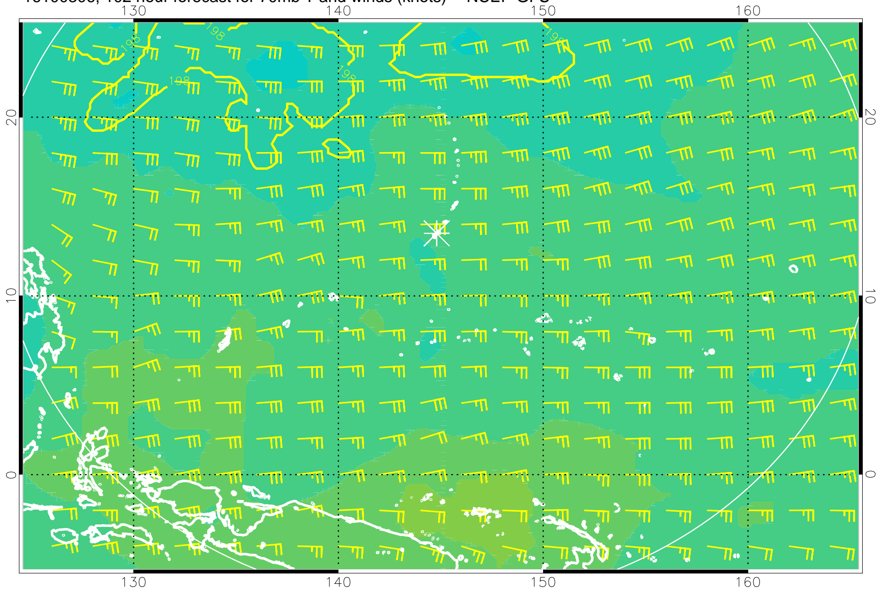
16100306, 102 hour forecast for 70mb T and winds (knots) -- NCEP GFS
