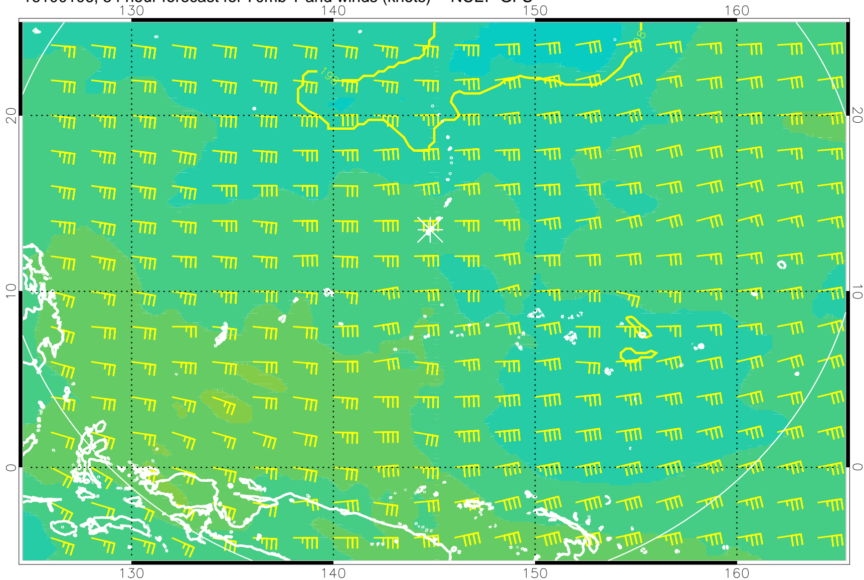
16100106, 54 hour forecast for 70mb T and winds (knots) -- NCEP GFS
