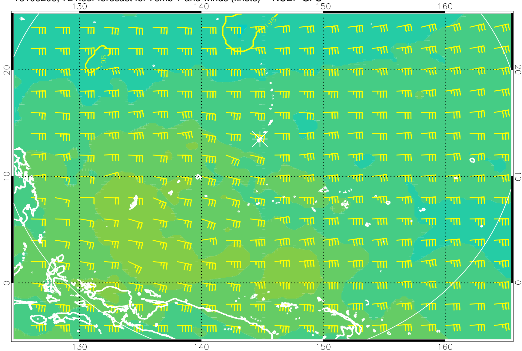
16100200, 72 hour forecast for 70mb T and winds (knots) -- NCEP GFS
