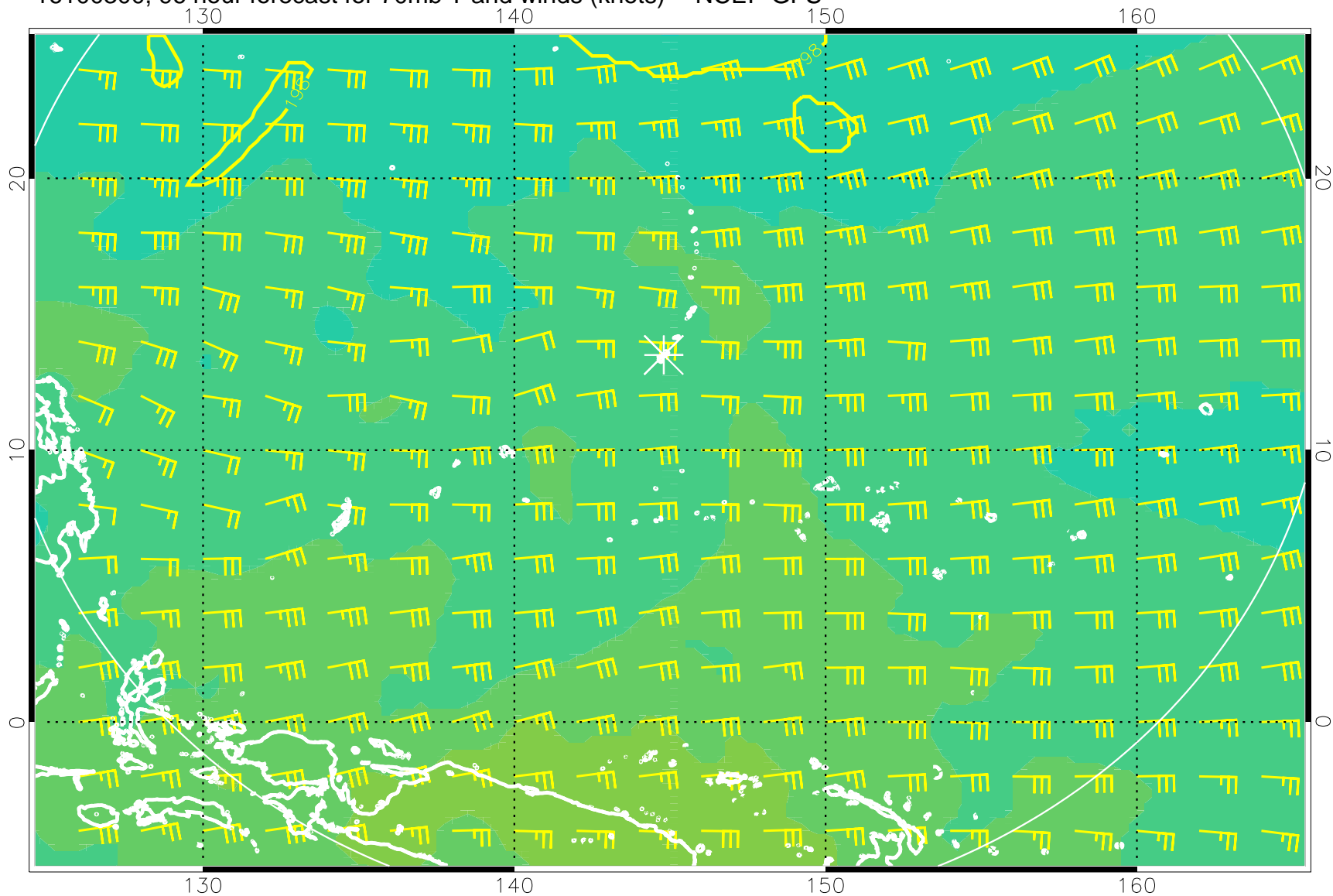
16100300, 96 hour forecast for 70mb T and winds (knots) -- NCEP GFS
