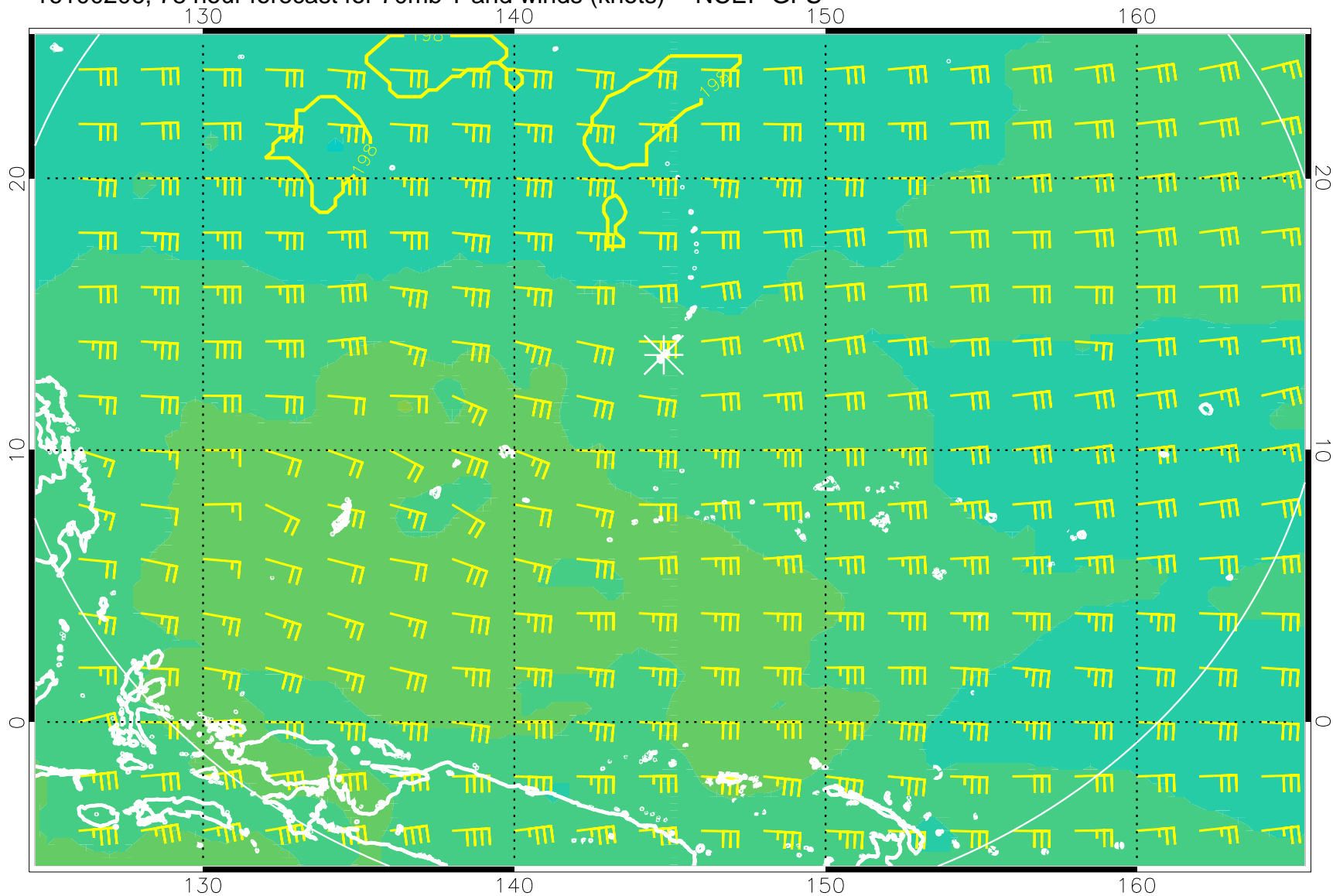
16100206, 78 hour forecast for 70mb T and winds (knots) -- NCEP GFS
