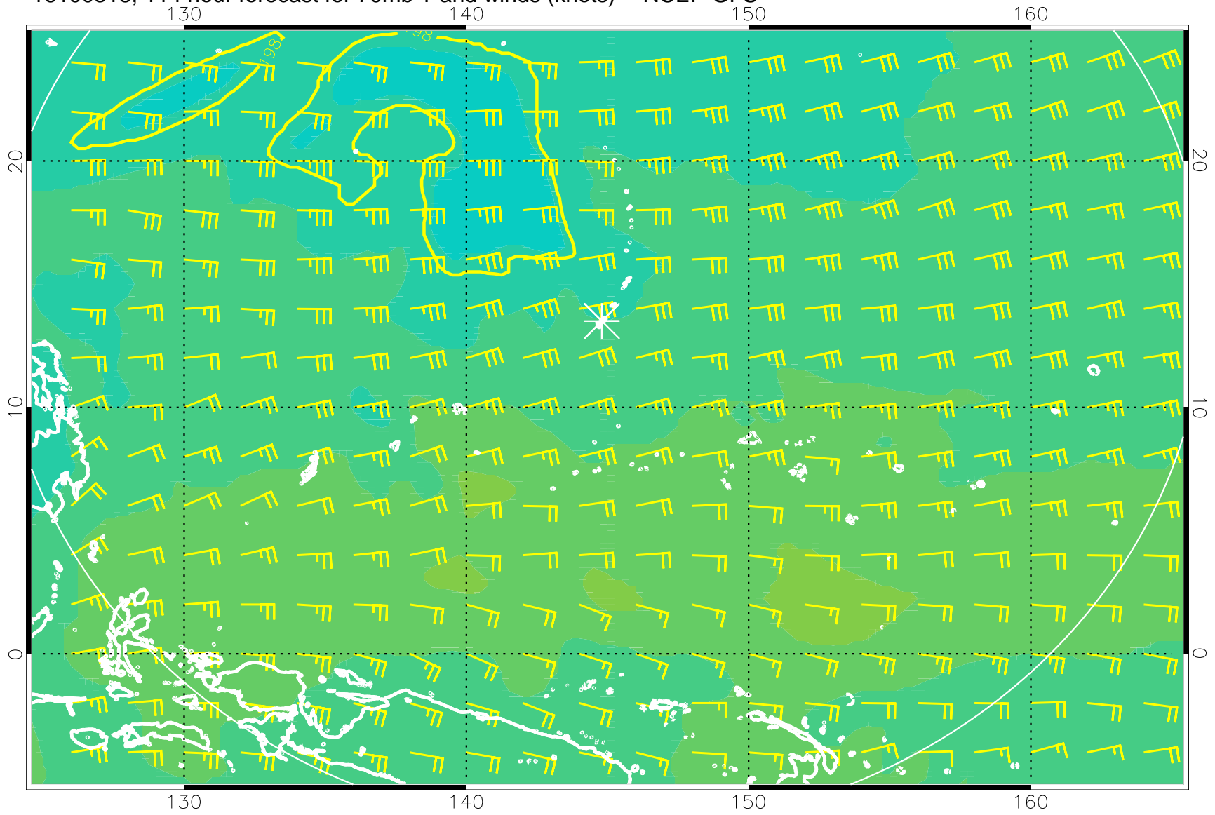
16100318, 114 hour forecast for 70mb T and winds (knots) -- NCEP GFS
