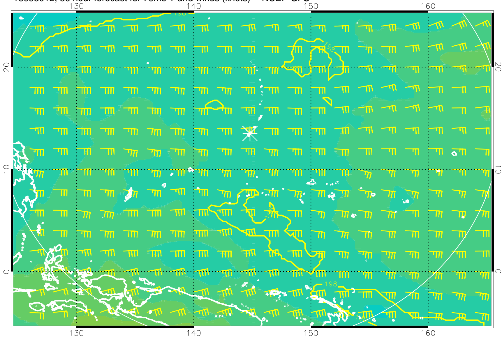
16093012, 36 hour forecast for 70mb T and winds (knots) -- NCEP GFS
