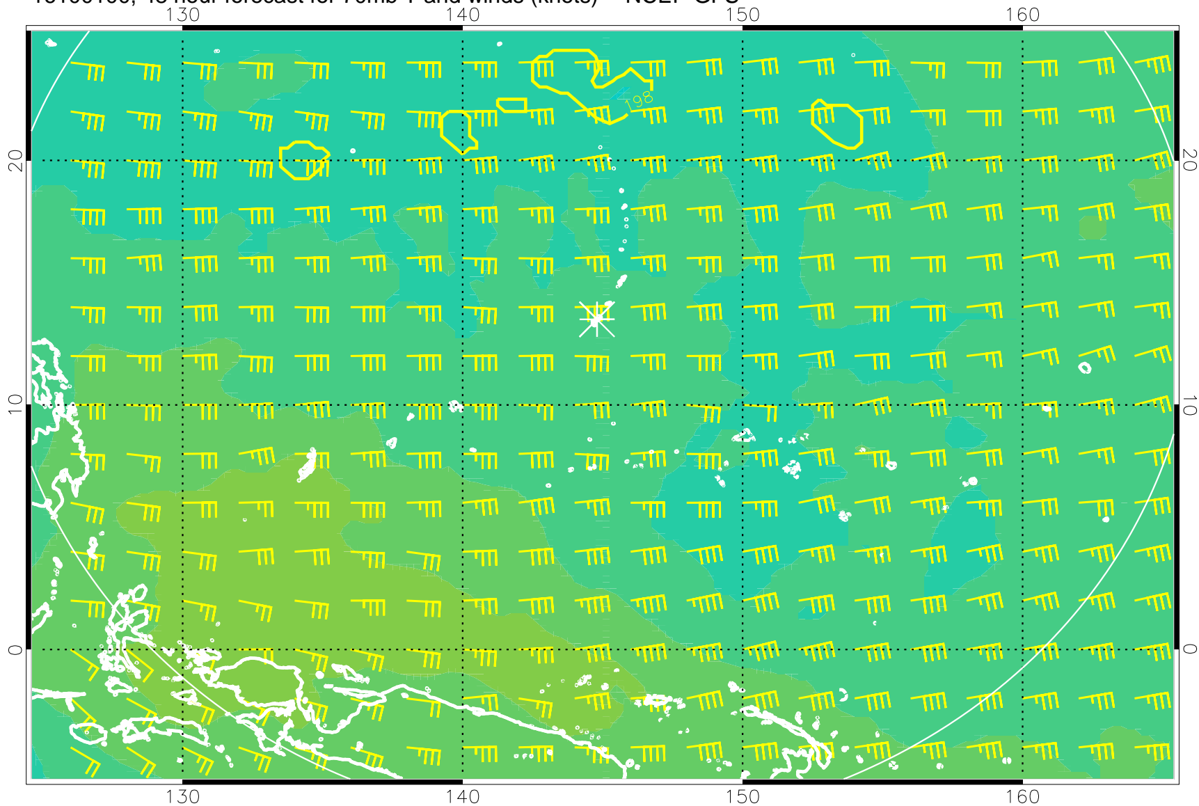
16100100, 48 hour forecast for 70mb T and winds (knots) -- NCEP GFS
