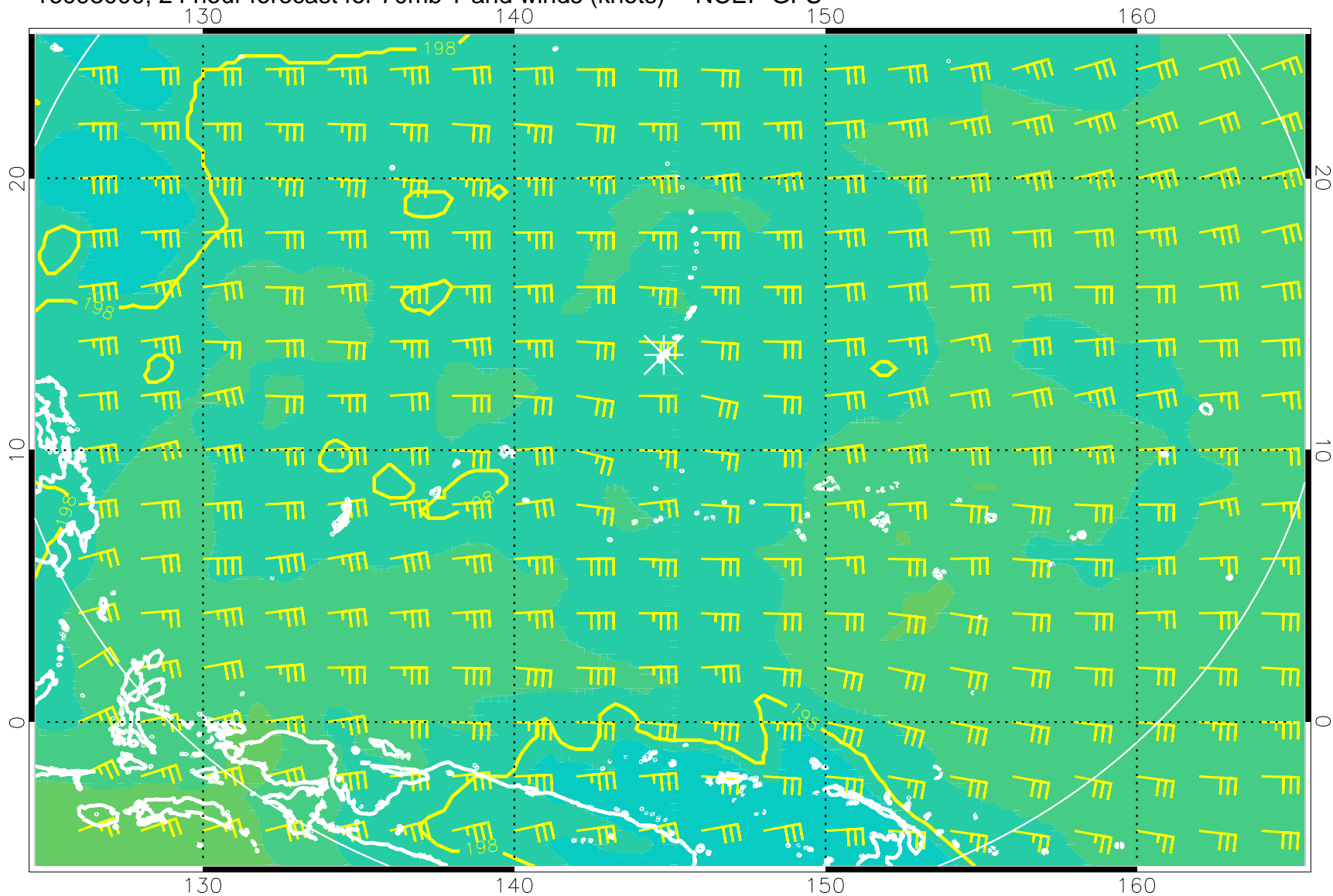
16093000, 24 hour forecast for 70mb T and winds (knots) -- NCEP GFS
