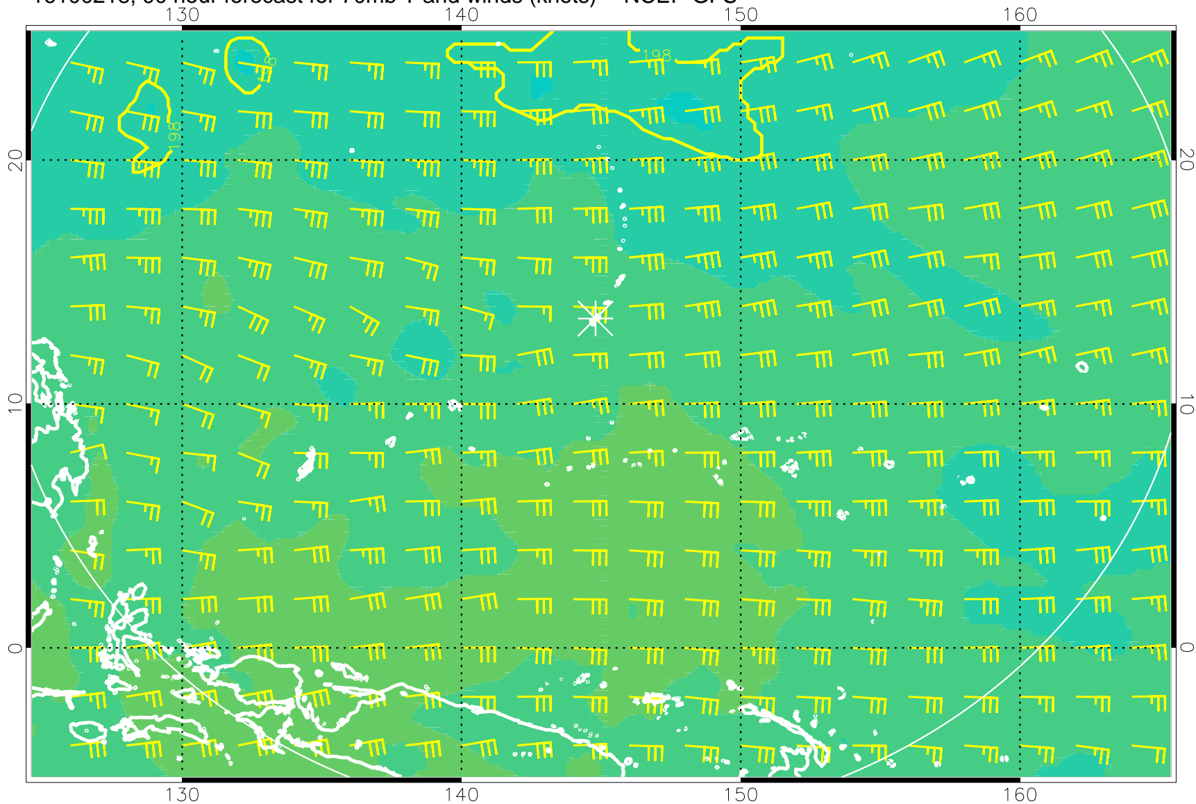
16100218, 90 hour forecast for 70mb T and winds (knots) -- NCEP GFS
