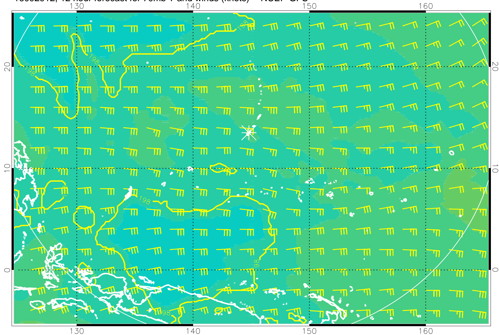
16092912, 12 hour forecast for 70mb T and winds (knots) -- NCEP GFS
