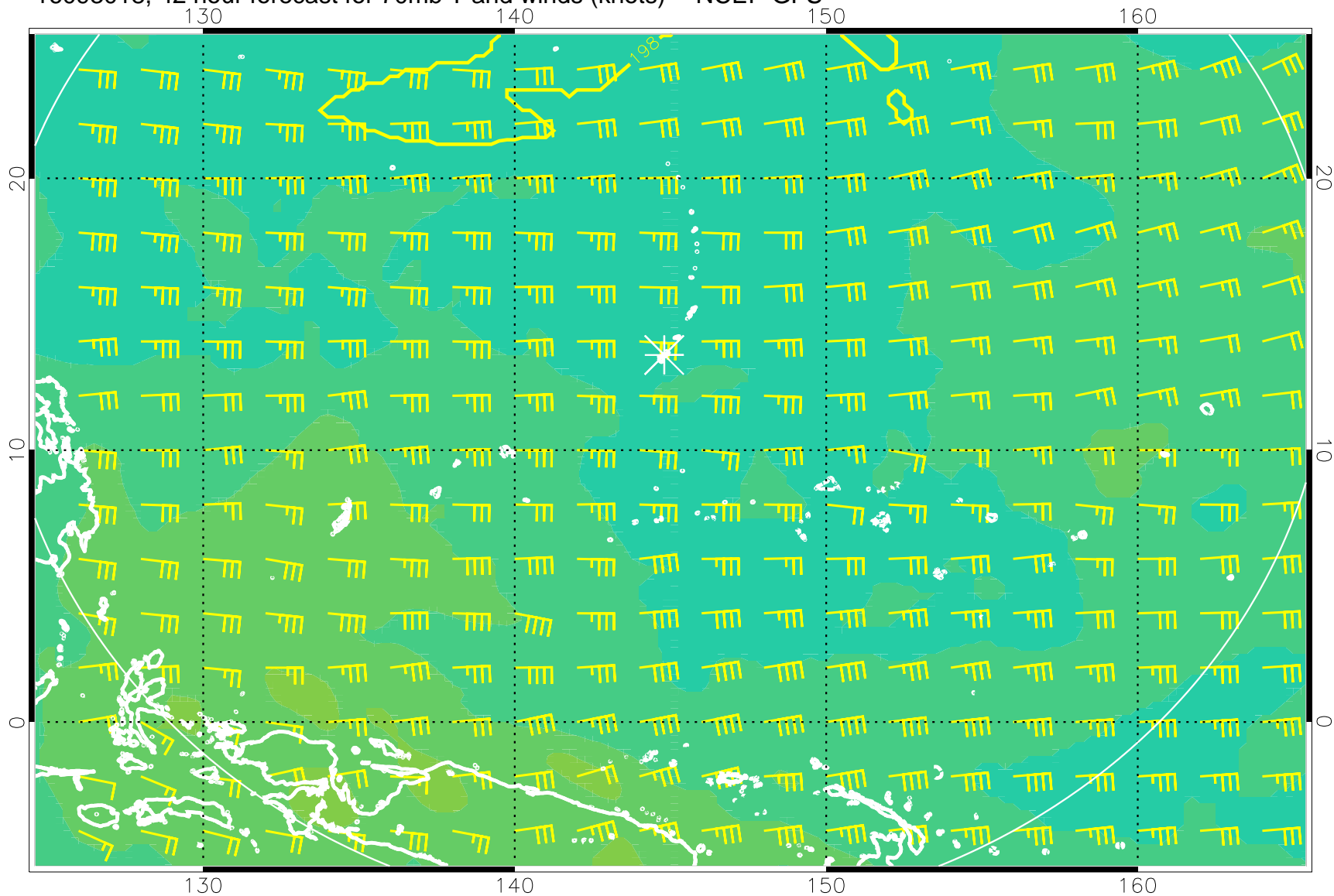
16093018, 42 hour forecast for 70mb T and winds (knots) -- NCEP GFS
