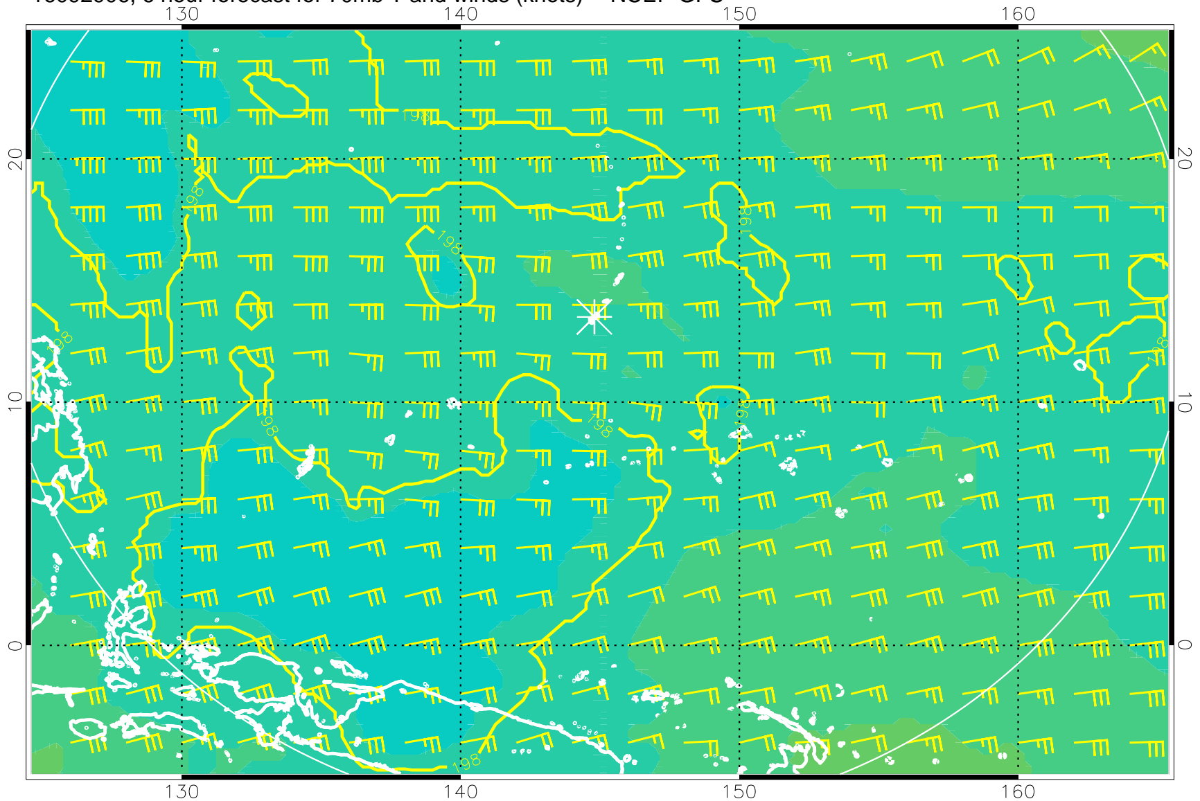
16092906, 6 hour forecast for 70mb T and winds (knots) -- NCEP GFS
