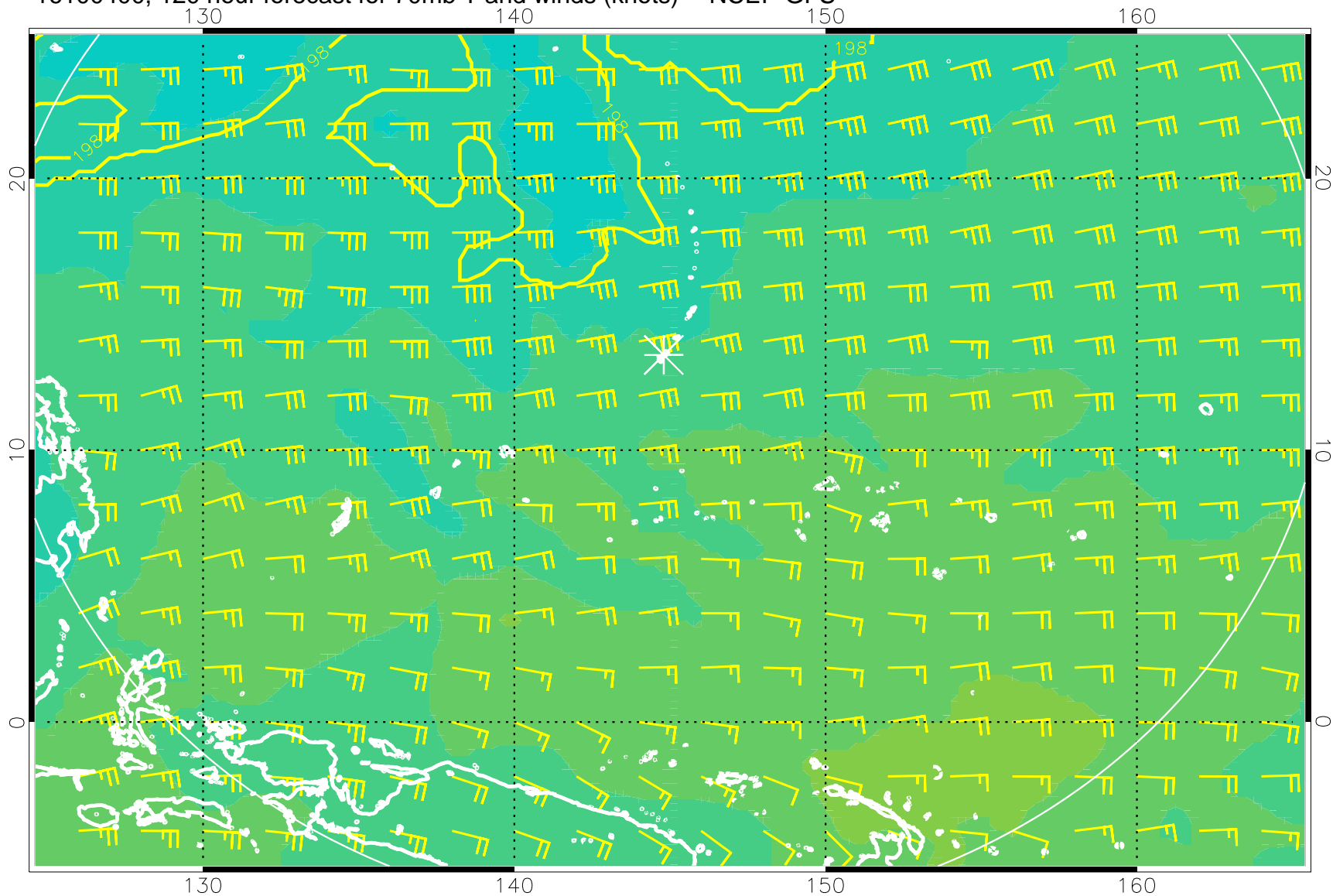
16100400, 120 hour forecast for 70mb T and winds (knots) -- NCEP GFS
