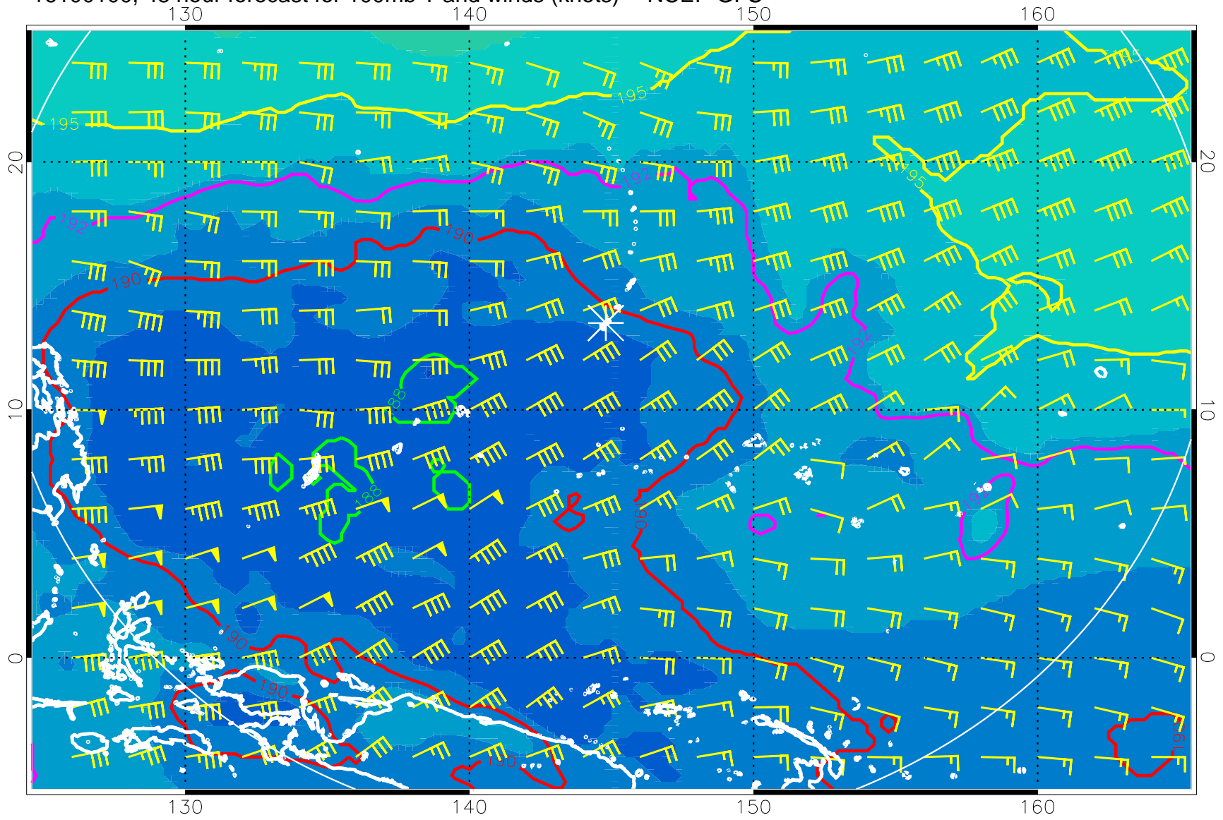
16100100, 48 hour forecast for 100mb T and winds (knots) -- NCEP GFS
