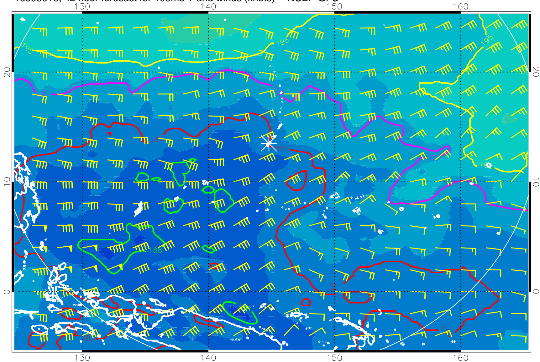
16093018, 42 hour forecast for 100mb T and winds (knots) -- NCEP GFS
