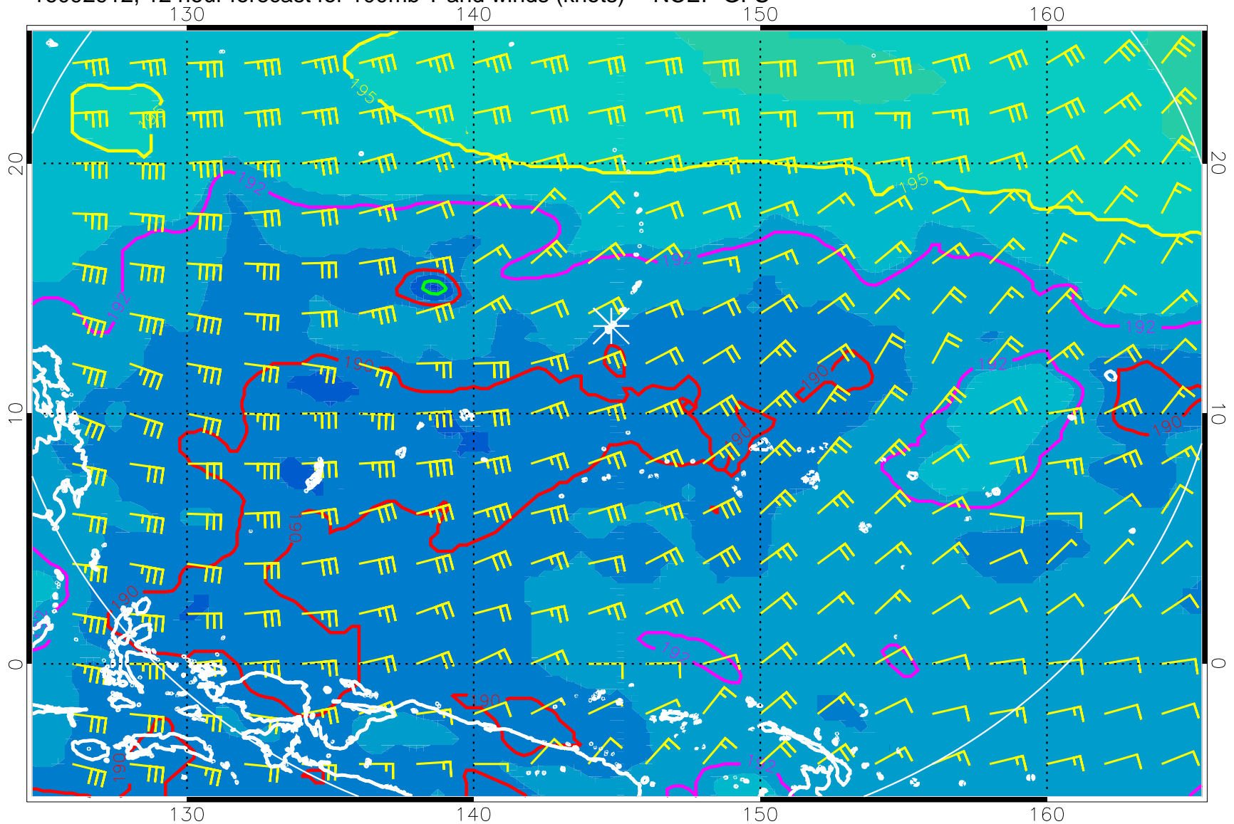
16092912, 12 hour forecast for 100mb T and winds (knots) -- NCEP GFS
