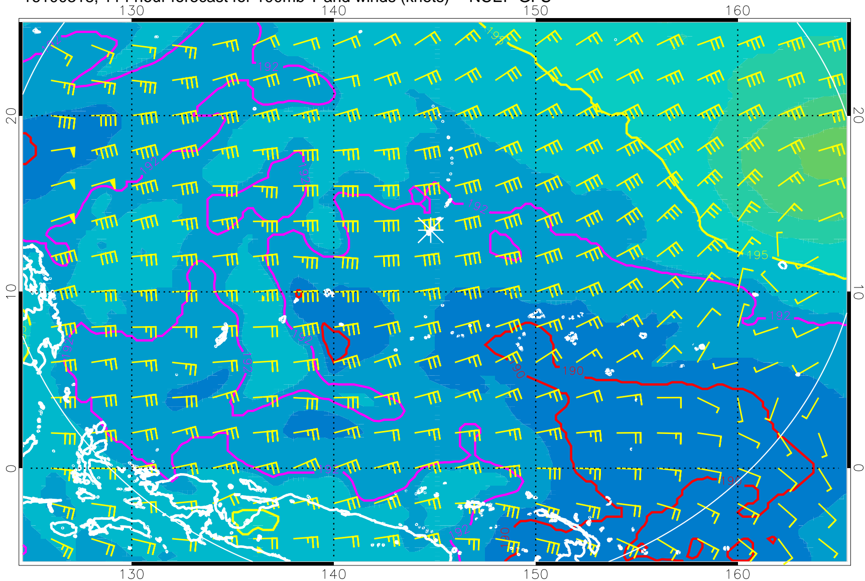
16100318, 114 hour forecast for 100mb T and winds (knots) -- NCEP GFS
