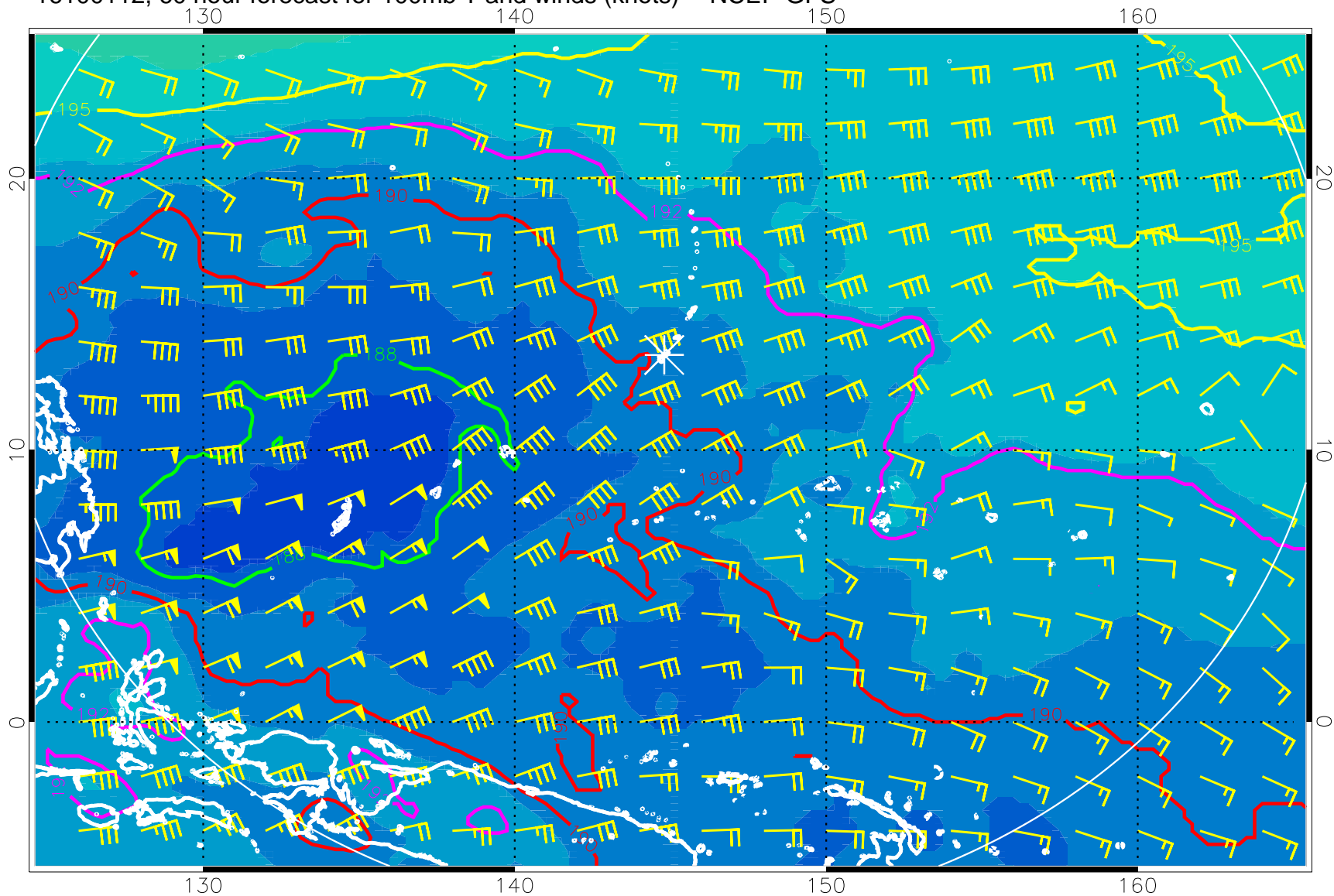
16100112, 60 hour forecast for 100mb T and winds (knots) -- NCEP GFS
