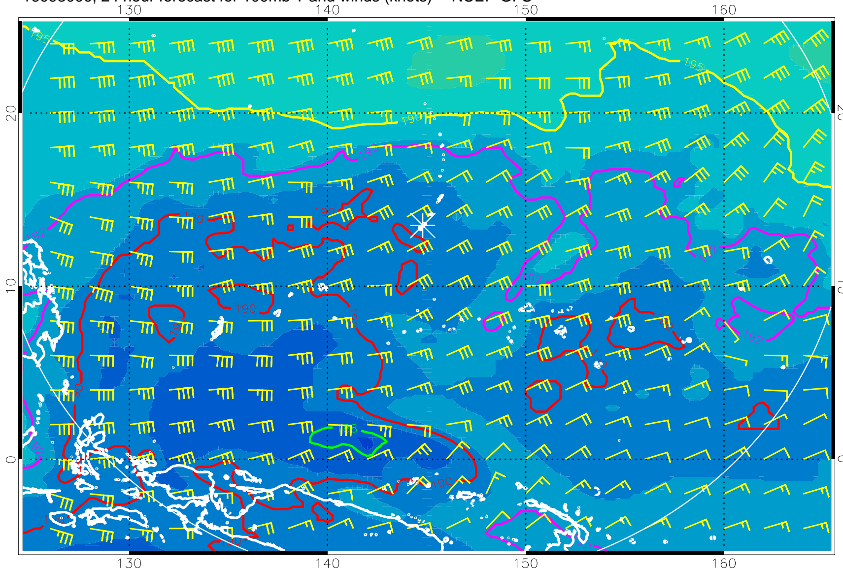
16093000, 24 hour forecast for 100mb T and winds (knots) -- NCEP GFS
