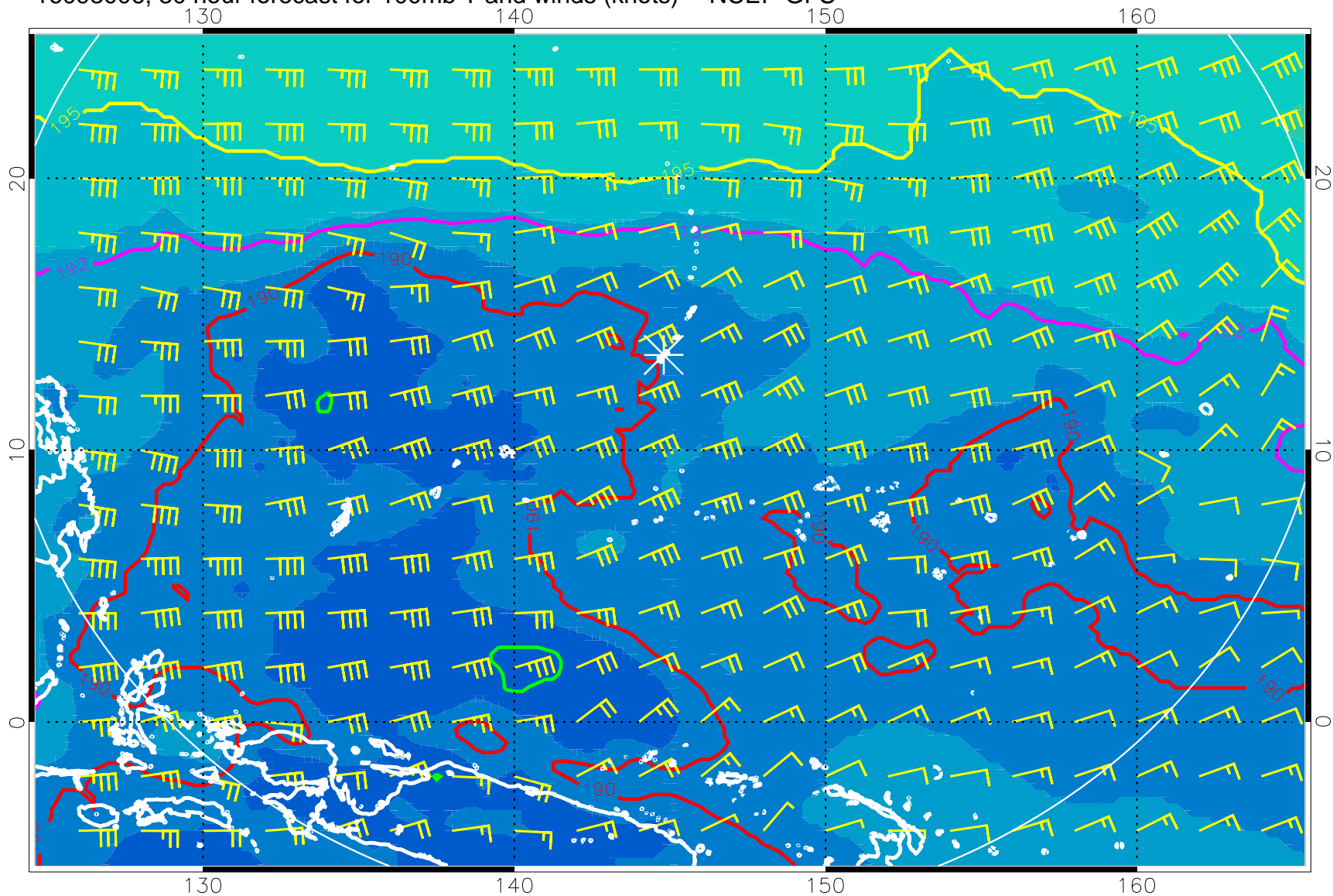
16093006, 30 hour forecast for 100mb T and winds (knots) -- NCEP GFS
