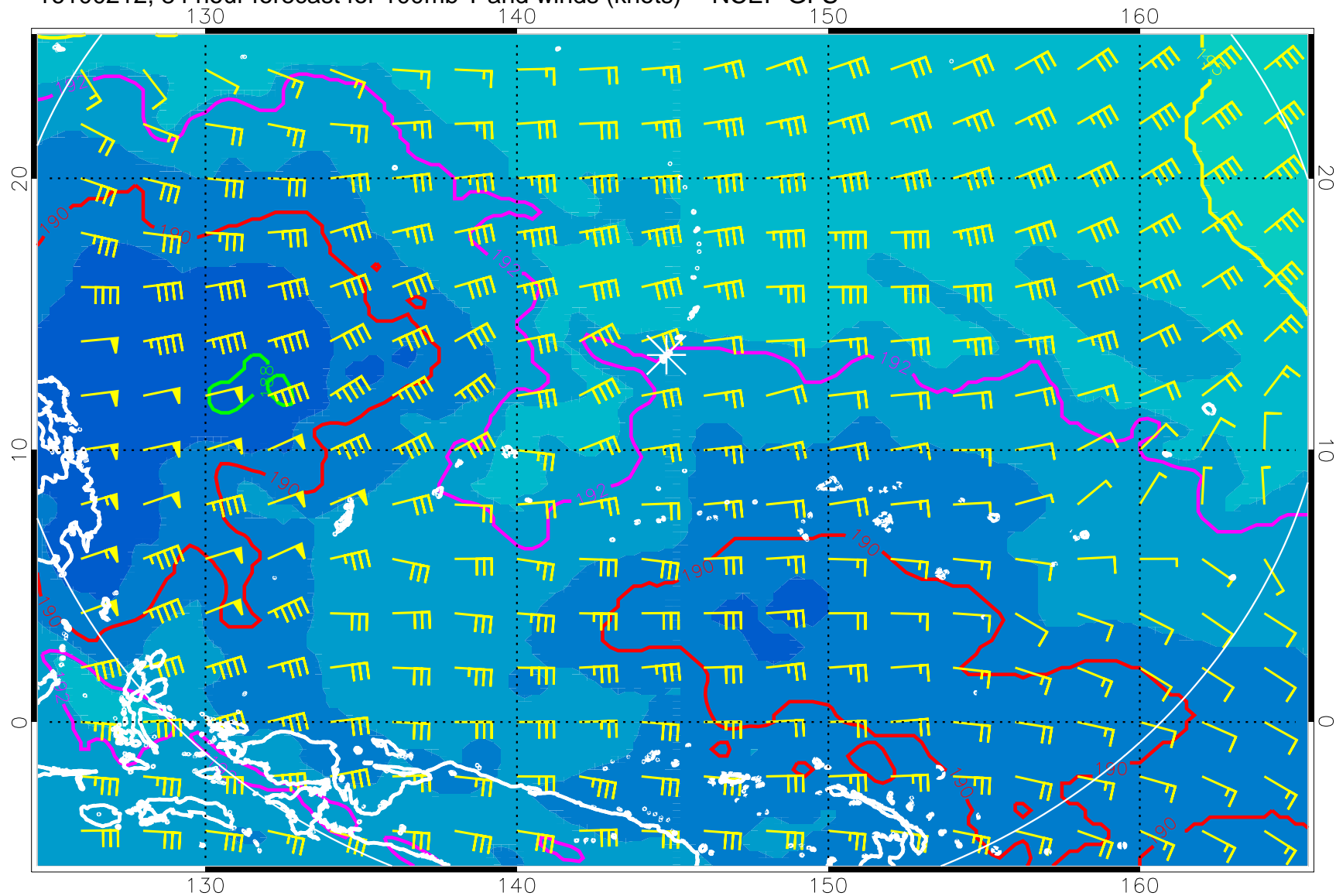
16100212, 84 hour forecast for 100mb T and winds (knots) -- NCEP GFS
