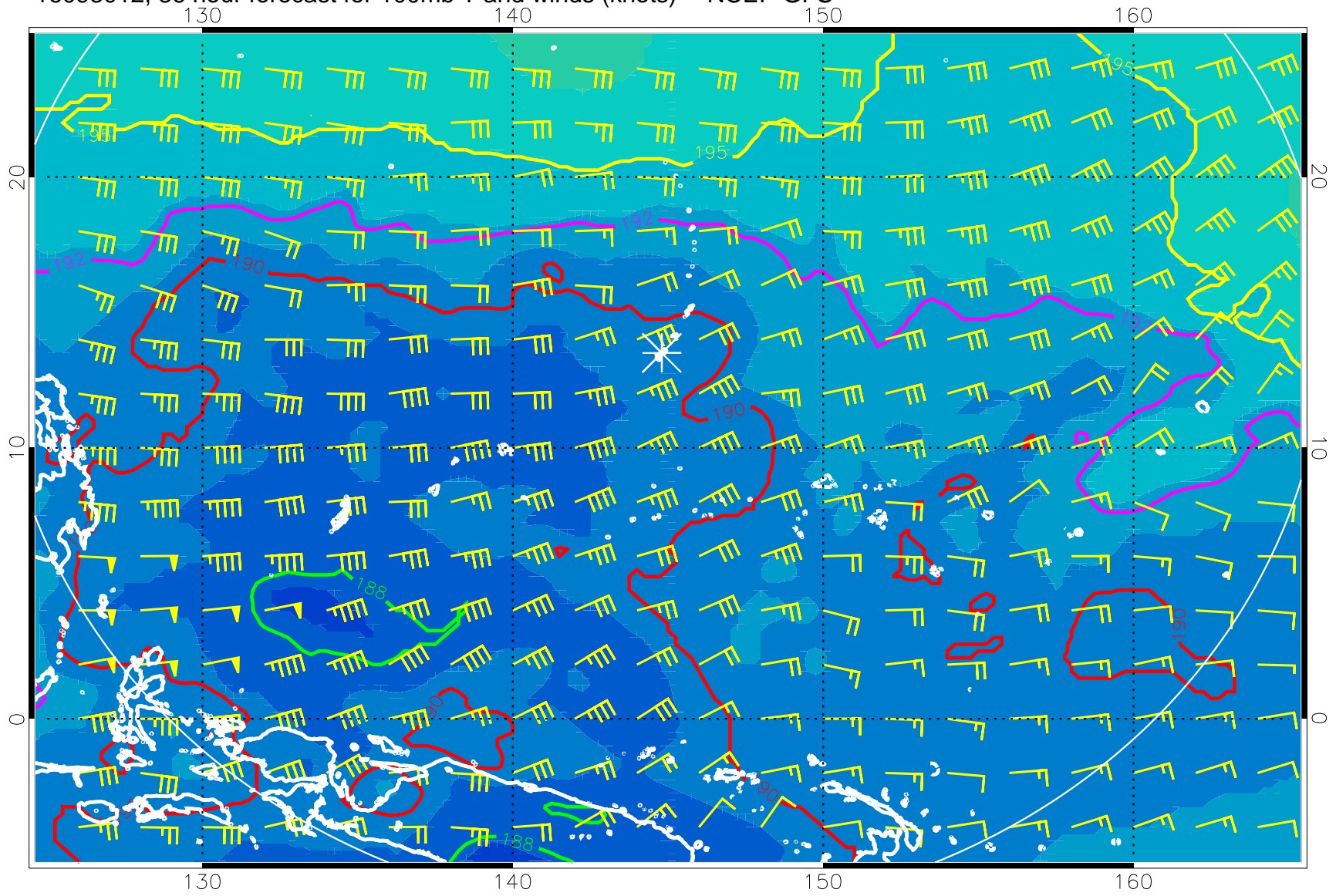
16093012, 36 hour forecast for 100mb T and winds (knots) -- NCEP GFS
