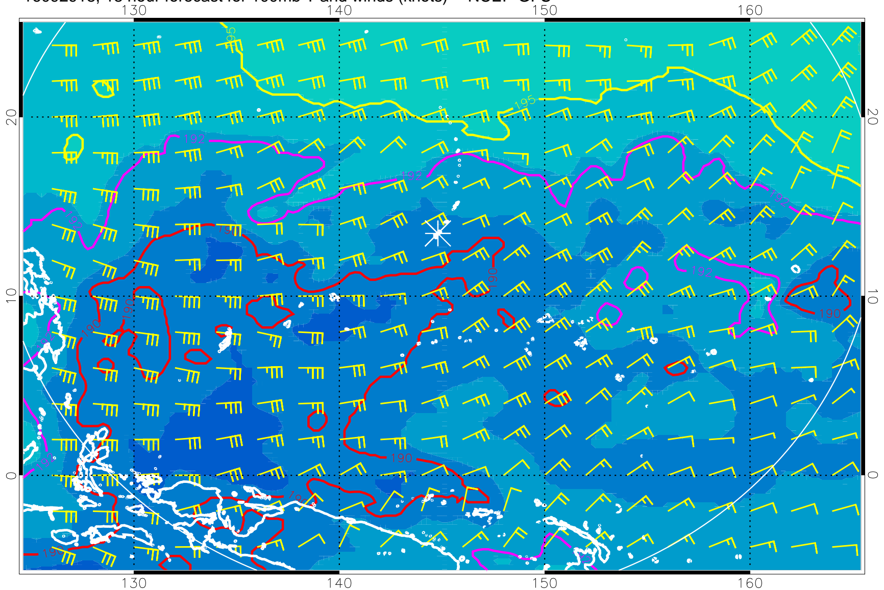
16092918, 18 hour forecast for 100mb T and winds (knots) -- NCEP GFS
