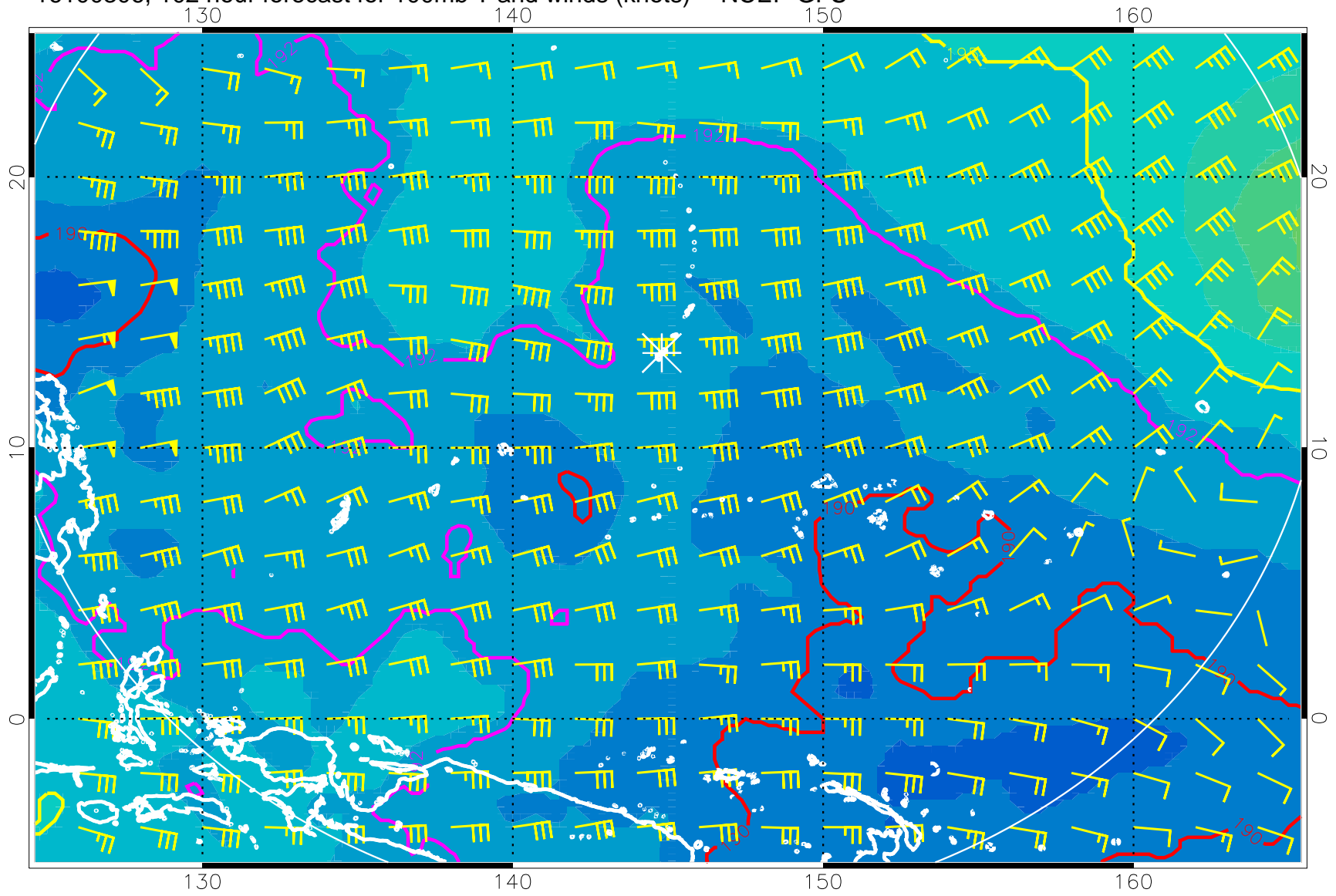
16100306, 102 hour forecast for 100mb T and winds (knots) -- NCEP GFS
