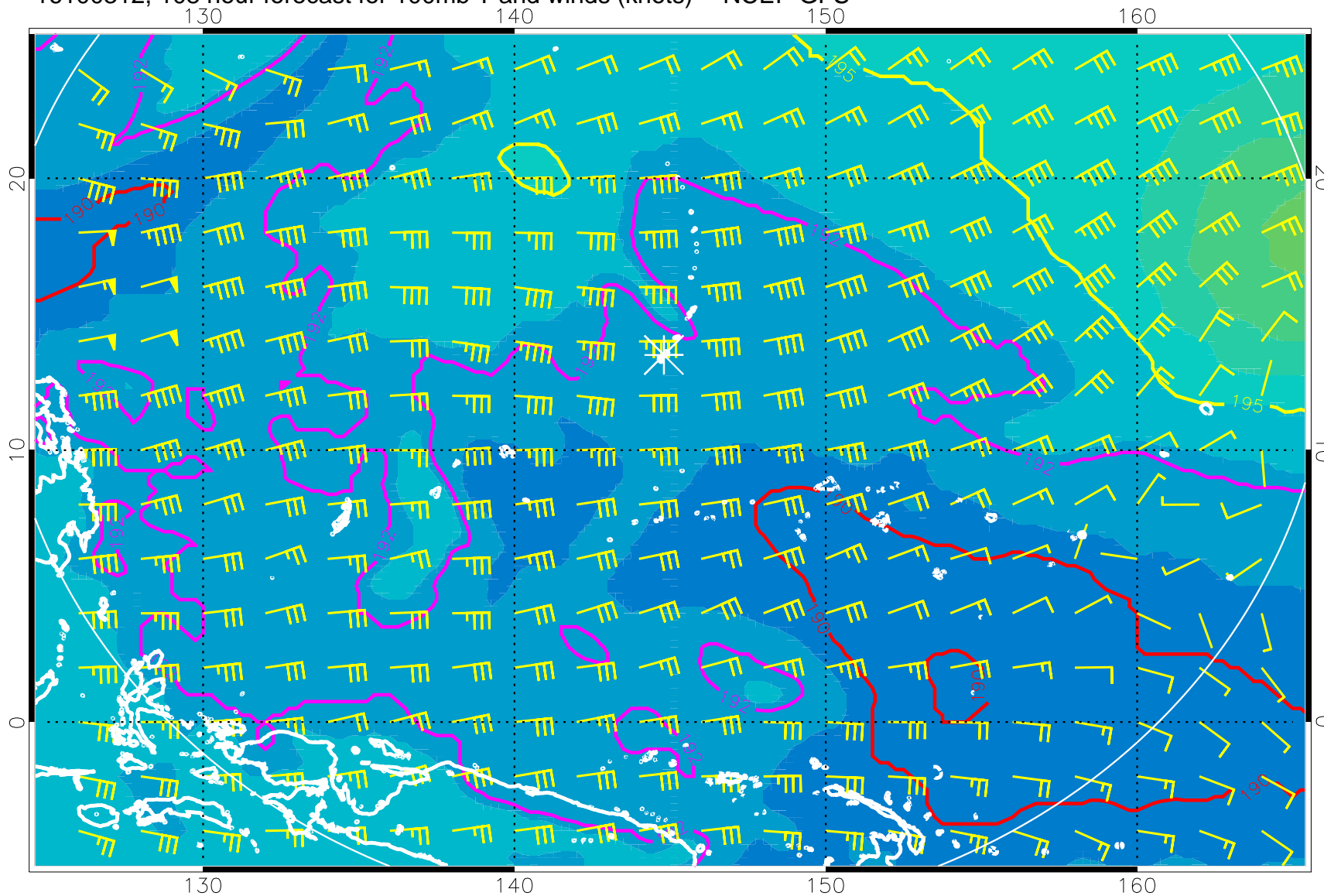
16100312, 108 hour forecast for 100mb T and winds (knots) -- NCEP GFS
