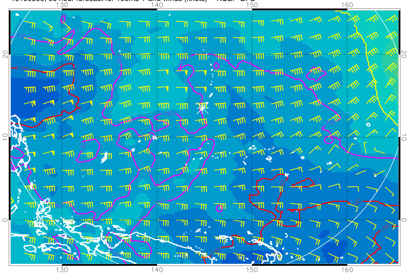
16100300, 96 hour forecast for 100mb T and winds (knots) -- NCEP GFS
