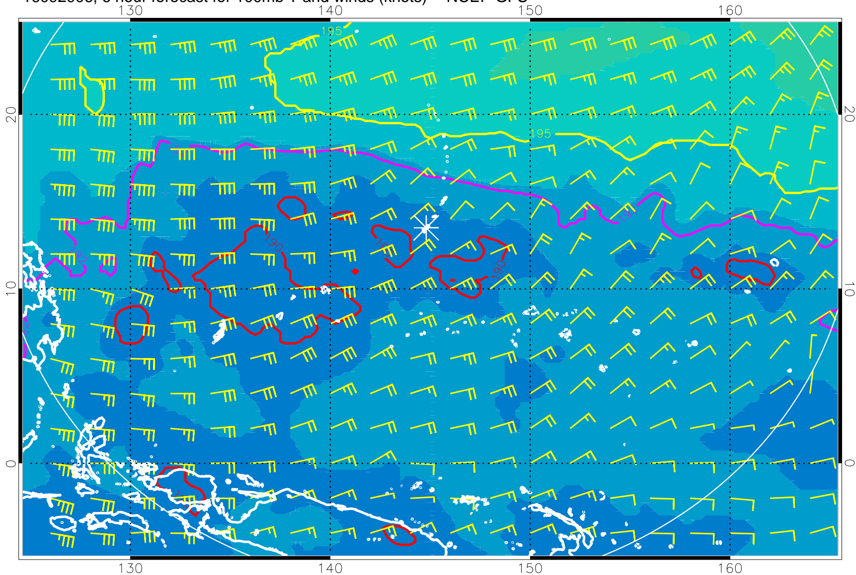
16092906, 6 hour forecast for 100mb T and winds (knots) -- NCEP GFS
