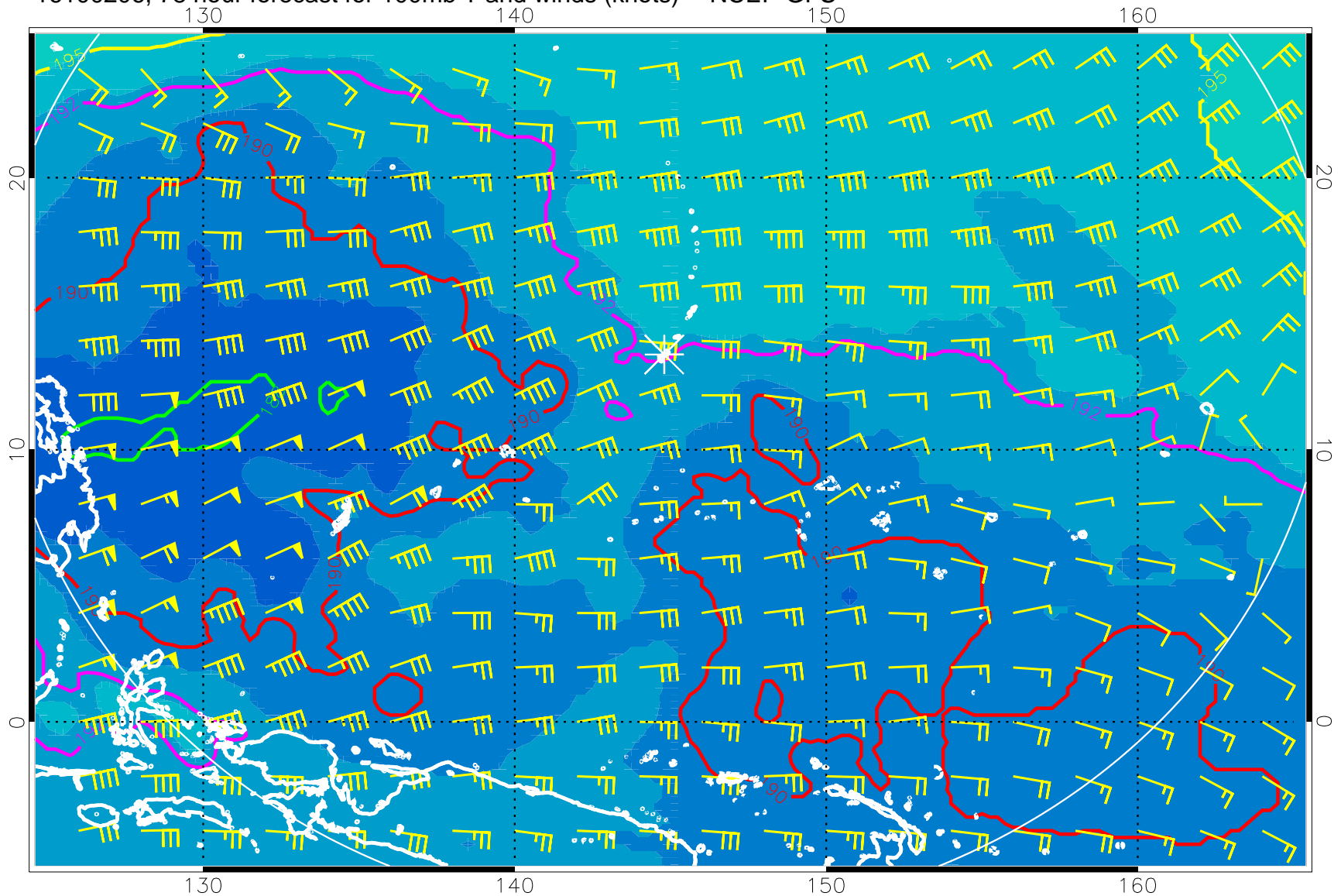
16100206, 78 hour forecast for 100mb T and winds (knots) -- NCEP GFS
