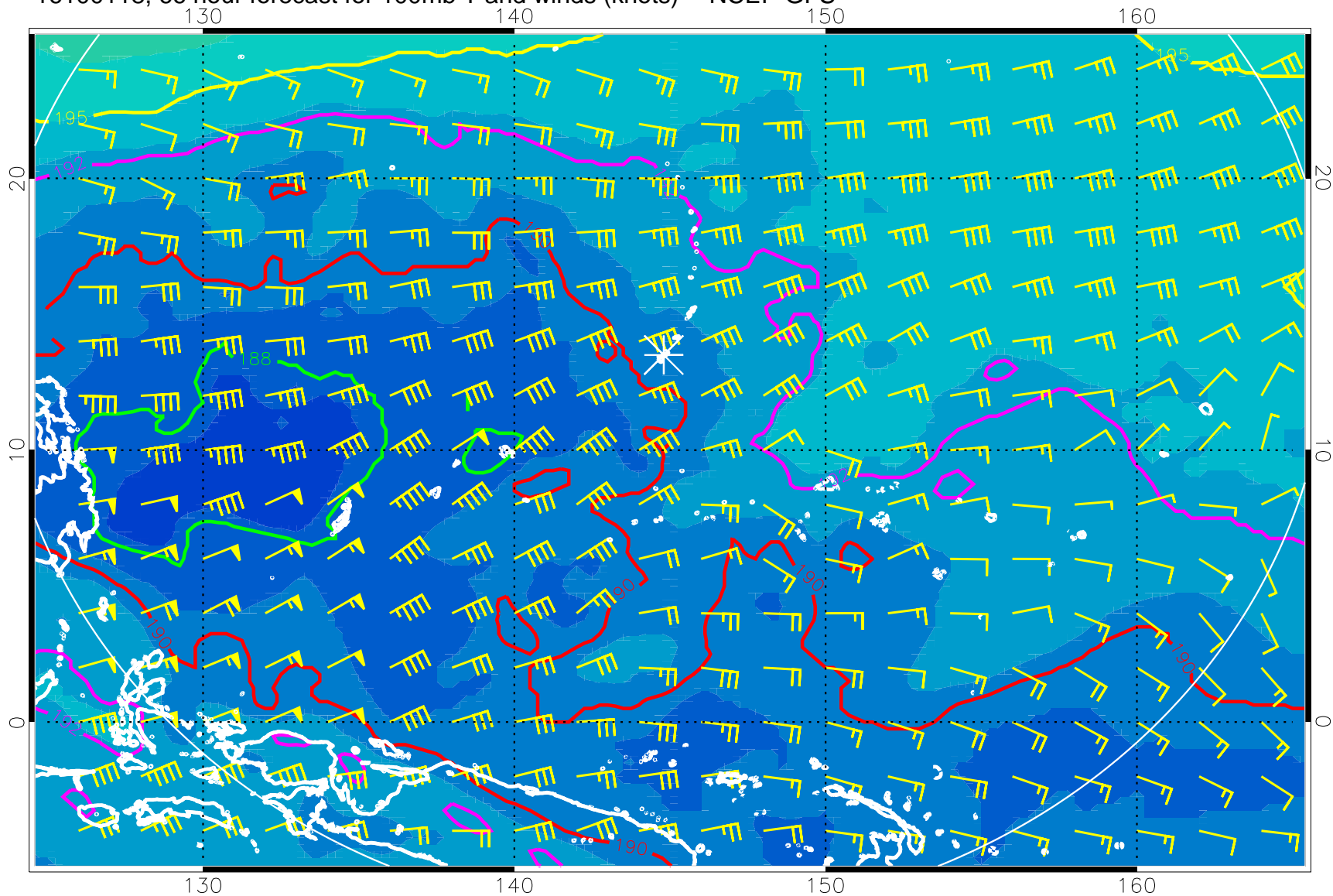
16100118, 66 hour forecast for 100mb T and winds (knots) -- NCEP GFS
