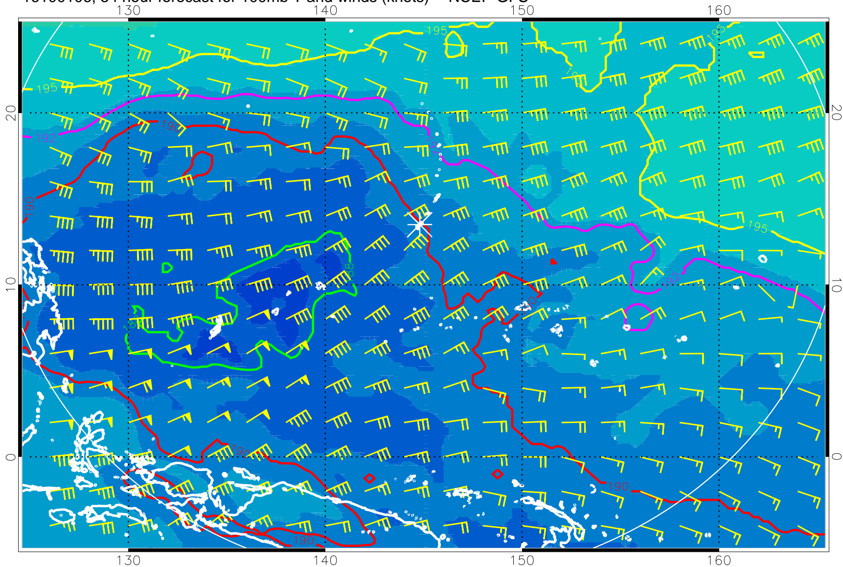
16100106, 54 hour forecast for 100mb T and winds (knots) -- NCEP GFS
