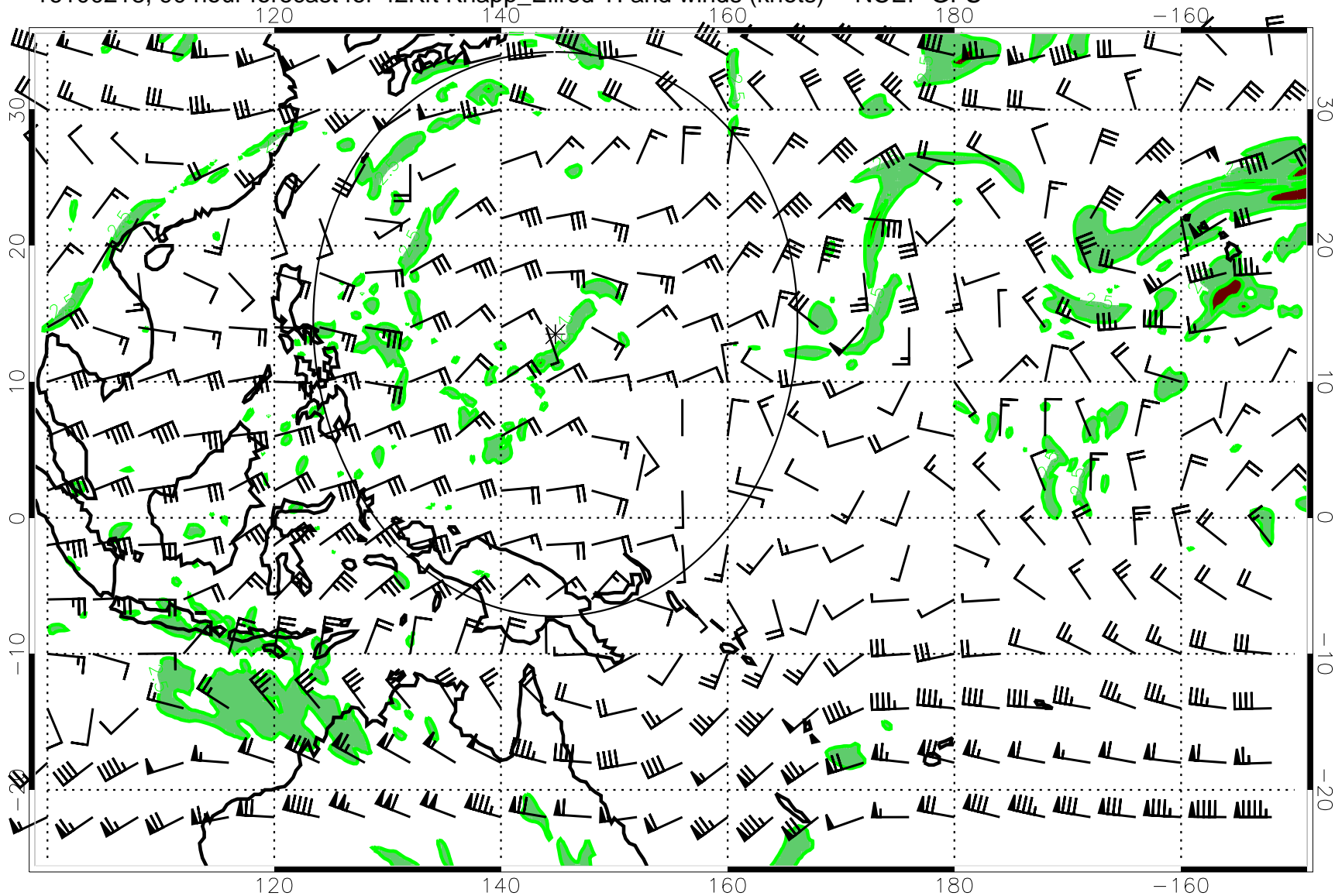
16100218, 90 hour forecast for 42Kft Knapp_Ellrod TI and winds (knots) -- NCEP GFS
