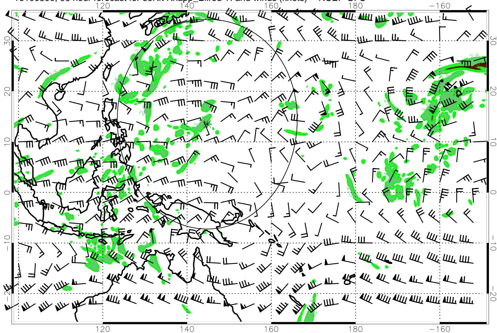
16100300, 96 hour forecast for 39Kft Knapp_Ellrod TI and winds (knots) -- NCEP GFS
