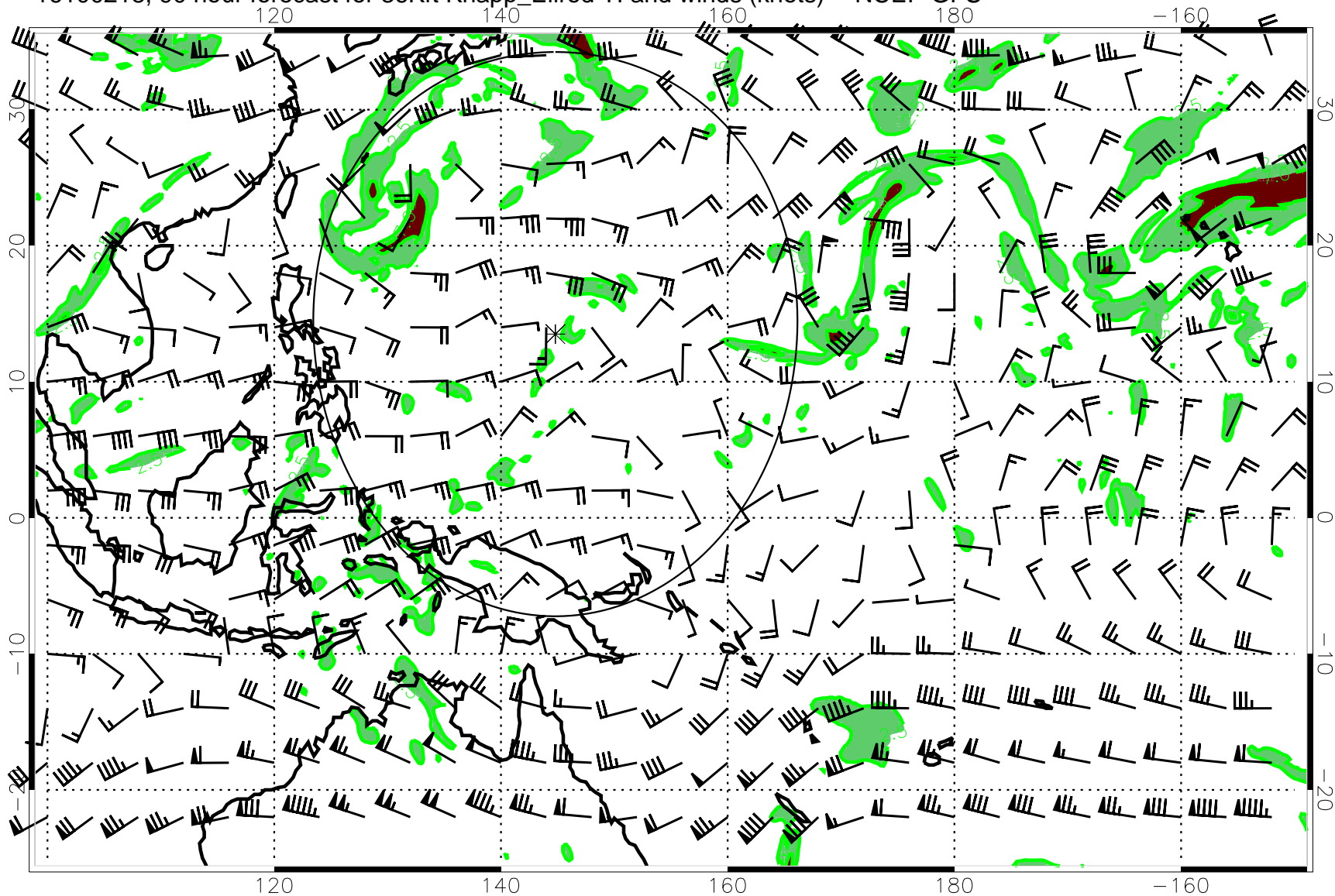
16100218, 90 hour forecast for 36Kft Knapp_Ellrod TI and winds (knots) -- NCEP GFS
