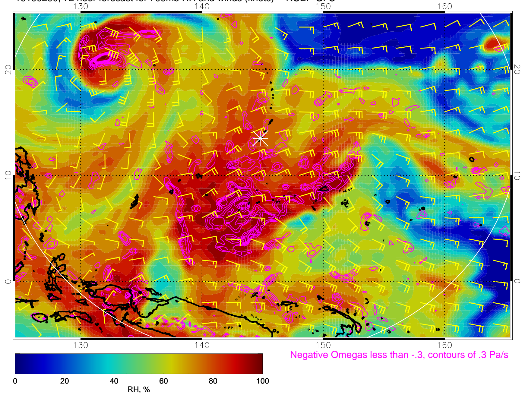
16100200, 72 hour forecast for 700mb RH and winds (knots) -- NCEP GFS
