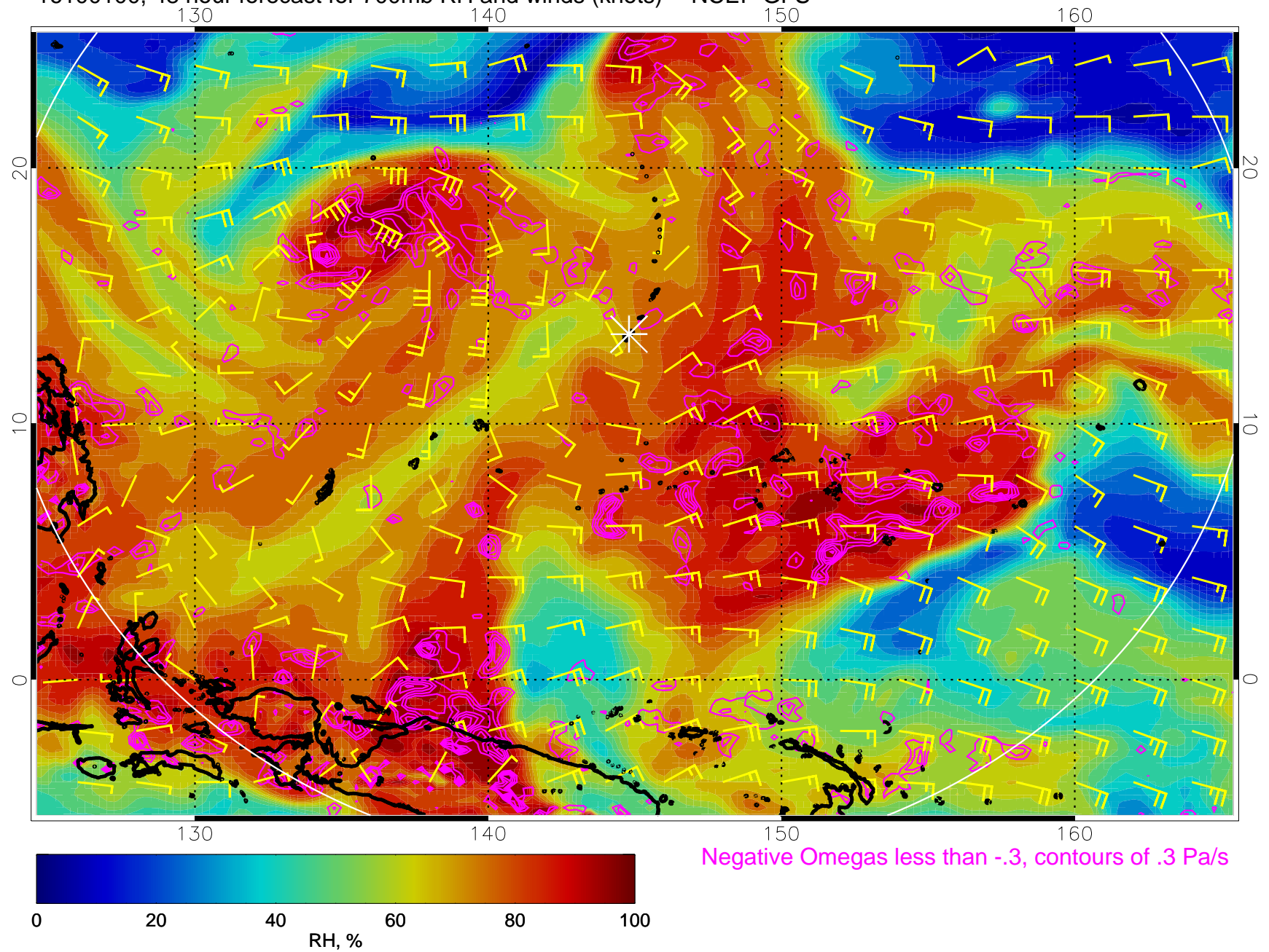
16100100, 48 hour forecast for 700mb RH and winds (knots) -- NCEP GFS
