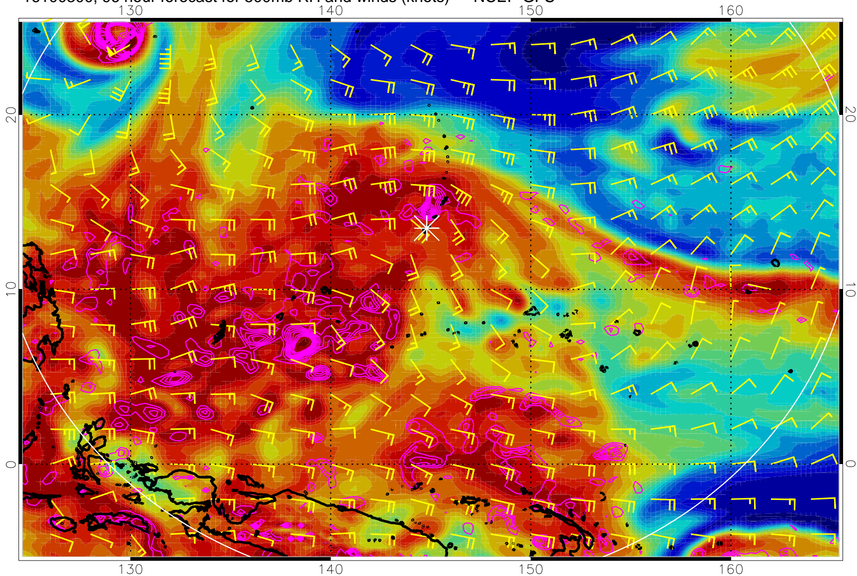
16100300, 96 hour forecast for 500mb RH and winds (knots) -- NCEP GFS
