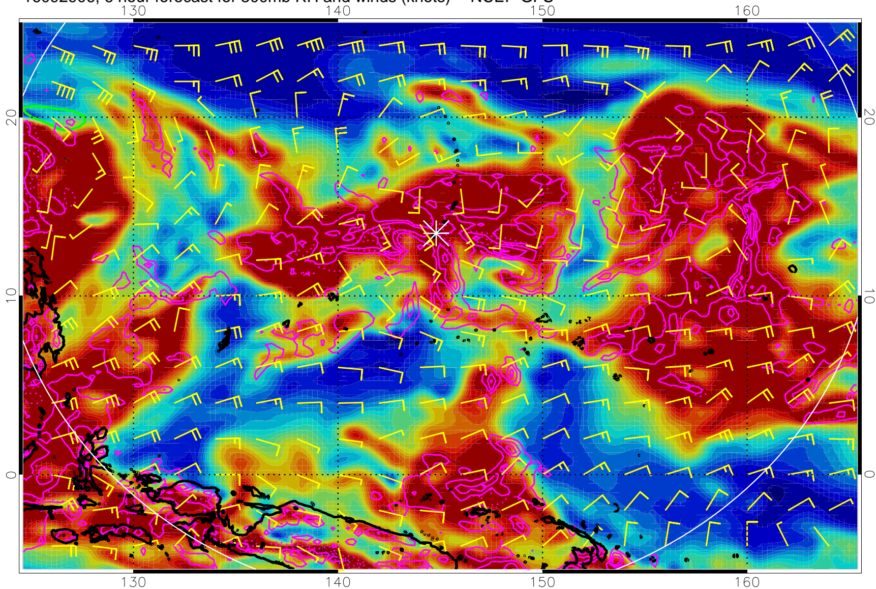
16092906, 6 hour forecast for 300mb RH and winds (knots) -- NCEP GFS
