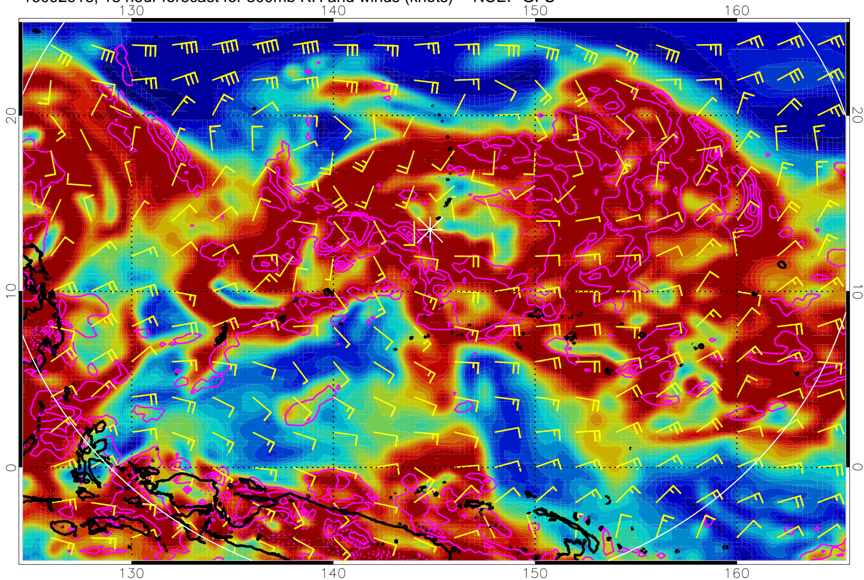
16092918, 18 hour forecast for 300mb RH and winds (knots) -- NCEP GFS
